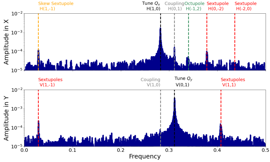
(B) Working point Q_x = 5.28, Q_y = 5.31
