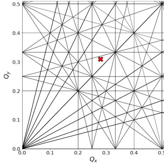
FIGURE 2.4: Tune diagram with resonances up to order |m| + |n| = 5 and with the working point of LHC at injection energy of Q_x = 0.28/Q_y = 0.31 . Synchrotron resonances ( \nu \neq 0 ) have been omitted here.
