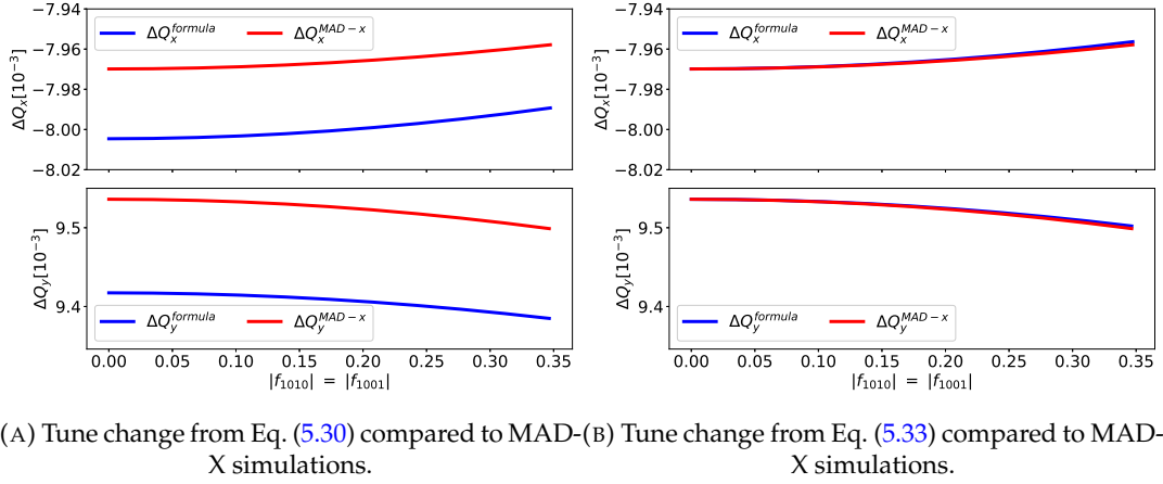
FIGURE 5.2: Comparison of tune change from quadrupole modulation with coupling to MAD-X simulations.
