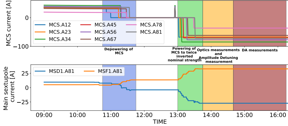
FIGURE 4.1: Evolution the current from the power supplies of the sextupole spool piece (MCS) correctors (top) and of the arc sextupole, grouped into sextupoles close to the focusing (MSF) and defocusing quadrupoles (MSD) (bottom). Here, only the current for the MS in Arc81 is displayed. The MS in the other arcs were powered with the same current.
