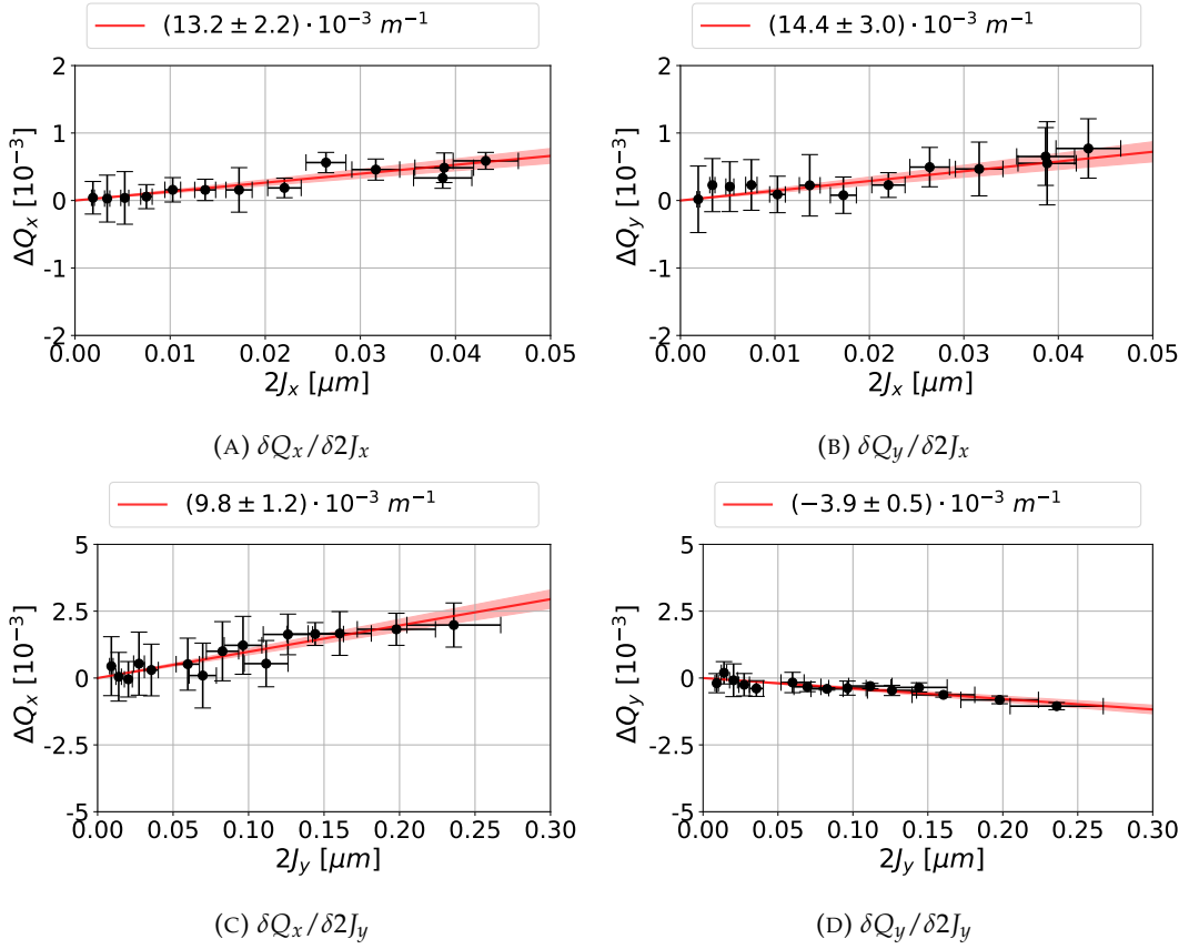
FIGURE 4.10: Measured amplitude detuning for the targeted MCS powering. Note that here the direct amplitude detuning is factor 2 larger compared to the case of free excitations due to the use of the AC-Dipole [125].
