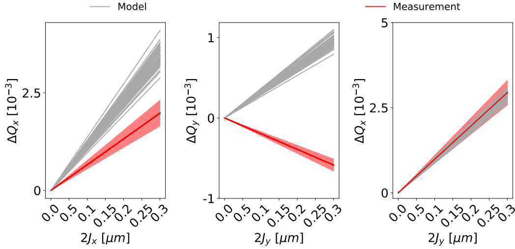
FIGURE 4.20: Comparison between the measured amplitude detuning and the amplitude detuning for the WISE seeds.
