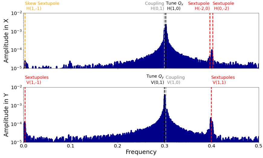
(A) Working point Q_x = Q_y = 5.30
