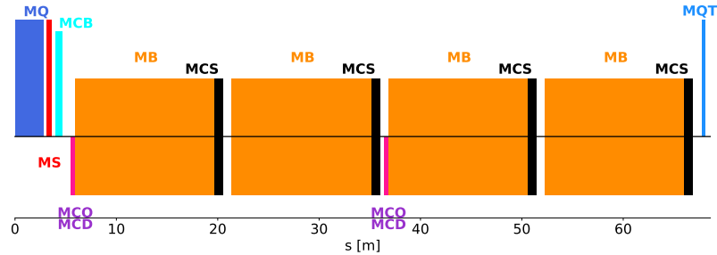
(A) One half-cell in the 18 cells layout
