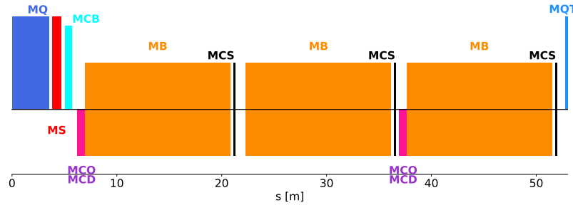
(B) One half-cell in the 23 cells layout
