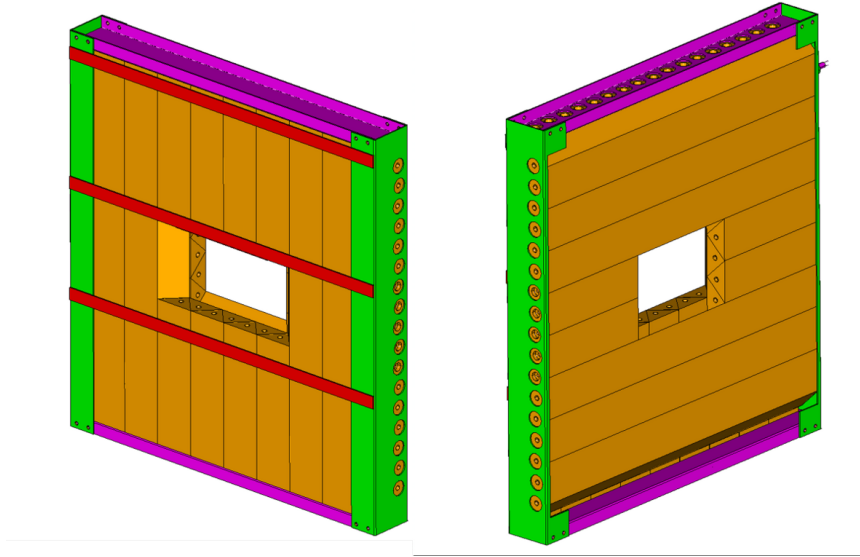
Figure 4.6: A sketch of a single CHANTI station, with the elements of the supporting frame (in green, violet and red). Left: beam view; right: rear view.
