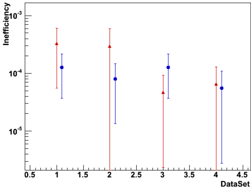
Figure 3.13: Comparison between data (in red) and Monte Carlo (in blue) for inefficiency of 5x5 OPAL prototype, different data sets are compared.
