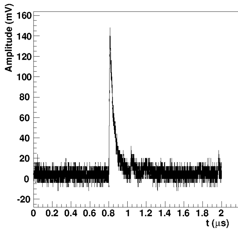
Figure A.5: Signal from a Hamamatsu SiPM (amplified 10\times ).
