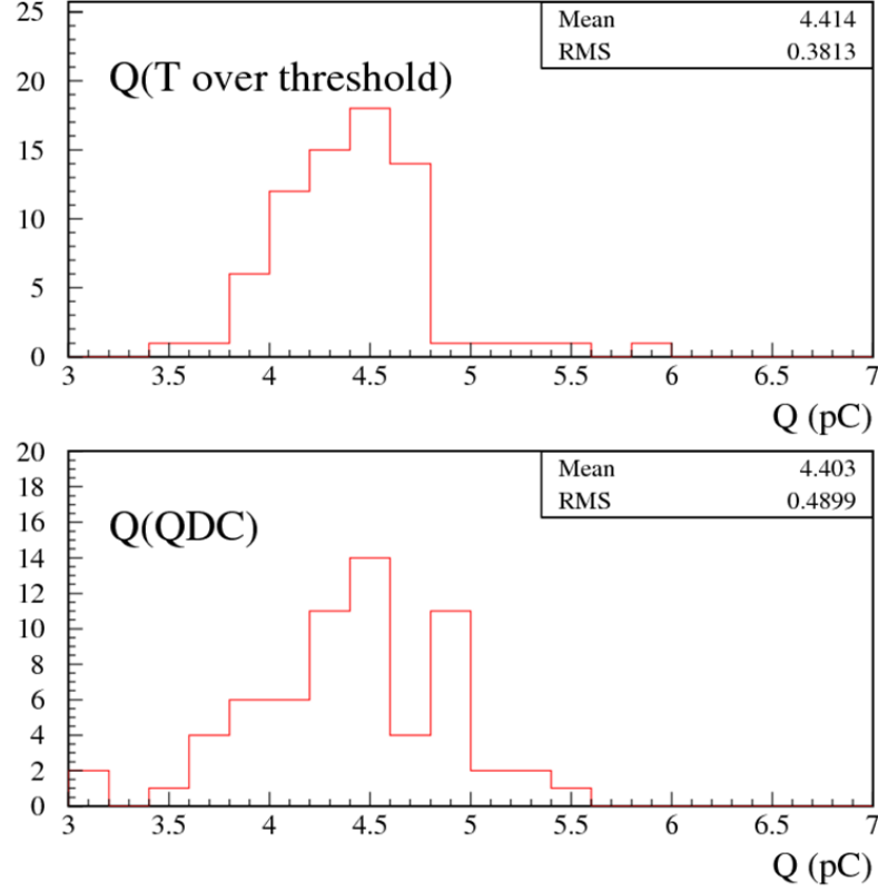
Figure 3.31: QDC (bottom) compared with ToT (top) response.
