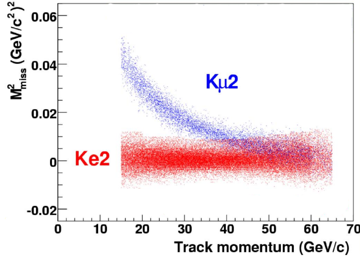
Figure 1.7: M_{miss}^2 vs track momentum in electron mass hypothesis.
