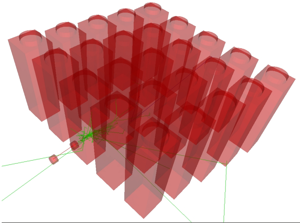
Figure 3.14: An electron event of prototype simulation.
