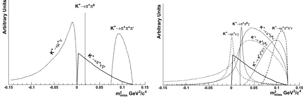
Figure 2.2: On left side constraints on kinematics, on right side not kinematically constrained decays.
