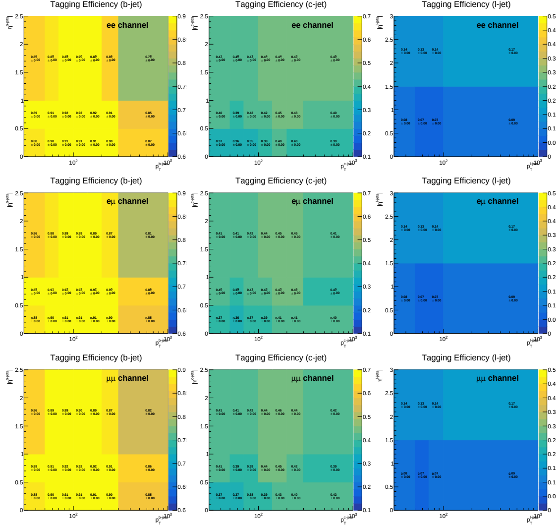
Figure F.2: The b-tag efficiency and mistag rates are computed in bins of jet p_T and eta and are shown for 2017 in the e^\pm e^\mp (top row), e^\pm \mu^\mp (middle row) and \mu^\pm \mu^\mp (third row) channels. The b-tagging efficiency is shown in the first column while the mistag rates for c- and light-jets are shown in the second and third column respectively.
