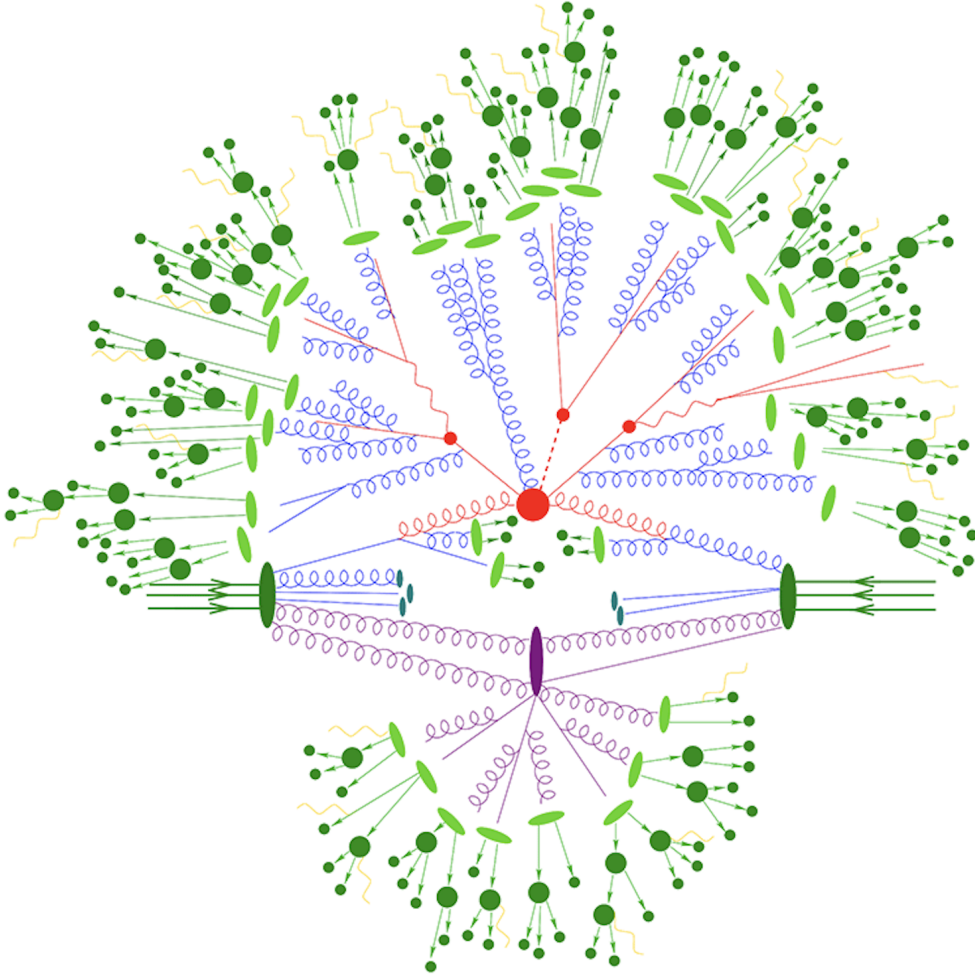
Figure 4.1: An overview of the steps involved in MC simulations [59]; the hard process is shown in red, the parton shower modelling is illustrated in blue, the hadronization process is shown in green and the underlying event is depicted in purple.
