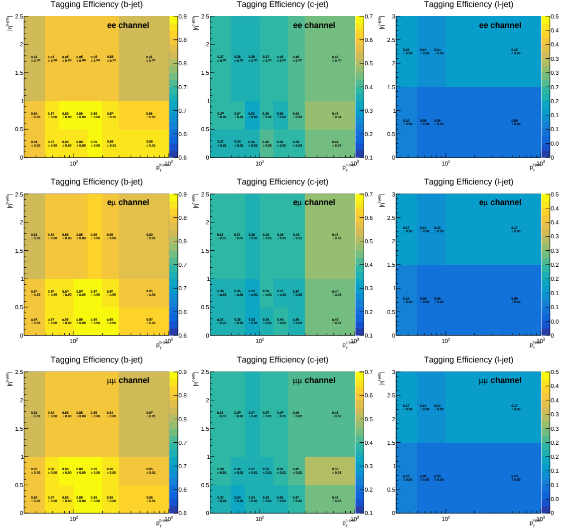
Figure F.1: The b-tag efficiency and mistag rates are computed in bins of jet p_T and eta and are shown for 2016 in the e^\pm e^\mp (top row), e^\pm \mu^\mp (middle row) and \mu^\pm \mu^\mp (third row) channels. The b-tagging efficiency is shown in the first column while the mistag rates for c- and light-jets are shown in the second and third column respectively.
