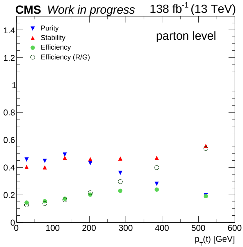
Figure 6.4: The purity, stability and efficiency for the single-differential measurement of the transverse momentum of the top, p_T(t) , in the full phase at parton level.
