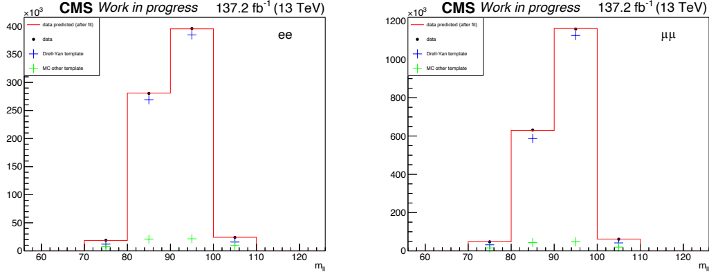
Figure 5.1: Dilepton mass distributions in the Z-peak control region, i.e. 76 \leq m_{\ell\ell} \leq 106 GeV, are shown for the e^\pm e^\mp (left) and \mu^\pm \mu^\mp (right) channels for Run 2, after the event selection according to step 6 (see Section 5.9). The input data distributions are illustrated by black dots, the Z+jets templates are shown in blue and the MC other templates are depicted in green. The red histograms illustrate the results of the fits performed by TFractionFitter.
