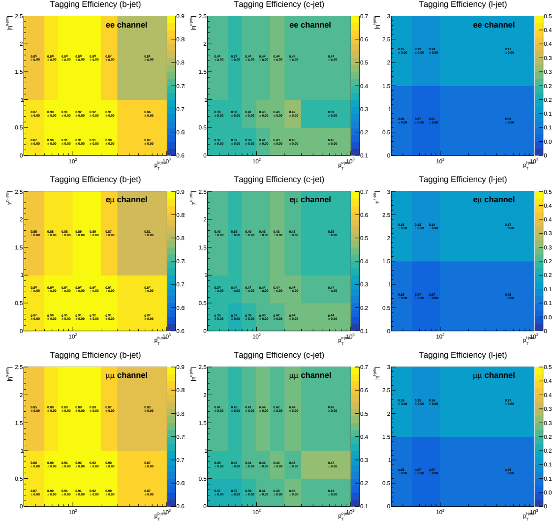
Figure F.3: The b-tag efficiency and mistag rates are computed in bins of jet p_T and eta and are shown for 2018 in the e^\pm e^\mp (top row), e^\pm \mu^\mp (middle row) and \mu^\pm \mu^\mp (third row) channels. The b-tagging efficiency is shown in the first column while the mistag rates for c- and light-jets are shown in the second and third column respectively.
