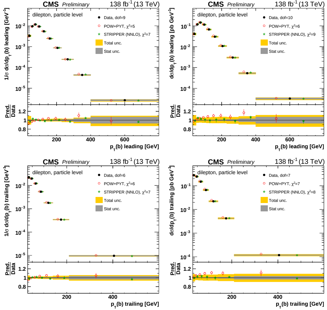
Figure 8.43: Differential t\bar{t} cross sections measured as functions of the transverse momentum of the leading b quark, p_T(b) leading, in the top row and the transverse momentum of the trailing b quark, p_T(b) trailing, in the bottom row. The measurements are performed in the fiducial phase space at particle level. The left and right columns show normalized and absolute cross sections, respectively. For further details see Figure 8.28.
