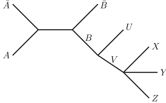
Figure C.1: Example process, A\bar{A} \rightarrow B\bar{B} , B \rightarrow UV , V \rightarrow XYZ , used to illustrate phase space factors.
