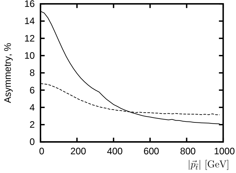
Figure 6.1: The asymmetry \mathcal{A}_T , Eq. (3.36), as a function of the stop momentum, |\vec{p}_t| , in the laboratory frame. The solid line is the asymmetry for the triple product \mathcal{T}_{\ell_N} , Eq. (6.11) and the dotted line is for the triple product \mathcal{T}_{\ell\ell} , Eq. (6.13). The respective masses are given in Tab. 6.2, Tab. 6.3 and Tab. 6.4.
