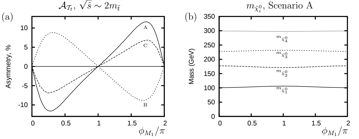
Figure 4.3: The asymmetry at threshold for the production process gg \rightarrow t\bar{t}^* for scenarios A, B and C for (a) \mathcal{A}_{T_t} as a function of \phi_{M_1} , and (b) the masses of the neutralinos as functions of \phi_{M_1} .
