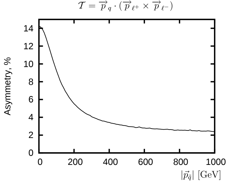
Figure 5.2: The parton-level asymmetry \mathcal{A}_{\mathcal{T}} , Eq. (5.7), for the single decay chain given in Eq. (5.4) as a function of the squark momentum, |\vec{p}_q| , in the laboratory frame. Only the \tilde{q} asymmetry is shown and the dilution due to \tilde{q}^* is not included. The scenario is given in Table 5.1 with the phase \phi_{M_1} = 3\pi/2 .
