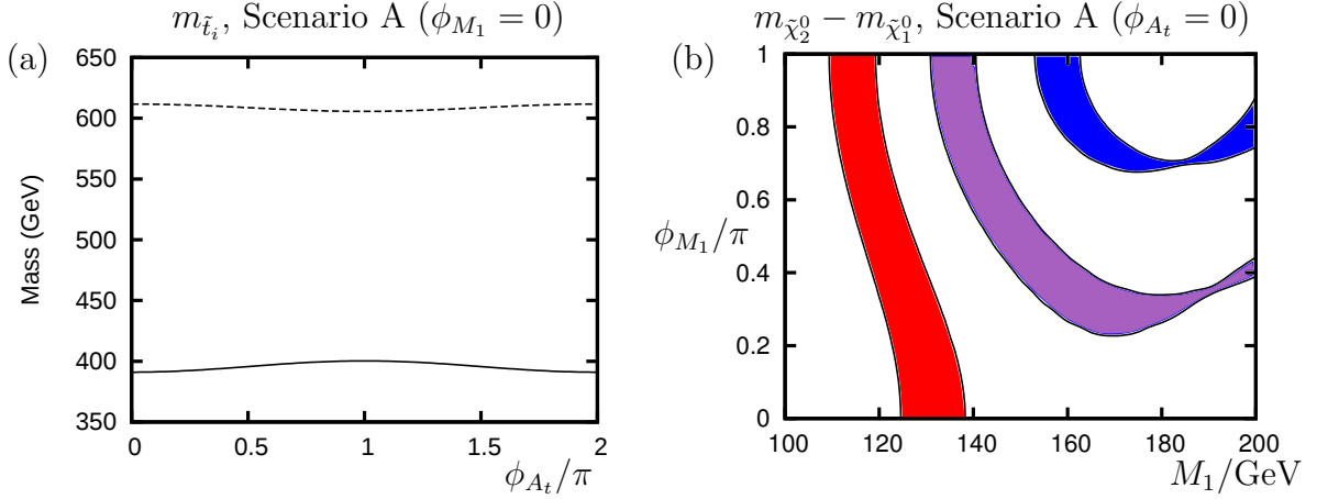
Figure 4.14: (a) The mass of the stop squarks \tilde{t}_j , j=1,2 as functions of \phi_{A_t}/\pi , and (b) contour plot showing the areas of the (M_1, \phi_{M_1}) parameter plane consistent with a mass difference between \tilde{\chi}_2^0 and \tilde{\chi}_1^0 of 20 GeV (blue), 40 GeV (purple) and 60 GeV (red) respectively. The bands assume a 1% error in experimental measurement of the mass difference and a 5% error in M_2 .
