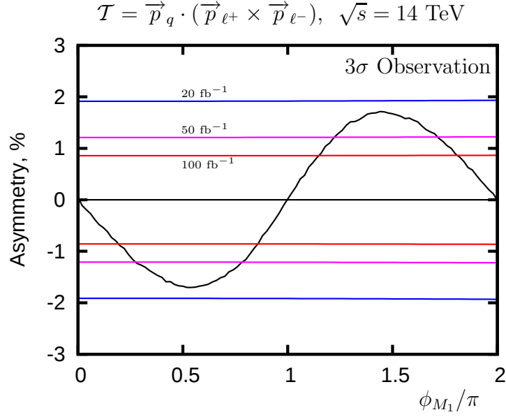
Figure 5.6: The parton-level asymmetry \mathcal{A}_T , Eq. (5.7), in the laboratory frame with PDFs included in the analysis using the scenario shown in Tab. 5.1. The coloured lines show the size of the asymmetry needed for a 3\sigma observation at the given luminosity, \mathcal{L}=(20 \text{ fb}^{-1}, 50 \text{ fb}^{-1}, 100 \text{ fb}^{-1}) , assuming squarks were produced via the channels shown in rows 3 and 4 of Tab. 5.2. All produced \tilde{q} and \tilde{q}^* that follow the decay chain given in Eq. (5.4) are taken into account.
