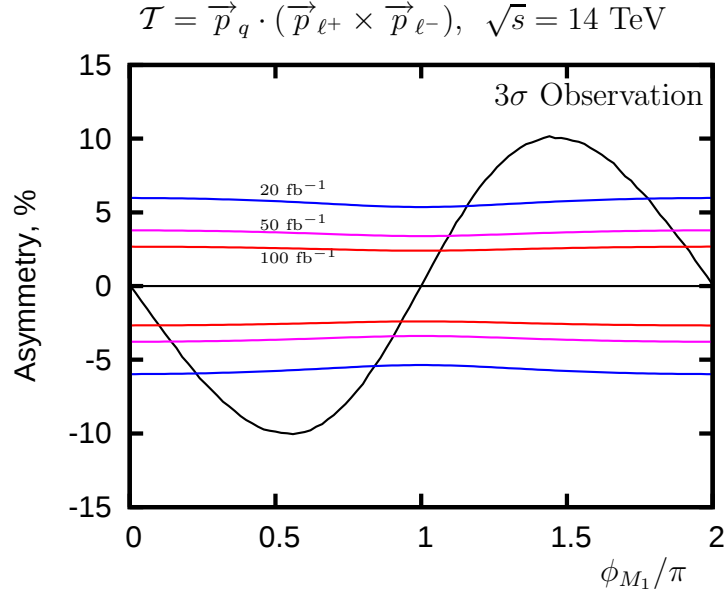
Figure 5.7: The parton-level asymmetry \mathcal{A}_T , Eq. (5.7), in the reconstructed \tilde{q}_L rest frame. The coloured lines show the size of the asymmetry needed for a 3\sigma observation at the given luminosity, \mathcal{L}=(20 \text{ fb}^{-1}, 50 \text{ fb}^{-1}, 100 \text{ fb}^{-1}) for the production channels \tilde{q}_L\tilde{g}, \tilde{q}_L^*\tilde{g} Tab. 5.2. The decay chains included are shown in Eq. (5.4) and Eq (5.13). As explained in the text correct jet and lepton assignment is assumed.
