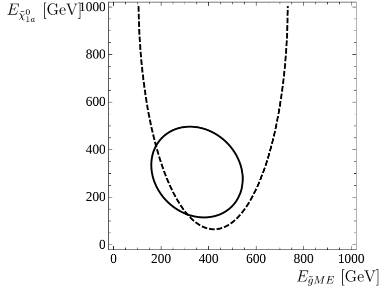
Figure 5.4: Ellipses in the E_{\tilde{\chi}_{1a}^0} and E_{\tilde{g}ME} plane corresponding to Equations (5.33) (solid line) and (5.34) (dashed line) for one sample event. Out of the two real solutions the lower right one gives the correct momenta of the original event.
