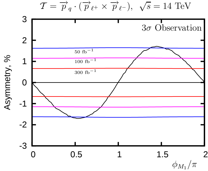
Figure 5.8: The asymmetry \mathcal{A}_T , Eq. (5.7), in the laboratory frame for the decay chain Eq. (5.4) after the cuts, Eqs. (5.47)-(5.51), have been applied. The coloured lines show the size of the asymmetry needed for a 3\sigma observation at the given luminosity, \mathcal{L}=(50 \text{ fb}^{-1}, 100 \text{ fb}^{-1}, 300 \text{ fb}^{-1}) , assuming squarks were produced via the channels shown in rows 3 and 4 of Tab. 5.2. Momentum smearing for both the leptons and quarks was studied and found to have a negligible effect. All other relevant experimental details are mentioned in the text.
