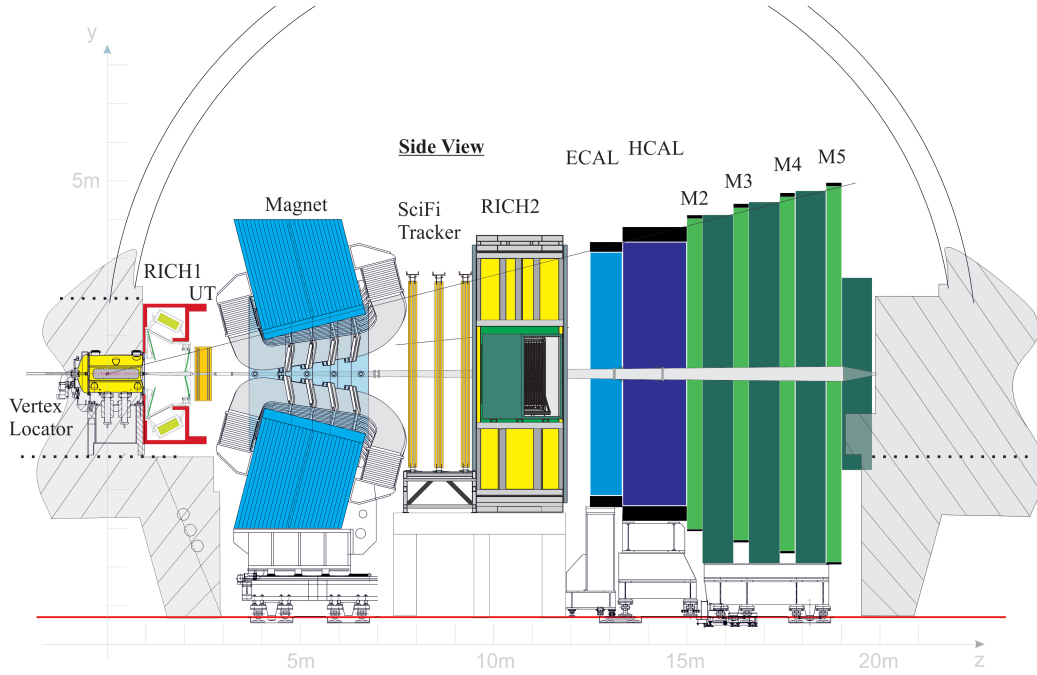
Figure 2.3: Schematic view of the upgraded LHCb detector, taken from Ref. [23].
