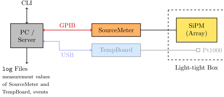
Figure 4.5: SiPM test setup C.
