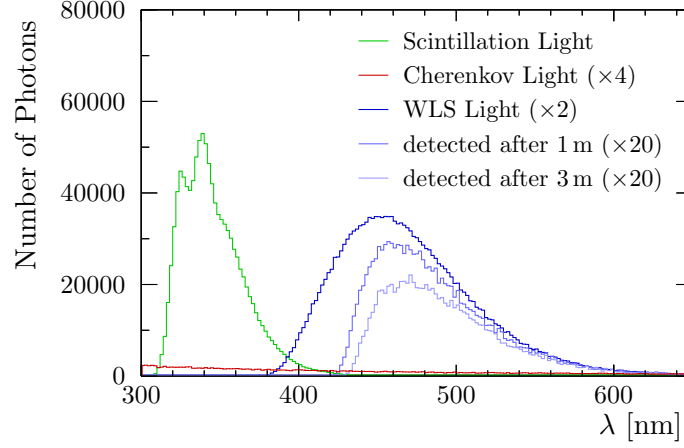
Figure 3.24: Wavelength spectra generated by physical processes in a simulated scintillating fibre of type SCSF-78MJ. Minimum ionising muons serve as exciting particles. Apart from scintillation light data, all distributions are multiplied by a scale factor (quoted in parentheses) to be distinguishable.
