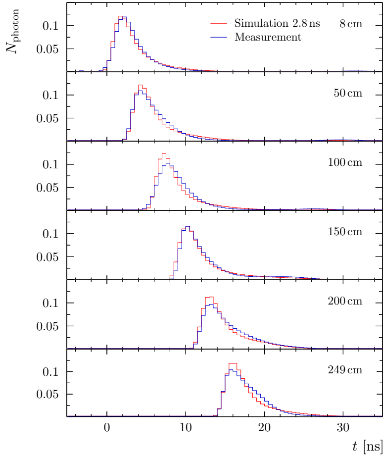
Figure 3.61: Measured and simulated time distributions of photon number N_{\text{photon}} with untreated fibre end. Results from several excitation positions x are shown. Simulated data are due to the decay time given in the legend. They include uncertainties resulting from the deconvolution process, see text. Each distribution is normalised so that the sum over all bins is 1.
