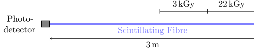
Figure 3.43: Simulated dose profile of fibre irradiation at CERN PS.
