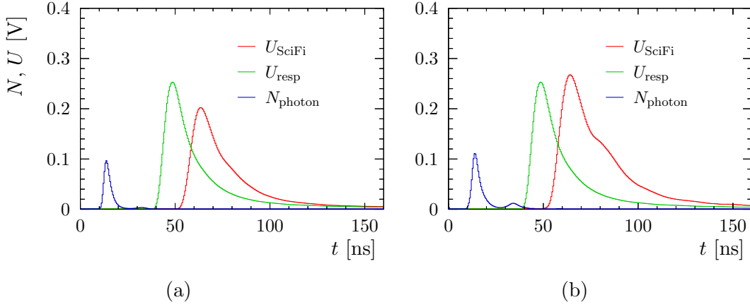
Figure 3.59: Measured MPPC output U_{\text{ScFi}} corresponding to fibre excitation at x = 100 cm. Plots (a) and (b) show acquired curves before and after metallisation of the fibre end, respectively. Deconvolution results for photon number distributions N_{\text{photon}} as well as the used response function U_{\text{resp}} are also drawn. U_{\text{ScFi}} and N_{\text{photon}} are scaled by a factor of 2 in (a) and 5 in (b) for the purpose of visibility.
