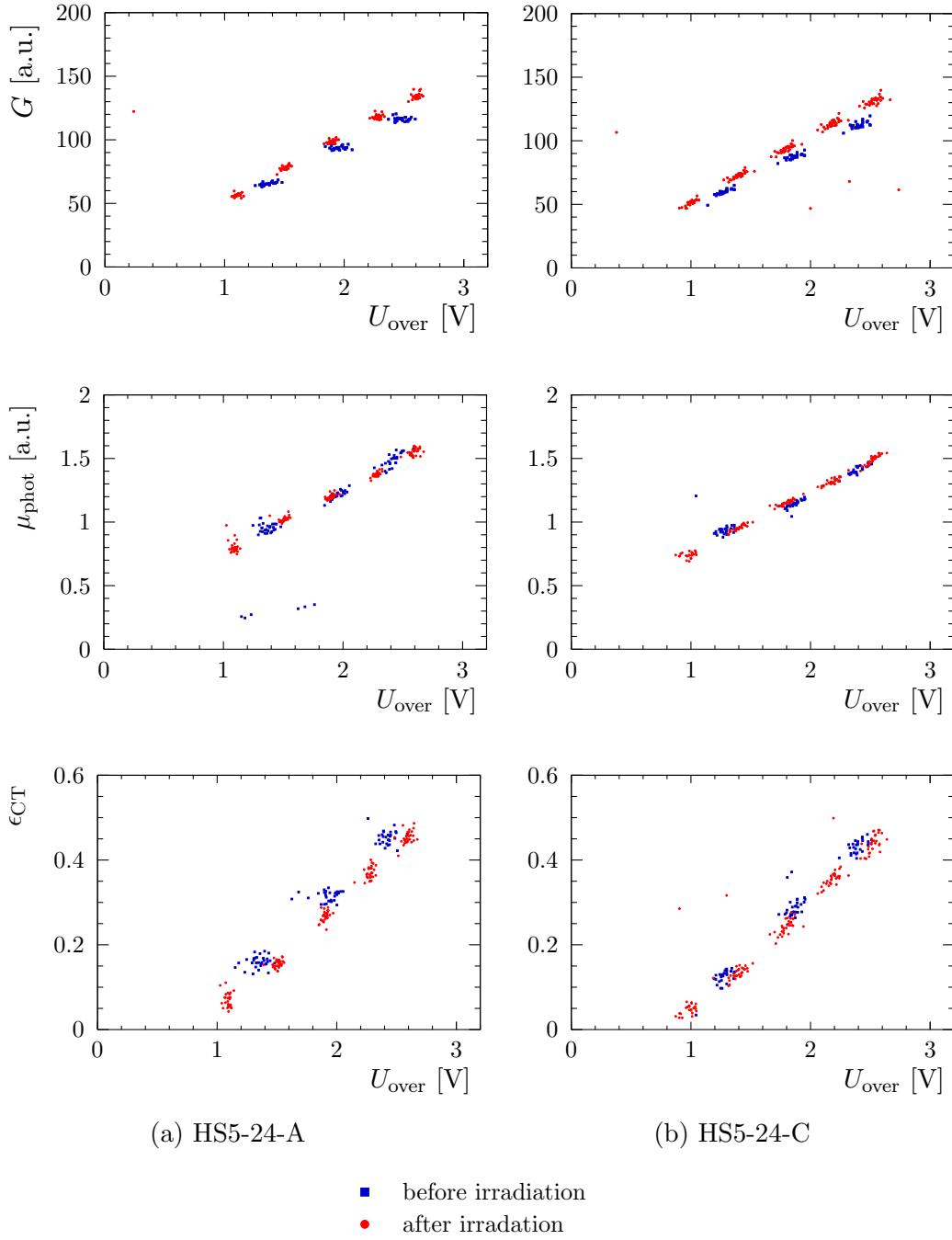
Figure 4.34: Gain G , mean number of detected photons per LED pulse \mu_{\text{phot}} (normalised) and cross-talk probability \epsilon_{\text{CT}} as a function of over-voltage U_{\text{over}} . Data points are obtained from signal spectra of individual channels of the respective SiPM array. Measurements were taken immediately before and 30 months after proton irradiation at MLL.
