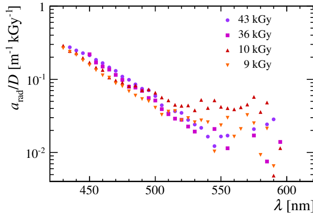
Figure 3.11: Additional radiation-induced absorption coefficient a_{\text{rad}} per dose D vs. photon wavelength \lambda in scintillating fibre SCSF-78MJ after accumulation of different doses. The values are calculated from attenuation length data from Ref. [58]. The data points of different doses are consistent with each other within their uncertainties. For the purpose of clarity the uncertainties are not shown.
