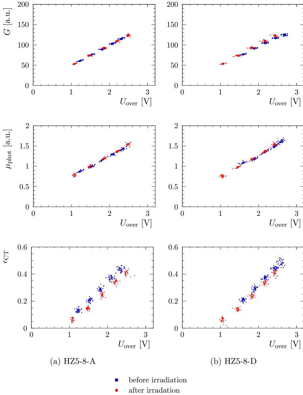
Figure 4.38: Gain G , mean number of detected photons per LED pulse \mu_{\text{phot}} (normalised) and cross-talk probability \epsilon_{\text{CT}} as a function of over-voltage U_{\text{over}} . Data points are obtained from signal spectra of individual channels of the respective SiPM array.
