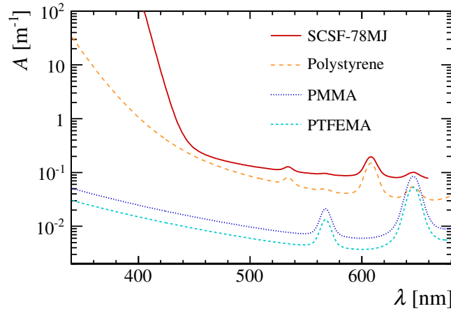
Figure 3.9: Estimated intrinsic loss coefficient of PMMA and PTFEMA vs. wavelength. Curves obtained from a fit to polystyrene and SCSF-78MJ data are shown for comparison.
