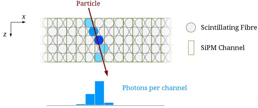
Figure 2.4: Arrangement of scintillating fibres and SiPM channels in a fibre tracker module. The fibre diameter in the LHCb SciFi Tracker is 250\text{ }\mu\text{m} . The coordinates given in the figure are those of the right-handed coordinate system of LHCb with beam-pipe direction z and vertical direction y , compare Fig. 2.3.
