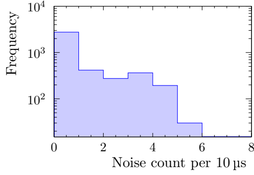
Figure 4.22: Noise count measured with HZ5-7-A at 0.13 V below U_{BD} .
