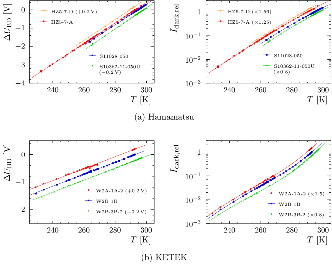
Figure 4.29: Change of breakdown voltage \Delta U_{\text{BD}} and relative dark current I_{\text{dark,rel}} as function of temperature T . Data and fit curves are shifted or scaled by values given in parentheses to improve visibility of individual curves.
