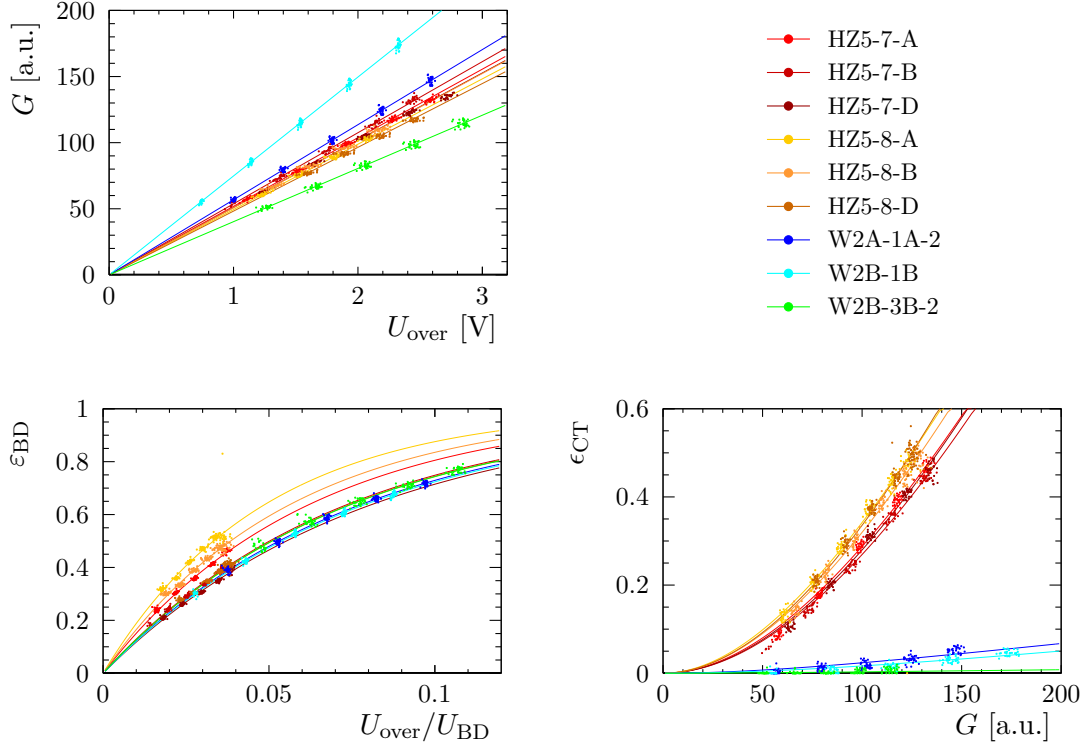
Figure 4.13: Parameters of 32-channel SiPM arrays from Hamamatsu and KETEK obtained from fitting signal spectra of individual channels. Curves are according to Eq. (4.23), (4.24) and (4.26) with parameters given in Tab. 4.2 and 4.3.
