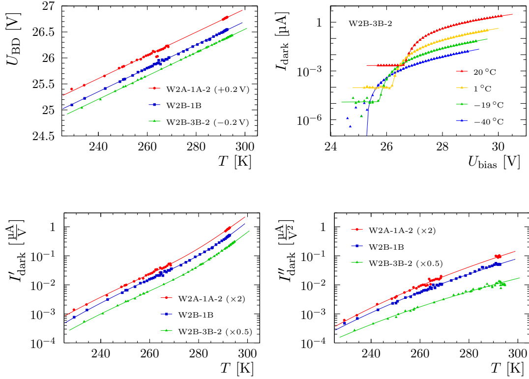
Figure 4.31: Temperature dependence of breakdown voltage U_{BD} and dark current coefficients I'_{dark} , I''_{dark} used in Eq. (4.38) with (4.48). Parameters are determined by fitting Eq. (4.38) to I - U data of KETEK SiPMs. Four exemplary I - U data sets and corresponding fit curves are shown in the top right plot.
