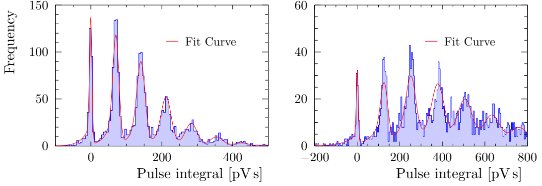
Figure 4.41: SiPM signal spectra of S11028-050 measured with test setup B at over-voltages 1.03 V (left) and 1.83 V (right) after irradiation. The ambient temperature during measurement is -17.3^\circ\text{C} .
