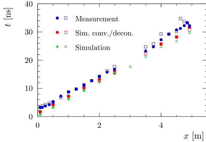
Figure 3.65: Arrival times t of signal peaks at the photodetector as function of fibre length x from the excitation to the instrumented fibre end. Open symbols denote results from fibre with mirrored end face. The abbreviation conv./decon. refers to simulation data being convolved with U_{\text{resp}} and subsequently deconvolved to include correspondent uncertainties.
