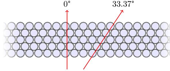
Figure 3.37: Two particles crossing a mat of scintillating fibres under different angles \varphi relative to the surface normal. The mat is made up from five layers of fibres with a diameter of 250\ \mu\text{m} and 275\ \mu\text{m} horizontal pitch. The particles' momentum directions are perpendicular to the fibre axes.
