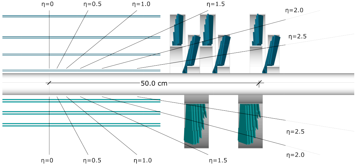
Figure 3.6: A cross-section comparison of the Phase 0 CMS pixel tracker (turquoise, bottom) and Phase 1 pixel tracker (blue, top) .[51]
