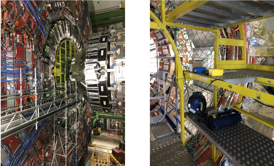
Figure 4.11: The left image shows the minus-side Surkov frame, connected via the passerelle. The right image was taken from the central platform inside the frame looking out of the frame, with the endcap nose in view.
