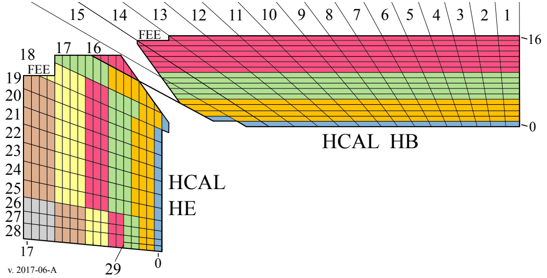
Figure 4.5: An yz -plane slice of the Phase 1 HCAL Barrel and Endcap. Towers and scintillating layers are indicated. Colored regions show the summed readout per-tower of the upgraded Phase 1 system. “FEE” indicates the location of the front end electronics, or the “RBx”.
