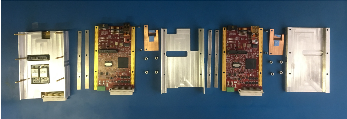
Figure 4.8: All components of a ngCCM, partially disassembled. Module is constructed left to right. The clock card is already installed between the bottom and a middle layer of housing in the leftmost part of the image. Additional copper heat sinks, called cooling fins, are also installed over the VTRx. The blue thermal gap pads used are visible on the heat sinks.
