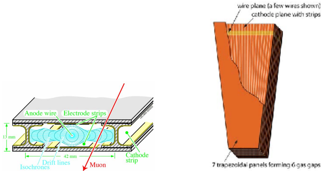
Figure 3.9: Left: Stylized diagram of a functioning cross-section of a drift tube. Right: Stylized diagram of a CSC showing the azimuthal wires, and the perpendicular strips.[44]
