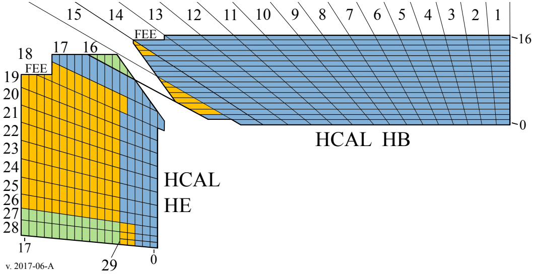
Figure 4.3: An yz -plane slice of the Phase 0 HCAL Barrel and Endcap. Towers and scintillating layers are indicated. Colored regions show the summed readout per-tower in the Phase 0 system. “FEE” indicates the location of the front end electronics, or the “RBx”.
