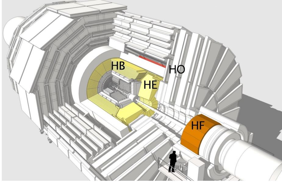
Figure 3.7: Labeled locations of the the HCAL subdetectors.
