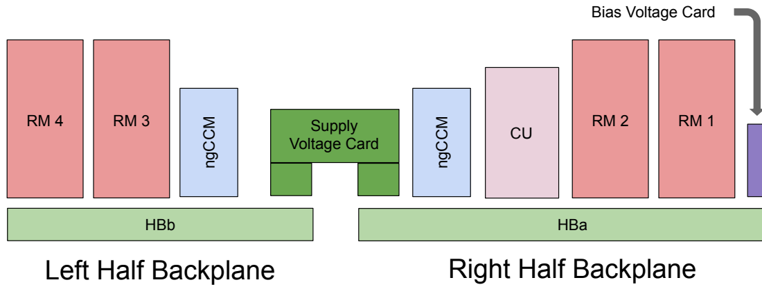
Figure 4.6: A schematic showing the naming, constituents, and organization of an HB RBx. Since HB RBxs are in 360°C, this specific orientation would only be found in the 6 o’clock position of either HB half.
