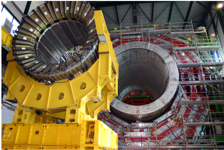
Figure 4.4: An image of HBP prior to insertion into the magnet's vacuum tank above ground in SX5 in March, 2006. [54]. Image shows not only the scale of one half of the HCAL Barrel, but the layered structure of the absorber. This is no longer visible, as it has been covered by the cable trays of the tracker.
