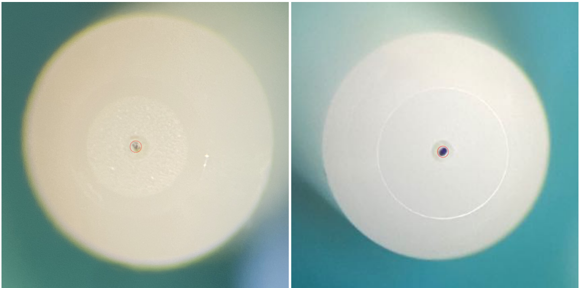
Figure 4.15: Image of fiber face after removal from drifting VTRx (left). Outgassed material appears as a white substance causing the perceived texture on the fiber face, and obscuring the central part of the fiber where light is transmitted(see red circle). Image of clean fiber for comparison (right).Red circled region is clear.
