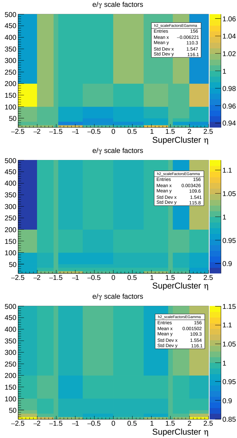
Figure A.5: Electron ID scale factors applied. From top to bottom: 2016, 2017, 2018. [80].
