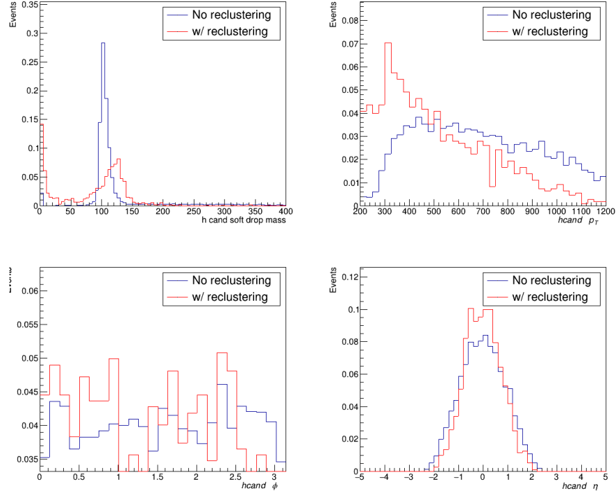
Figure 6.8: Kinematic plots of the m_{Z'} 3000 \text{ GeV} m_{N_D} 1200 \text{ GeV} m_{N_S} 1 \text{ GeV} signal mass point at skim level selections, in the Z candidate and H candidate overlap region ( \Delta R(Z, H) < 0.8 ). Skims selections require the Z candidate reconstruction, p_T^Z > 150.0 \text{ GeV} , and at least one fat jet. H candidate chosen as the fat jet closest to the Higg's mass. Distributions are normalized to unit area to show shape differences.
