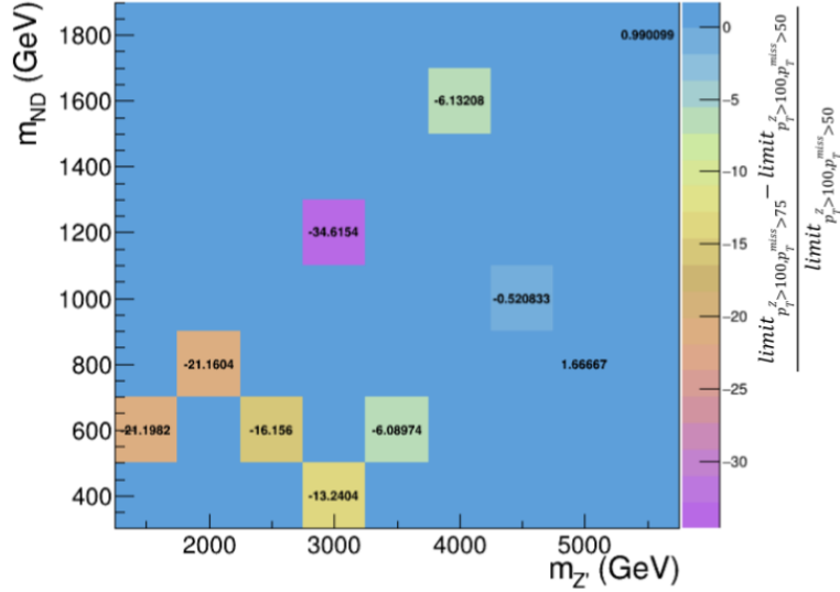
Figure 6.12: Percent difference between expected limits for the cut scenarios Z candidate p_T > 100 GeV, p_T^{\text{miss}} > 75 GeV and Z candidate p_T > 100 GeV, p_T^{\text{miss}} > 50 GeV. Negative values indicate that the limit of the p_T^{\text{miss}} > 75 GeV scenario is lower (more sensitive) than the limit of the p_T^{\text{miss}} > 50 GeV.
