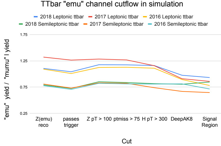
Figure 7.2: Value of e\mu/\mu\mu in simulation versus cut for leptonic and semileptonic t\bar{t} . Overall, the e\mu and \mu\mu channels of t\bar{t} respond similarly to the selections, producing a flat cutflow. This changes with the DeepAK8 tagger requirement in the leptonic channel. This produces about a 20% difference in efficiency between the e\mu and \mu\mu channels.
