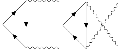
Figure 2.6: Triangle diagrams of an axial current vertex.
