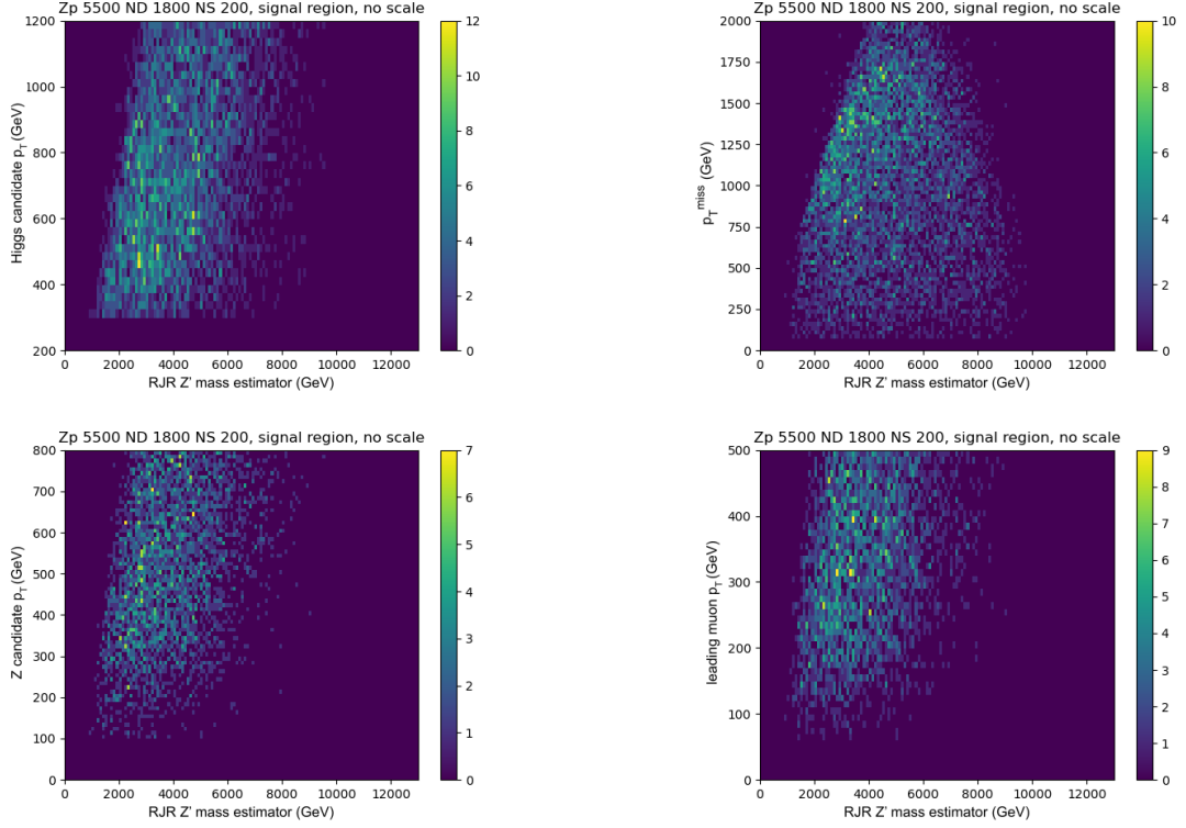
Figure 9.1: Relationship between the RJR Z' mass estimator and select kinematic inputs. Relationship is shown for the m_{Z'} 5500, m_{N_D} 1800, and m_{N_S} 200 signal mass point in the signal region. No cross section scaling is applied.
