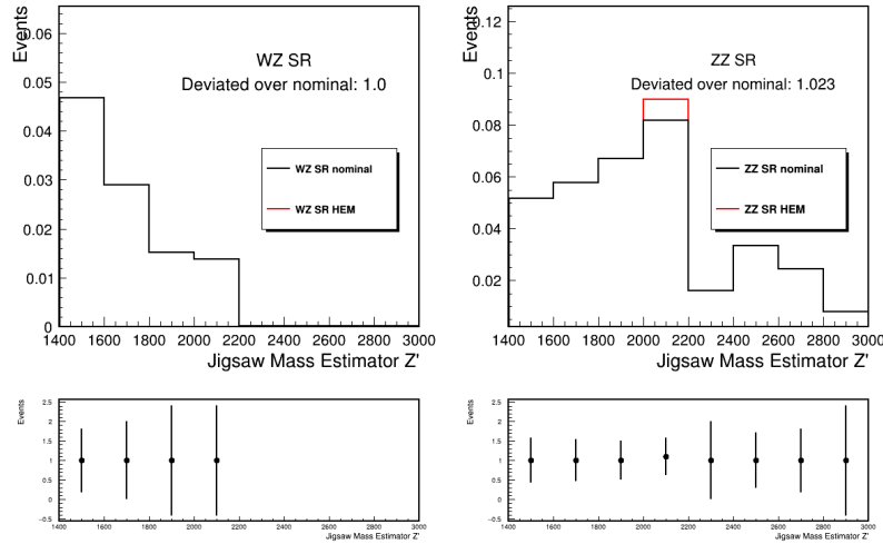
Figure 8.16: 2018 MC input distributions for the diboson background. Entire 2018 luminosity scaled, so any deviations over-estimate their expected value. Deviations are negligible, especially once combined with 2016 and 2017, as is done.
