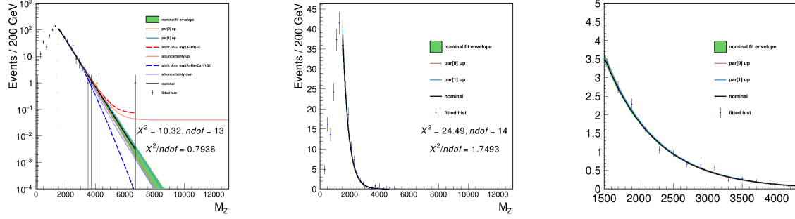
Figure 8.3: Left: data sideband region fits for full Run 2. Each additional fit represents the fit result with the labeled parameter shifted up in the decorrelated space. Middle: Same description but for the t\bar{t} MC contribution. Right: Same description but for the diboson contribution. The t\bar{t} and diboson functions are subtracted from the data sideband distribution to form the distribution that gets multiplied by the \alpha ratio.
