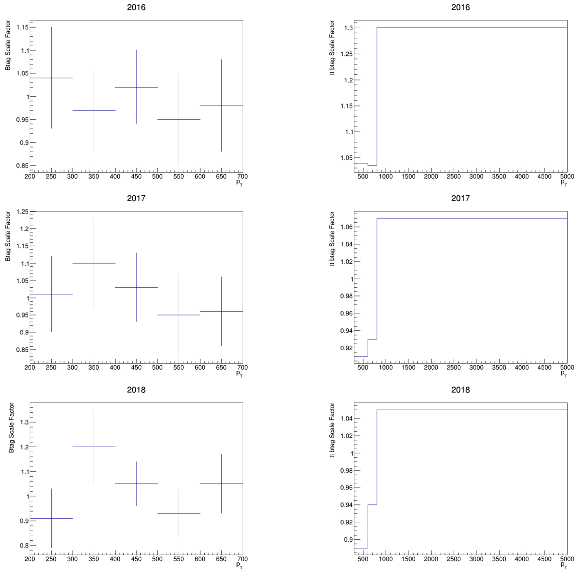
Figure A.6: Left column: Generic btagging scale factors. Right column: Btagging scale factors for t\bar{t} MC.
