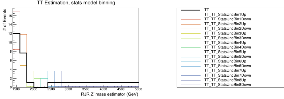
Figure 9.2: The t\bar{t} background estimation, taken from the electron and muon final-state t\bar{t} data.
