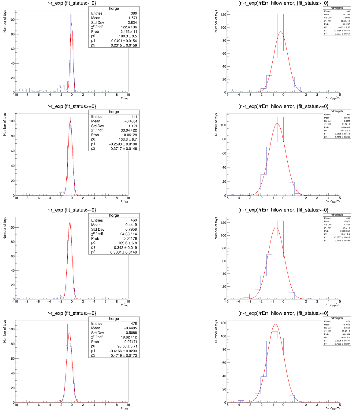
Figure 9.15: Differences (left) and pulls (right) for the measured and expected signal strengths for m_{Z'} = 2000 , m_{N_D} = 400 , m_{N_S} = 200 . First row has an injected signal of 0, the second has the lower expected limit, the third the median expected limit, and the final the upper expected limit.
