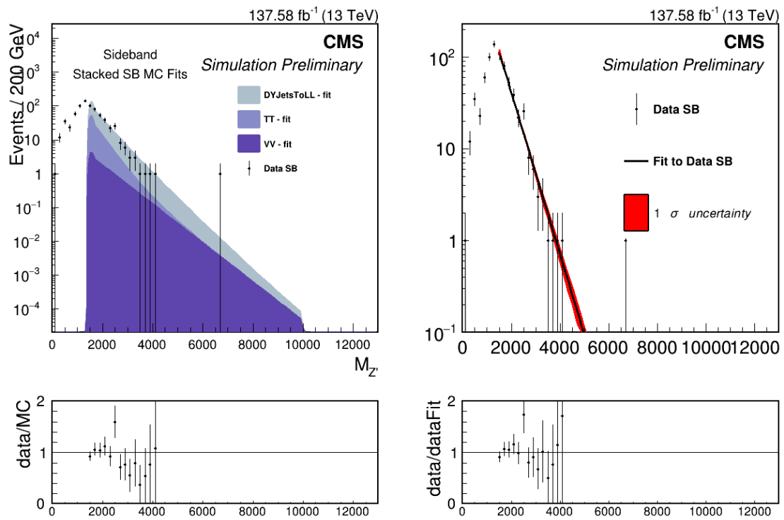
Figure 7.10: Plots showing the fit agreement with the data sideband. The left plot shows the sideband data overlaid with the individual background fits. The right plot shows the agreement between the sideband data and the fit.
