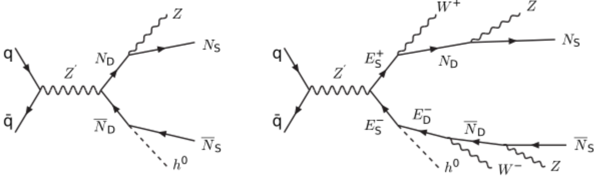
Figure 2.7: Illustrative decays of the baryonic Z' to anomalons.
