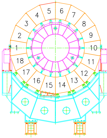
Figure 4.1: The numbering begins on the inside edge of the LHC ring. For example, looking at HBM while standing on a cherry picker in front of HEM, HBM1 would be at 9 o'clock, and HBM10 would be a 3 o'clock. [44]
