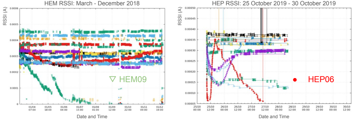
Figure 4.14: RSSI plot for all active links in the affected endcap over the lost module’s corresponding drift period. The HEM09 and HEP06 deviations are clear in comparison to the relative stability in the other modules.
