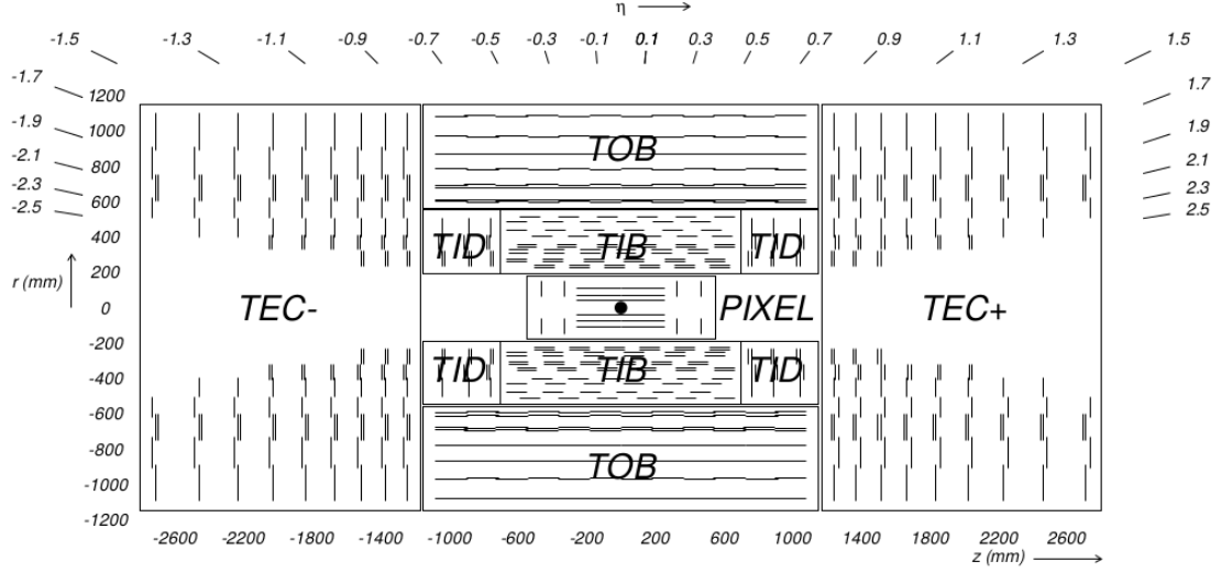
Figure 3.5: A cross-section schematic of the Phase 0 CMS tracker.[44]
