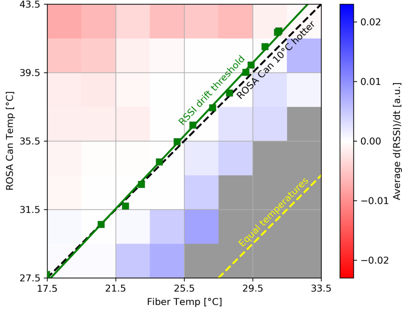
Figure 4.16: Mapping of operational phase space taken from measurements of a single, illustrative VTRx experiencing RSSI drift. This shows how the temperature difference between the fiber ferrule and the VTRx receiver influences the condensation of the outgassed material. The z -axis is the derivative of the RSSI, with a negative trend indicating the RSSI was decreasing, and a positive trend indicating that the RSSI was increasing. The trend in the RSSI reveals if the temperature settings either encourage condensation, or are unfavorable to condensation. Measurements are not available for the gray region.
