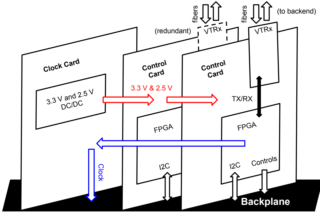
Figure 4.7: A block diagram of an HB ngCCM. Only one control card interfaces with the backend concurrently.
