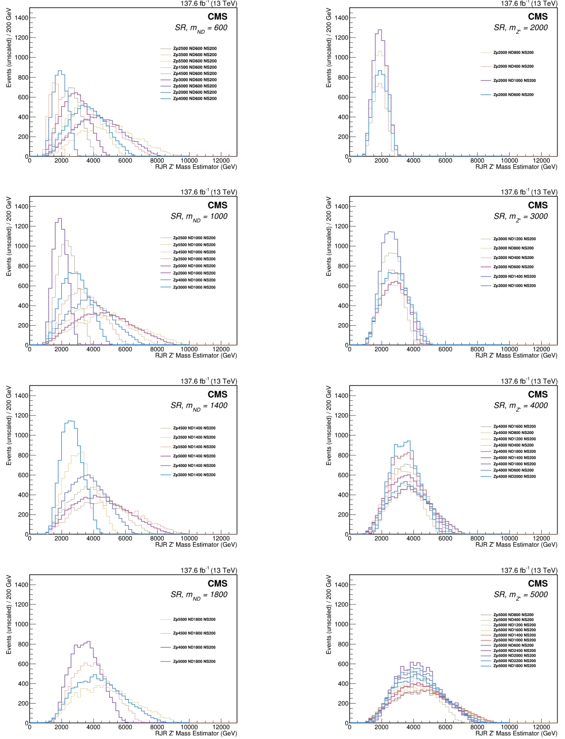
Figure 9.6: Selected values of fixed m_{N_D} and m_{Z'} comparing the Monte Carlo generated signal samples and the interpolated samples (bold lines). The left column is at fixed m_{N_D} , and the right column is at fixed m_{Z'} . All plots are for the m_{N_S} = 200 GeV case. The interpolation appears to be correctly modeling the shape and normalization trends.
