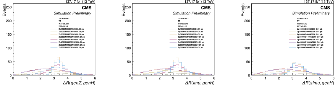
Figure 6.7: The figure on the left shows the generator-level \Delta R distribution at preselection for the Z and H in select signal samples. The middle and right figures show the \Delta R distribution at preselection of the reco level leading (middle) or subleading (right) muon and the generator-level H. The overlap region corresponds with \Delta R < 0.8 . Plots with reconstruction level objects were taken from samples with reclustering performed. The preselections applied are summarized in Section 6.5.
