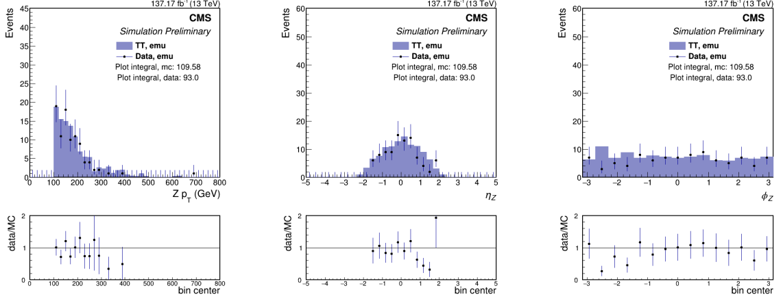
Figure B.2: Z to e\mu at preselection in the jet mass signal region featuring dilepton fake Z candidate kinematic distributions.
