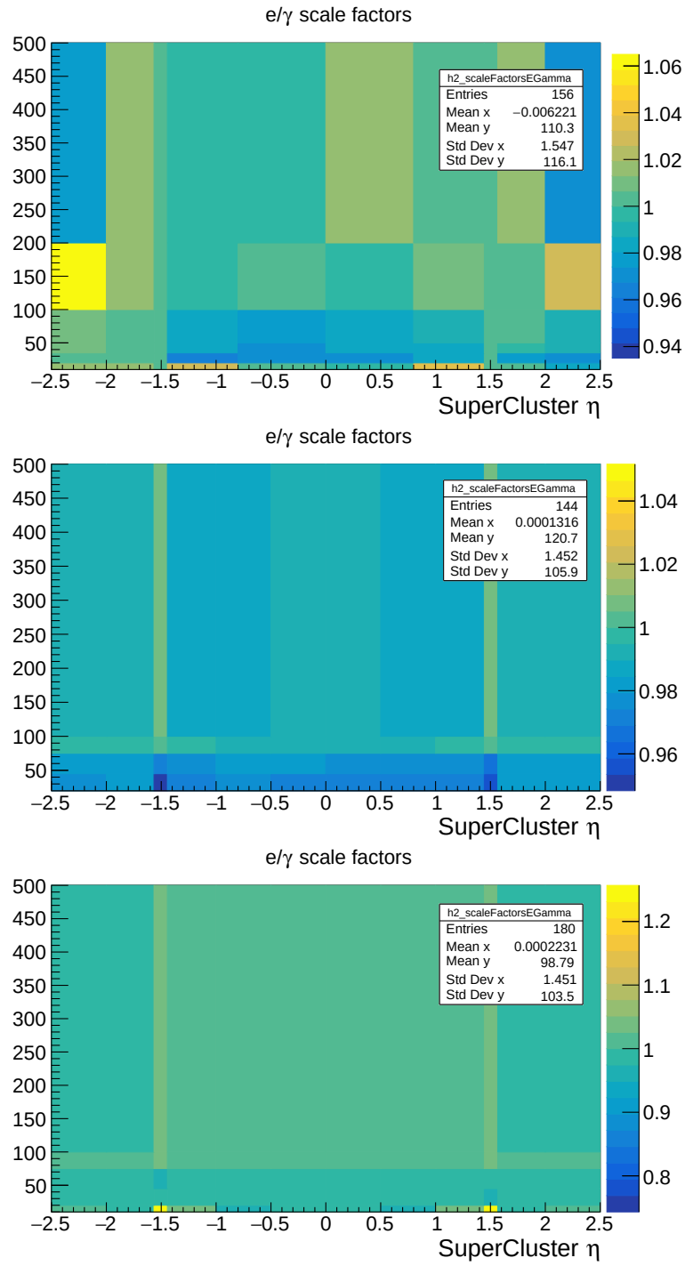
Figure A.4: Electron reconstruction scale factors applied. From top to bottom: 2016, 2017, 2018. [81].
