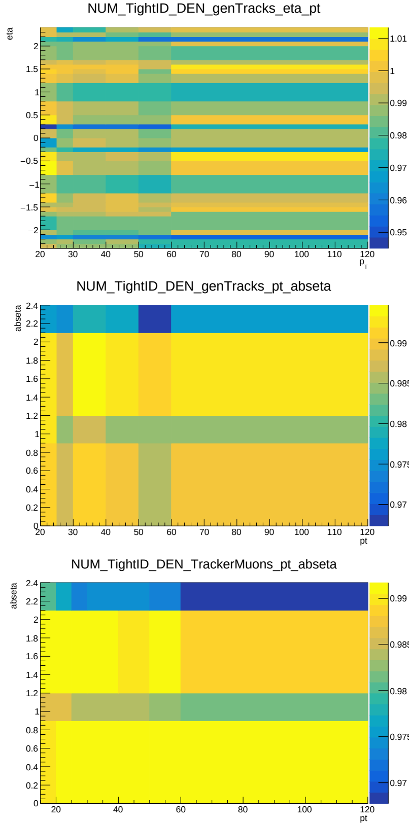
Figure A.3: Muon ID scale factors applied. The top figure shows the luminosity weighted 2016 scale factors [84]. The middle shows 2017 [85], and the bottom shows 2018 [86].
