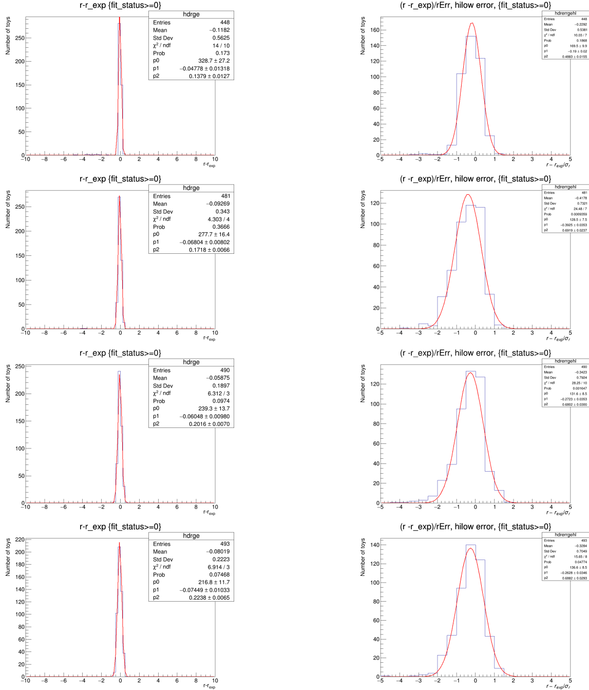
Figure 9.17: Differences (left) and pulls (right) for the measured and expected signal strengths for m_{Z'} = 5500 , m_{N_D} = 1800 , m_{N_S} = 200 . First row has an injected signal of 0, the second has the lower expected limit, the third the median expected limit, and the final the upper expected limit.
