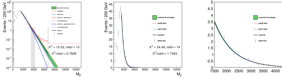
Figure 8.4: Left: data sideband region fits for full Run 2. Each additional fit represents the fit result with the labeled parameter shifted down in the decorrelated space. Middle: Same description but for the t\bar{t} MC contribution. Right: Same description but for the diboson contribution. The t\bar{t} and diboson functions are subtracted from the data sideband distribution to form the distribution that gets multiplied by the \alpha ratio.
