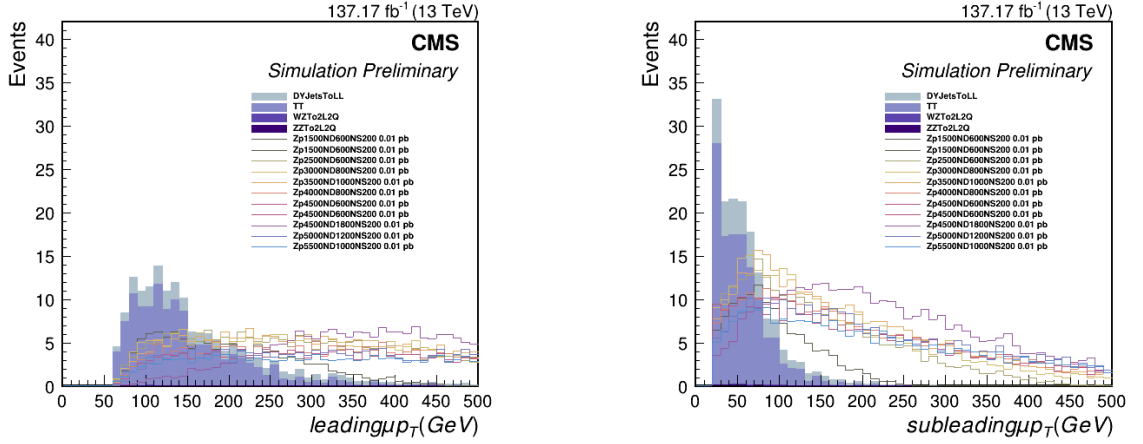
Figure A.1: Leading and subleading muon p_T in the signal region for a signal cross section of 10 fb. Boosted signal is possible, hence the addition of the last bin. No trigger scale factors applied.
