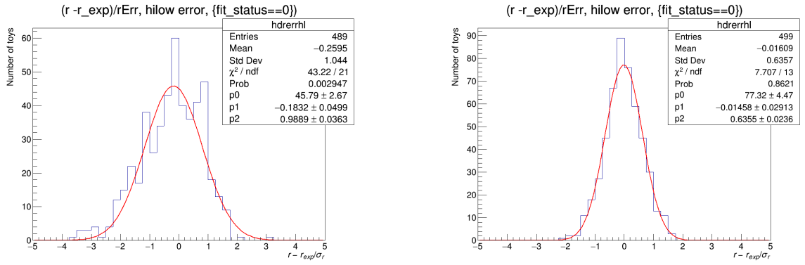
Figure D.3: Comparison between the unscaled (left) and scaled by 10 (right) pull distributions for the m_{Z'} = 5500 , m_{N_D} = 1800 , m_{N_S} = 200 signal mass point at 0.0 injected signal strength. Slight excess at negative pull values gone in the scaled version.
