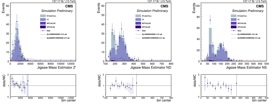
Figure 6.14: The soft drop mass sideband plots at preselection featuring the RJR mass estimator spectra. The plots are in units of GeV. The normalization for Drell-Yan MC derived in Section 7.2.1 is applied, but otherwise the filled histograms are nominal simulation.
