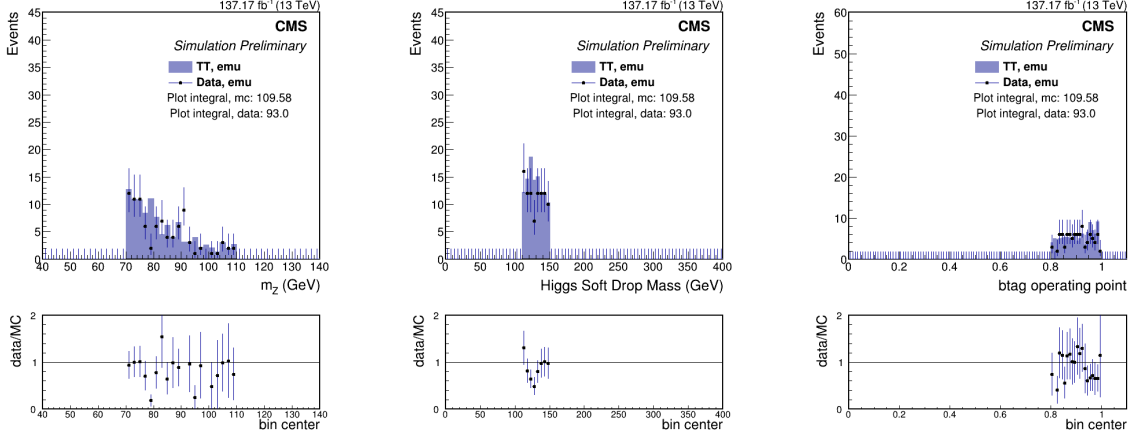
Figure B.4: Z to e\mu at preselection in the jet mass signal region featuring mass variables, and btagging values.
