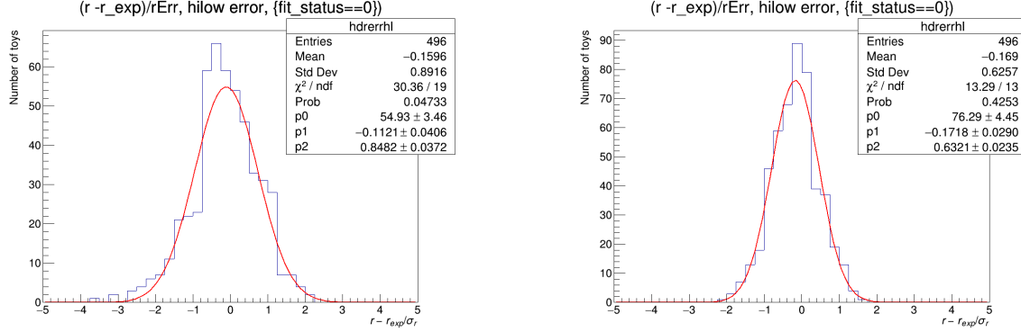
Figure D.1: Comparison between the unscaled (left) and scaled by 10 (right) pull distributions for the m_{Z'} = 2000 , m_{N_D} = 400 , m_{N_S} = 200 signal mass point at the median expected limit injected signal strength.
