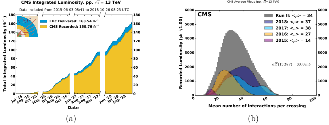
Figure 3.3: Total delivered and recorded integrated luminosity (3.3a) and average number of pile-up interactions (3.3b) measured at CMS during Run 2 of the LHC. Blank periods in the integrated luminosity plot show the periods of Year End Technical Stop (YETS) when the machine is down for maintenance.[47]
