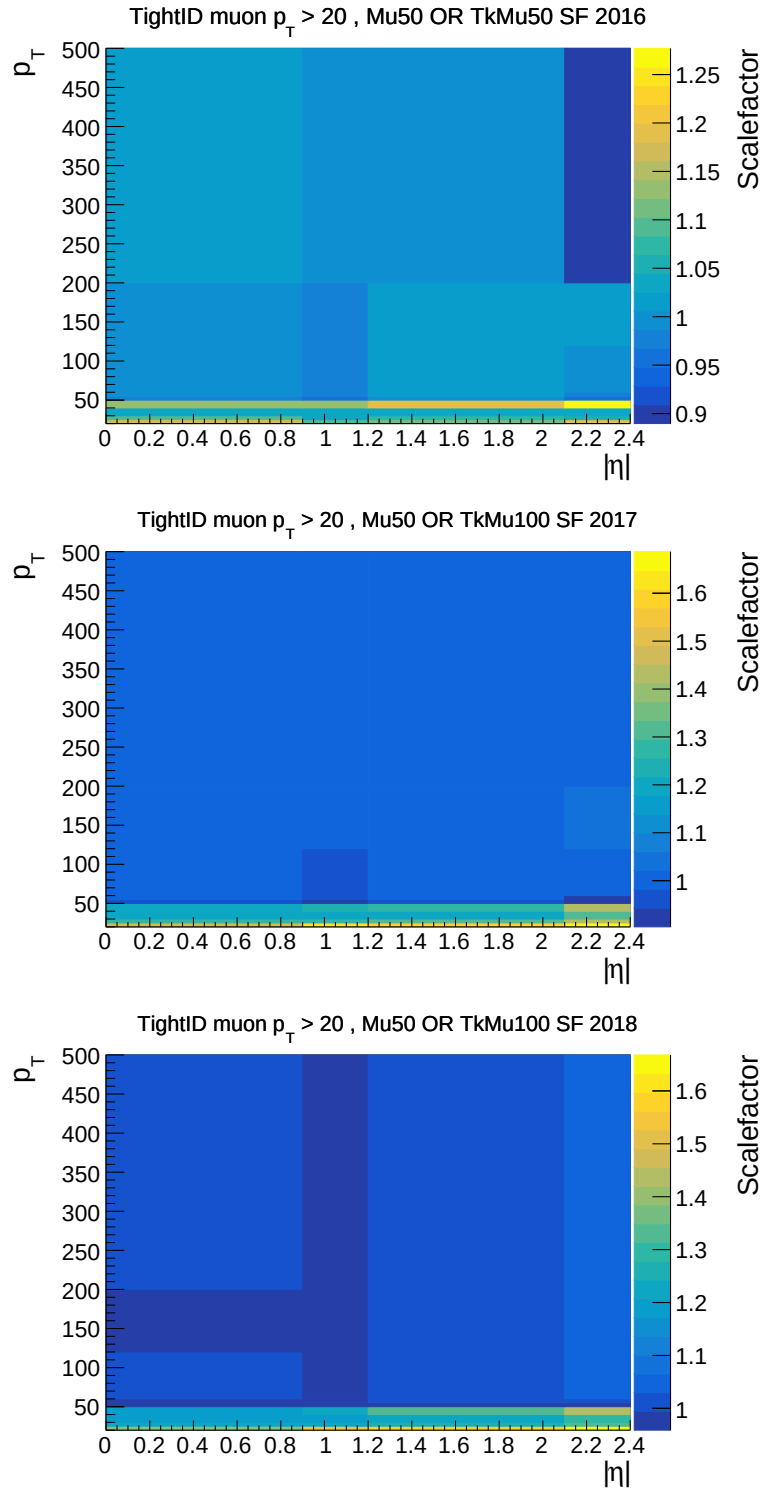
Figure A.2: Privately generated muon trigger scale factors for 2016 (top), 2017 (middle), and 2018 (bottom).
