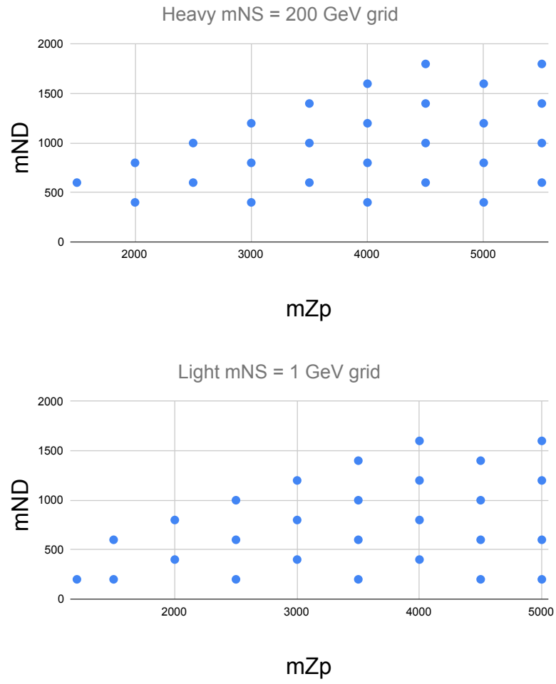
Figure 6.3: Grid of mass points generated for signal production.
