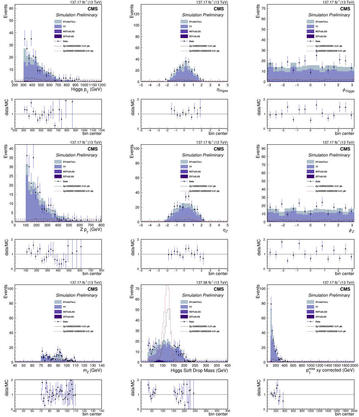
Figure 6.13: The soft drop mass sideband region plots of select final state particle object kinematic distributions. The normalization for Drell-Yan MC derived in Section 7.2.1 is applied, but otherwise the filled histograms are nominal simulation.
