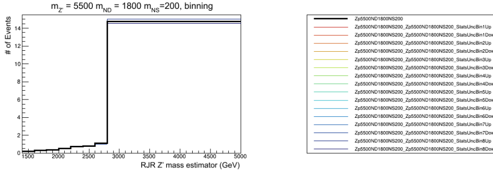
Figure 9.4: Highest m_{Z'} and m_{ND} signal mass point with the final statistical model binning.
