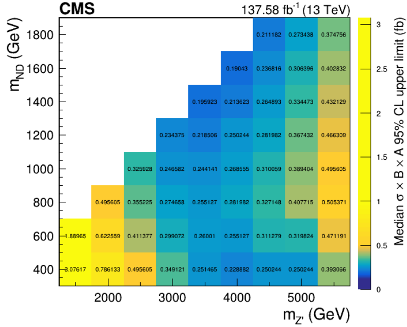
Figure 9.18: Asymptotic fiducial cross section upper limits for 2016-2018 are shown in the m_{N_D} and m_{Z'} plane for the m_{N_S} = 200 GeV scenario. Limits shown in fb.
