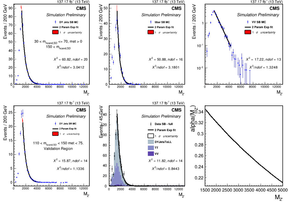
Figure 7.13: Top Left: Sideband Drell-Yan + jets MC RJR Z' mass estimator distribution with derived normalization. Top Middle: Sideband of t\bar{t} . Top Right: WZ and ZZ sideband. Bottom Left: validation region Z + jets MC. Bottom Right: \alpha ratio formed from the ratio of the fits in the bottom left and top left plots. Bottom Middle: data sideband and fit.
