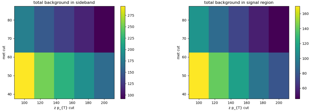
Figure 6.11: The cutflow of total background in the sideband and the signal region for different Z candidate p_T and p_T^{\text{miss}} cut values. The H candidate has a p_T > 300 GeV. The grid was chosen to maintain the Z + jets and t\bar{t} yields necessary to maintain the Z + jets estimation method. Roughly 200 background events are needed in the signal region.
