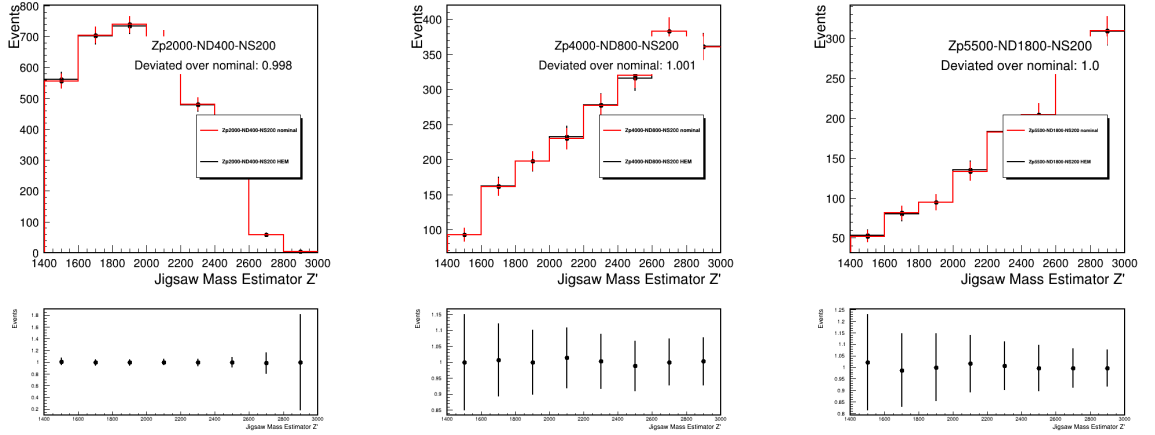
Figure 8.17: Observable signal distributions in the dimuon channel with the HEM scaling applied. Entire sample scaled, so any deviations over-estimate their expected value. Deviations are negligible, especially once combined with 2016 and 2017, as is done.
