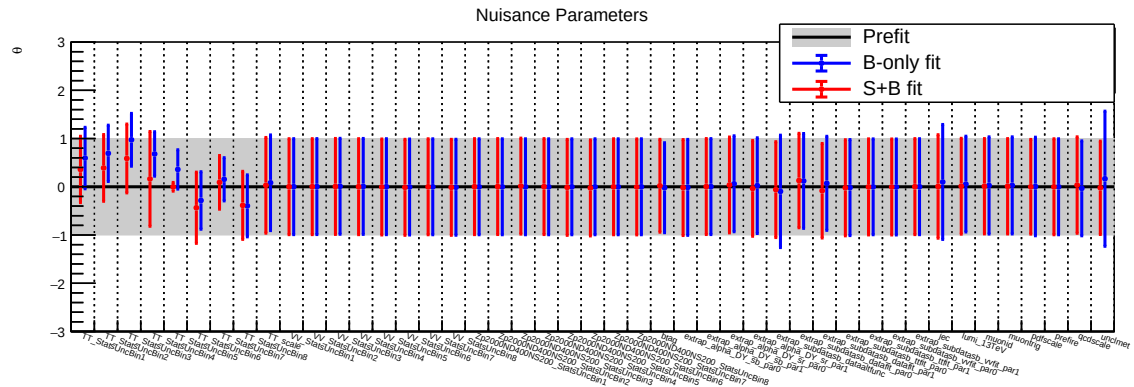
Figure 9.8: Nuisance parameter pulls for fits to 500 toys with an expected signal strength equal to the median expected limit for mass point m_{Z'} 2000 m_{N_D} 400 m_{N_S} 200 GeV. Pre-Fit line indicates the bare nuisance parameter value, not a pull.
