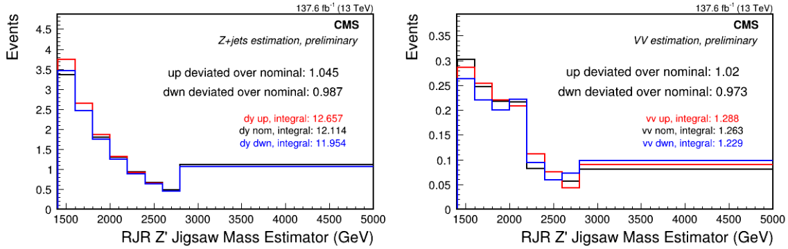
Figure 8.9: Plots showing the application of the up/down systematic uncertainties for the JES. The left plot is Z + jets with the full \alpha -method applied, and the plot is the diboson MC.
