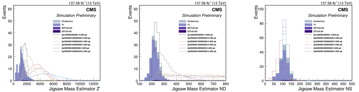
Figure 6.16: The soft drop mass signal region plots at preselection featuring the RJR mass estimator spectra. Preselections are described in Section 6.5. The plots are in units of GeV. The normalization for Drell-Yan MC derived in Section 7.2.1 is applied, but otherwise the filled histograms are nominal simulation.
