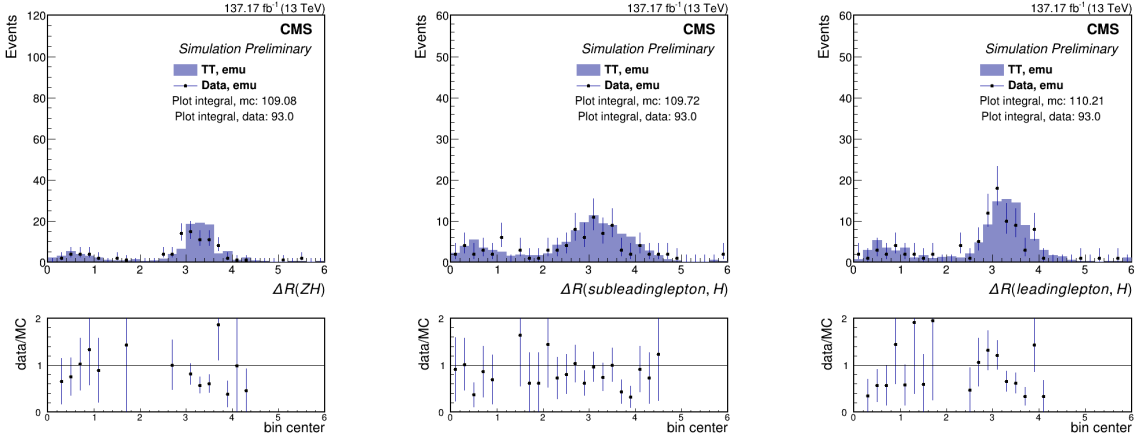
Figure B.9: Z to e\mu at preselection in the jet mass signal region \Delta R plots for Higgs candidate jet and Z constituents.
