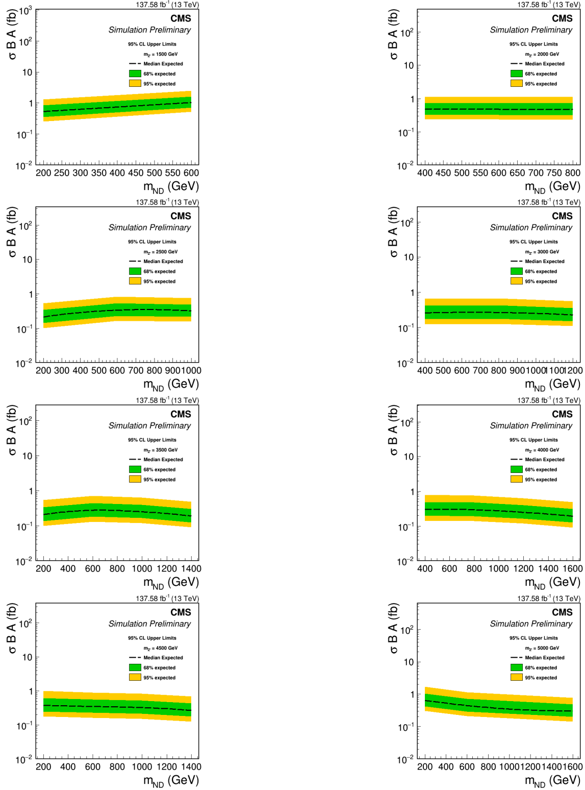
Figure 9.21: Asymptotic fiducial cross section upper limits for 2016-2018 as a function of m_{ND} for fixed values of m_{Z'} for the m_{N_S} = 1 GeV scenario. Limits shown in fb.
