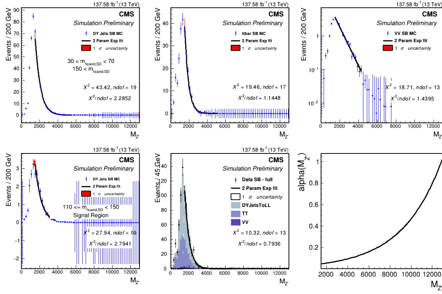
Figure 7.9: Distributions used in \alpha -method background estimation. The lower range of the fitted region implies a final cut at 1400. The red bands are the fit uncertainties. Top Left: Sideband Drell-Yan + jets MC RJR Z' mass estimator distribution. Top Middle: RJR mass estimator sideband of t\bar{t} . Top Right: WZ and ZZ sideband RJR mass estimator. Bottom Left: Signal region Drell-Yan + jets MC RJR mass estimator distribution. Bottom Right: \alpha ratio formed from the ratio of the fits in the bottom left and top left plots. Bottom Middle: Data sideband and fit.
