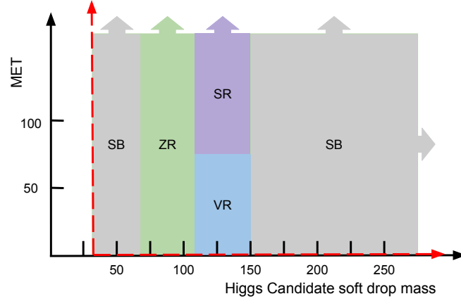
Figure 7.6: Illustration of regions used in the \alpha -method. All considered regions have a fat jet with p_T > 300.0 GeV and a DeepAK8 working point > 0.8 , the Z candidate p_T > 100.0 GeV, and an |\eta| < 2.4 . The SR label indicates the signal region, SB the sideband, VR the validation region, and ZR the blinded region around Z peak.
