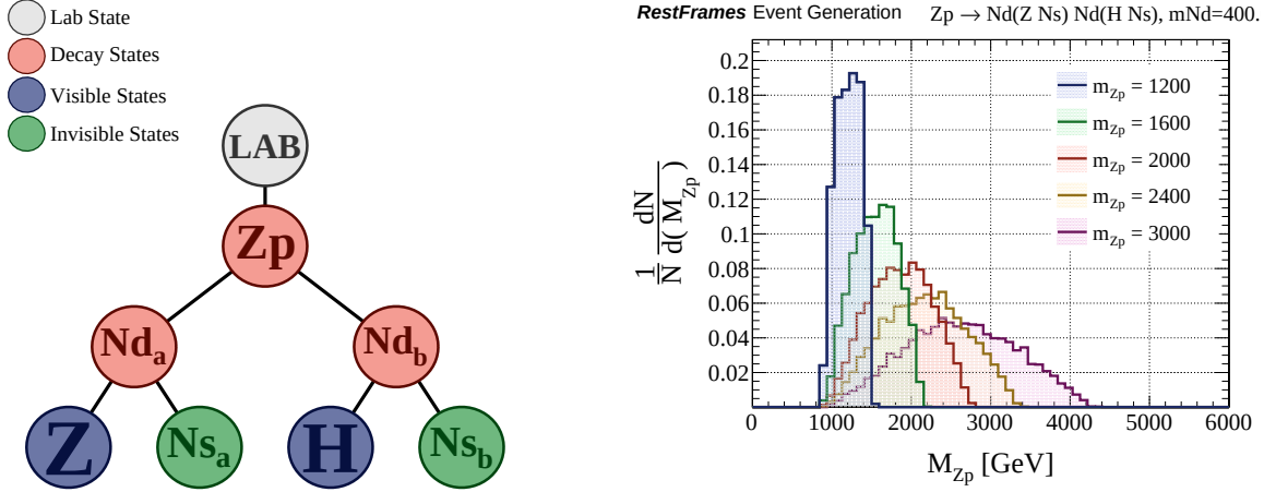
Figure 6.4: Overview of recursive jigsaw reconstruction. The left image shows the decay tree and rest frames for the reconstruction analysis. Example of correlation between mass estimator and input m_{Z'} for various working points (arbitrary normalization).
