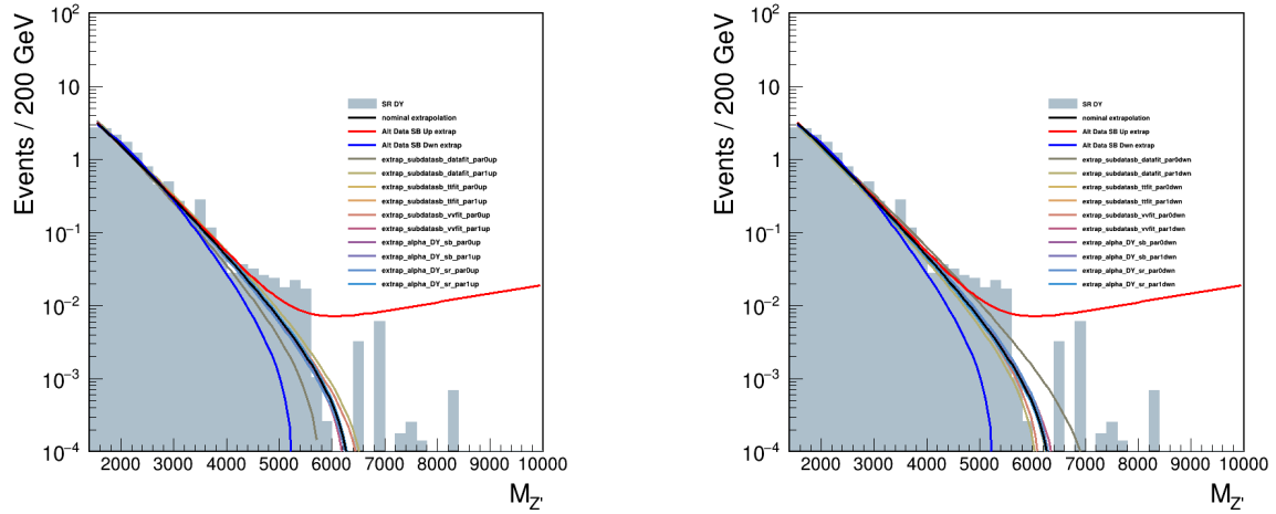
Figure 8.8: Shifted extrapolations with log scale and extended range. Same as the right-most plots in Figs. 8.5 and 8.6, but with extended range and logarithmic scale.
