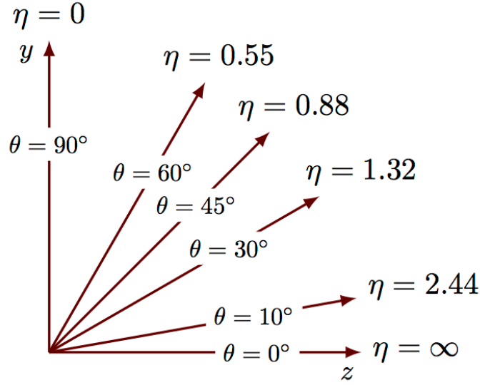
Figure 3.4: A diagram of the relationship between \eta and \theta . Pseudorapidity values mirrored across the z -axis are negative.[50]
