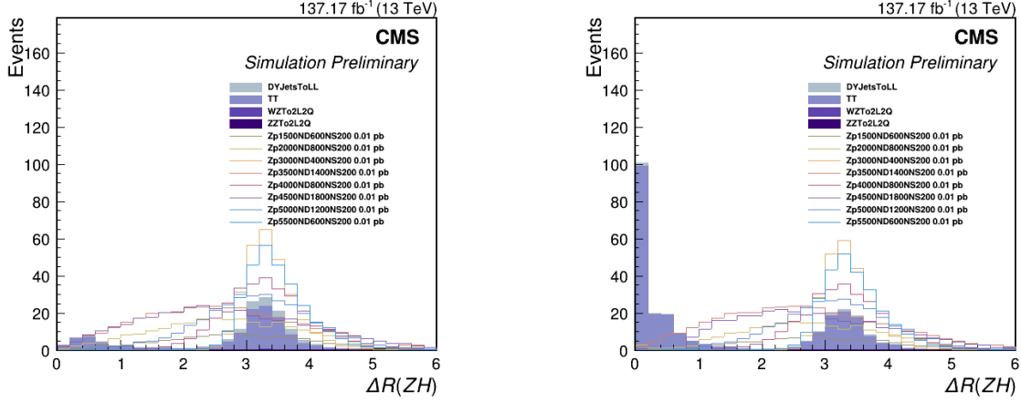
Figure 6.9: \Delta R distribution between the Z candidate and H candidate at preselection in the H channel signal region for a few benchmark signal mass distributions. Scaled to full Run 2 luminosity, and a cross section of 10 \text{ fb}^{-1} . Left figure is reclustered. Right figure is not reclustered.
