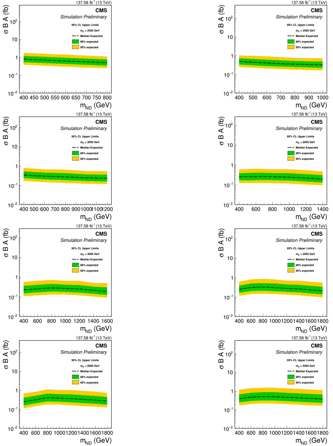
Figure 9.20: Asymptotic fiducial cross section upper limits for 2016-2018 as a function of m_{N_D} for fixed values of m_{Z'} for the m_{N_S} = 200 GeV scenario. Limits shown in fb.
