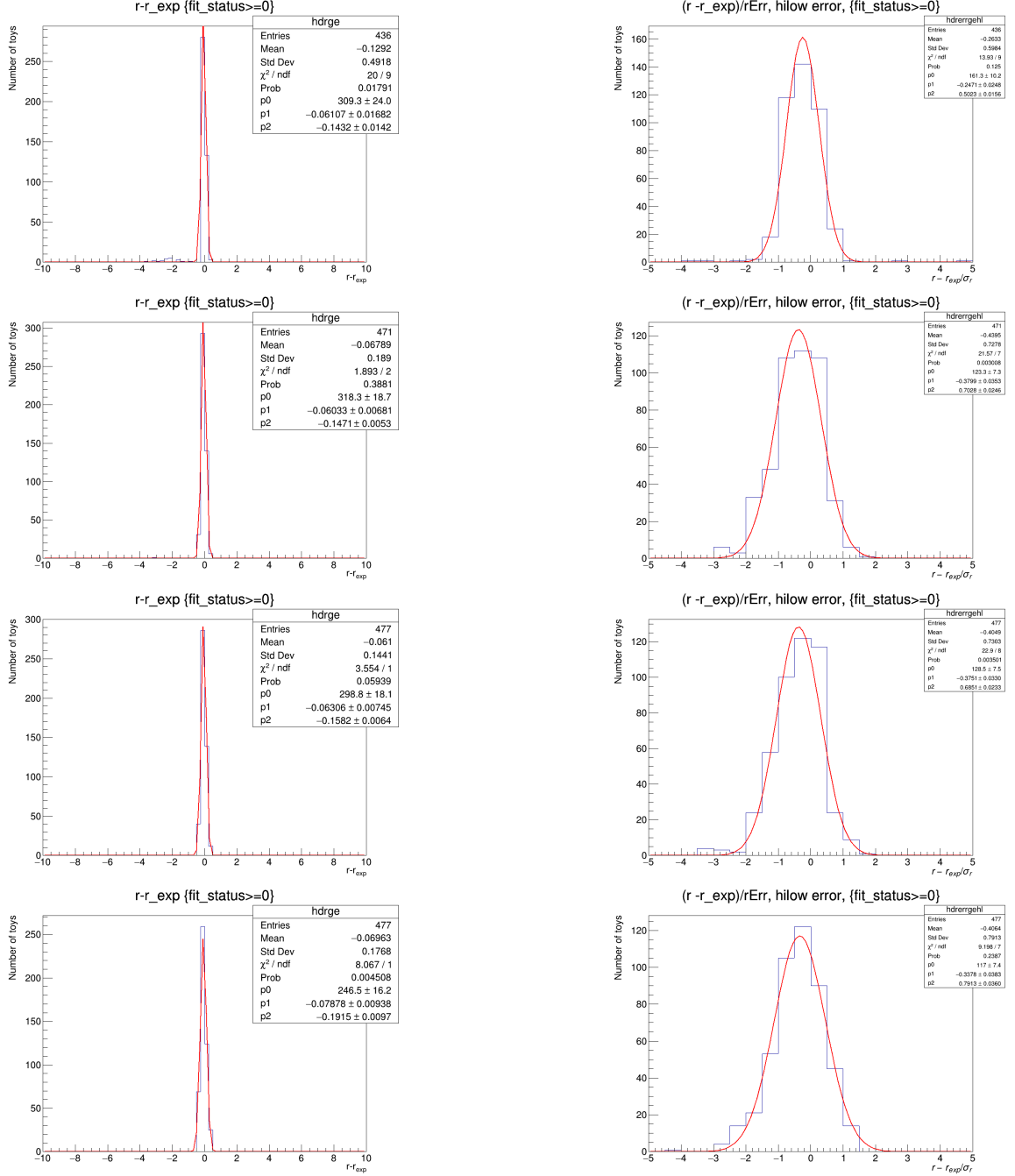
Figure 9.16: Differences (left) and pulls (right) for the measured and expected signal strengths for m_{Z'} = 4000 , m_{N_D} = 800 , m_{N_S} = 200 . First row has an injected signal of 0, the second has the lower expected limit, the third the median expected limit, and the final the upper expected limit.
