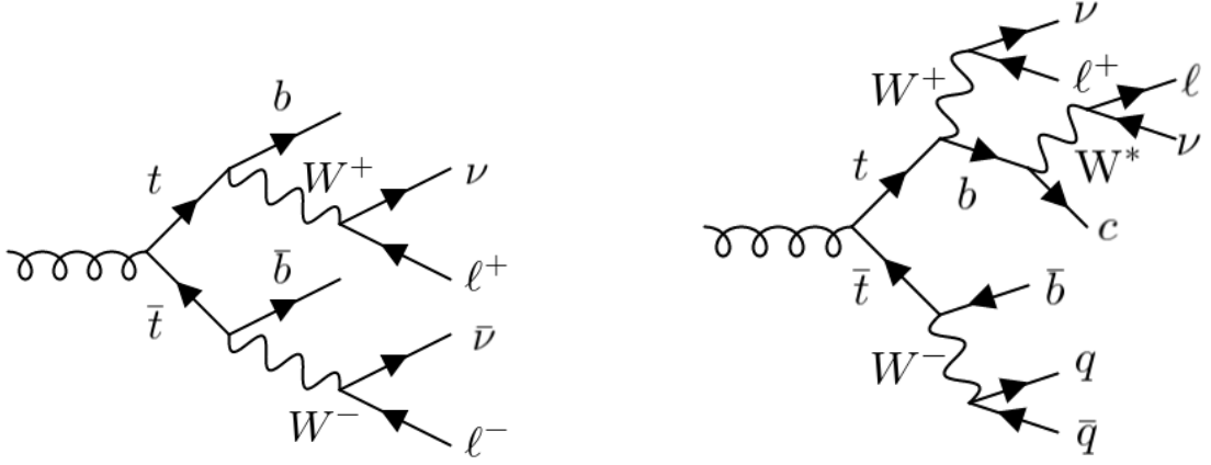
Figure 7.1: Illustrative Feynman diagrams of leptonic (left) and semileptonic (right) t\bar{t} decay channels. In the leptonic-case, the two leptons from the leptonic W decay fake the Z candidate and the two b -jets merge to fake the Higgs candidate jet. In the semileptonic case, a lepton from the leptonic W fakes one of the leptons in the Z candidate, but the second lepton comes from the decay of the b -quark via a virtual W boson. The hadronic top produces the fat jet candidate.
