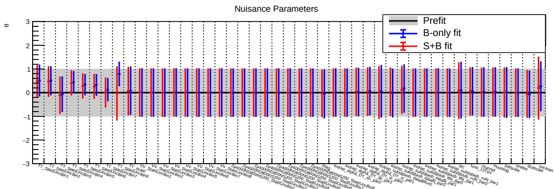
Figure 9.9: Nuisance parameter pulls for fits to 500 toys with an expected signal strength of 0 for mass point m_{Z'} 4000 m_{N_D} 800 m_{N_S} 200 GeV. Pre-Fit line indicates the bare nuisance parameter value, not a pull.
