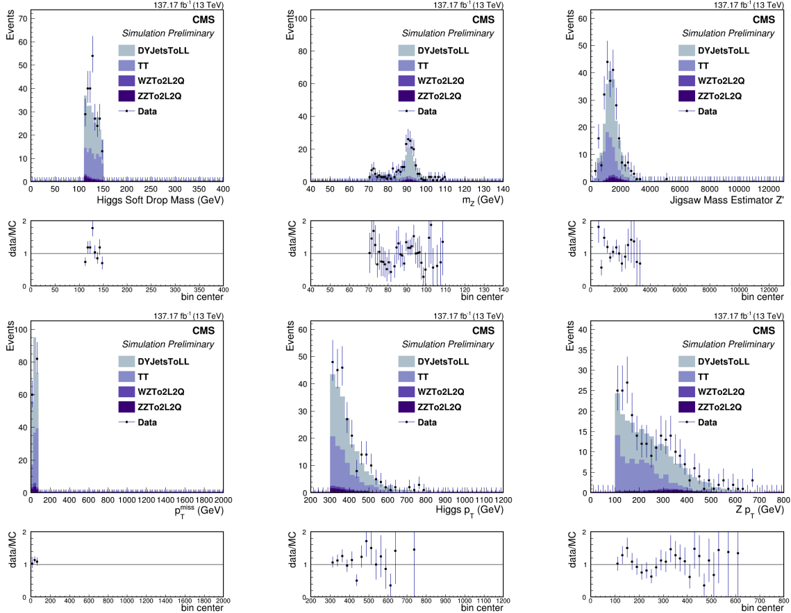
Figure C.1: Additional closure plots in the validation region. Same selection as preselection signal region except the p_T^{\text{miss}} cut is reversed.
