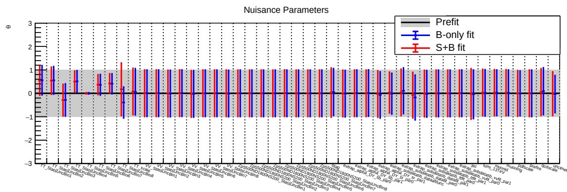
Figure 9.11: Nuisance parameter pulls for fits to 500 toys with an expected signal strength equal to the median expected limit for mass point m_{Z'} = 5500 m_{N_D} 1800 m_{N_S} 200 GeV. Pre-Fit line indicates the bare nuisance parameter value, not a pull.
