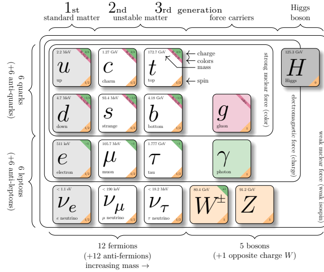
Figure 2.1: Summary of the SM particles and their properties. [5, 6, 7]
