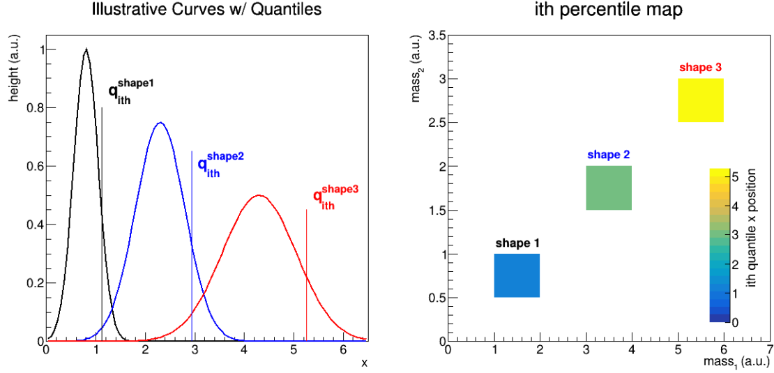
Figure 9.5: Cartoon of the relationship between the q_{ith} quantiles and the plane in mass_1 mass_2 -plane used to interpolate the quantile position for new mass points. In the figure, mass_1 and mass_2 are arbitrary stand-ins for m_{Z'} and m_{N_S} in our signal model.
