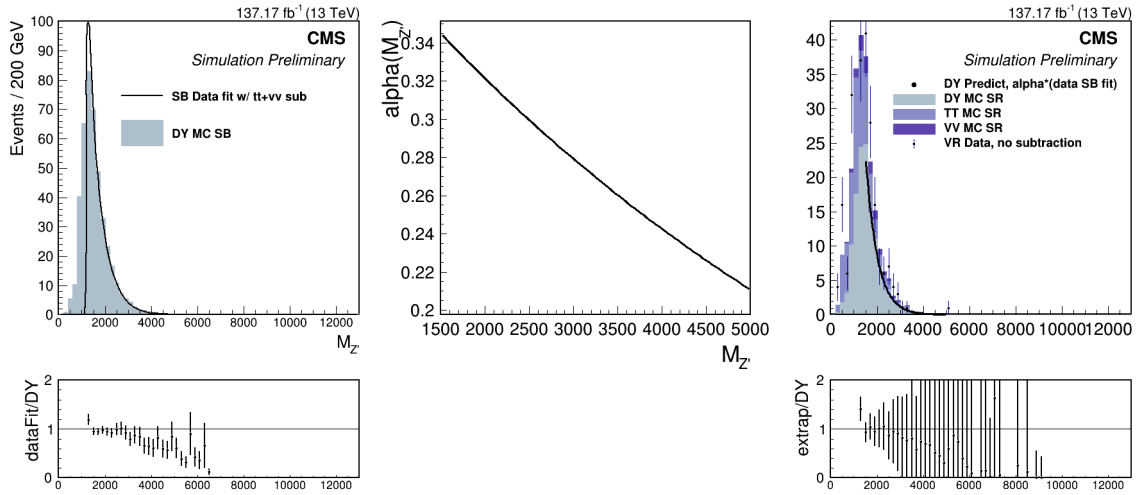
Figure 7.14: Plots showing the application of the \alpha -method in the validation region. The left plot shows the fit to the sideband data with the t\bar{t} and VV components subtracted. The middle plot is the \alpha ratio between the sidebands and the validation region. The right plot is the estimation of the Z + \text{jets} contribution in the validation region through the multiplication of the functions in the two plots to the left. MC included to guide the eye. Perfect agreement between data and MC is not expected in this data-driven background.
