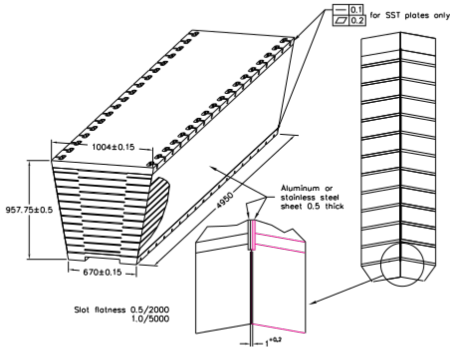
Figure 4.2: A diagram of an HCAL Barrel wedge to show staggered layers [44].
