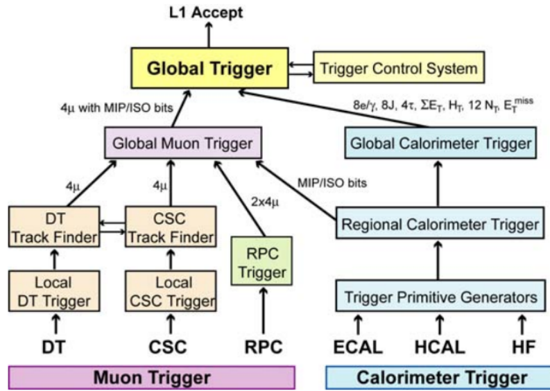
Figure 3.12: Diagram of flow of L1 trigger.[44].
