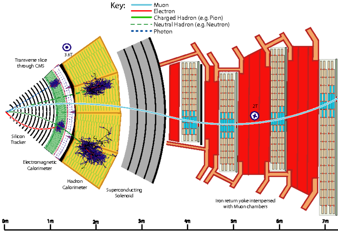
Figure 5.1: Transverse section of CMS illustrating locations of different particle interactions. [63]
