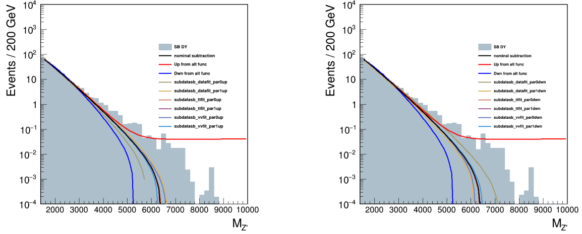
Figure 8.7: Subtracted sideband distributions. Same as the middle plots in Figs. 8.5 and 8.6, but with extended range and logarithmic scale.
