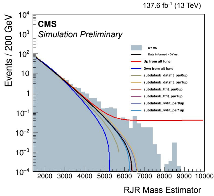
Figure 7.11: The subtracted data sideband distribution. The black line represents the Z + \text{jets} contribution in the data sideband. This plot is the difference between the data sideband fit, and the t\bar{t} and VV fits. Uncertainty bands are discussed in Chapter 8.
