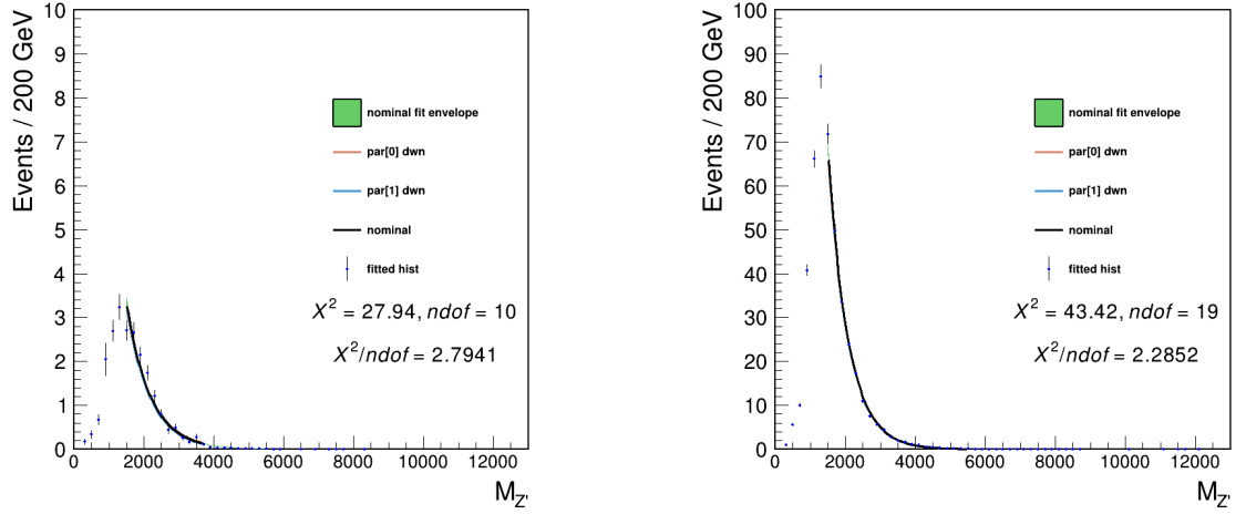
Figure 8.2: Left: Drell-Yan signal region fits for full Run 2. Each additional fit represents the fit result with the labeled parameter shifted down in the decorrelated space. Right: Same distributions but for the Drell-Yan sideband. These functions are used to build the \alpha ratio. The uncertainties are small, but are noticeable when propagated through the method.
