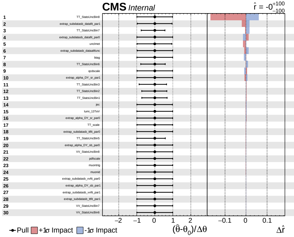
Figure 9.13: Impact of nuisance parameters for the background only hypothesis with a signal hypothesis of m_{Z'} 5500 GeV, m_{N_D} 1800 GeV, m_{N_S} 200 GeV. The \Delta r is the change in the extracted signal strength with respect to the nominal when the nuisance parameter is set to its \pm 1\sigma value and the fit repeated.
