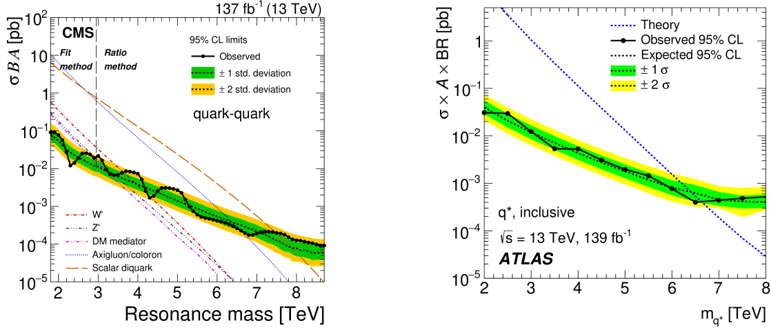
Figure 10.1: Left: Latest CMS Experiment narrow-resonance dijet limits [36]. Right: Latest ATLAS Experiment narrow-resonance dijet limits on excited quark q^* models [92]. Other signal interpretations have similar limits. These results can be interpreted to set limits on the hadronic channel of a leptophobic Z' .
