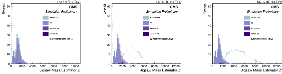
Figure 9.7: Signal region distributions for the example signal points used to test the statistical model.
