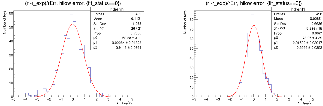
Figure D.2: Comparison between the unscaled (left) and scaled by 10 (right) pull distributions for the m_{Z'} = 4000 , m_{N_D} = 800 , m_{N_S} = 200 signal mass point at the median expected limit injected signal strength. Slight excess at negative pull values gone in the scaled version.
