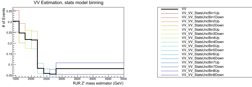
Figure 9.3: The diboson background estimation, taken from Monte Carlo.
