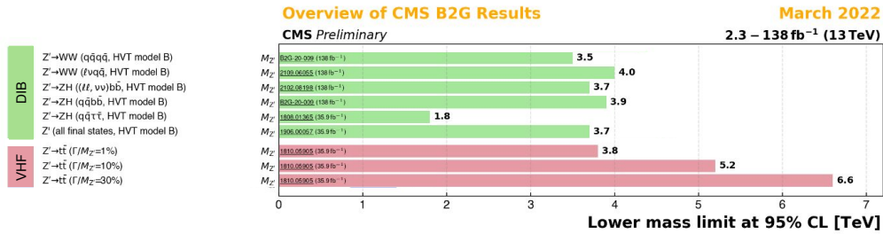
Figure 2.4: Summary of the Compact Muon Solenoid Experiment’s “Beyond Two (2) Generations” (B2G) physics analysis group 2016, 2017, and 2018 Z’ results [34]. The B2G group is a BSM search group in CMS that specializes in intermediate vector bosons in the final state.
