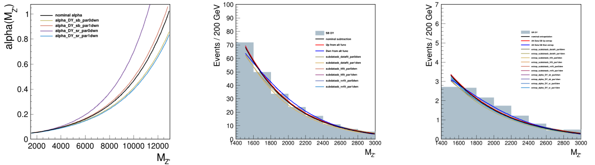
Figure 8.6: Left: Different \alpha ratio that are generated by varying one of the input function's parameters down . Middle: Different subtracted data sideband functions generated by varying one of the input function's parameters down . Right: The extrapolation to the signal region when one of the input parameters has been varied down . See Figs. 8.7 and 8.8 for larger range, logarithmic scale versions of the middle and right plots.
