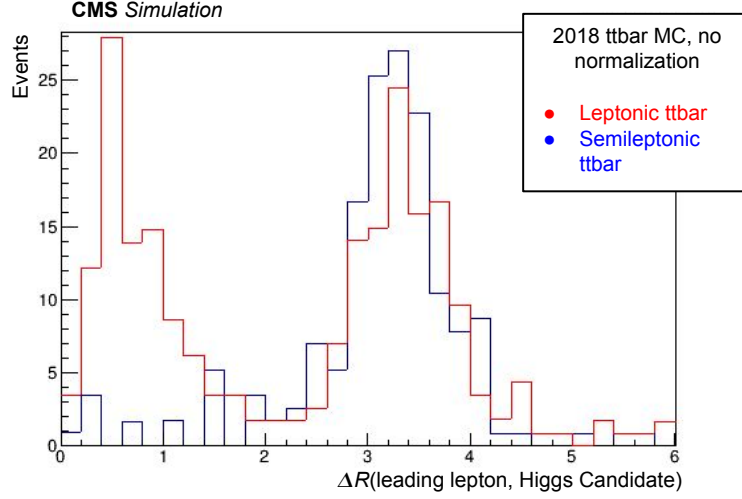
Figure 7.3: Distribution of \Delta R between the leading lepton in the e\mu fake “Z” candidate and the selected Higgs boson candidate fat jet. Semileptonic t\bar{t} is back-to-back, while leptonic t\bar{t} has events where the dilepton and the fat jet overlap.
