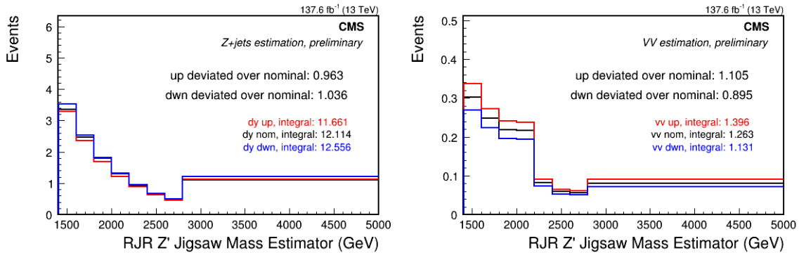
Figure 8.11: Plots showing the application of the up/down systematic uncertainties for b-tagging. The left plot is Z + jets with the full \alpha -method applied, and the plot is the diboson MC.
