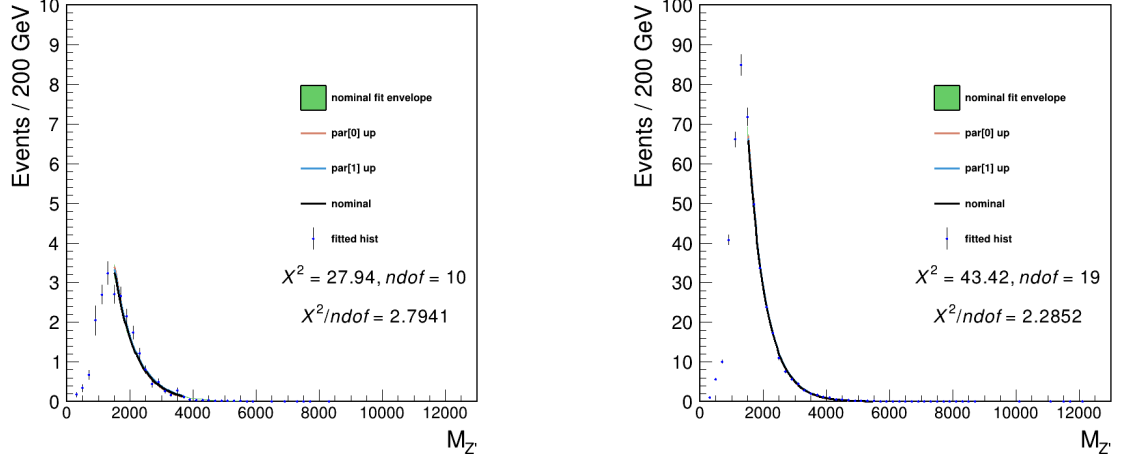
Figure 8.1: Left: Drell-Yan signal region fits for full Run 2. Each additional fit represents the fit result with the labeled parameter shifted up in the decorrelated space. Right: Same distributions but for the Drell-Yan sideband. These functions are used to build the \alpha ratio. The uncertainties are small, but are noticeable when propagated through the method.
