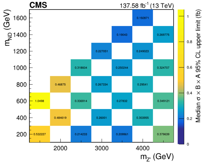
Figure 9.19: Asymptotic fiducial cross section upper limits for 2016-2018 are shown in the m_{N_D} and m_{Z'} plane for the m_{N_S} = 1 GeV scenario. Interpolated signals are not included. Limits shown in fb.
