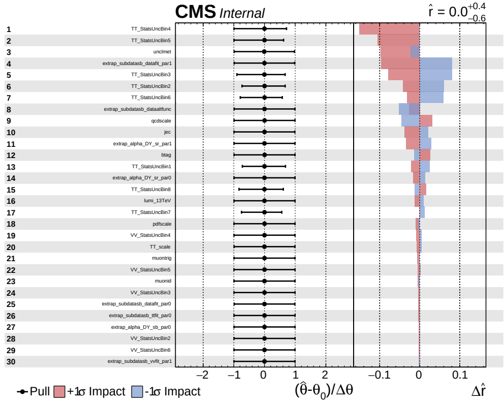
Figure 9.12: Impact of nuisance parameters for the background only hypothesis with a signal hypothesis of m_{Z'} 2000 \text{ GeV} , m_{N_D} 400 \text{ GeV} , m_{N_S} 200 \text{ GeV} . The \Delta r is the change in the extracted signal strength with respect to the nominal when the nuisance parameter is set to its \pm 1\sigma value and the fit repeated.
