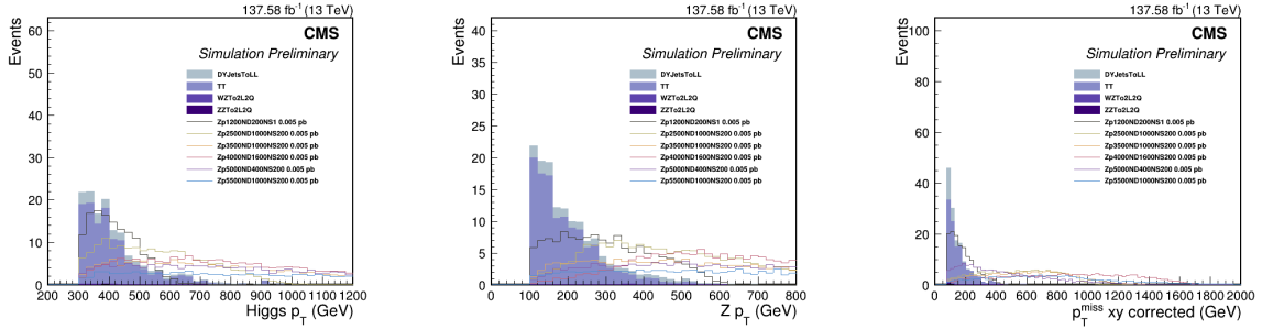
Figure 6.15: The soft drop mass signal region particle object p_T spectra. The normalization for Drell-Yan MC derived in Section 7.2.1 is applied, but otherwise the filled histograms are nominal simulation.
