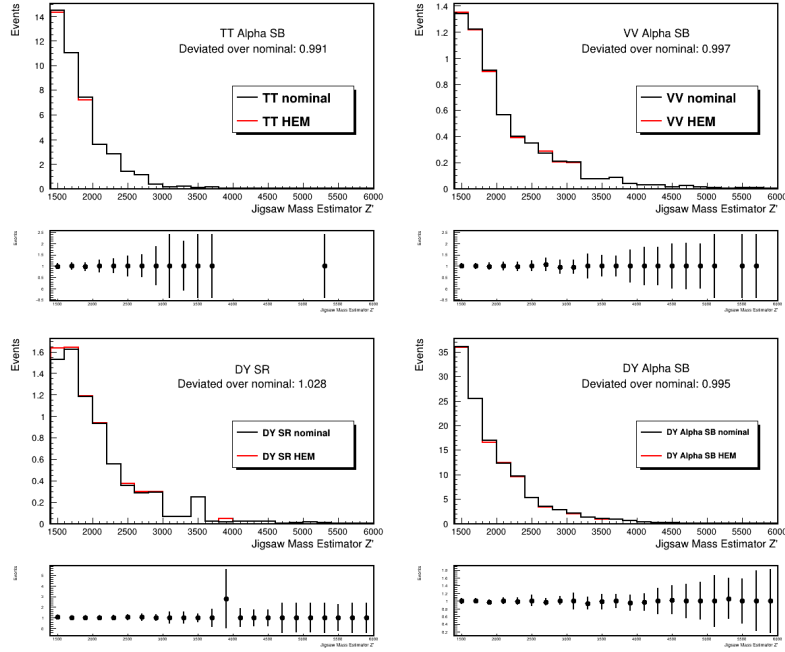
Figure 8.15: 2018 MC input distributions to the alpha method for the Z + \text{jets} estimation. Entire 2018 luminosity scaled, so any deviations over-estimate their expected value. Deviations are well within the fit uncertainties for the method, especially once combined with 2016 and 2017, as is done.
