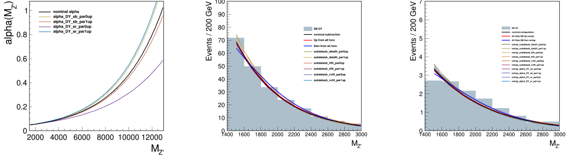
Figure 8.5: Left: Different \alpha ratio that are generated by varying one of the input function's parameters up . Middle: Different subtracted data sideband functions generated by varying one of the input function's parameters up . Right: The extrapolation to the signal region when one of the input parameters has been varied up . See Figs. 8.7 and 8.8 for larger range, logarithmic scale versions of the middle and right plots.
