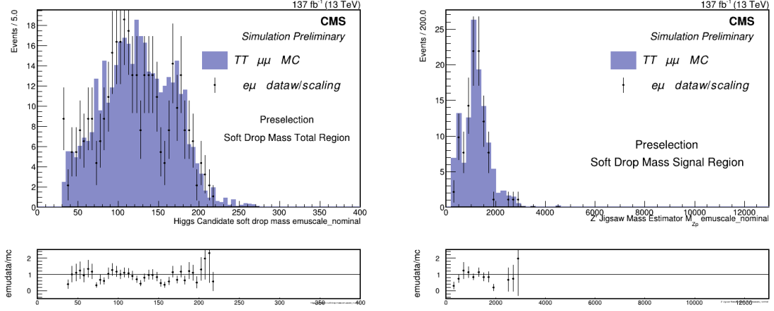
Figure 7.5: Overlays of the normalized e\mu extrapolation (data set with scaling) and the \mu\mu channel MC for preselection cuts. The plot on the left is the soft drop mass distribution. The right plot is the t\bar{t} background estimation for the recursive jigsaw mass estimator of the Z' in the soft drop mass signal region.
