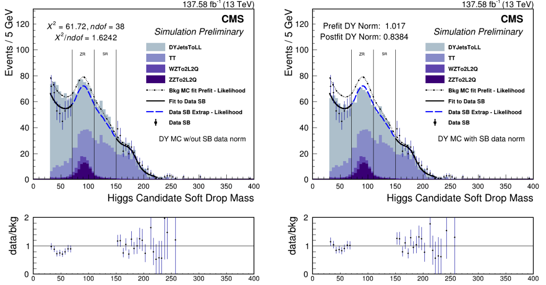
Figure 7.8: Stacked plots showing the full soft drop mass sideband fit. Left stack has the Z + \text{jets} plotted without the derived normalization, the right stack has the normalization applied. Both plots include the full background template fit to MC only, and the data sideband fit.
