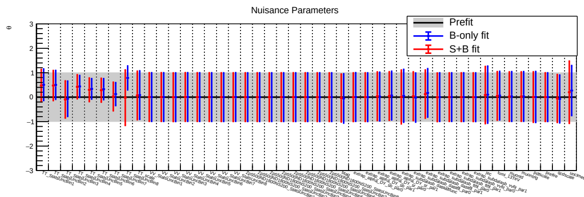
Figure 9.10: Nuisance parameter pulls for fits to 500 toys with an expected signal strength of 0 for mass point m_{Z'} \ 5500 \ m_{N_D} \ 1800 \ m_{N_S} \ 200 \text{ GeV} . Pre-Fit line indicates the bare nuisance parameter value, not a pull.
