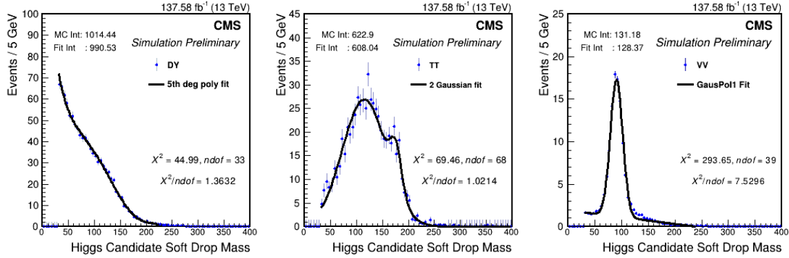
Figure 7.7: Individual backgrounds in the soft drop mass spectrum, and their respective fits. Distributions shown at preselection with the p_T^{\text{miss}} cut released, with no SR and SB separation.
