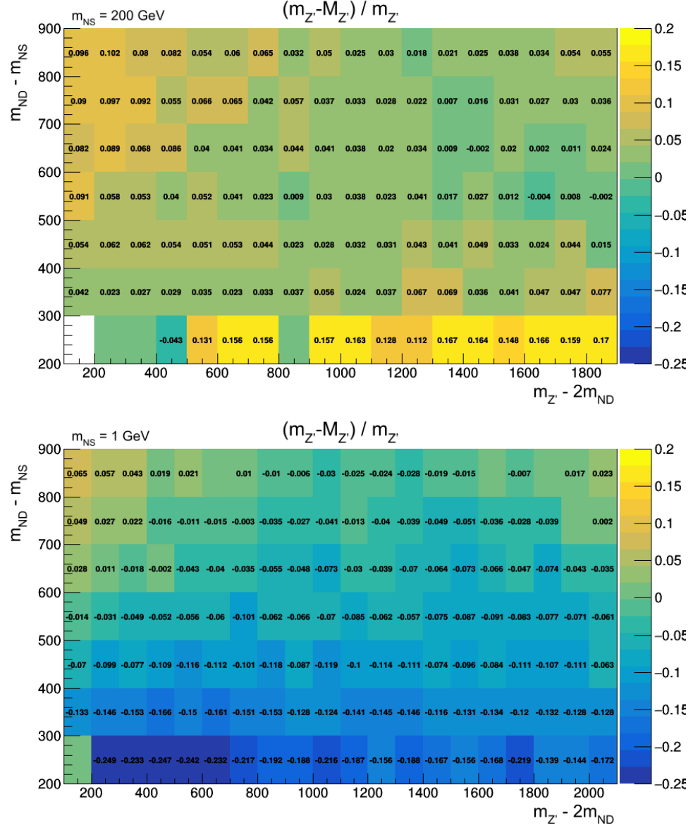
Figure 6.5: Accuracy of RJR Z' mass estimator ( M_{Z'} ) using the Recursive Jigsaw Reconstruction scenario JR V.1, JR VI.1, and JR VI.3, the Contra-Boost Invariant. The greener the better. The top plot is for a signal sample grid with a fixed m_{NS} of 200 GeV. The bottom is a signal sample grid with a fixed m_{NS} of 1 GeV.
