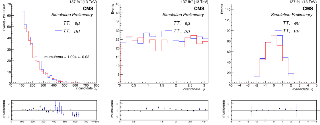
Figure 7.4: A comparison of the shapes of the t\bar{t} MC in the e\mu and \mu\mu channels, with the normalization scale between them. This yield is expected based on the relative inefficiency between muon and electron identification, and the make-up of our control region.
