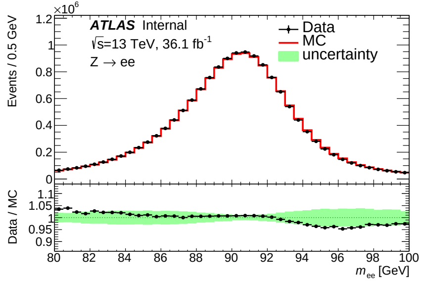
Fig. 3.7: Comparison of the invariant mass distribution of the two electrons in selected Z \rightarrow ee candidates, after the calibration and resolution corrections are applied. The total number of events in the simulation is normalized to the data. The ratio is shown in the bottom plot. The uncertainty band of the bottom plot corresponds to the impact of the uncertainties on the calibration and resolution correction factors. This plot is taken from Ref. [138].
