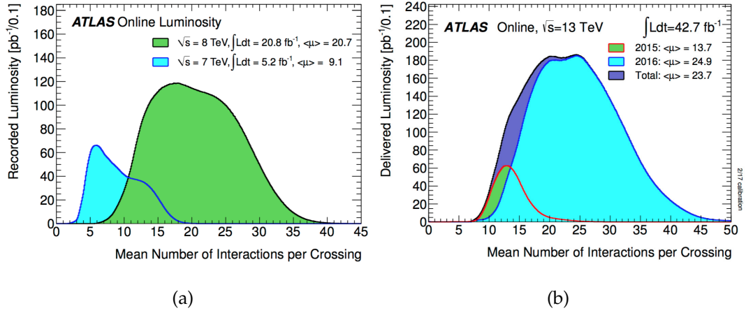
Fig. 2.4: Luminosity weighted distributions of the mean number of interactions per bunch crossing for (a) 2011-2012 and (b) 2015-2016 data taking, respectively.
