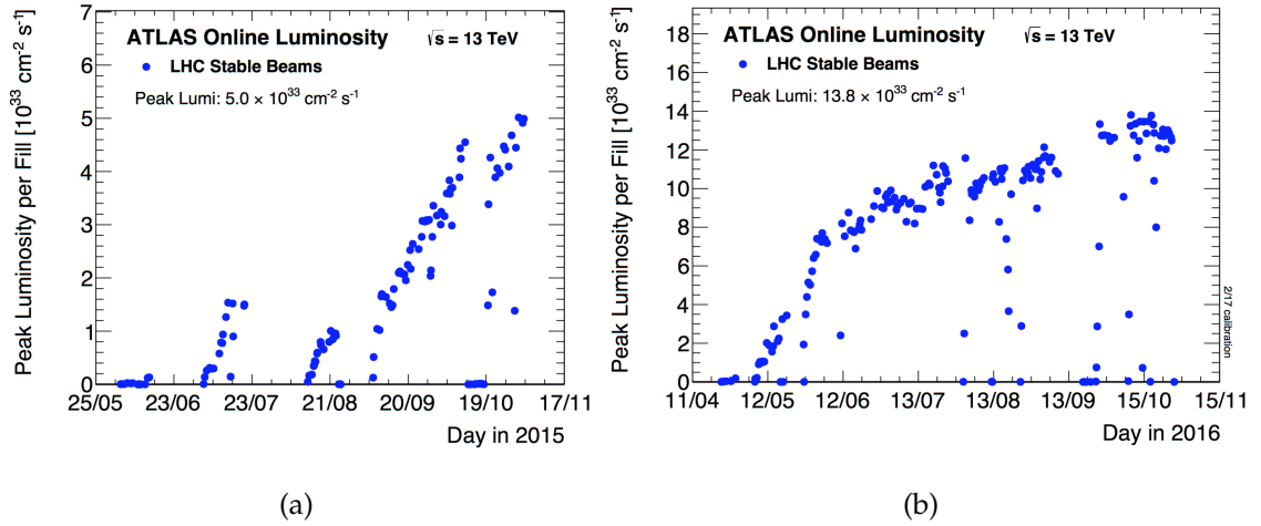
Fig. 2.5: Peak instantaneous luminosity delivered to ATLAS during stable beams for pp collisions at 13 TeV centre-of-mass energy for each LHC fill as a function of time in (a) 2015 and (b) 2016.
