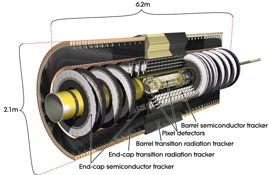
Fig. 2.12: A cut-away view of the ATLAS Inner Detector.
