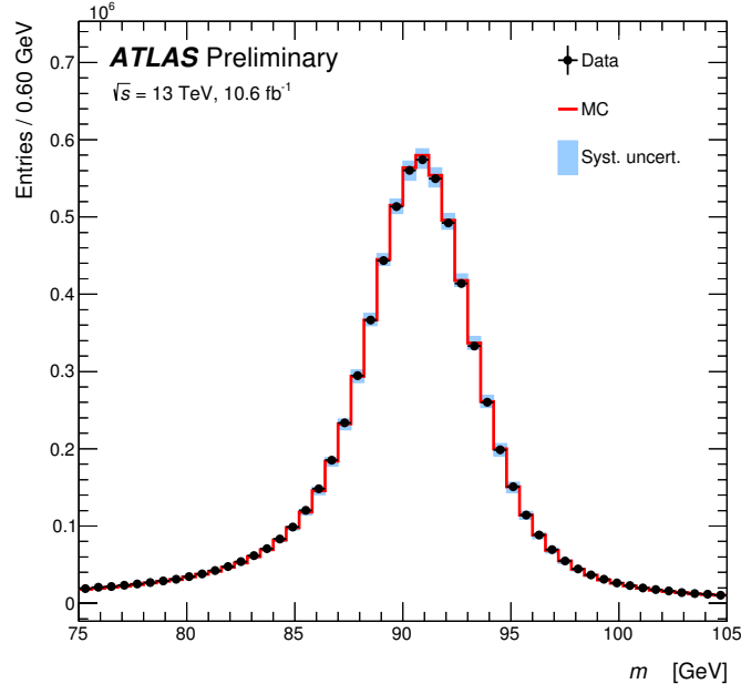
Fig. 3.2: Dimuon invariant mass distribution of Z \rightarrow \mu^+\mu^- events reconstructed with combined muons. The points show the data. The continuous line corresponds to the simulation with the momentum corrections applied. The band represents the effect of the systematic uncertainties on the momentum corrections. Simulations are normalised to data. The plot is taken from Ref. [128].
