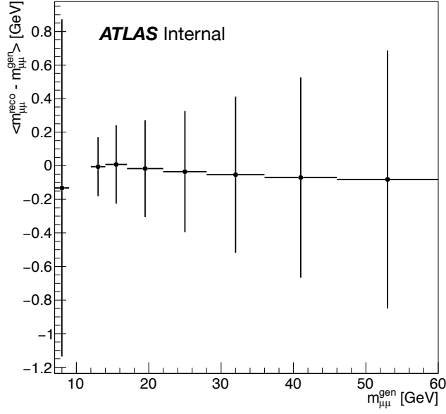
Fig. 6.46: Average ATLAS di-muon mass resolution as simulated by DY MC signal samples in the complete mass range 7 < m_{\mu\mu} < 60 GeV.
