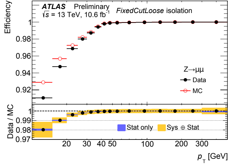
Fig. 3.4: Isolation efficiency for the FixedCutLoose muon isolation working points. The efficiency is shown as a function of the muon transverse momentum p_T and is measured in Z \rightarrow \mu^+\mu^- events. The full (empty) markers indicate the efficiency measured in data (MC) samples. The errors shown on the efficiency are statistical only. The bottom panel shows the ratio of the efficiency measured in data and simulation, as well as the statistical uncertainties and combination of statistical and systematic uncertainties. The plot is taken from Ref. [128].
