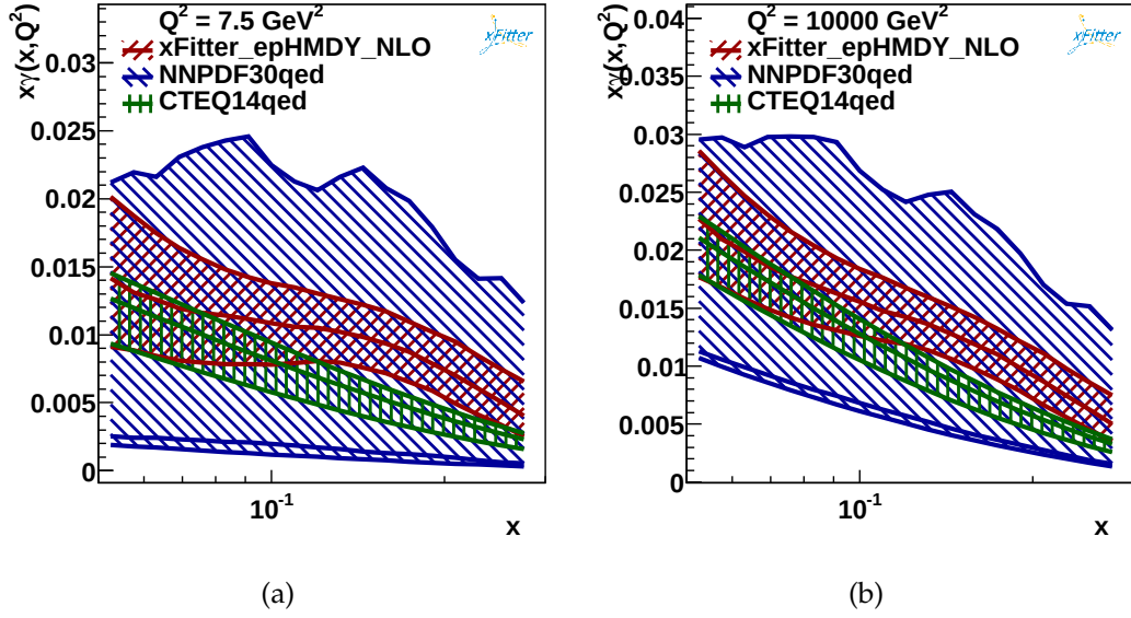
Fig. 4.11: Comparison between the NLO photon PDF distributions for the present analysis, NNPDF3.0QED, CT14qed (68% C.L.): (a) at scale 7.5 GeV 2 ; (b) at the evolved scale 10 4 GeV 2 .
