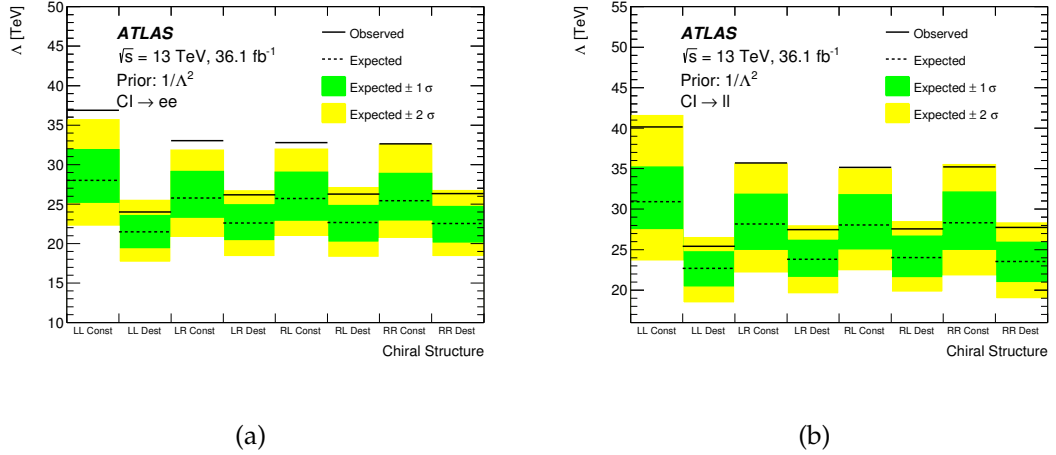
Fig. 5.12: Lower limits on the energy scale \Lambda at 95% C.L., for the CI model with constructive ('Const' in the labels on the x-axis) and destructive ('Dest' in the labels on the x-axis) interference (for all considered helicities). Results are shown for the (a) di-electron and (b) di-lepton channels.
