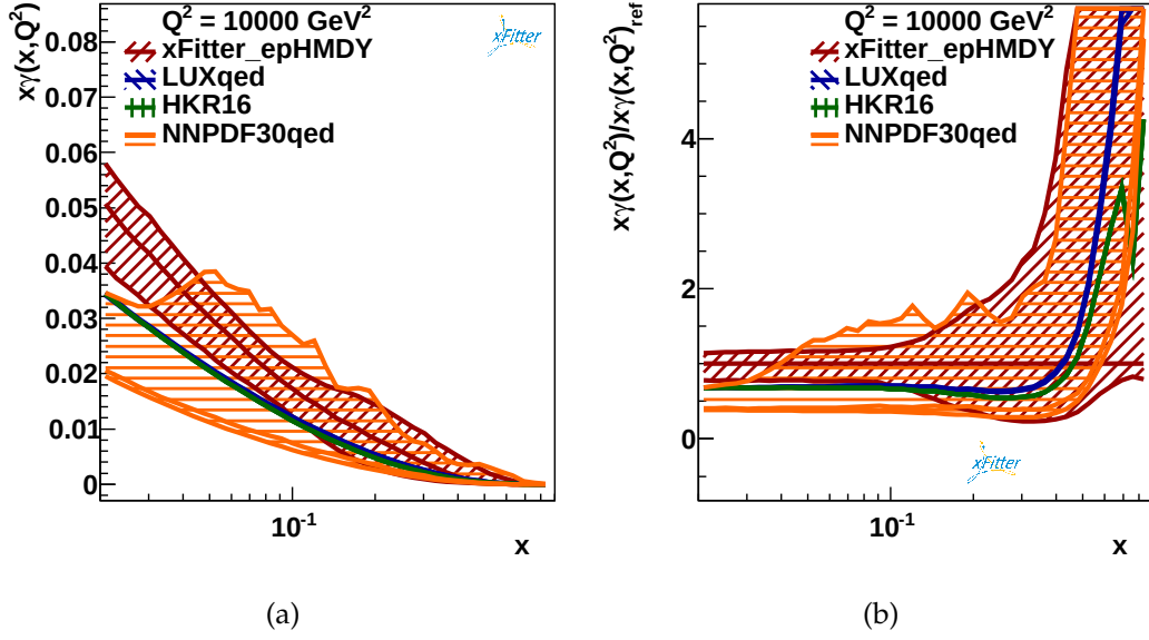
Fig. 4.10: (a) Comparison between the photon x\gamma(x, Q^2) at Q^2 = 10^4 \text{ GeV}^2 from the present NNLO analysis ( \text{xFitter\_epHMDY} ) with the corresponding results from NNPDF3.0QED, LUXqed and HKR16; (b) the same comparison, now with the results normalized to the central value of \text{xFitter\_epHMDY} . For the present fit, the PDF uncertainties are shown at the 68% CL obtained from the MC method, while model and parametrisation uncertainties are discussed below. For HKR16 only the central value is shown, while for LUXqed the associated PDF uncertainty band [52] is included.
