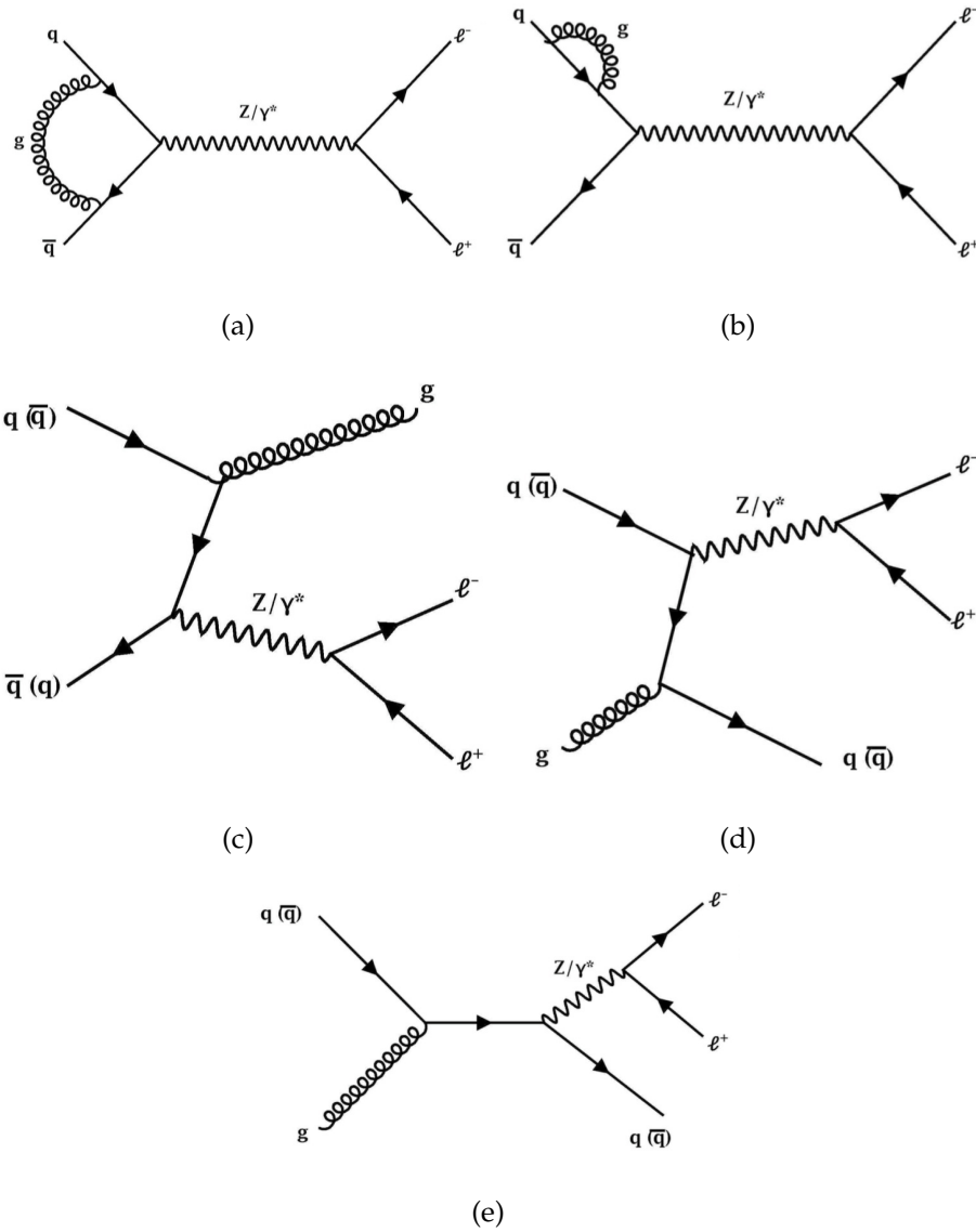
Fig. 1.8: NLO contributions to the Drell-Yan process.
