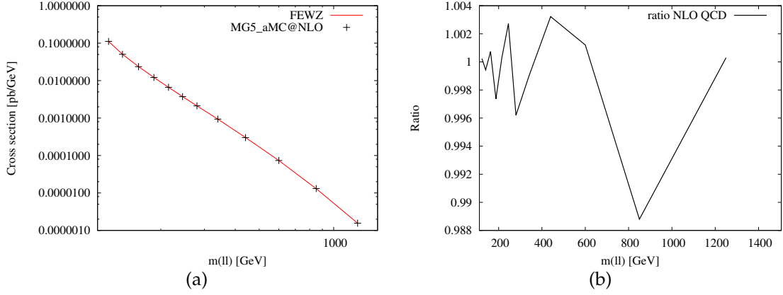
Fig. 4.2: (a) Comparison regarding the cross section as a function of the invariant mass of the lepton pair between NLO QCD + LO EW predictions evaluated with MG5_aMC@NLO interfaced with APPLgrid and aMCfast (black marker) and the ones computed with FEWZ (red solid line); (b) ratio between the two different predictions.
