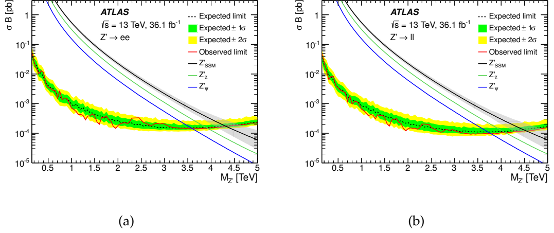
Fig. 5.11: Upper 95% C.L. limits for Z' production cross section times branching ratio to two leptons as a function of Z' pole mass ( M_{Z'} ). The signal theory lines are calculated with Pythia8 using the NNPDF23LO PDF set and corrected to NNLO in QCD using VRAP and the CT14NNLO PDF set. The signal theoretical uncertainties are shown as a band on the Z'_{SSM} theory line. Shown are results for: (a) the di-electron channel; (b) the combined channel ( ee, \mu\mu ).
