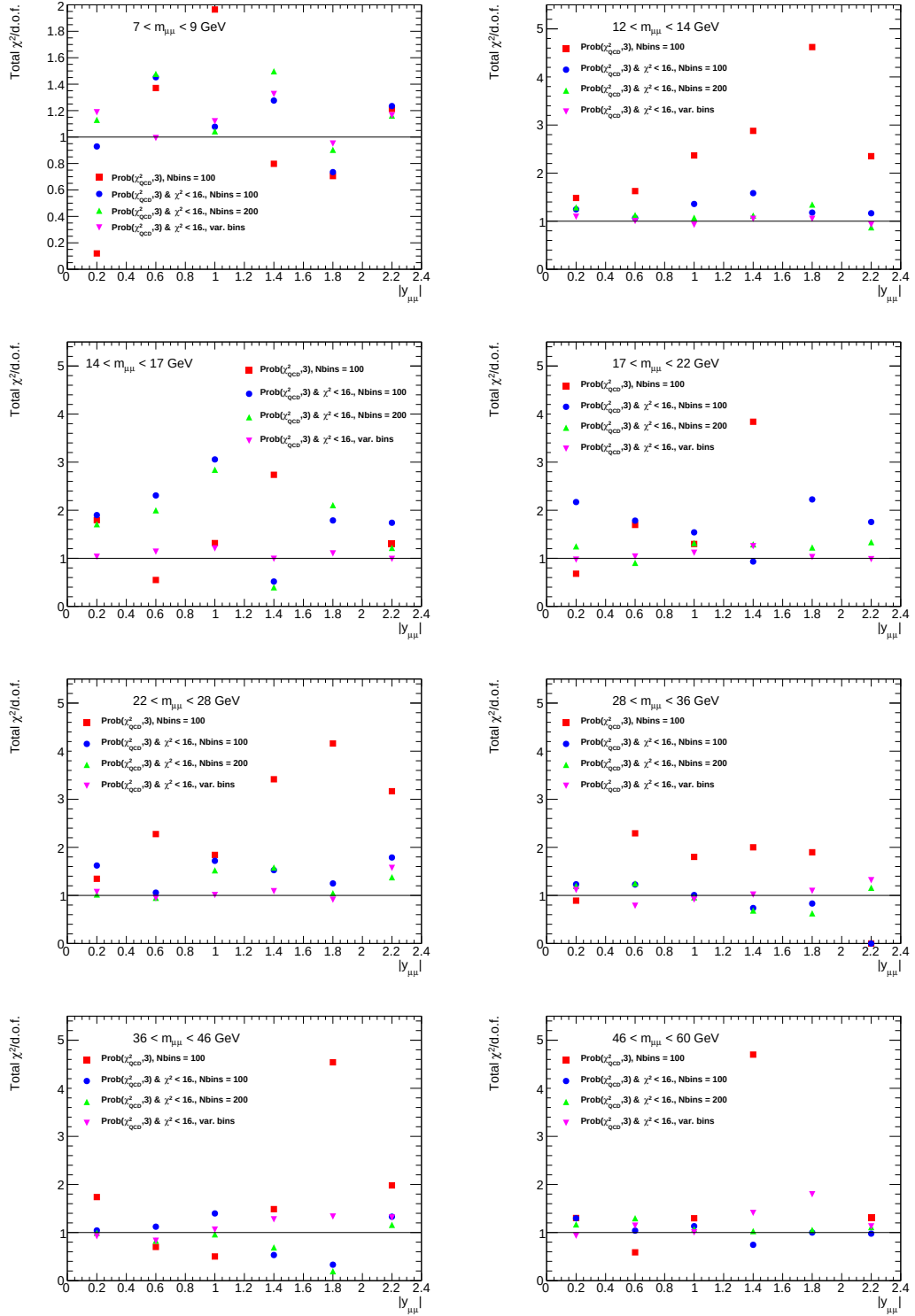
Fig. 6.31: Comparison between the \chi^2/\text{n.d.f.} obtained using: \text{Prob}(\chi^2_{\text{QCD}}, \text{n.d.f.} = 3) and 100 bins (red squares); \text{Prob}(\chi^2_{\text{QCD}}, \text{n.d.f.} = 3) , \chi^2_{\text{QCD}} < 16 and 100 bins (blue circles); \text{Prob}(\chi^2_{\text{QCD}}, \text{n.d.f.} = 3) , \chi^2_{\text{QCD}} < 16 and 200 bins (green triangles); \text{Prob}(\chi^2_{\text{QCD}}, \text{n.d.f.} = 3) , \chi^2_{\text{QCD}} < 16 and bins with variable widths (magenta triangles).
