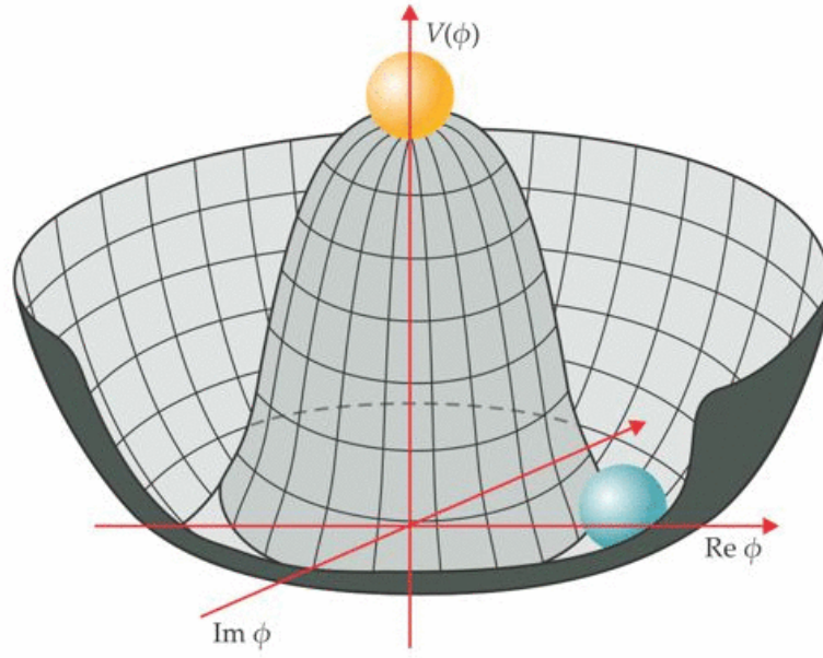
Fig. 1.1: Higgs potential V(\Phi) in the Re(\phi) , Im(\phi) plane.
