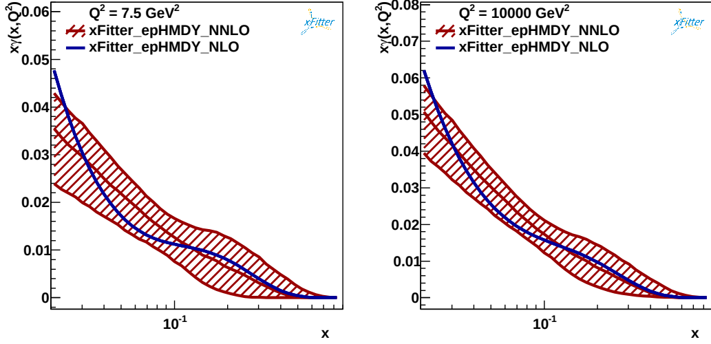
Fig. 4.15: Left plot: comparison between the reference \text{xFitter\_epHMDY} fit of x\gamma(x, Q^2) , based on NNLO QCD and NLO QED theoretical calculations, with the central value of the corresponding fit based on NLO QCD and QED theory, at Q^2 = 7.5 \text{ GeV}^2 . In the former case, only the experimental MC PDF uncertainties are shown. Right plot: same comparison, now presented at the higher scale of Q^2 = 10^4 \text{ GeV}^2 .
