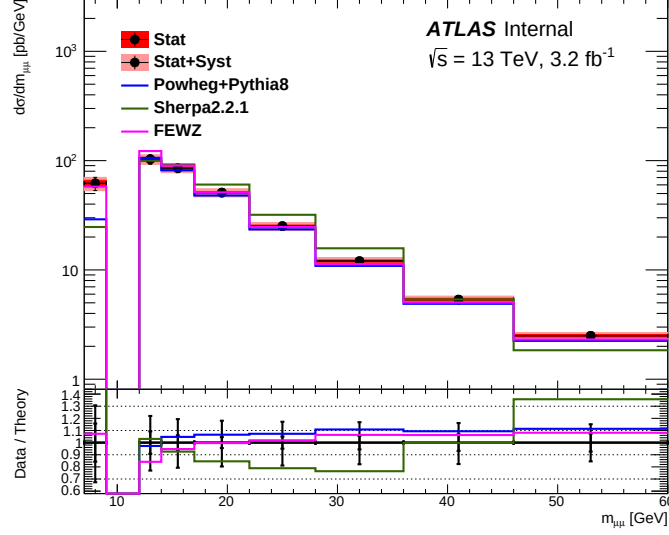
Fig. 6.51: Measured fiducial lmDY single-differential cross sections d\sigma/dm_{\mu\mu} , defined in Eq. 6.12. The inner band represents the statistical uncertainty, while the outer band represents the sum in quadrature of statistical and systematic uncertainties, as described in Sec. 6.4.4. The solid blue line shows the theoretical predictions from Powheg+Pythia, while the predictions from Sherpa are plotted with a solid green line. NNLO QCD + NLO EW predictions computed with FEWZ are represented by a magenta solid line. The ratios of all two theoretical predictions (solid lines) to the data are shown in the lower panels. The data (solid points) are displayed at unity with the statistical (inner) and total (outer) measurement uncertainties. The discrepancy observed in the 7-9 GeV bin for Powheg+Pythia and Sherpa predictions is probably due to the breakdown of the theory predictions, given that the considered phase space is very tiny and close to the cut imposed on the lepton p_T . In addition to that, the invariant mass range covered in the first bin probes the very high- p_T tail and it could be that NLO MC predictions do not reproduce kinematic distributions so well, taking into account that the p_T of the di-muon system is much more greater than the invariant mass in this region.
