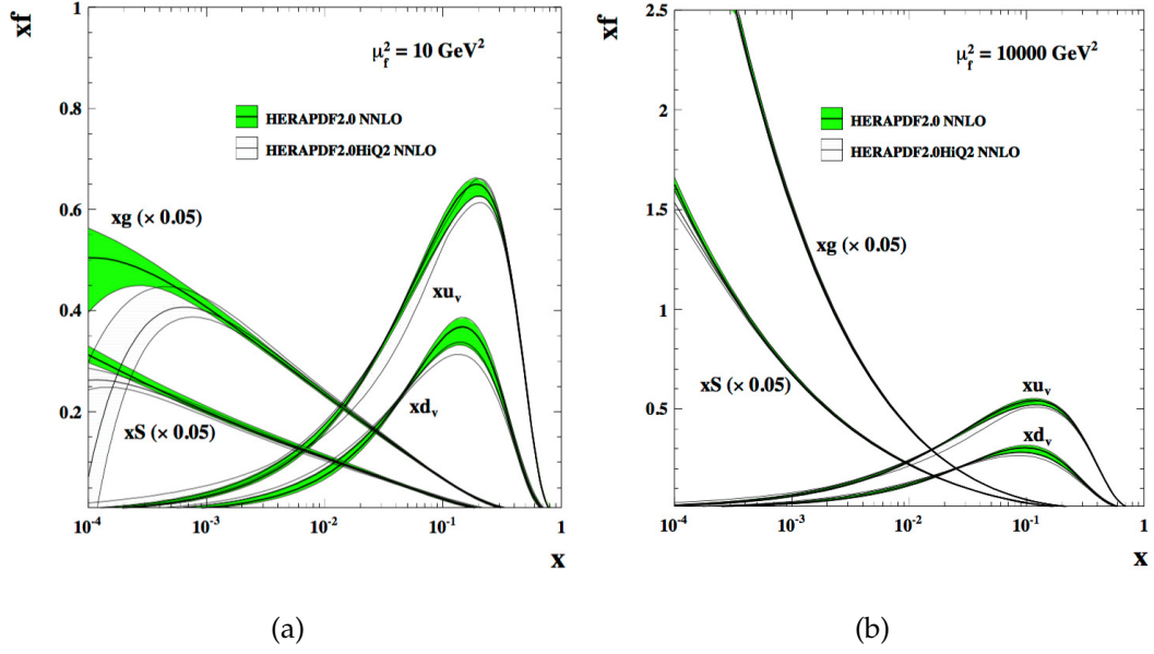
Fig. 1.5: PDFs for quarks, anti-quarks and gluons for energy scale Q^2 = 10 \text{ GeV}^2 (a) and Q^2 = 10^4 \text{ GeV}^2 (b). The distributions are determined from the H1 and ZEUS Collaborations from global fits to data [34].
