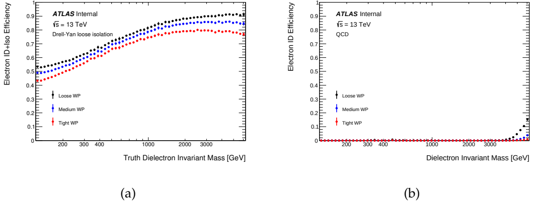
Fig. 5.5: Full selection efficiency for various working points as applied to (a) DY MC as a function of di-lepton truth mass. The same study is performed for (b) di-jet MC as a function of di-lepton reconstructed mass.
