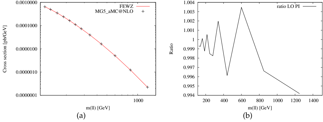
Fig. 4.4: (a) Comparison regarding the cross section as a function of the invariant mass of the lepton pair between LO PI predictions evaluated with MG5_aMC@NLO interfaced with APPLgrids and aMCfast (black marker) and the ones computed with FEWZ (red solid line); (b) ratio between the two different predictions.
