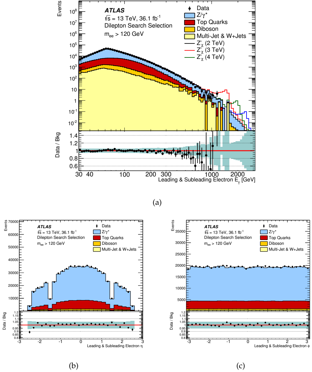
Fig. 5.7: Reconstructed electron (a) E_T (or p_T ), (b) \eta and (c) \phi after selection. "Leading" denotes the electron with the highest E_T ( p_T ) of the selected pair, while "Sub-leading" denotes the second electron. The distributions are shown for di-electron invariant masses greater than 120 GeV. Data and the SM background estimates as well as their ratio are displayed. The shaded band in the lower panel illustrates the total systematic uncertainty, as explained in Section 5.6. The data points are shown together with their statistical uncertainty and the MC expectation is normalised to the expected integrated luminosity.
