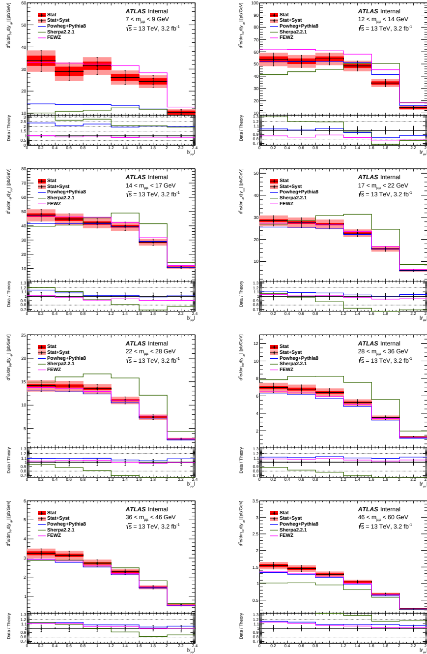
Fig. 6.50: Measured fiducial \text{lmDY} double-differential cross sections d^2\sigma/dm_{\mu\mu}d|y_{\mu\mu}| , defined in Eq. 6.13. The inner band represents the statistical uncertainty, while the outer band represents the sum in quadrature of statistical and systematic uncertainties, as described in Sec. 6.4.4. The solid blue line shows the theoretical predictions from Powheg+Pythia , while the predictions from Sherpa are plotted with a solid green line. NNLO QCD + NLO EW predictions computed with FEWZ are represented by a magenta solid line. The ratios of all two theoretical predictions (solid lines) to the data are shown in the lower panels. The data (solid points) are displayed at unity with the statistical (inner) and total (outer) measurement uncertainties.
