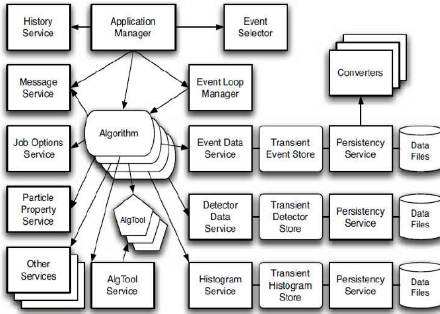
Fig. 2.22: The Athena architecture.
