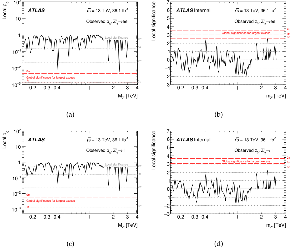
Fig. 5.9: The local (left-hand column) p -value and (right-hand column) significances derived from ideal Z'_\chi signals between 0.15 and 3.0 TeV. Shown are results for the (upper) di-electron and (lower) di-lepton channels. Also shown are local (dot-dashed line) and global (broad dashed line) significance levels, where the global levels apply only to the most significant local excess. The binning used in each channel is optimised for the mass resolution.
