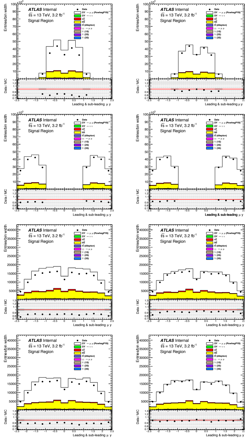
Fig. 6.18: Inclusive rapidity distribution (left) before and (right) after applying the trigger SF for the 2mu6 triggers. First row: region A; second row: region B; third row: region C; fourth row: region D. The statistical uncertainties for the signal and background distributions are shown in the shaded band in the ratio panel (lower panel), and the statistical uncertainties on the data points are represented by the vertical bars.
