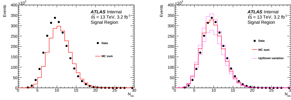
Fig. 6.6: Control distributions of the average number of reconstructed vertices before (left) and after (right) application of the PileupRewightingTool . All MC expectations are scaled to the integrated luminosity of the data using predicted MC cross sections of each sample. The magenta band in the right plot denotes the systematic variation of 1/1.09 scaling factor (varied between 1/1.0 and 1/1.18 ).
