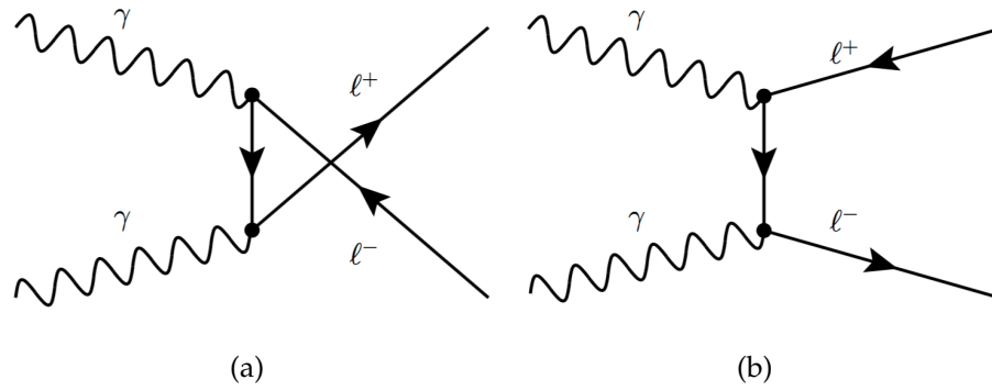
Fig. 1.10: LO photon-induced Feynman diagrams which contribute to di-lepton production. (a) u -channel diagram; (b) t -channel diagram
