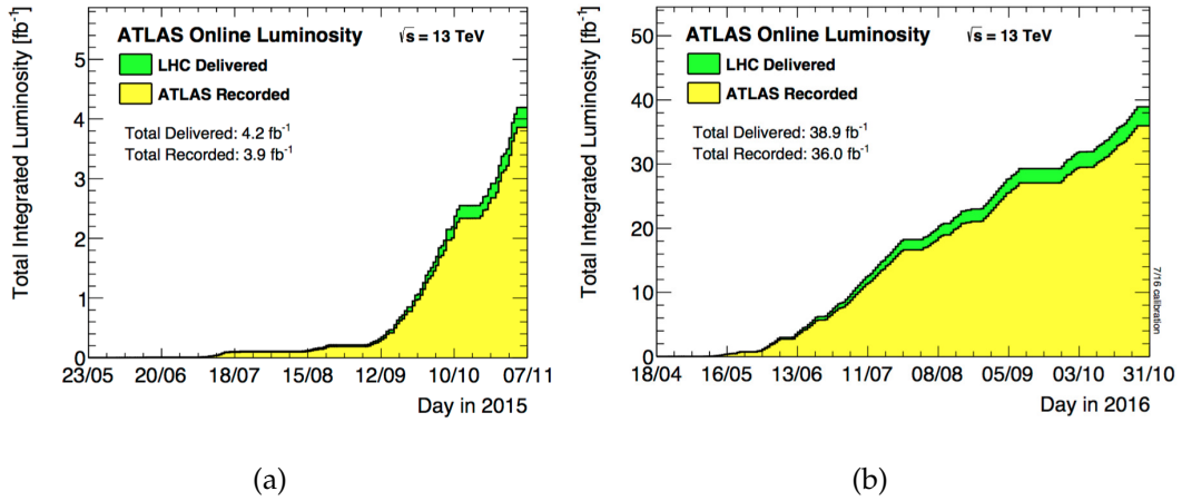
Fig. 2.3: Luminosities delivered by the LHC (green) and recorded by ATLAS (yellow) at \sqrt{s} = 13 TeV in 2015 (left plot) and 2016 (right plot).
