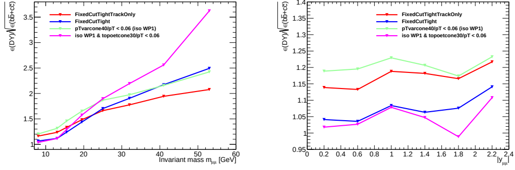
Fig. 6.30: Ratio between the efficiency on the DY signal and the square root of the efficiency on the b\bar{b} + c\bar{c} background as a function of ( Left) the invariant mass of the di-muon system and (Right) the di-muon system in the lowest invariant mass bin (from 7 to 9 GeV) for four different isolation WPs, namely FCTTO (red solid line), FCT (blue solid line), iso WP1 (green solid line) and iso WP2 (magenta solid line).
