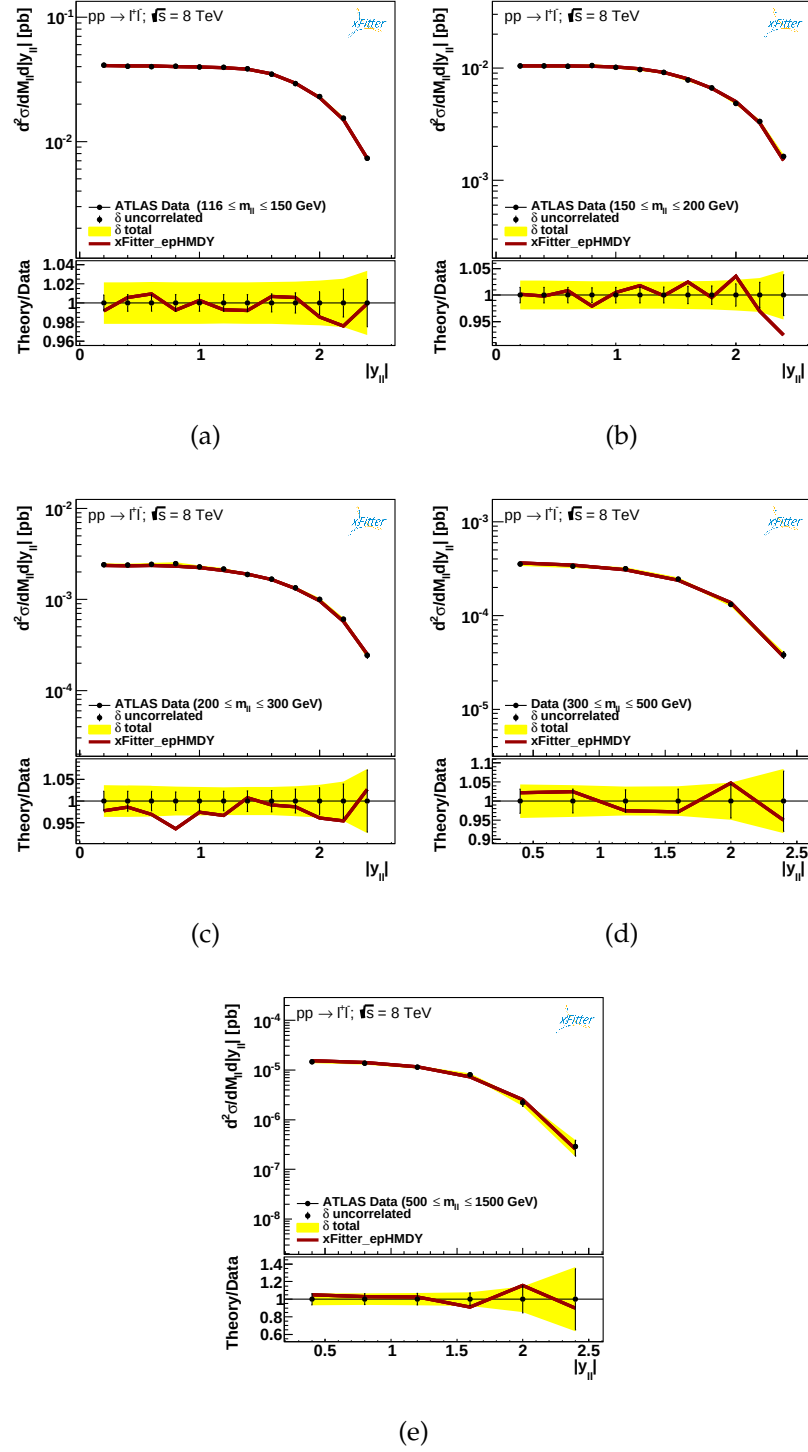
Fig. 4.9: Comparison between the results of the fit and the ATLAS data for the (m_{\ell\ell}, |y_{\ell\ell}|) double-differential DY cross-sections as function of |y_{\ell\ell}| . The comparisons are shown both in an absolute scale and as ratios to the central value of the experimental data in each y_{\ell\ell} bin. The error bars on the data points correspond to the bin-to-bin uncorrelated uncertainties, while the yellow bands indicate the size of the correlated uncertainties. The solid lines indicate the results of this fit xFitter_epHMDY.
