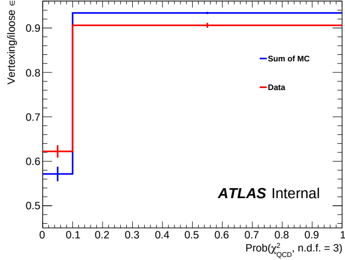
Fig. 6.33: Vertexing and isolation requirement efficiency (defined in Eq. 6.11) as a function of \text{Prob}(\chi^2_{QCD}, \text{n.d.f.} = 3) for both data (solid red line) and MC (blue solid line).
