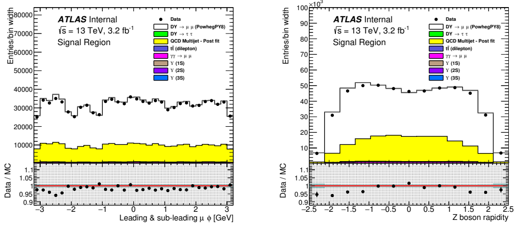
Fig. 6.21: Inclusive lepton \phi (left) and Z boson rapidity (right) distributions. All selection criteria are applied. The statistical uncertainties for the signal and background distributions are combined in the shaded band in the ratio panel (lower panel), and the statistical uncertainties are shown on the data points (vertical bars).
