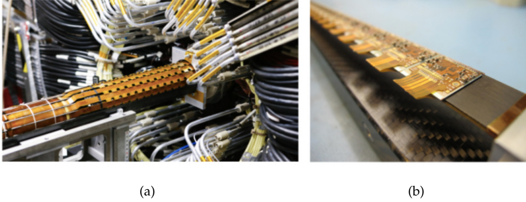
Fig. 2.14: The ATLAS IBL detector before the insertion (left hand-side) and an IBL stave where the single detector modules are mounted on carbon fibre support structures (right hand-side).
