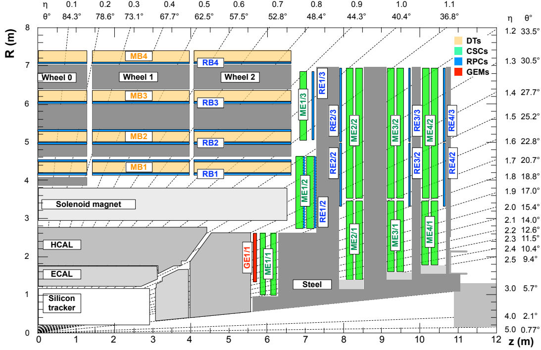
Figure 3.5: Cross-sectional view of the CMS quadrant highlighting the proposed location of GEM detectors (red).
