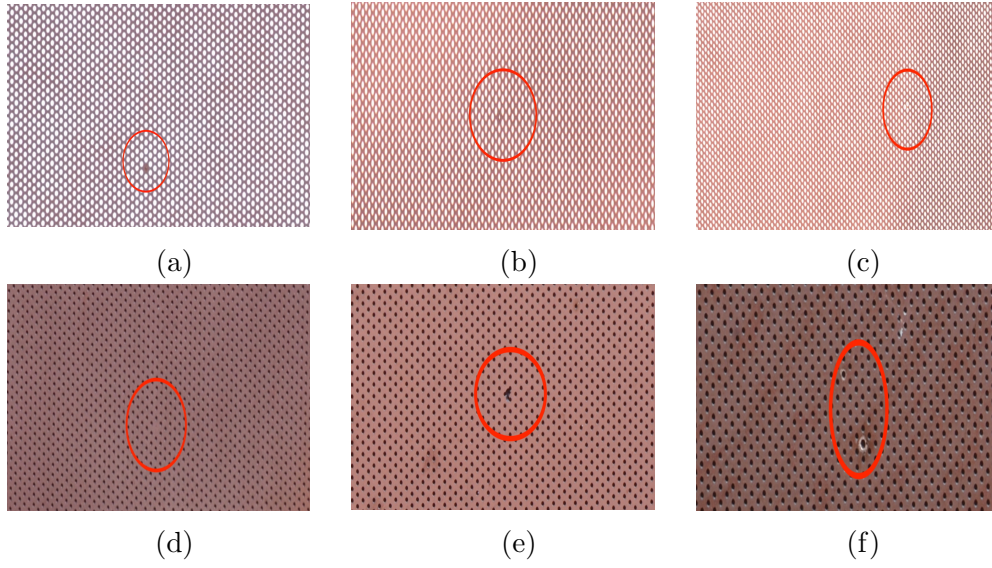
Figure 3.34: Observed imperfections in the GEM foils: (a) Un-etched area, (b) under-size hole, (c) over-size hole (d) missing hole, (e) excess etching and (f) burnt area.
