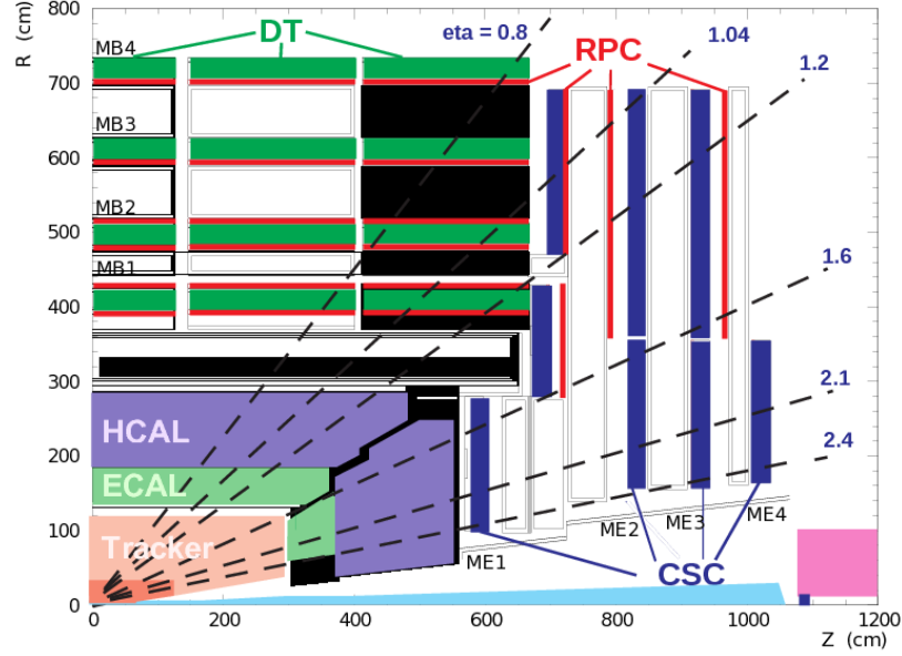
Figure 2.14: Longitudinal layout of one quadrant of the CMS detector. There are four DT stations named MB1-MB4 marked with green colour. Four CMS systems in high pseudo-rapidity region named ME1-ME4 in blue colour. Also, there are several RPC stations in barrel region and part of endcap region marked with red colour.
