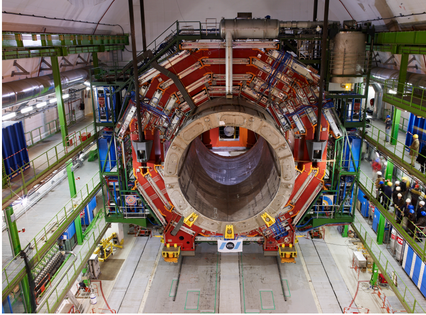
Figure 2.11: CMS Magnet system [48].
