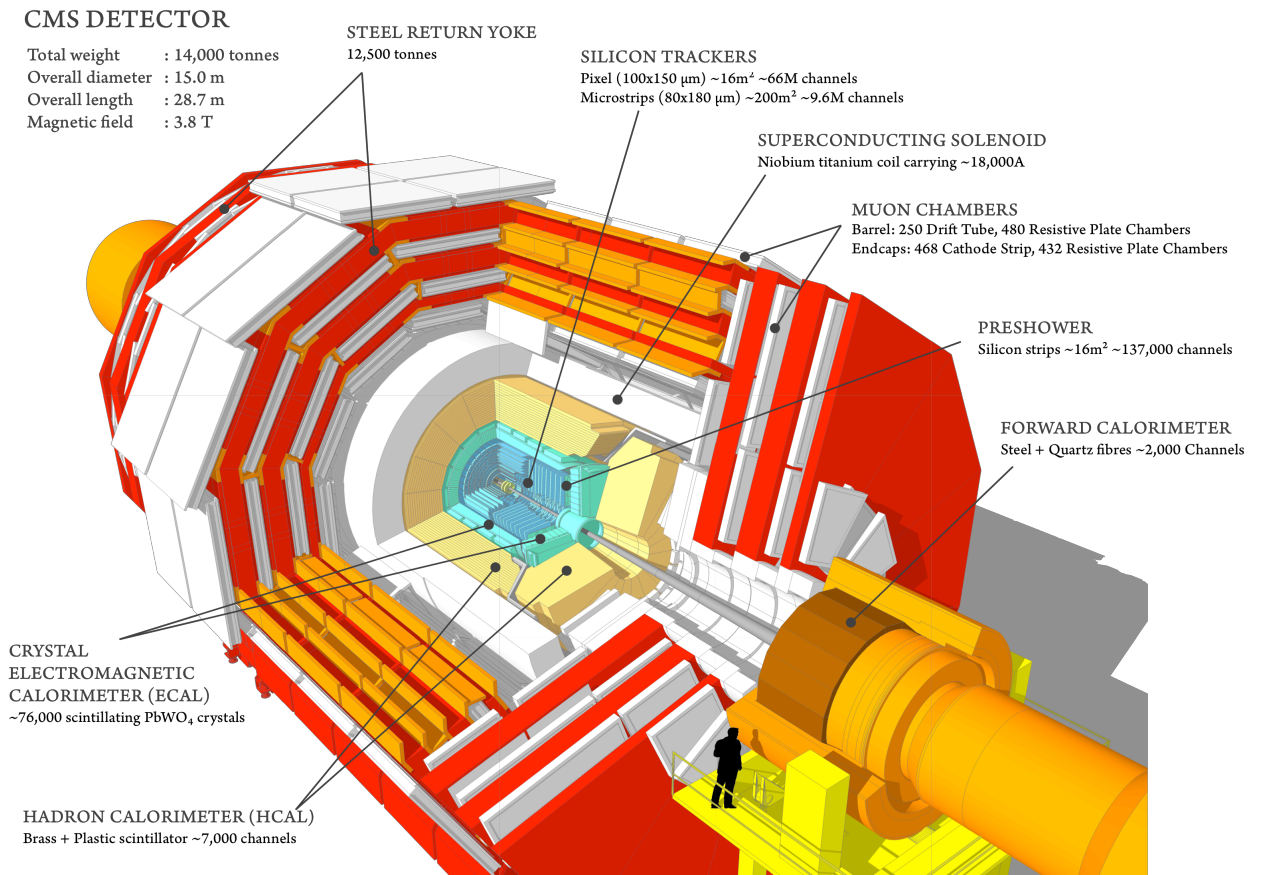
Figure 2.9: CMS detector drawing [47].
