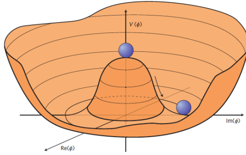
Figure 1.2: Higgs potential [16]
