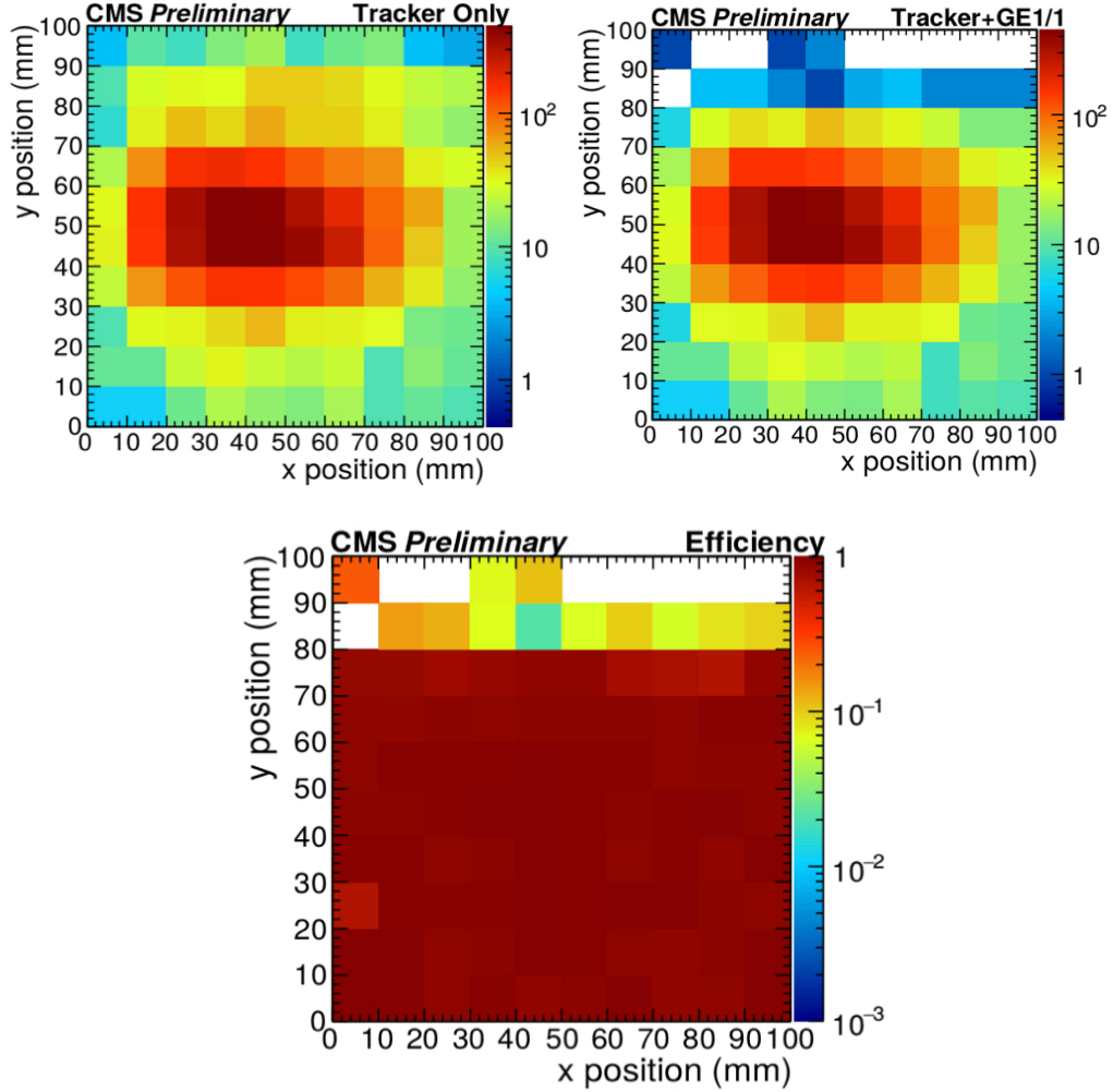
Figure 3.23: 2D distributions showing events with hits registered in the trackers (top left), events registered in three trackers and GE1/1's (top right) and the division of the two histograms used to define the fiducial region for GE1/1 efficiency measurements (bottom).
