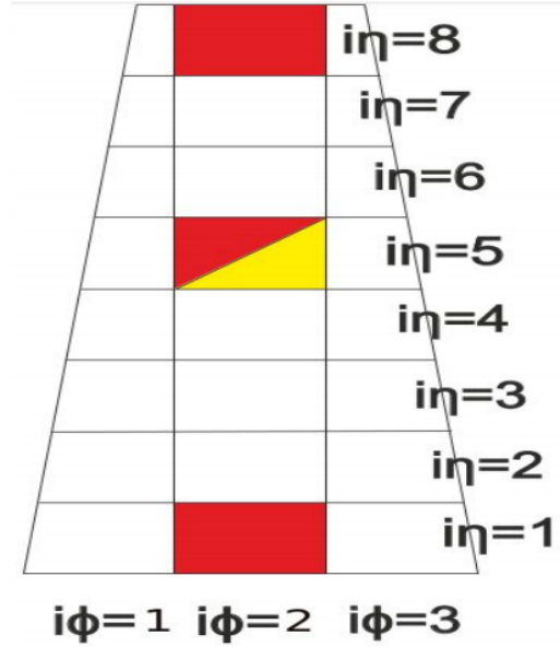
Figure 3.18: Different (i\eta, i\phi) sectors of a full-size GE1/1 detector prototype. The red and yellow colour shows which sector of GE1/1 is exposed to the beam. Red sectors are collected with Ar/CO_2/CF_4 (45/15/40) gas mixture while the yellow sectors are taken with Ar/CO_2 (70/30) gas mixture.
