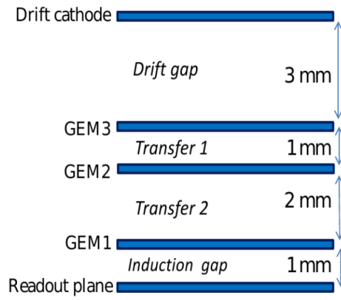
Figure 3.6: The layout of different GEM layers inside a CMS GE1/1 detector.
