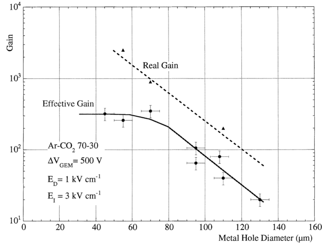
Figure 3.32: Real gain and effective gain variation with GEM hole diameter [91] having a foil thickness of 60 \mu m (= 50 \mu m + 5 \mu m + 5 \mu m) . As the hole diameter decreases, the effective gain increases till 70 \mu m and after that it reaches saturation. This is due to loss of generated electrons in the avalanche to the bottom of the GEM electrode when hole diameter is reduced below the foil thickness.
