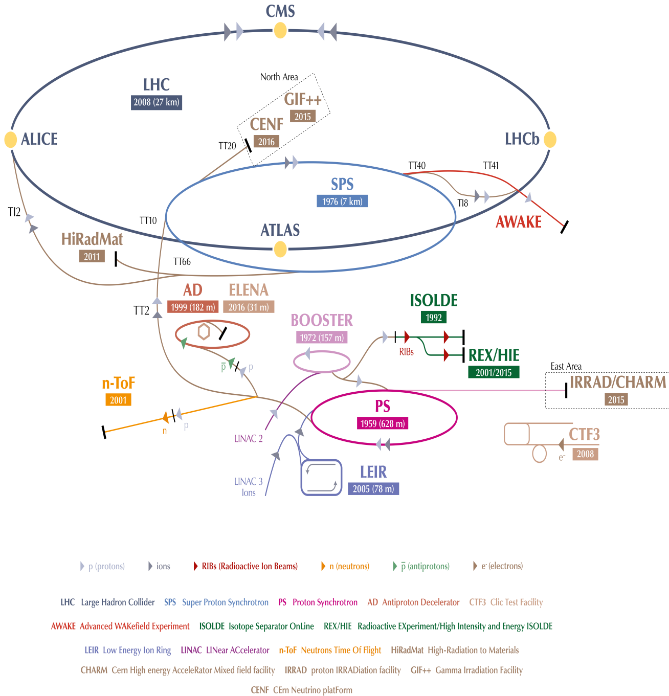
Figure 2.2: The LHC accelerator chain along with all its other experiments which use proton beam from different parts of the accelerator, either from PSB, PS or SPS [31]
