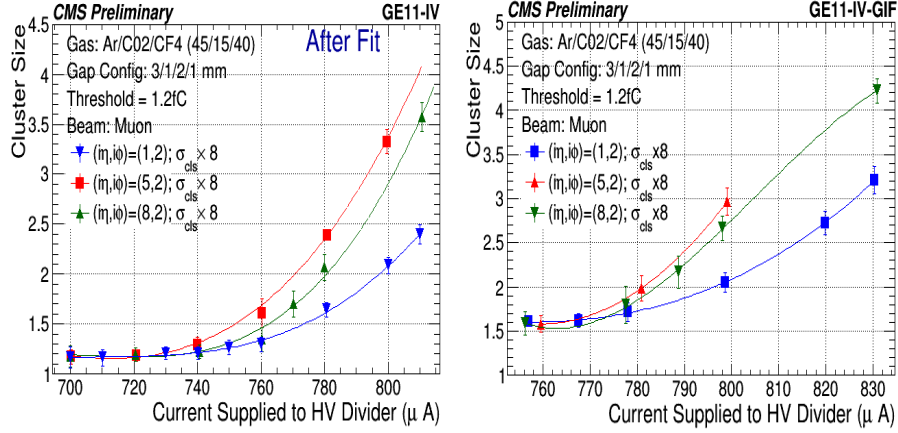
Figure 3.28: Cluster size distribution: Left - GE1/1-IV, Right - GE1/1-IV-GIF
