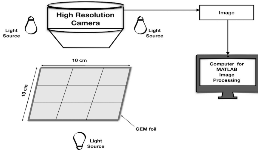
Figure 3.33: Sketch of the set-up used for optical measurements of the GEM foil.
