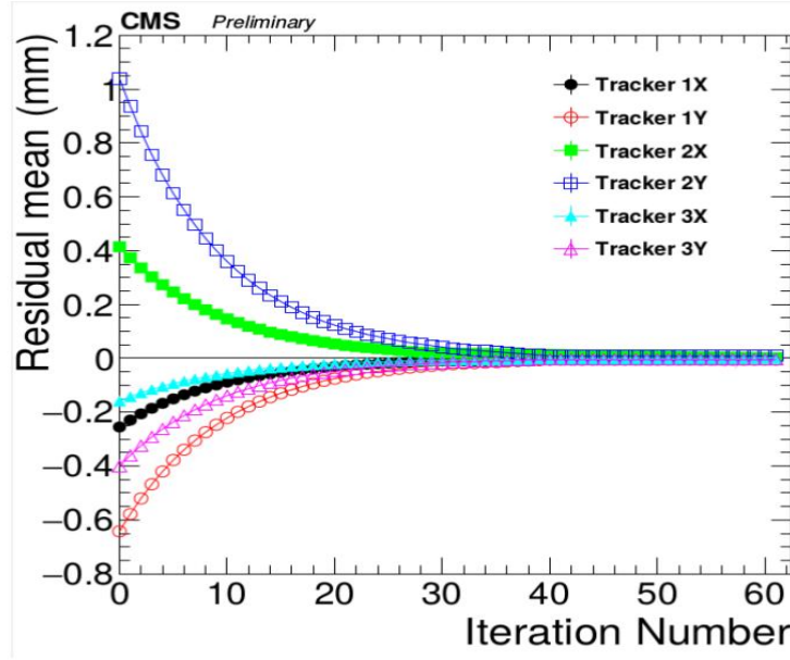
Figure 3.22: Variation of track residuals for three trackers with respect to the iteration number along different directions
