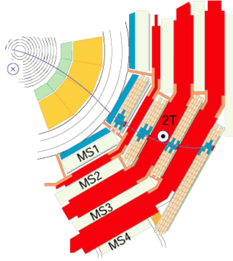
Figure 2.13: A muon leaves curved trajectory in LHC and the bending changes as the magnetic field direction of solenoid inside and outside are opposite.
