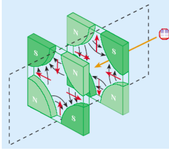
Figure 2.4: Pair of quadrupole magnets [34].
