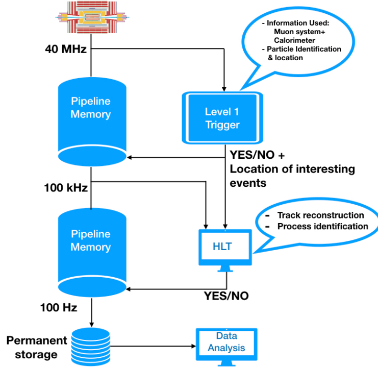
Figure 2.16: CMS trigger flow diagram that uses two level trigger. At Level 1, CMS uses information from muon system and calorimeter. Using this information it decides to reject or pass the event to the HLT farm for further processing. HLT uses fast offline reconstruction algorithm that uses information from all sub-system, i.e., calorimeters, muon system as well as tracker to decide to keep or reject the event.
