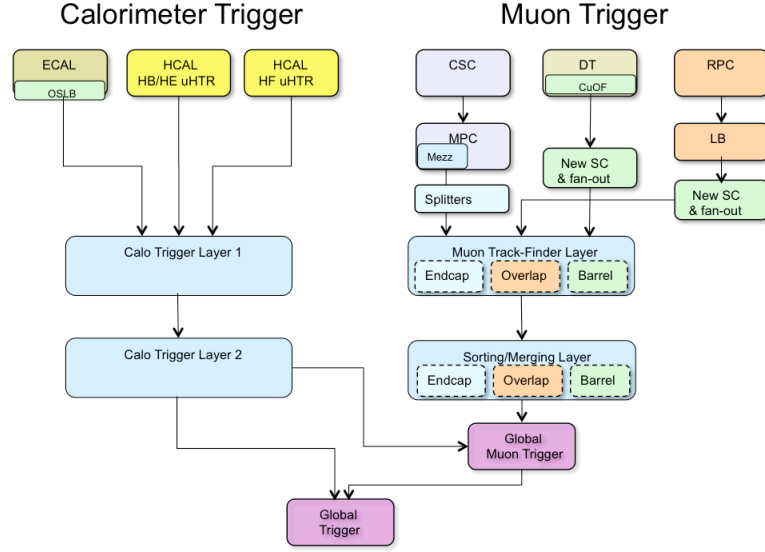
Figure 2.17: CMS Level-1 trigger flow diagram [56]. On left the hierarchy of calorimeter trigger is shown. On right the different layers of the muon trigger system is shown. Finally the global trigger combines information from both system to take the Level-1 decision.
