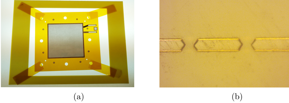
Figure 3.29: (a) 10\ \text{cm} \times 10\ \text{cm} GEM foil encapsulated in a frame and (b) Cross-sectional view of the foil showing the double cone structure of the engraved holes, developed by Micropack.
