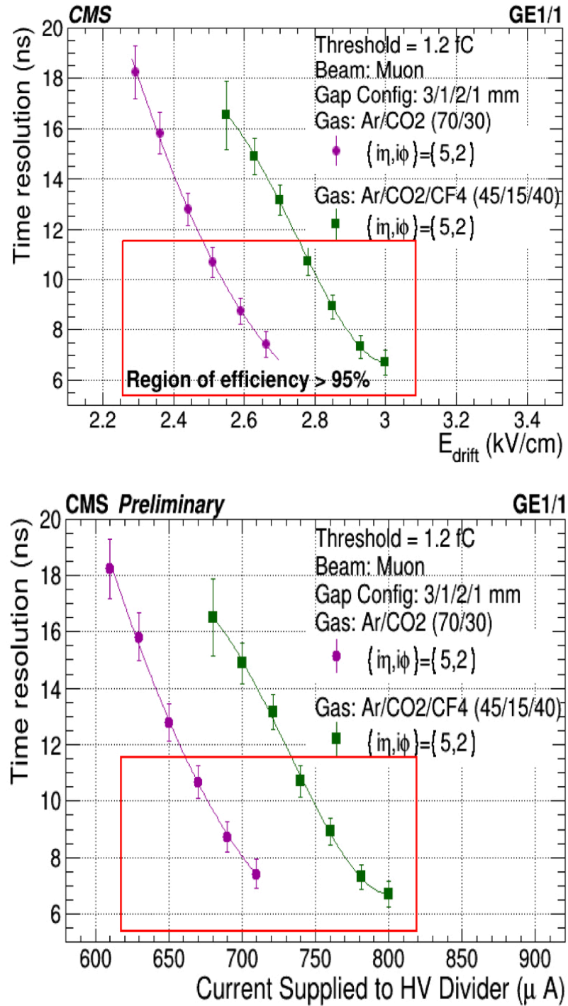
Figure 3.26: Time-resolution with respect to E_{drift} (top) and current supplied to high voltage divider (bottom) for two different gas mixture.
