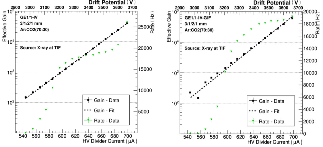
Figure 3.14: Gain and rate variation for Ar : CO_2 (70:30) with respect to the current supplied to the high voltage divider for GE1/1-IV (left) and GE1/1-IV-GIF (right).
