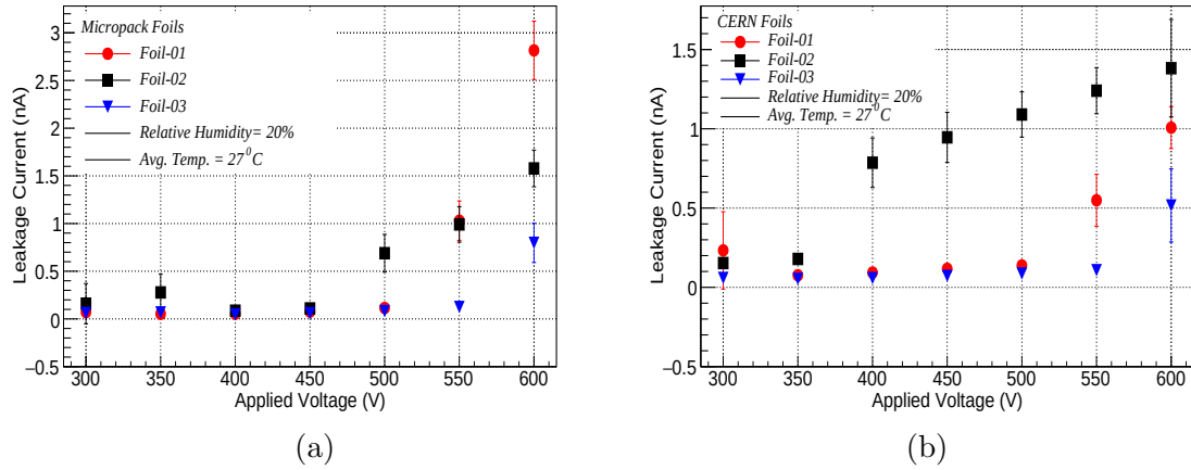
Figure 3.37: Leakage Current for (a) Micropack Foils and (b) CERN Foils, at an average temperature of T = 27^\circ\text{C} and 20% relative humidity.
