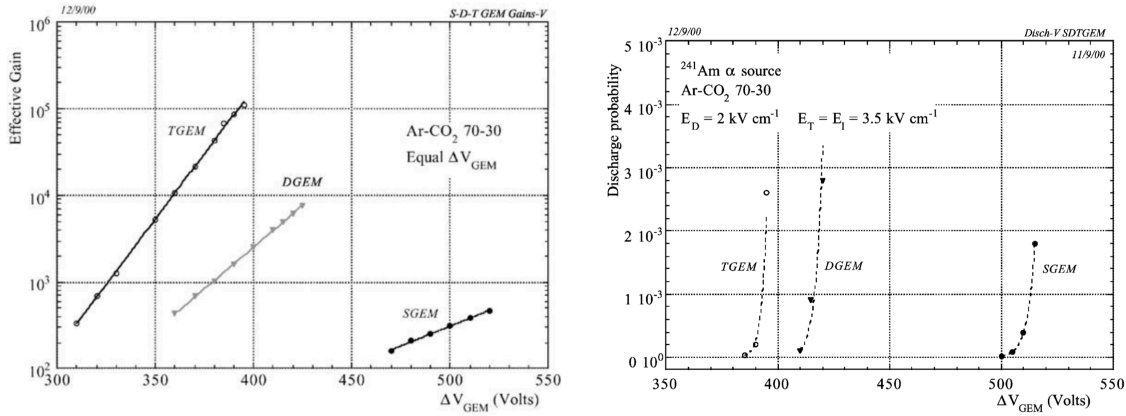
Figure 3.3: Comparison of total effective gain on anode as a function of applied voltage for single, double and triple layered GEM detectors (left). The discharge probability as a function of applied voltage is shown for the single, double and triple layered GEM detectors (right) [77].
