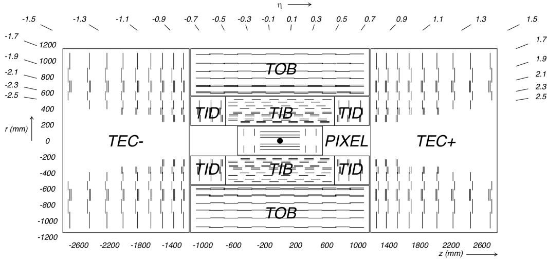
Figure 2.12: A systematic cross section view of CMS tracker showing silicon pixel and strip detectors. Double lines show back-to-back modules that deliver stereo hits.
