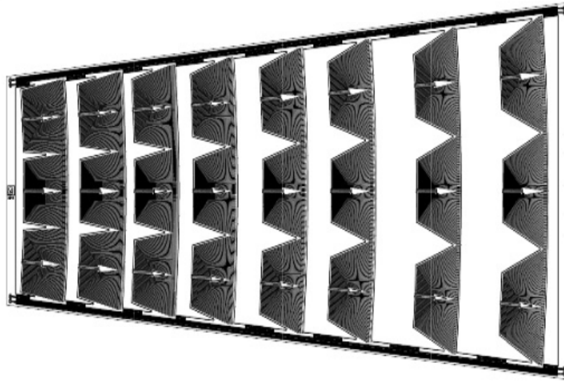
Figure 3.7: Drawing of a large trapezoidal CMS GEM chamber showing 8 - \eta and 3 - \phi par partitions.
