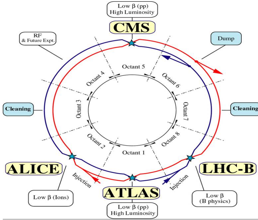
Figure 2.7: LHC geometry with arcs and straight sections [45].
