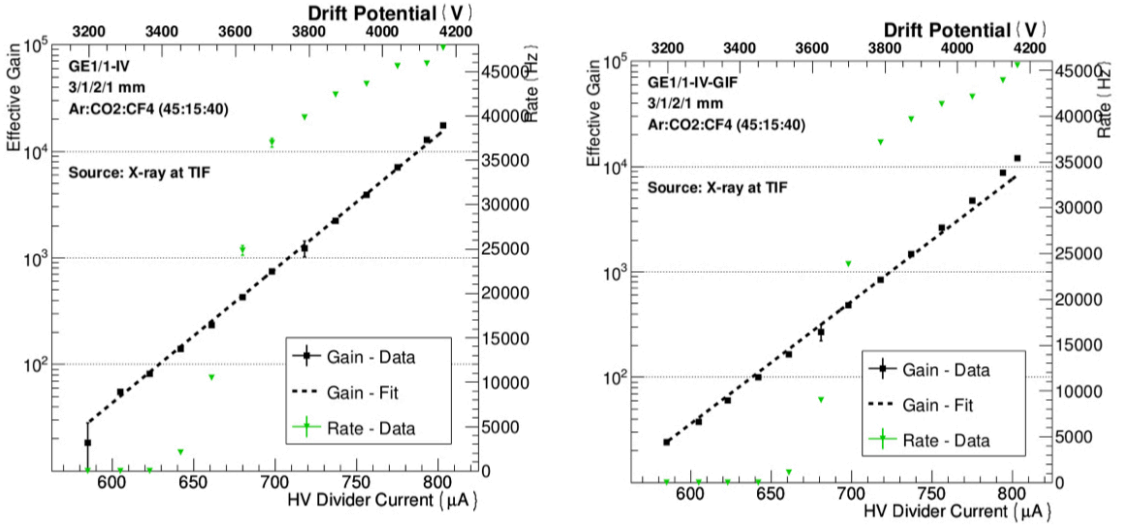
Figure 3.15: Gain and rate variation for Ar : CO_2 : CF_4 (45:15:40) with respect to the current supplied to the high voltage divider for GE1/1-IV (left) and GE1/1-IV-GIF (right).
