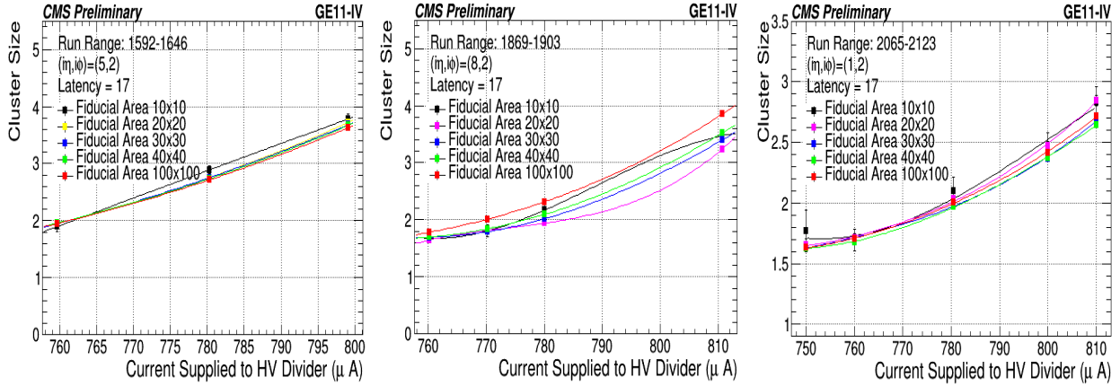
Figure 3.27: Mean value of cluster size distribution at different current supplied to high voltage divider obtained during the beam test campaign: for 2014H4A which was taken for region (\eta, \phi) = (5, 2) (left), for 2014H4C taken for region (\eta, \phi) = (8, 2) (middle) and for 2014H4D taken for region (\eta, \phi) = (1, 2) .
