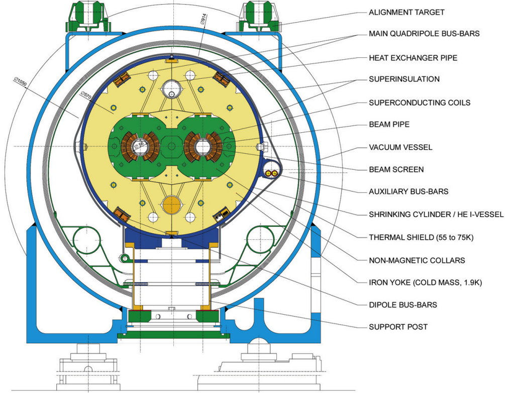
Figure 2.3: Diagram showing the cross-section of an LHC dipole magnet with cold mass and vacuum chamber [33].
