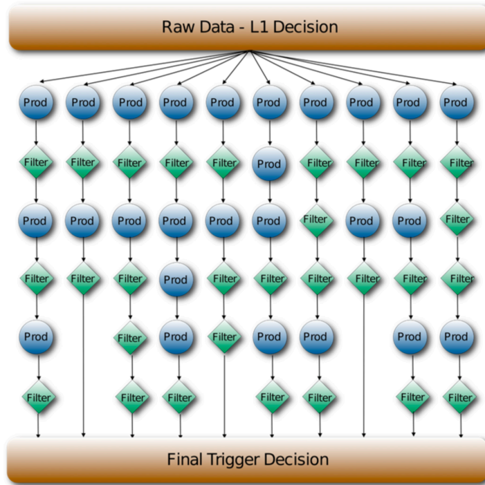
Figure 2.18: The systematic representation of HLT menu and its path[58].
