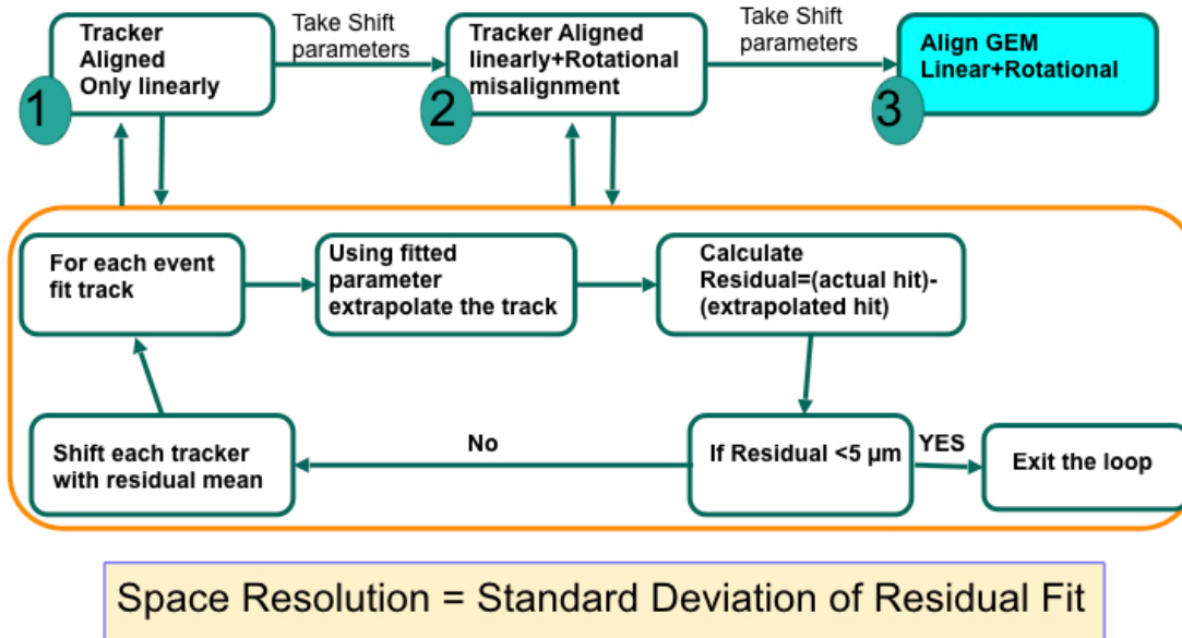
Figure 3.21: Flowchart illustrating the work flow of detector alignment algorithm.
