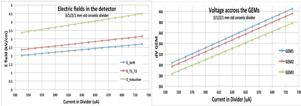
Figure 3.13: (Left) Electric field of the induction region (green), drift region (blue) and between the transfer region (red) is shown. (Right) Voltage across each GEM foil for the tested GE1/1 detector is shown.
