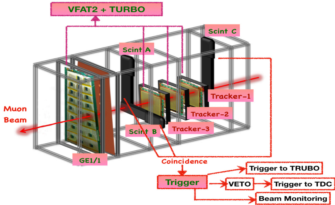
Figure 3.16: Schematic view of the beam test set-up with the three tracking GEM detectors and a GE1/1 prototype.
