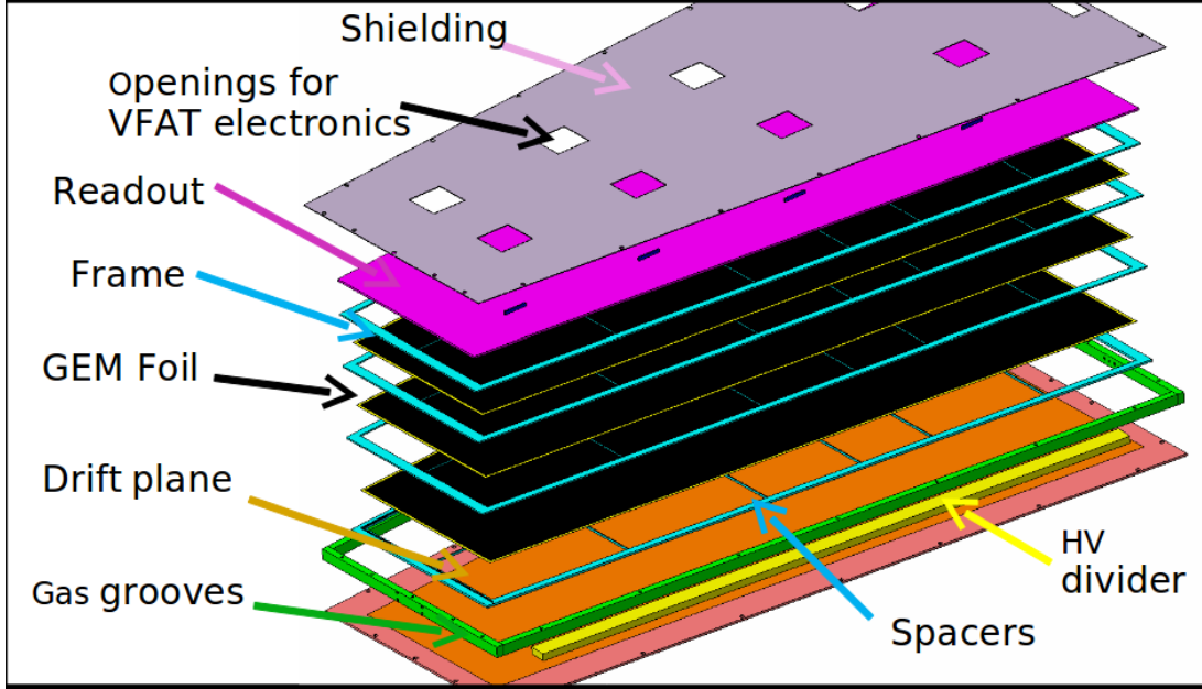
Figure 3.8: Layer by layer view of CMS GE1/1 detector
