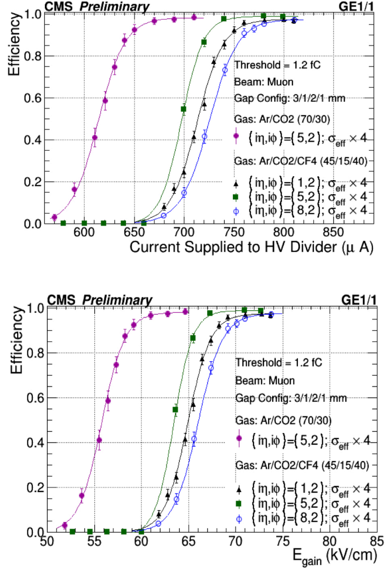
Figure 3.25: Efficiency with respect to E_{\text{gain}} for two different gases and three different (i\eta, i\phi) sectors.
