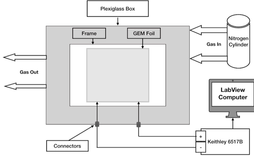
Figure 3.36: Sketch of the set-up used for the measurement of leakage current.
