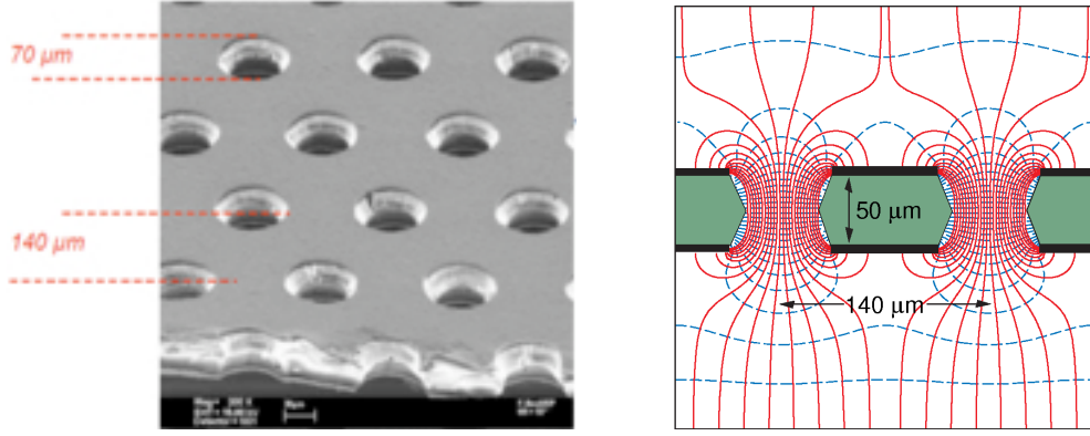
Figure 3.1: Cross-sectional view of a GEM foil etched with holes (left) [26]. The strong electric field generated in the vicinity and inside the holes after the application of potential difference across the GEM foil (right) [14]. Here, electric field lines (solid) and equipotential (dashed) are shown.
