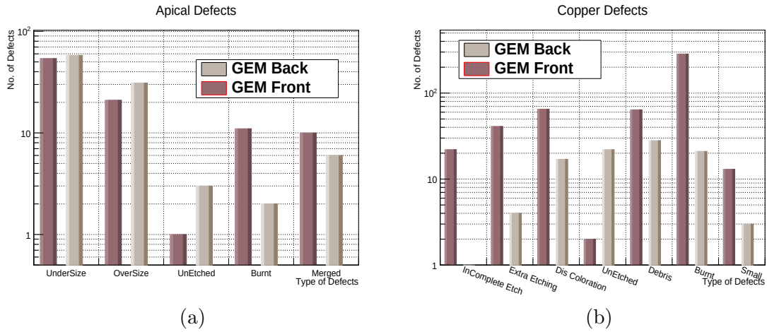
Figure 3.35: Number of defects seen in (a) Insulator (Apical Type NP) and (b) Copper, for one of the 10 cm \times 10 cm foil.
