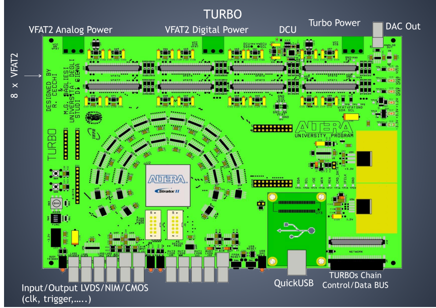
Figure 3.11: TURBO board [87].
