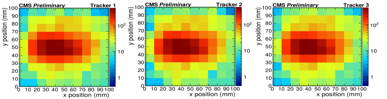
Figure 3.20: 2D- beam profile plot for the first, second and third tracker. The X and Y axis of the plots correspond to the distance (in mm) measured from the central position of the trackers in X and Y direction respectively. The different colours in the colour palette correspond to the number of hits registered in the detector at a particular (x,y) position.
