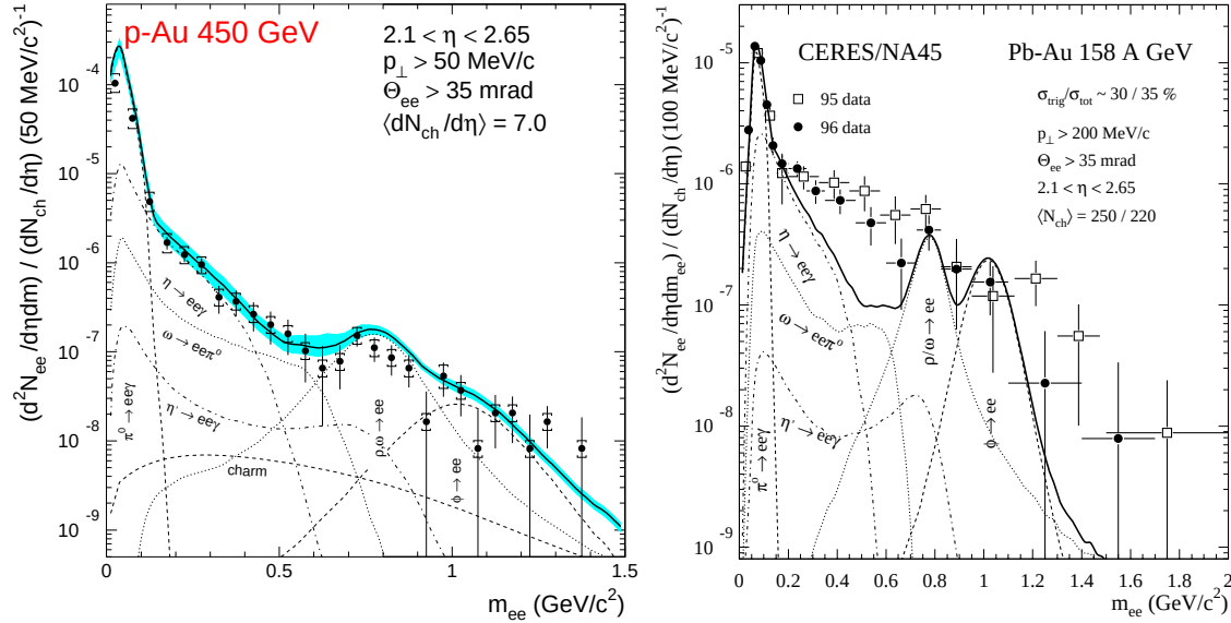
Figure 1.4. Dilepton invariant mass spectrum in p-Au (left) and in Pb-Au (right) collisions, compared to the expected yield (solid line) from known sources [6].
