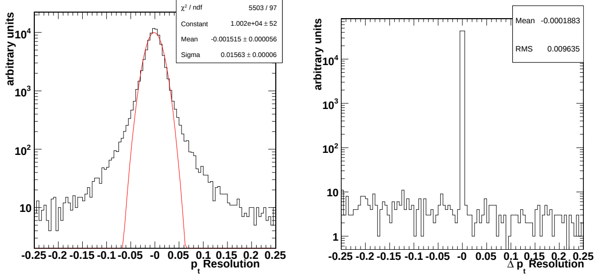
Figure 5.14: On the left: Resolution (defined according to Equation 5.2) of the transverse momentum of muons that have been selected with the likelihood method. On the right: Resolution difference between the selection with the likelihood method and angular matching to generator muons.
