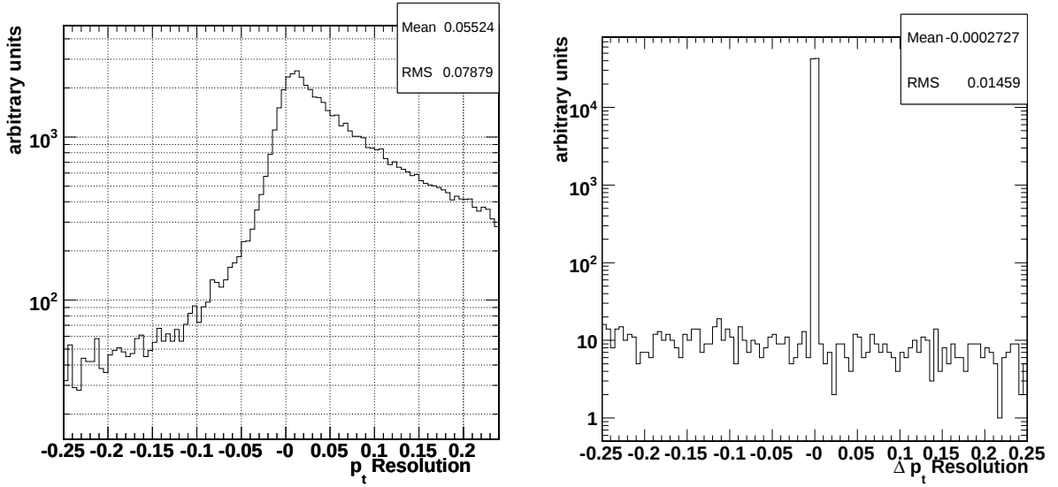
Figure 5.18: On the left: Resolution (defined according to Equation 5.2) of the transverse momentum of electrons that have been selected with the likelihood method. On the right: Resolution difference between the selection with the likelihood method and angular matching to generator electrons.
