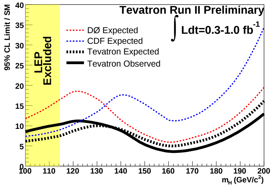
Figure 3.5: Limits on the Higgs boson production cross section normalized to the Standard Model prediction as function of the Higgs mass m_H for the combined CDF and DØ analyses. The dashed lines show the expectations determined from background-only pseudo-experiments. The solid line shows the observation. [37]
