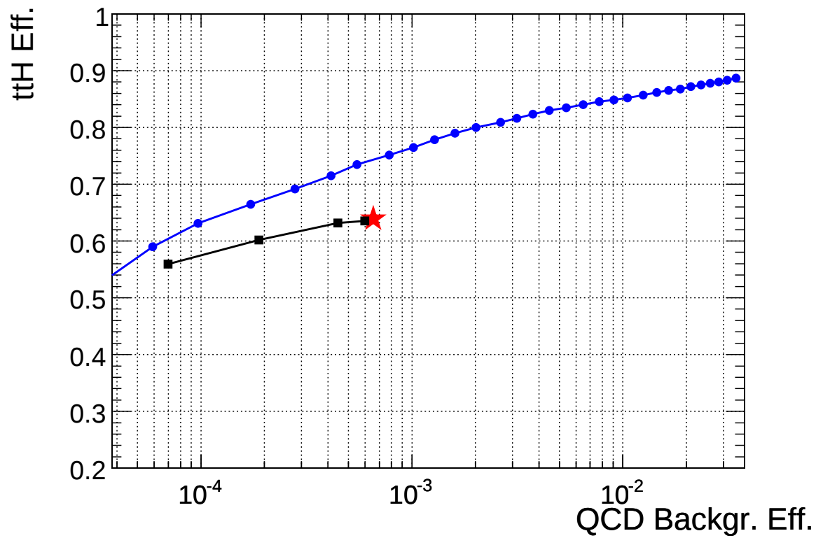
Figure 5.13: t\bar{t}H signal efficiency versus QCD ( \hat{p}_t > 170 \text{ GeV}/c ) efficiency. Circles: Likelihood performance without HLT selection; Star: HLT selection; Squares: Likelihood performance after the HLT selection.
