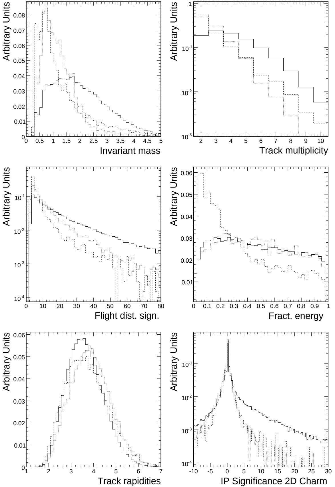
Figure 4.10: Observables used for the calculation of the b-tagging discriminator in the “RecoVertex” category. The solid lines refer to b-jets, the dotted line to c-jets and the dashed line to light flavour (uds-) jets.
