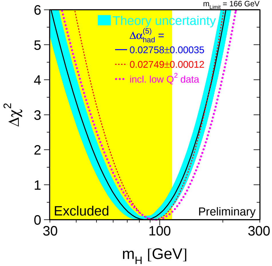
Figure 3.6: \Delta\chi^2(m_H) = \chi_{min}^2(m_H) - \chi_{min}^2 as function of m_H . The band around the curve represents the theoretical uncertainty due to missing higher order corrections. The vertical band shows the exclusion limit at m_H > 114.4 GeV/ c^2 from direct measurements. [2] [38]
