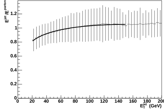
Figure 4.18: E_{jet}^{et}/E_{parton}^{et} vs. E_T^{jet} for the IC algorithm with a cone radius of 0.4 applied on a final state with four primary quarks. The vertical bars illustrate the resolution. For this plot, only well matched ( \alpha_{jp} < 0.3 ) and non-overlapping jets were taken into account in order to determine the optimal energy resolution.
