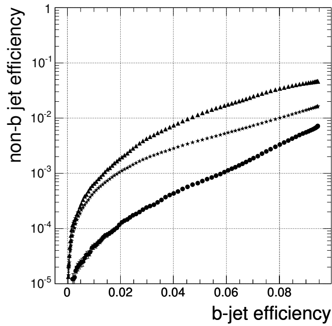
Figure 4.16: Mistagging rates versus b-tagging efficiency for the soft muon b-tagging algorithm. Triangles refer to c-jets, circles to uds-jets and stars to g-jets. The “physics” definition of the true jet flavour has been used. The results have been obtained with fully leptonic and semileptonic t\bar{t} events and QCD events. [40]
