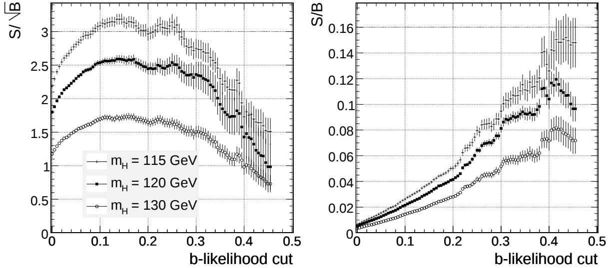
Figure 5.34: Observability in terms of significance S/\sqrt{B} (left plot) and purity S/B (right plot) for three different Higgs boson mass hypotheses (115, 120 and 130 \text{GeV}/c^2 ) in dependence on the cut on the b-tagging likelihood L_{bTag} , after an integrated luminosity of 60 \text{ fb}^{-1} for the semileptonic (muon and electron) t\bar{t}H decay channel. No mass window has been applied. The error bars indicate the statistical error due to the finite size of datasets. Also here, bin-to-bin correlations occur because of the sliding cut on the b-tagging likelihood.
