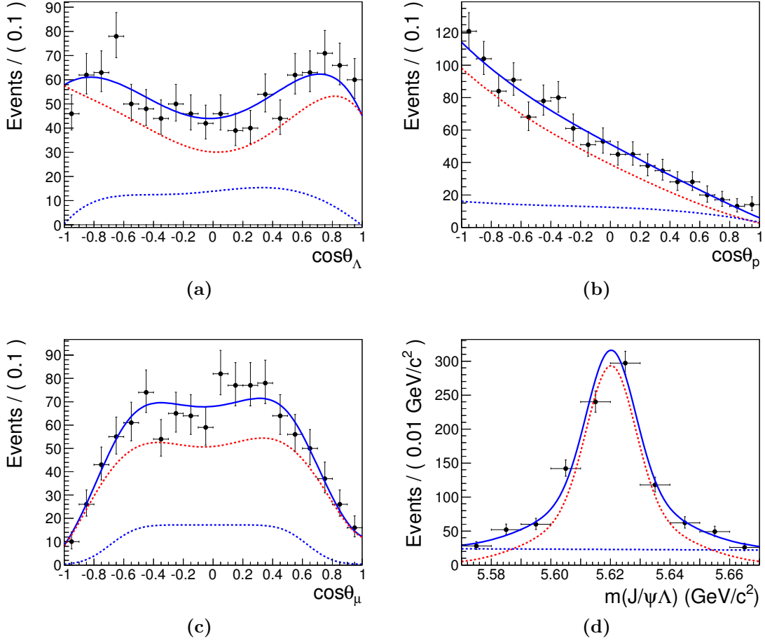
Figure 5.12: The full likelihood fit to data. Projections of the fit result in (a) \cos \theta_\Lambda , (b) \cos \theta_p , (c) \cos \theta_\mu , (d) m(J/\psi \Lambda) , for \bar{\Lambda}_b candidates. The projection of the total fit is shown in solid blue line, the signal folded with efficiency in dashed red, and the background component in dashed blue.
