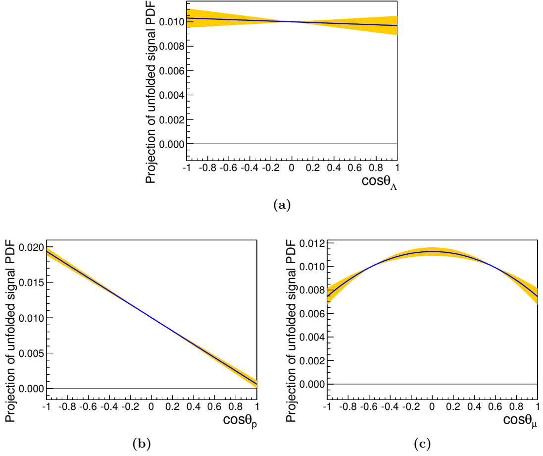
Figure 5.13: Simulation of the signal angular distributions, corrected for efficiency and detector effects, with the physics parameters obtained by the fit to data. The color band represents one statistical standard deviation as obtained by the fit. Projections in (a) \cos\theta_\Lambda , (b) \cos\theta_p , (c) \cos\theta_\mu .
