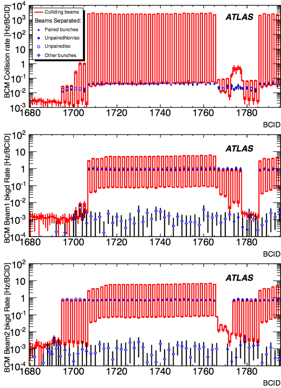
Fig. 4.6 BCM collision rate (top) and background rates for beam 1 (middle) and beam 2 (bottom) per BCID before and during collisions [112].
