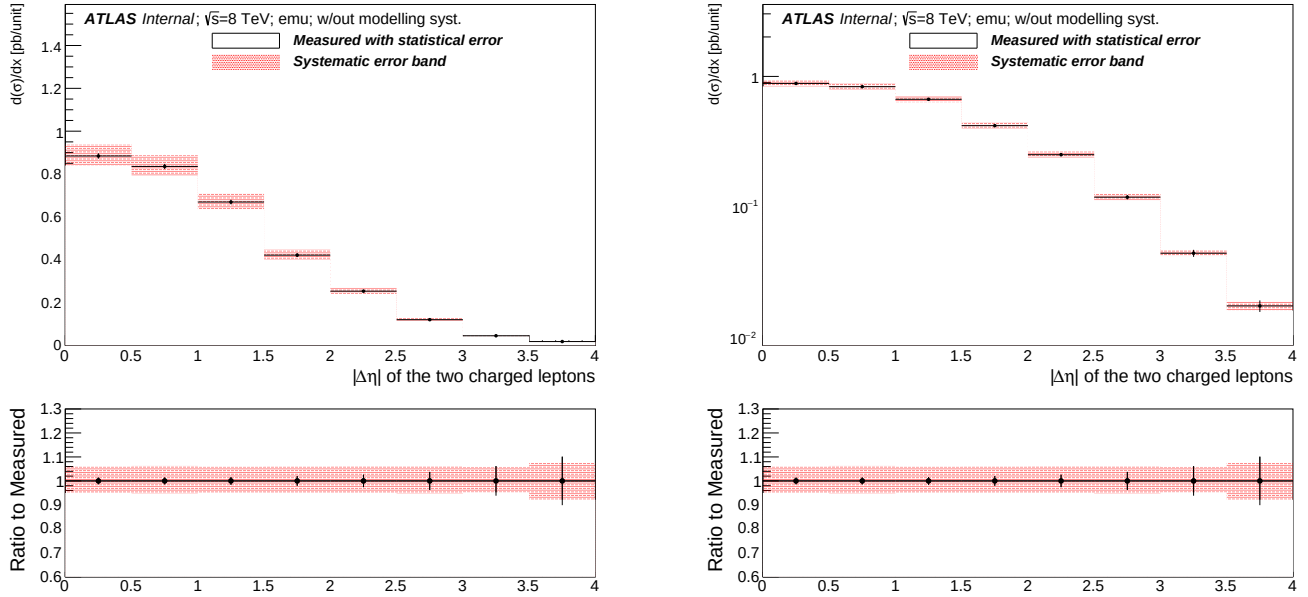
Fig. 8.13 Fiducial differential distribution as a function of the absolute difference of pseudorapidity of the dilepton, |\Delta\eta_{\ell\bar{\ell}}| plotted on the linear (left) and semi-log (right) scale. Only the detector modelling systematics are included on the systematic error band.
