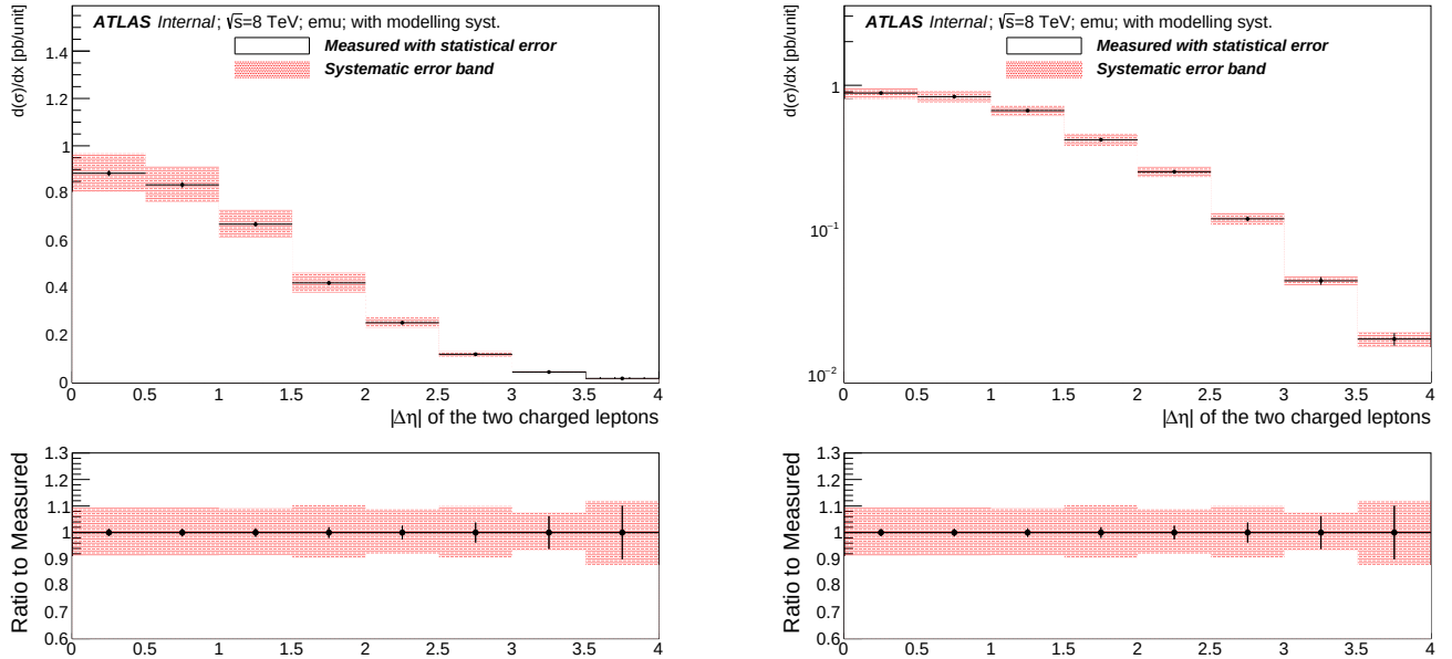
Fig. 8.14 Fiducial differential distribution as a function of the absolute difference of pseudorapidity of the dilepton, |\Delta\eta_{\ell\bar{\ell}}| plotted on a linear (left) and semi-log (right) scale. The detector modelling, signal modelling and background modelling systematics are included on the systematic error band.
