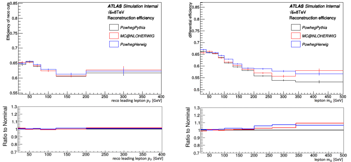
Fig. 6.23 Comparison of the reconstruction efficiency for different MCs as a function of the leading lepton p_T on the left, and the dilepton mass m_{ll} on the right.
