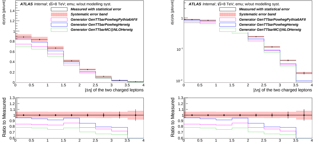
Fig. 8.15 Fiducial differential distribution as a function of the absolute difference of pseudo-rapidity of the dilepton, \Delta\eta_{ll} plotted on a linear (left) and semi-log (right) scale. Only the detector modelling systematics are included on the systematic error band.
