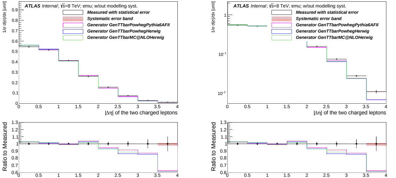
Fig. 8.16 Comparison of the measured fiducial differential distribution as a function of the absolute difference of pseudorapidity of the dilepton, |\Delta\eta_{ll}| plotted on a linear (left) and semi-log (right) scale. Only the detector modelling systematics are included on the systematic error band.
