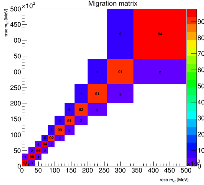
Fig. 6.20 Migration matrix for the dilepton invariant mass.
