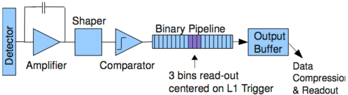
Fig. 4.9 SCT binary read-out circuits with important components.
