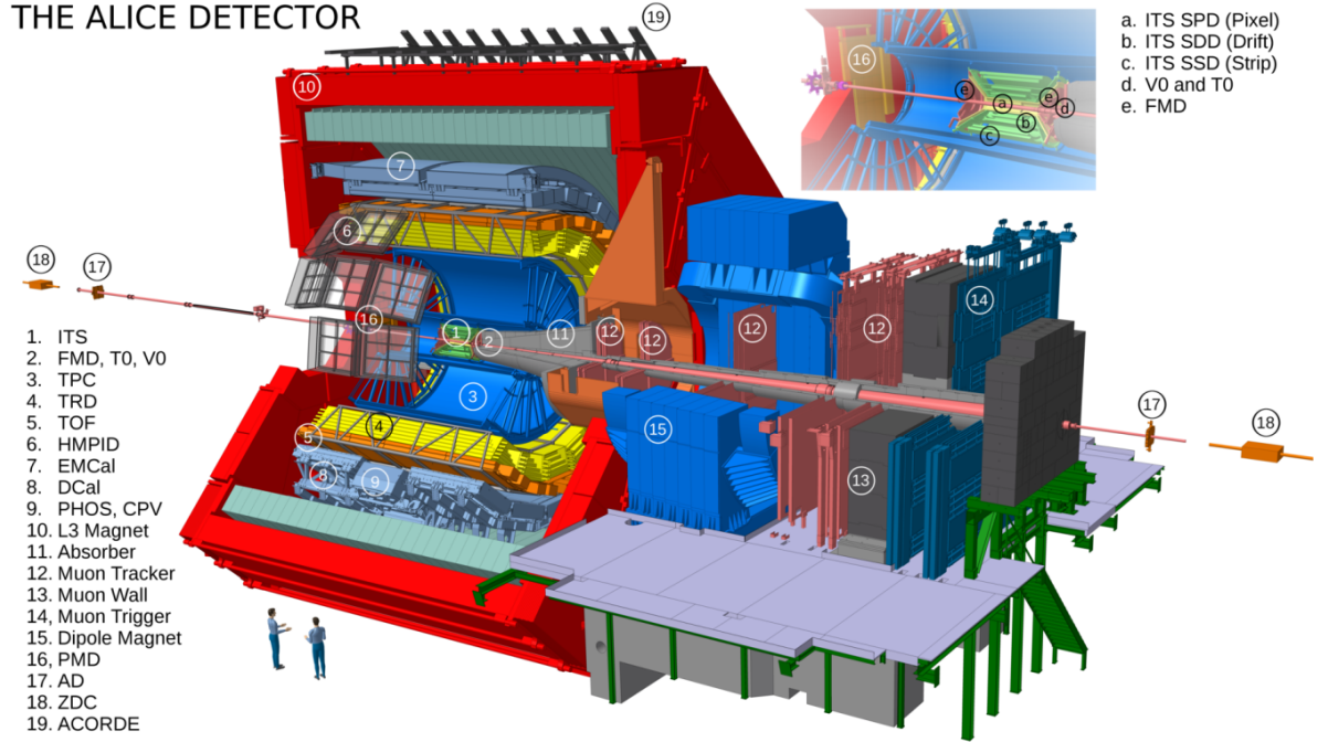
Figure 2.2: Schematics of the ALICE apparatus at the LHC (Run 2 configuration) [55].
