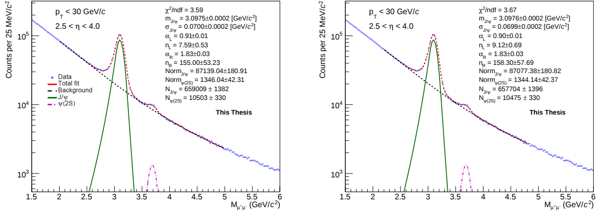
Figure 3.4: Tail parameter extraction using CB2+CB2+VWG function fitting to the p_T , y and S_0 integrated dimuon invariant mass spectrum in pp collisions at \sqrt{s} = 13 TeV in V0M (0 – 100)% centrality class. Fit ranges are 2.0 < M_{\mu^+\mu^-} < 5.0 GeV/ c^2 (left) and 2.2 < M_{\mu^+\mu^-} < 4.8 GeV/ c^2 (right).
