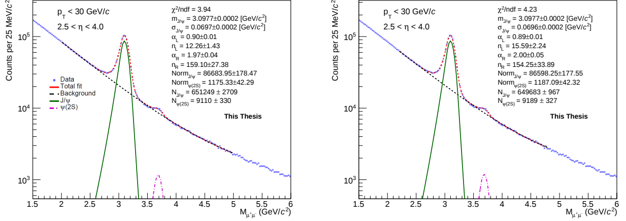
Figure 3.5: Tail parameter extraction using CB2+CB2+DoubleExp function fitting to the p_T , y and S_0 integrated dimuon invariant mass spectrum in pp collisions at \sqrt{s} = 13 \text{ TeV} in V0M (0 – 100)% centrality class. Fit ranges are 2.0 < M_{\mu^+\mu^-} < 5.0 \text{ GeV}/c^2 (left) and 2.2 < M_{\mu^+\mu^-} < 4.8 \text{ GeV}/c^2 (right).
