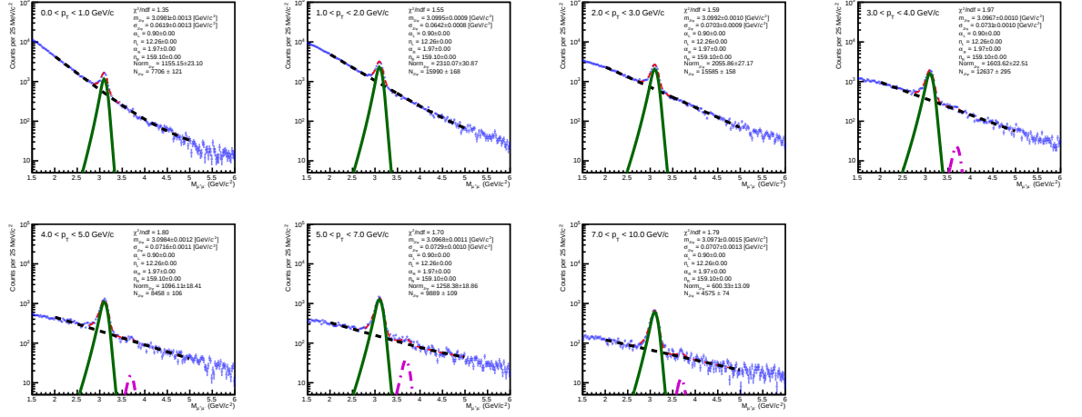
Figure 3.20: Yield extraction using CB2+CB2+DoubleExp fit function in fit range 2.0 < M_{\mu^+\mu^-} < 5.0 \text{ GeV}/c^2 for isotropic events.
