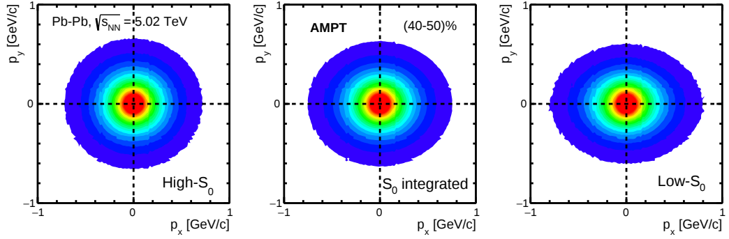
Figure 4.2: Transverse momentum space correlation ( p_x vs. p_y ) as a function of sphericity for (40–50)% central Pb–Pb collisions at \sqrt{s_{\text{NN}}} = 5.02 TeV in AMPT model [100]. Here, z -axis is the beam direction.
