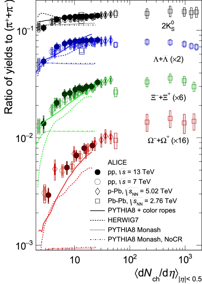
Figure 1.6: Multiplicity dependent yield ratios of strange and multi-strange hadrons to (\pi^+ + \pi^-) in pp, p–Pb, and Pb–Pb collisions at the LHC [23, 24].
