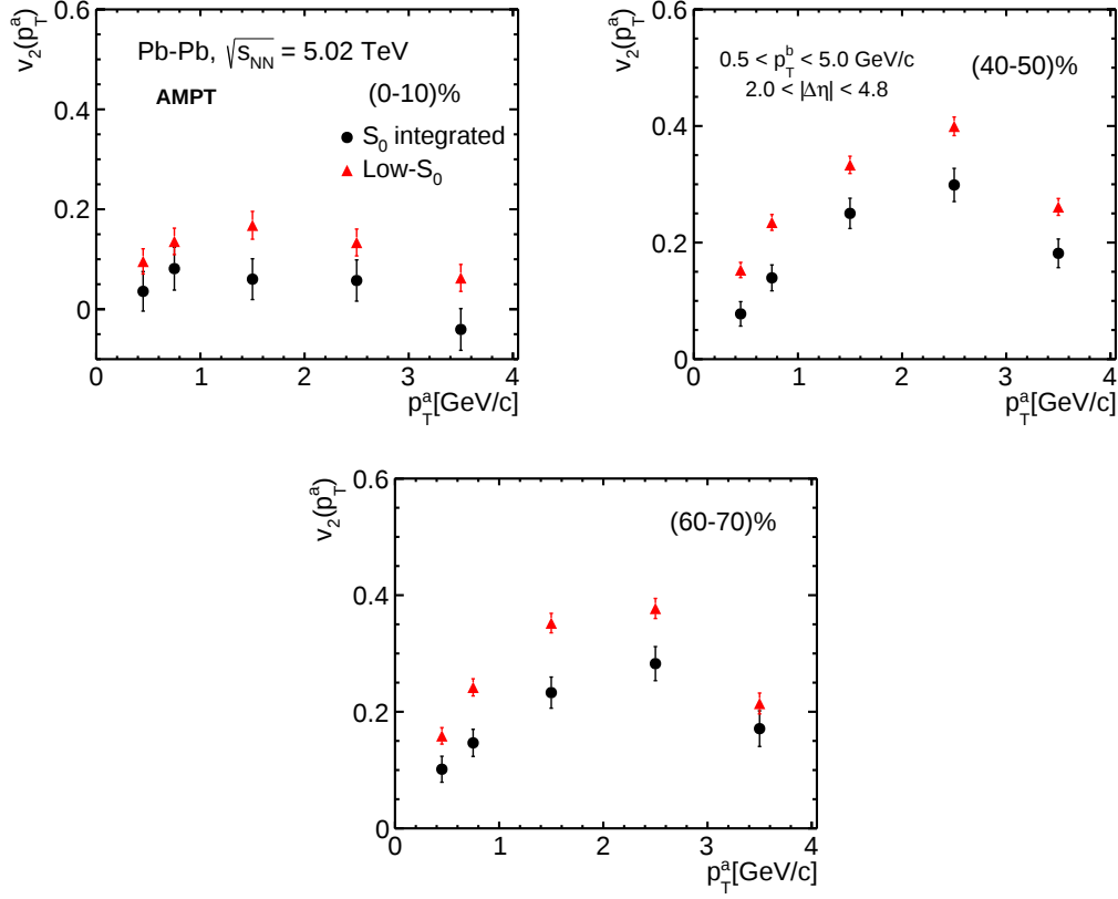
Figure 4.6: Spherocity dependence of single particle elliptic flow coefficient, v_2(p_T^a) , of all charged particles in (0-10)%, (40-50)% and (60-70)% central Pb-Pb collisions at \sqrt{s_{NN}} = 5.02 TeV from AMPT model [100].
