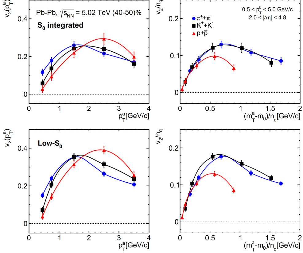
Figure 4.7: Left column shows the transverse momentum dependence of elliptic flow, v_2(p_T^a) , for \pi^+ + \pi^- , K^+ + K^- , and p + \bar{p} in S_0 -integrated (top panel) and low- S_0 (bottom panel) events in (40–50)% central Pb–Pb collisions at \sqrt{s_{NN}} = 5.02 TeV from AMPT model [114]. The right column shows the respective NCQ scaling behavior.
