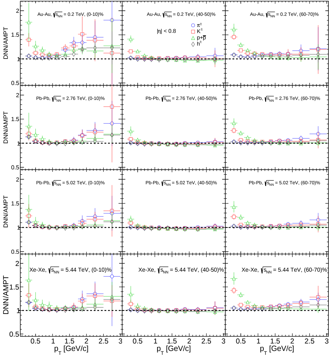
Figure 5.9: Ratio of DNN predictions to AMPT results for the transverse momentum dependence of elliptic flow for \pi^\pm , K^\pm , and p + \bar{p} , and all charged hadrons ( h^\pm ) [145].
