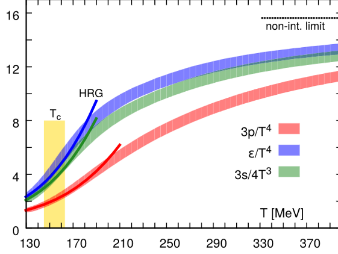
Figure 1.4: Lattice QCD predictions for the normalized pressure, energy density, and entropy density as a function of temperature at vanishing \mu_B . The solid lines show the predictions from the Hadron Resonance Gas (HRG) model [13].
