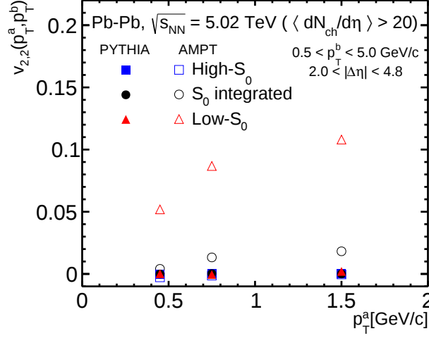
Figure 4.3: Transverse momentum ( p_T^a ) and spherocity dependence of two-particle elliptic flow coefficient ( v_{2,2}(p_T^a, p_T^b) ) in minimum bias Pb–Pb collisions at \sqrt{s_{NN}} = 5.02 TeV using PYTHIA8 (close markers) and AMPT (open markers) models [100]. Events are selected having \langle dN_{ch}/d\eta \rangle > 20 in mid-rapidity ( |\eta| < 0.8 ).
