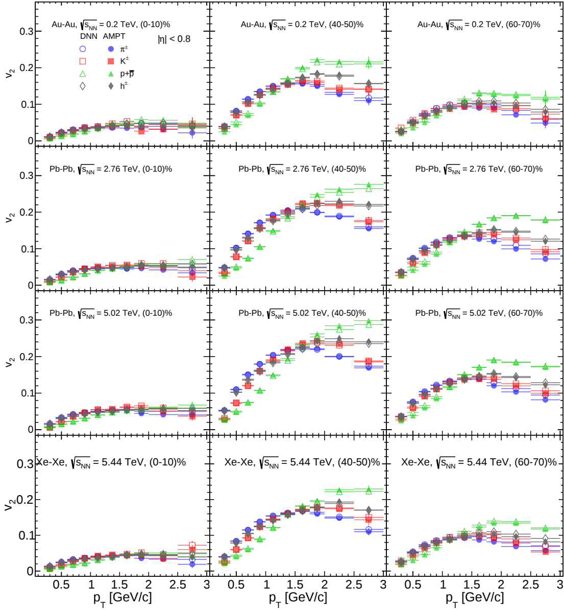
Figure 5.8: DNN predictions and AMPT results for the transverse momentum dependence of elliptic flow for \pi^\pm , K^\pm , and p+\bar{p} , and all charged hadrons ( h^\pm ) [145].
