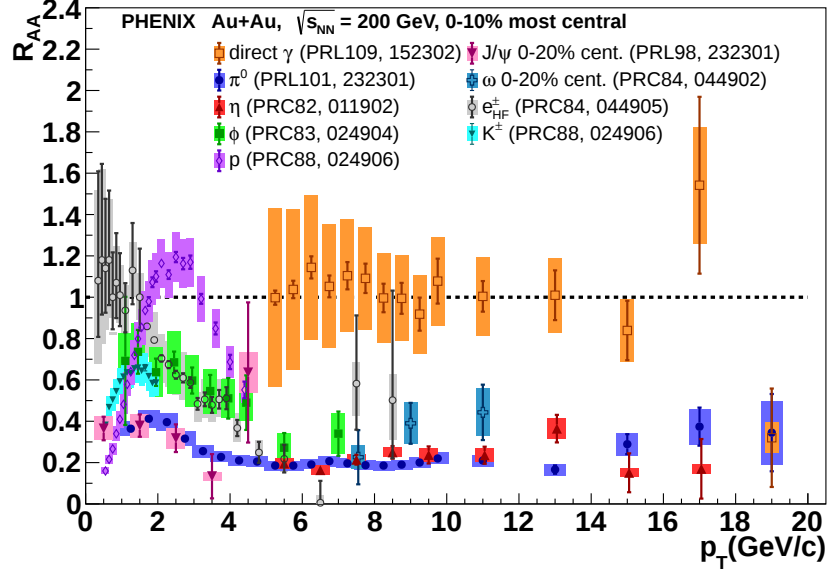
Figure 1.7: Transverse momentum dependence of nuclear modification factor for various particles in Au–Au collisions \sqrt{s_{NN}} = 200 GeV from the PHENIX experiment [32].
