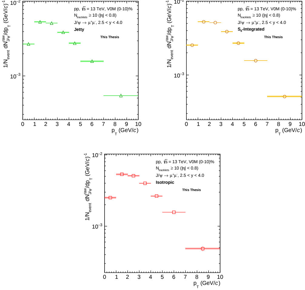
Figure 3.6: Event normalized raw p_T spectra of inclusive J/\psi integrated over 2.5 < y < 4.0 for the jetty, S_0 -integrated, and isotropic events in pp collisions at \sqrt{s} = 13 TeV in V0M (0 – 10)% centrality class.
