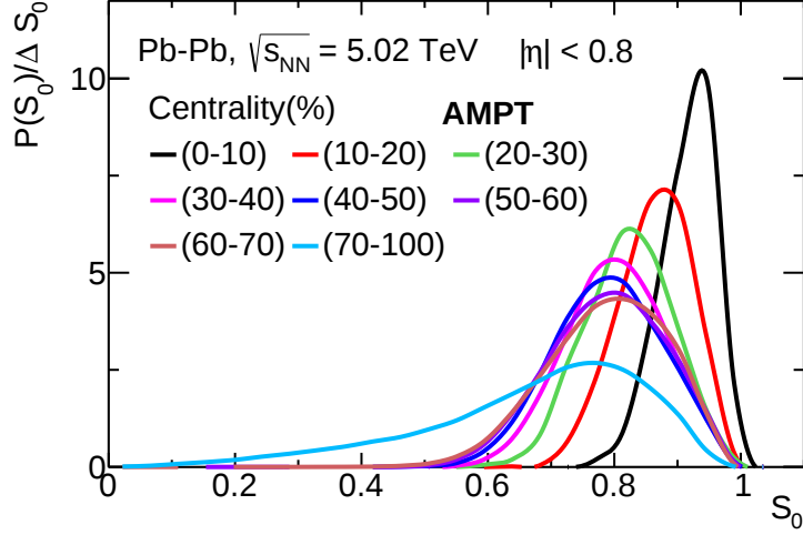
Figure 4.1: Centrality wise transverse sphericity ( S_0 ) distribution in Pb–Pb collisions at \sqrt{s_{\text{NN}}} = 5.02 TeV from AMPT model [100].
