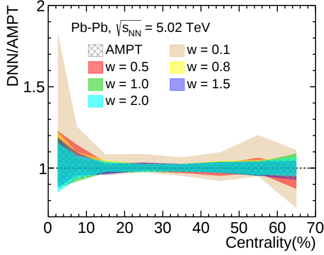
Figure 5.6: The DNN model predictions on a noisy dataset compared to the AMPT simulation without any noise. The smaller value of the parameter w corresponds to a greater noise in the dataset [144].
