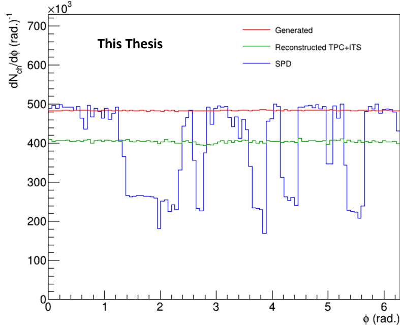
Figure 3.8: The azimuthal angle ( \phi ) distribution of the generated tracks (red), reconstructed tracks with ITS+TPC matching (green), and the tracklets from the SPD (blue) for the MC production LHC17f5 anchored to LHC16h.
