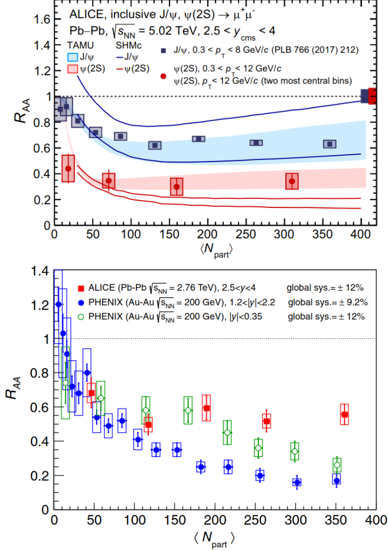
Figure 1.8: Top: The nuclear modification factor ( R_{AA} ) showing the suppression of J/\psi and \psi(2S) at the LHC [36]. Bottom: Inclusive J/\psi R_{AA} at the LHC compared to RHIC [39].
