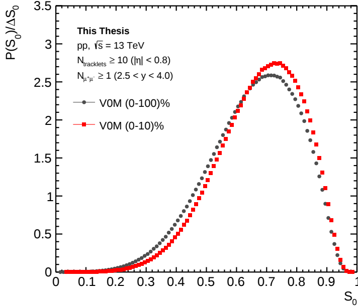
Figure 3.2: Normalized sphericity distribution measured with SPD tracklets in dimuon triggered events for V0M (0 – 100)% (black) and (0 – 10)% (red) multiplicity classes in pp collisions at \sqrt{s} = 13 TeV.
