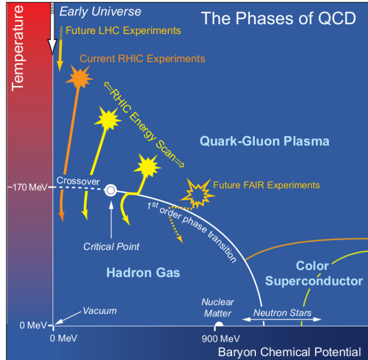
Figure 1.3: Conjectured QCD phase diagram [9].
