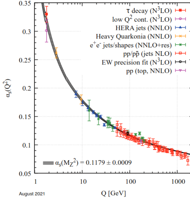
Figure 1.2: Running coupling constant \alpha_s(Q^2) plotted as a function of momentum transfer ( Q ), extracted using different degrees of QCD perturbation theory which are mentioned in the legend [8].
