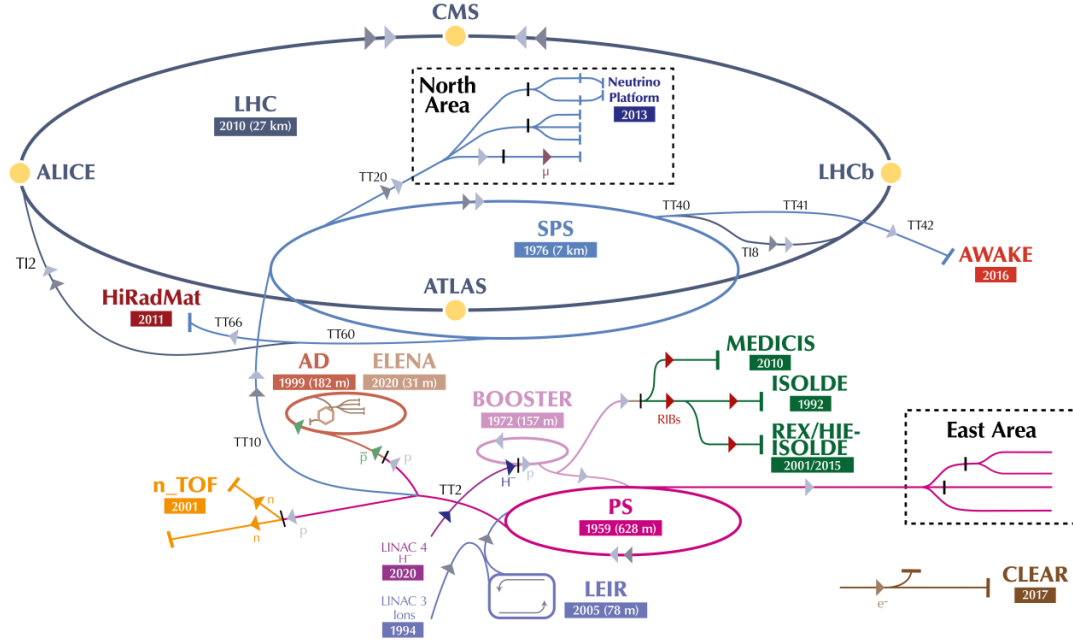
Figure 2.1: CERN accelerator complex showing the four major LHC experiments (ATLAS, ALICE, CMS, and LHCb). The Proton Synchrotron Booster (PSB), Proton Synchrotron (PS), and Super Proton Synchrotron (SPS) rings are also shown [54].
