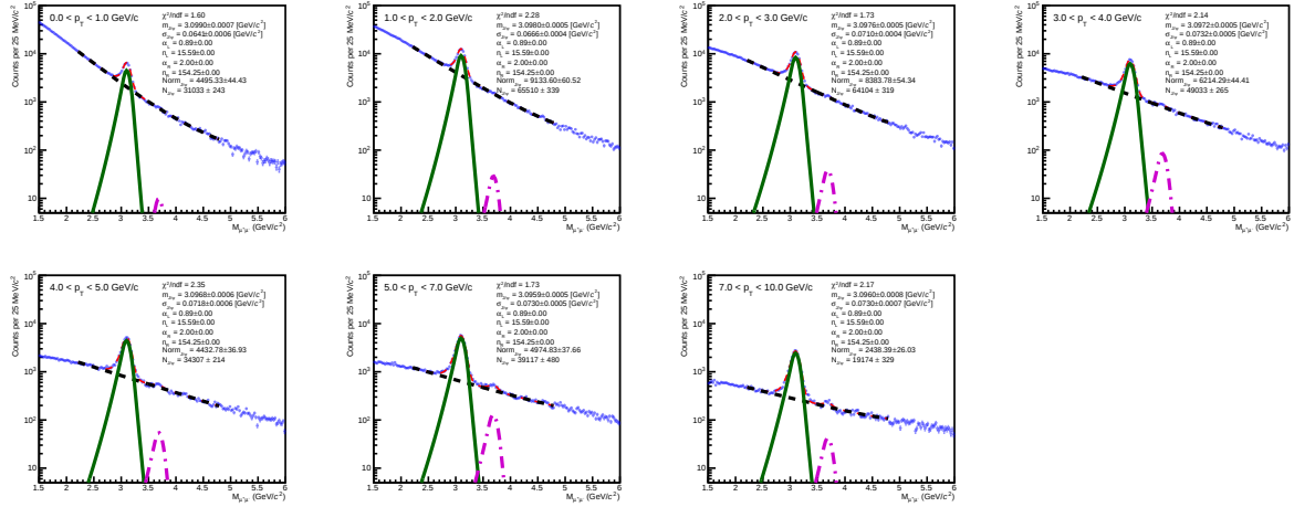
Figure 3.21: Yield extraction using CB2+CB2+DoubleExp fit function in fit range 2.2 < M_{\mu^+\mu^-} < 4.8 \text{ GeV}/c^2 for S_0 -integrated events.
