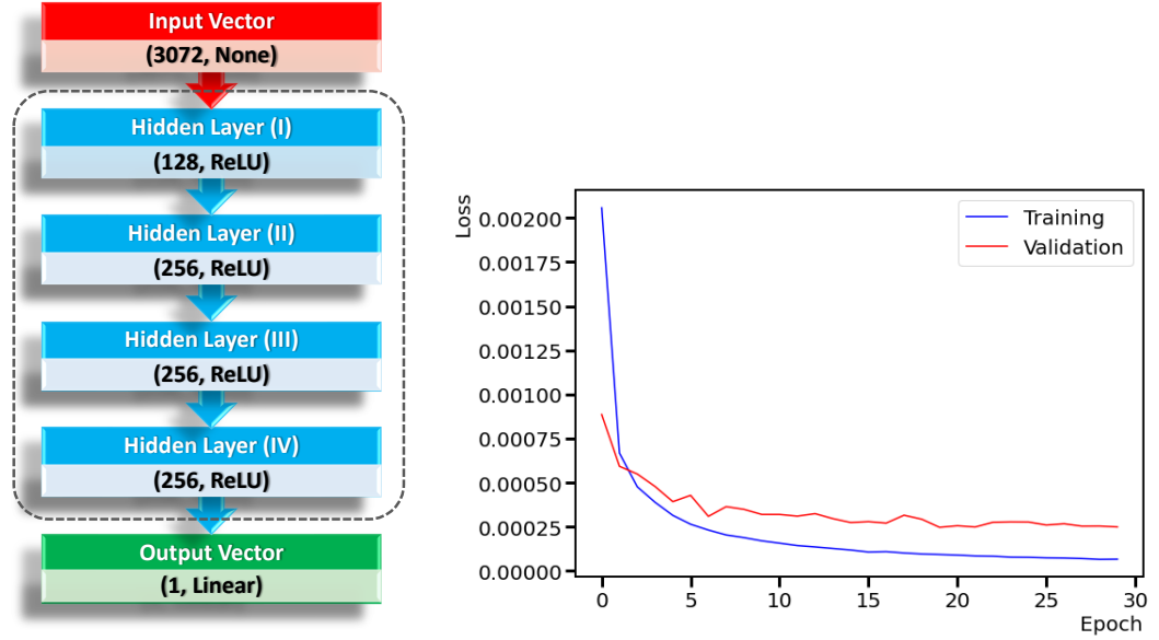
Figure 5.4: Left: Schematics of the deep neural network architecture with the number of nodes in each layer and the corresponding type of activation function mentioned. Right: Evolution of the mean squared loss function versus epoch size during the training and validation runs of the proposed deep neural network [144, 145].
