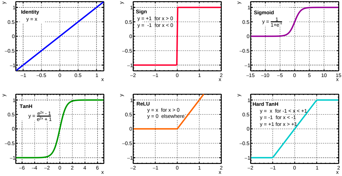
Figure 5.2: Definition and nature of a few popular activation functions.
