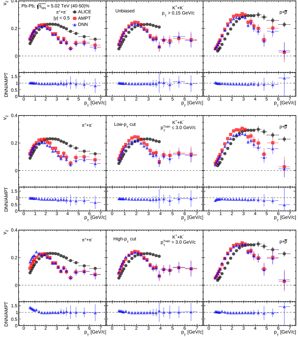
Figure 5.12: Effect of transverse-momentum-dependent training on the DNN predictions of identified particle elliptic flow. The results for (40 – 50)% central Pb–Pb collisions at \sqrt{s_{\text{NN}}} = 5.02 TeV with models trained on an unbiased (top), low- p_{\text{T}} (middle), and high- p_{\text{T}} (bottom) particle groups are presented [145]. The ALICE results are shown for comparison [171].
