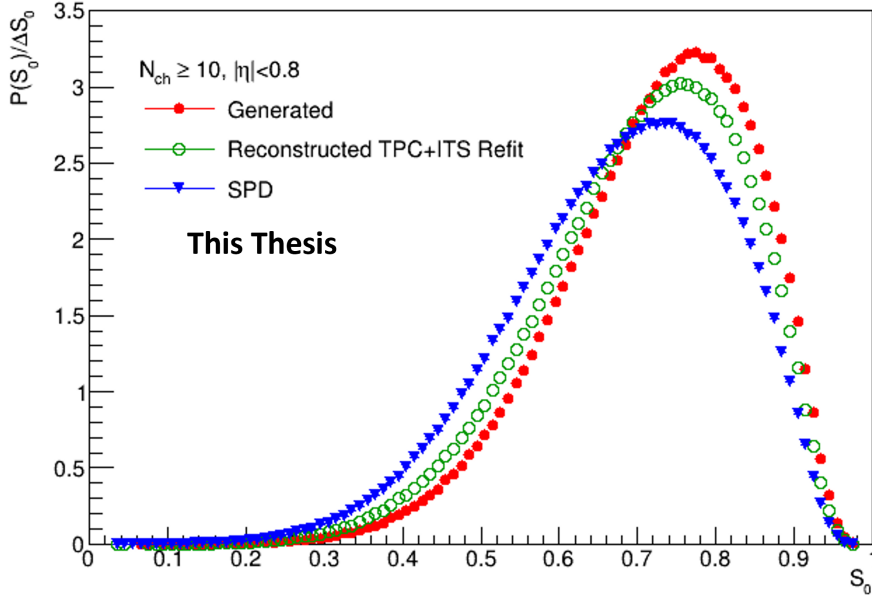
Figure 3.9: The sphericity distribution obtained using the generated (red), reconstructed tracks with ITS+TPS refit (green), and the SPD tracklets (blue) with N_{\text{ch}} \geq 10 in |\eta| < 0.8 for the V0M (0 – 10%) multiplicity class.
