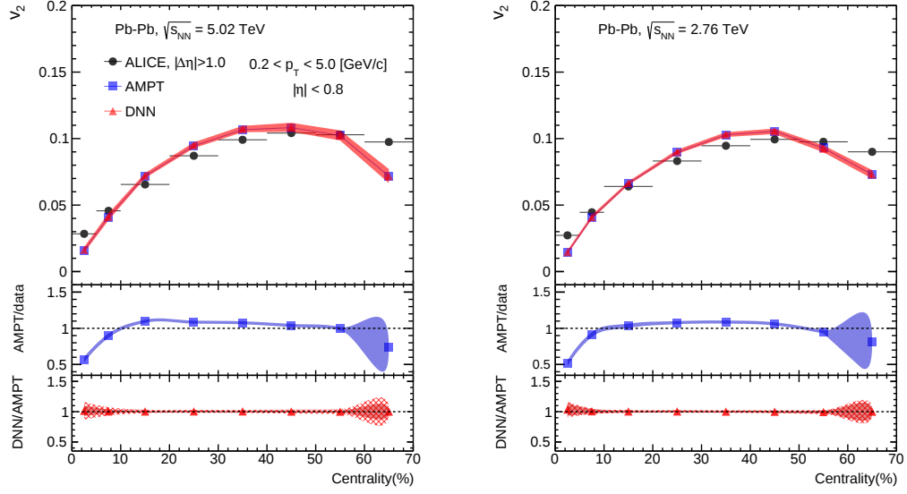
Figure 5.7: DNN predictions for the centrality dependence of p_T -integrated elliptic flow for Pb–Pb collisions at \sqrt{s_{NN}} = 2.76 and 5.02 TeV [144]. Results from AMPT simulation and ALICE [115] are shown for comparison.
