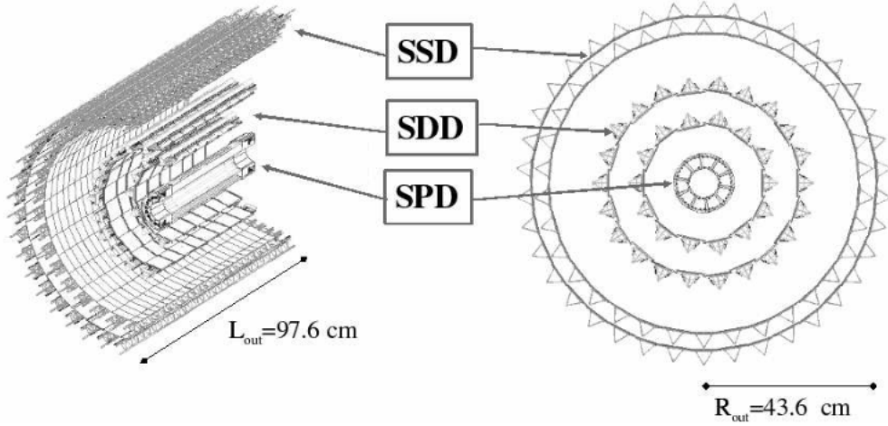
Figure 2.3: Schematics of the Inner Tracking System [53].
