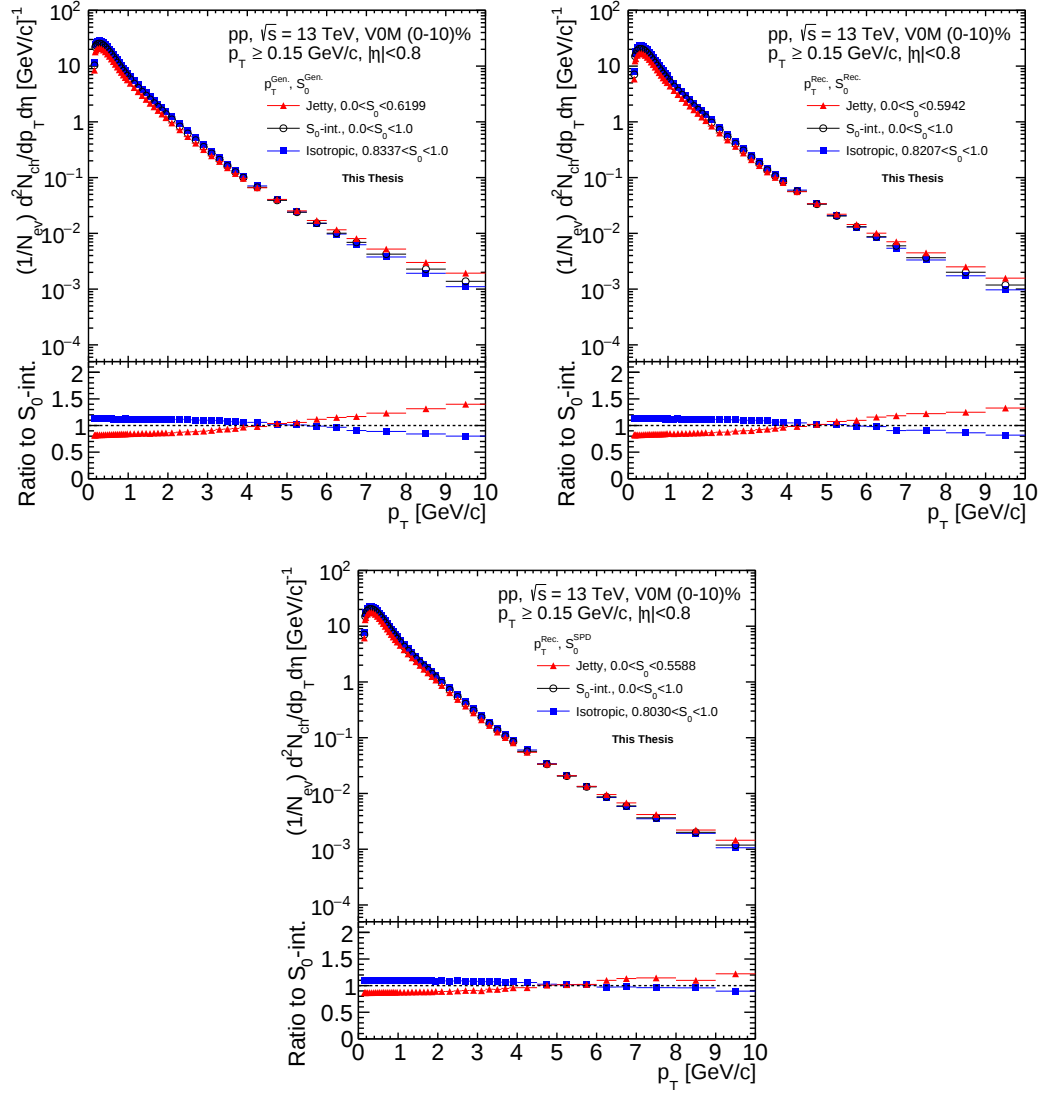
Figure 3.10: Transverse momentum ( p_T ) spectra of the global charged particles for jetty (red), S_0 -integrated (black), and isotropic (blue) events for the generated, reconstructed with ITS+TPC refit, and SPD are shown. The bottom panels show the ratio of jetty and isotropic spectra to the respective S_0 -integrated spectra.
