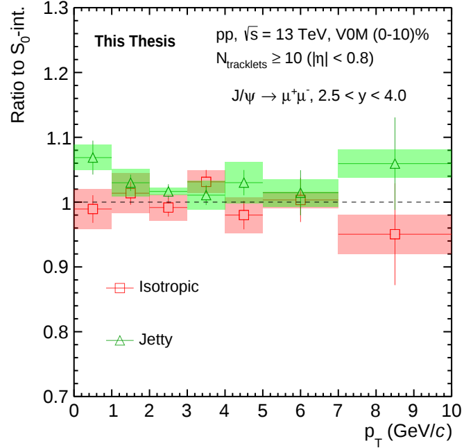
Figure 3.7: p_T -differential yield ratio of inclusive J/\psi in jetty to S_0 -integrated events (green) and isotropic to S_0 -integrated events (red), integrated over 2.5 < y < 4.0 in pp collisions at \sqrt{s} = 13 TeV in V0M (0 – 10)% centrality class.
