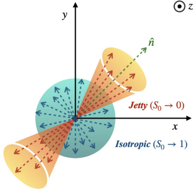
Figure 3.1: Pictorial representation of particle production in jetty and isotropic events in single pp collision on the transverse plane [69].
