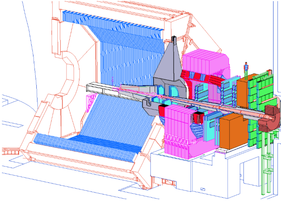
Figure 2.5: Location of the muon spectrometer and its major components in ALICE [53].
