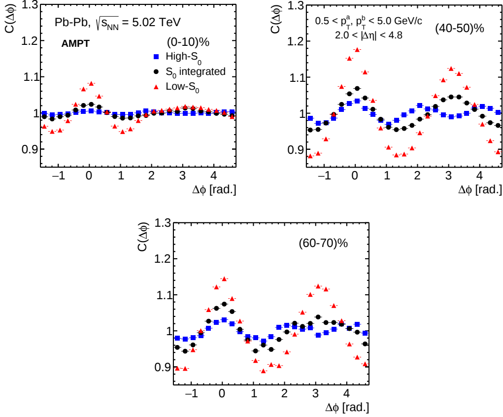
Figure 4.4: Spherocity dependence of two-particle azimuthal correlation function, C(\Delta\phi) , of all charged particles in (0–10)%, (40–50)% and (60–70)% central Pb–Pb collisions at \sqrt{s_{\text{NN}}} = 5.02 TeV from AMPT model [100].
