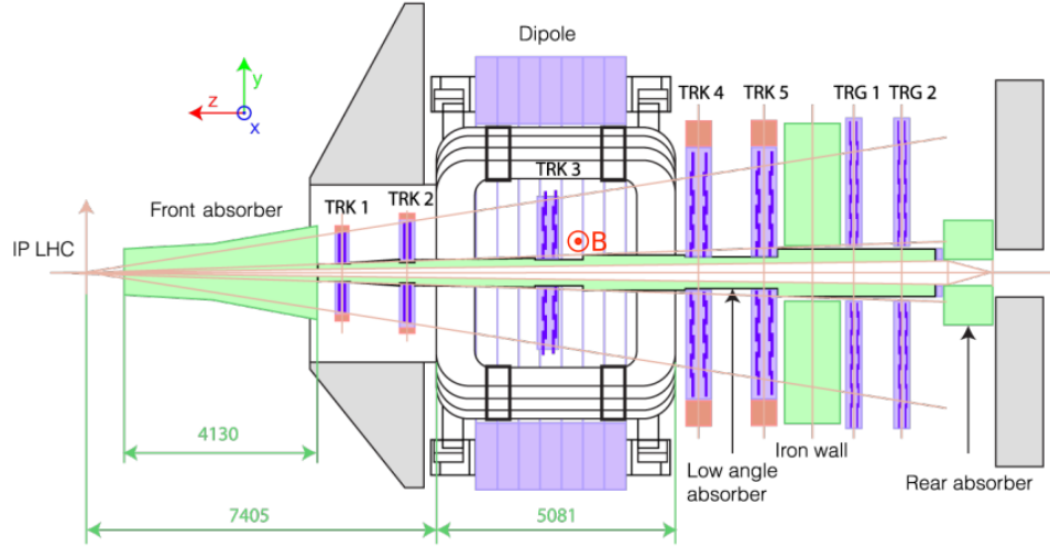
Figure 2.6: Schematics of the muon spectrometer with the layout of the front absorber, the tracking chamber, the dipole magnet, the trigger chamber, and the rear absorber [61].
