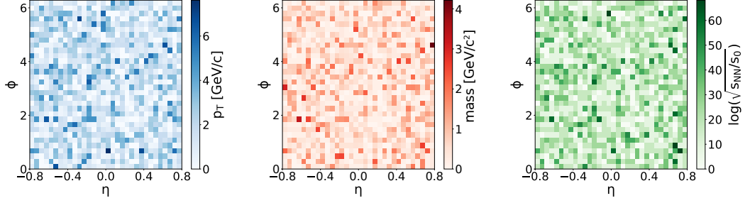
Figure 5.3: The (\eta-\phi) freezeout surface obtained from a single minimum bias Pb–Pb collision at \sqrt{s_{\text{NN}}} = 5.02 TeV from AMPT with 32 \times 32 bins each, displaying the three layers of input for the deep neural network [144].
