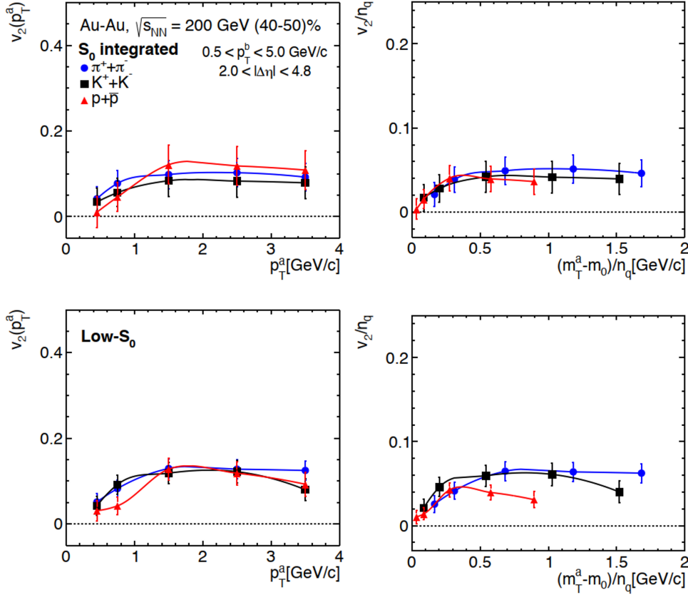
Figure 4.8: Left column shows the transverse momentum dependence of elliptic flow, v_2(p_T^a) , for \pi^+ + \pi^- , K^+ + K^- , and p + \bar{p} in S_0 -integrated (top panel) and low- S_0 (bottom panel) events in (40–50)% central Au–Au collisions at \sqrt{s_{NN}} = 200 GeV from AMPT model [114]. The right column shows the respective NCQ scaling behavior.
