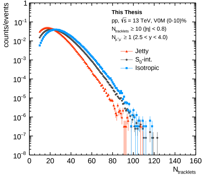
Figure 3.3: SPD tracklets distribution in jetty (red), S_0 -int. (black), and isotropic (blue) events in pp collisions at \sqrt{s} = 13 TeV in V0M (0 – 10)% centrality class.
