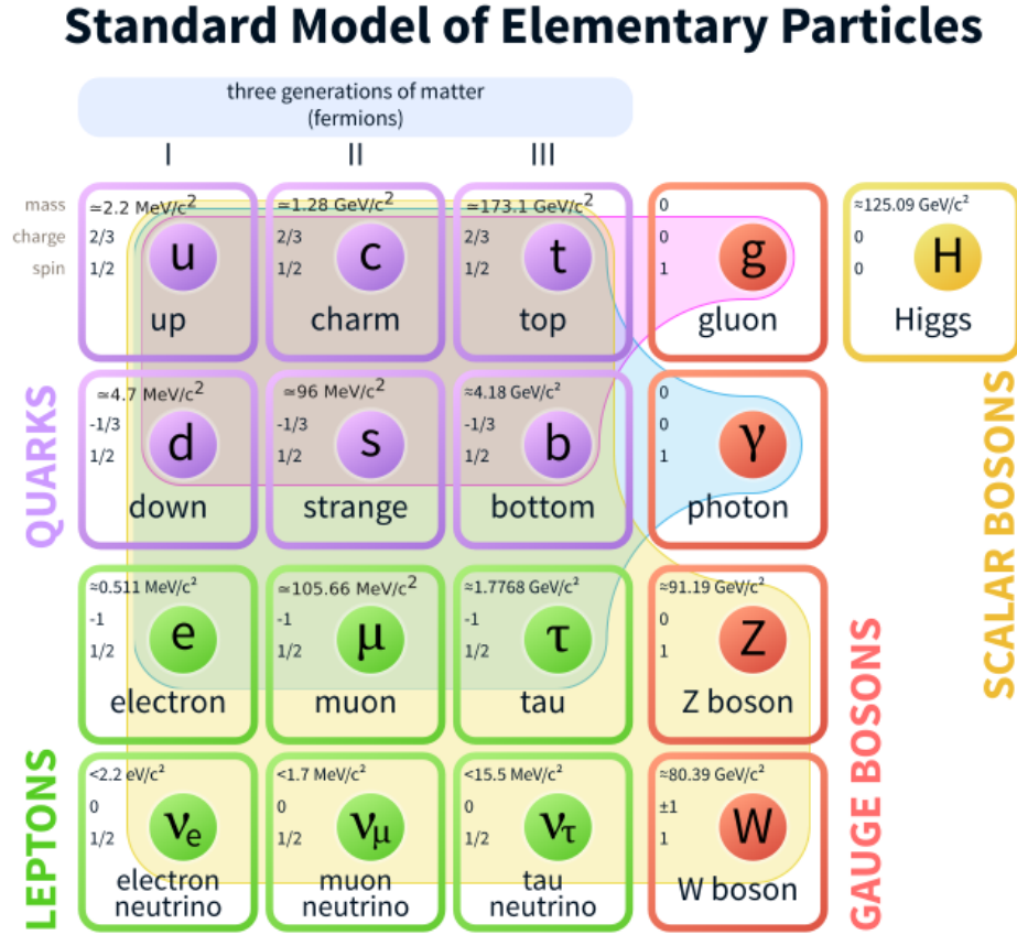
Figure 1.1: Schematic representation of the elementary particles in the Standard Model.
