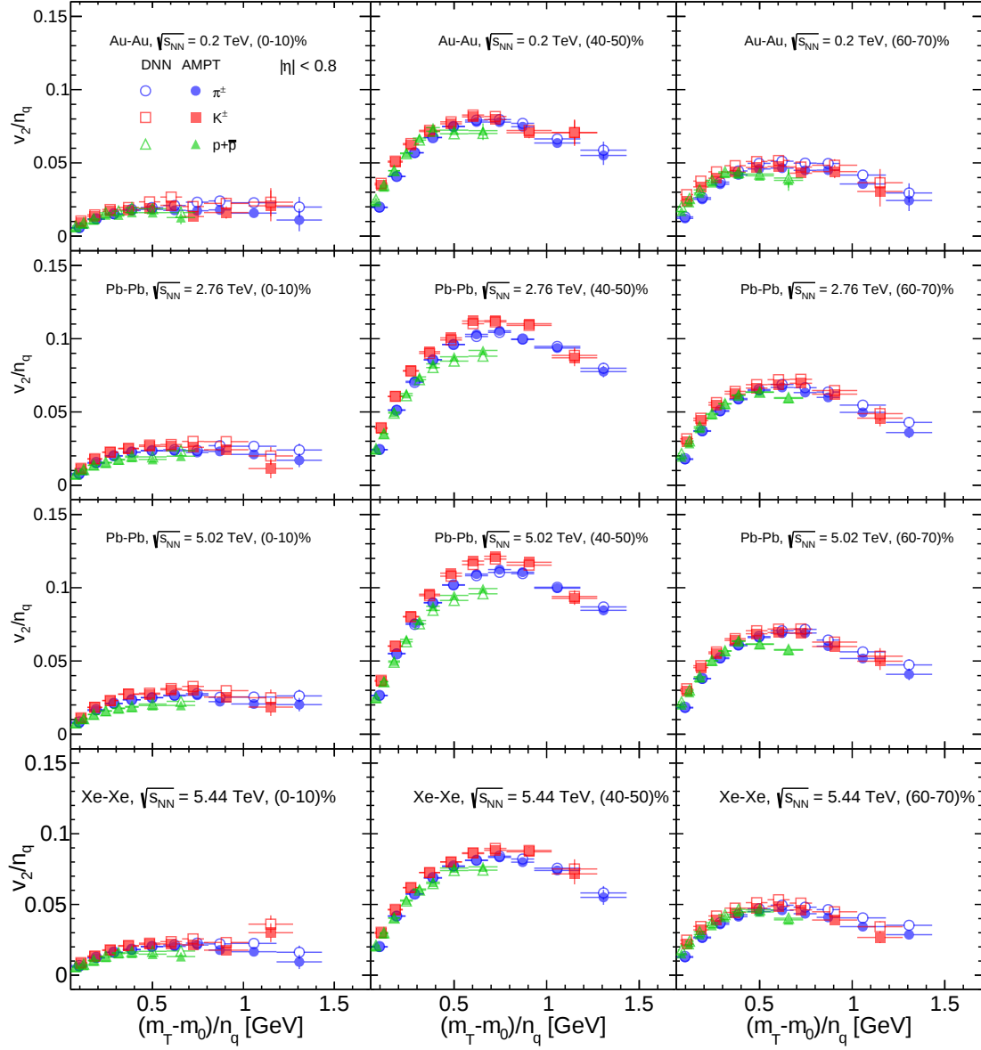
Figure 5.10: DNN predictions and AMPT results for the constituent quark number scaling in different centrality classes in different collision systems from RHIC to LHC energies [145].
