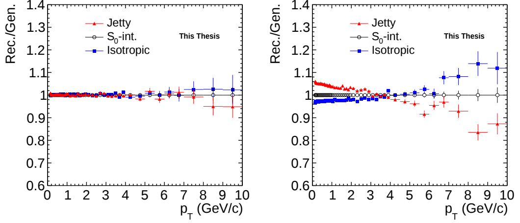
Figure 3.11: Ratio of reconstructed to generated p_T spectra for jetty (red), S_0 -integrated (black), and isotropic (blue) events. The event selection is performed based on the estimated S_0 using the reconstructed ITS+TPC tracks and SPD tracklets, on the left and right plots, respectively.
