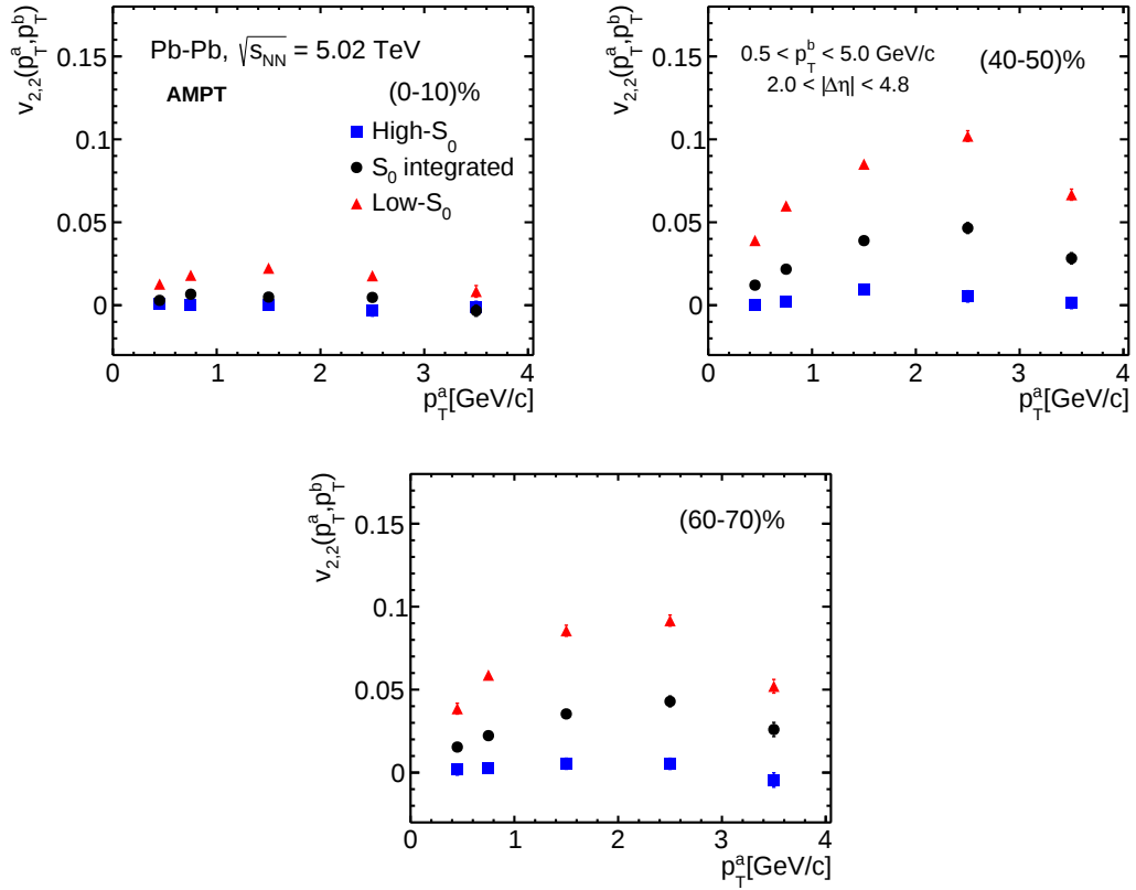
Figure 4.5: Sphericity dependence of two-particle elliptic flow coefficient, v_{2,2}(p_T^a, p_T^b) , of all charged particles in (0–10)%, (40–50)% and (60–70)% central Pb–Pb collisions at \sqrt{s_{NN}} = 5.02 TeV from AMPT model [100].
