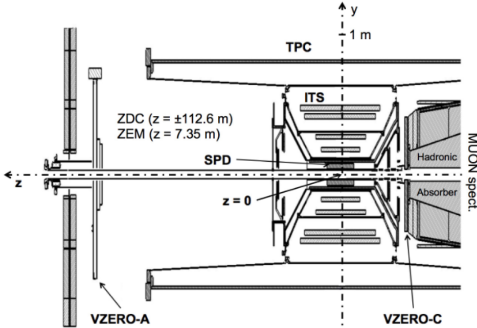
Figure 2.4: Placement of ALICE V0 detectors on either side of the interaction point [60].
