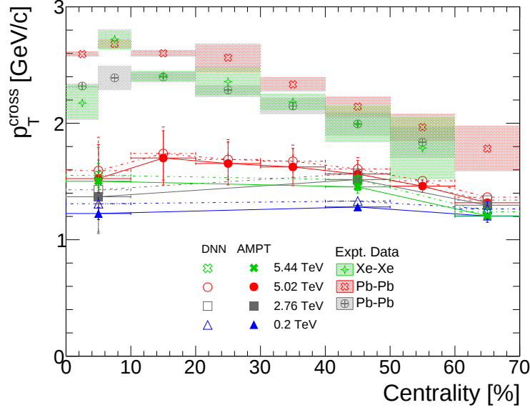
Figure 5.11: The baryon-meson elliptic flow crossing point, p_T^{\text{cross}} , at the intermediate p_T regime plotted against the centrality of the collisions [145]. The ALICE results are obtained from Refs. [111, 171, 172].
