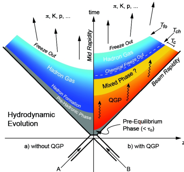
Figure 1.5: Schematic representation of the spacetime evolution of relativistic hadronic and nuclear collisions [18].
