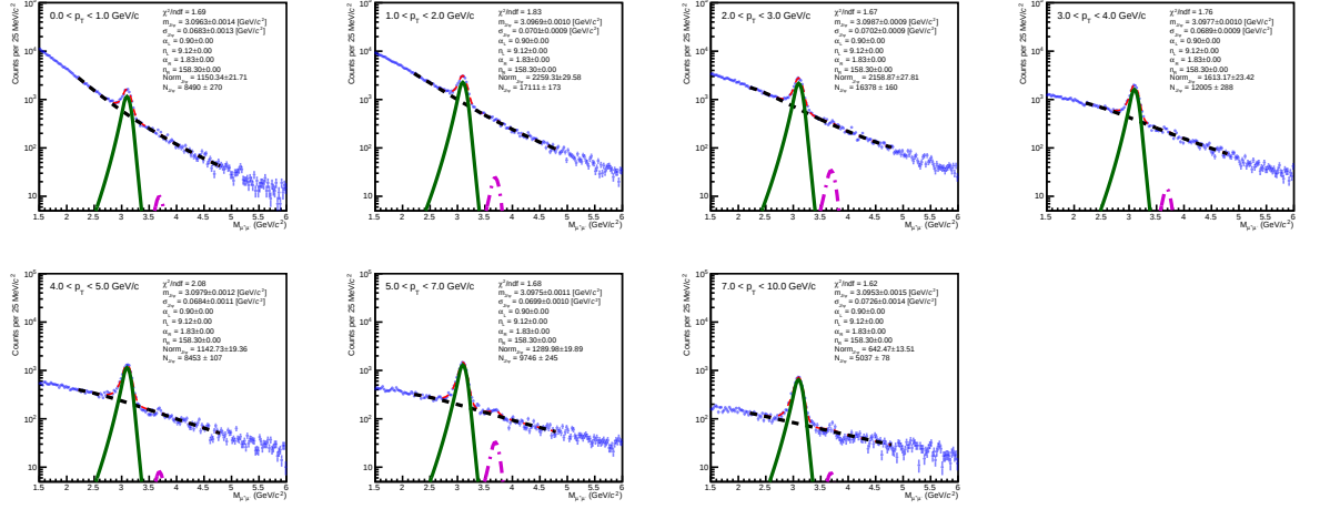
Figure 3.16: Yield extraction using CB2+CB2+VWG fit function in fit range 2.2 < M_{\mu+\mu-} < 4.8 \text{ GeV}/c^2 for jetty events.
