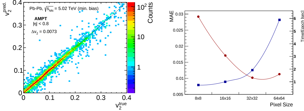
Figure 5.5: Left: Event-by-event predictions versus the true values of elliptic flow plotted for 10K minimum bias Pb–Pb collisions at \sqrt{s_{\text{NN}}} = 5.02 TeV from the AMPT model. Right: Mean absolute error on testing data and time/epoch in seconds during training for various input bin size [144, 145]
