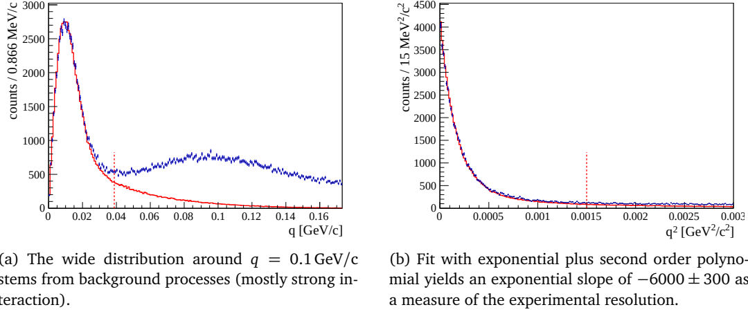
Figure 4.6: \pi^- \gamma momentum transfer to the nucleus
