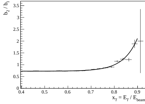
Figure 7.8: determination of the b_2/b_1 constraint from \pi \gamma simulation
