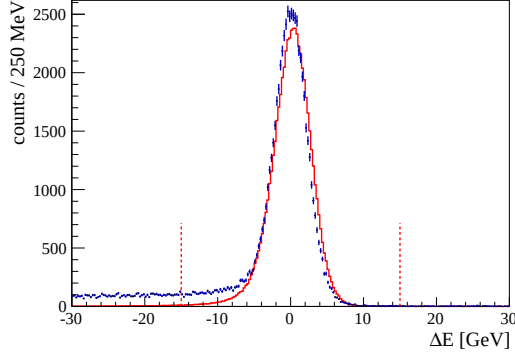
Figure 4.12: energy balance of \pi^-\gamma^* \rightarrow \pi^-\gamma
