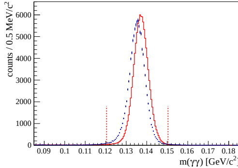
(a) combined mass of the event's two highest-energetic photons, Gaussian fit yields \sigma = 3.8 \text{ MeV}
