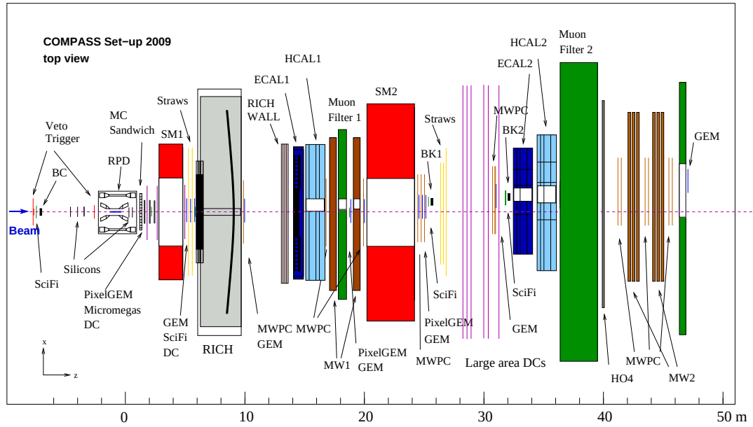
Figure 2.2: top view of the COMPASS spectrometer, cut at beam axis, from [COM12]
