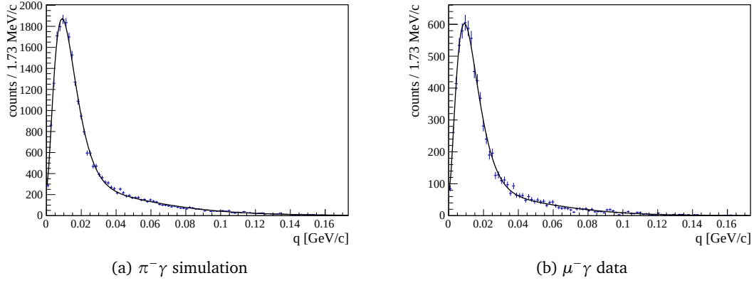
Figure 7.6: tests of Primakoff signal shape S(q)
