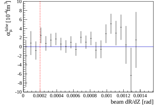
(b) false muon polarizability obtained in slices of beam divergence
