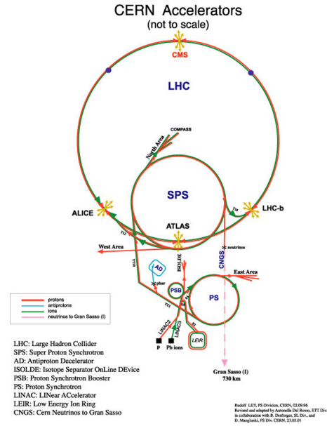
Figure 2.1: overview of CERN accelerators (not to scale), from [CER]
