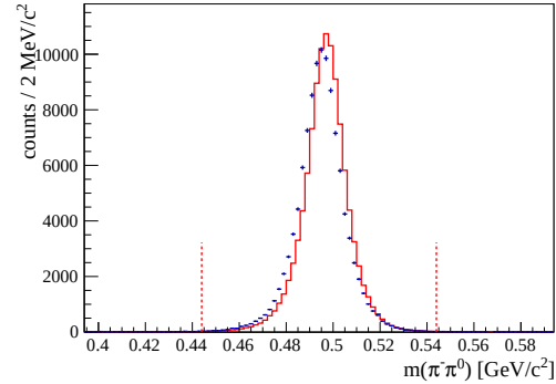
(b) combined mass of \pi^- and \pi^0 , Gaussian fit to the center of the distribution yields \sigma = 9 \text{ MeV}
