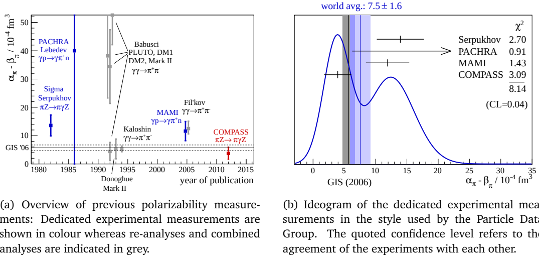
Figure 8.2: Previous measurements of \alpha_\pi - \beta_\pi : The ChPT prediction by [GIS06] and its error margins are indicated by the solid/dashed lines and the grey band respectively. A more detailed description of the plots is given in Section 1.1 together with the corresponding plots before the COMPASS measurement.
