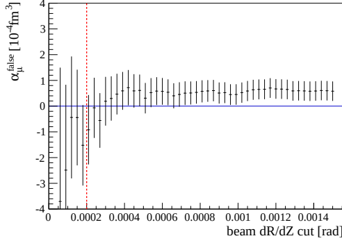
(a) false muon polarizability depending on beam divergence cut
