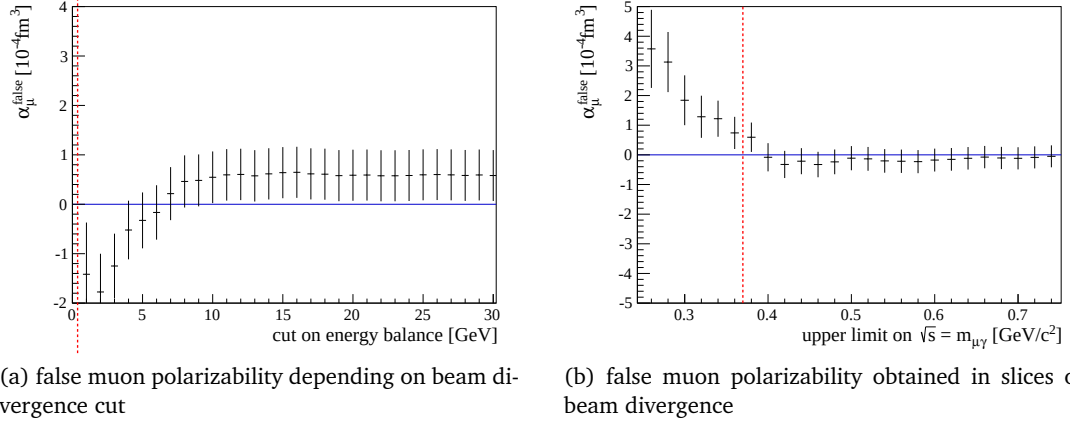
Figure A.3: Studies of false muon polarizability: For comparison the cut on hadron beam divergence is indicated by the red dashed line.
