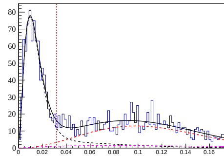
(b) 0.775 < x_\gamma < 0.8
