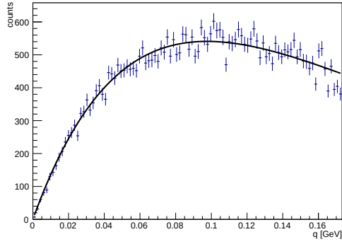
Figure 7.7: \pi^- \pi^0 simulation fitted with B_\pi(q)
