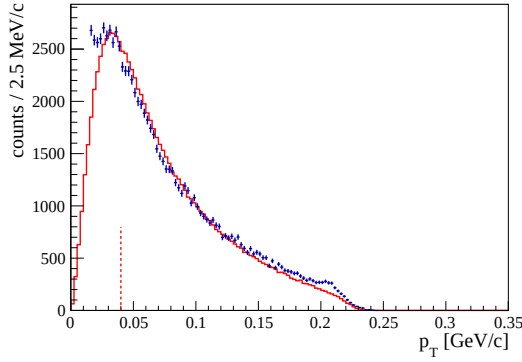
Figure 4.8: Transverse momentum of scattered pion. Around 0.21 GeV/c a small contribution of \pi^- e^- scattering is visible, cf. Section 7.1. The distribution is cut around 0.22 GeV/c due the indirect effect of the cut on the final state mass.
