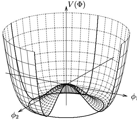
Figure 1.1: The potential of the field \Phi [49]: The set of minima of the potential is a circle in the complex plane. By choosing one minimum to be the vacuum expectation value the symmetry of \Phi is broken spontaneously.
