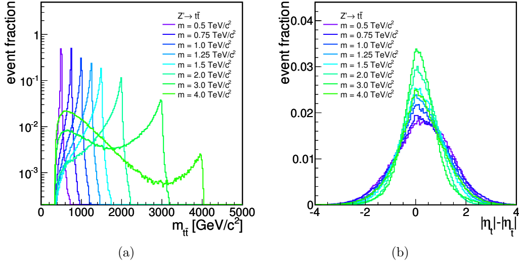
Figure 3.5: Comparison of the distribution of the invariant mass spectrum of the t\bar{t} system (a) and of |\eta_t| - |\eta_{\bar{t}}| (b) in simulated Z' \rightarrow t\bar{t} events for several Z' boson masses.
