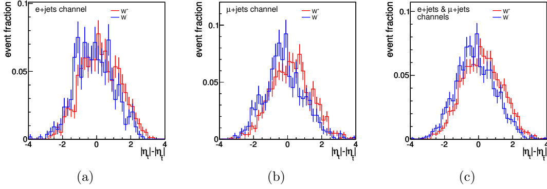
Figure 5.9: Distribution of |\eta_t| - |\eta_\ell| in W+jets Monte Carlo events with positively and negatively charged leptons after the final selection in the electron+jets channel (a), the muon+jets channel (b), and both channels combined (c).
