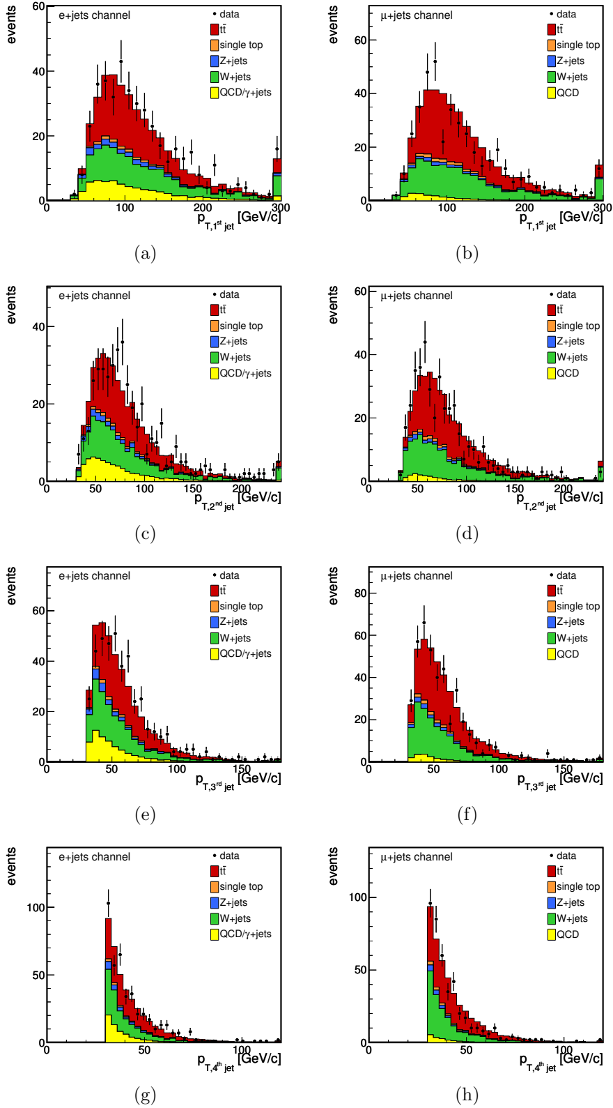
Figure 5.1: Data to Monte Carlo comparison of the transverse momentum p_T of the four leading jets in the electron+jets channel (a,c,e,g) and in the muon+jets channel (b,d,f,h). Jets are ordered by their p_T from higher to lower values. Only the QCD multi-jet production is modelled from data. All templates are normalised to the fit result of the cross section measurement [23].
