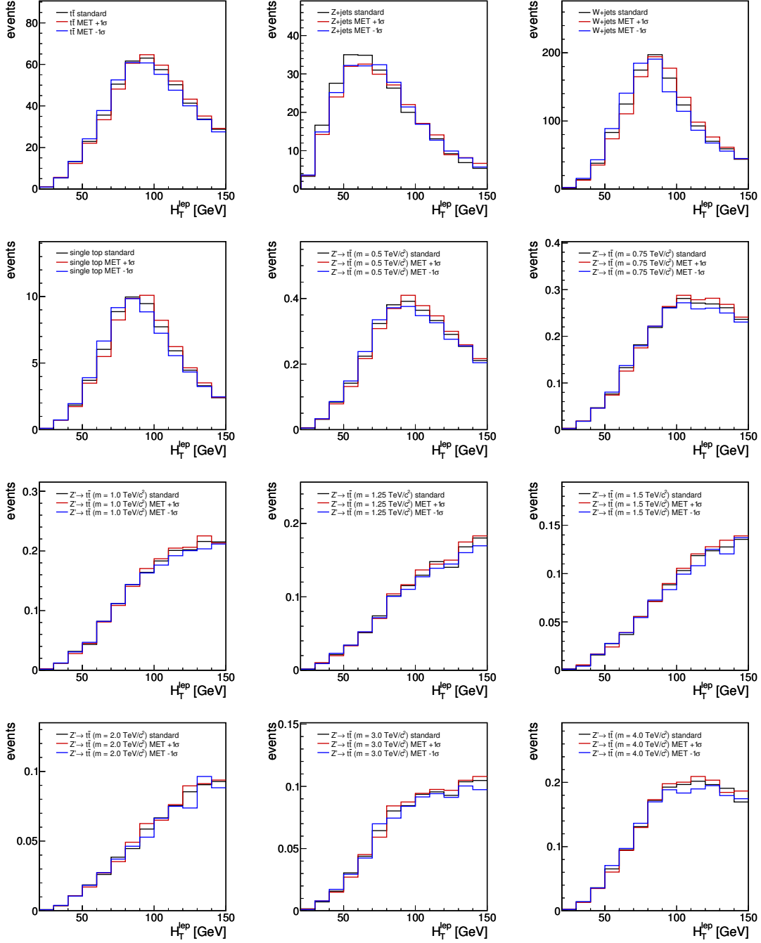
Figure A.9: Impact of varying the unclustered energy contributions to E_T on the shape and rate of H_T^{\text{lep}} after the final selection with H_T^{\text{lep}} < 150 GeV. The Z' \rightarrow t\bar{t} signal samples are normalised to an arbitrary cross section of 1 pb.
