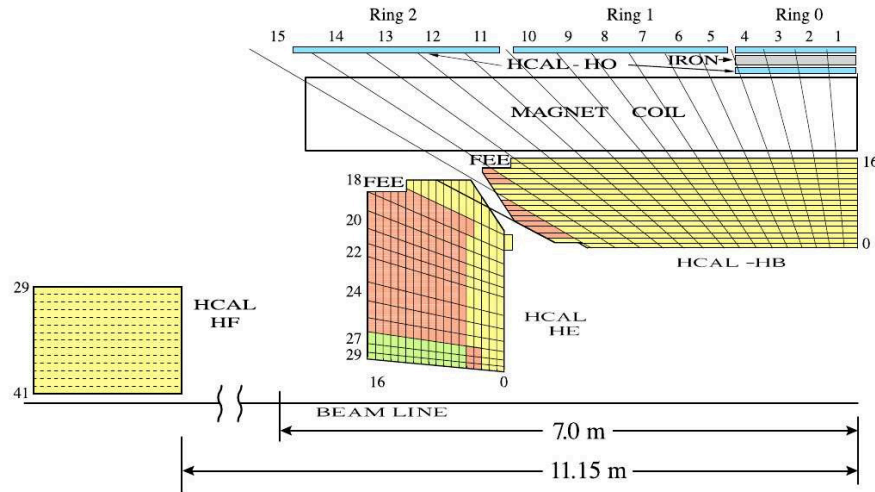
Figure 2.7: Transverse view through one quarter of the CMS HCAL [126] showing the HCAL barrel (HB), the HCAL endcap (HE), and the HCAL forward (HF). The HCAL outer (HO) is placed outside the coil of the CMS solenoid. The label FEE indicates the position of the front-end read-out electronics.
