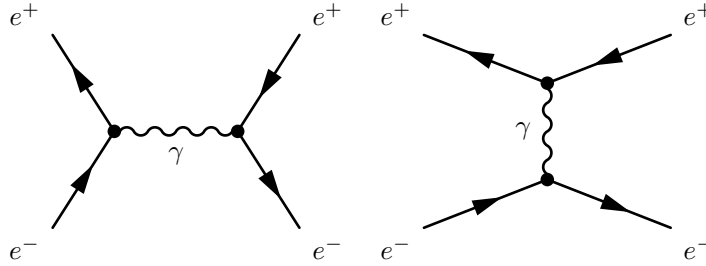
Figure 1.2: The leading order Feynman diagrams for the QED process e^+e^- \rightarrow e^+e^- .
