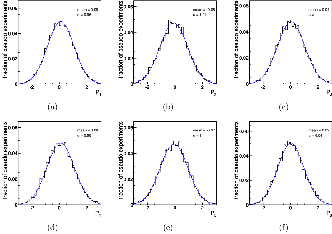
Figure 5.23: Pull distributions in each bins for the unfolding performed with TRUEE in pseudo experiments approximated with Gaussian functions. Given are the fitted mean and width ( \sigma ) of the respective Gaussian.
