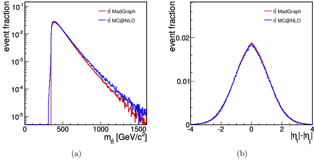
Figure 3.3: Comparison of the distribution of the invariant mass spectrum of the t\bar{t} system (a) and of |\eta_t| - |\eta_{\bar{t}}| (b) in top quark pair events generated with MADGRAPH/MadEvent and MC@NLO.
