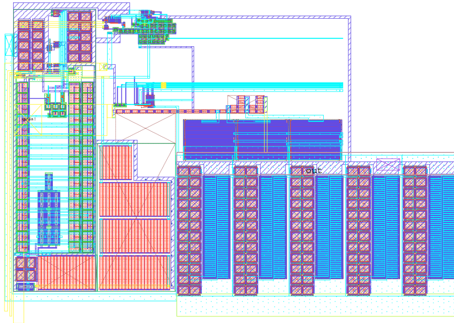
Abbildung 7.9: Layout des FE-I2.1-Linear-Regulators
