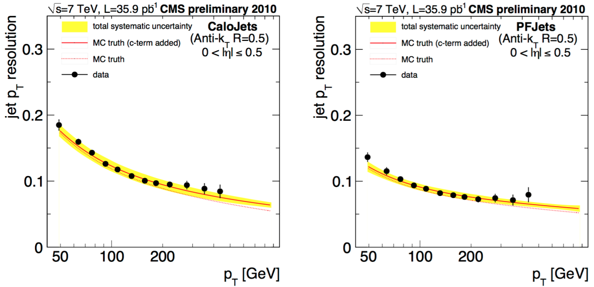
Figure 2.16: Jet transverse momentum resolution measured in Monte-Carlo simulation and 2010 data, for calo-jets (left) and Particle-Flow jets (right) [129]
