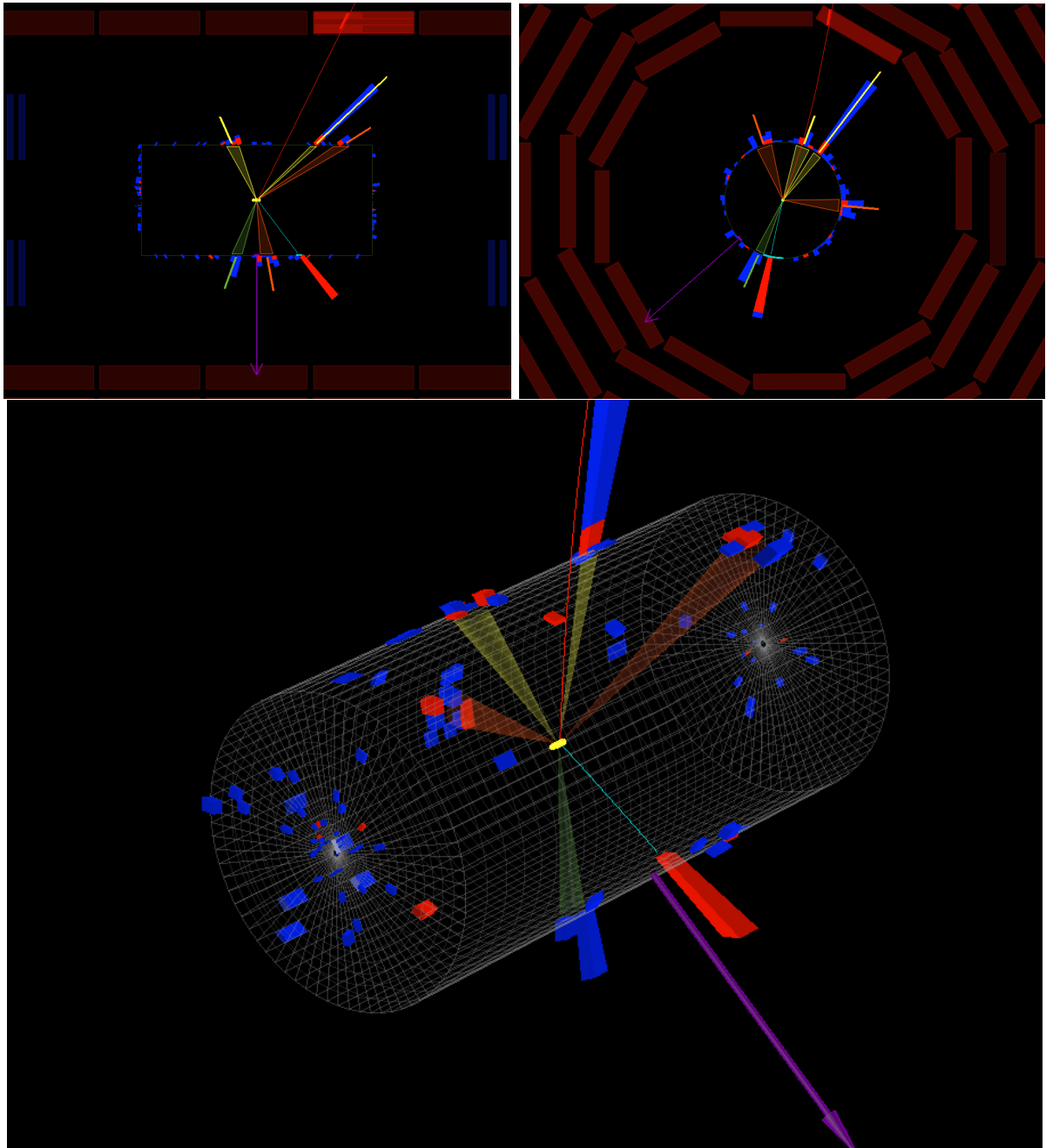
Figure 5.8: Event display of an event entering the 2\ell_{ss} + 1\tau_h category in 2016 data. The red (blue) rectangles correspond to ECAL (HCAL) energy deposits. The red (cyan) line represents a reconstructed muon (electron) and the green shaded area a reconstructed \tau_h . The orange shaded areas correspond to reconstructed jets identified as b -jets while the yellow shaded areas are for other jets. The purple arrow represents the E_T^{miss} .
