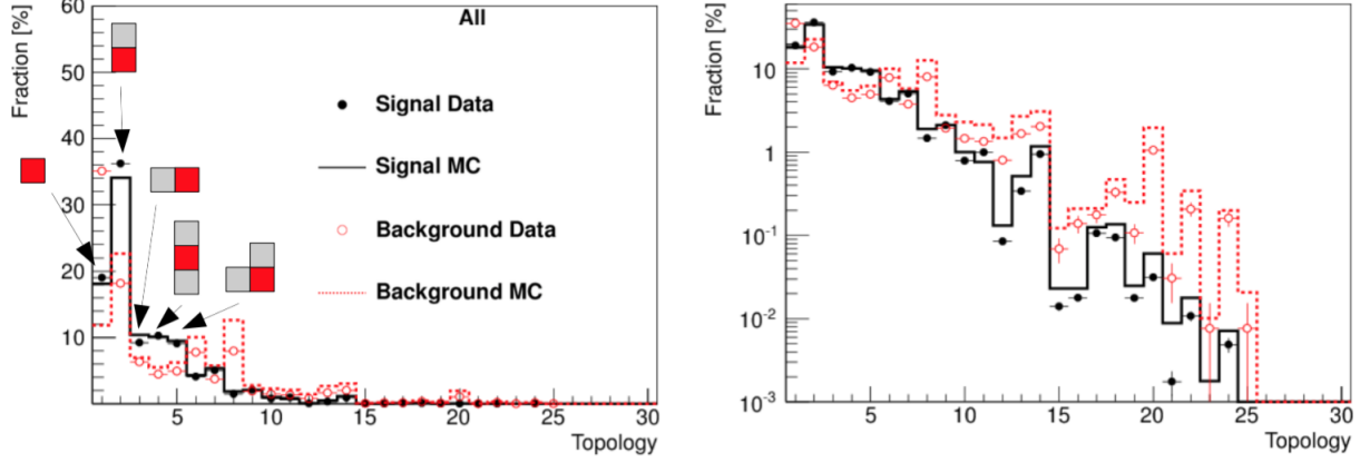
Figure 3.8: Distribution of the shapes obtained with the dynamic clustering algorithm for real electrons (signal) and for the background, in 8 TeV data and in Monte-Carlo simulation, in linear scale (left) and logarithmic scale (right) [140]
