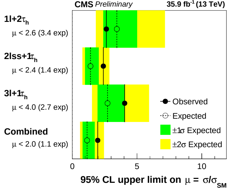
Figure 5.11: 95% CL upper limits on the t\bar{t}H signal rate, obtained in each of the categories 2\ell ss + 1\tau_h , 3\ell + 1\tau_h , and 1\ell + 2\tau_h individually and for the combination of all three event categories. The expected limits are computed for the background-only ( \mu = 0 ) hypothesis.
