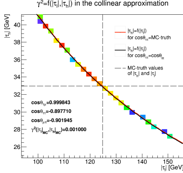
Figure A.2: Region where \gamma^2 > 0 (colored region, the color scale corresponding to the value of \gamma^2 ) for a single VBF event in the (|\vec{\tau}|, |\vec{\tau}_h|) space. The red line corresponds to the function |\vec{\tau}_h| = f(|\vec{\tau}_l|) determined from Eq. (A.28) using m_{\tau\bar{\tau}} = 125 GeV and the true value of \cos\theta_{\tau\bar{\tau}} , while for the black line \cos\theta_{\tau\bar{\tau}} = \cos\theta_{\ell\pi} was used.
