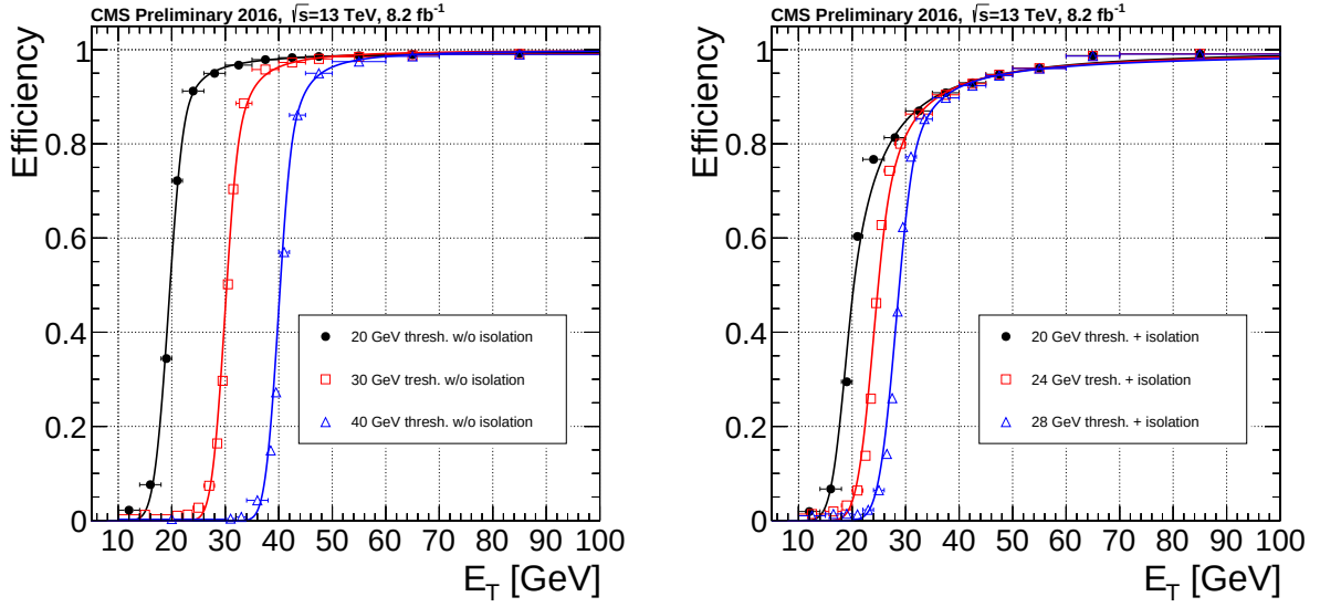
Figure 3.24: L1EG turn-on curves measured in 2016 data for different thresholds without isolation requirement (left) and with isolation requirement (right). The lines correspond to the result of an unbinned maximum likelihood with a Crystal-Ball integral function.
