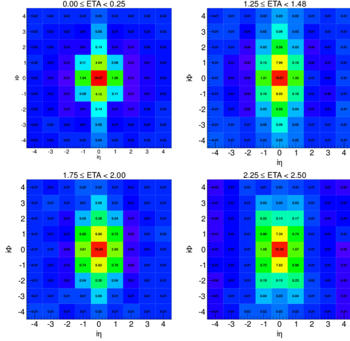
Figure 3.6: "Footprints" of the energy deposit from electrons in different \eta regions of the detector, observed in Run 1 data. The granularity shown here corresponds to the trigger towers ( 5 \times 5 ECAL crystals). The z axis represents the fraction of energy deposited by the electron in each tower around the maximum. [140]
