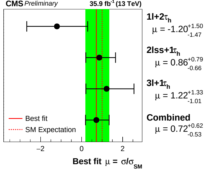
Figure 5.12: Signal rates \mu , in units of the SM t\bar{t}H production rate, measured in each of the categories 1\ell + 2\tau_h , 2\ell_{ss} + 1\tau_h and 3\ell + 1\tau_h individually and for the combination of all three categories. The expected signal rate is obtained using an Asimov dataset with \mu = 1 .
