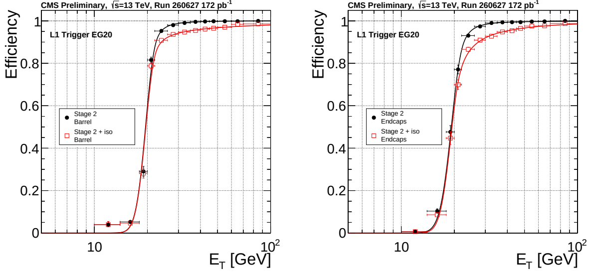
Figure 3.19: L1EG turn-on curves for a 20 GeV-threshold obtained in 2015 data with the re-optimized set of L1EG parameters in the barrel (left) and in the endcaps (right), without (black) and with (red) isolation requirement. The lines correspond to the result of an unbinned maximum likelihood with a Crystal-Ball integral function.
