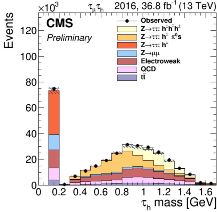
Figure 1.16: Observed and predicted distributions for the visible \tau_h mass, m_{vis}^{\tau_h} , for events with a reconstructed \mu and \tau_h in CMS data. The Z \rightarrow \tau\tau contribution is split according to its reconstructed decay mode. The mass distribution of the \tau_h built from one charged hadron and photons peaks around the mass of the intermediate \rho(770) resonance, while the one for \tau_h reconstructed from three charged hadrons peaks around the mass of the intermediate a_1(1200) resonance. By construction, the \tau_h built from one charged hadron and no photon are reconstructed with the \pi^\pm mass and represent the main contribution of the first bin. [64]
