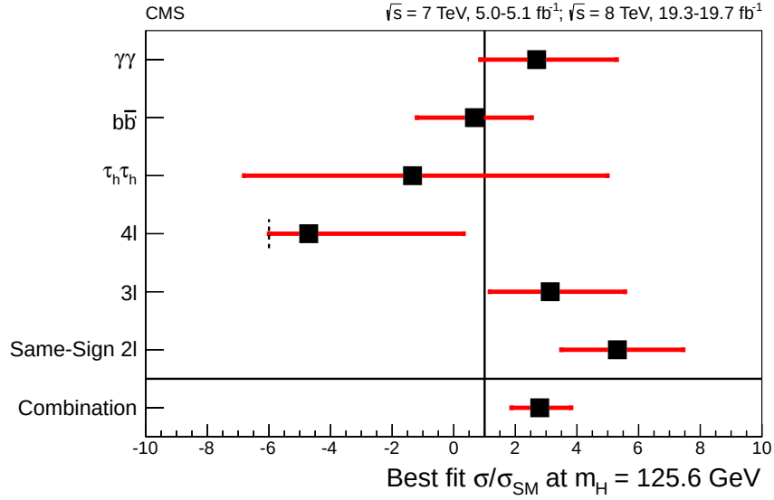
Figure 1.10: Best-fit values of \mu = \sigma/\sigma_{\text{SM}} for the t\bar{t}H process at m_H = 125.6 GeV, in each individual t\bar{t}H channel and for all channels combined [49]
