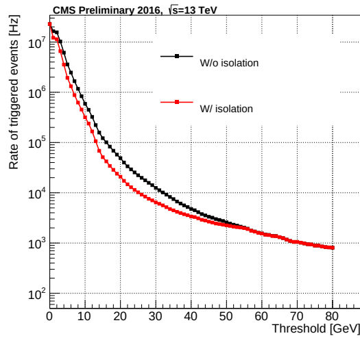
Figure 3.25: Rate of triggered events from ZeroBias data from 2016 run with initial luminosity of 7.2 \times 10^{33} \text{cm}^{-2} \text{s}^{-1} , without isolation requirement (black) and with isolation requirement (red). The lowest unprescaled SingleEG thresholds in that run were SingleEG40 (4.8 kHz) and SingleIsoEG24 (11.4 kHz).
