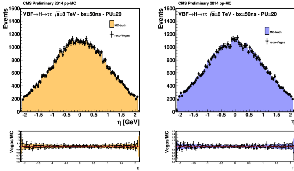
Figure 4.17: \eta distribution of the leptonic (left) and hadronic (right) \tau , directly from the Monte-Carlo (filled) and as reconstructed by the MEM algorithm (dots) [147]
