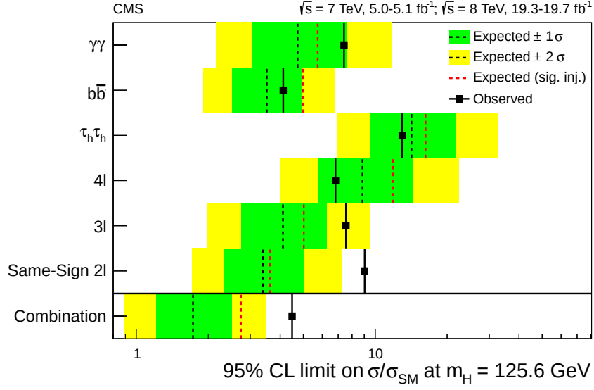
Figure 1.9: 95% CL upper limits on the signal strength parameter \mu = \sigma/\sigma_{\text{SM}} for the t\bar{t}H process at m_H = 125.6 GeV, in each individual t\bar{t}H channel and for all channels combined [49]
