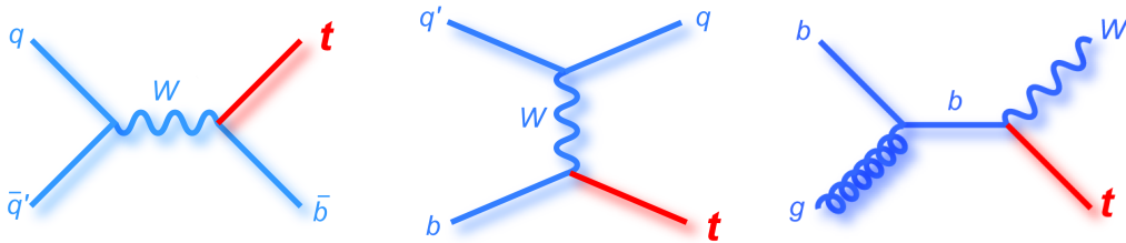
Figure 1.5 Examples of Feynman diagrams representing the single top quark production at leading order in the s -channel (left), t -channel (middle) and tW -channel (right). From [54].
