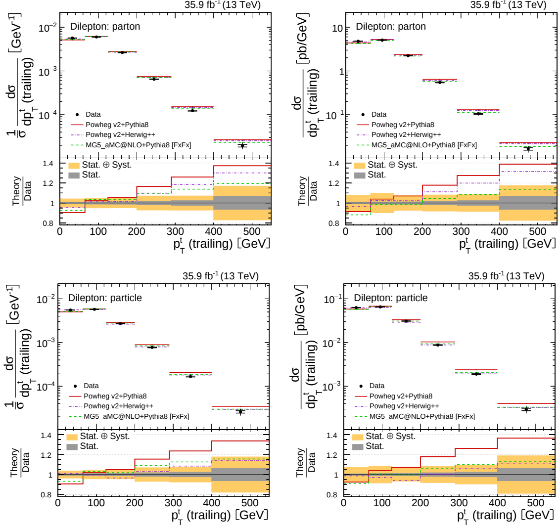
Figure 7.8 The normalized (left) and absolute (right) differential t\bar{t} production cross sections as a function of the transverse momentum of the trailing top quark p_T^t (trailing). Upper row corresponds to measurements at parton level in the full phase space. Lower row corresponds to measurements at particle level in a fiducial phase space. The data (black) are compared to the MC predictions from Powheg v2+Pythia8 (red), Powheg v2+Herwig++ (violet) and MG5_aMC@NLO+Pythia8 [FxFx] (green). The inner error bars show the statistical uncertainty, the outer error bars show a combination of the statistical and systematic uncertainties.
