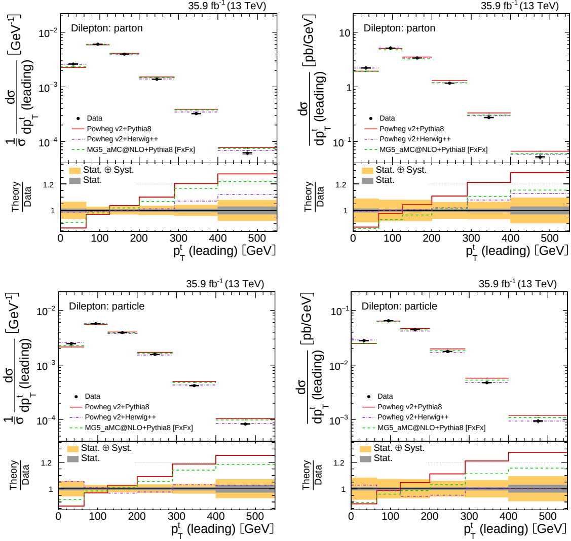
Figure 7.7 The normalized (left) and absolute (right) differential t\bar{t} production cross sections as a function of the transverse momentum of the leading top quark p_T^t ( leading ). Upper row corresponds to measurements at parton level in the full phase space. Lower row corresponds to measurements at particle level in a fiducial phase space. The data (black) are compared to the MC predictions from POWHEG v2+PYTHIA8 (red), POWHEG v2+HERWIG++ (violet) and MG5_aMC@NLO+PYTHIA8 [FxFx] (green). The inner error bars show the statistical uncertainty, the outer error bars show a combination of the statistical and systematic uncertainties.
