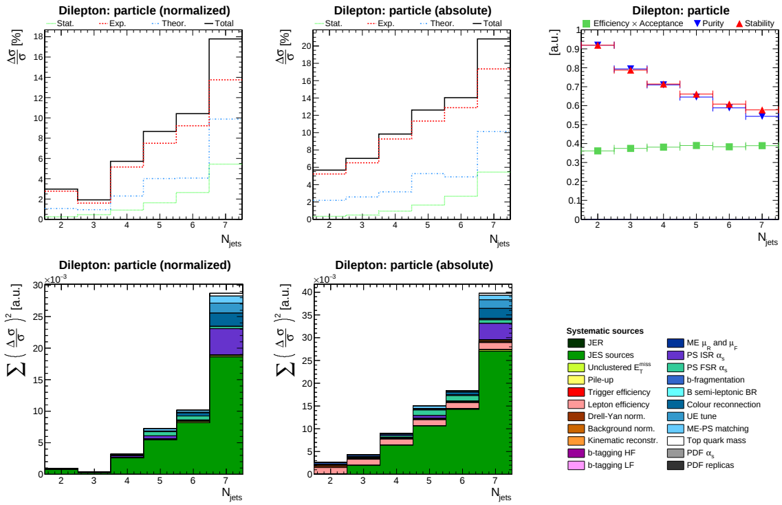
Figure C.25 A summary of the uncertainties and migrations among bins for the differential t\bar{t} production cross sections as a function of the jet multiplicity N_{jets} . Measurements are performed at particle level in a fiducial phase space. Upper row: a summary of uncertainties per bin for normalized (left) and absolute (middle) differential cross sections; efficiency \times acceptance, purity and stability per bin (right). Lower row: a summary of systematic uncertainties per bin for normalized (left) and absolute (middle; here, the uncertainties on the luminosity and decay branching ratio of the signal process are not shown) differential cross sections; sources of systematic uncertainty (right).
