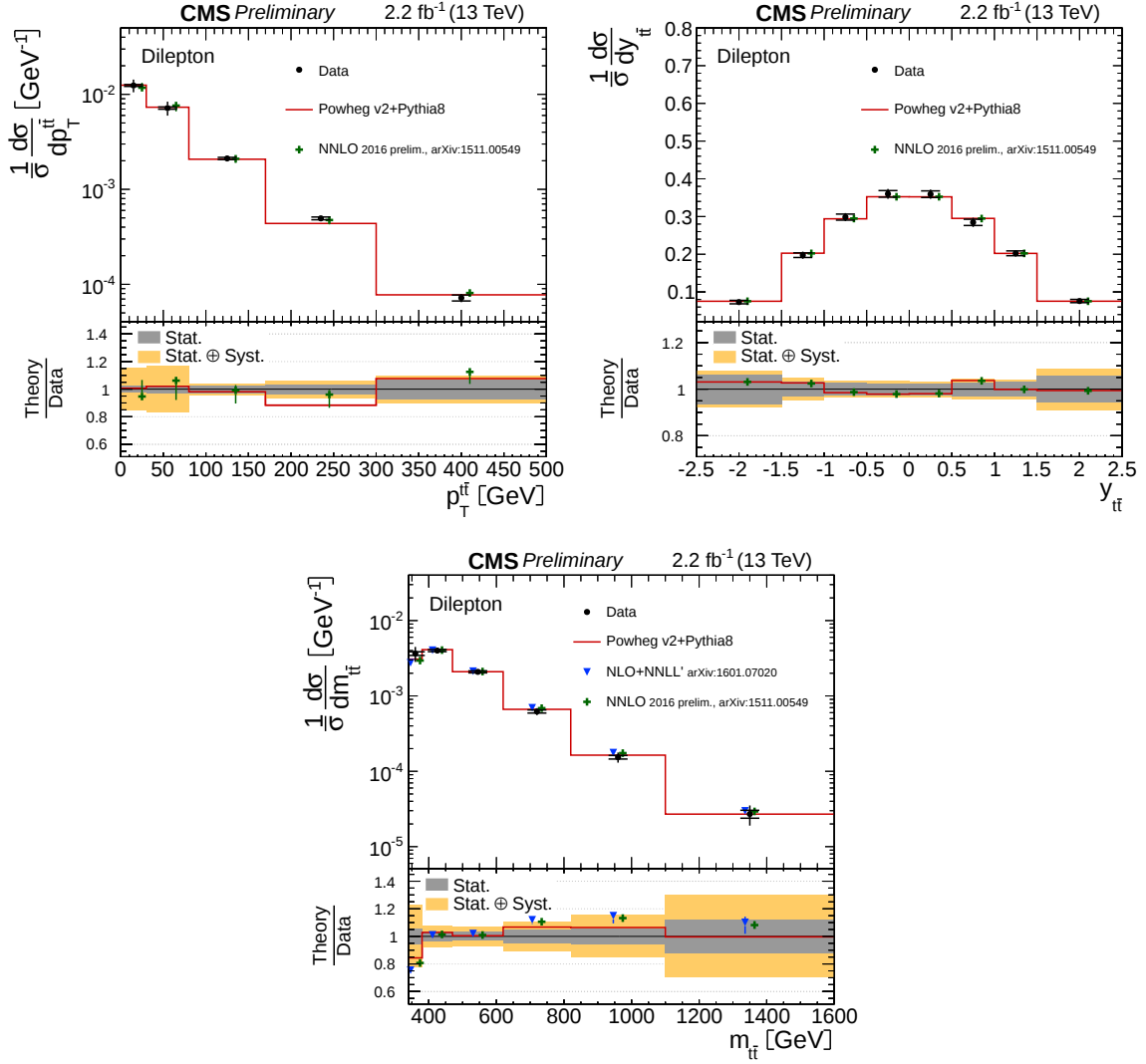
Figure 7.3 The normalized differential t\bar{t} production cross sections measured (using the complete 2015 dataset of L = 2.2 \text{ fb}^{-1} ) as a function of the transverse momentum (upper left), the rapidity (upper right) and the invariant mass (bottom) of the t\bar{t} -system. The results are presented at the parton level in the full phase space. The measured data are confronted with the Monte Carlo and fixed order SM predictions described in Section 7.1.2. The inner error bars show the statistical uncertainty, the outer error bars show a combination of the statistical and systematic uncertainties. Results published in [13].
