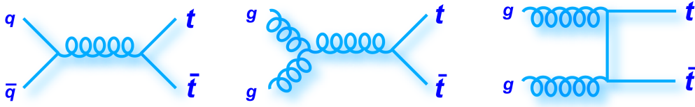
Figure 1.4 Examples of Feynman diagrams representing the t\bar{t} production via the q\bar{q} -annihilation (left) and the gg -fusion (middle, right) at leading order. From [54].
