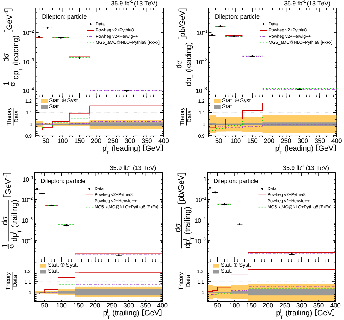
Figure 7.21 The normalized (left) and absolute (right) differential t\bar{t} production cross sections as a function of the transverse momentum of the leading lepton p_T^\ell ( leading ) (upper row) and as a function of the transverse momentum of the trailing lepton p_T^\ell ( trailing ) (lower row). Measurements are performed at particle level in a fiducial phase space. The data (black) are compared to the MC predictions from PowHEG v2+PYTHIA8 (red), PowHEG v2+HERWIG++ (violet) and MG5_aMC@NLO+PYTHIA8 [FxFx] (green). The inner error bars show the statistical uncertainty, the outer error bars show a combination of the statistical and systematic uncertainties.
