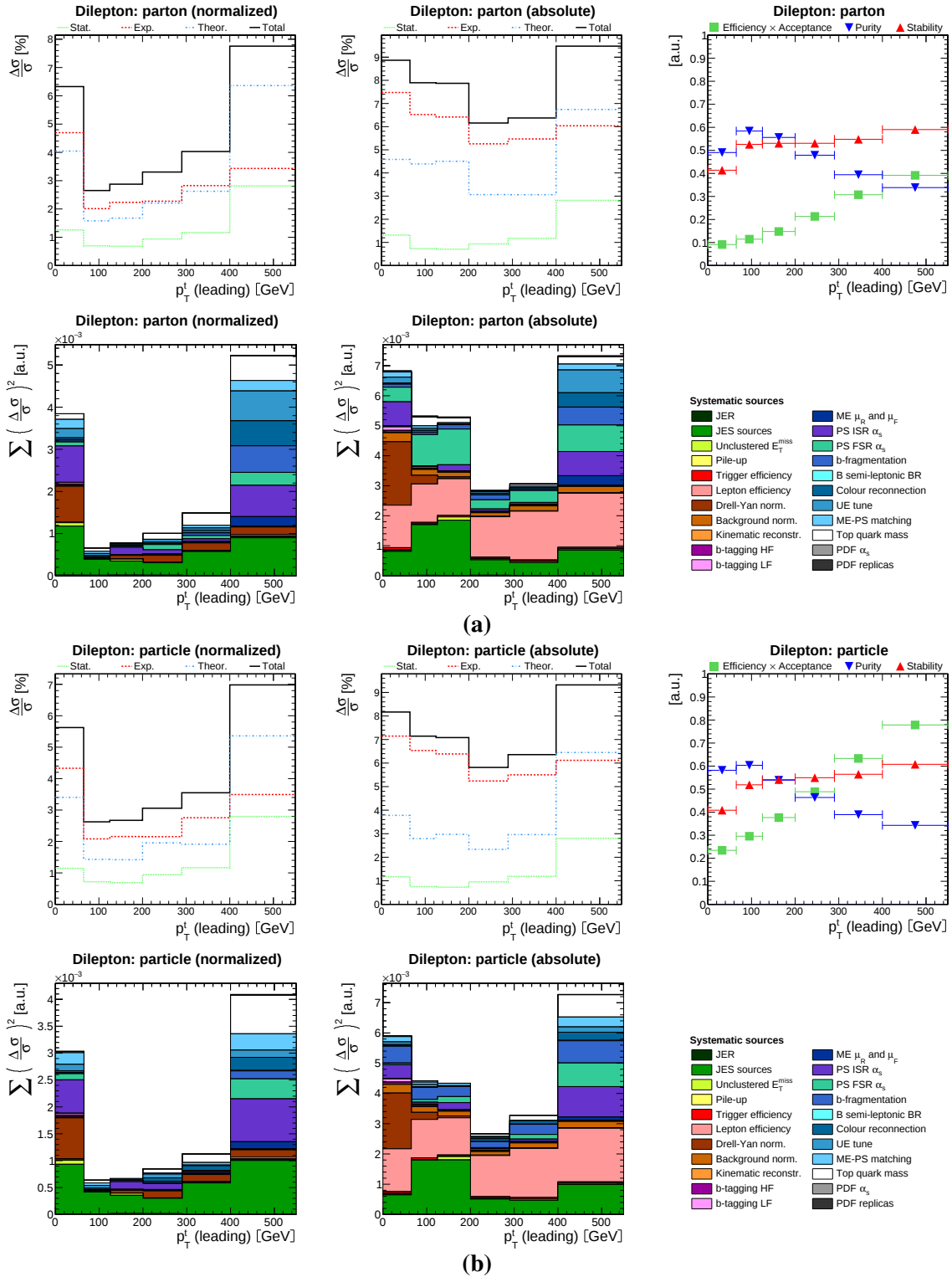
Figure C.3 A summary of the uncertainties and migrations among bins for the differential t\bar{t} production cross sections as a function of the transverse momentum of the leading top quark p_T^t ( leading ). Figure (a) corresponds to measurements at parton level in the full phase space. Upper row: a summary of uncertainties per bin for normalized (left) and absolute (middle) differential cross sections; efficiency \times acceptance, purity and stability per bin (right). Lower row: a summary of systematic uncertainties per bin for normalized (left) and absolute (middle; here, the uncertainties on the luminosity and decay branching ratio of the signal process are not shown) differential cross sections; sources of systematic uncertainty (right). Figure (b) shows the same for measurements at particle level in a fiducial phase space.
