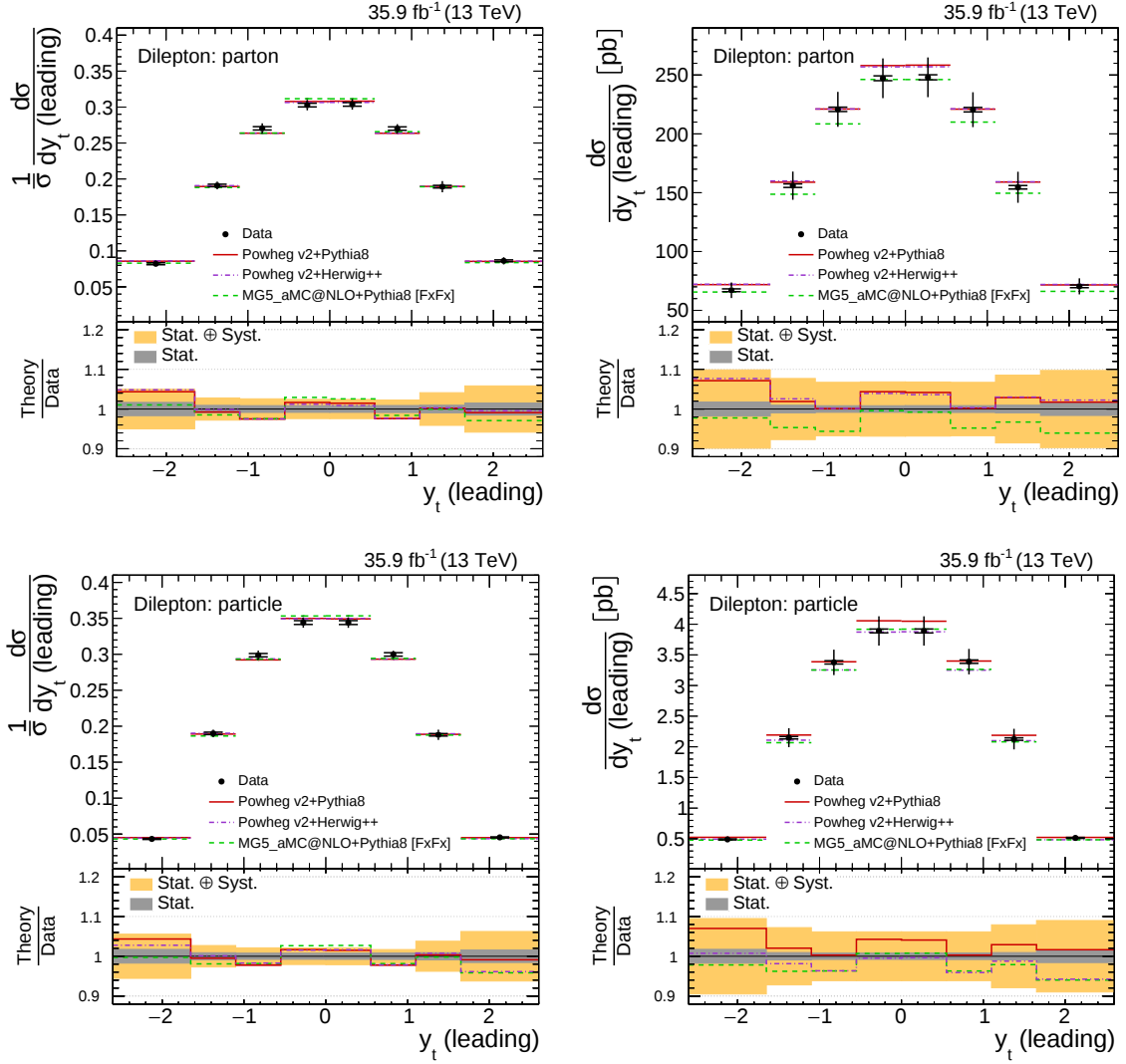
Figure 7.13 The normalized (left) and absolute (right) differential t\bar{t} production cross sections as a function of the rapidity of the leading top quark y_t ( leading ). Upper row corresponds to measurements at parton level in the full phase space. Lower row corresponds to measurements at particle level in a fiducial phase space. The data (black) are compared to the MC predictions from POWHEG v2+PYTHIA8 (red), POWHEG v2+HERWIG++ (violet) and MG5_aMC@NLO+PYTHIA8 [FxFx] (green). The inner error bars show the statistical uncertainty, the outer error bars show a combination of the statistical and systematic uncertainties.
