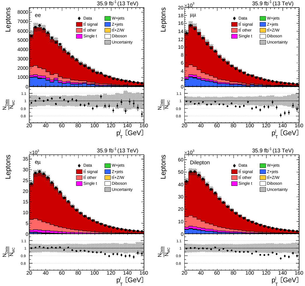
Figure 4.16 Transverse momentum of leptons. Events fulfill the lepton pair and jet-related selection requirements, as well as the criterion demanding the presence of at least one b-tagged jet in the event. In the e^+e^- and \mu^+\mu^- channels, events satisfying 76 \text{ GeV} < m_{\ell\bar{\ell}} < 106 \text{ GeV} and E_T^{\text{miss}} < 40 \text{ GeV} conditions are excluded. The distributions are separately shown for the e^+e^- (upper left), \mu^+\mu^- (upper right), e^\pm\mu^\mp (lower left) channels and for their combination “Dilepton” (lower right). The Z+jets simulation is scaled according to results of the data-driven background estimation. The hatched area indicates the shape systematic uncertainties on the t\bar{t} signal and backgrounds (see Chapter 6). The displayed quantities are used as an input to the top-quark pair kinematic reconstruction in each event.
