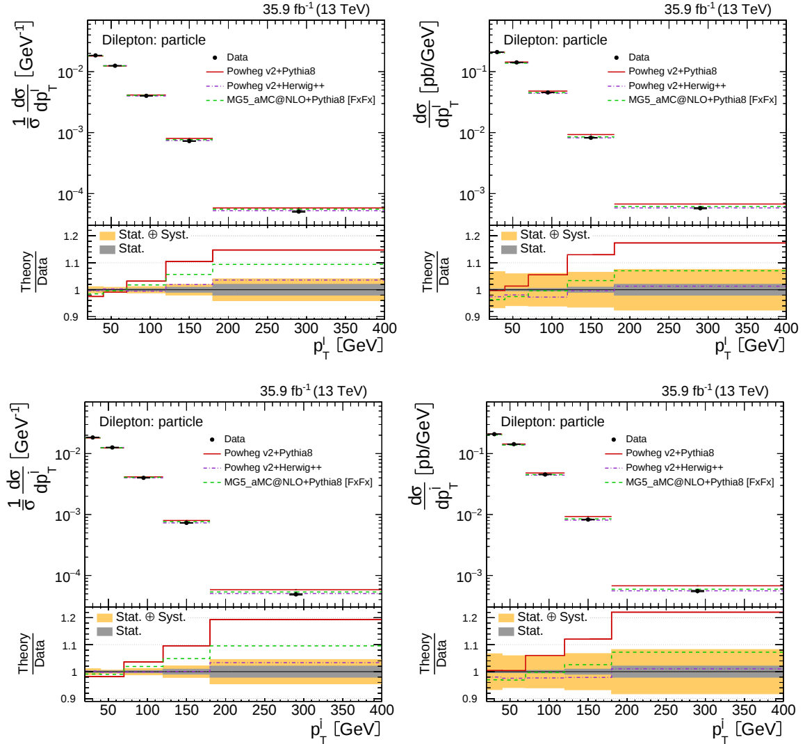
Figure 7.20 The normalized (left) and absolute (right) differential t\bar{t} production cross sections as a function of the transverse momentum of the lepton p_T^l (upper row) and as a function of the transverse momentum of the antilepton p_T^{\bar{l}} (lower row). Measurements are performed at particle level in a fiducial phase space. The data (black) are compared to the MC predictions from POWHEG v2+PYTHIA8 (red), POWHEG v2+HERWIG++ (violet) and MG5_aMC@NLO+PYTHIA8 [FxFx] (green). The inner error bars show the statistical uncertainty, the outer error bars show a combination of the statistical and systematic uncertainties.
