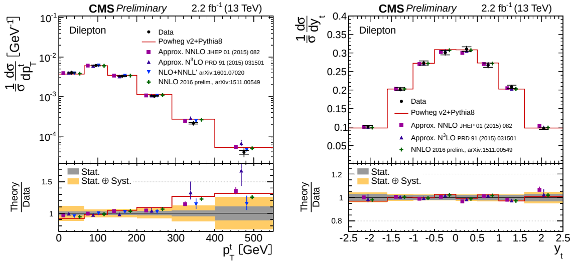
Figure 7.2 The normalized differential t\bar{t} production cross sections measured (using the complete 2015 dataset of L = 2.2 \text{ fb}^{-1} ) as a function of the transverse momentum (left) and the rapidity (right) of the top quarks and antiquarks. The results are presented at the parton level in the full phase space. The measured data are confronted with the Monte Carlo and fixed order SM predictions described in Section 7.1.2. The inner error bars show the statistical uncertainty, the outer error bars show a combination of the statistical and systematic uncertainties. Results published in [13].
