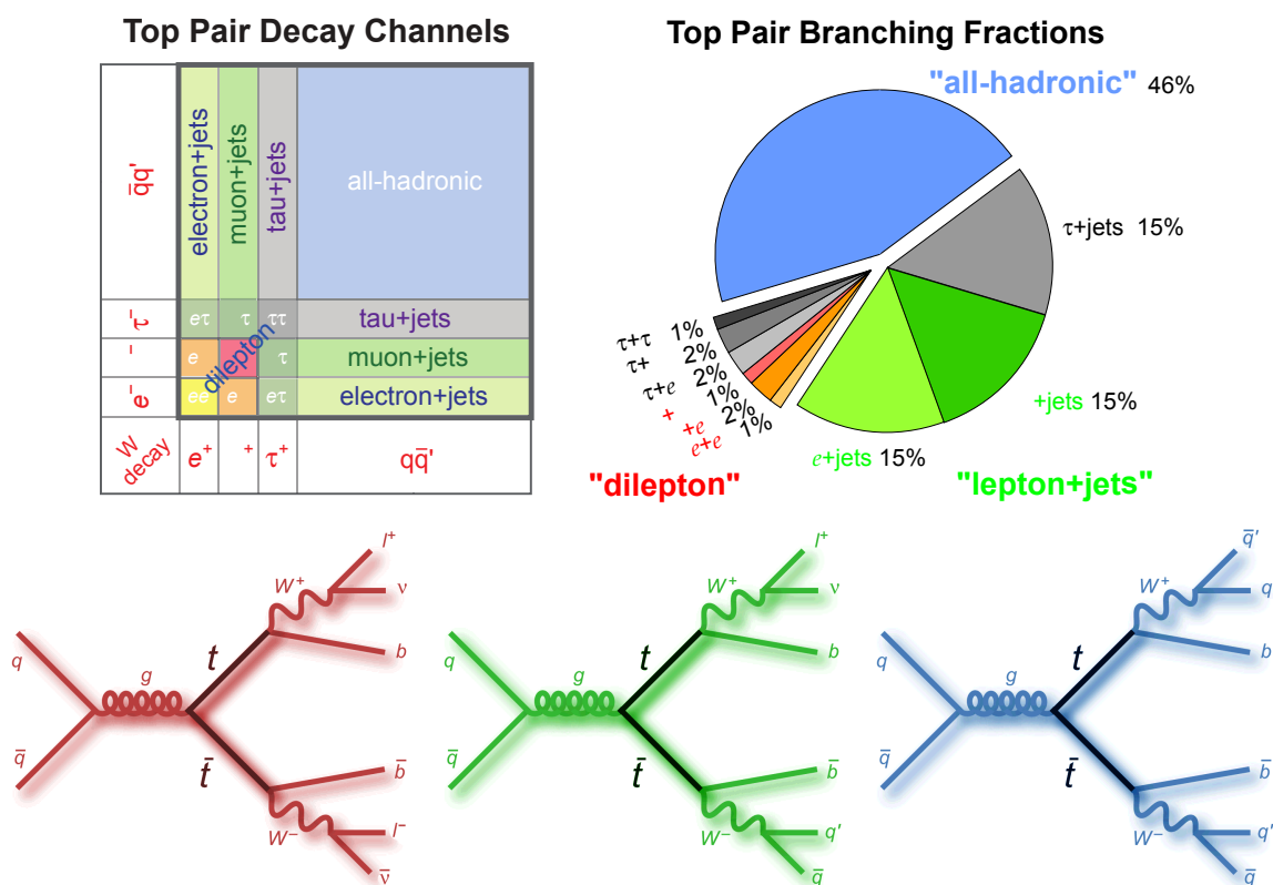
Figure 1.6 A schematic classification of the top-quark pair decay channels (upper left) is shown together with the distribution of corresponding branching ratios (upper right; numbers are approximate). In the lower row, examples of LO Feynman diagrams are shown for the t\bar{t} production with the subsequent decays in the dilepton (left), lepton+jets (middle) and all-hadronic (right) channels. From [54], modified.
