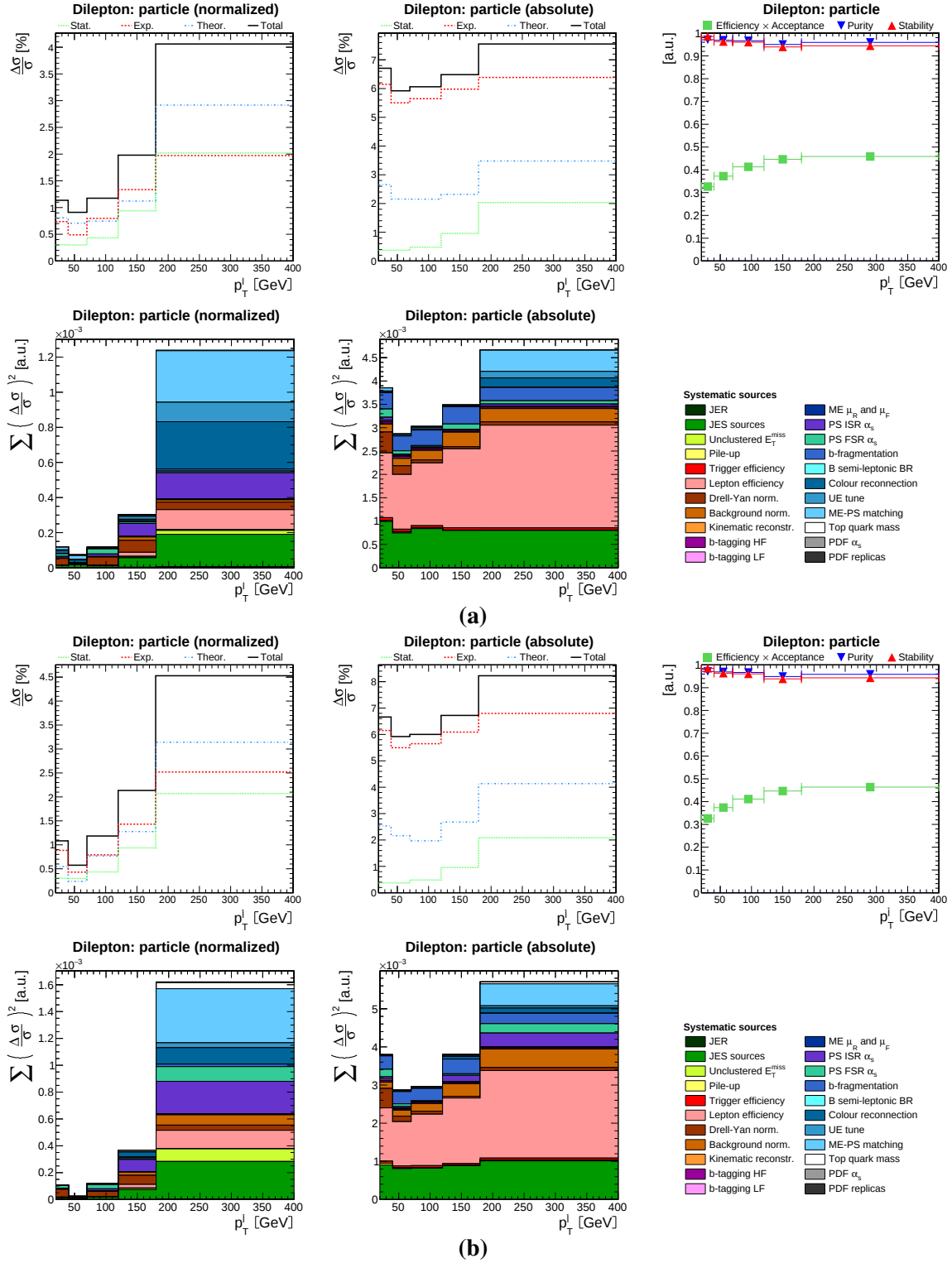
Figure C.16 In Figure (a), a summary of the uncertainties and migrations among bins for the differential t\bar{t} production cross sections as a function of the transverse momentum of the lepton p_T^l . Measurements are performed at particle level in a fiducial phase space. Upper row: a summary of uncertainties per bin for normalized (left) and absolute (middle) differential cross sections; efficiency \times acceptance, purity and stability per bin (right). Lower row: a summary of systematic uncertainties per bin for normalized (left) and absolute (middle; here, the uncertainties on the luminosity and decay branching ratio of the signal process are not shown) differential cross sections; sources of systematic uncertainty (right). Figure (b) shows the same for measurements as a function of the transverse momentum of the antilepton p_T^{\bar{l}} .
