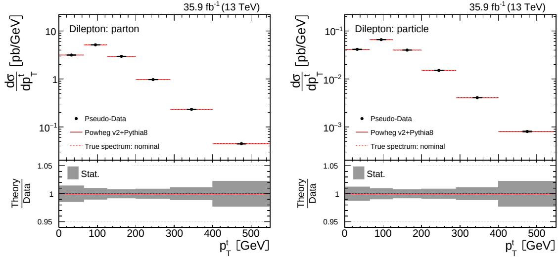
Figure 5.4 Absolute t\bar{t} differential cross sections, together with their statistical uncertainty, measured as a function of the top quark transverse momentum using the pseudo-data sample, constructed as a sum of all reference simulated samples without any additional variations. The pseudo-data is unfolded either to parton (left) or particle (right) level using the reference t\bar{t} simulation, i.e. POWHEG v2+PYTHIA8. The statistical uncertainty corresponds to the uncertainty of the unfolding method.
