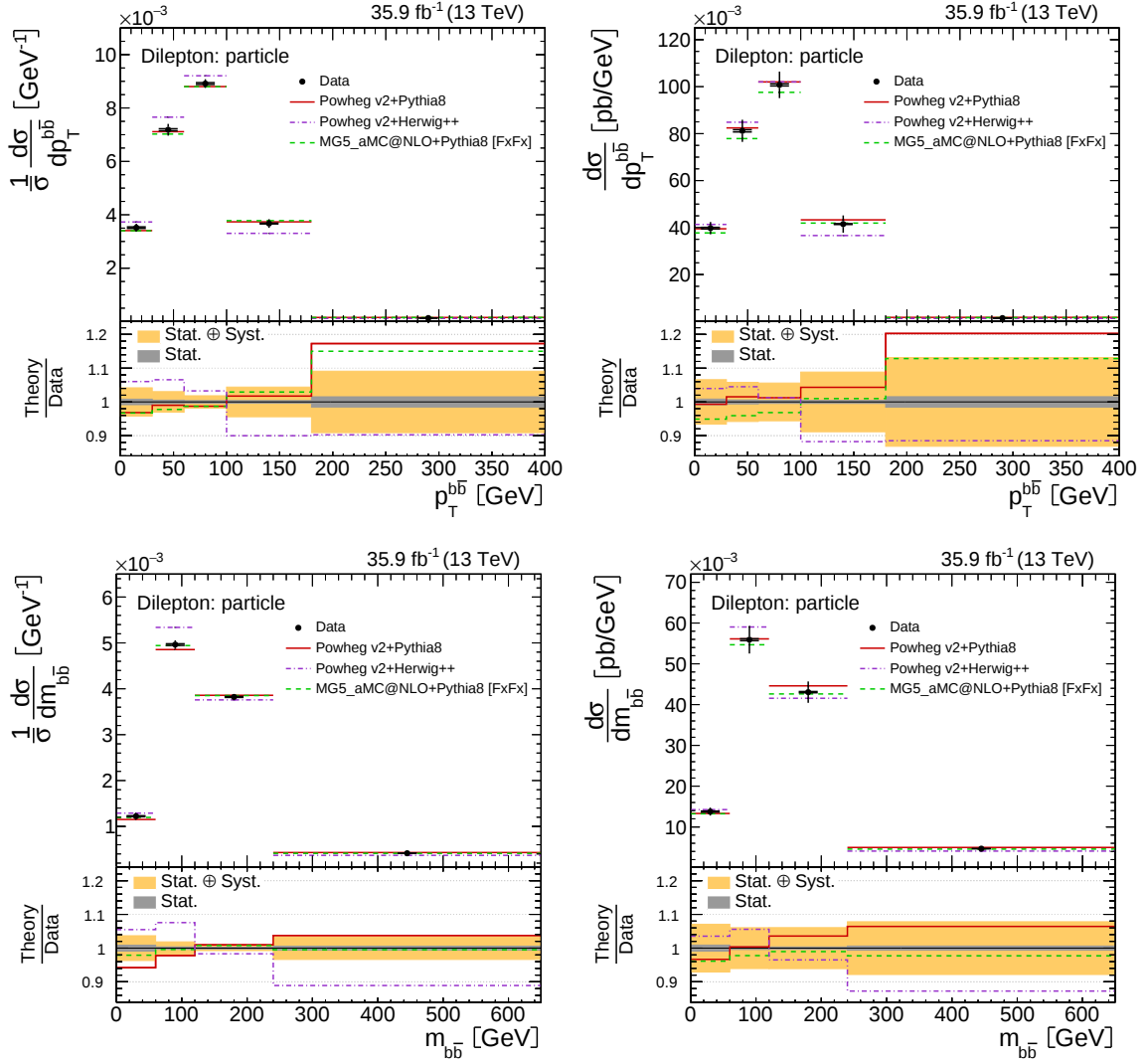
Figure 7.28 The normalized (left) and absolute (right) differential t\bar{t} production cross sections as a function of the transverse momentum of the b-jet pair p_T^{b\bar{b}} (upper row) and as a function of the invariant mass of the b-jet pair m_{b\bar{b}} (lower row). Measurements are performed at particle level in a fiducial phase space. The data (black) are compared to the MC predictions from POWHEG v2+PYTHIA8 (red), POWHEG v2+HERWIG++ (violet) and MG5_aMC@NLO+PYTHIA8 [FxFx] (green). The inner error bars show the statistical uncertainty, the outer error bars show a combination of the statistical and systematic uncertainties.
