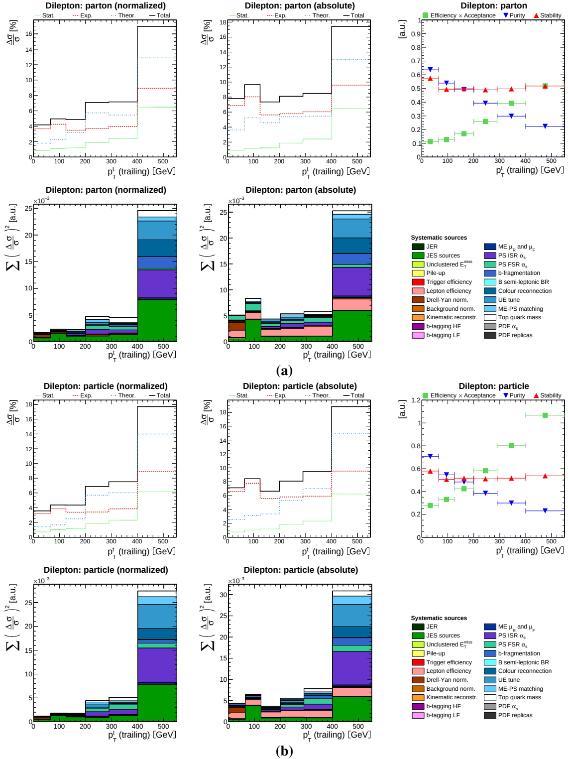
Figure C.4 A summary of the uncertainties and migrations among bins for the differential t\bar{t} production cross sections as a function of the transverse momentum of the trailing top quark p_T^t ( trailing ). Figure (a) corresponds to measurements at parton level in the full phase space. Upper row: a summary of uncertainties per bin for normalized (left) and absolute (middle) differential cross sections; efficiency \times acceptance, purity and stability per bin (right). Lower row: a summary of systematic uncertainties per bin for normalized (left) and absolute (middle; here, the uncertainties on the luminosity and decay branching ratio of the signal process are not shown) differential cross sections; sources of systematic uncertainty (right). Figure (b) shows the same for measurements at particle level in a fiducial phase space.
