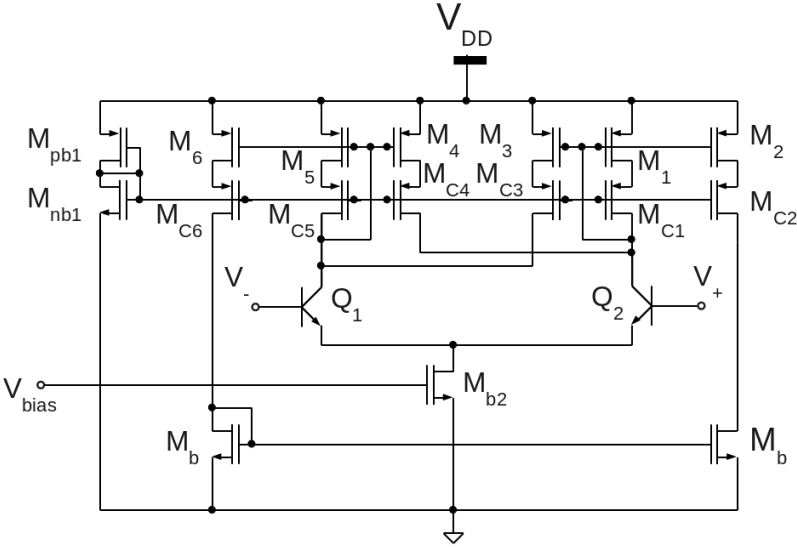
Figure 5.10: Hysteresis comparator schematic
