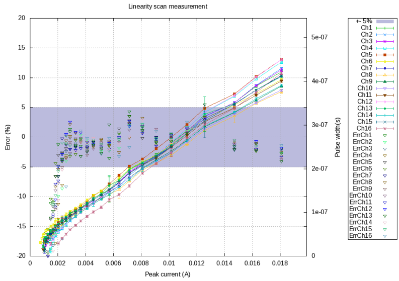
Figure 5.39: Linearity \tau \approx 36\text{ns} 18mA range
