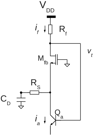
Figure 4.4: High Frequency feedback loop simplified circuit
