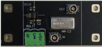
Figure 2.7: SiPM basic test board
