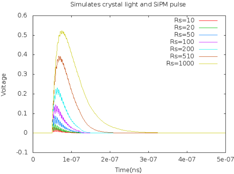
Figure 2.11: Crystal light simulation S10362-11-025P
