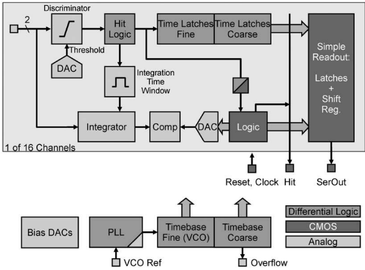
Figure 3.5: PETA block diagram [32]
