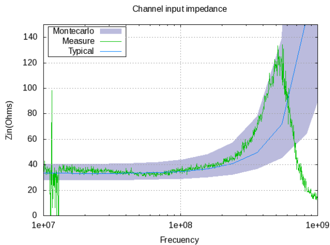
Figure 5.34: Input impedance
