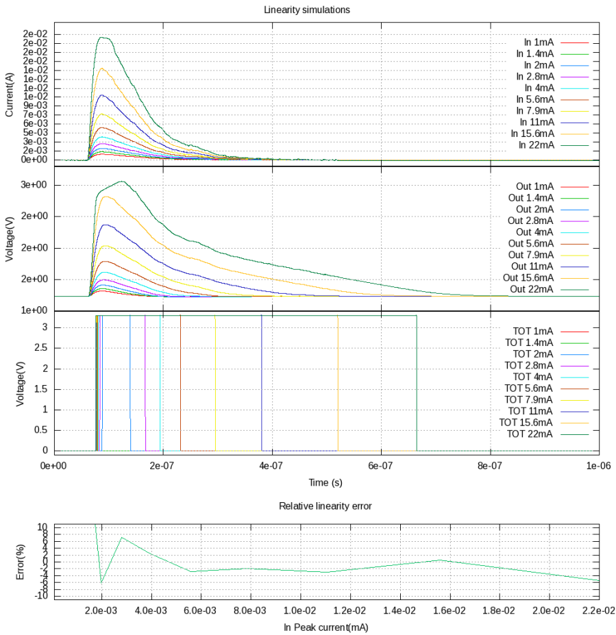
Figure 5.9: Linearity simulation
