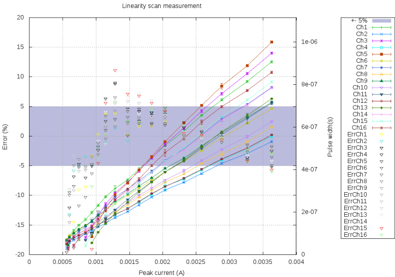
Figure 5.44: Linearity \tau \approx 110\text{ns} 3.5mA range
