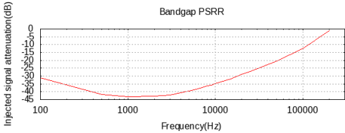
Figure 9: Bandgap PSRR in AC
