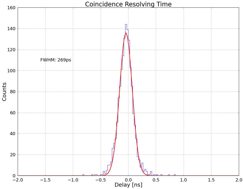
Figure 37: Coincidence Resolving Time measurement
