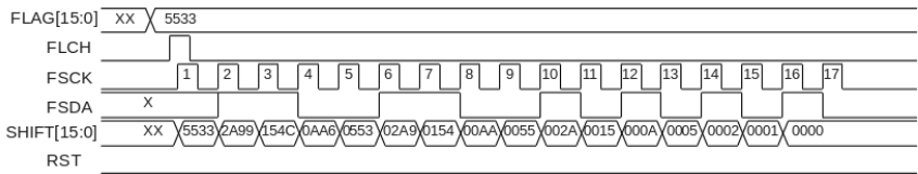
Figure 5.17: Pile up register readout
