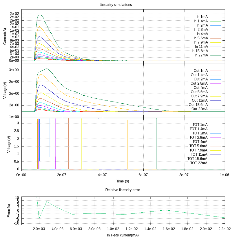
Figure 30: Linearity simulation
