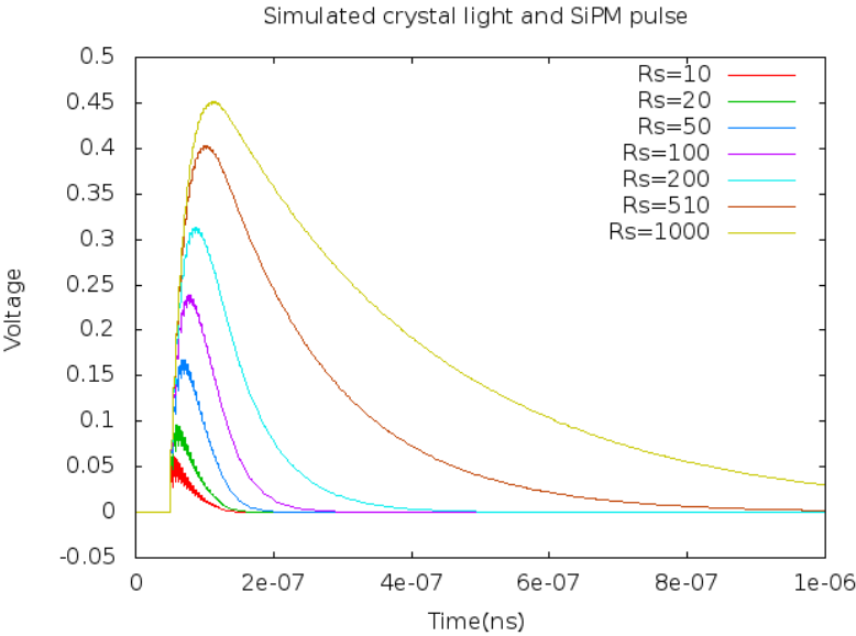
Figure 2.12: Crystal light simulation S10931-050P
