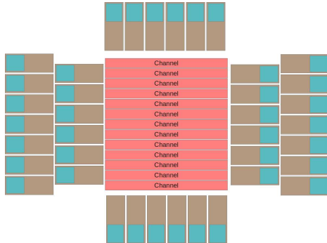
Figure 6.6: Staggered PADs
