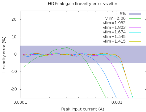
Figure 15: Saturation control of High Gain
