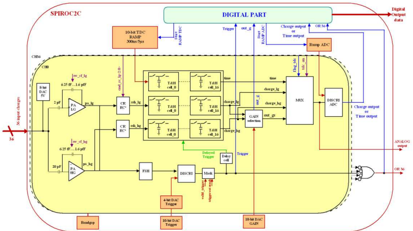
Figure 3.3: SPIROC2c block diagram [29]
