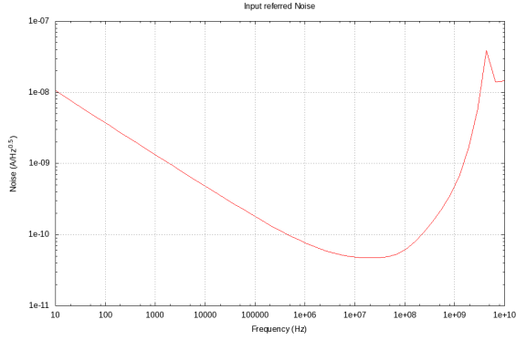
Figure 6.21: PACIFICr1 Noise simulation
