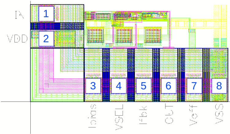
Figure 3: Pin configuration (Top view)
