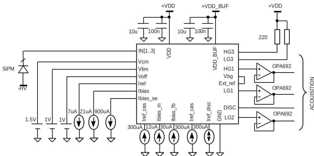
Figure 1: Typical application schematic
