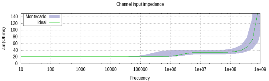
Figure 4.7: Input impedance
