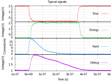
Figure 5.37: \tau \approx 36\text{ns}
