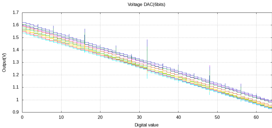
Figure 5.20: Voltage DAC(6b) MonteCarlo
