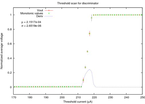
Figure 13: Noise measurement
