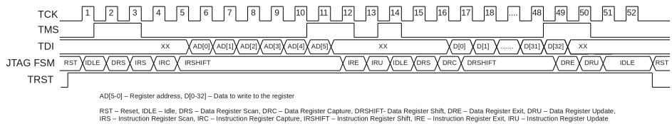
Figure 5.29: JTAG 33 bits register write
