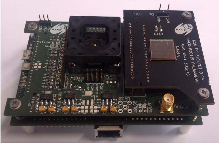
Figure 31: Test system setup
