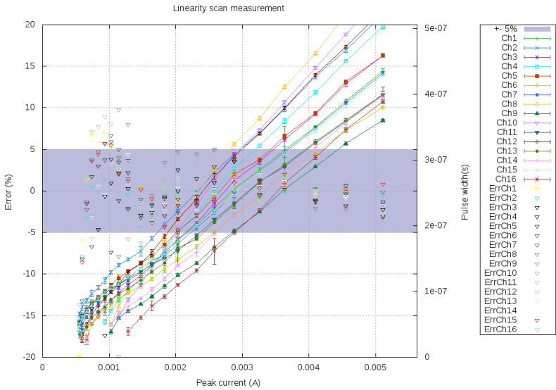
Figure 5.42: Linearity \tau \approx 110\text{ns} 5mA range
