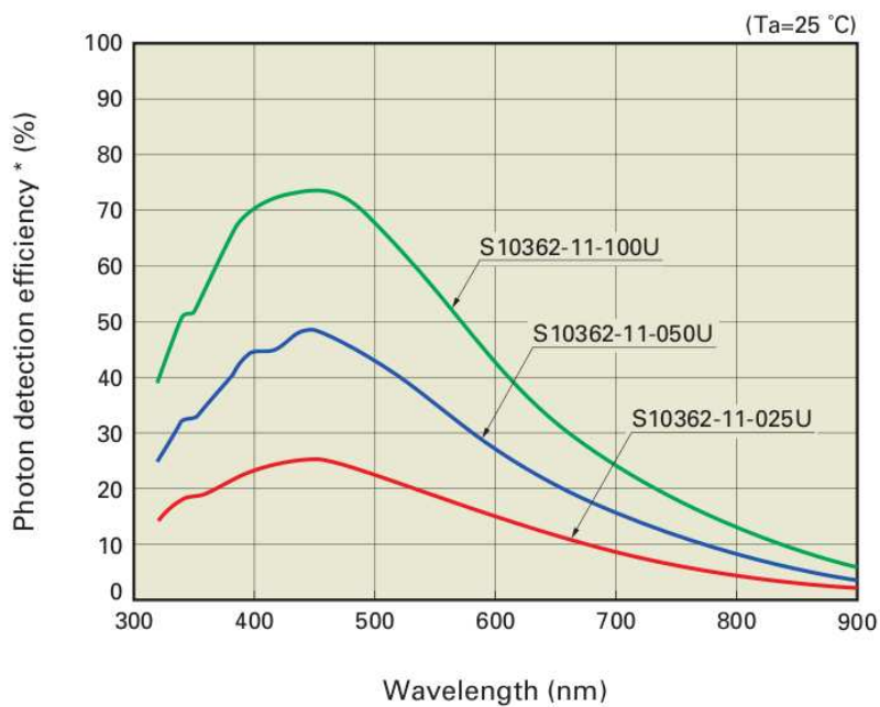
Figure 1.19: PDE variation with Wavelength
