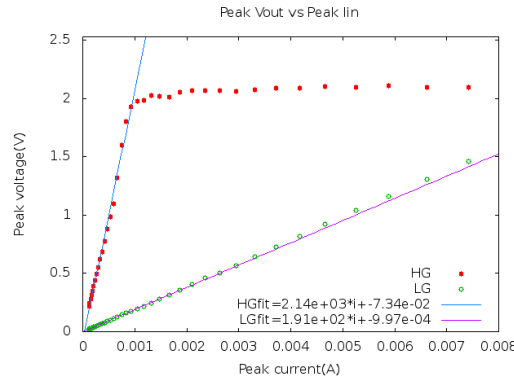
Figure 11: Linearity measurement
