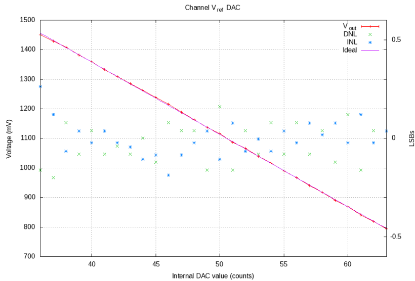
Figure 5.50: Single channel V_{\text{ref}} DAC measurement
