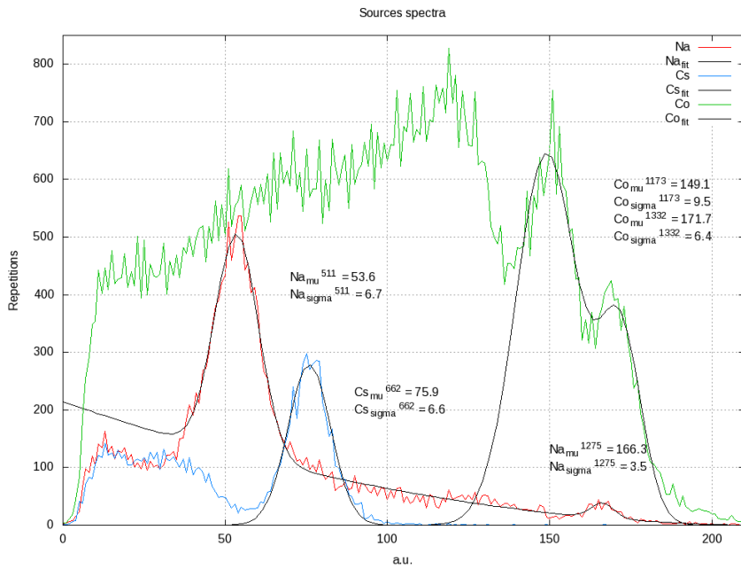
Figure 5.55: \text{Na}^{22} , \text{Co}^{60} , \text{Cs}^{137} spectra measurement
