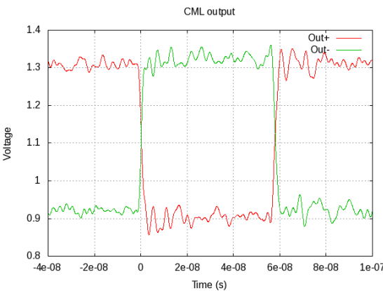
Figure 5.52: CML output
