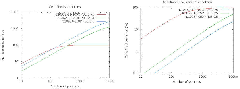
Figure 1.10: SiPM detection deviation
