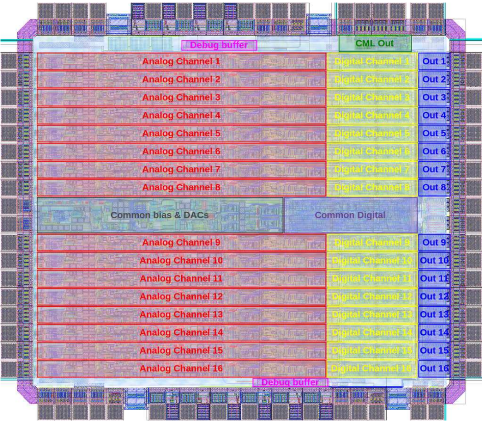
Figure 5.31: Final FLEXTOT layout
