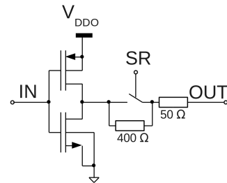
Figure 5.22: Output pad buffer with SR control schematic
