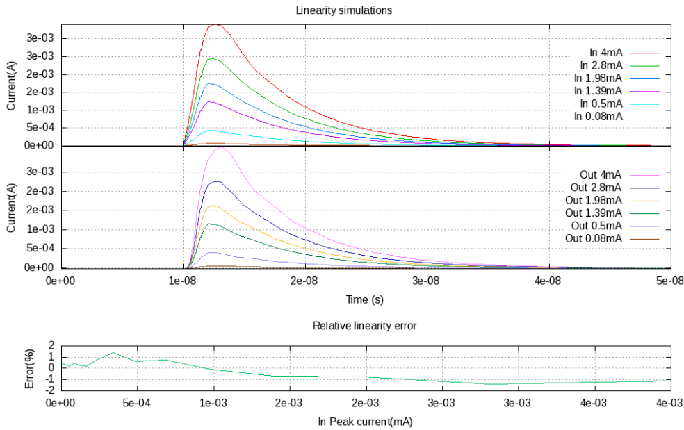
Figure 6: Linearity simulation
