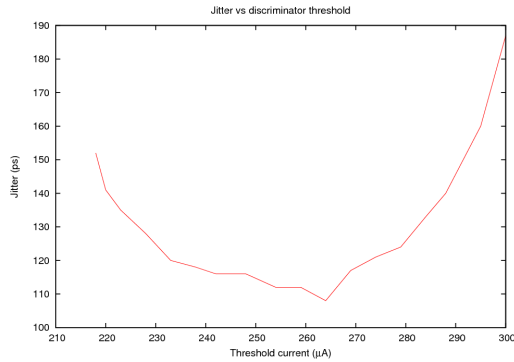
Figure 12: Jitter measurement
