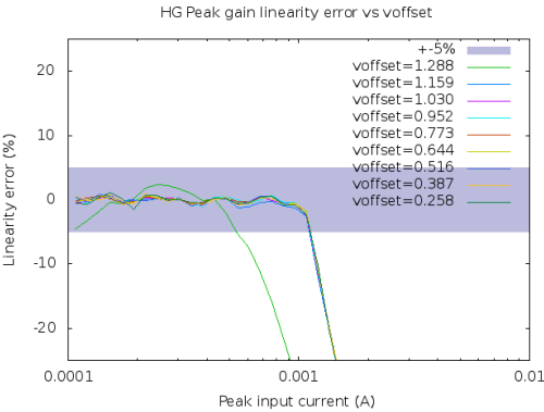
Figure 16: V_{off} variation effect in High Gain
