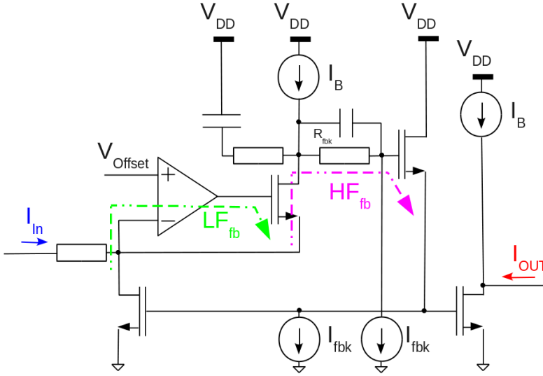
Figure 6.16: PACIFICr1 blocks
