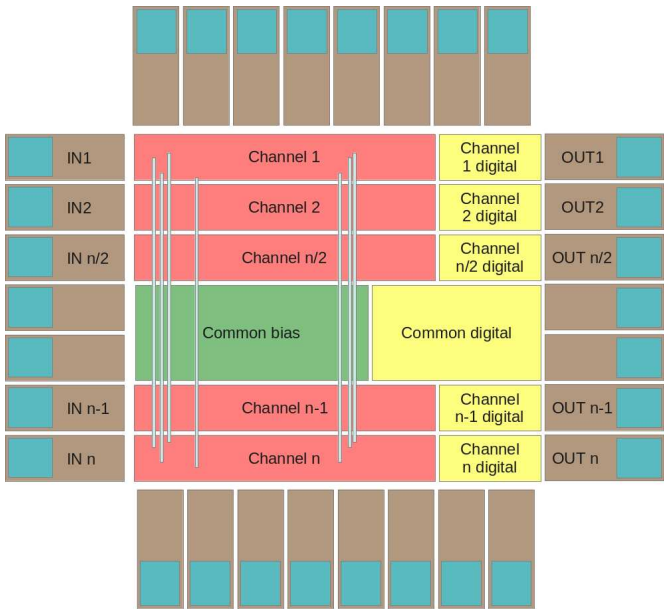
Figure 5.3: FLEXTOT floorplan
