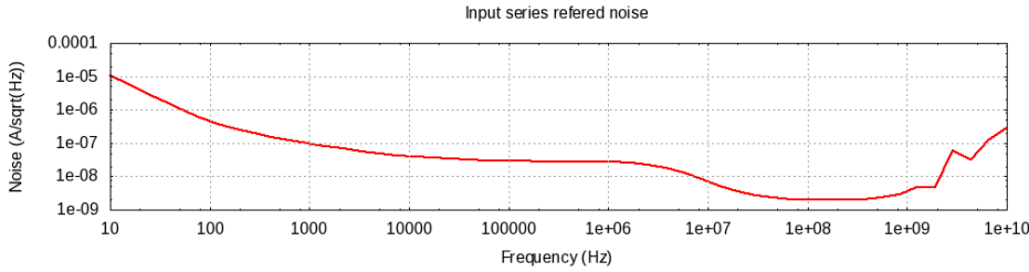
Figure 4.10: Series input referred noise
