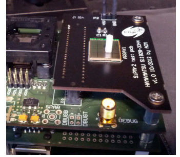
Figure 5.54: LSO setup detail
