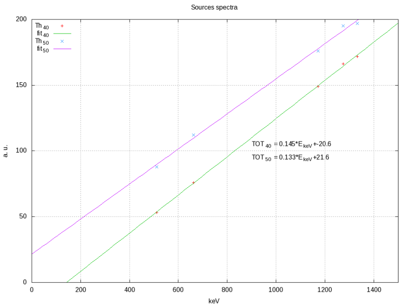
Figure 5.56: Linearity of the resulting spectra measurements
