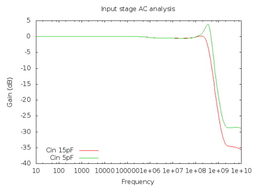
Figure 8: Input stage bandwidth
