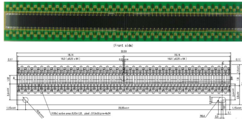
Figure 6.7: Hamamatsu SiPM array prototype
