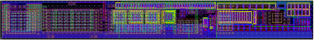
Figure 9: PACIFICr1 channel layout, 335\mu\text{m} \times 40\mu\text{m}
