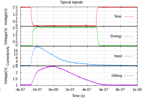
Figure 5.38: \tau \approx 110\text{ns}
