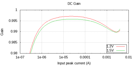
Figure 7: DC gain simulation
