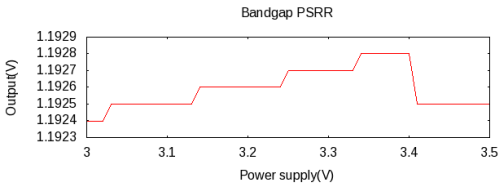
Figure 8: Bandgap PSRR
