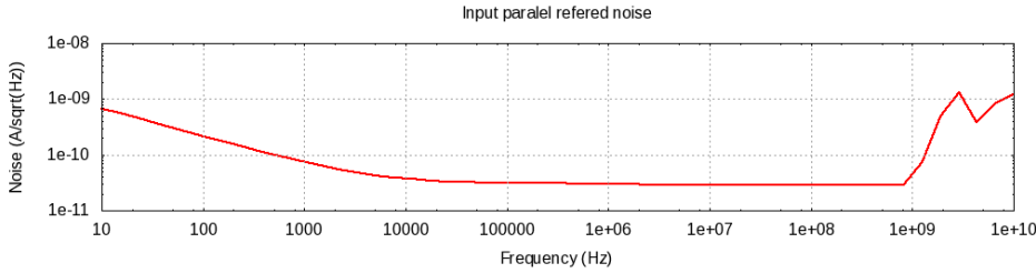
Figure 4.11: Parallel input referred noise
