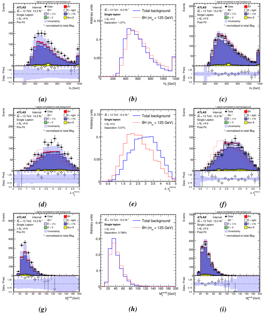
Figure B.3.: Input variables used for training the ANN in the (\geq 6j, \geq 4b) region. Variables from 7 to 9. The plots show pre-fit distributions, separation plots, post-fit distributions.
