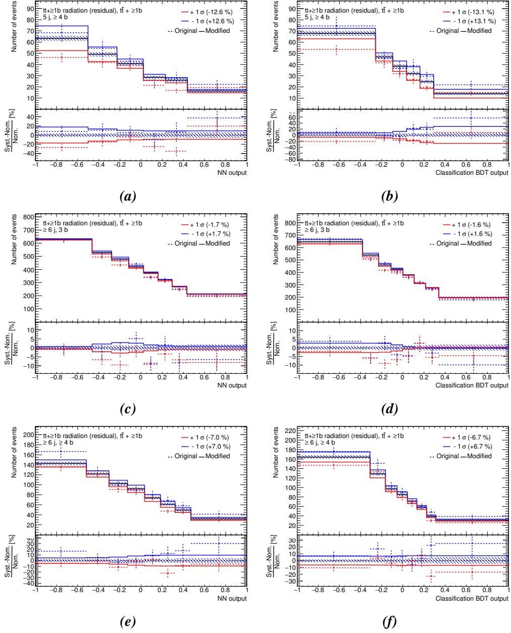
Figure D.1.: Comparison of the systematic uncertainty associated to t\bar{t} + 1b radiation residual variation for ANN and BDT
