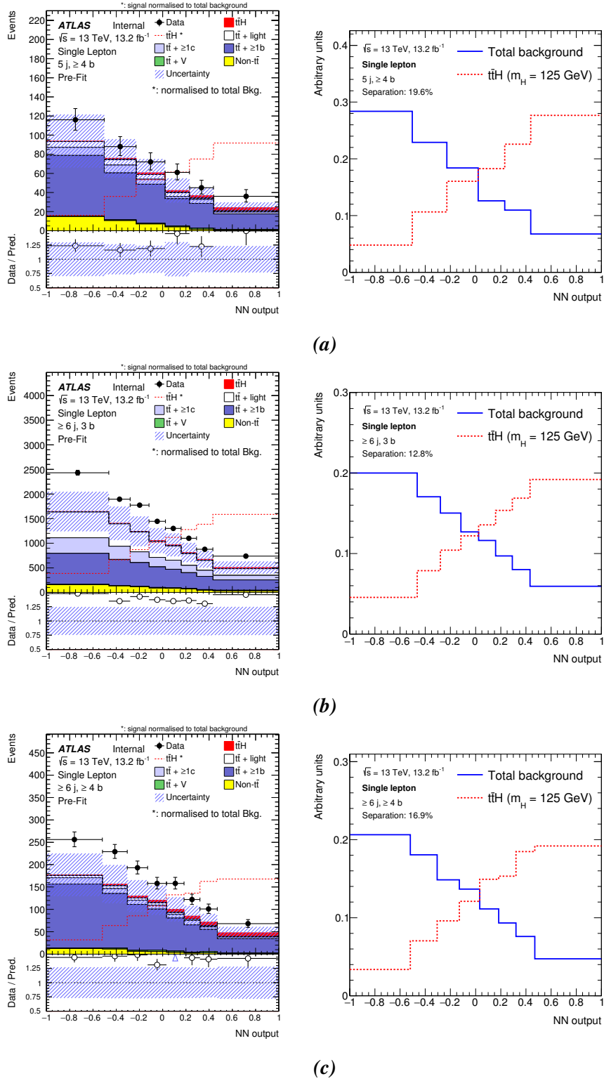
Figure 6.17.: Final ANN discriminants. For each training region both the data-prediction comparison (left) and separation of the normalised plots (right) are shown. The binning choice is done in order to achieve the best possible separation. (a) (5j, \geq 4b) . (b) (\geq 6j, 3b) . (c) (\geq 6j, \geq 4b)
