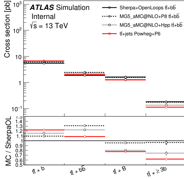
Figure 4.8.: The predicted cross sections for each of the t\bar{t} + \geq 1b sub-categories [61]. The inclusive prediction obtained with POWHEG+Pythia 6 is compared to the four-flavour calculations from Sherpa+OpenLoops and from MG5_aMC with different parton showers. The reweighting to Sherpa+OpenLoops has not been applied.
