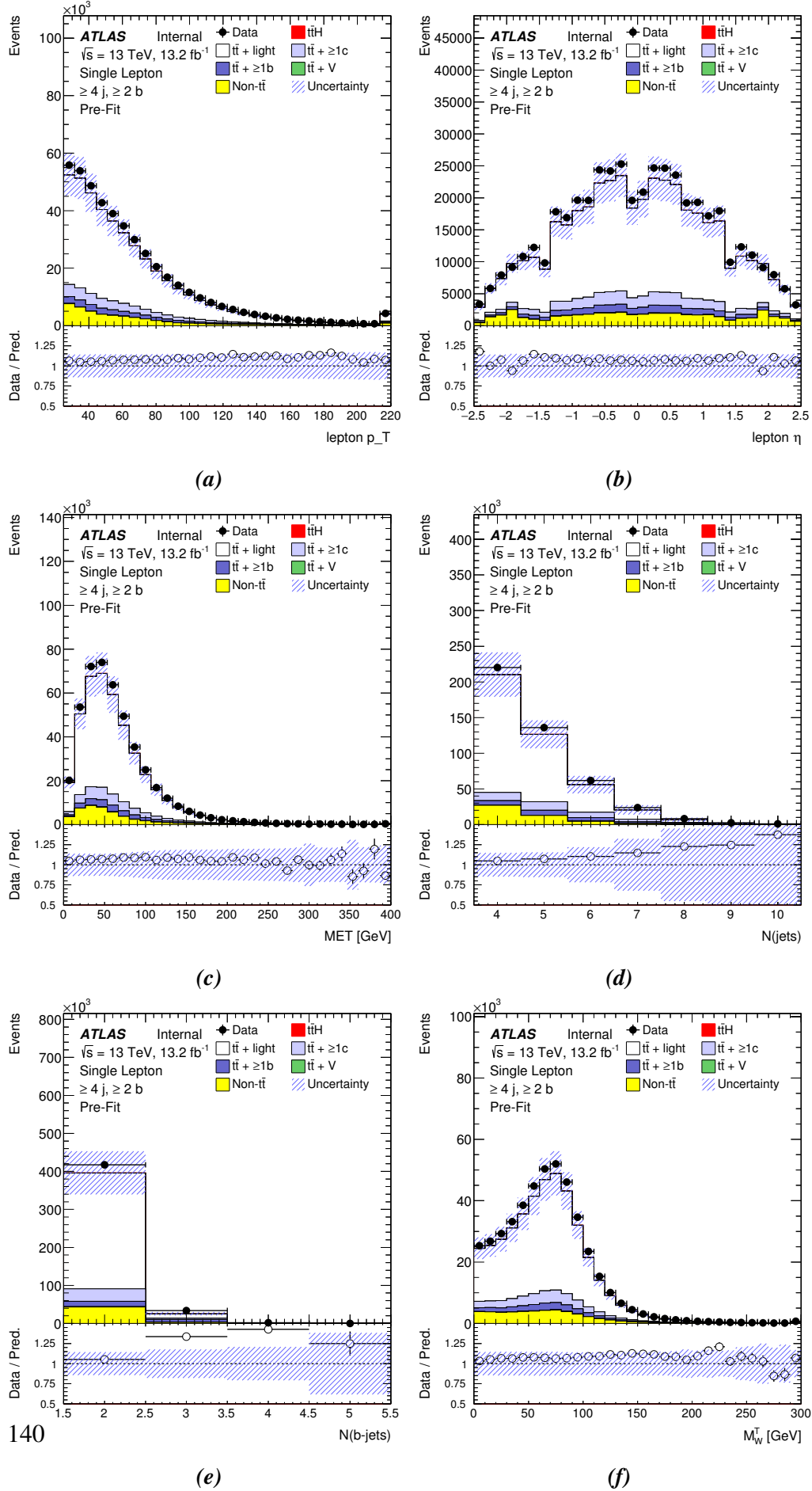
Figure A.2.: Plots of basic distributions: (a) p_T of the lepton, (b) \eta of the lepton, (c) E_T^{\text{miss}} , (d) jets multiplicity, (e) b-tag multiplicity, (f) transverse mass of the W boson
