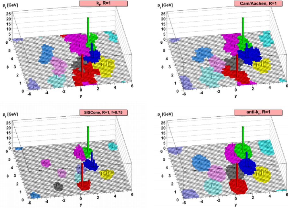
Figure 5.5.: A sample parton-level event clustered with four different jet algorithms [105].
