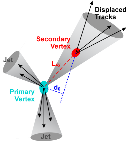
Figure 5.7.: Visual representation of a b -hadron decay within a jet resulting in a secondary vertex displaced to the primary vertex
