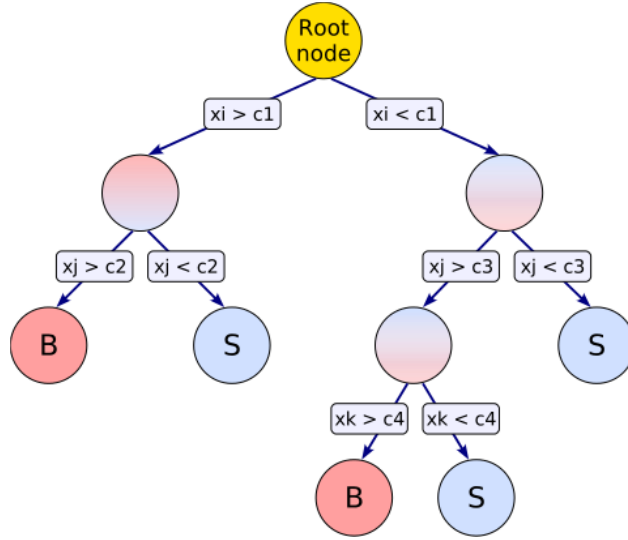
Figure 6.9.: A visual representation of a DT
