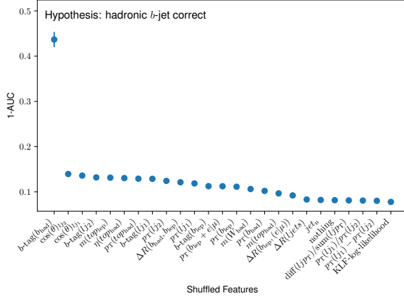
(a) Feature importance diagram of the b_{\text{had,correct}} -DNN.
