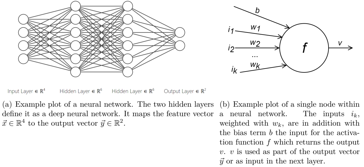
Figure 5.1: Example plots of a feedforward neural network. Figure 5.1(a) shows a whole neural network architecture while Figure 5.1(b) shows a single node with its in and output values.
