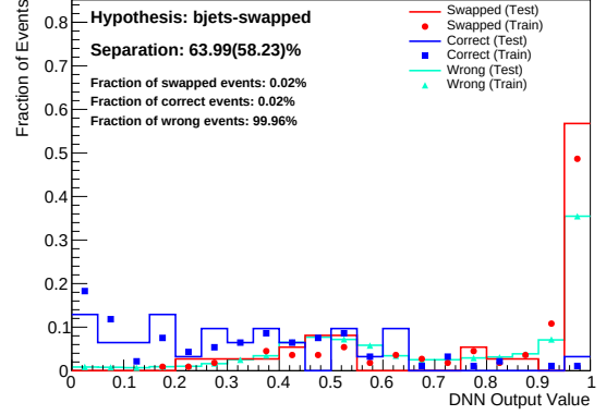
(b) Output value histogram of permutation 24 of the “ b -jets swapped”-DNN.
