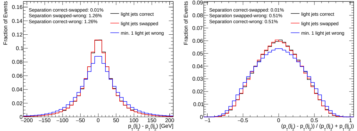
(a) Separation plot of the difference between lj_1 and lj_2 . The difference between the momenta is not a good separation value.
