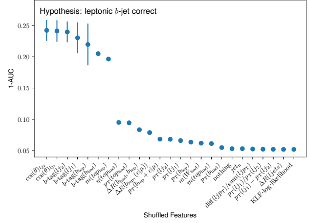
(b) Feature importance diagram of the b_{\text{lep,correct}} -DNN.
