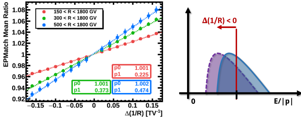
FIGURE C.6: (Left) Calibration curves for the effect of a rigidity scale in the mean value of the energy-momentum matching distribution for three different rigidity ranges. (Right) Illustration of the effect of a rigidity scale in the mean value of the energy-momentum matching distribution.
