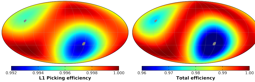
FIGURE 5.22: Galactic skymap of the spherical harmonic parametrization of the proton layer 1 picking efficiency ( left ) and the proton total efficiency ( right ) up to \ell = 2 , where only the significant components are included.
