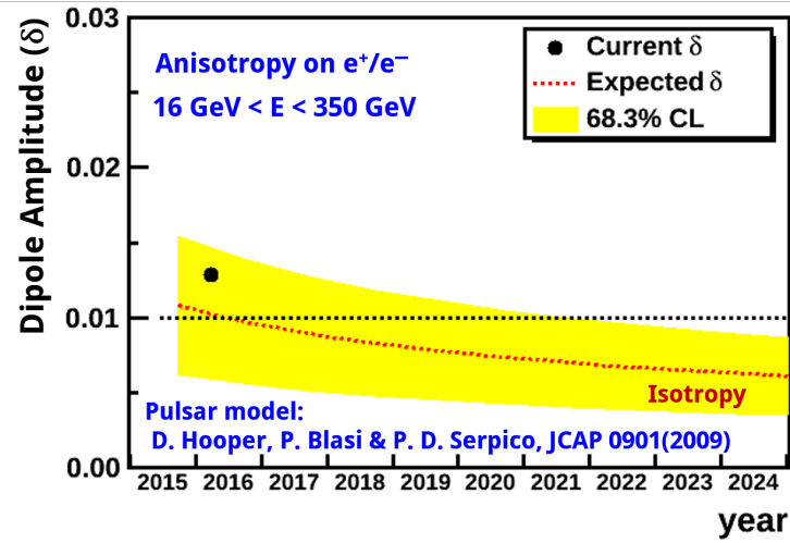
FIGURE 7.1: Projection of the expected dipole amplitude on the e^+/e^- anisotropy for 16 < E < 350 GeV up to the end of the data taking in 2024. The current dipole amplitude (black dot) and the isotropic expectation (dashed red line and yellow band) projected to 2024 are displayed. In addition, the expectation from a pulsar model based on [146] is shown.
