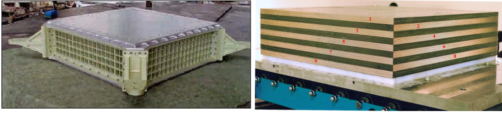
FIGURE 2.15: (Left) ECAL honeycomb structure. PMTs are installed on the squared holes. (Right) Distribution of the nine superlayers, with the fibers arranged in alternating directions.
