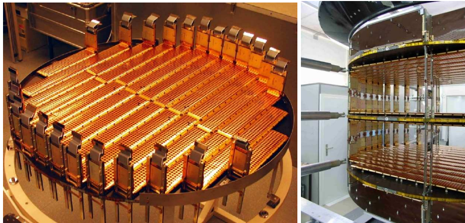
FIGURE 2.5: (Left) AMS-02 Tracker silicon ladders in a single plane. (Right) Three inner tracker planes, composed of double-sided layers with silicon detectors.
