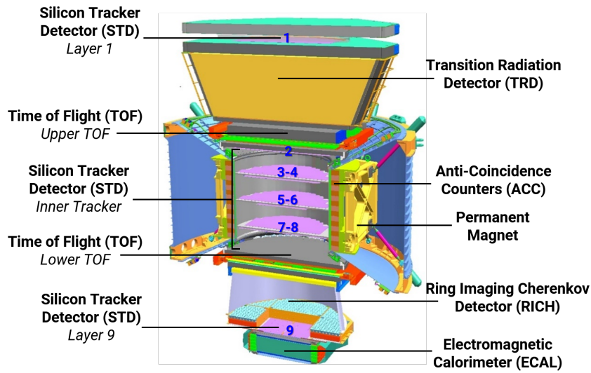
FIGURE 2.3: AMS-02 detector schematic layout.
