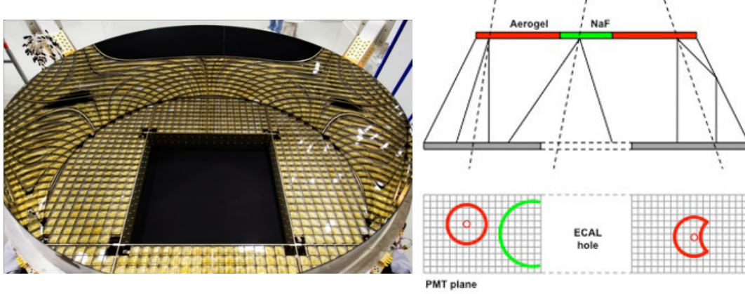
FIGURE 2.13: (Left) RICH detector, showing the PMT detection plane, the conical mirror and the ECAL hole. (Right) Cherenkov cones emitted by a charged particle crossing the radiator plane at the aerogel or NaF regions. Cherenkov cone emitted by a particle traversing the NaF region has a higher aperture angle, thus producing a circle despite of the ECAL hole.
