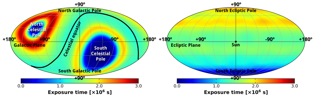
FIGURE 4.6: AMS-like exposure time maps in galactic ( left ) and GSE ( right ) coordinates.
