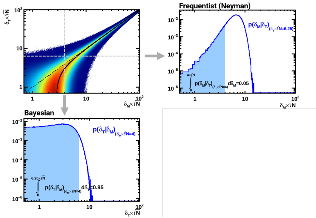
FIGURE B.1: (Top-left) Distribution of \delta_M for different values of \delta_T , both scaled by the sample size, \sqrt{N} . Solid black line shows the expected value of \delta_M according to the p(\delta_M|\delta_T) distribution for each value of \delta_T . (Top-right) Probability distribution function p(\delta_M|\delta_T) that ensures a probability content of 1 - \alpha = 0.05 for \delta_M \times \sqrt{N} = 4 according to Neyman prescription. (Bottom-left) Posterior probability p(\delta_T|\delta_M) for \delta_M \times \sqrt{N} = 4 and upper limit computation according to Bayesian prescription.
