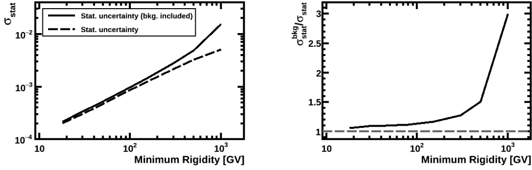
FIGURE 5.28: ( Left ) Absolute values of the statistical uncertainty for the proton sample when the sample is assumed to be pure (dashed line) and in the presence of background due to proton rigidity migrations (solid line). ( Right ) Ratio of the statistical uncertainties in the two cases, which quantifies the worsening in the uncertainty due to the background contamination in the proton sample.
