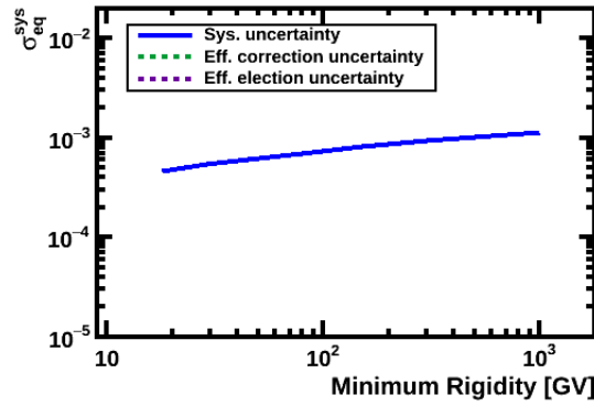
FIGURE 5.27: Contributions to the systematic uncertainty (blue solid line) from the efficiency correction uncertainty (green dotted line) and efficiency election uncertainty (purple dotted line). The systematic uncertainty is dominated by the efficiency correction one, without any contribution from the variation due to the election of significant corrections.
