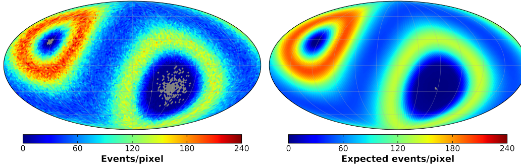
FIGURE 6.22: Skymap distribution of measured electrons ( left ) and expected number of events from the exposure time ( right ) in the energy range 16 < E < 350 GeV in galactic coordinates.
