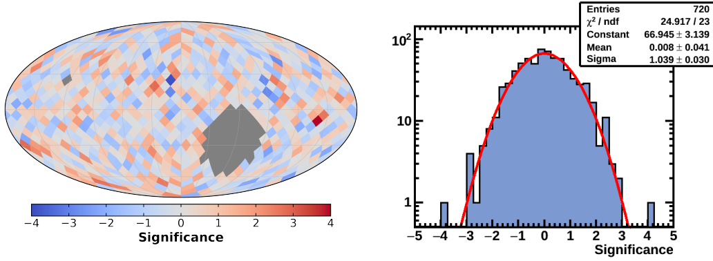
FIGURE 6.30: Significance skymap ( left ) and distribution ( right ) of the positron to electron skymap comparison for the energy range 16 < E < 350 GV in galactic coordinates.
