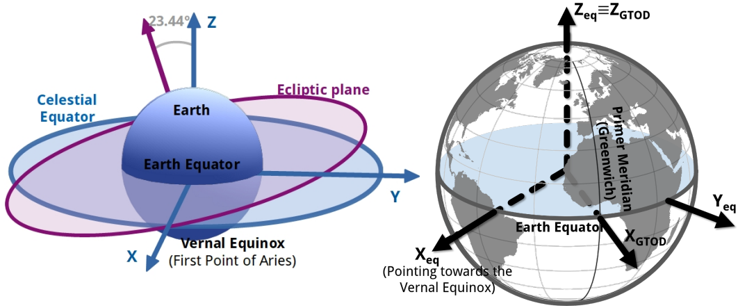
FIGURE 3.3: (Left) Definition of the equatorial coordinate system, with the X direction pointing towards the vernal equinox, and the celestial equator corresponding to the earth equatorial plane. The ecliptic plane, defined by the Earth's orbit around the Sun, is tilted 23.44^\circ with respect to the equatorial plane. (Right) Relation between GTOD and equatorial coordinates.
