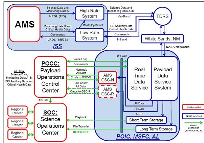
FIGURE 2.22: AMS-02 data flow. Data transmission to ground, by means of the HRDL and LRDL interfaces, is done by the NASA Tracking and Data Relay Satellites (TDRS). Data is received at ground at NASA White Sands Test Facility and directed to the Payload Operations Integration Center (POIC) at the Marshall Space Flight Center (MSFC). Finally, data is copied to the Payload Operations Control Center (POCC) and Science Operations Center (SOC) both at CERN Preveessin site, where operations take place [200].
