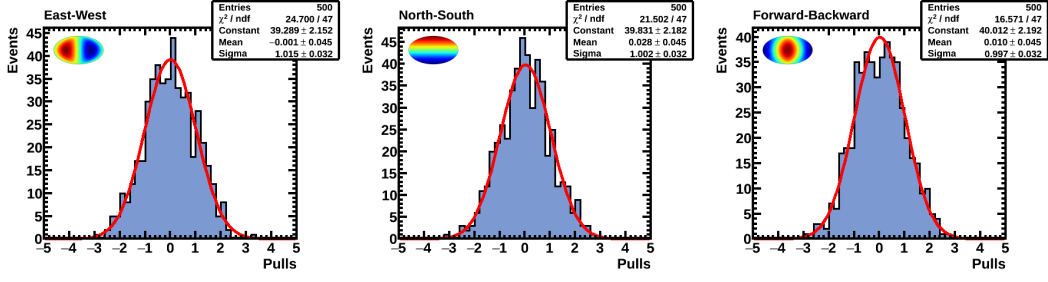
FIGURE 4.8: Distribution of pulls for the three dipole components obtained from a sampling of 500 Toy Monte Carlo simulations. The agreement with a normal distribution in each case is also displayed, and indicates that the statistical tools developed allow to determine the dipole components without bias.
