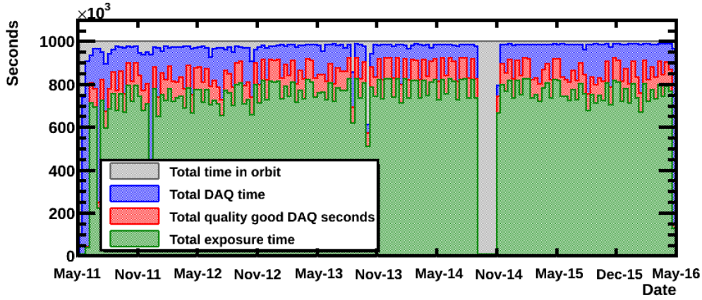
FIGURE 4.2: Time stability of the AMS-02 DAQ during the first 5 years in orbit analyzed in this thesis. The initial gap corresponds to the period of comissioning, from the AMS-02 activation to June 5, 2011. Finally, the gap from October till the end of November 2014 is due to a test of the tracker thermal control system.
