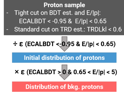
FIGURE 6.5: Scheme of the estimation of proton contamination according to method II.
