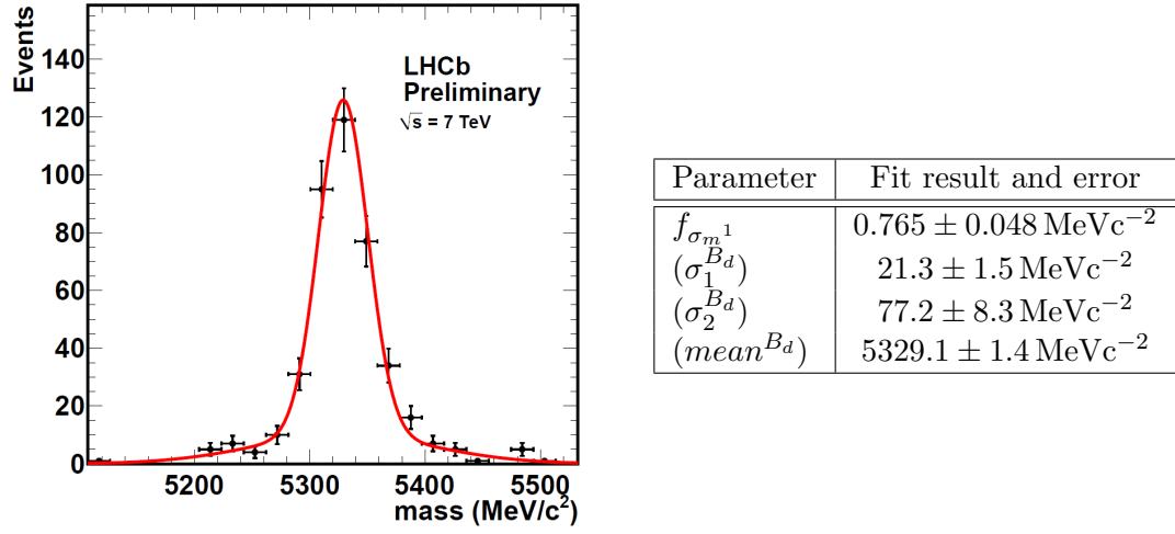
FIGURE 6.15: The mass projection and the fit results of the mass fit to the B_d \rightarrow D\pi data set selected using SelB.
