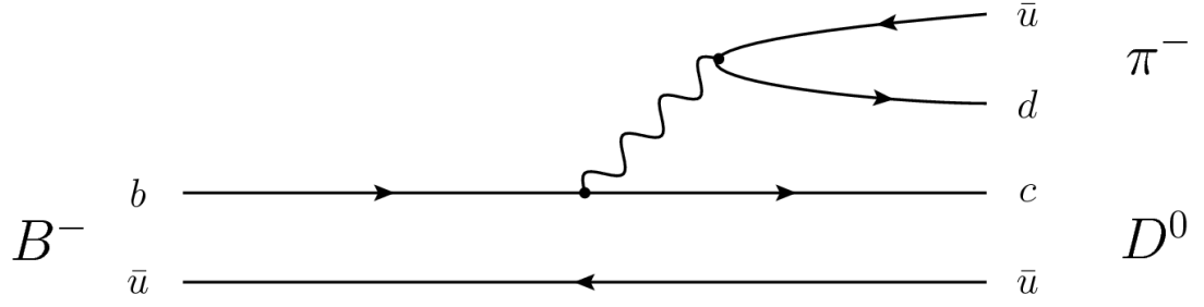
B^- decay via an external emission of a W boson.
