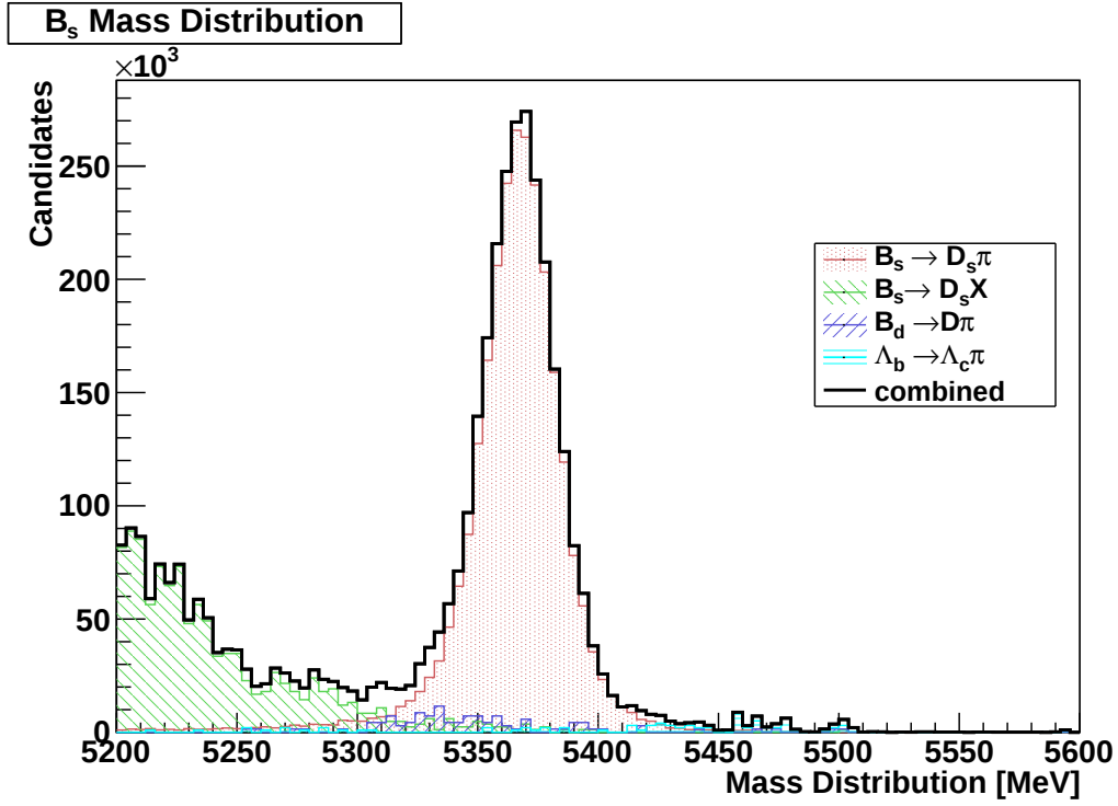
FIGURE 6.2: A normalised mass distribution of MC10 events passing the cuts SelA.
