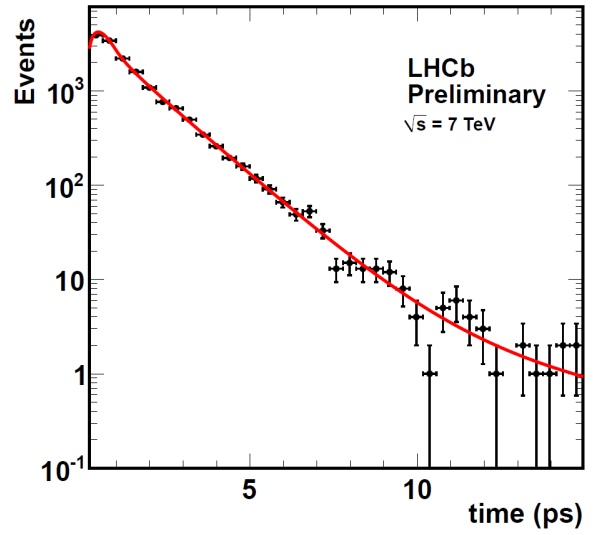
FIGURE C.8: SelB time projection of a full simultaneous fit to SelA and SelB data in the range 0 – 15 ps.
