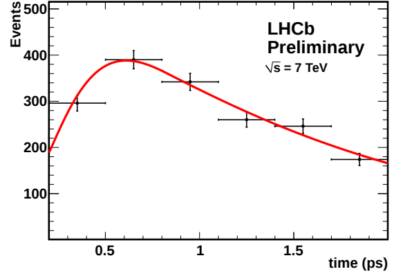
FIGURE 7.9: Projection of the upper side-band time distribution and fit to the SelA dataset in the lower proper-time acceptance region to demonstrate the fit to the proper-time acceptance.
