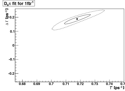
Figure 8: The 2d NLL contour plot corresponding to Figure 5. The solid line is 1\sigma and the dotted line is 2\sigma . The contours are now not symmetric about zero as the 1\sigma and 2\sigma boundaries are now constrained within one trough of \Delta\Gamma_s 's NLL. This results in a precision on \Delta\Gamma_s that cannot be believed.
