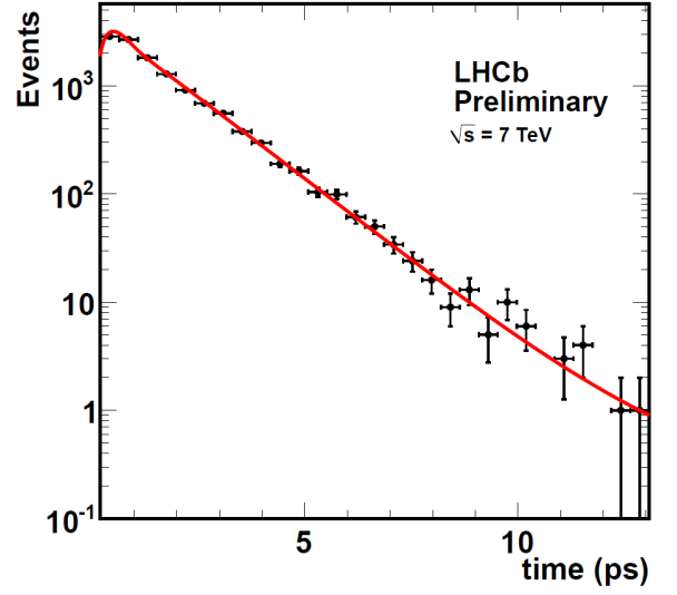
FIGURE C.2: Time projection of 0 – 15 ps fit to SelA with signal proper-time acceptance parameters fixed from MC.
