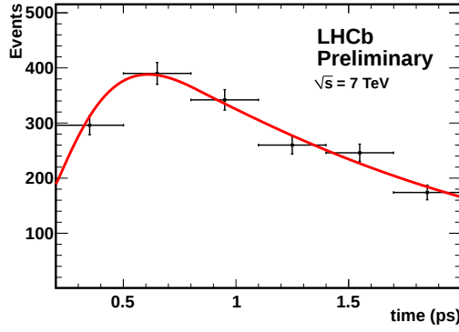
FIGURE 7.8: Projection of the lower side-band time distribution and fit to the SelA dataset in the lower proper-time acceptance region to demonstrate the fit to the proper-time acceptance.
