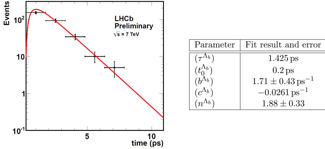
FIGURE 6.14: The time projection and the fit results of the proper-time fit to the \bar{\Lambda}_b \rightarrow \Lambda_c X MC10 data set.
