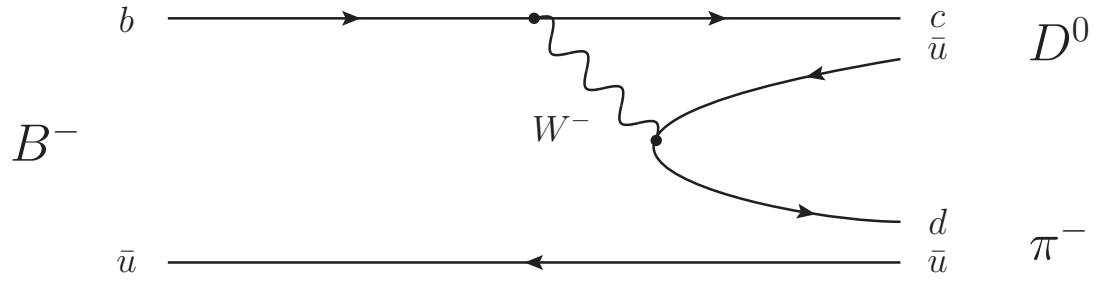
B^- decay via an internal emission of a W boson.
