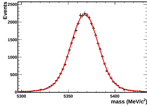
FIGURE 8.5: MC10 signal data fitted with a triple Gaussian function.
