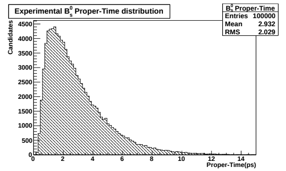
FIGURE 5.18: Example proper-time distribution after acceptance
