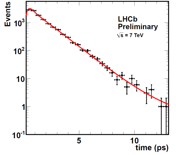
FIGURE C.7: SelA time projection of a full simultaneous fit to SelA and SelB data in the range 0 – 15 ps.
