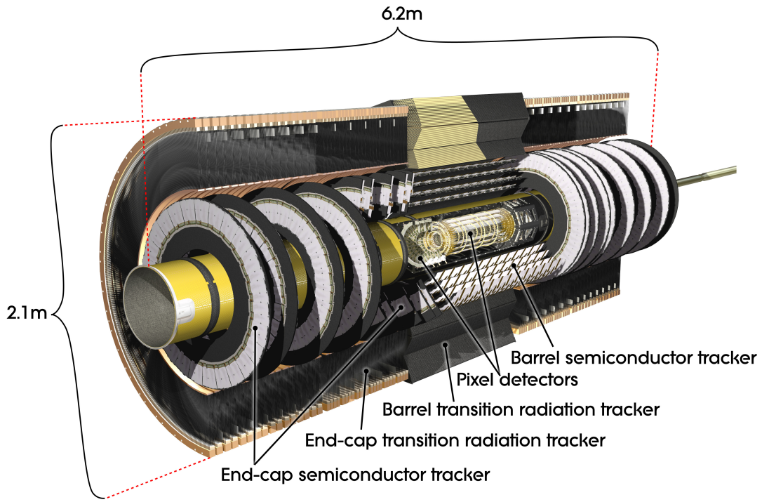
Figure 3.5: The ATLAS Inner Detector [49]
