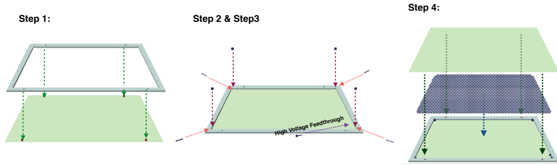
Figure 6.6: Schematic illustration of the drift panel construction.
