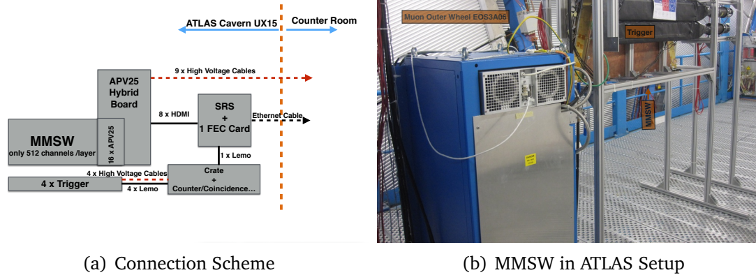
Figure 6.25: The cable connection and the operation scheme for the prototype test in the ATLAS cavern (left plot). And the set up for the test of MMSW in the ATLAS cavern (right plot).
