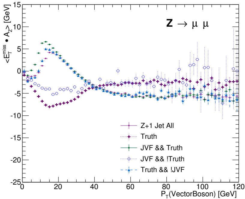
Figure 4.14: Response of E_T^{\text{miss}} with varying truth central jet matching and JVF cut conditions are as shown. The jet p_T threshold is kept at 20 GeV, and the thresholds on |JVF| are at 0.25.
