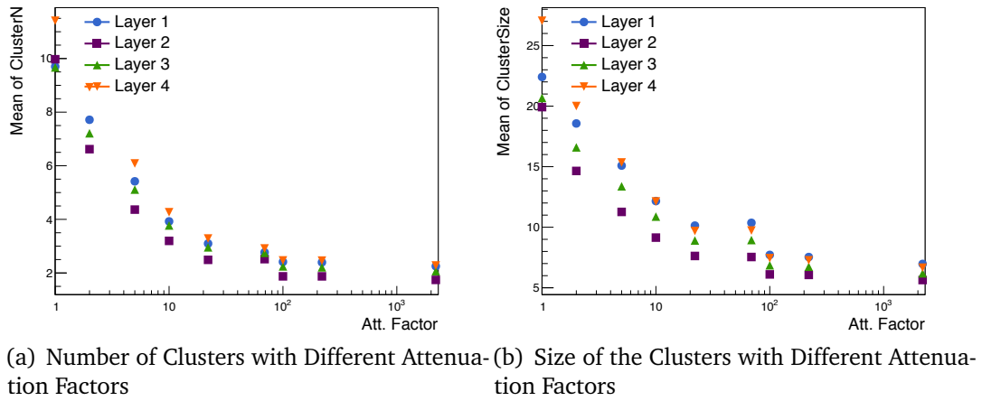
Figure 6.24: The features of the clusters with different attenuation factors in the GIF++ measurement. The higher attenuation gives a smaller clusters size, and fewer clusters.
