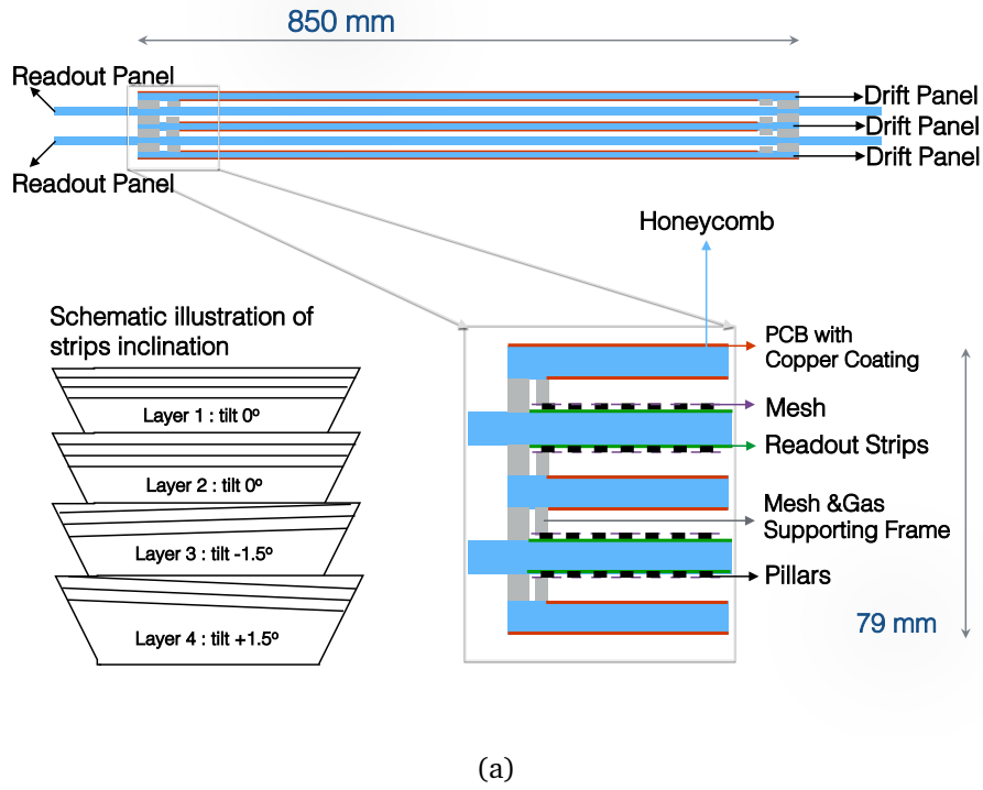
Figure 6.4: The layout design of the MMSW detector is summarized on the plot. The upper plot is the bottom view of the chamber, two readout panels are between three drift panels and are 20 cm longer to hold the electronics. The bottom left plot indicates the geometry of the readout strips with parallel strips in the first two layers and a tilt of \pm 1.5 degrees for the third and fourth layers. The detailed cut-away view is shown in the bottom right plot.
