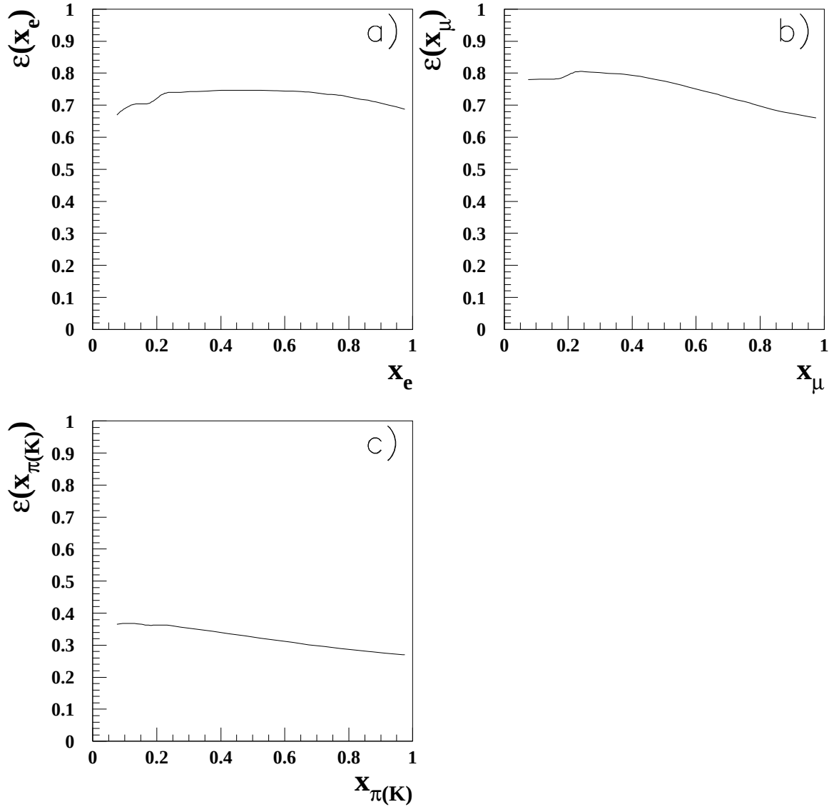
Figure 5.6: Global efficiencies as a function of x for a) \tau \rightarrow e \bar{\nu}_e \nu_\tau b) \tau \rightarrow \mu \bar{\nu}_\mu \nu_\tau and c) \tau \rightarrow \pi(K) \nu_\tau decays. The efficiencies include the 93% tau-pair selection efficiency and are after the fiducial cut of |\cos \theta| < 0.68 . The complex behavior in the low and high x regions of a) and b) are caused by requirements designed to remove two-photon, Bhabha and mu-pair events.
