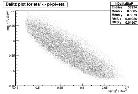
(c) Dalitz plot for the \eta' decay. The plot is much more homogeneous than the corresponding Fig. 4.8c for the \eta \rightarrow \pi^-\pi^+\pi^0 decay.
