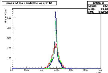
Figure 4.13.: Effect of kinematical fit. The picture shows how the kinematical fit of the \eta' \rightarrow 4\pi\gamma\gamma improves the quality of the selection. Details, see text.
