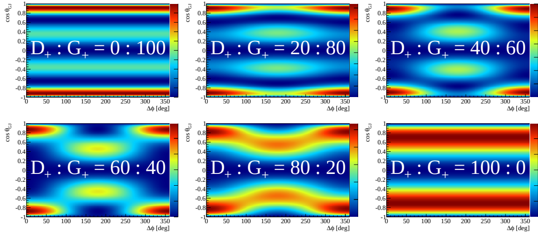
Figure 7.3.: As Fig. 7.1 for D_+ and G_+ wave interference.
