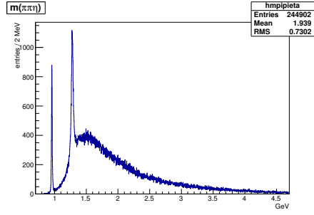
(a) Intermediate \pi^-\pi^+\eta spectrum showing \eta'(958) and f_1(1285) peaks. Two entries per event.
