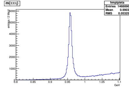
(b) Zoom on the \eta' region in Fig. 4.9a.
