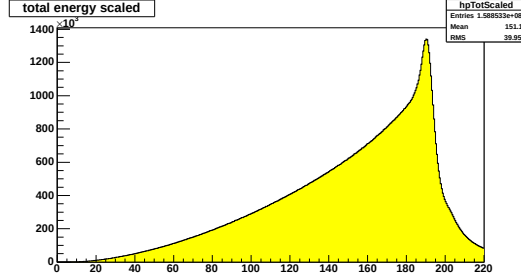
Figure 4.5.: Total energy distribution in the pre-selection sample.
