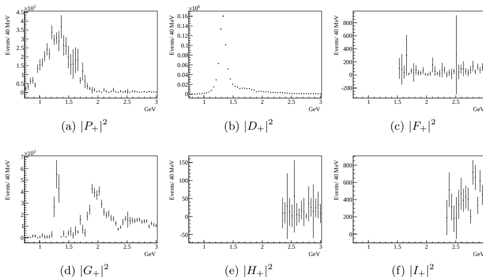
Figure 8.22.: Intensitis of natural-parity waves for the \eta\pi^- data when including additional waves (see text).
