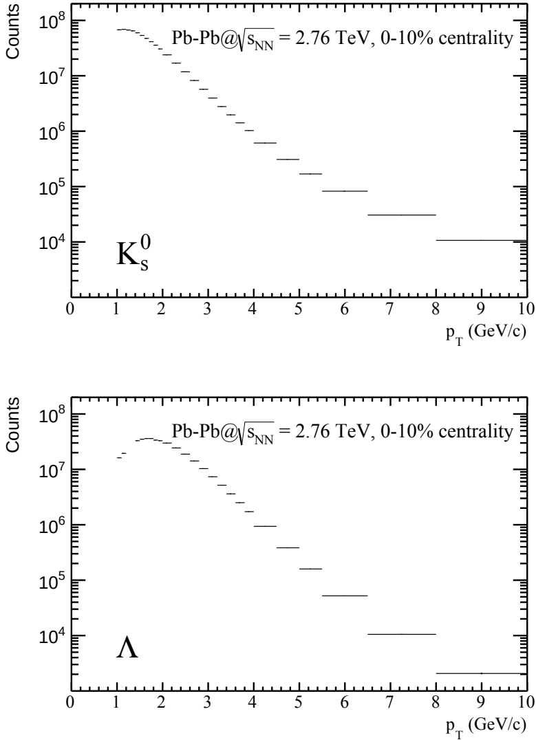
Figure 5.13: Uncorrected (with respect to efficiency and feed-down) p_T spectra for Pb-Pb at \sqrt{s_{NN}} = 2.76 TeV, 0-10% centrality. The spectra are normalized to the p_T bin width.
