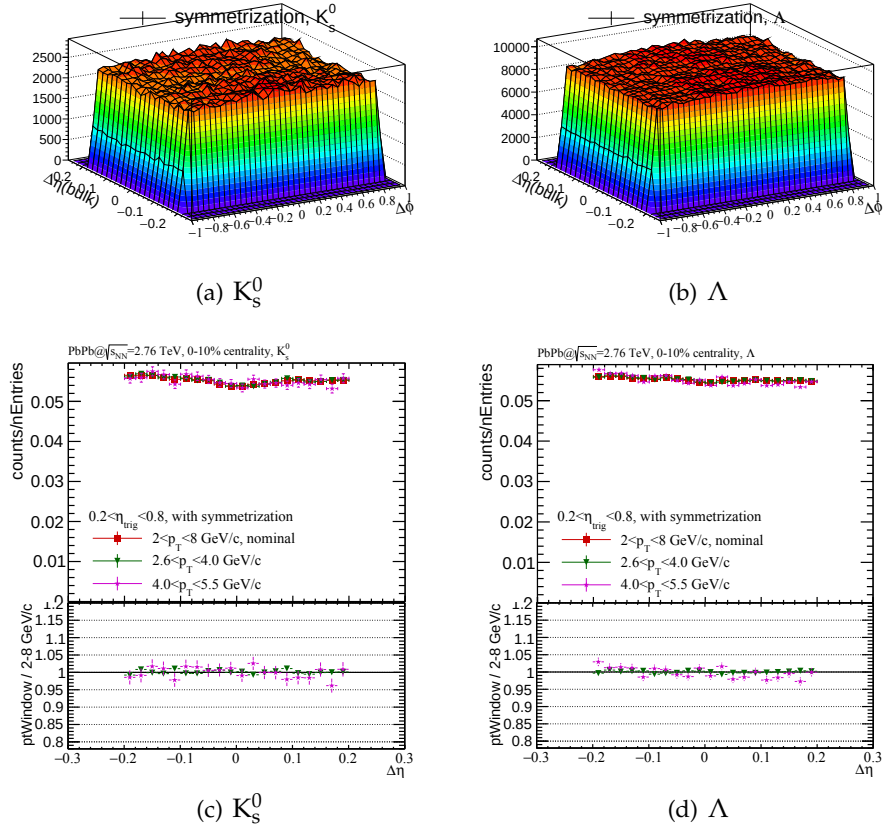
Figure 5.33: Top: \Delta\eta\Delta\phi for the bulk region with trigger particle acceptance region 0.2 < |\eta_{trig}| < 0.8 , and symmetrization applied. Bottom: Projection of \Delta\eta for the bulk region for different p_T -intervals.
