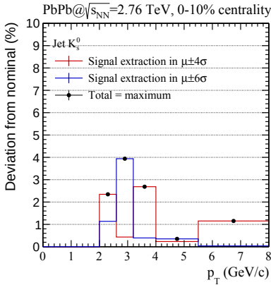
(e) K_s^0 jet
