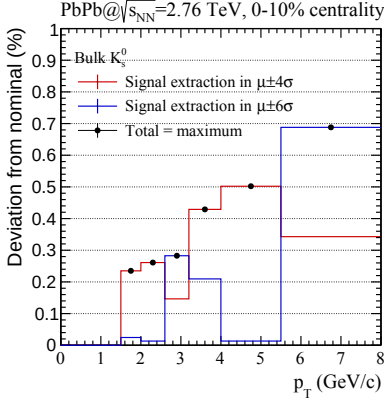
(a) K_s^0 bulk
