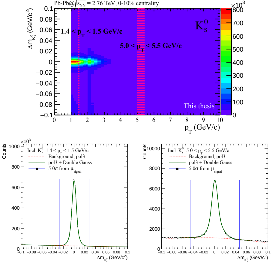
Figure 5.11: Invariant mass distribution of K_S^0 candidates in Pb-Pb at \sqrt{s_{NN}} = 2.76 TeV, 0-10% centrality. The top figure shows the invariant mass vs. p_T , with two red bands indicating where the example projections are done for the lower two histograms. The projection-histograms thus show the invariant mass distribution for 1.4 < p_T < 1.5 GeV/c and 5.0 < p_T < 5.5 GeV/c, with the double Gaussian (signal) + polynomial (background) fitting function (green). The polynomial part of the fitting function is shown as the dashed red line to indicate the background. The two vertical blue lines represent the 5\sigma region in which the signal is extracted.
