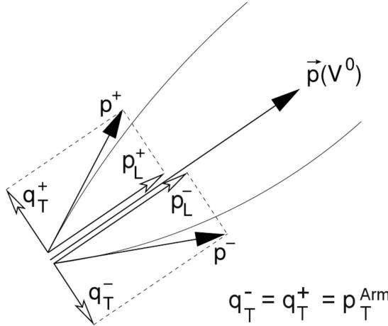
Figure 5.9: The parameters of the Armenteros-Podolanski Diagram derived from the transverse and longitudinal momentum components of the positively and negatively charged track, with respect to the direction of the reconstructed V0 momentum.
