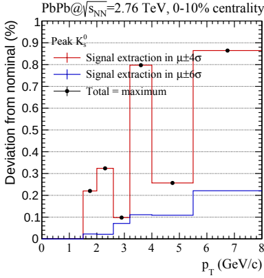
(c) K_s^0 peak
