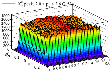
(a) K_S^0 : 2.0 < p_T < 2.6 GeV/c
