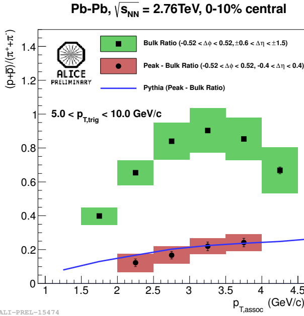
Figure 7.5: p/\pi ratio as a function of associated particle p_T , in bulk and peak-bulk for 0-10% central Pb-Pb collisions at \sqrt{s_{NN}} = 2.76 \text{ TeV} , with a leading (trigger) particle p_T between 5 – 10 GeV/c [96].
