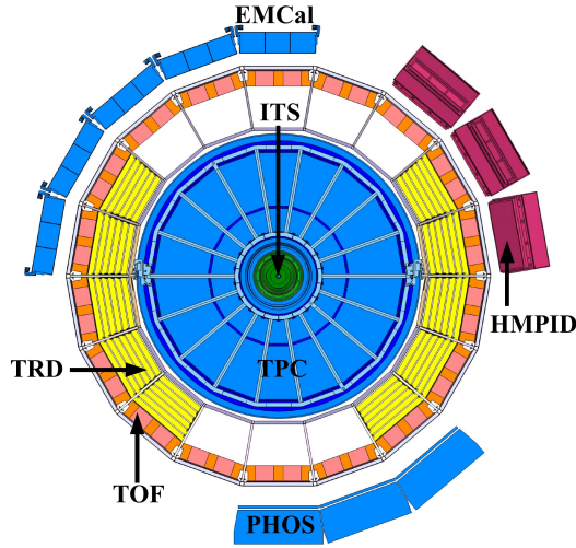
Figure 4.2: Cross section of the ALICE central barrel detectors. Schematic Illustration Credits: Jochen Thaeder (ALICE).
