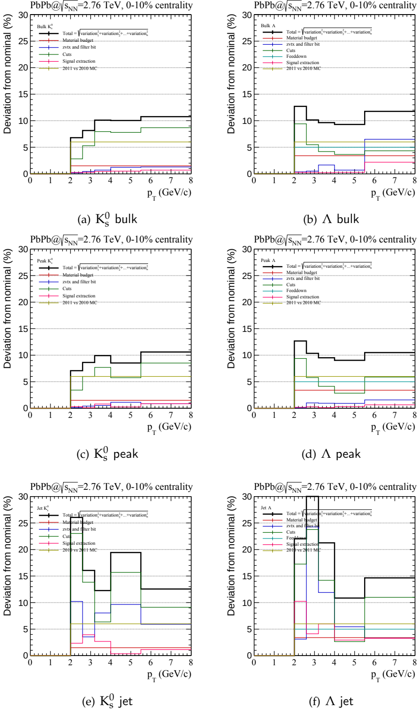
Figure 5.50: Total systematic uncertainty.
