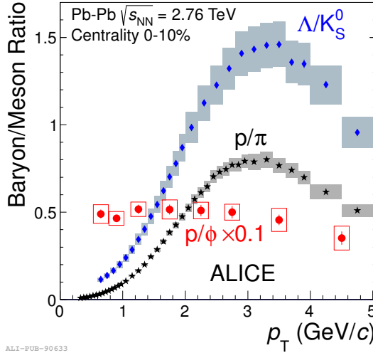
Figure 3.15: Ratio p/\phi (scaled with 0.1 for visibility) as a function of p_T up to 5 GeV/c for 0-10% central Pb-Pb collisions at \sqrt{s_{NN}} = 2.76 TeV, compared to \Lambda/K_S^0 and p/\pi in the same centrality bin. Figure taken from [69].
