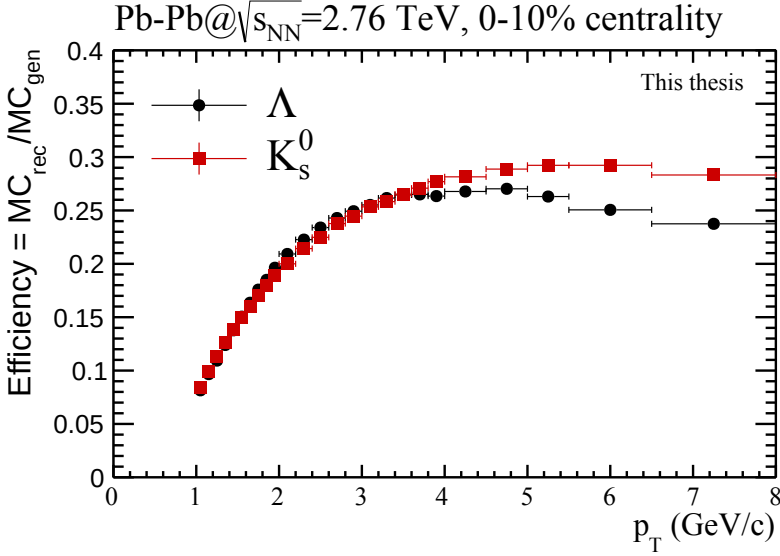
Figure 5.15: K_S^0 and \Lambda efficiency for Pb-Pb at \sqrt{s_{NN}} = 2.76 TeV, 0-10% centrality.
