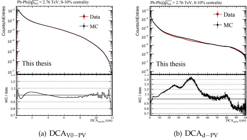
Figure 5.6: The different cut parameters for V0 candidates with p_T > 1.0 GeV/ c
