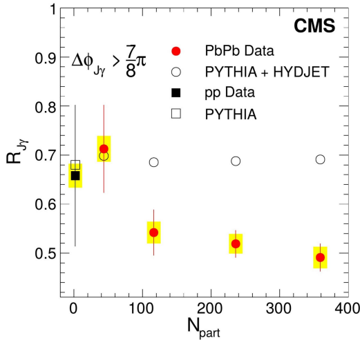
Figure 7.3: Average fraction of isolated photons with an associated jet above 30 GeV/ c , R_{J\gamma} , as a function of N_{part} . The yellow boxes indicate point-to-point systematic uncertainties and the error bars denote the statistical uncertainty. Figure and caption taken from [94].
