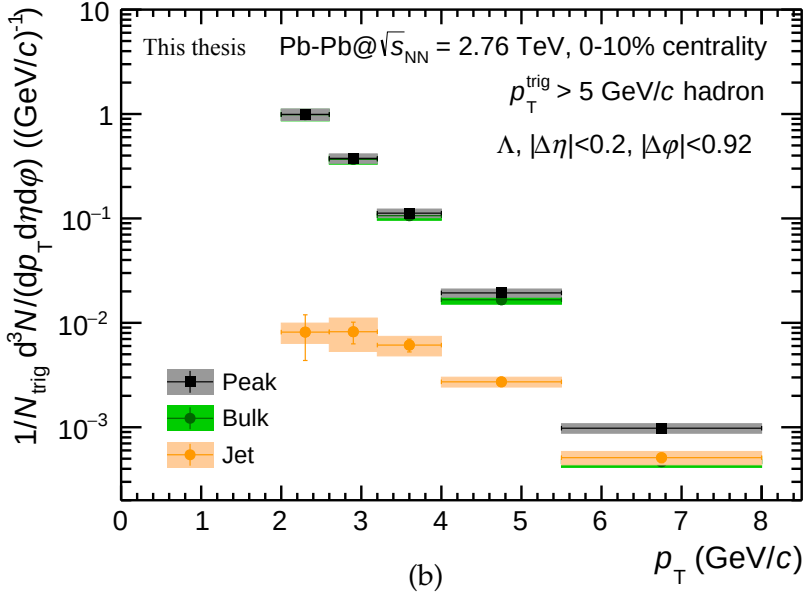
Figure 6.1: Corrected bulk, peak and jet yields as a function of p_T , for (a) K_S^0 , and (b) \Lambda , with the 2011-recorded Pb-Pb collisions at the center-of-mass energy \sqrt{s_{\text{NN}}} = 2.76 TeV, in the 0-10% centrality bin. Full statistical (bars) and systematic (boxes) uncertainties are applied.
