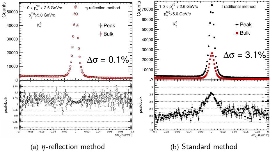
Figure 5.2: \Delta m_{K_S^0} for the peak and bulk regions in 1.0 < p_T < 2.6 GeV/c comparing the different analysis methods. The ratio plot shows the peak/bulk.
