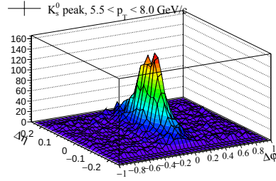
(b) K_S^0 : 5.5 < p_T < 8.0 GeV/c
