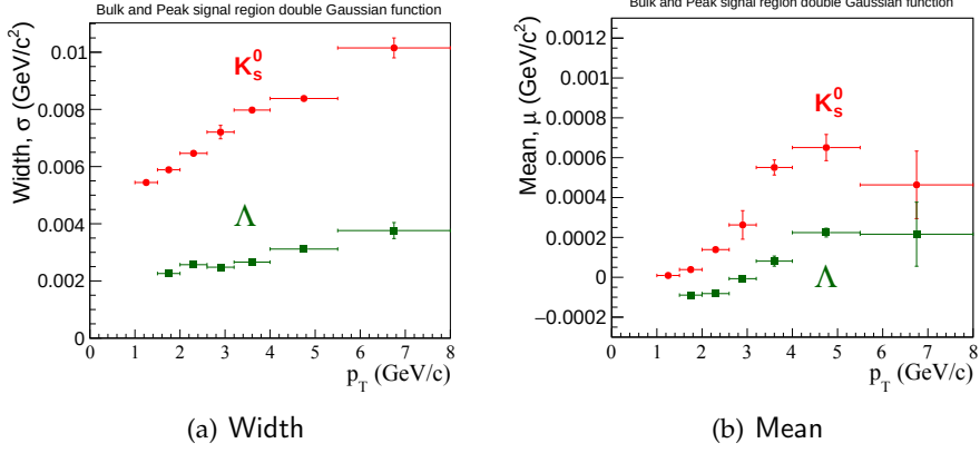
Figure 5.28: The means and widths of the double Gaussian fitted to the peak and bulk signal region.
