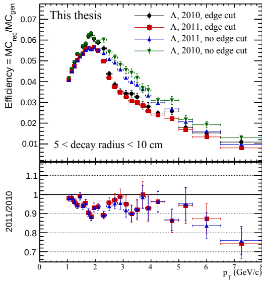
Figure 5.22: \Lambda efficiency for 5 < r_T^{dec} < 10 cm, with and without the edge cut.
