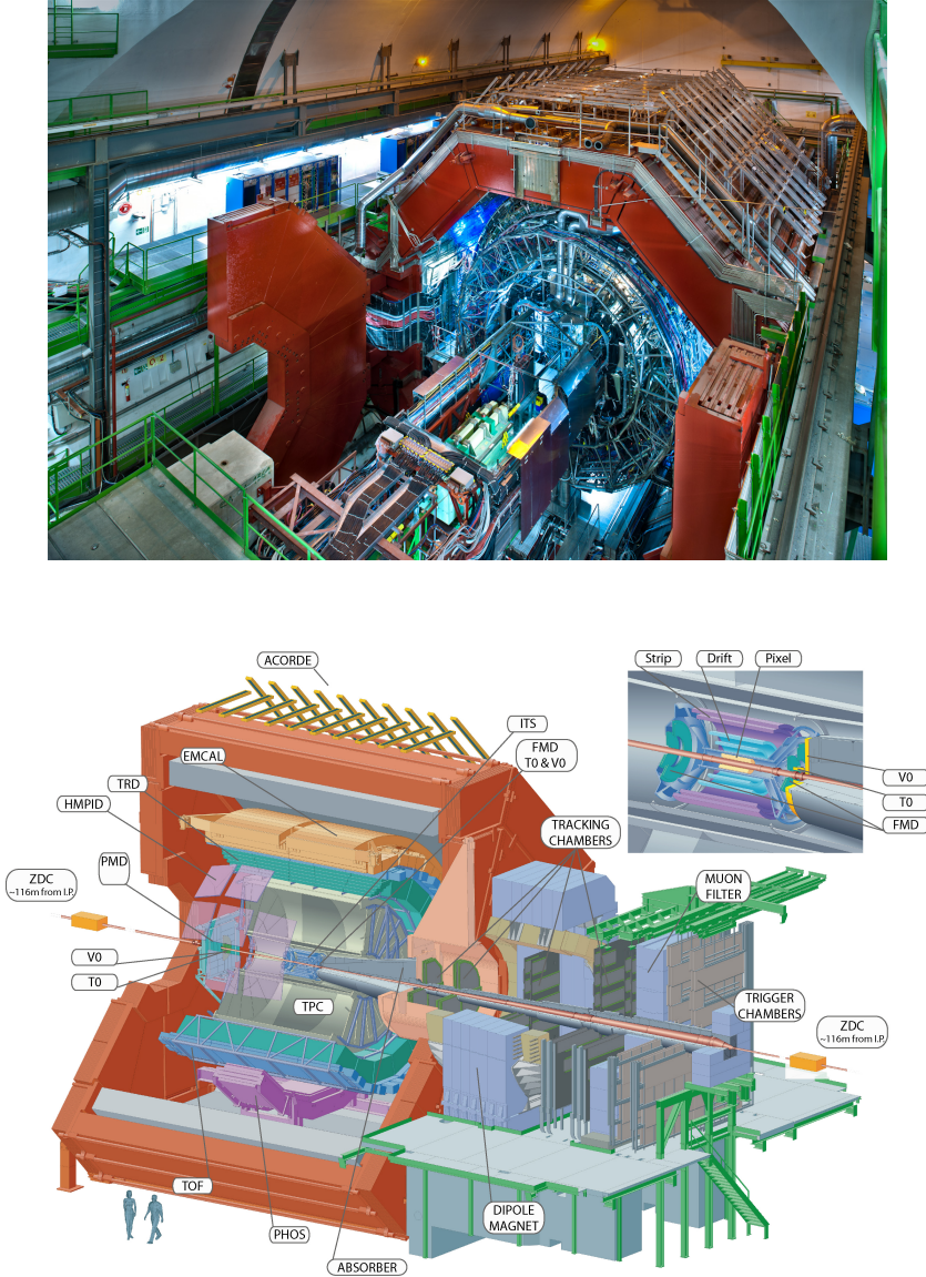
Figure 4.1: The ALICE experiment. The central-barrel detectors (ITS, TPC, TRD, TOF, PHOS, EMCal, and HMPID) are inside in a solenoid with magnetic field B = 0.5 T and address particle production at mid-rapidity. Forward detectors (PMD, FMD, V0 (called VZERO in the text), T0, ZDC, and the MUON-arm) are used for triggering, event characterization, and multiplicity studies. Photo from CERN Document Server: ALICE-PHO-GEN-2012-001-12. Schematic Illustration Credits: Jochen Thaefer (ALICE).
