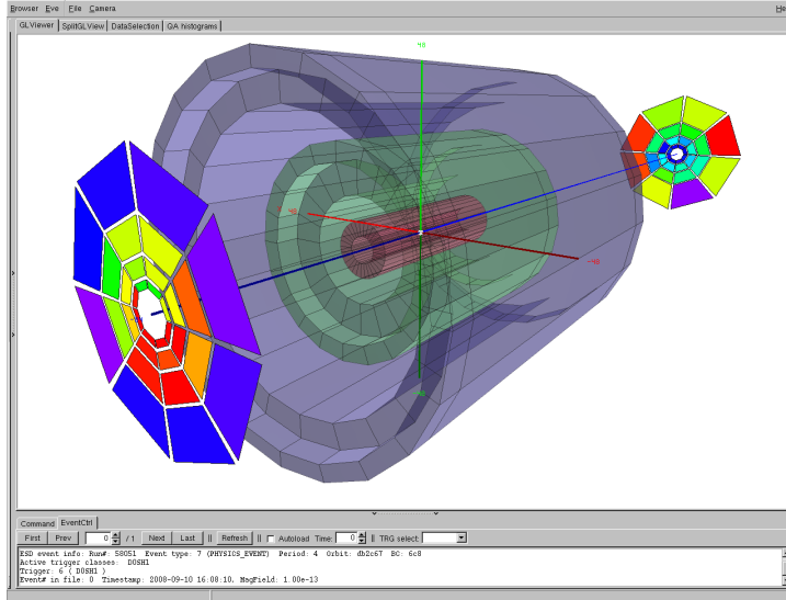
Figure 4.6: A display with the ITS and VZERO detector, illustrating the detector layout.
