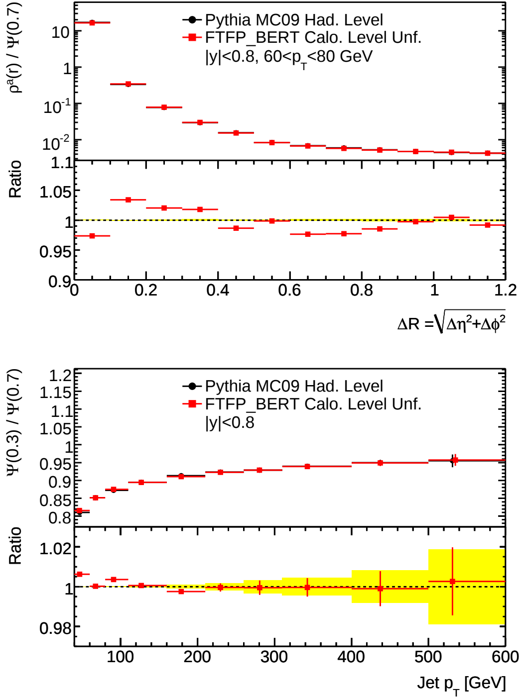
Figure 5.14: Comparison of the jet shapes \rho^a(r) / \Psi(0.7) (top) and \Psi(0.3) / \Psi(0.7) (bottom) with the FTFP_BERT physics list after unfolding using the QGSP_BERT physics list. The difference between the hadron-level distribution and the unfolded calorimeter-level distribution is the unfolding bias in this sample.
