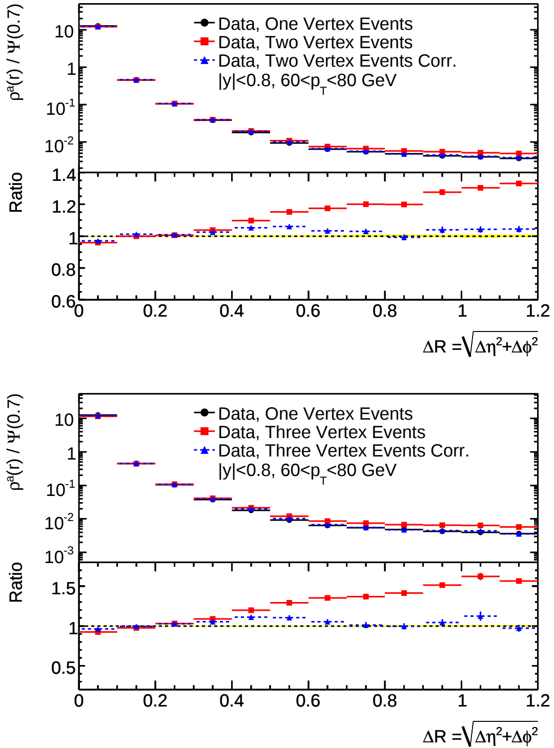
Figure 5.28: Comparison of jet shapes in events with one and two (top) or one and three (bottom) vertices, before and after an offset correction has been applied.
