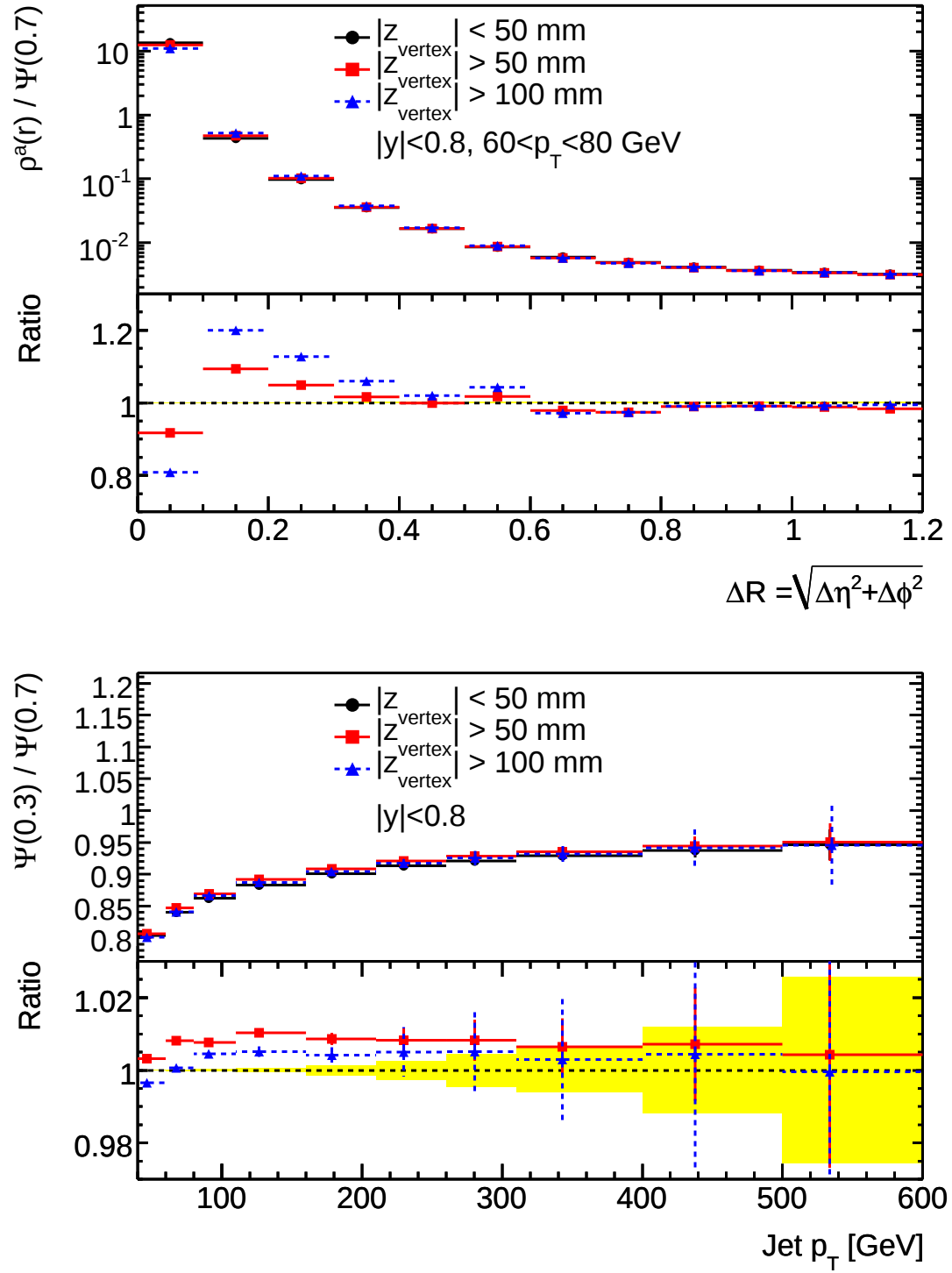
Figure 5.17: Comparison of unfolded reconstructed and hadron-level jet shapes in events with a displaced reconstructed vertex.
