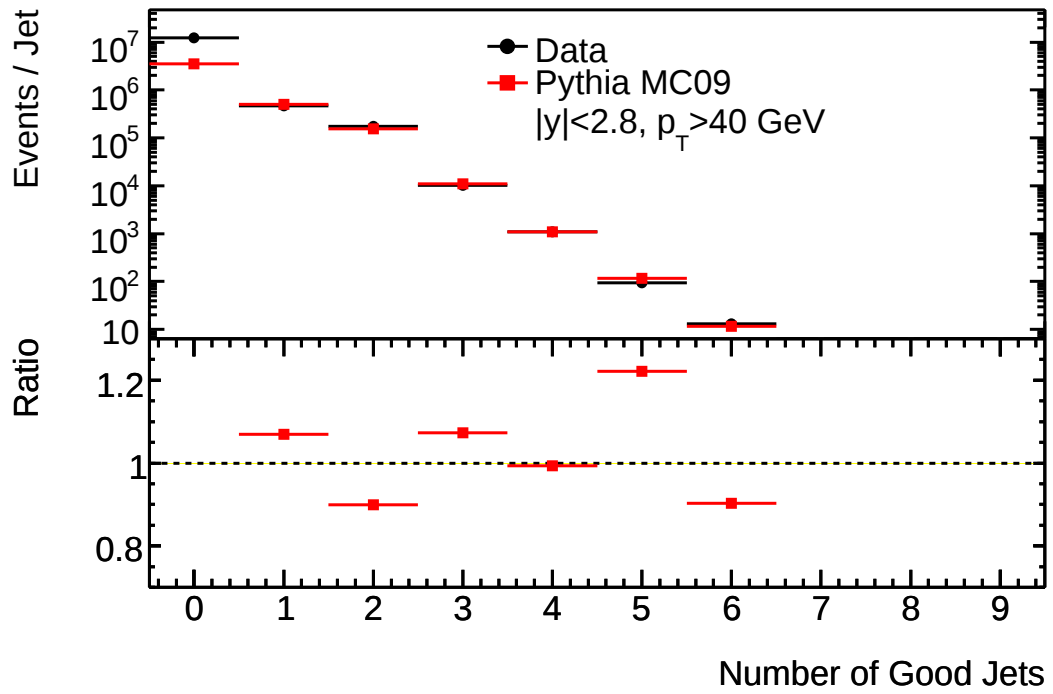
Figure 5.11: Number of jets per event passing all quality cuts with |y| < 2.8 and p_T > 40 \text{ GeV} . The samples are scaled to the same number of good jets.
