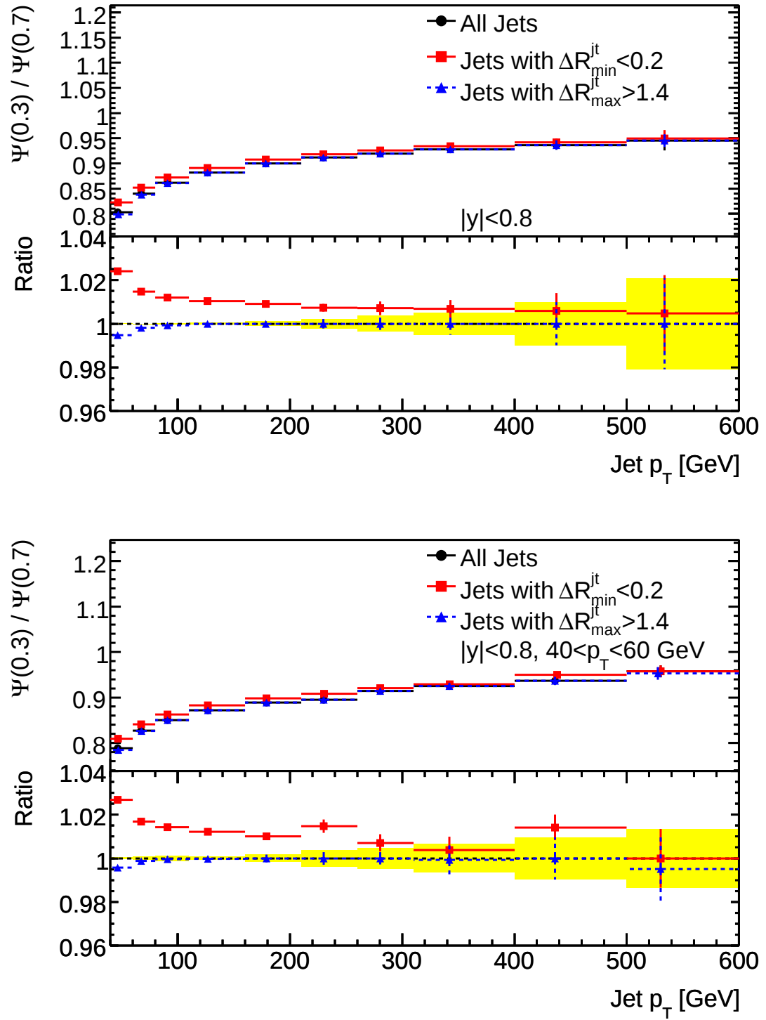
Figure 5.23: Comparison of jet shapes in jets which overlapped in various ways with a trigger jet in Monte Carlo (top) and data (bottom).
