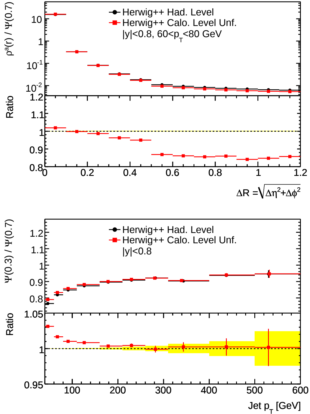
Figure 5.16: The jet shapes \rho^a(r) / \Psi(0.7) (top) and \Psi(0.3) / \Psi(0.7) (bottom) in Herwig++ at the hadron level and after unfolding based on Pythia's MC09 tune.
