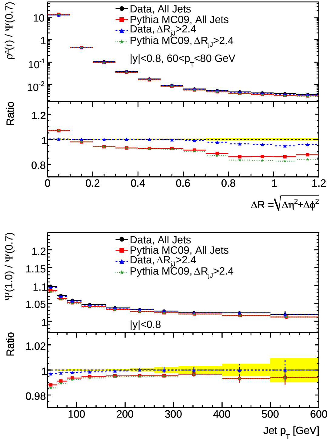
Figure 5.25: Comparison of jet shapes in jets which were far from ( \Delta R > 2.4 ) any jet of higher p_T and all jets.
