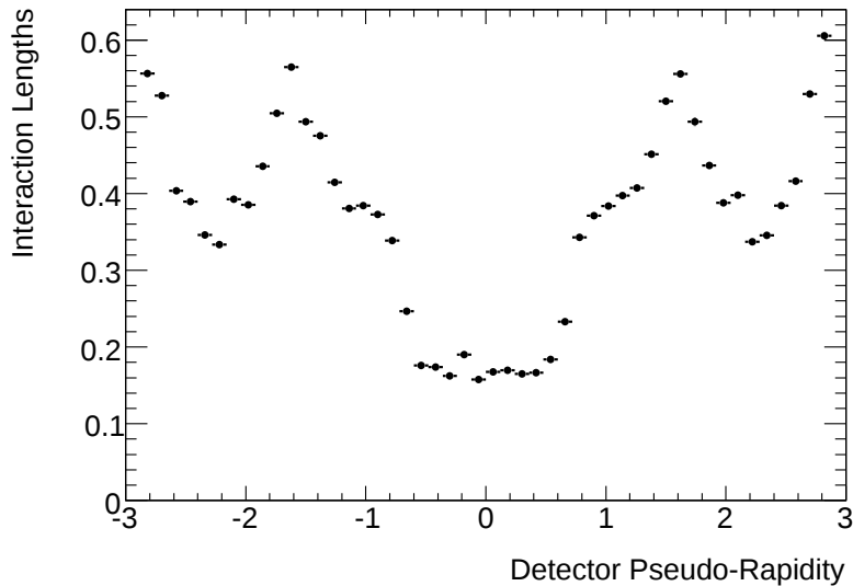
Figure 5.15: The number of interaction lengths before entering an active portion of the calorimeter.
