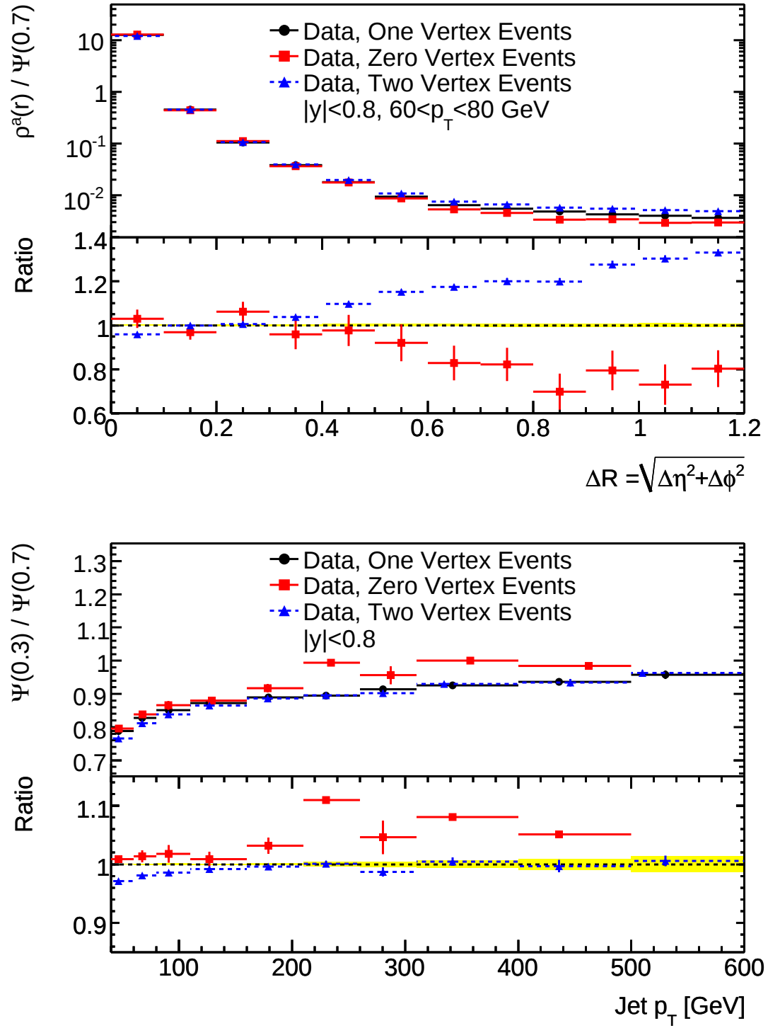
Figure 5.24: Comparison of jet shapes in events with varying numbers of reconstructed primary vertices. Two-vertex events are markedly wider than single-vertex events.
