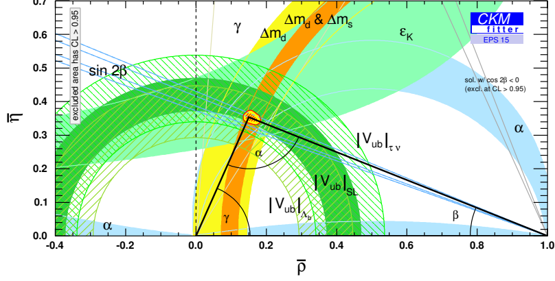
Figure 1.2: Constraints in the (\bar{\rho}, \bar{\eta}) plane [44], updated results and plots available at: http://ckmfitter.in2p3.fr . Testing the unitarity of the CKM matrix is an important consistency check of the SM.
