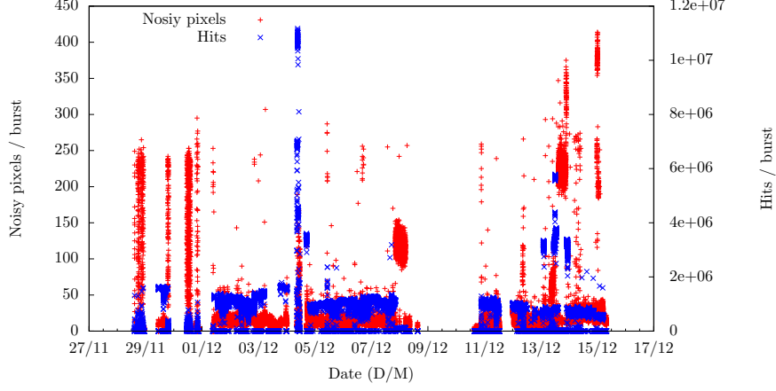
Figure 4.23: The number of noisy pixels varies greatly and returns to the baseline when the DAQ is reset. This behaviour is surprising at the first sight. The data are from the detector GTK_1.
