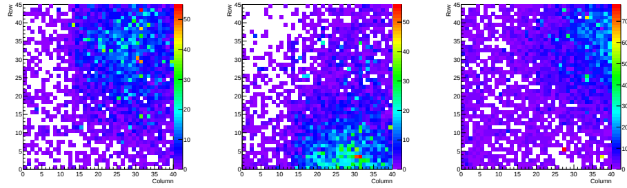
Figure 4.31: Hit maps of the coincidences between the three stations, dataset P3. The pixels of the column 0 and 39 are larger ( 400\text{ }\mu\text{m} instead of 300\text{ }\mu\text{m} ). The color scale indicates the number of coincidence between a particular pixel of a station and any pairs of pixels of the two other station. GTK_2 (first station) is on the left, GTK_3 (second station) is in the centre and GTK_1 (third station) is on the right.
