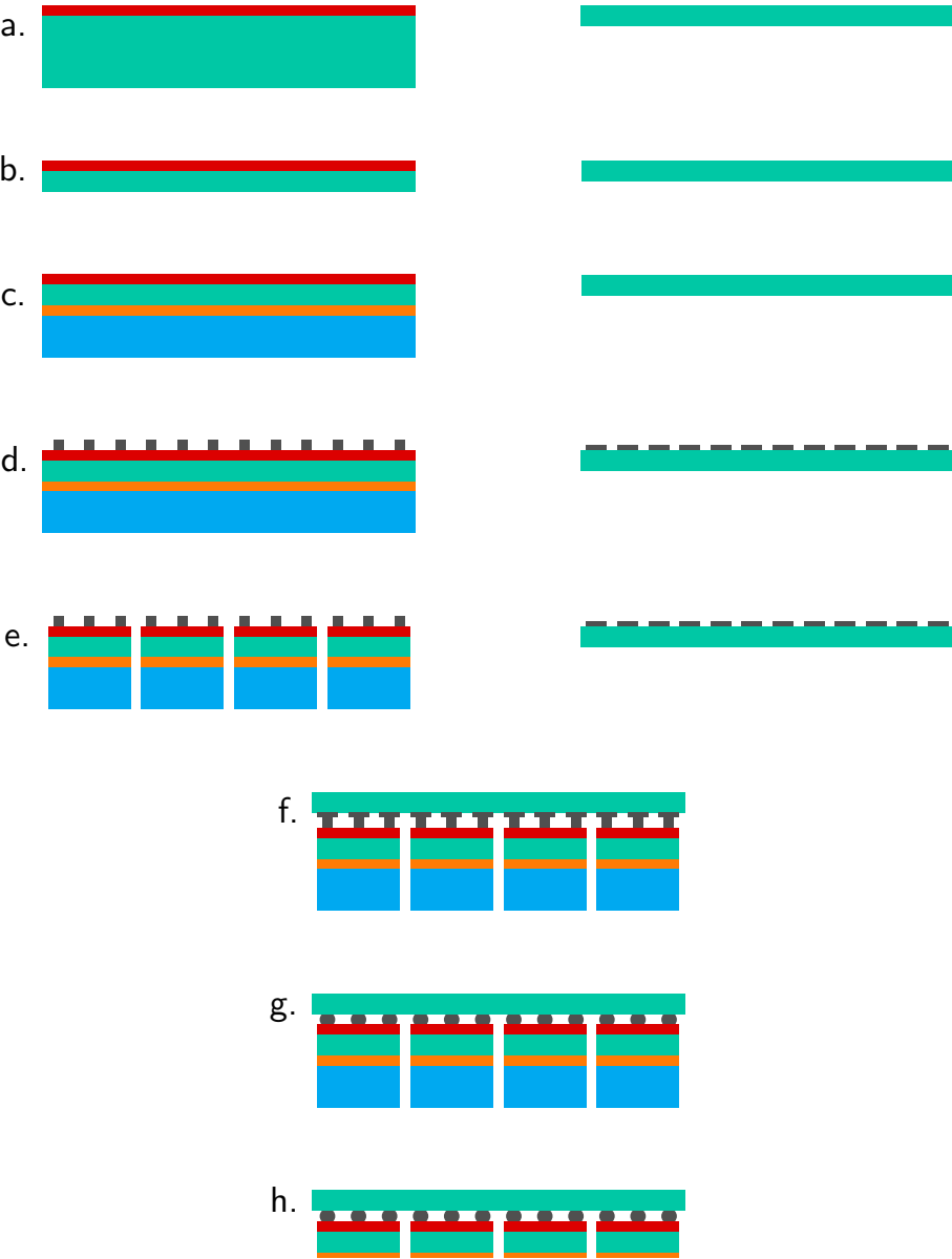
Figure H.1: Simplified sketch of the flip chip process. See the text for details.
