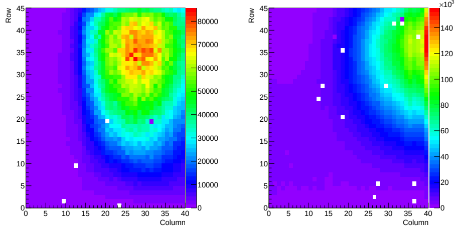
Figure 4.30: Hit maps of the coincidences between the first and third stations, dataset P5. The pixels of the column 0 and 39 are larger ( 400\text{ }\mu\text{m} instead of 300\text{ }\mu\text{m} ). The color scale indicates the number of coincidence between a particular pixel of a station and all the others pixels of the other station. GTK_2 (first station) is on the left and GTK_1 (third station) is on the right. We see the focusing effect of the magnetic field on the beam.
