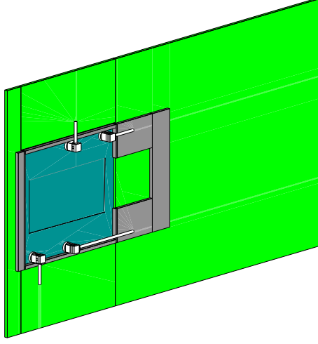
Figure 3.19: Downstream view, aluminum frame (gray).
