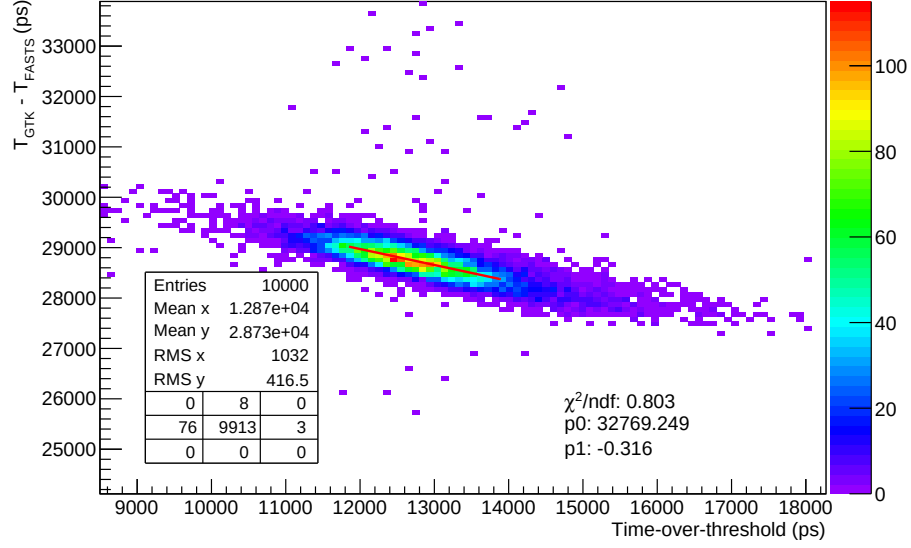
Figure 3.25: Typical linear ( TW_{\text{corr}} = p_0 + p_1 \cdot \text{ToT} ) time walk correction curve. This particular one is for the pixel 44 of the GTK2 demonstrator at a bias voltage of 300 V. The FASTS detector provided an accurate time reference. The color scale indicates the number of entries per 97.7 \text{ ps} \times 97.7 \text{ ps} bin. The results obtained with the GigaTracker demonstrator are described in Section 4.1.
