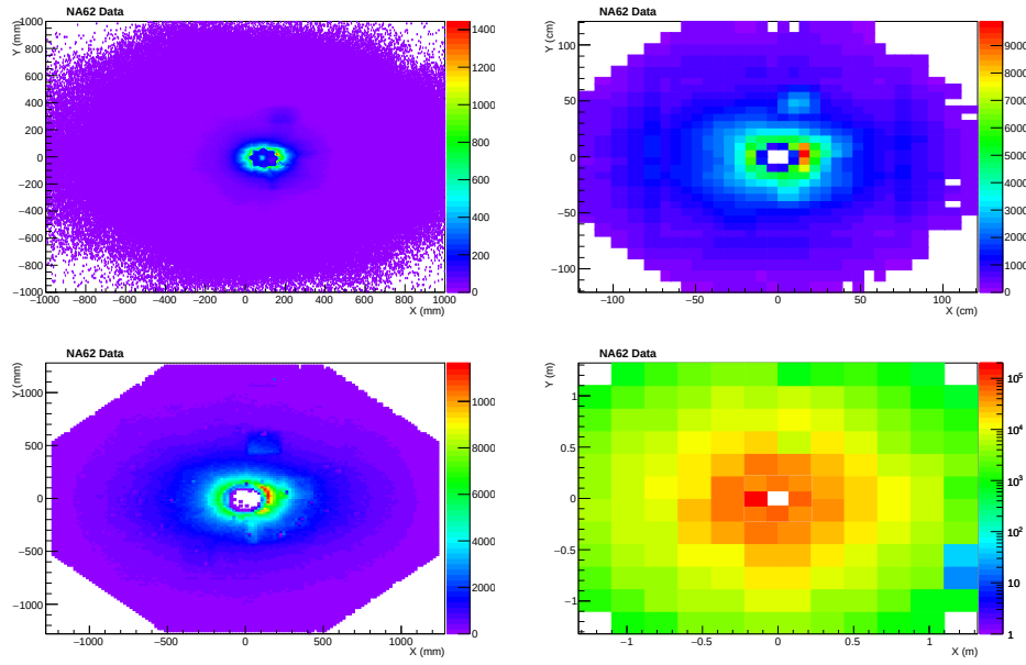
Figure 4.50: STRAW (top left), CHOD (top right) LKr (bottom left) subdetector illumination under the Q1 \times \text{!MUV3} condition. The beam component is visible on the right of the beam pipe gap. MUV3 (bottom right) illumination under the Q1 condition. A tile close to the center is clearly inefficient. The beam direction points out of the page.
