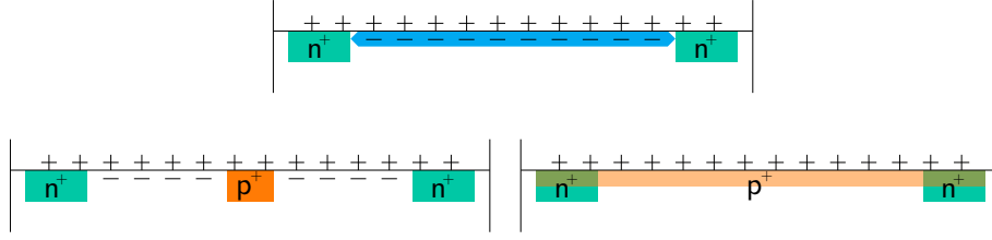
Figure 3.5: Sketch of an n-in-p type sensor. Positive charges tends to accumulate at the silicon oxide-silicon interface. If nothing is done, an electron layer just below the silicon oxide creates a low resistivity path between adjacent pixel implants (top). Two common techniques to circumvent to problem are the p-stop (bottom left) and the p-spray (bottom right) implantation.
