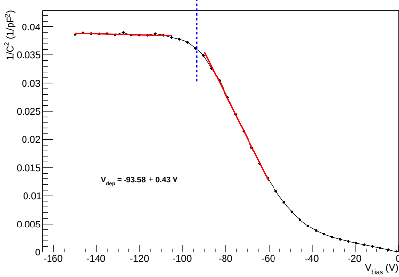
Figure 3.13: Typical 1/C^2 -V curve. The full depletion voltage is determined by the intersection of the two fitted curves. This particular curve is for the diode 2 diced from the wafer 1; it was exposed to 10^{14} 1 MeV eq. n \text{cm}^{-2} .
