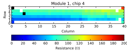
Figure H.9: Daisy chain resistance measurements on chip 4 of assembly 1.
