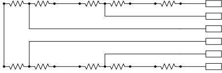
Figure H.3: Simplified electric scheme of the daisy chains. The rectangles represent the dummy chip pads.
