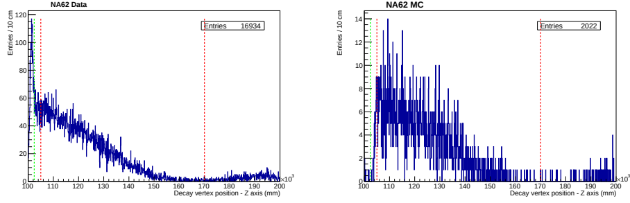
Figure 4.55: Reconstructed decay vertices of the three charged tracks decays. The red lines indicates the selection while the green line shows the position of the third GigaTracker station.
