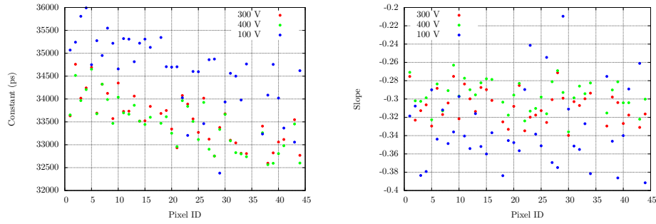
Figure 3.26: Illustration of the variation of the time walk correction factors. We see that the correction has to be computed separately for every pixel and every bias voltage. These correction factors were computed for the GTK2 demonstrator using data collected during a test beam; refer to Section 4.1 for more details.
