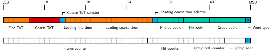
Figure E.3: timestamp - (top) and frame - (bottom) type 48-bit data word. The orange and red bit fields contain information about the timing while the green fields allow to reconstruct the position of the hit. The orange fields are encoded in Gray, all the other are encoded in binary.
