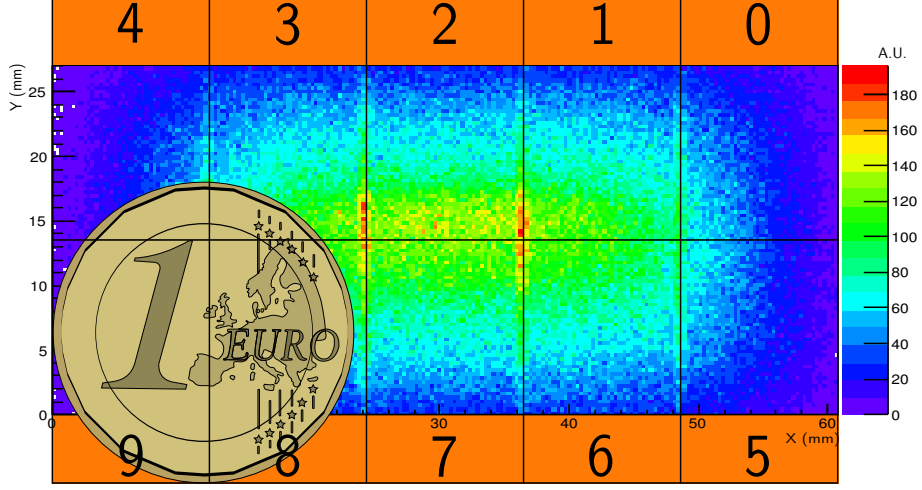
Figure 3.6: GigaTracker readout ASIC numbering scheme superimposed on the simulated illumination of the sensor. The orange areas represent the “end of column” regions of the readout chips where most of the TDCpix digital logic is implanted. The higher rates in the inter-chip regions is due to the larger pixel size.
