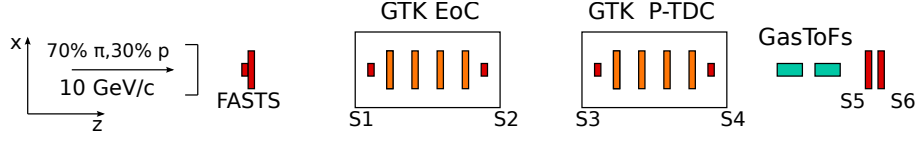
Figure 4.1: Schema of test beam experimental setup viewed from the top. Only the FASTS and the GTK EoC detectors were used in the present analysis. The beam is going from left to right.
