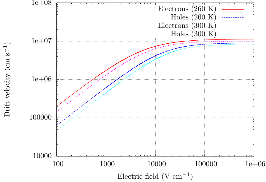
Figure 2.2: Charge carrier drift velocity in silicon at 300 K and 260 K.
