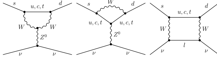
Figure 1.3: K \rightarrow \pi\nu\bar{\nu} topologies in the SM.
