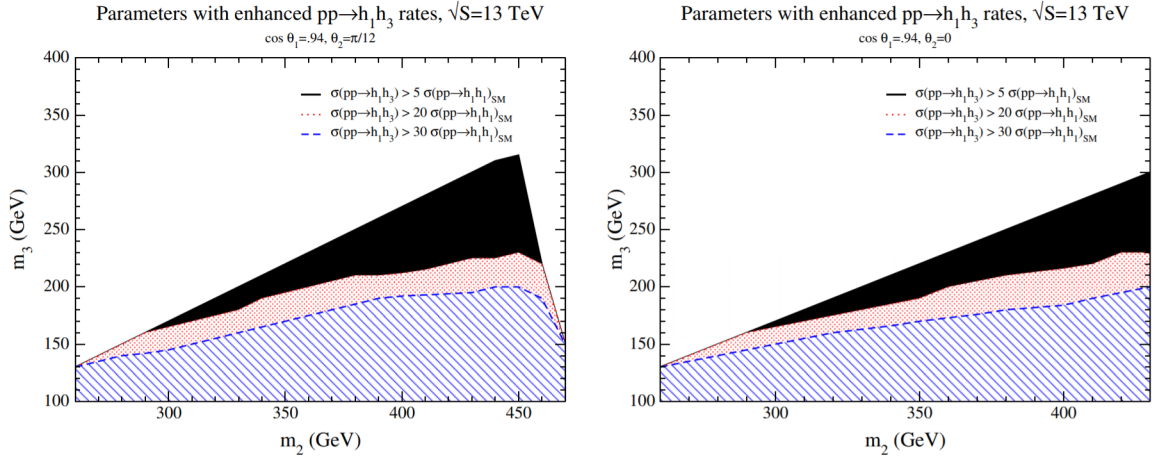
FIGURE 2.4. Regions of parameter space allowed by limits on oblique parameters S T and U from Ref [17], perturbative unitarity of 2 \rightarrow 2 scattering process [18], and the minimization of the potential where the rate for h_1 h_3 production is significantly larger than the SM h_1 h_1 rate at \sqrt{S} = 13 TeV.
