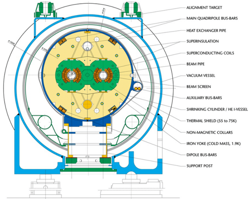
FIGURE 3.2. Cross-section of cryodipole (lengths in mm)
