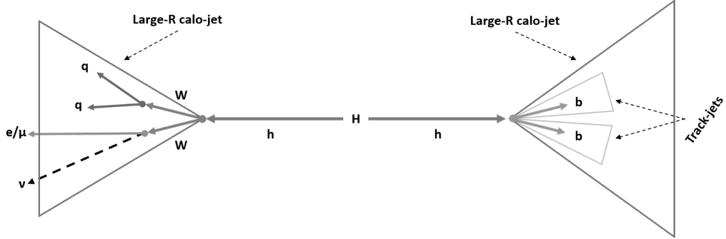
FIGURE 6.2. Diagram of the fully-boosted event topology
