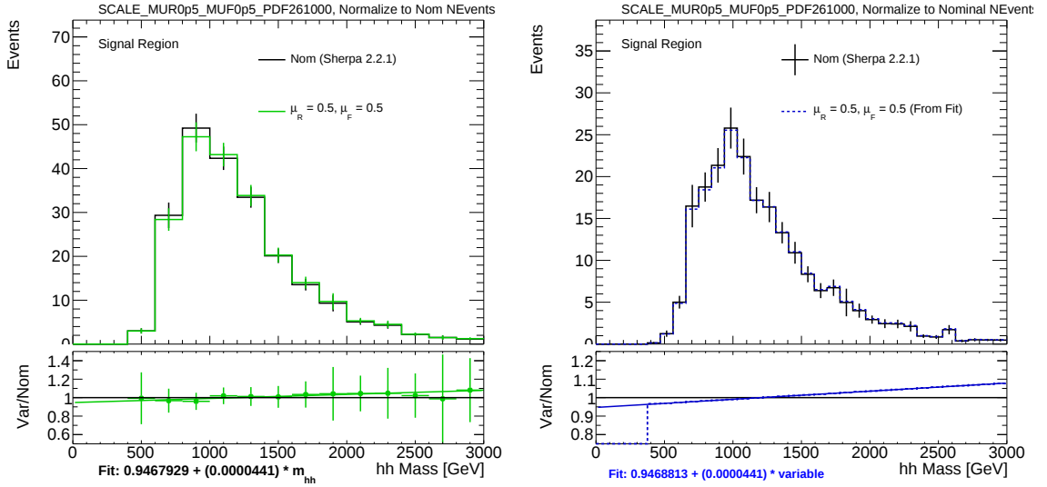
FIGURE 5.28. m_{HH} distribution shape comparison between nominal W+jets sample and scale variation ( \mu_R=0.5 , \mu_F=0.5 ) sample. Plot on the left is a direct comparison between the nominal and variation sample while on the right, the variation comes from the reweighted function applied to the nominal W+jets sample. The linear fit in the ratio of the left plot is used as the reweighted function.
