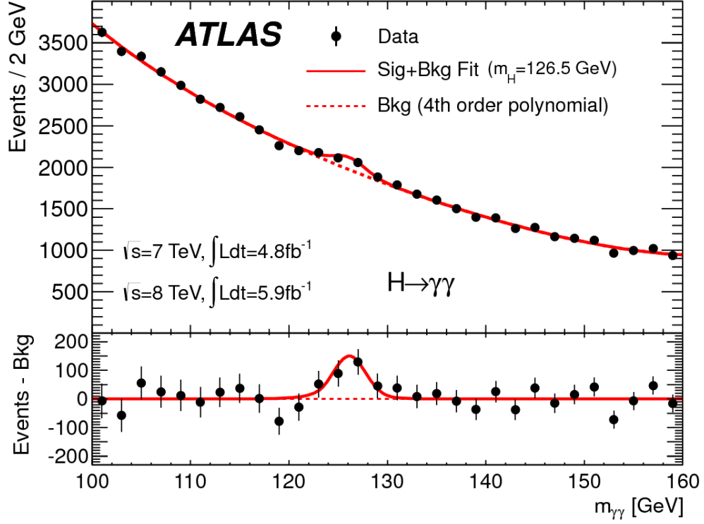
FIGURE 1.4. Invariant mass distribution of di-photon candidates for the combined root \sqrt{s}=7 TeV and \sqrt{s}=8 TeV data samples. The result of a fit to the data of the sum of a signal component fixed to m_H = 126.5 GeV and a background component described by a fourth-order Bernstein polynomial is superimposed. The bottom inset displays the residuals of the data with respect to the fitted background component.
