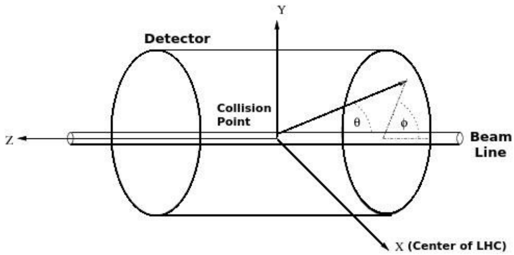
FIGURE 3.6. Detector coordinate system [27]
