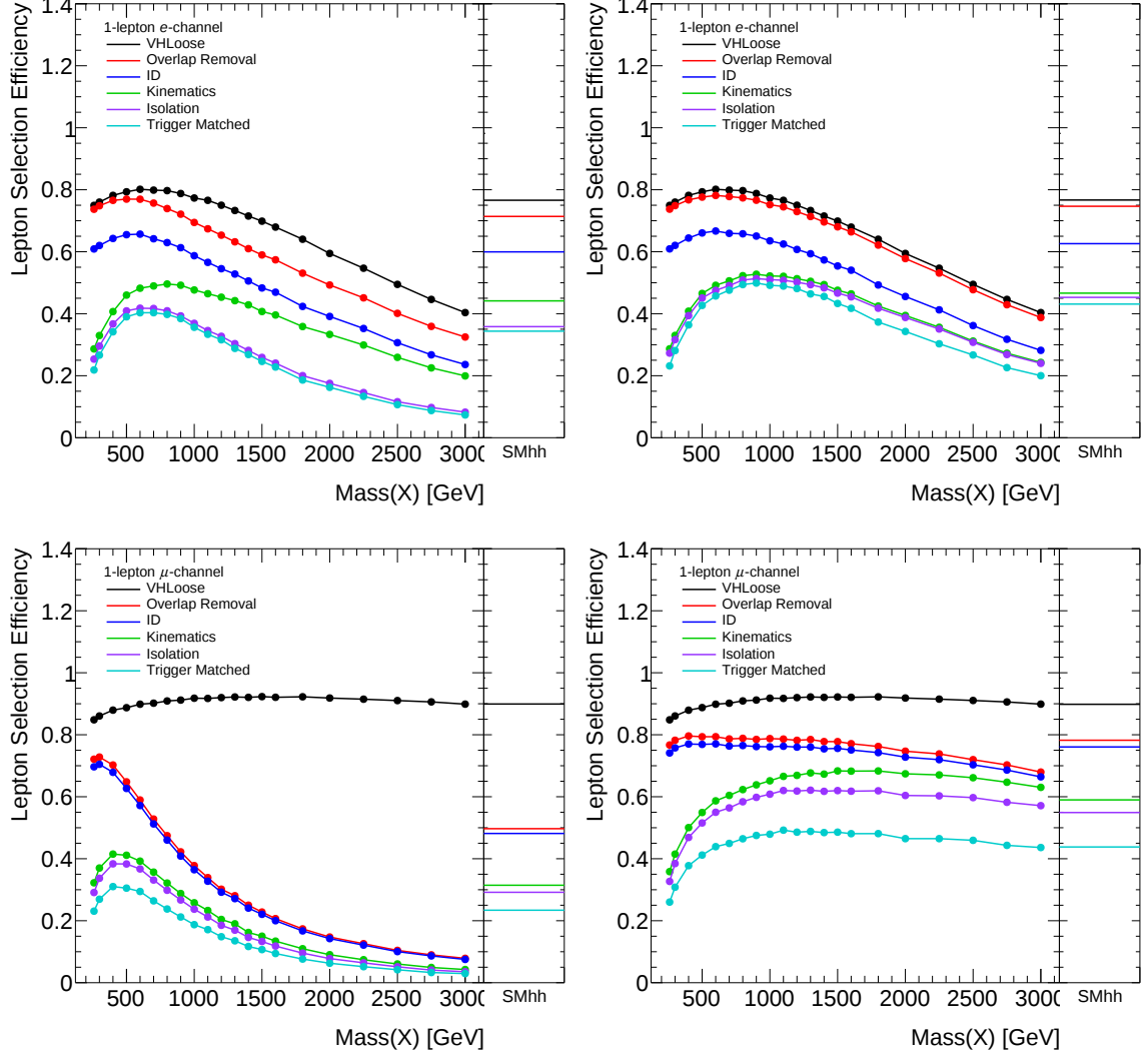
FIGURE D.1. Lepton selection efficiency as a function of signal Scalar resonance mass for the electron-channel (top) and the muon-channel (bottom). The efficiency for the SM di-Higgs signal sample (SMhh) is also shown. The plots on the left are efficiencies for the lepton selections as used in the ICHEP 2016 analysis while the plot on the right are the optimised baseline lepton selections.
