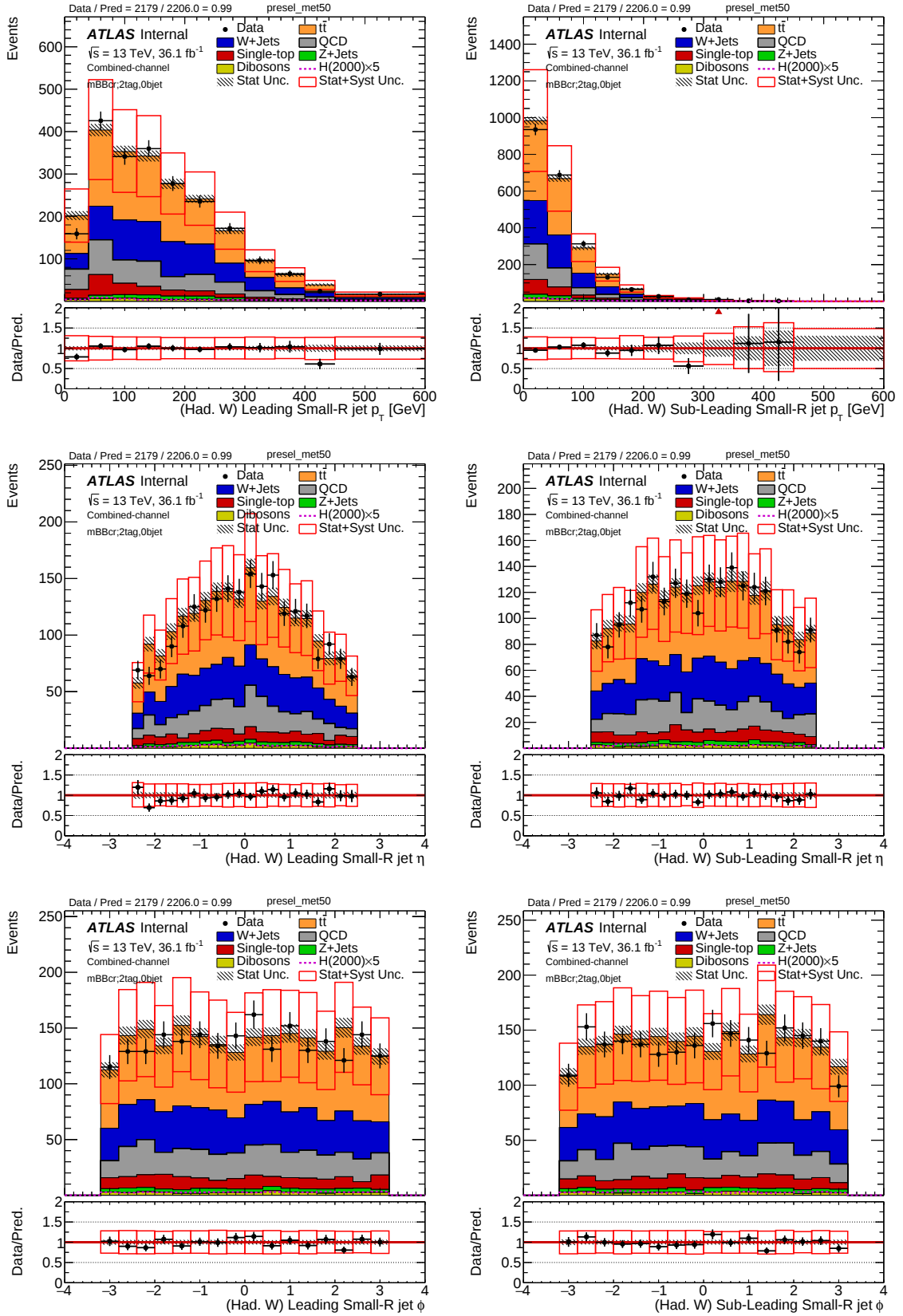
FIGURE 5.23. Kinematic distributions of the leading and sub-leading small- R jets (of the reconstructed hadronic W ) in the m\text{BBcr} control region ( m\text{BBcr} ).
