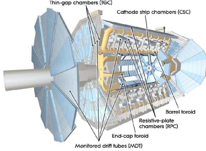
FIGURE 3.13. Cut-away view of the ATLAS muon system [38]
