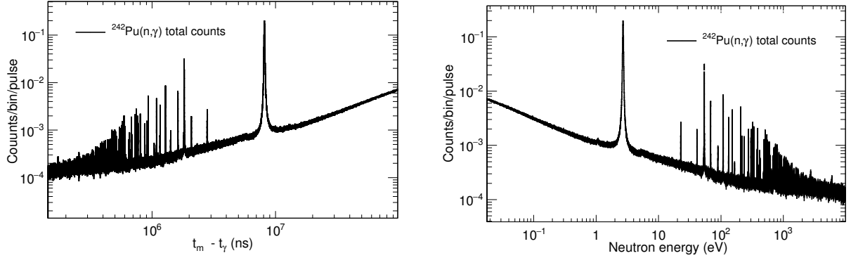
Figure 6.11: Left: Total counting rate registered in the ^{242}\text{Pu}(n,\gamma) measurement as a function of the measured time ( T_\gamma subtracted). Right: Same distribution as a function of the reconstructed neutron energy calculated with Eq. (6.5).
