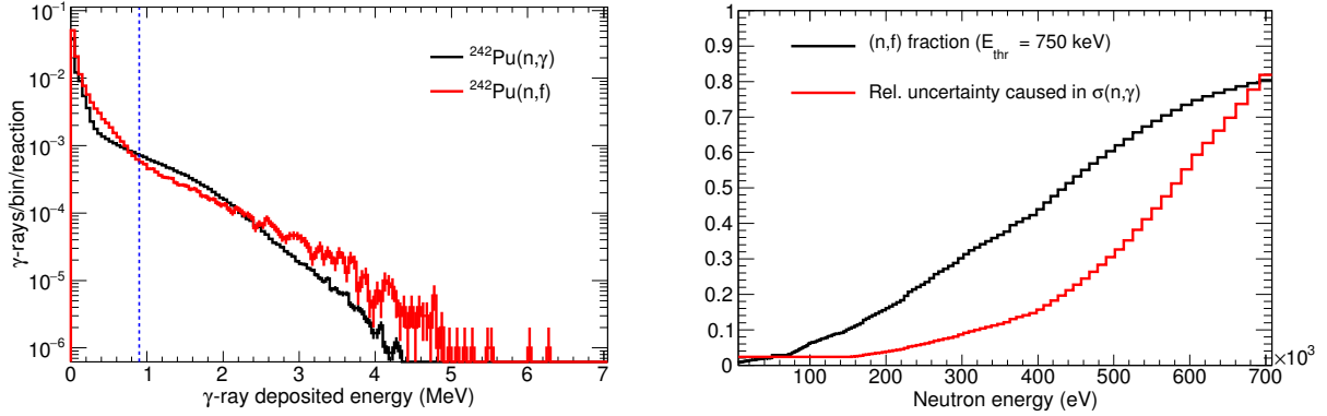
Figure 6.21: Left: Simulated response of Detector #1 to capture and fission events. The dashed line indicates the detection threshold that optimises the capture/fission efficiency ratio. Right: The black line represents the relative contribution of the fission channel to the background-subtracted counting rate calculated with a threshold of 750 keV using the ENDF/B-VII.1 library. The red curve corresponds to the systematic uncertainty in the cross section associated to the uncertainty in the fission background.
