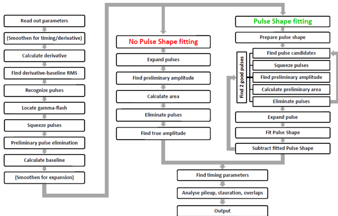
Figure 6.1: Flowchart of the Pulse Shape Analysis Routine showing the steps followed to extract the relevant parameters of each signal identified in the digitised movies. Source: Ref. [214].
