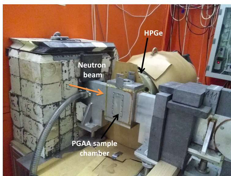
Figure 3.3: PGAA facility in one of the beam lines of the Budapest Research Reactor.
