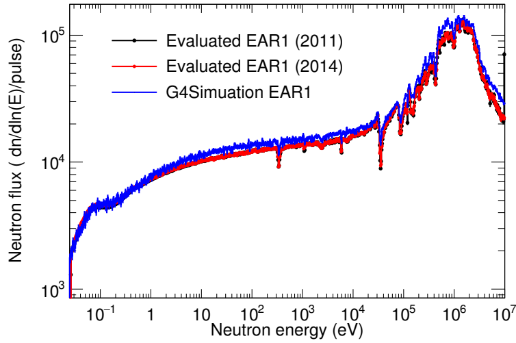
Figure 5.11: Evaluated flux measured in 2011 and 2014 from Ref. [173] compared to the result obtained from a MC simulation carried out with the Geant4 toolkit [157]. The neutron flux is shown only up to 10 MeV since this is the highest energy in the measurement of 2014.
