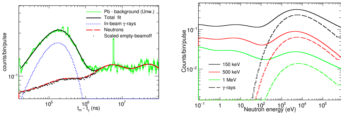
Figure 6.17: Left: Pb counting rate as a function of the time-of-flight fitted to the expression in Eq. (6.11) (black curve). The contribution of the in-beam \gamma -rays (blue) and the remaining scattered neutron component (red) have been fitted separately. The shape of the scattered neutron background below the \gamma -ray hub is extracted from the empty measurement (black dots). Right: fitted Pb( n,\gamma ) (solid lines) and in-beam \gamma -ray counting rate as a function of the reconstructed neutron energy for different detection thresholds.
