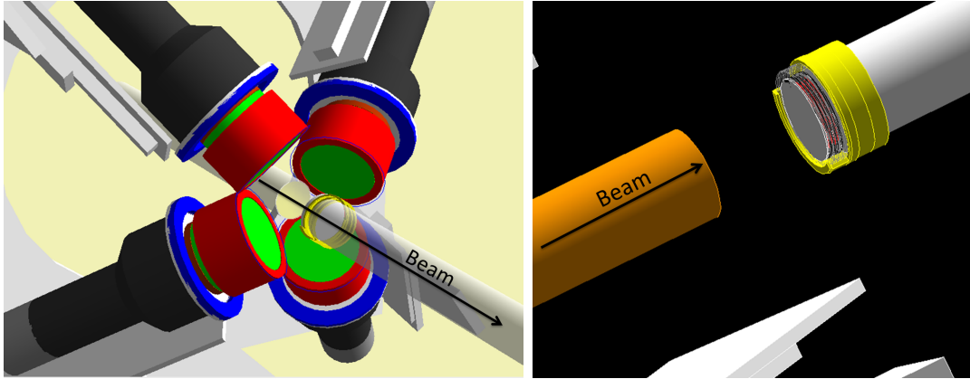
Figure 6.23: Left: General view of the geometry implemented in Geant4 to simulate the response of the detection setup. Right: Detailed implementation of the 7-target stack and the purpose-built sample holder in the Geant4 geometry model.
