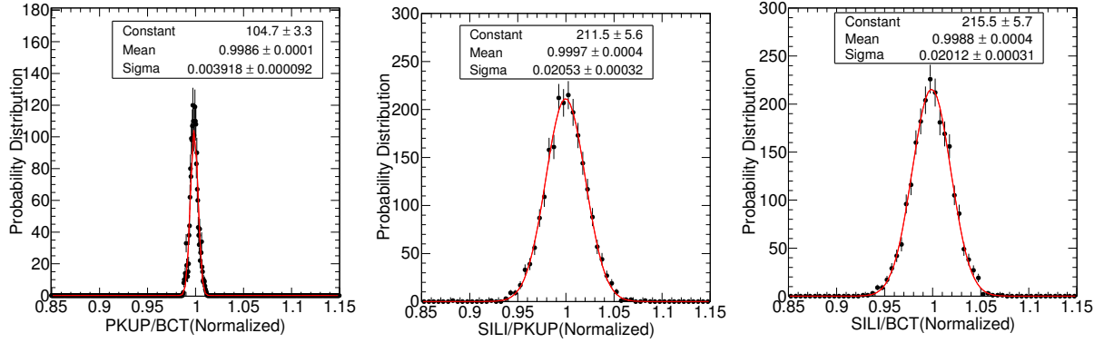
Figure 6.8: Distribution of the ratios between beam monitors for the runs corresponding to the ^{242}\text{Pu}(n,\gamma) measurement normalised to the average value of the whole campaign: \text{PKUP/BCT} (left), \text{SiMon/PKUP} (centre) and \text{SiMon/BCT} (right).
