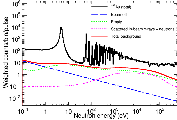
Figure 6.30: Total weighted counting rates per pulse of ^{197}\text{Au} and contribution of the different background components using a detection threshold ( E_{thr} ) of 250 keV.
