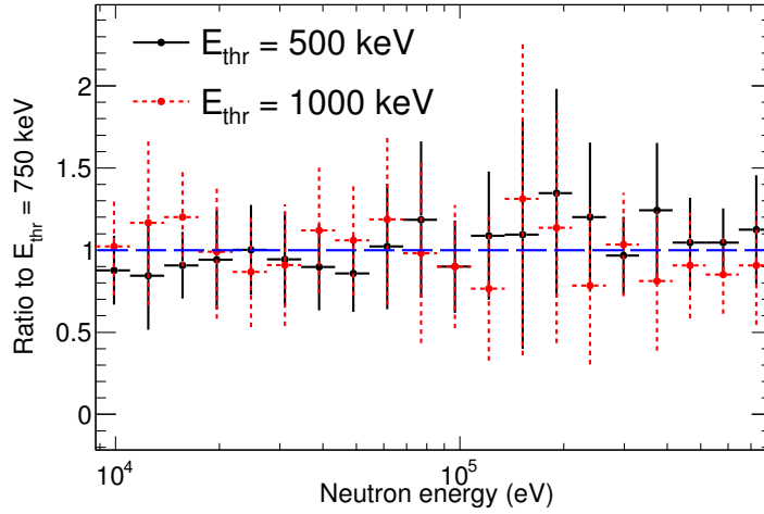
Figure 6.22: Ratio of the fission-corrected counting rate between 10 and 500 keV obtained with three different detection thresholds (500 keV, 750 keV and 1 MeV).
