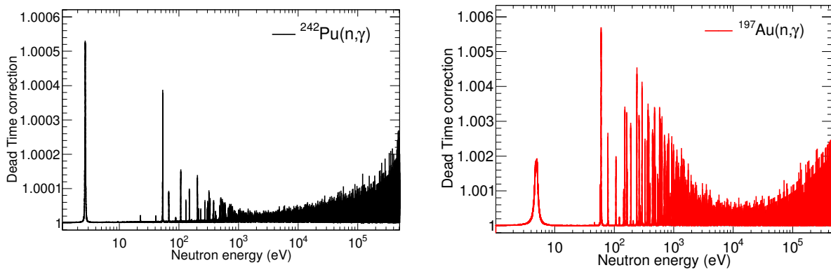
Figure 6.13: Dead time correction for C_6D_6 detector #4 during the ^{242}\text{Pu}(n,\gamma) (left) and ^{197}\text{Au}(n,\gamma) (right) measurements calculated under the non-paralyzable approximation given by Eq. (6.9).
