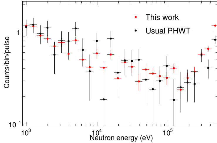
Figure 6.34: Background-subtracted ^{242}\text{Pu}(n,\gamma) in the URR calculated with the usual PHWT method (black) compared to the approach followed in this work (red). The compatibility of both methods and the reduction of the statistical fluctuations in this work are clearly appreciated.
