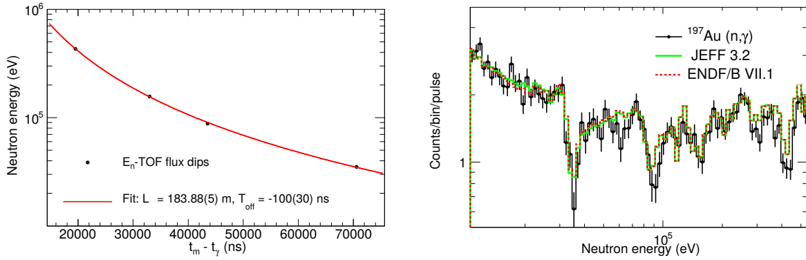
Figure 6.12: Left: Time-of-flight ( t_m - t_\gamma ) position of the dips in the ^{197}\text{Au} counting rate vs. the corresponding neutron energy in the evaluated neutron flux. The red line is a fit of the time offset T_{off} in Eq. (6.6) using the fixed flight path L = 183.88 m that matches the low energy resonances. Right: ^{197}\text{Au}(n,\gamma) counting rate as a function of the reconstructed neutron energy using Eq. (6.6) compared to the ENDF and JEFF cross sections convoluted with the n_TOF evaluated flux [173].
