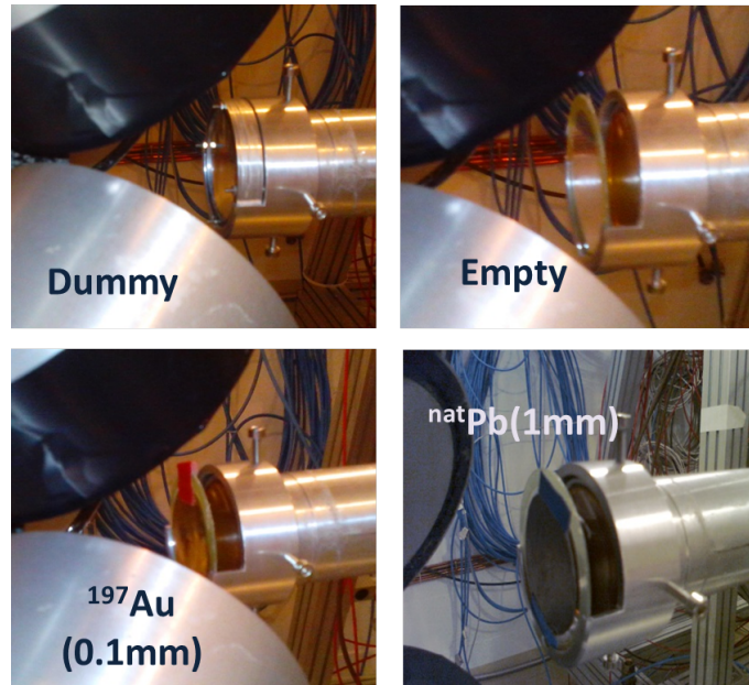
Figure 5.23: Pictures of the ancillary samples during the measurements for background assessment, normalisation and validation purposes.
