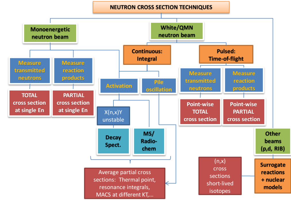
Figure 2.10: Scheme of available experimental techniques for the determination of neutron cross-sections depending on the properties of the beam.
