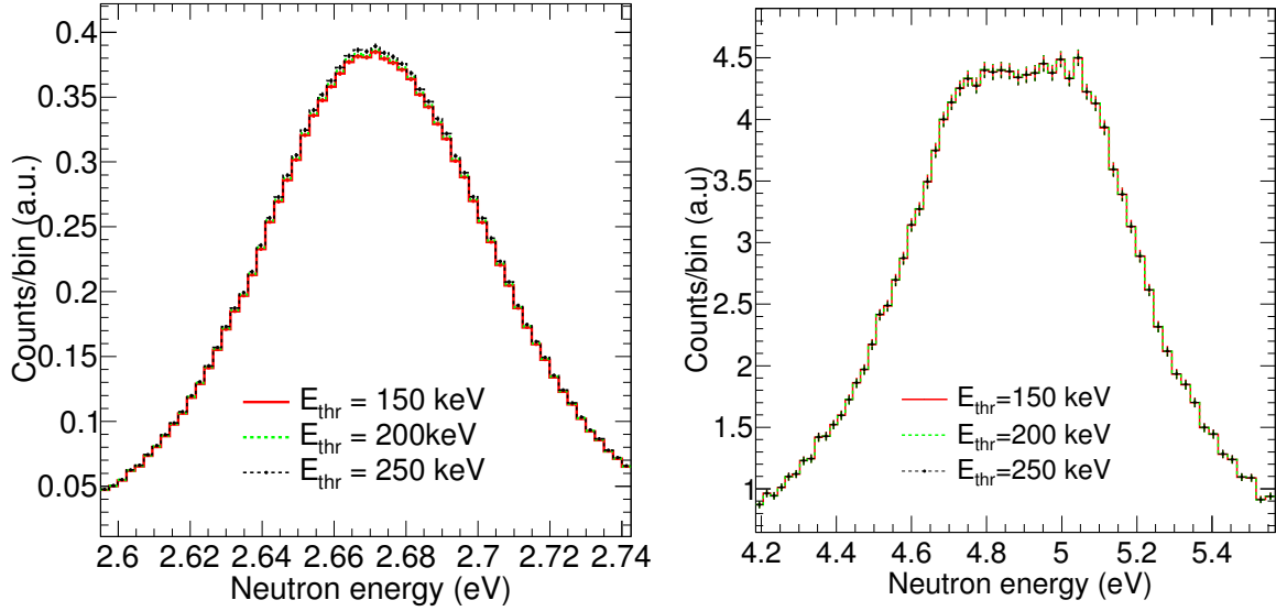
Figure 6.28: Background subtracted counting rates obtained with three different detection thresholds after being corrected for f_{thr} : ^{242}\text{Pu}(n,\gamma) resonance at 2.67 eV (left) and 4.9 eV resonance of ^{197}\text{Au}(n,\gamma) (right).
