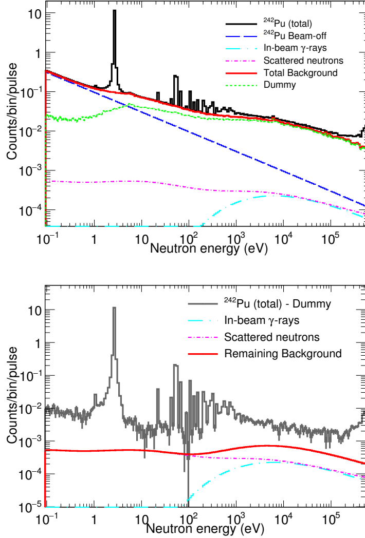
Figure 6.16: Top: Total counting rate per pulse of ^{242}\text{Pu} and contribution of the different background components using a detection threshold ( E_{thr} ) of 250 keV. The counting rate in the URR ( E_n > 1 keV) is dominated by the beam related background (dummy) (see text for details). Bottom: Counting rate after the dummy and beam-off are subtracted compared to the remaining background (i.e. scattered in-beam neutrons and gammas).
