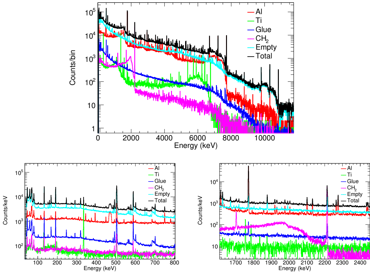
Figure 4.8: Contribution of each ancillary measurement to reproduce the total background in the PGAA measurement of the ^{242}\text{Pu} sample #1 (see Figure 4.7). The full spectrum is shown in the top panel. The bottom panels show different zooms into the energy ranges 0-800 keV and 1600-2400 keV.
