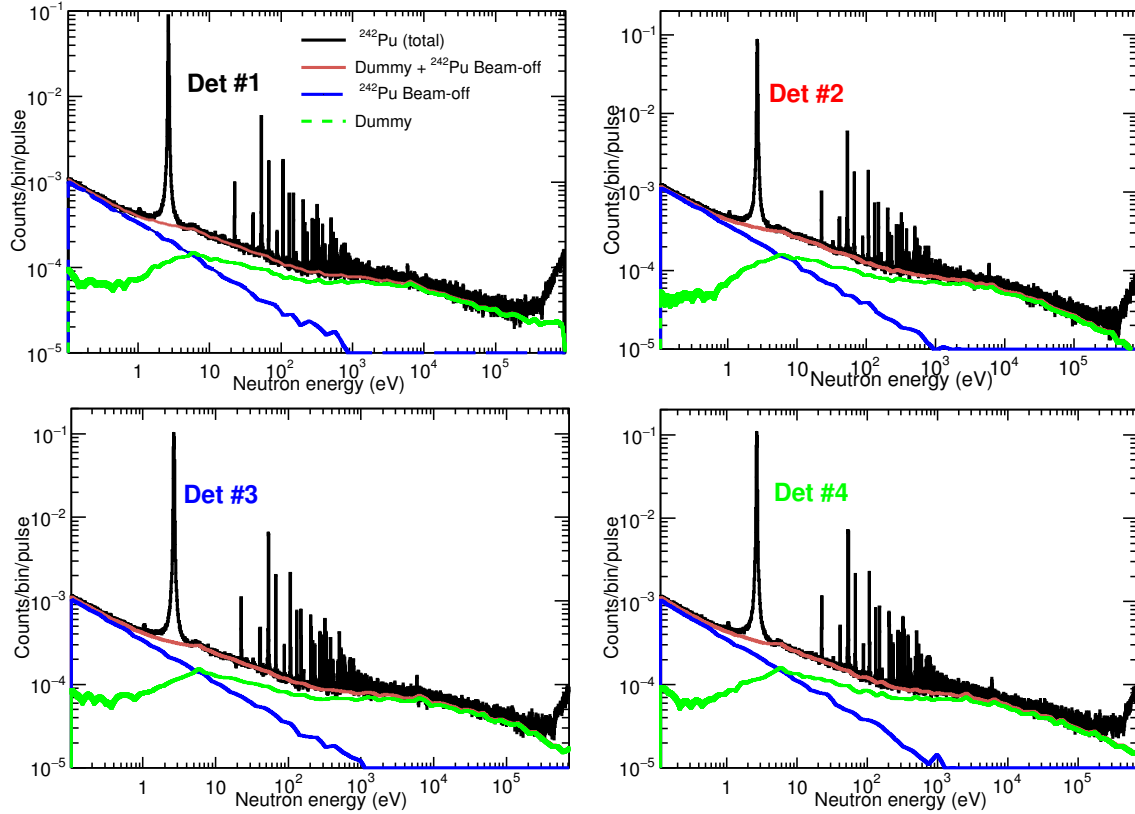
Figure 6.14: Total counting rates per pulse registered in the individual the four \text{C}_6\text{D}_6 detectors and major background contributions as a function of the neutron energy.
