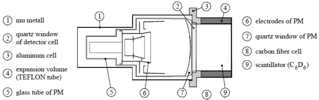
Figure 5.20: Sketch of the commercial BICRON C_6D_6 detector extracted from Ref. [160].
