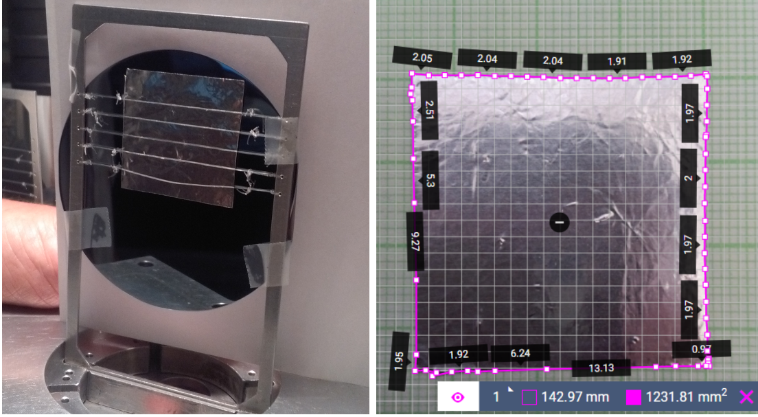
Figure 3.9: Left: Sample holder prepared for the irradiation of the aluminium foil combined with a silicon wafer aiming at providing an absolute normalisation to the number of neutrons. Right: Graphical determination of the surface of the aluminium foil using a commercial software [124].
