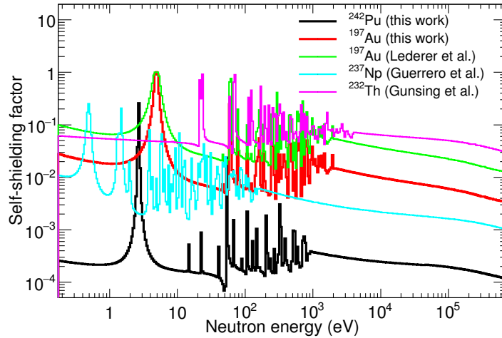
Figure 8.1: Neutron self-shielding factor as a function of the neutron for the two samples measured in this work, ^{197}\text{Au} and ^{242}\text{Pu} , compared to other measurements at n_TOF.
