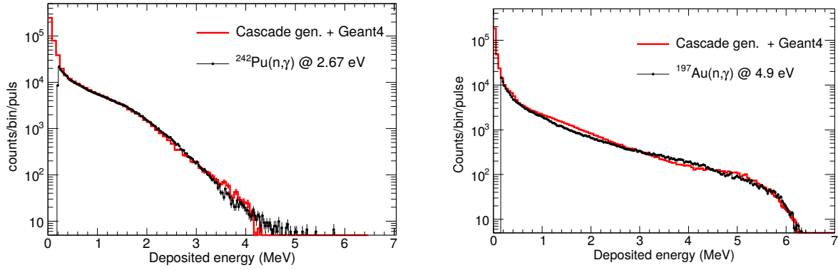
Figure 6.27: Left: Energy deposited spectrum in the C_6D_6 in the 2.67 eV ^{242}\text{Pu}(n,\gamma) resonance compared to the simulated response. Right: Experimental response compared to the simulated one for the 4.9 eV resonance of ^{197}\text{Au}(n,\gamma) cross section. The low energy fraction missing in the experimental spectra f_{thr} is corrected according to the simulations.
