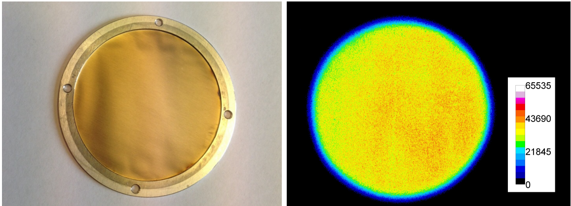
Figure 3.6: Left: Picture of a thin target backing. Right: \alpha -particle RI showing the homogeneity of the activity distribution of the deposited ^{242}\text{Pu} in one of the target backings.
