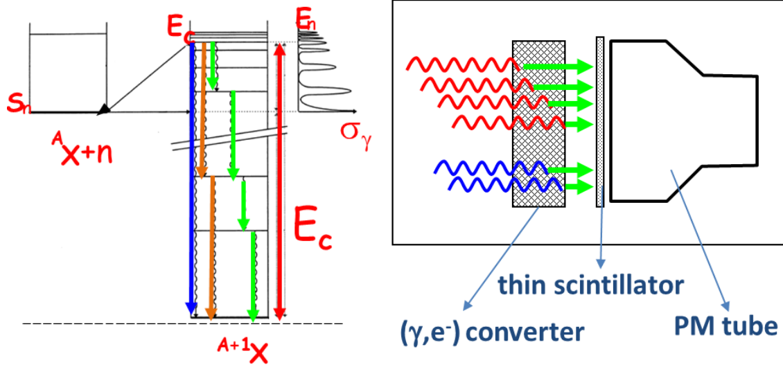
Figure 5.19: Left: Scheme showing in different colours the variable cascade pattern emitted after a neutron capture. Right: Sketch of a Moxon-Rae detector indicating its main components.
