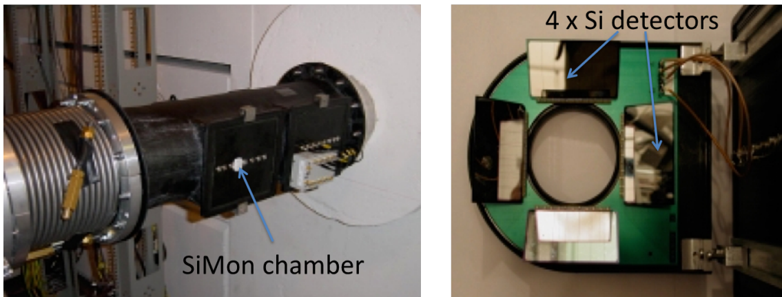
Figure 5.25: General view of the SiMon chamber in the beam line entrance to EAR1 (left) and detailed view of the opened SiMon detector showing the four Si detectors (right).
