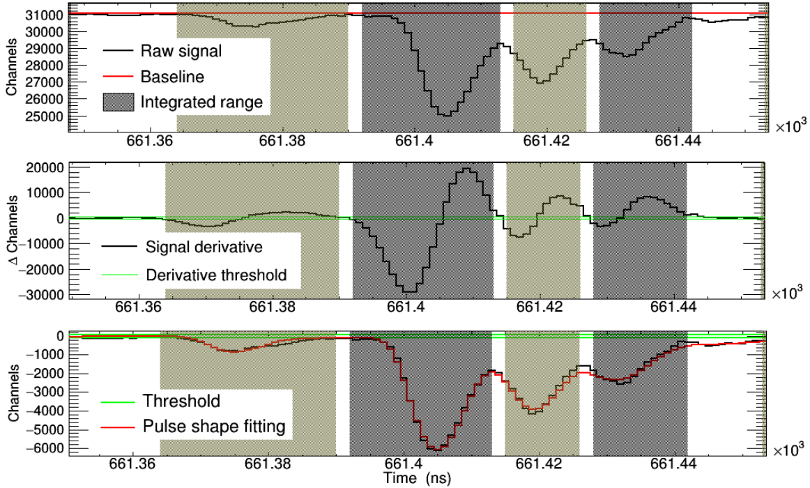
Figure 6.2: Peak fitting procedure followed by the Pulse Shape Analysis routine: fragment of the raw digitised movie and baseline determination (top), signal derivative used for pulse identification (middle), Pulse Shape Fitting of the baseline-subtracted (clean) signal (bottom).
