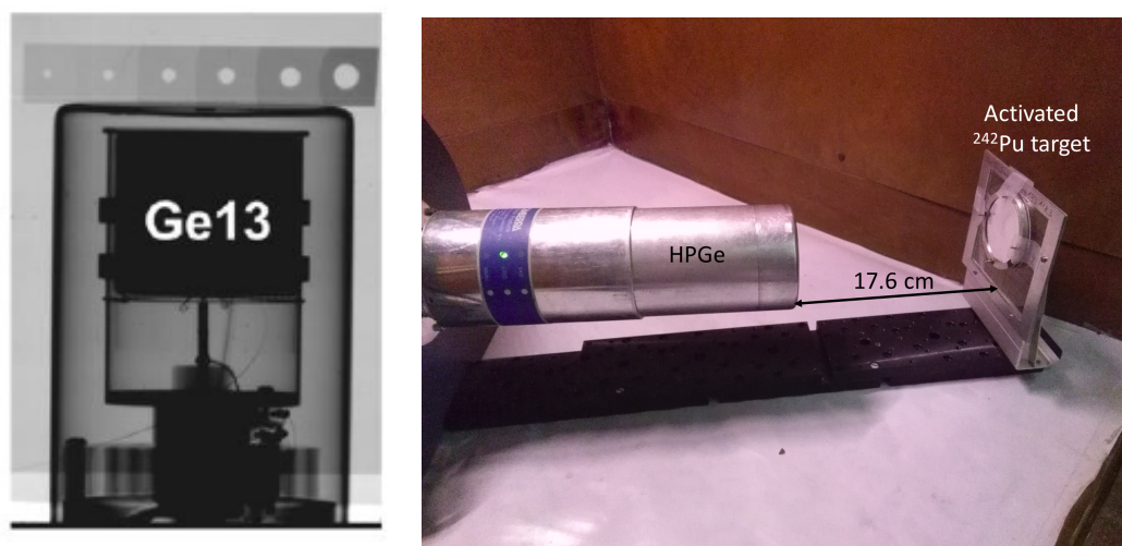
Figure 3.13: Left: X-Ray image of the n-type Canberra Model GR1319 installed in the DÖME low-background chamber for activation measurements (taken from Ref. [126]). Right: a closer view detection setup showing the HPGe detector, the aluminium pieces that keep the sample at a fixed position and the sample frame holding the activated ^{242}\text{Pu} sample #2.
