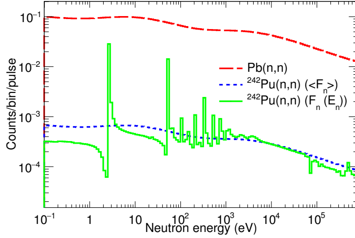
Figure 6.18: Neutron scattering background fitted from the Pb measurement (red dashed curve) scaled to the ^{242}\text{Pu} using the energy dependent scaling factor F_n(E_n) (green solid line) or the average factor \langle F_n \rangle (blue dotted line).
