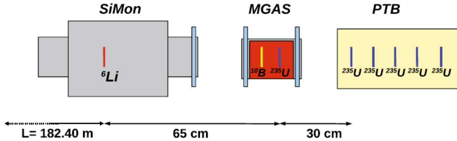
Figure 5.10: Schematic view of the detection set-up used to characterise the neutron flux. The distance between the neutron source and the SiMon detector in EAR1 is indicated, together with the relative distances along the experimental area between the different detectors (from Ref. [173]).
