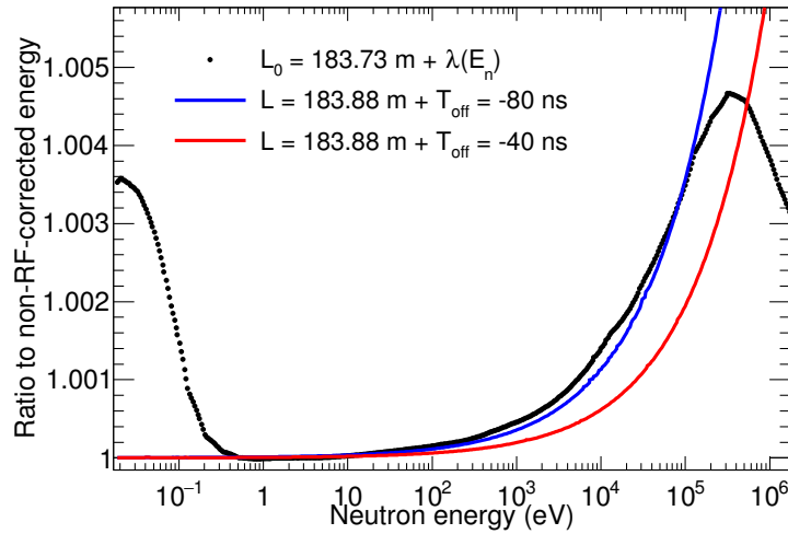
Figure 6.10: Ratio between reconstructed neutron energy using methods (2) and (3) and the non-RF-corrected energy of method (1). Two different time values of T_{off} for method (3) are compared to illustrate that none of them is able of reproducing the real shift extracted from the MC simulations.
