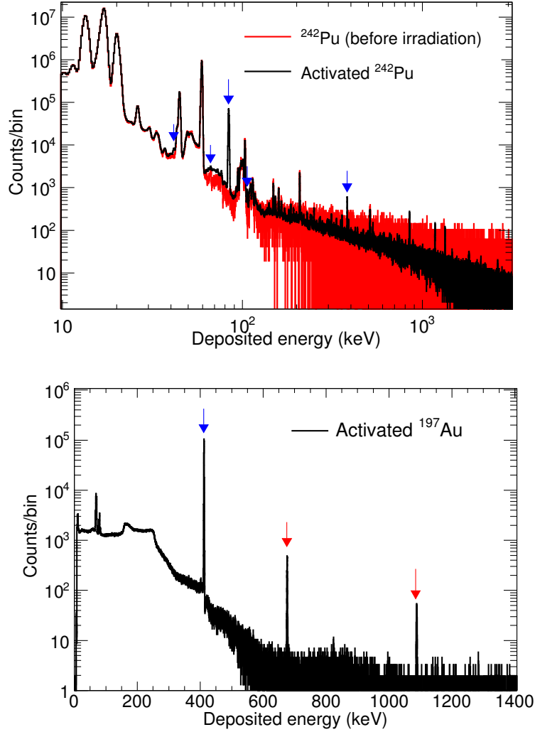
Figure 4.1: Top: spectra of \gamma -ray energy deposition acquired with the HPGe detector in the activation station before (red) and after (black) activating the ^{242}\text{Pu} sample. The bottom panel shows the spectra of the activated ^{197}\text{Au} target. The analysed lines are pointed with blue arrows.
