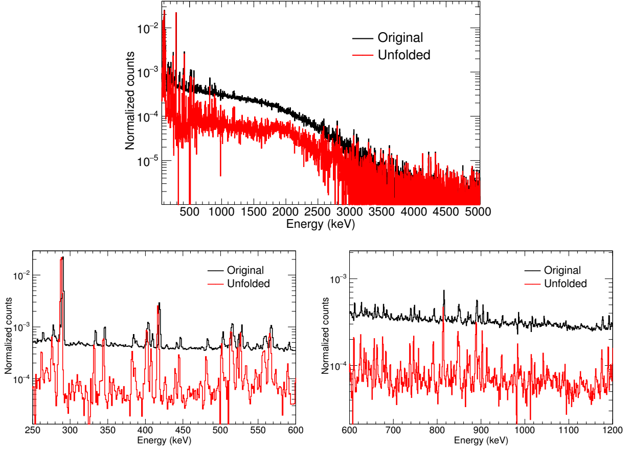
Figure 4.11: Experimental background-subtracted ^{242}\text{Pu}(n,\gamma) spectrum (black) compared to the unfolded spectrum (red), where only the full energy deposition events remain. The top panel shows the full energy range up to the neutron binding energy while the bottom panels zoom into different energy ranges. The integral of the measured spectrum was normalised to 1.
