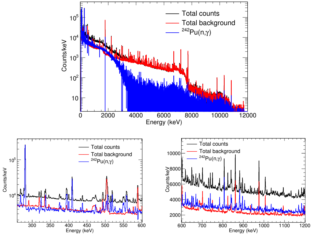
Figure 4.7: Top: Total counting rate (black) registered by the HPGe as a function of the deposited \gamma -ray energy in the full energy range up to 12 MeV. The red curve shows the total background while the blue line is the background-subtracted response to the ^{242}\text{Pu}(n,\gamma) cascade. The bottom panels zoom into different low energy intervals.
