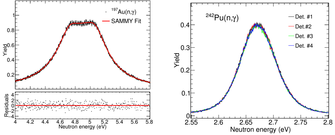
Figure 6.31: Left: saturated resonance at 4.9 eV in the experimental capture yield of ^{197}\text{Au} fitted with the SAMMY code. The average of the four detectors is shown. Right: Individual capture yields of ^{242}\text{Pu} in the 2.67 eV resonance after being normalised to ^{197}\text{Au} .
