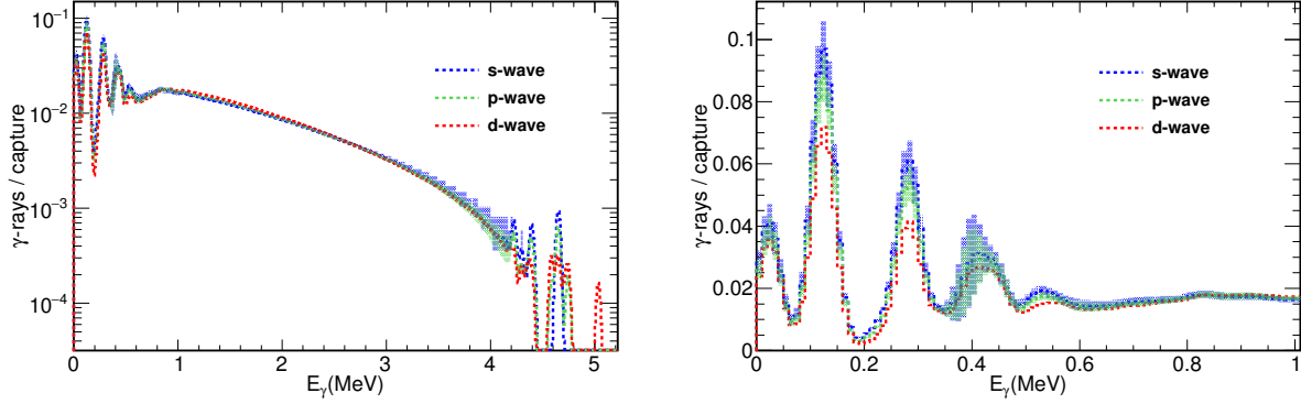
Figure 6.29: Energy distribution of the statistically generated ^{242}\text{Pu}(n,\gamma) capture cascades for s-, p- and d-waves. The right panel zooms into the low energy region to show the good agreement within standard deviation (shadowed region) for s- and p-wave cascades and the small deviation for the d-wave. The spectra are convoluted with a experimental resolution of \text{FWHM} = 50 \text{ keV} .
