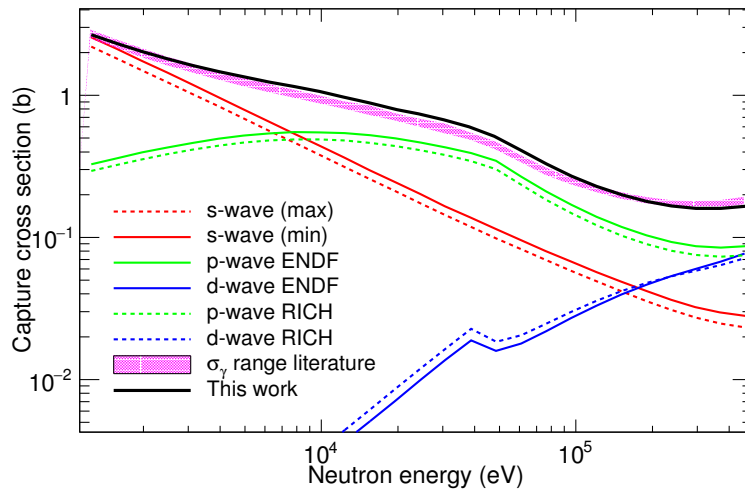
Figure 8.7: FITACS calculation in this work (black line) compared to the expected cross section range (shadowed area) (see text for details). The expected upper and lower limits for the partial cross sections ( s -, p - and d -waves) are shown with solid and dashed lines.
