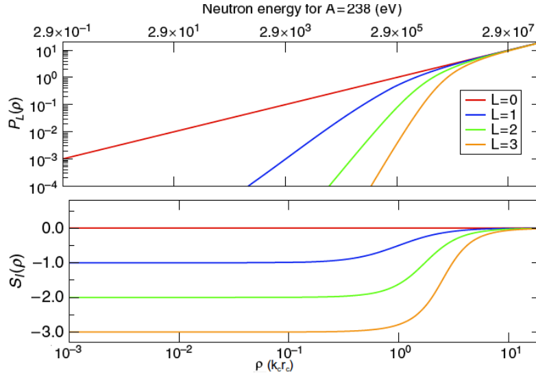
Figure 2.5: R -Matrix parameters for the neutron exit channel as a function of the angular momentum L \equiv l and k_c r_c . The equivalent neutron energy (for A=238 ) is shown in the upper x -axis. From Ref. [57].
