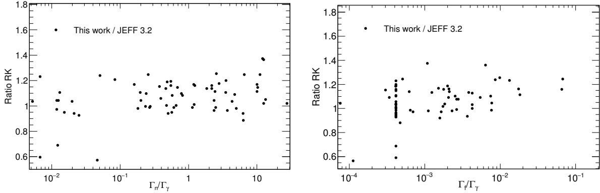
Figure 7.9: Ratio of individual radiative kernels obtained in this work with respect to JEFF-3.2 as a function of \Gamma_n/\Gamma_\gamma (left) and as a function of \Gamma_f/\Gamma_\gamma (right).
