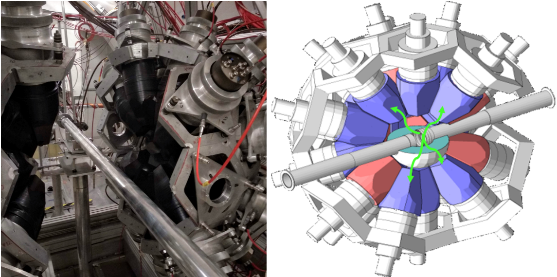
Figure 5.17: Left: Inner view of the separated TAC hemispheres with the neutron beam line of EAR1 between them. Right: Geant4 model developed for the assesment of the detection efficiency (from Ref. [189]).
