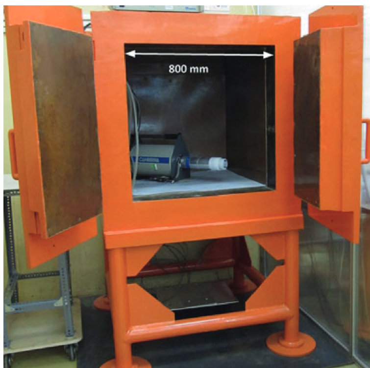
Figure 3.12: General view of the DÖME set-up chamber from the outside (taken from Ref. [130]).
