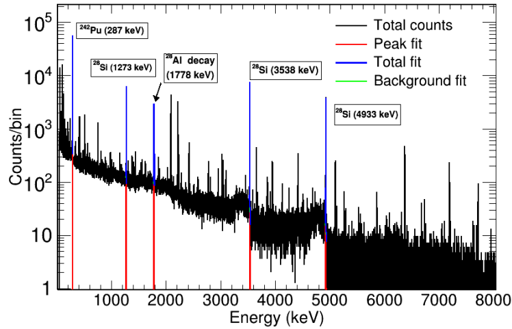
Figure 4.9: Prompt \gamma -ray spectrum measured during the irradiation of ^{242}\text{Pu} sample #1 + Si comparator. The analysed prompt \gamma -ray transitions originated in captures on ^{242}\text{Pu} , Al (target backings) and the Si comparator foil are labelled on the plot.
