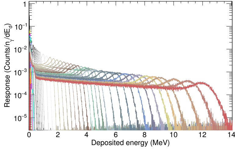
Figure 6.24: Simulated response of Detector #1 to mono-energetic \gamma -rays of 45 different energies ranging from 50 keV to 14 MeV. The experimental resolution broadening has been included.
