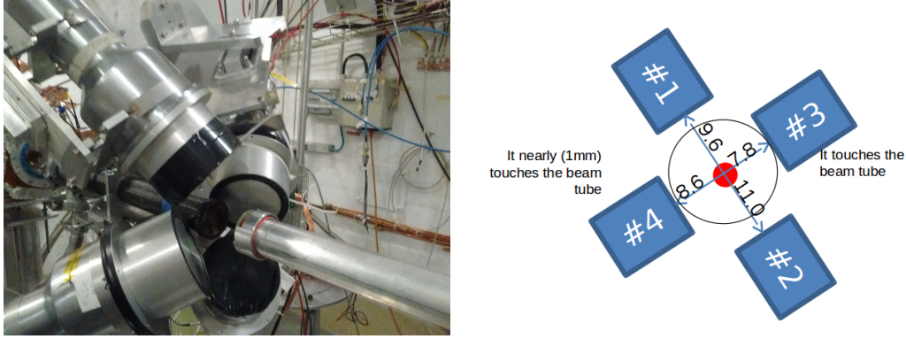
Figure 5.24: Left: Array of four BICRON \text{C}_6\text{D}_6 detectors used to detect the \gamma -ray cascades emitted following the neutron capture on the ^{242}\text{Pu} sample. Right: Sketch of the four BICRON detectors indicating the distances from the detectors to the target centre.
