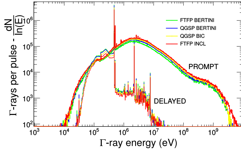
Figure 5.16: Energy distribution of the two \gamma -ray components produced in the spallation target assembly obtained from the Geant4 simulations of Ref. [157]. The prompt component includes the \gamma -rays reaching EAR1 within 1 \mu s and the delayed one those arriving at larger times. The different curves correspond to the results of different Physics Lists.
