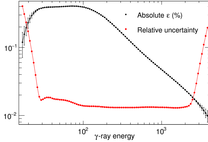
Figure 3.14: Absolute peak efficiency (black) and its relative uncertainty (red) of the DÖME low-background counter as a function of the \gamma -ray energy [130].
