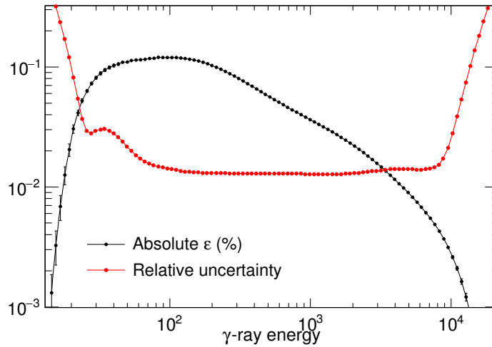
Figure 3.11: Absolute peak efficiency (%) as a function of the \gamma -ray energy (black) and its relative uncertainty (red) for the Compton-unsuppressed HPGe detection set-up of the PGAA facility.
