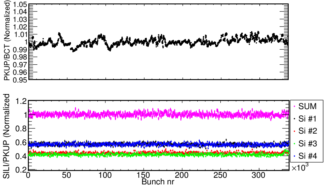
Figure 6.7: Top: Ratio of the PKUP area to the BCT value as a function of the bunch number. Bottom: Ratio of the SiMon counting rates (i.e. integral of the triton peak, for neutron energies from thermal to 1 keV) to the area of the PKUP signal (see text for details).
