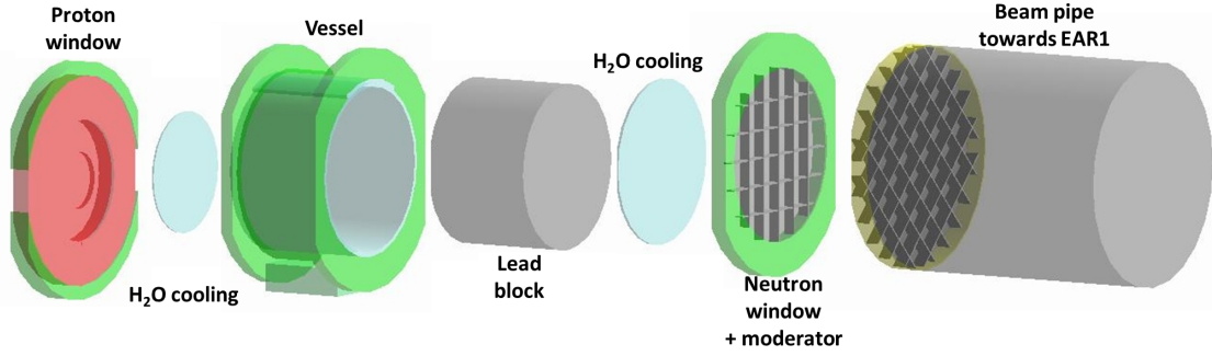
Figure 5.3: Exploded-view of the various elements of the n TOF-spallation target implemented in the Geant4 simulations.
