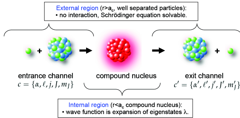
Figure 2.4: Scheme of the basic principles of the R-Matrix theory (see text for the details). From Ref. [57].
