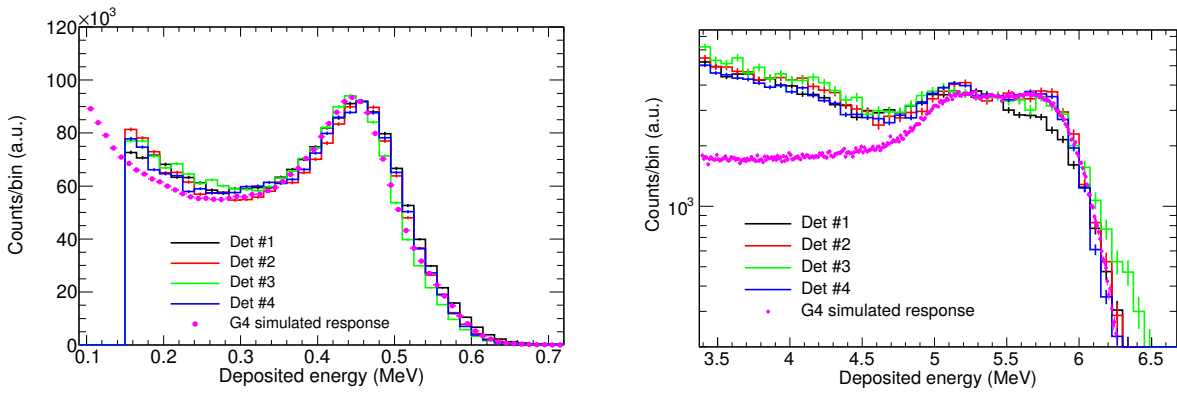
Figure 6.4: Comparison between the simulated (broadened) response and the experimental energy-calibrated response of the individual C_6D_6 detectors to the \gamma -rays emitted from ^{137}\text{Cs} (left) and ^{244}\text{Cm-}^{13}\text{C} (right).
