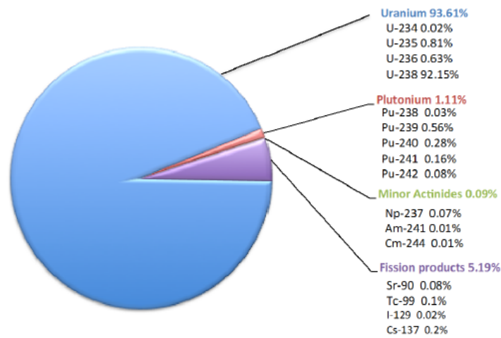
Figure 1.9: Isotopic composition of the burned fuel from a PWR with initial enrichment of 4.5 wt% after a 45 GWd/MTU burn-up. Source: Ref. [9].
