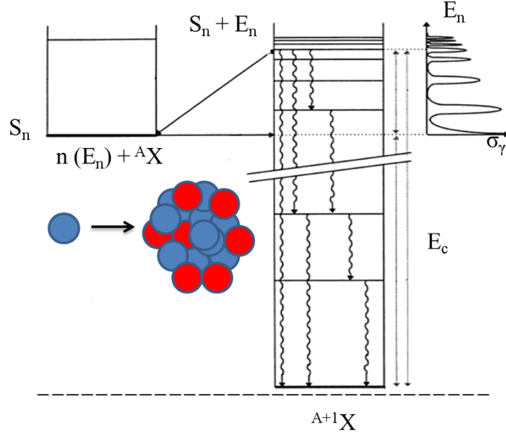
Figure 2.3: Sketch of the Compound Nucleus formation when a neutron of energy E_n interacts with {}^A X nucleus. The quasi-stationary states on the Compound Nucleus above the neutron separation energy S_n lead to resonances in the cross section. The total excitation energy to be released in the decay of the compound nucleus is noted as E_c \simeq S_n + E_n .
