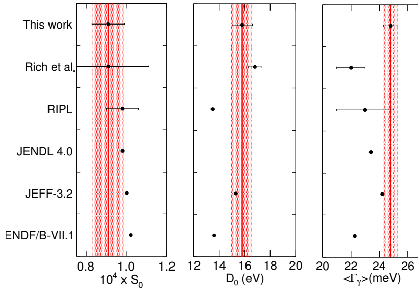
Figure 7.18: Average resonance parameters obtained in this work compared to the values in the literature: S_0 (left), D_0 (middle), \langle\Gamma_\gamma\rangle (right). The shadowed area corresponds to the uncertainty from our analysis.
