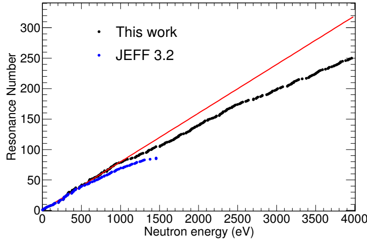
Figure 7.11: Cumulative number of resonances as a function of the neutron energy showing a compatible D_0 for JEFF-3.2 and this work up to \sim 500 eV. The solid red line corresponds to the linear fit of this distribution in the energy region below 1.1 keV (see text for the details).
