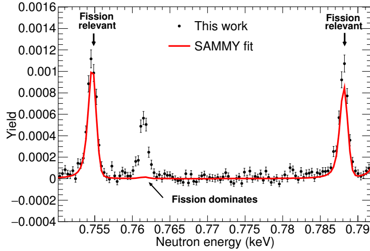
Figure 7.2: Experimental capture yield as a function of the neutron energy showing the resonances with the largest fission contribution below 1 keV (left out of the analysis). The red curve corresponds to the capture yield calculated by SAMMY, which clearly underestimates the experimental data for these resonances, especially for the one at 762 eV.
