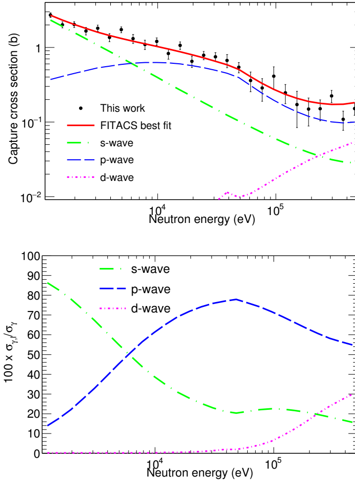
Figure 8.4: Top: Capture cross section in the URR obtained in this work together with the Hauser-Feshbach calculation that provides the best fit to the data. The bottom panel shows the relative contribution of the different partial waves.
