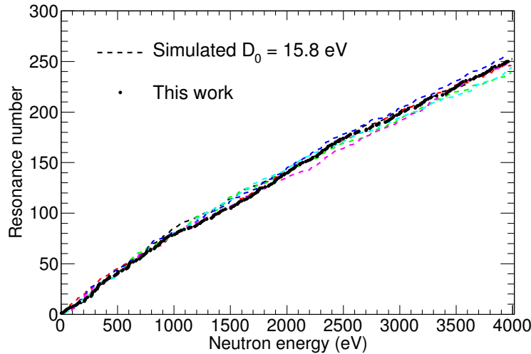
Figure 7.13: Experimental cumulative energy distribution of observed resonances compared to the observable resonances according to several individual resonance sequences obtained from statistical model simulations. The simulated sequences were generated with D_0 = 15.8 eV, S_0 = 0.91 \cdot 10^{-4} and S_1 = 2.07 \cdot 10^{-4} [42].
