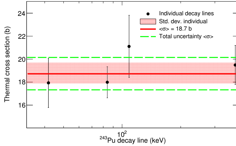
Figure 4.6: Thermal capture cross section values obtained from the analysis of the four most intense decay lines of the produced ^{243}\text{Pu} nuclei. The weighted average is indicated as a solid line and the shadowed corridor represents the standard deviation of the individual values, assumed as the final energy-dependent uncertainty. The total uncertainty in the thermal cross section is indicated with the green dashed lines.
