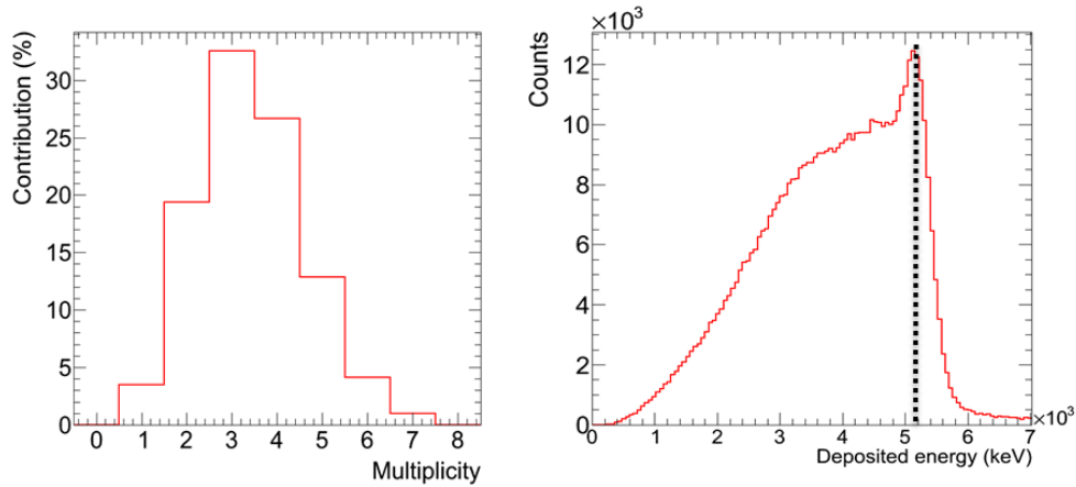
Figure 5.18: Left: Typical multiplicity distribution of the events in the ^{237}\text{Np}(n,\gamma) measurement with the TAC [190]. Right: Total \gamma -ray energy deposited in the TAC crystals E_{\text{sum}} peaked at the neutron separation energy indicated with a dashed line.
