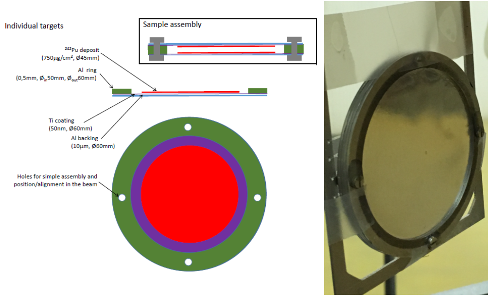
Figure 3.7: Left: Sketch of the ^{242}\text{Pu} samples irradiated in the PGAA facility consisting in a stack of two fission-like targets. Right: Actual picture of a 2-target ^{242}\text{Pu} sample mounted on the PGAA sample holder. The ^{197}\text{Au} foil was placed downstream with respect to the ^{242}\text{Pu} target to avoid the absorption of low energy neutrons in the former.
