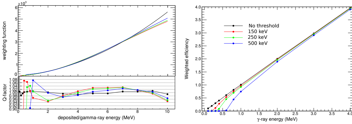
Figure 6.25: Left: Analytical weighting function for detector #1 calculated with different values of E_L and the associated Q-factor as a function of the \gamma -ray energy (residual). Right: Weighted efficiency as a function of the \gamma -ray energy showing the deviation from proportionality as the lower energy limit E_L increases.
