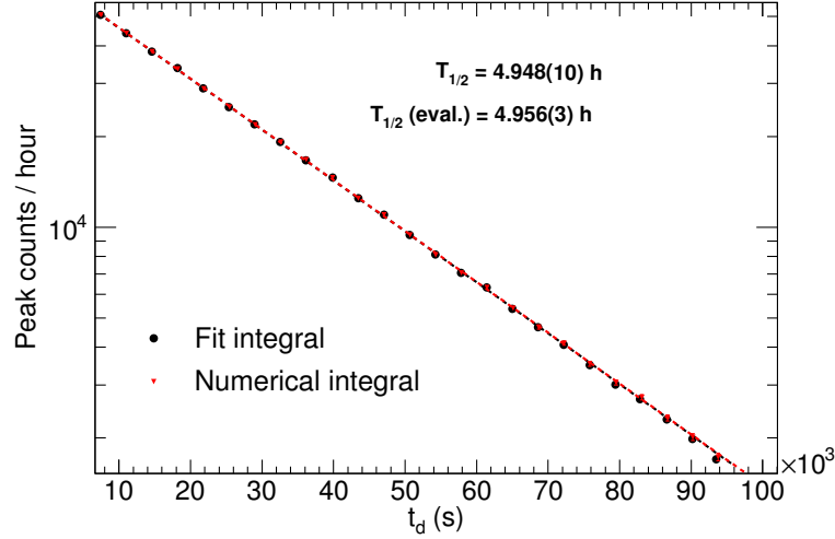
Figure 4.3: Time evolution of the 84 keV peak area fitted to the expected exponential decay. The peak integral extracted from the fit peak (black) shows compatible results with the direct numerical integration on top of the background (red). The fitted half-life T_{1/2} is compared to the evaluated one.
