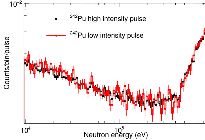
Figure 6.20: Total counting rate as a function to the neutron energy showing the very good agreement of the dedicated (full intensity) and the parasitic (low intensity) bunches.
