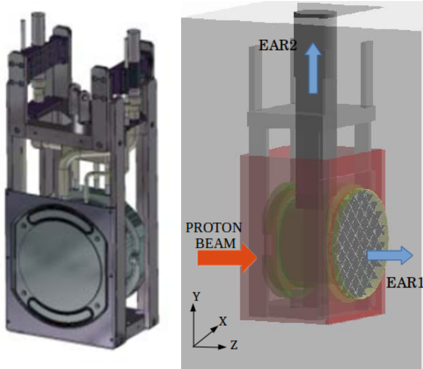
Figure 5.2: General view of the spallation target geometry shown in a CAD drawing (left) and in a Geant4 geometry model (right), where we indicate the direction of incidence of the proton bunches and the exit towards both EARs.
