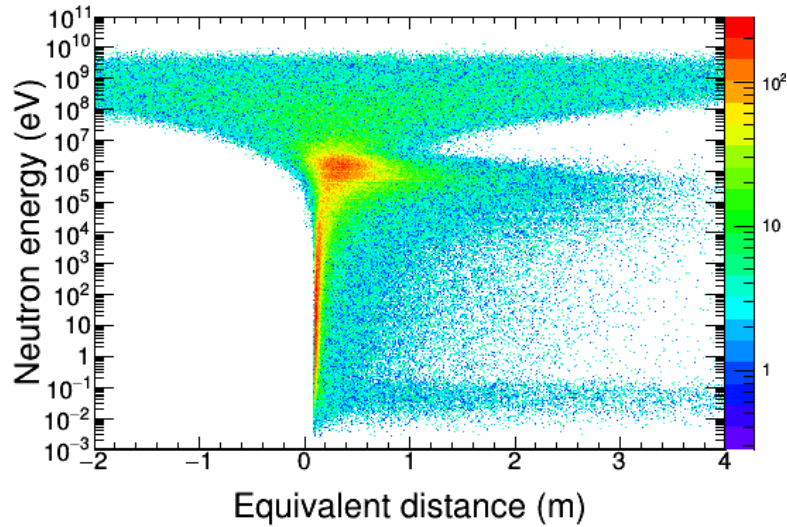
Figure 5.13: Probability distribution of the equivalent moderation distance as a function of neutron energy, obtained from GEANT4 simulations of the n_TOF spallation target. The simulated moderation time was convoluted with the Gaussian distribution of the proton pulse (7 ns RMS). The latter dominates the broadening above 10 MeV.
