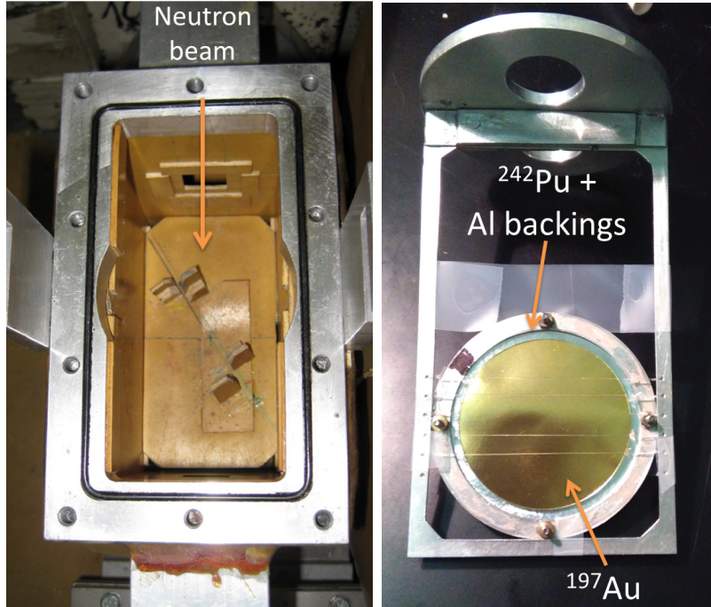
Figure 3.8: Left: Neutron irradiation chamber covered with a ^6\text{Li} -plastic to absorb scattered neutrons. The tilted position of the sample is shown by the orientation of the slits on the chamber floor. Right: ^{242}\text{Pu} target assembly and ^{197}\text{Au} reference sample of the same diameter placed in the PGAA sample holder. The latter is placed downstream with respect to the direction of incidence of the neutron beam to avoid the absorption of low energy neutrons.
