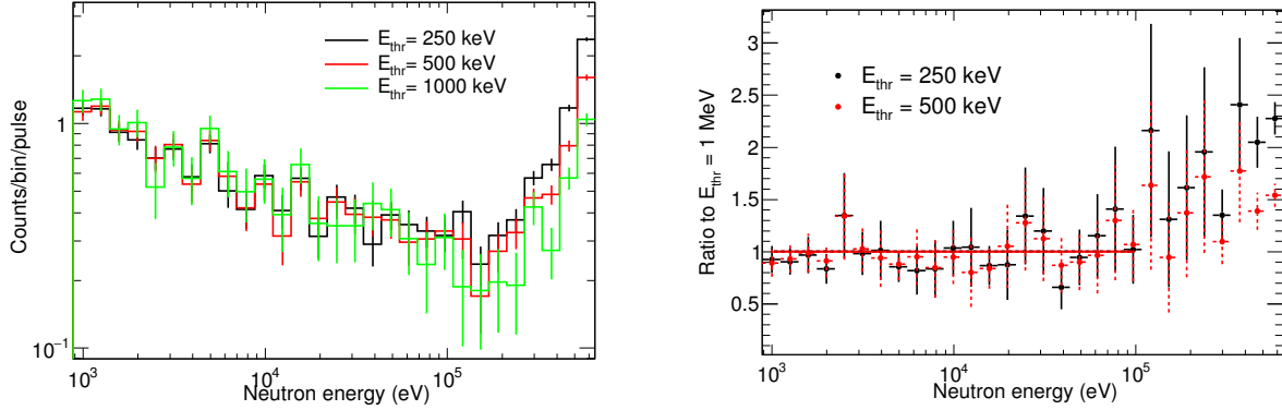
Figure 6.19: Left: ^{242}\text{Pu}(n,\gamma) counting rate per pulse in the URR as a function of the neutron energy obtained with different thresholds ( E_{\text{thr}} ). Right: Ratio of counting rates with respect to the results with E_{\text{thr}} = 1 \text{ MeV} . The solid lines correspond to the average ratios, presented in Table 6.4.
