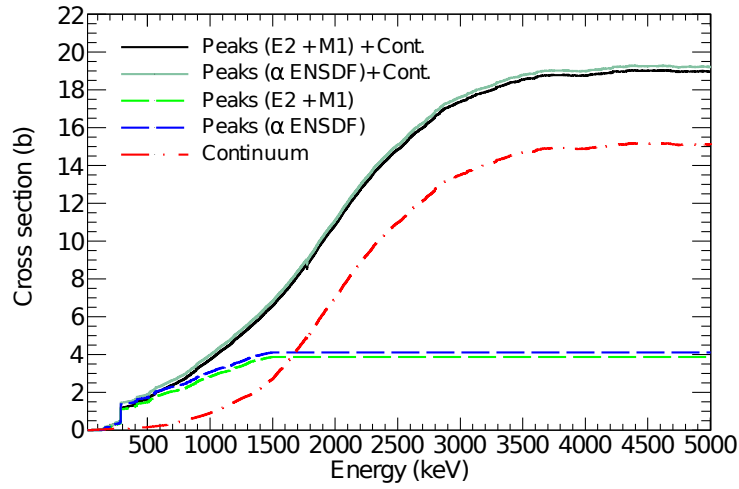
Figure 4.14: Cumulative capture cross section as a function of the \gamma -ray energy calculated with the weighted running sum of the spectrum of partial \gamma -ray production cross section. The contribution of the continuum and peaks are shown separately. For the latter, two approaches for the internal conversion correction are compared (see text for details).
