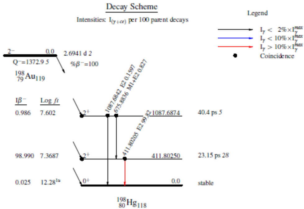
Figure A.1: Scheme of the \beta^- decay of ^{198}\text{Au} to ^{198}\text{Hg} . (from Ref. [19]).
