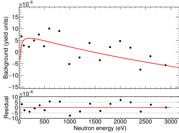
Figure 7.1: Residual background in the capture yield as a function of the neutron energy fitted with SAMMY. The red line corresponds to the parametrisation using Eq. (7.4). The bottom panel shows the reduced background oscillating around zero after the fit is subtracted.
