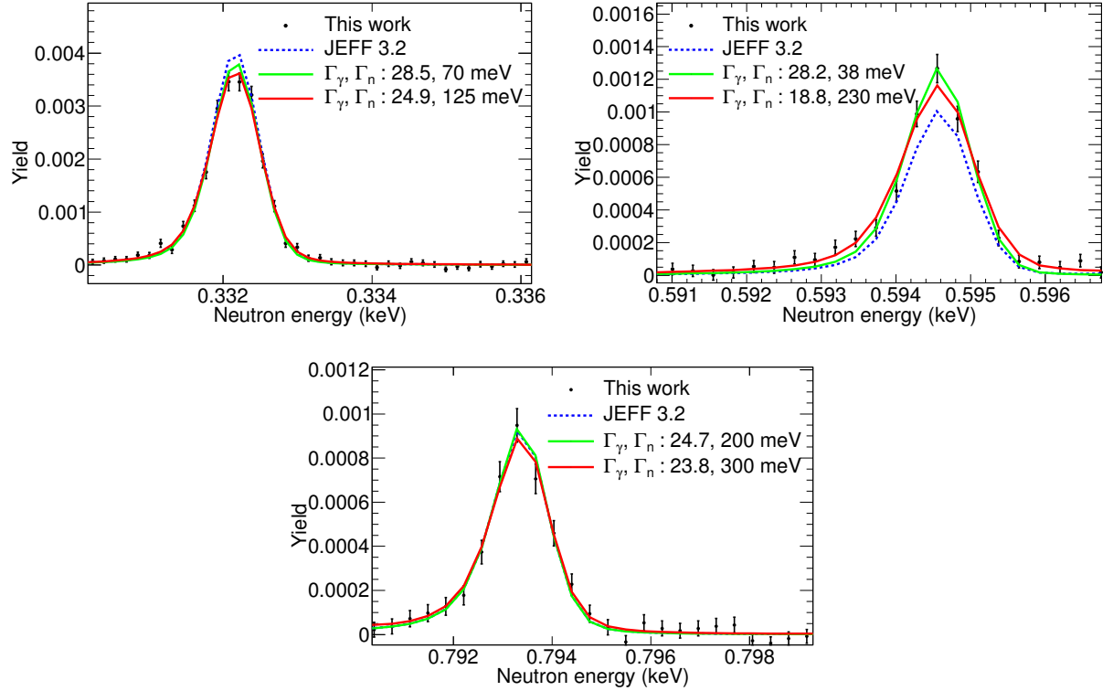
Figure 7.4: Examples of the low sensitivity of some SAMMY fits to the choice of \Gamma_n , showing the compatibility of the fit with overestimated \Gamma_n (red) compared to the fit with a \Gamma_n value consistent with previous multi-channel measurement (green). JEFF-3.2 is shown as a reference (dotted blue line).
