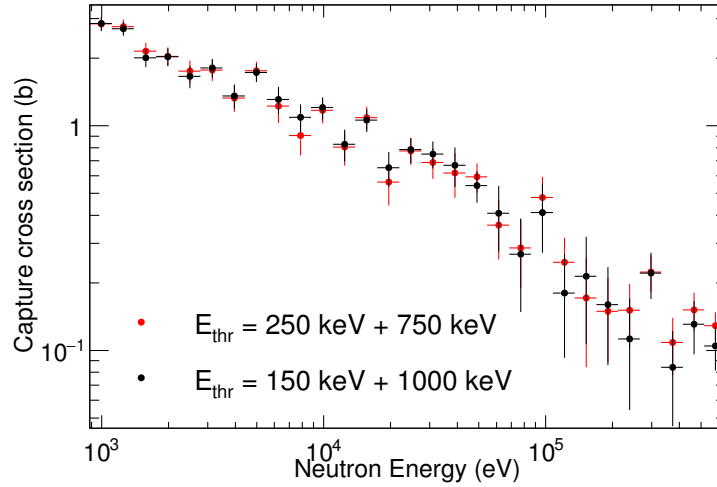
Figure 8.3: Final ^{242}\text{Pu} capture cross section obtained in this work with different threshold combinations: Low thresholds of 150 and 250 keV can be applied for neutron energies below 100 keV to maximize the statistics. For energies beyond 100 keV, a consistent result is obtained after we correct for the (n,f) background using a threshold higher than 750 keV, that allows removing the (n,n') background up to a neutron energy of 500 keV.
