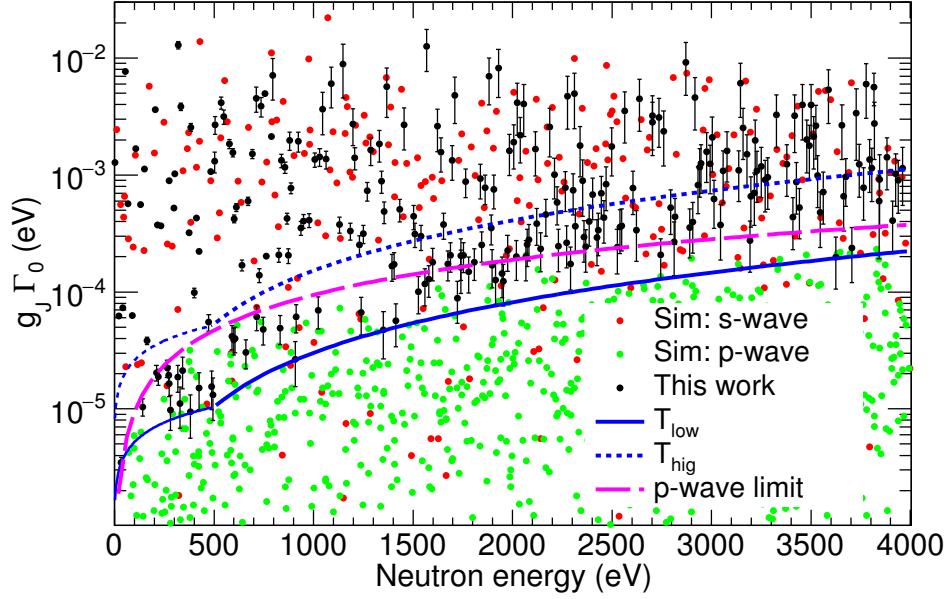
Figure 7.12: Experimental distribution of reduced neutron widths as a function of the neutron energy together with a random simulated set of s- and p-wave resonances ( D_0 = 12.5 eV). Different thresholds for observation of resonances and the p-wave identification threshold used in the study are shown on top (see text for details).
