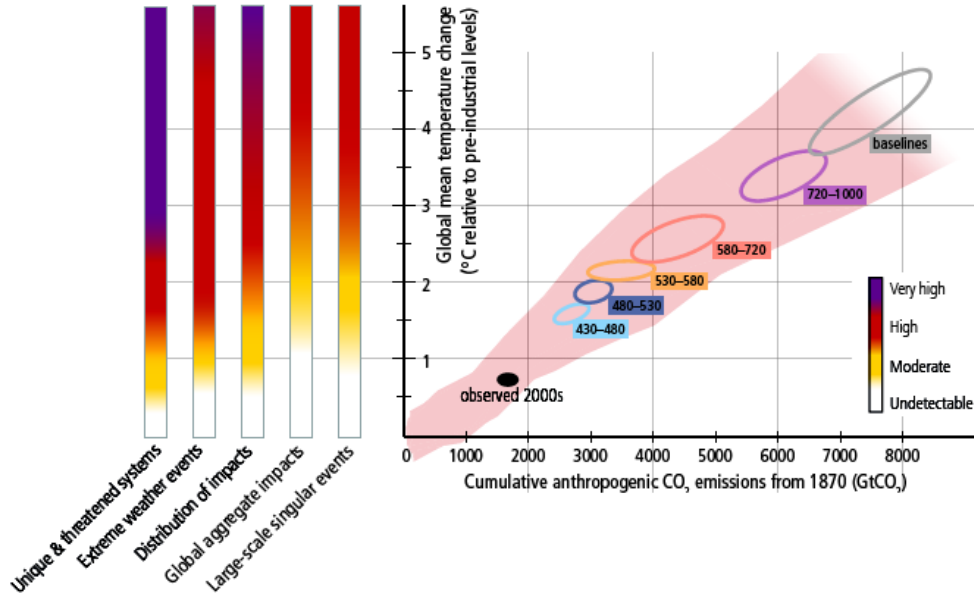
Figure 1.4: Correlation between the predicted average temperature increase and the cumulative CO 2 emissions. The circles indicate the expected results of different CO 2 mitigation scenarios (see text for details). From Ref. [2].
