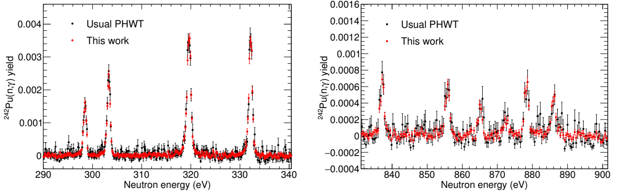
Figure 6.33: Capture yield of ^{242}\text{Pu} calculated with the usual PHWT method (black) compared to the approach followed in this work (red). The comparison is shown in two different energy regions in the RRR below 1 keV.
