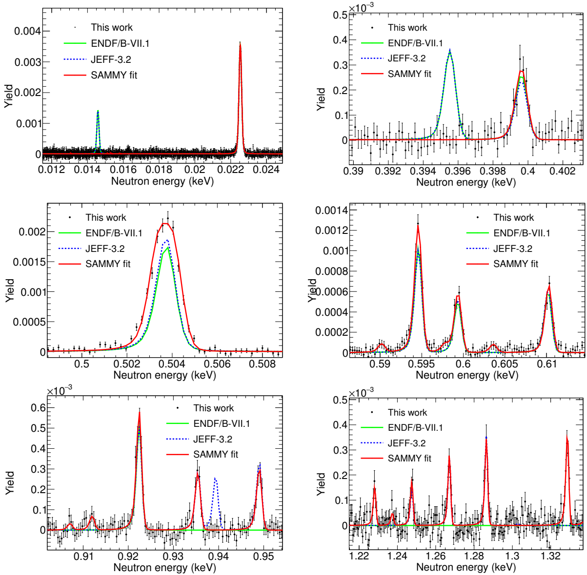
Figure 7.8: Capture yield from n -TOF together with the SAMMY fit (red) and the predictions from JEFF-3.2 (blue dashed) and ENDF/B-VII.1 (green) in several neutron energy ranges below 1.3 keV where significant differences are found.
