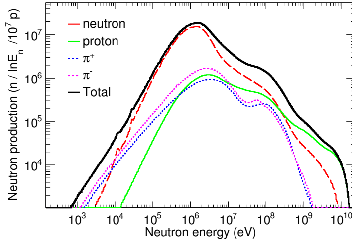
Figure 5.4: Energy distribution of neutrons produced inside the lead spallation target as a function of the neutron-producing particle.
