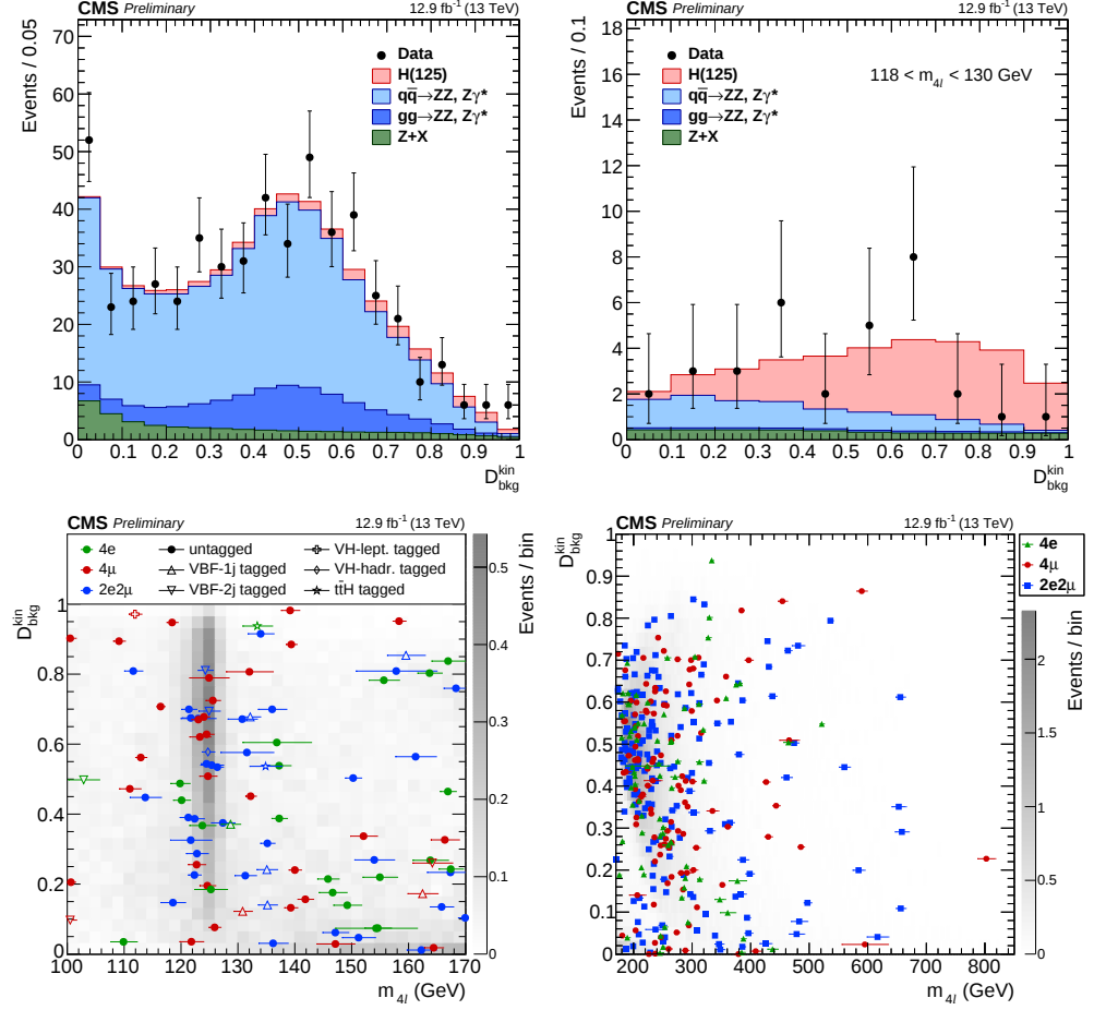
Figure 7.7: Top row: Distribution of the kinematic discriminant \mathcal{D}_{\text{bkg}}^{\text{kin}} in the full mass range (left) and in the mass region 118 < m_{4\ell} < 130 GeV (right). Points represent the data, with statistical uncertainties shown as vertical bars, and stacked histograms represent expected distributions. The H(125) signal and the ZZ backgrounds are normalized to the SM expectation, the Z+X background to the estimation from data. Bottom row: Distribution of \mathcal{D}_{\text{bkg}}^{\text{kin}} versus the four-lepton reconstructed mass m_{4\ell} in the low-mass region (left) and in the high-mass region (right). The grey scale represents the expected relative density of ZZ background plus H(125) signal. The points show the data and the horizontal bars represent the measured per-event mass uncertainties.
