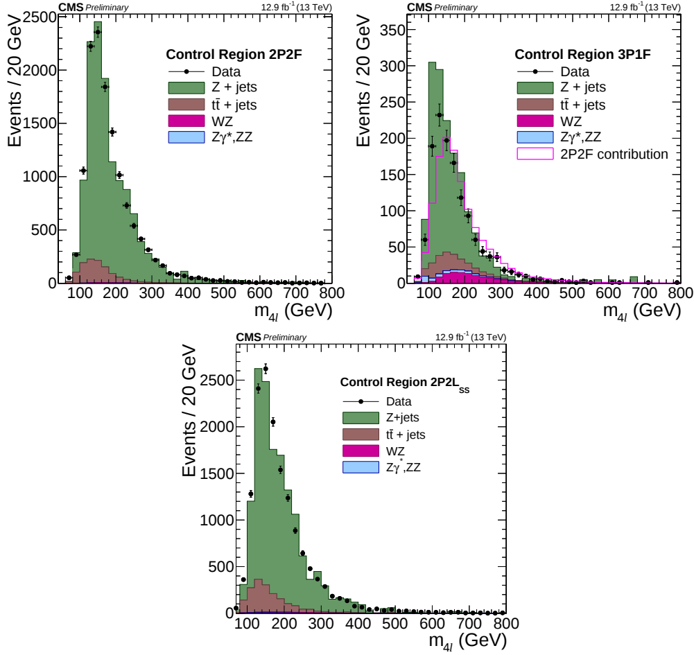
Figure 7.1: Distribution of the four-lepton invariant mass m_{4l} in the 2P2F (top left), 3P1F (top right) and 2P2L ss (bottom) control regions, for the sum of all final states and event categories. Points represent the data, with statistical uncertainties shown as vertical bars, and stacked histograms represent expected distributions from simulation, for the main contributing processes. The empty pink histogram in the 3P1F plot represents the predicted contribution of 2P2F-type processes to this region, which has to be subtracted when estimating the Z+X background (see Eq. 5.14).
