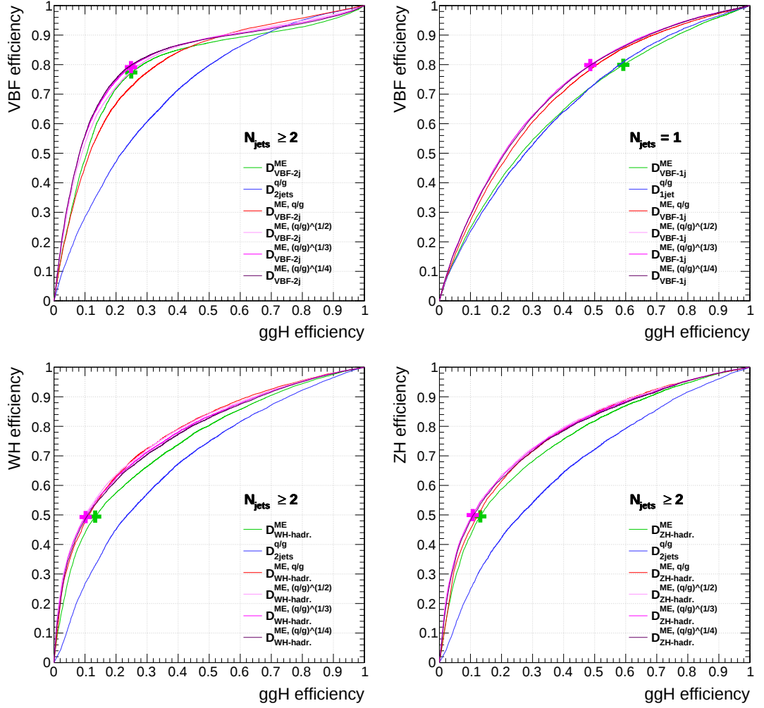
Figure 5.9: Performance comparison of matrix-element based, quark-gluon based and combined discriminants. Four cases are studied: 2-jet VBF vs. gluon fusion H + 2 jets (top left), 1-jet VBF vs. gluon fusion H + 1 jet (top right), hadronic WH vs. gluon fusion H + 2 jets (bottom left), and hadronic ZH vs. gluon fusion H + 2 jets (bottom right). The combined discriminants are shown in an untransformed version, and with three transformations of the \mathcal{G}/\mathcal{Q} ratio (square, cube and quartic root). Samples are generated with m_H = 125 GeV; events are required to pass the full analysis selection and to be in a 118 < m_{4\ell} < 130 GeV window. The cross markers represent operating points for event categorization, which will be defined in Section 5.4.
