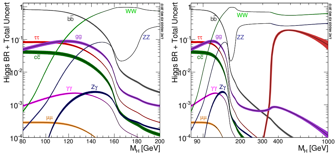
Figure 1.3: Decay branching ratios with uncertainties for the SM Higgs boson as a function of m_H , in a low-mass range (left) and in a range extending to high mass (right).
