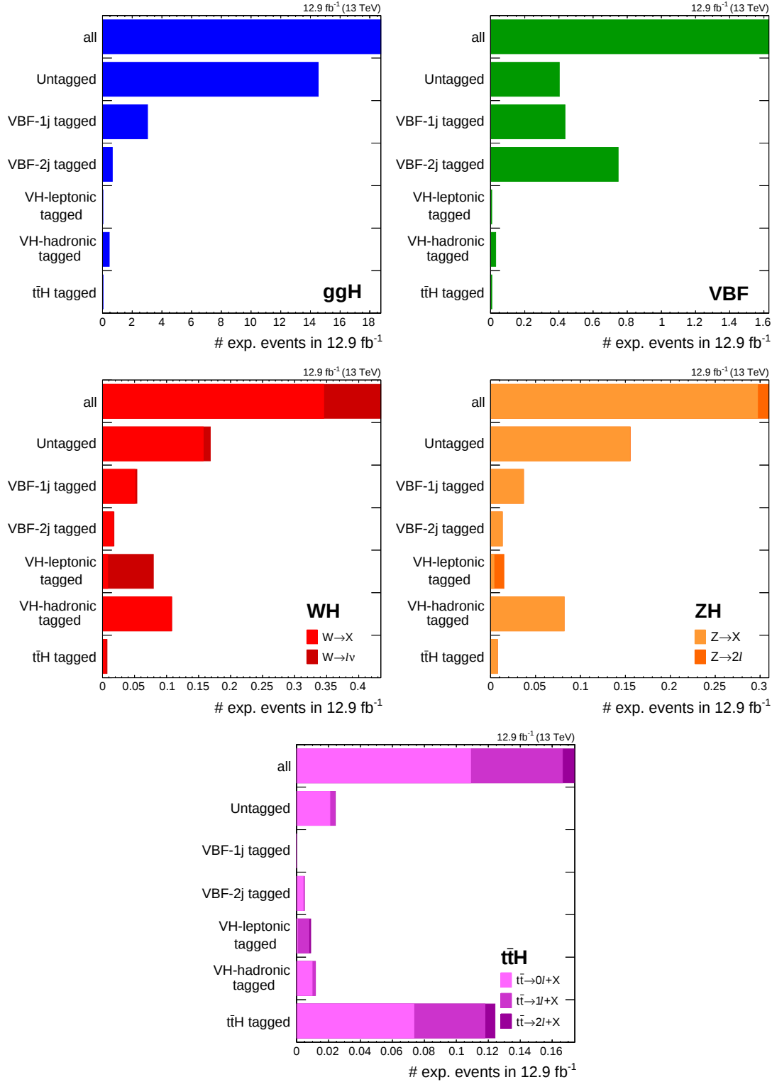
Figure 5.12: Distributions of signal processes in the six categories, for the categorization of the 2016 analysis. The ggH, VBF, WH, ZH, and ttH processes are presented in that order. The three latter processes are split according to the generated decay of the associated W, Z, or tt system, whereby the X symbol stands for a set of any other particles than electrons or muons. Samples are generated with m_H = 125 \text{ GeV} ; events are required to pass the full analysis selection and to be in a 118 < m_{4\ell} < 130 \text{ GeV} window. The first line of each plot shows the expected yield of the full selected event sample.
