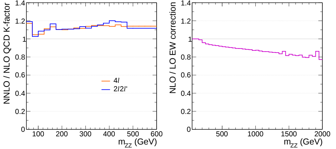
Figure 5.16: (left) NNLO/NLO QCD K-factor for the q\bar{q} \rightarrow ZZ background, as a function of generator-level m_{ZZ} , for the 4\ell and 2\ell 2\ell' final states. (right) Average impact of the NLO/LO electroweak correction for the q\bar{q} \rightarrow ZZ background on its yields, as a function of generator-level m_{ZZ} .
