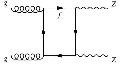
FIGURE 5.10: Leading-order diagram for the non-resonant process gg \rightarrow ZZ^{(*)} .
