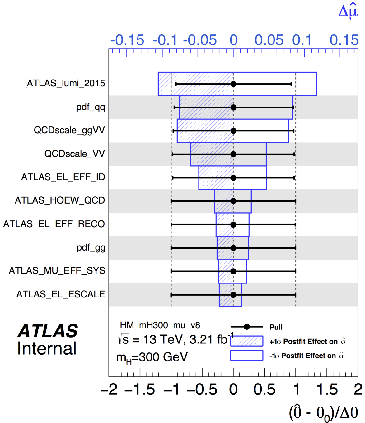
FIGURE 7.8: Nuisance parameter ranking performed with Asimov data generated at \mu = 0 at m_H = 300 \text{ GeV} .
