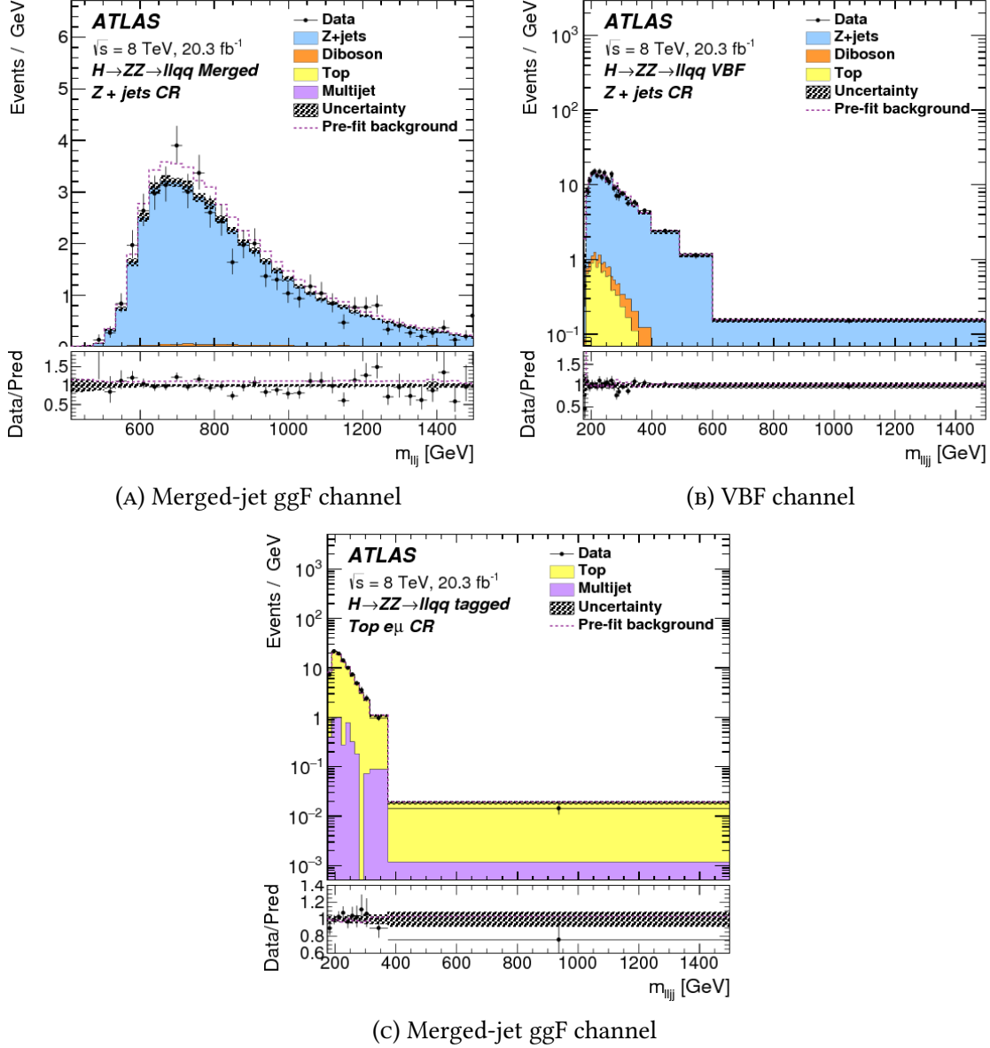
FIGURE A.1: The distributions of m_{\ell\ell jj} or m_{\ell\ell j} in the Z +jets control region of the H \rightarrow ZZ^{(*)} \rightarrow 2\ell 2q search in merged-jet ggF (A), VBF (B) event categories and the distribution of m_{\ell\ell jj} in the e\mu top-quark control region (C). The dashed line shows the total background used as input to the fit. The contribution labelled as "Top" includes both the t\bar{t} and single-top processes. The bottom panels show the ratio of the observed data to the predicted background
