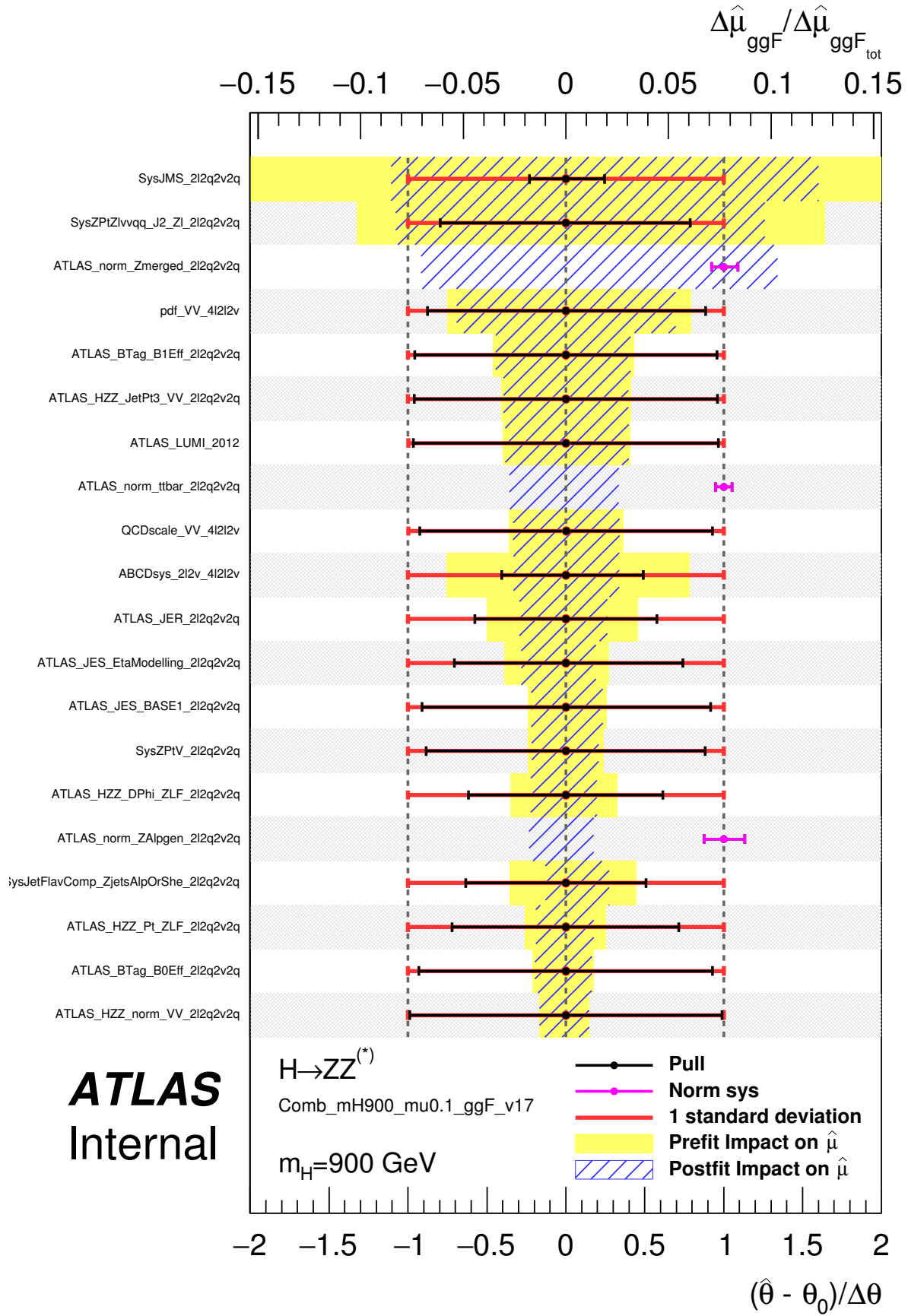
FIGURE 6.7: Nuisance parameter ranking for the combined fit performed at m_H = 900 \text{ GeV} with Asimov data generated with \mu_{\text{ggF}} = 0.1 .
