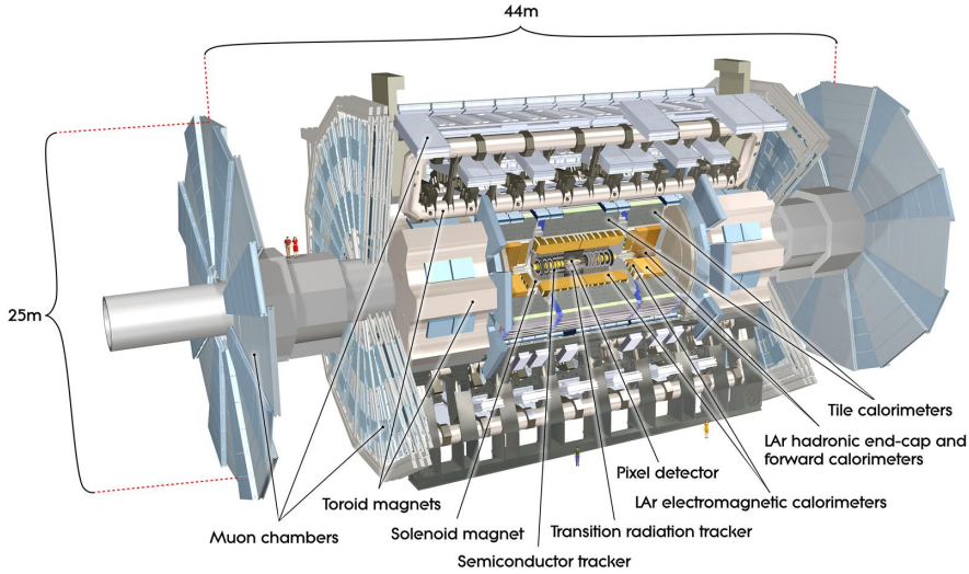
FIGURE 3.3: Schematic of the full ATLAS detector. The individual detector components of the Inner Detector, the Calorimeters and Muon Spectrometer are marked [66].
