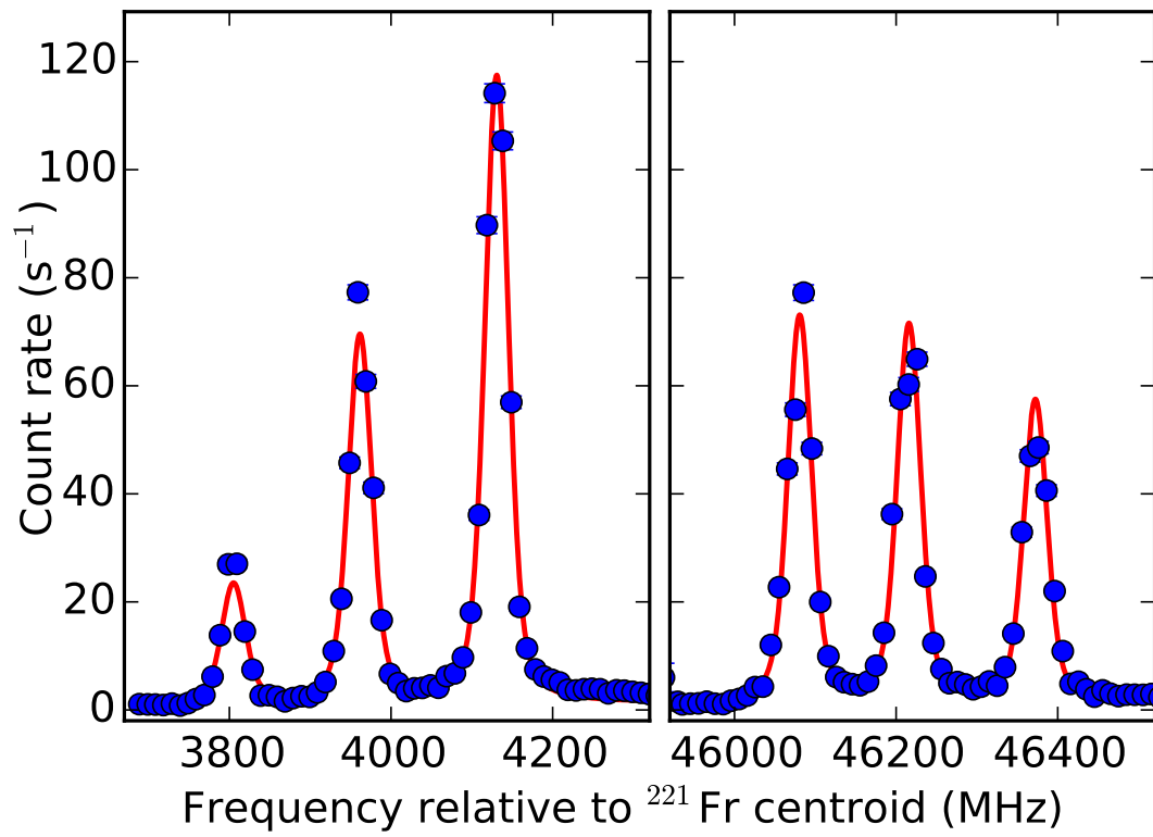
FIGURE A.4: Example spectrum of the 7s\ ^2S_{1/2} \rightarrow 8p\ ^2P_{3/2} transition in ^{207}\text{Fr} .
