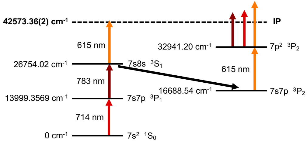
FIGURE 6.8: Atomic-radium ionization scheme used in the first radium experiment.
