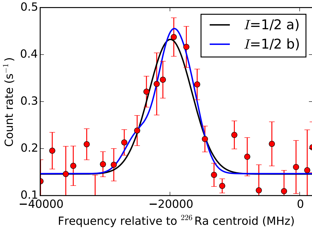
FIGURE 8.6: Example low-resolution spectrum of the 7s\ ^1S_0 \rightarrow 7s7p\ ^3P_1 transition in ^{233}\text{Ra} . The black and blue lines are fits of the data assuming spins of I = 1/2 . Fit I = 1/2 a) sets the hyperfine A and B parameters to zero and fit I = 1/2 b) allows non-zero values of A and B .
