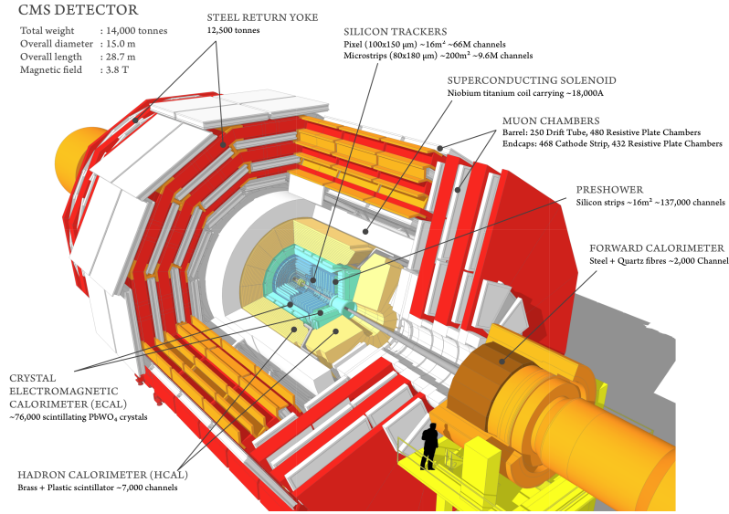
Figure 2.3: Schematic view of the CMS detector showing its subdetectors.
