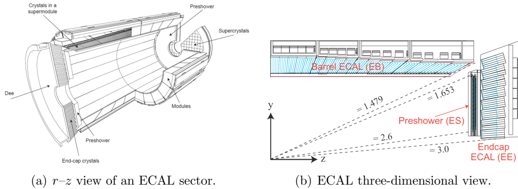
Figure 2.9: Schematic representation of the CMS electromagnetic calorimeter.
