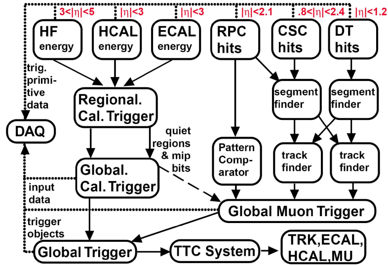
Figure 2.14: Schematic representation of the Level-1 trigger components.
