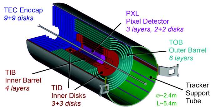
Figure 2.5: Three-dimensional schematic view of the CMS silicon tracker.
