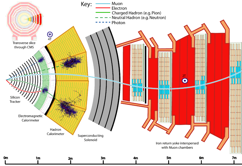
Figure 2.4: Schematic view of a slice of the CMS detector, showing the subdetectors response to the passage of different types of particles.
