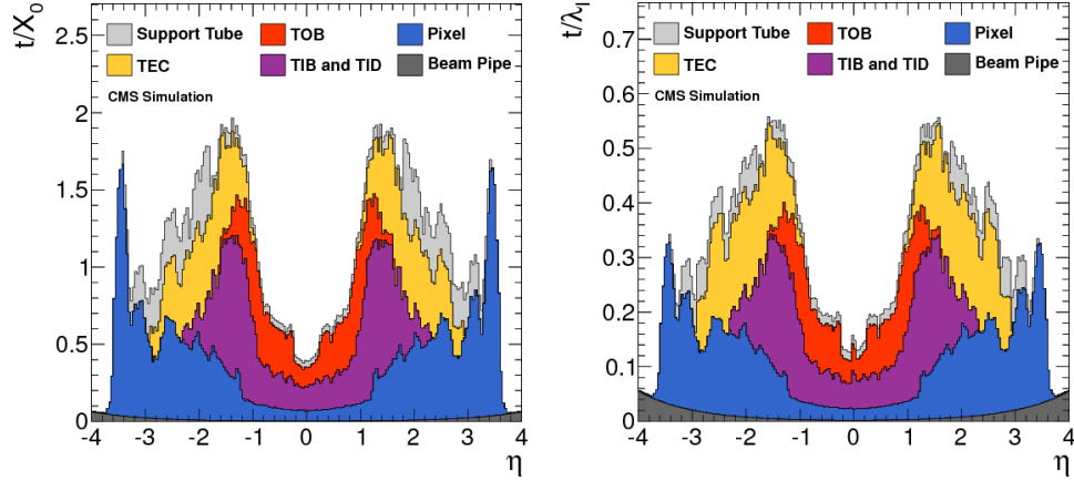
Figure 2.7: Total thickness t of the tracker material expressed in units of X_0 (left) and \lambda_I (right), as a function of \eta . The contribution to the total material budget of each region of the detector is shown.
