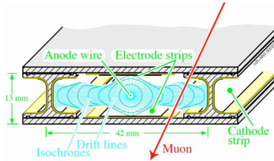
Figure 2.12: Schematic representation of a drift tube chamber, showing the drift lines in presence of magnetic field.
