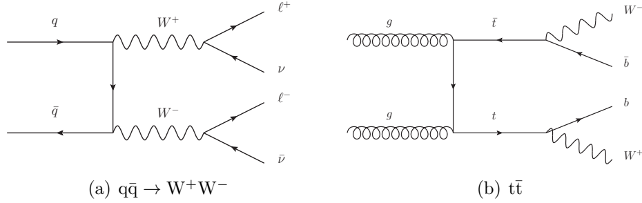
Figure 1.4: Feynman diagrams corresponding to the q\bar{q} \rightarrow W^+W^- (left) and t\bar{t} (right) processes. The t\bar{t} diagram represents just one of the possible ways to produce a pair of top quarks at hadron colliders.
