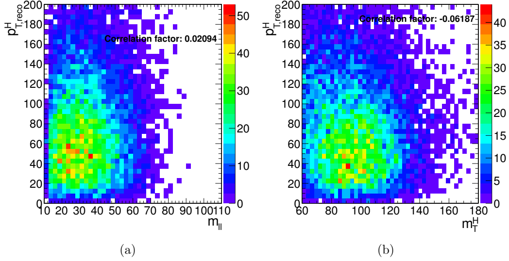
Figure 4.19: Correlation between p_T^H and m_{\ell\ell} (a) and between p_T^H and m_T (b) after the full selection for the VBF production mode.
