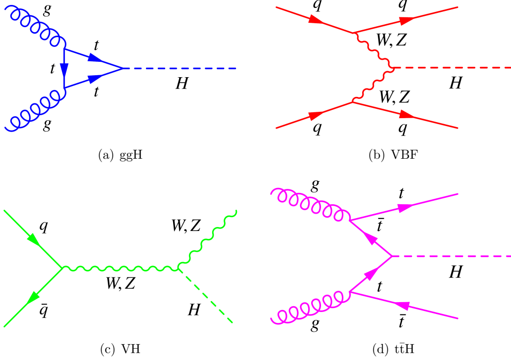
Figure 1.1: Main Higgs boson production processes at LHC.
