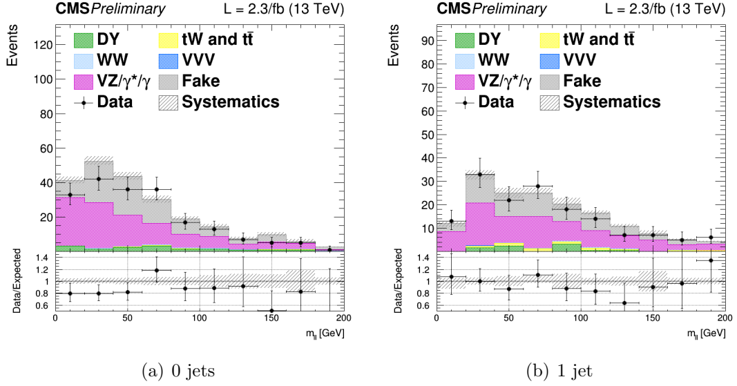
Figure 5.11: Control plots for m_{\ell\ell} in a Fake enriched phase space for events with 0 and 1 jet with p_T > 30 GeV, in e\mu final state. The normalization factor is not applied.
