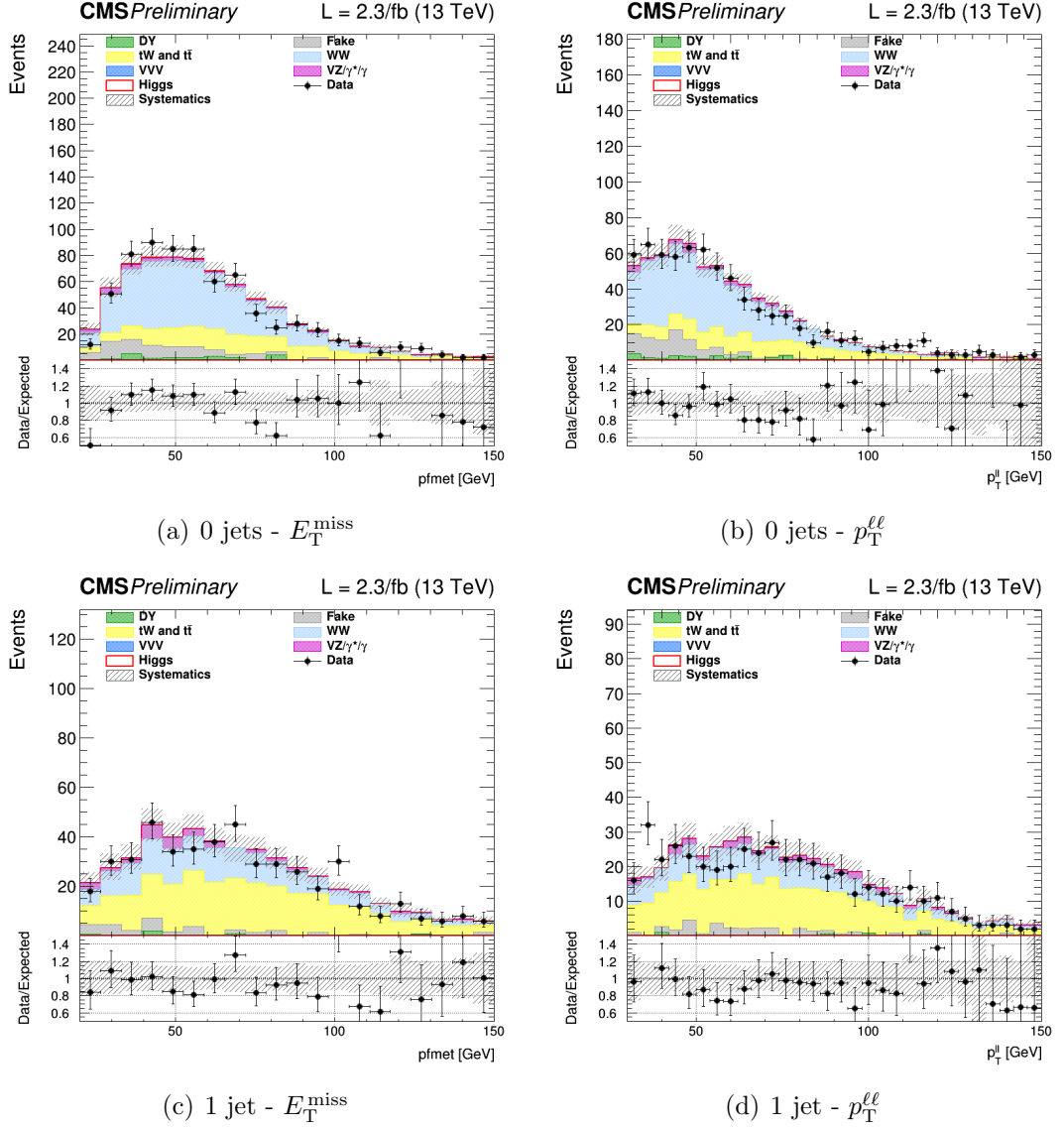
Figure 5.9: Distributions of E_T^{\text{miss}} (left) and p_T^{\ell\ell} (right) in events with 0 jets (upper row) and 1 jet (bottom row), for the main backgrounds (stacked histograms), and for a SM Higgs boson signal with m_H = 125 GeV (superimposed and stacked red histogram) after the analysis event selection.
