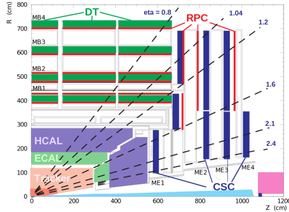
Figure 2.11: Schematic view of a quadrant of the CMS muon system.
