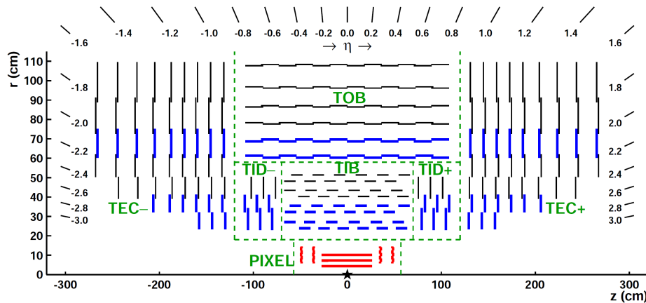
Figure 2.6: Pictorial view of a tracker slice in the r - z plane. Pixel modules are shown in red, single-sided strip modules are depicted as black thin lines and strip stereo modules are shown as blue thick lines.
