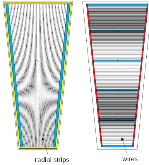
Figure 2.13: Schematic representation of CSC cathode (left) and anode (right) panels.
