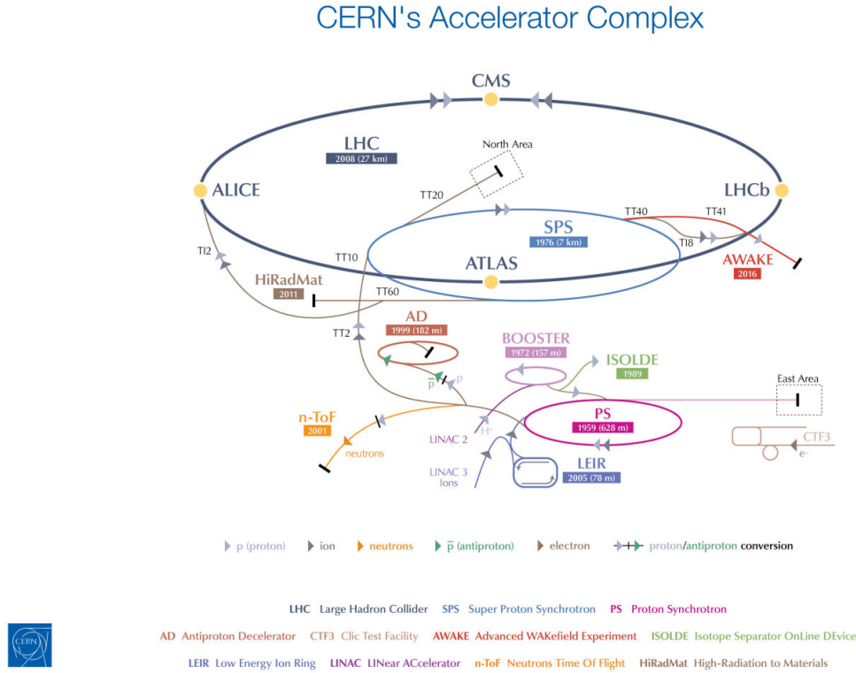
Figure 2.1: Schematic description of the accelerator complex installed at CERN.
