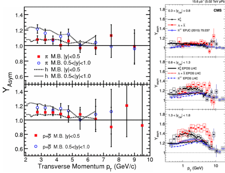
FIGURE 1.17: Left: rapidity yield asymmetry ( Y_{\text{asym}} ) as a function of transverse momentum ( p_T ) for d–Au collisions at \sqrt{s_{\text{NN}}} = 200 GeV for identified particle ( \pi , h and p(\bar{p}) ). Right: Y_{\text{asym}} as a function of p_T for multi-strange hadrons ( K_S^0 , \Lambda ) and inclusive charged hadrons in p–Pb collisions at \sqrt{s_{\text{NN}}} = 5.02 TeV. This figure is taken from [75, 76].
