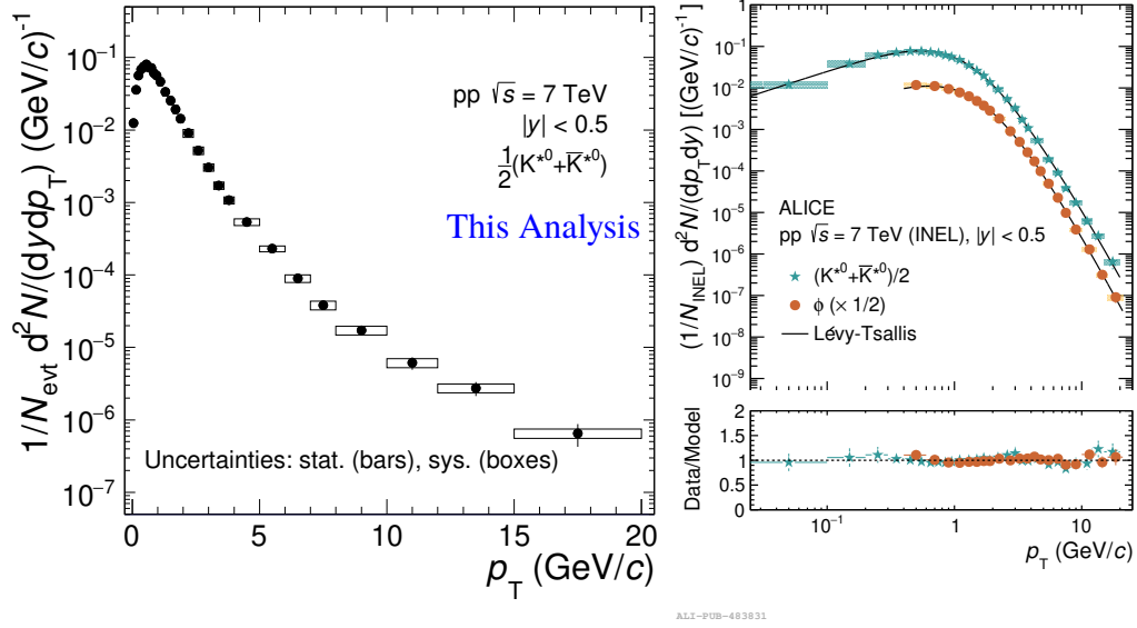
FIGURE 5.5: Left figure: measurement of K^{*0} p_T spectrum in p_T range up to 20 \text{GeV}/c at midrapidity in pp collisions at \sqrt{s} = 7 \text{ TeV} . The errors shown includes both statistical (bars) and systematic (boxes) uncertainties. Right figure: Upper panel comparison of p_T spectrum of K^{*0} and \phi , is fitted with Lévy-Tsallis function in pp collisions at \sqrt{s} = 7 \text{ TeV} . Lower panel shows the ratio of data to the Lévy-Tsallis fit. Here, the bars show the systematic uncertainty.
