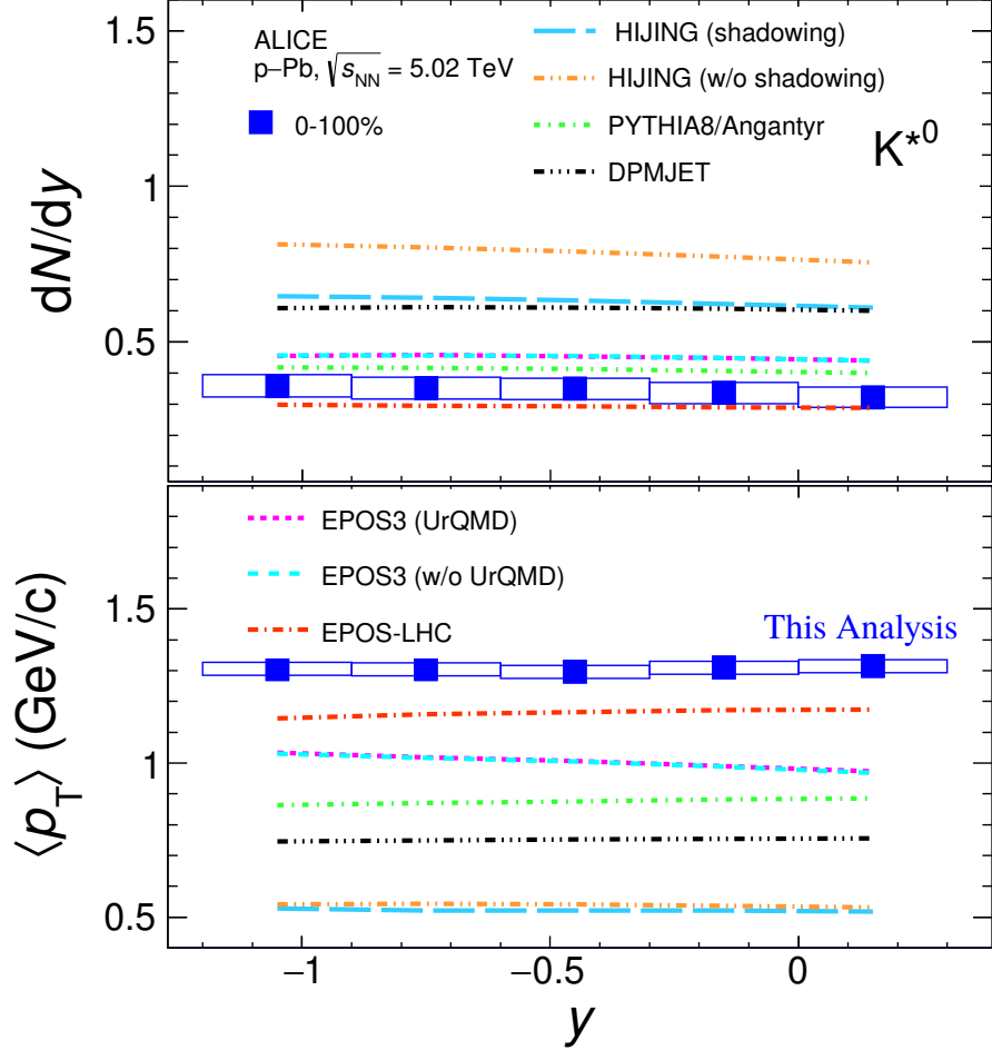
FIGURE 4.11: The p_T integrated yield, dN/dy (top) and mean transverse momentum, \langle p_T \rangle (bottom) for K^{*0} as a function of y measured for multiplicity class 0-100% in p - Pb collisions at \sqrt{s_{NN}} = 5.02 TeV. The predictions from EPOS-LHC [21], DPMJET [24], HIJING [25], PYTHIA(Angantyr) [26] and EPOS with and without UrQMD [22, 23] are also shown as different curves. The statistical uncertainties are represented as bars whereas the boxes indicate total systematic uncertainties.
