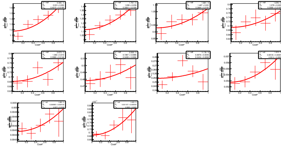
FIGURE D.17: Angular distribution of decay daughter of K^{*0} for 10–50% centrality class in Pb–Pb collisions at \sqrt{s_{\text{NN}}} = 5.02 TeV using helicity frame analysis.
