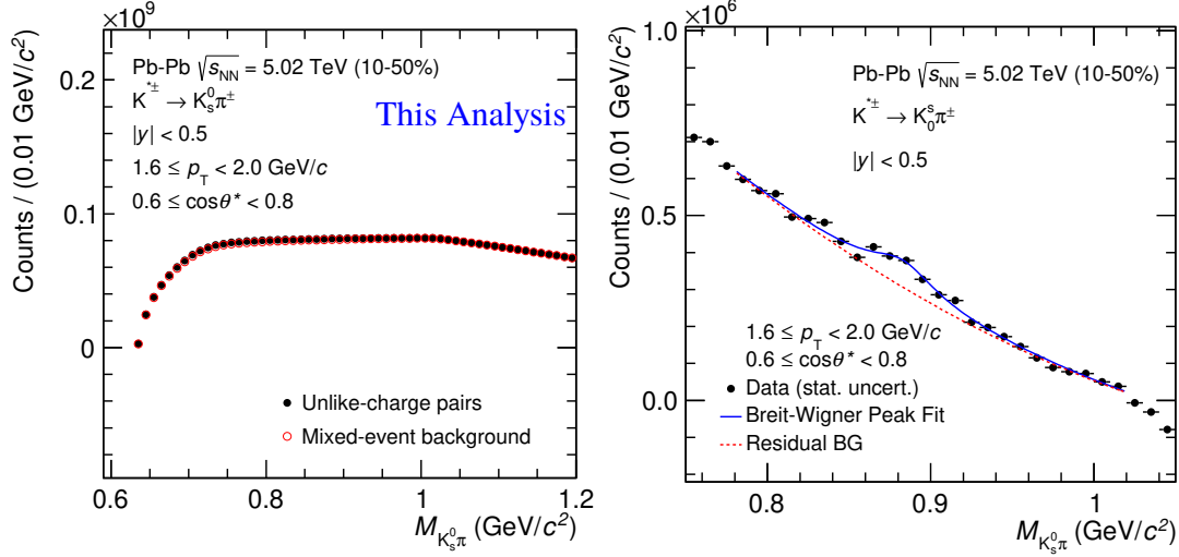
FIGURE 6.4: Left figure shows invariant mass distribution of K_S^0 \pi same event pairs (black markers) and mixed-event background pairs (red markers). Right panel shows invariant mass distribution of K_S^0 \pi pairs after normalized mixed-event background subtraction. The invariant mass distribution is fitted with Breit-Weigner distribution function (blue line) for signal and exponential plus polynomial function of second order for residual background function (red dotted lines) in the p_T interval 1.6 \leq p_T < 2.0 \text{ GeV/c} for \cos\theta^* interval 0.6 to 0.8 in the 10–50% centrality class for Pb–Pb collisions at \sqrt{s_{NN}} = 5.02 TeV. Quantization axis is normal to the production plane.
