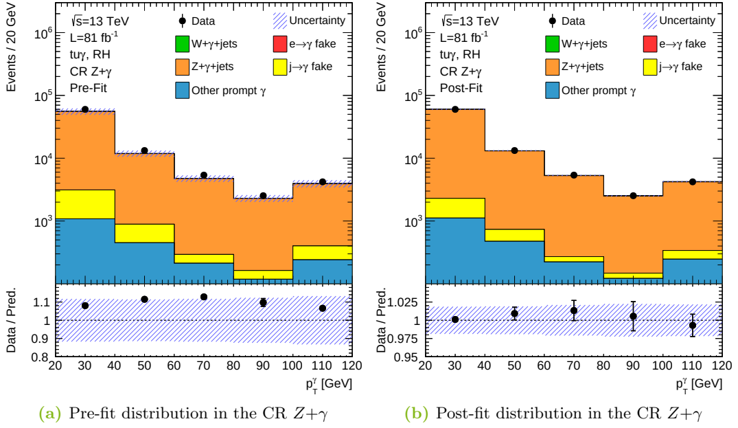
Figure 55: Pre- (a) and post-fit distribution (b) of the photon p_T spectrum in the CR Z+\gamma for the RH t\bar{t}\gamma coupling. All uncertainties are included. Since the signal contribution is negligible in this region, its shape is not overlaid.
