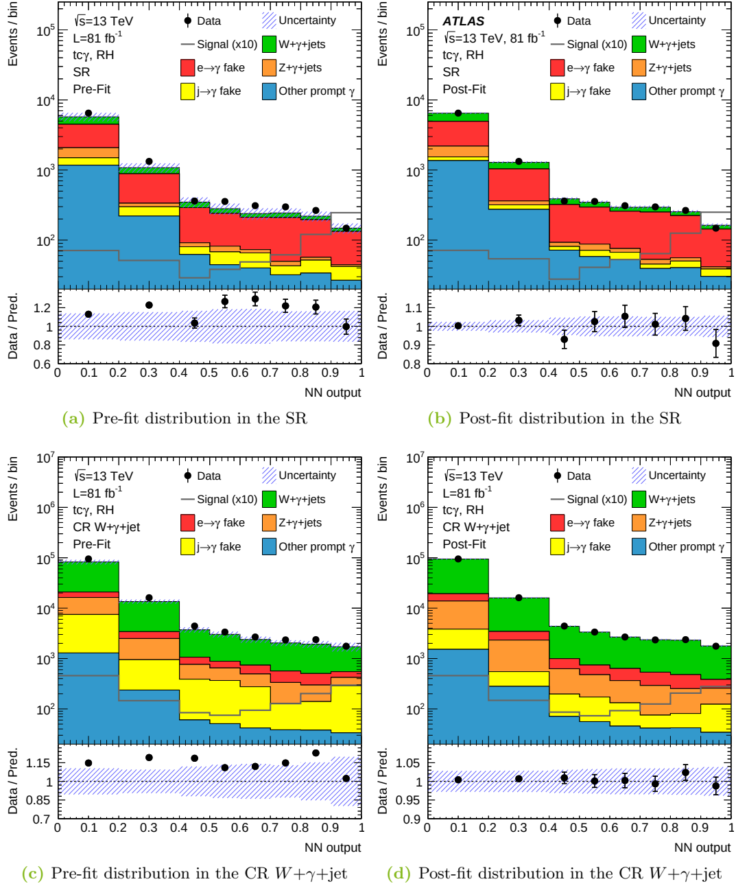
Figure 70: Pre- and post-fit distributions of the NN output in the SR (a,b) and CR W+\gamma+jet (c,d) for the RH tc\gamma coupling. All NPs are included. The signal shape is overlaid scaled to the observed limit multiplied by ten. The post-fit plot for the SR is published in the auxiliary material of Ref. [11]. It is also shown in Figure 45c and here to enable for a direct comparison to the pre-fit plot.
