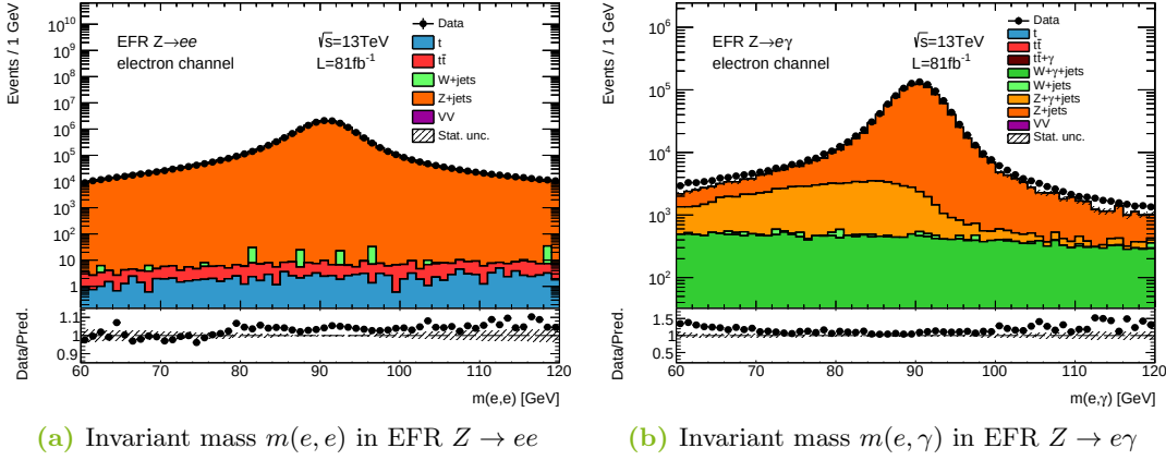
Figure 25: Observed and expected distributions of the invariant mass m(e, e) in the EFR Z \rightarrow ee (a) and m(e, \gamma) in the EFR Z \rightarrow e\gamma (b). In the bottom plot, the ratio between data and MC simulation is shown. Only statistical uncertainties are shown.
