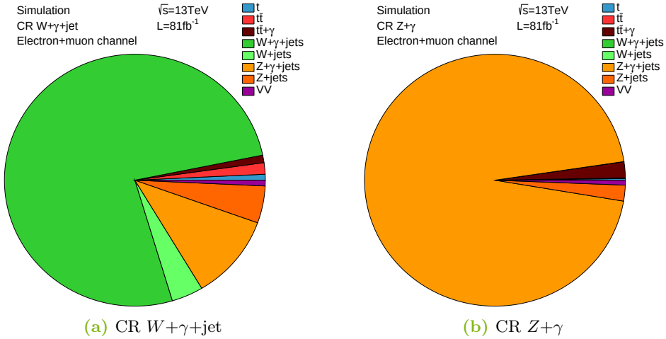
Figure 21: Illustration showing the composition of the SM processes in the CR W+\gamma+\text{jet} (a) and CR Z+\gamma (b).
