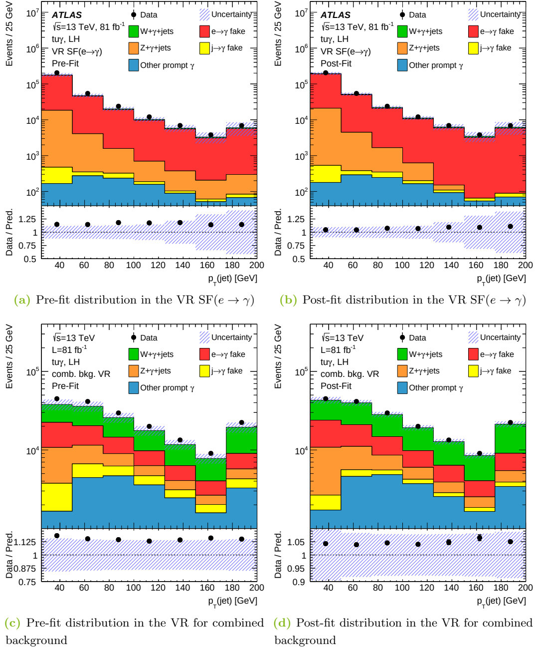
Figure 48: Pre- and post-fit distributions of the jet p_T in the VR \text{SF}(e \rightarrow \gamma) (a,b) and in the VR for combined background (c,d) for validating the fit outcome of the LH t\bar{u}\gamma coupling. All uncertainties are included. The plots for the VR \text{SF}(e \rightarrow \gamma) are published in the auxiliary material of Ref. [11].
