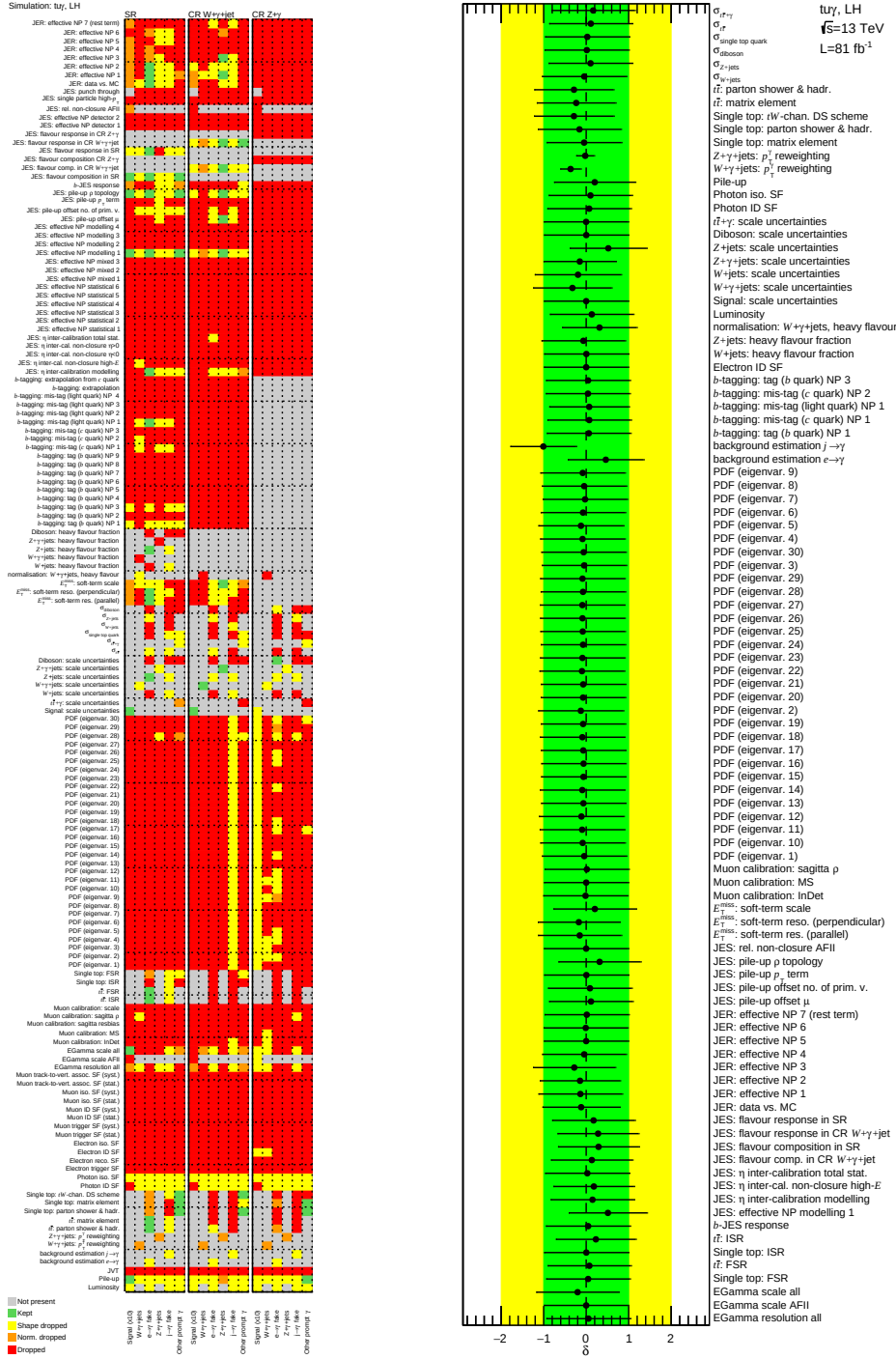
Figure 40: Illustration of the treatment of every systematic NP considered in the fit for the LH t\gamma coupling in each region for each signal and background category. Figure 41: Pull values, \delta , for the systematic NPs considered and determined in the fit for the LH t\gamma coupling.
