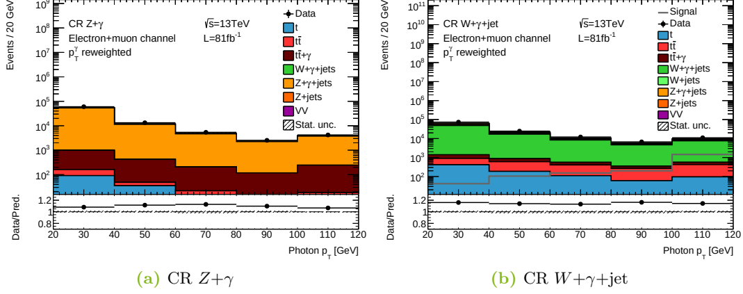
Figure 24: Observed and expected distributions of the photon p_T spectrum after the p_T reweighting in the CR Z+γ (a) and in the CR W+γ+jet (b). In the CR Z+γ, the signal contribution is negligible and not drawn, while it is overlaid in the CR W+γ+jet. In the bottom panel, the ratio between data and background prediction is depicted. Only the statistical uncertainties are shown and the overflow is included.
