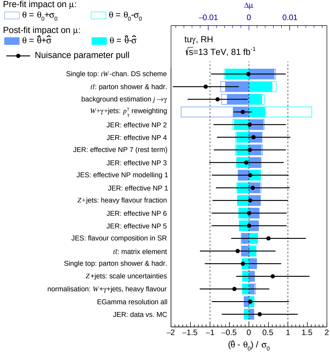
Figure 56: Ranking of the NPs with the largest impact on the signal strength, \mu , for the RH tu\gamma coupling. The signal strength of unity corresponds to the branching ratio \mathcal{B}_{\text{in}}(t \rightarrow u\gamma) = 10^{-3} . The ranking is determined in fits fixing the NP under study to its pre-fit value \theta_0 and adding or subtracting its pre-fit uncertainty, \sigma_0 , and analogously for the post-fit value, \hat{\theta} , and its uncertainty, \hat{\sigma} . The rectangles refer to the upper axis, while the black dots refer to the bottom scale.
