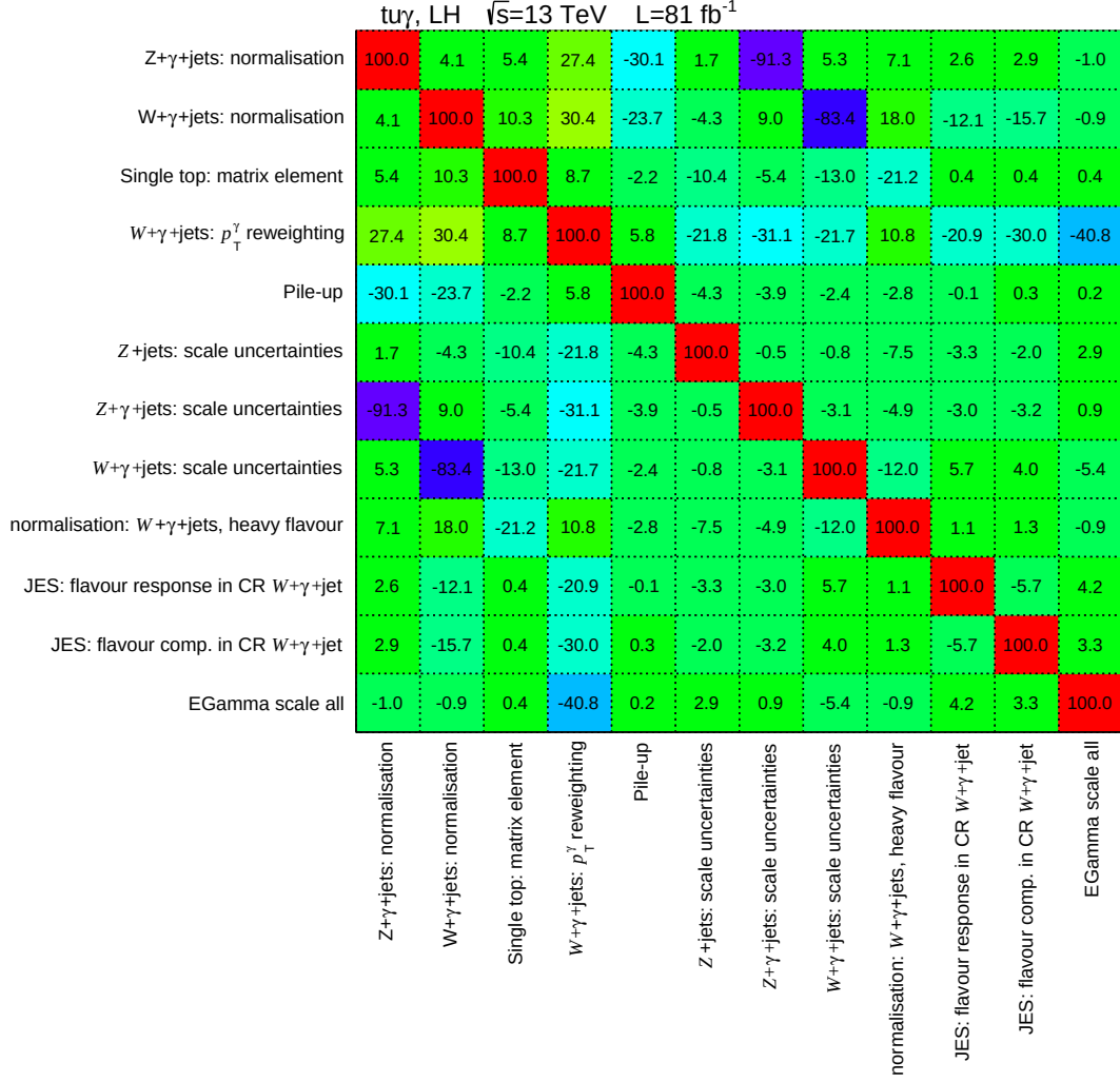
Figure 39: Visualisation of the correlation coefficients between the NPs of systematic nature for the LH tu\gamma coupling. Only uncertainties with the absolute value of at least one coefficient above 0.2 are drawn.
