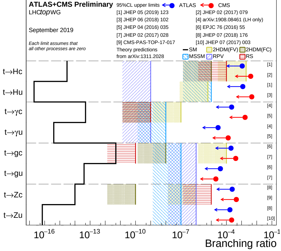
Figure 1: Summary [1] of the currently best observed 95 % CL limits on the branching ratios of the top quark decaying via an FCNC involving a neutral boson t \rightarrow Xq ( X = g, Z, \gamma, H; q = u, c ) by the ATLAS and CMS collaborations. For the exclusion limits for the decay t \rightarrow \gamma q set by the ATLAS collaboration, only the left-handed coupling is assumed. These observed limits are compared to the SM predictions [2] and the maximal predictions of several BSM theories. These BSM models are the 2HDM with flavour violating Yukawa coupling ( 2HDM(FV) ) [3, 4], the 2HDM with flavour conservation ( 2HDM(FC) ) [5], the MSSM with 1 TeV squarks and gluinos ( MSSM ) [6], the MSSM with R -parity violation ( RPV ) [7, 8], and the model with a warped extra dimension in the Randall-Sundrum framework ( RS ) [9, 10].
