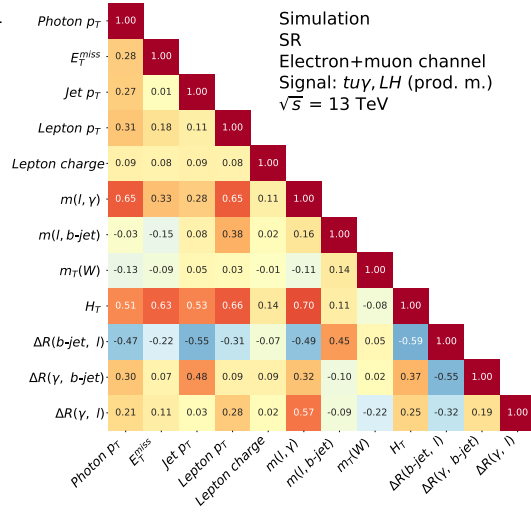
Figure 30: Illustration for the correlation coefficients of the potential input variables for signal of the LH tu\gamma coupling in the production mode in the SR.
