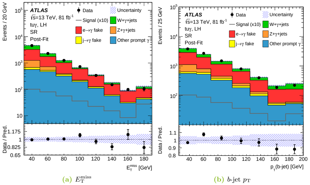
Figure 73: Post-fit distributions of the E_T^{\text{miss}} (a) and b -jet p_T (b) in the SR. All uncertainties are included. The signal shape is overlaid scaled to the observed limit. The plots are published in the auxiliary material of Ref. [11].
