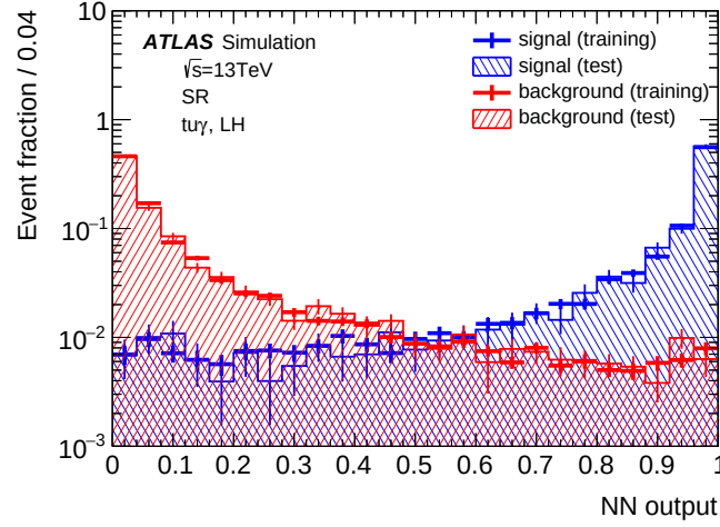
Figure 35: Shapes of the training and test datasets for both the production-mode signal and the background for the deep NN output for the LH t\bar{u}\gamma coupling. Only the statistical uncertainties are included. The plot is published in the auxiliary material of Ref. [11].
