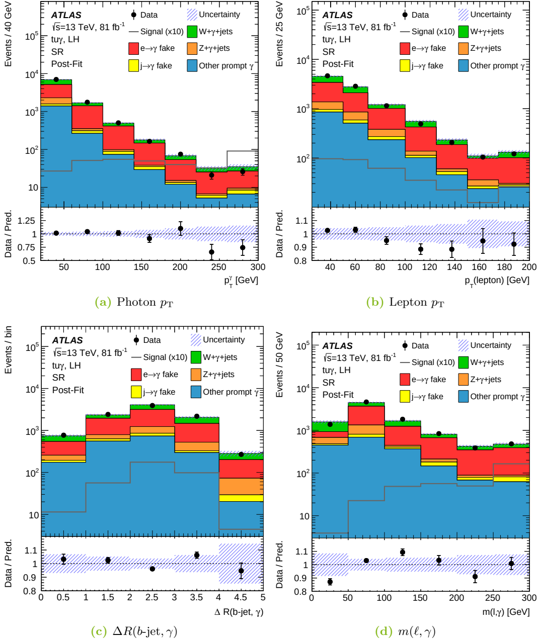
Figure 47: Post-fit distributions of the photon p_T (a), lepton p_T (b), distance \Delta R between the b -tagged jet and photon (c) and the invariant mass m(\ell, \gamma) (d) in the SR for the LH t\gamma coupling. All uncertainties are included. The signal is overlaid scaled to the observed limit multiplied by ten. The plots are published in the auxiliary material of Ref. [11].
