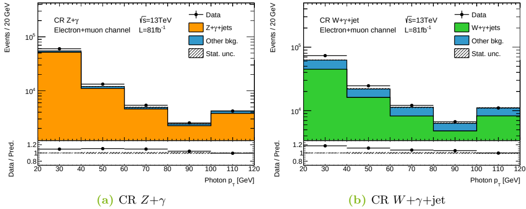
Figure 22: Observed and expected distributions of the photon p_T in the CR Z+\gamma (a) and in the CR W+\gamma+\text{jet} (b). In the bottom plot, the ratio between data and background prediction is depicted. Only the statistical uncertainties are shown and the overflow is included.
