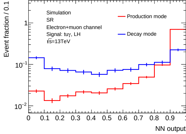
Figure 36: Shapes of the production- and decay-mode signal for the NN output for the LH t\gamma coupling. Only the statistical uncertainties are included.
