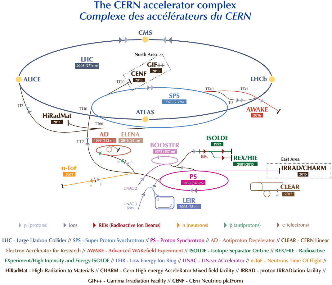
Figure 11: Overview of the current accelerator complex at CERN with its various experiments [70]. Different types of particles are accelerated and led into different machines. For the different facilities, the year of commissioning is given. For storage rings, the circumference is indicated.
