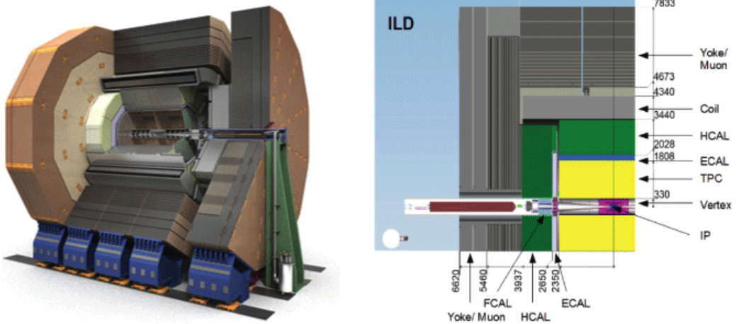
Figure 12: ILD schematic view (left) and quadrant section (right) [57]
