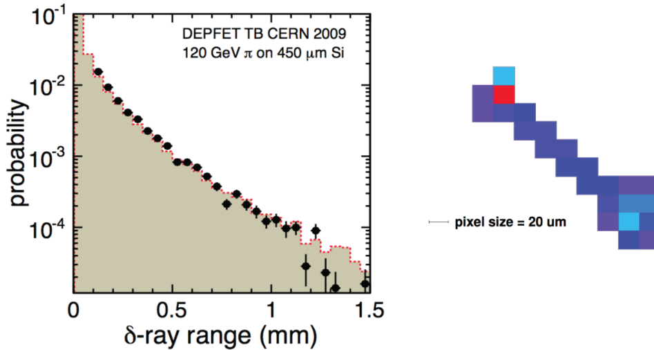
Figure 37: Left: Probability of \delta -electron emission by a 120 GeV pion traveling perpendicularly on a 450 \mu\text{m} thick Silicon sensor. The black points are data from DEPFET test beam data and the dashed line represents the GEANT4 simulation. Right: \delta -electron candidate detected with a DEPFET pixel detector [75].
