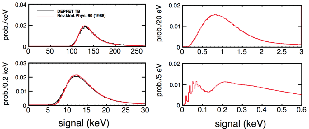
Figure 36: Energy deposition distribution in Silicon sensors with different thickness (450 \mu\text{m} - top-left, 50 \mu\text{m} - bottom-left, 5 \mu\text{m} - top-right, 1 \mu\text{m} - bottom-right). The plots on the left contains a comparison to the charge distribution collected by a DEPFET prototype with the corresponding thickness [75].
