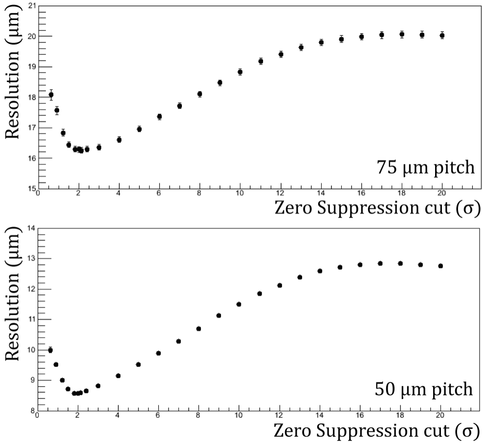
Figure 35: DEPFET sensor resolution as a function of the zero suppression cut. Upper plot shows the results on the rows direction (pitch 75 μm) and the bottom plot on the columns direction (pitch 50 μm) [73].
