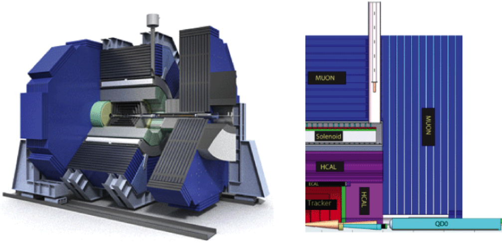
Figure 11: SiD schematic view (left) and quadrant section (right) [57]
