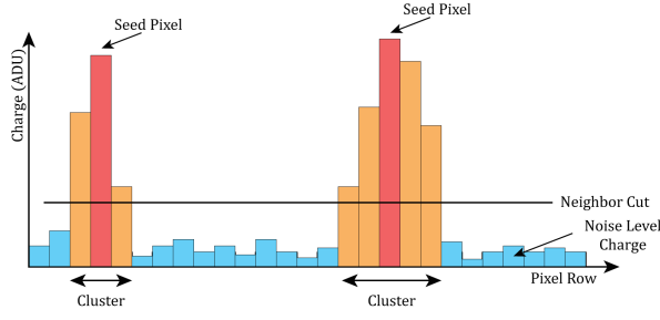
Figure 33: Charge deposited by two impinging particles in one row. The neighbor cut should be high to exclude noisy pixels but has to include all the cluster information.
