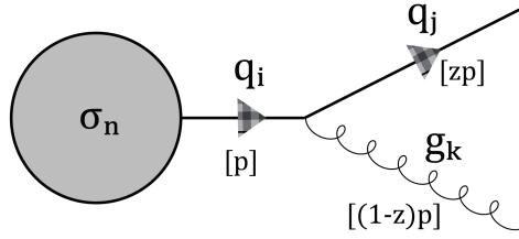
Figure 90: Quarks i , splits in quark j and gluon k .
