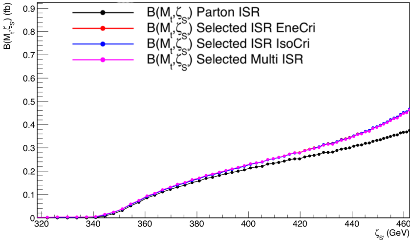
Figure 150: B_\gamma(m_t, \zeta_{S'_\gamma}) comparison, using a final selection criteria, in case multiple photos survive to the selection process. Black: B(m_t, \zeta_{S'}) in at partonic level. Red: Most energetic photon selected. Blue: Most isolated photon selected. Purple: Multiple photon calculation.
