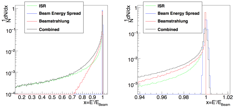
Figure 119: Differential luminosity spectrum and the different contributions (left). Expanded scale around the peak(left) [107]
