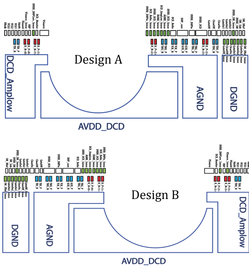
Figure 75: Pad distribution layout of the two PXD9 module flavor, with 59 Al pads and 4 Cu pads. In red, the 8 pads of the LVDS high speed lines. In blue, the pads related with JTAG configuration. In green, the pads corresponding to the sense lines.
