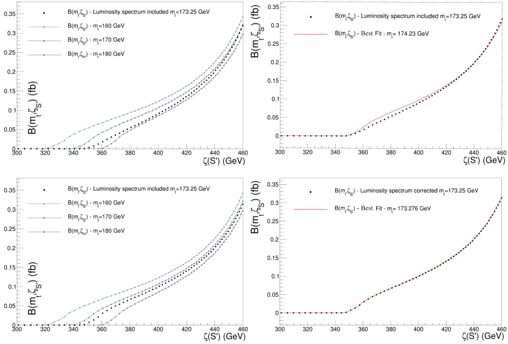
Figure 122: Upper plots: B_\gamma(m_t, \zeta_{S'}) distribution obtained with the luminosity spectrum included ( m_t = 173.25 GeV). It has been compared to the partonic distributions (left). The data-set has been fitted with the partonic distributions (right - m_t = 174.23 GeV). Lower plots: B_\gamma(m_t, \zeta_{S'}) distribution with the migrations due to the luminosity spectrum corrected ( m_t = 173.25 GeV). The final mass obtained after the correction was m_t = 173.276 GeV (right)
