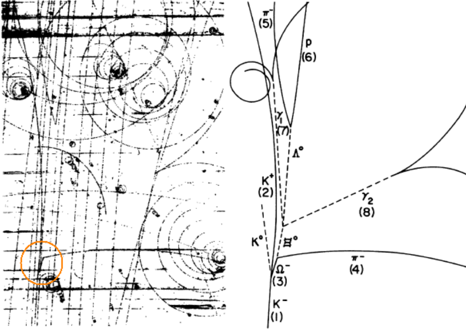
Figure 4: Discovery of \Omega^- in a bubble chamber [29].
