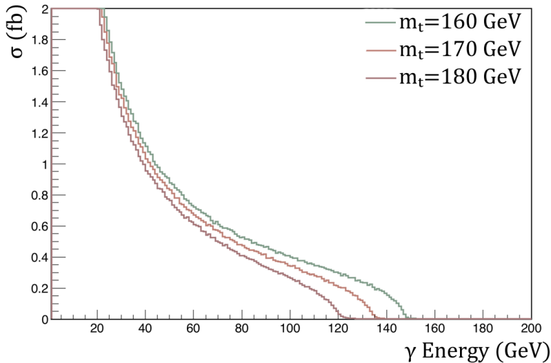
Figure 97: Energy distribution on the ISR Photons, in e^+e^- \rightarrow t\bar{t} events with a Monte Carlo mass m_t = 160 \text{ GeV}, 170 \text{ GeV}, 180 \text{ GeV}
