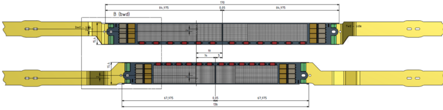
Figure 46: DEPFET ladder design picture (top: outer module, bottom: inner module). The size of the pixels on each ladder will vary to optimize the sharing of charge between pixels. On the central region the pixel density will be higher since more perpendicular tracks are expected [79].
