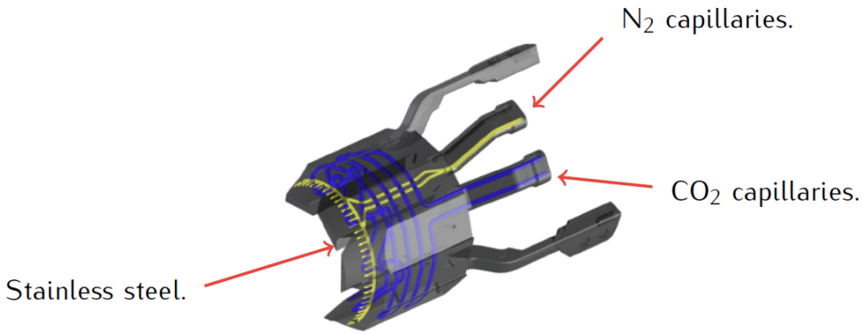
Figure 49: Support and cooling block (SCB). The \text{CO}_2 at -30^\circ\text{C} flows through the blue circuit and the \text{N}_2 at 0^\circ\text{C} through the yellow circuit [80].
