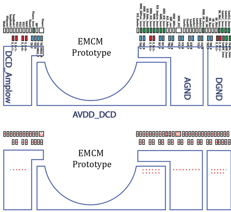
Figure 130: Top: EMCM pad distribution. Bottom: Contact distribution of the needles over the EMCM pad footprint, the red dots represent the place where the needle will perform the touchdown.
