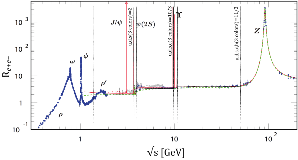
Figure 7: World data R_{e^+e^-} ratio[45] as a function of the center-of-mass energy. The center-of-mass energy regions are separated, with vertical lines, in terms of the quarks that the processes are capable to generated, the R_{e^+e^-} ratio changes when new quarks can be produces.
