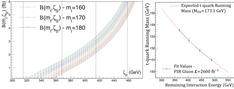
Figure 108: Left: Pseudo-theoretical distributions of B_g(m_t, \zeta_{S'}) . The vertical lines are the division of the B_g(m_t, \zeta_{S'}) regions uses to perform the fit. Right: the corresponding running mass obtained at 2600\text{fb}^{-1} . The black dots represent the mean mass obtained on the fits, considering the selected B_g(m_t, \zeta_{S'}) regions and the sensitivity is represented with the error bars. They have been plotted over the expected top-quark running mass calculated in the range of scales with a m_{t_{OS}} = 173.1\text{GeV} (red line)
