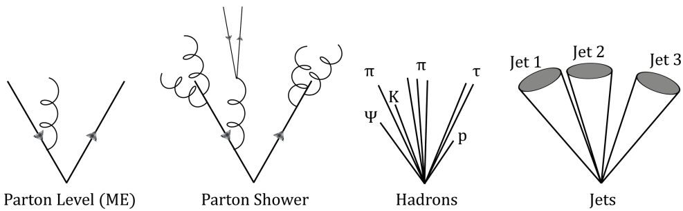
Figure 91: Jets algorithms have to provide a number of jets, insensitive to the soft and collinear emissions.
