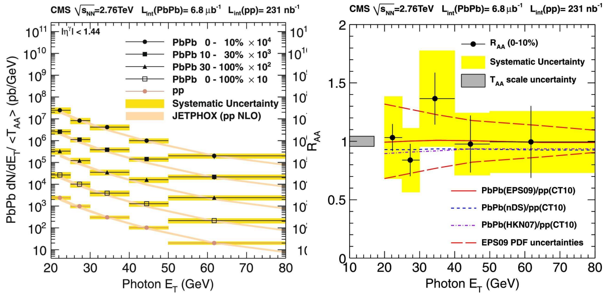
Figure 2.8: On the left, the differential isolated photon cross-section measured in pp and Pb-Pb collisions at \sqrt{s} = 2.76 \text{ TeV} with the CMS experiment. The theoretical calculation from JetPHOX are shown. On the right plot, the corresponding R_{AA} is plotted as well as the expected values of the ratio of the calculations performed with JetPHOX for Pb-Pb and pp collisions [28].
