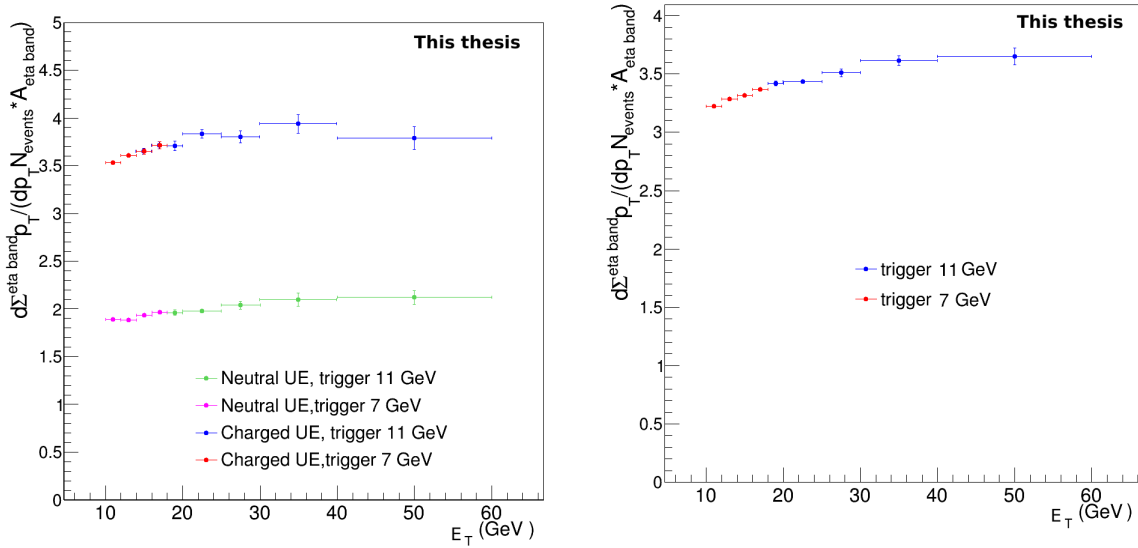
Figure 6.8: Left plot: < \sum p_T^{E\eta \text{ Band}} > depending on E_T for neutral and charged contribution in EM-Cal acceptance using LHC13d+e+f data set. Right plot: < \sum p_T^{E\eta \text{ Band}} > depending on E_T for charged contribution in TPC acceptance using LHC13d+e+f data set.
