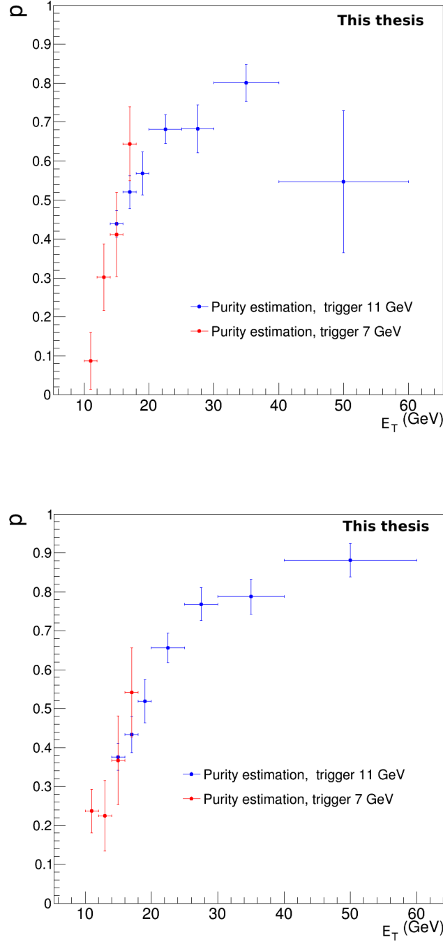
Figure 7.2: \mathbb{P} , purity obtained with the ABCD method and the isolation on charged and neutral particles LHC13d and LHC13e data (top plot) and using LHC13f events (bottom plot). In red: results obtained with the EG2 trigger. In blue: results obtained with the EG1 trigger.
