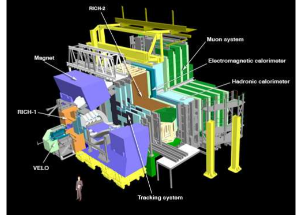
Figure 3.4: On the left: photograph of the LHCb detector. CERN©. On the right: detailed view of the LHCb experiment and its sub-detectors.
