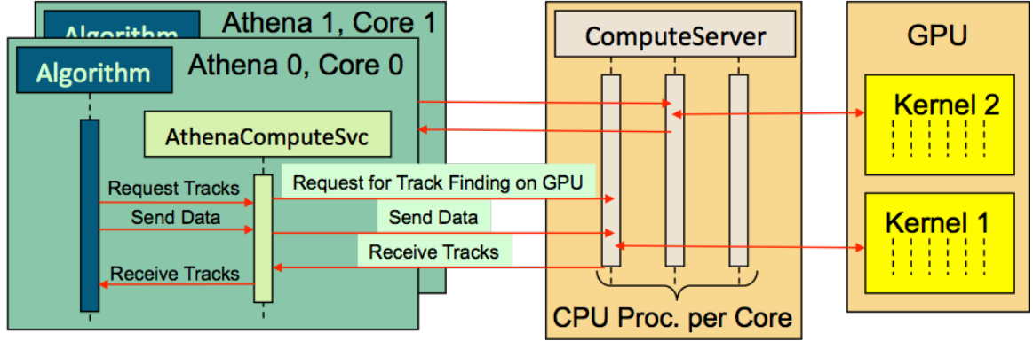
Figure 5.5: Client server architecture for GPU resource sharing [65].
