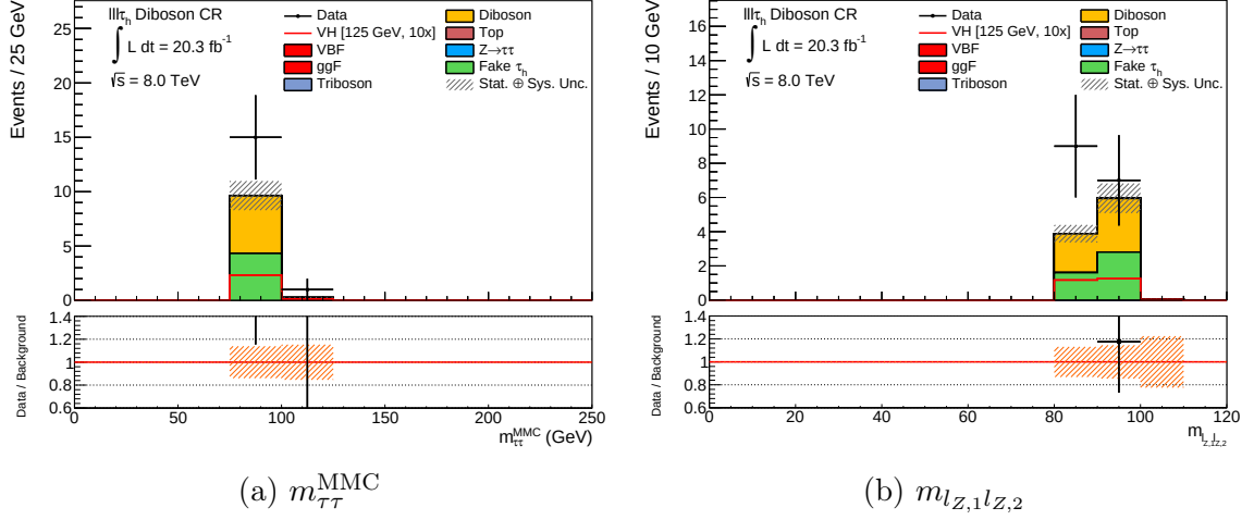
Figure 7.5: The (a) m_{\tau\tau}^{\text{MMC}} and (b) m_{l_{Z,1}l_{Z,2}} distributions in the Z_l H \rightarrow \tau_l \tau_h diboson control region.
