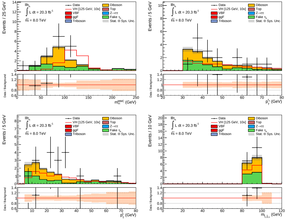
Figure 6.8: Various distributions in the signal region of the Z_l H \rightarrow \tau_l \tau_h analysis with 20.3 \text{ fb}^{-1} of 8 TeV data. These plots are constructed using pre-fit background estimation.
