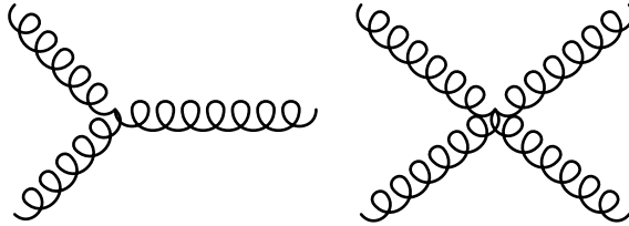
Figure 2.8: Three and four gluon QCD vertices.
