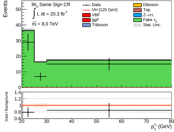
Figure 8.2: p_T^{\tau_h} distributions in the same-sign control region of the Z_{ll}H \rightarrow \tau_l \tau_h analysis with 20.3 \text{ fb}^{-1} of 8 TeV data.
