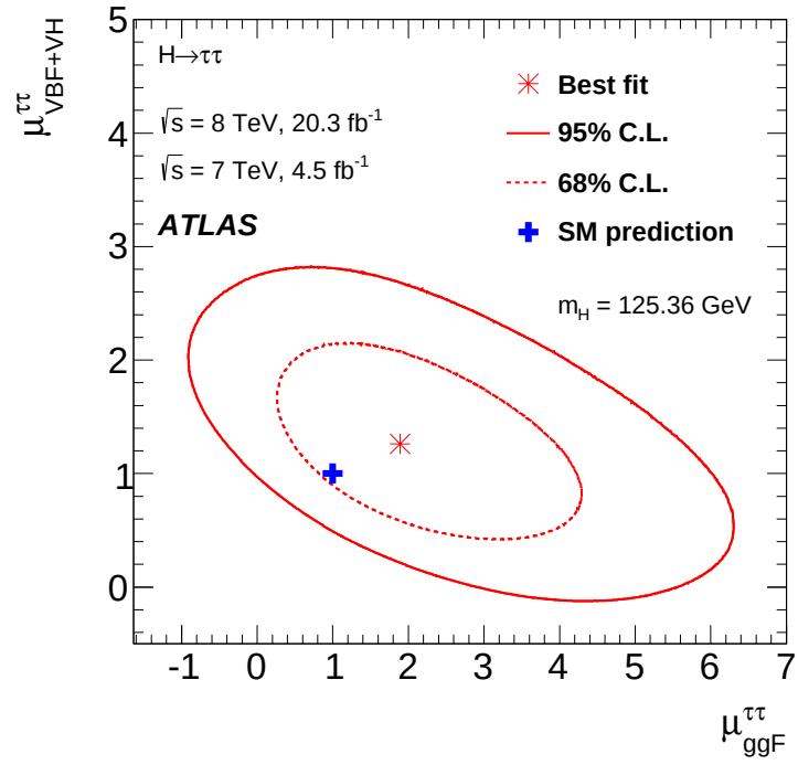
Figure 9.3: The best-fit value of the signal strength parameter in the (\mu_{\text{ggF}}^{\tau\tau}, \mu_{\text{VBF+VH}}^{\tau\tau}) plane, with likelihood contours shown at the 68% (dashed) and 95% (solid) confidence levels and the Standard Model expectation indicated by the blue cross at (1, 1) [76].
