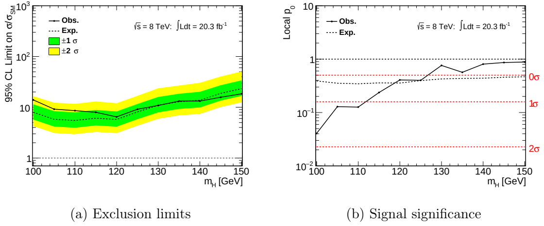
Figure 9.6: The results of the Z_u H \rightarrow \tau_l \tau_h analysis with 20.3 fb -1 of 8 TeV data as a function of hypothetical Higgs boson mass. Figure (a) shows expected and observed limits on Z_u H \rightarrow \tau_l \tau_h signal strength at the 95% confidence level using the CL s method. Figure (b) shows expected and observed significance of deviations from the background-only hypothesis.
