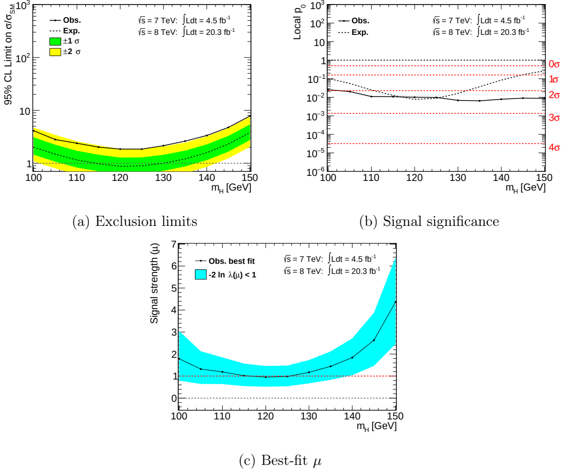
Figure 9.2: The results of the H \rightarrow \tau_l \tau_h analysis with 4.5 \text{ fb}^{-1} of 7 TeV data and 20.3 \text{ fb}^{-1} of 8 TeV data as a function of hypothetical Higgs boson mass. Figure (a) shows expected and observed limits on H \rightarrow \tau_l \tau_h signal strength at the 95% confidence level using the CL_s method. Figure (b) shows expected and observed significance of deviations from the background-only hypothesis. Figure (c) shows the best-fit value of the signal strength parameter \mu given the observed data.
