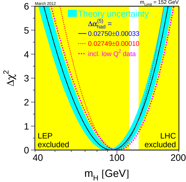
Figure 2.6: Best-fit values for the Higgs boson mass with experimental exclusions indicated [30].
