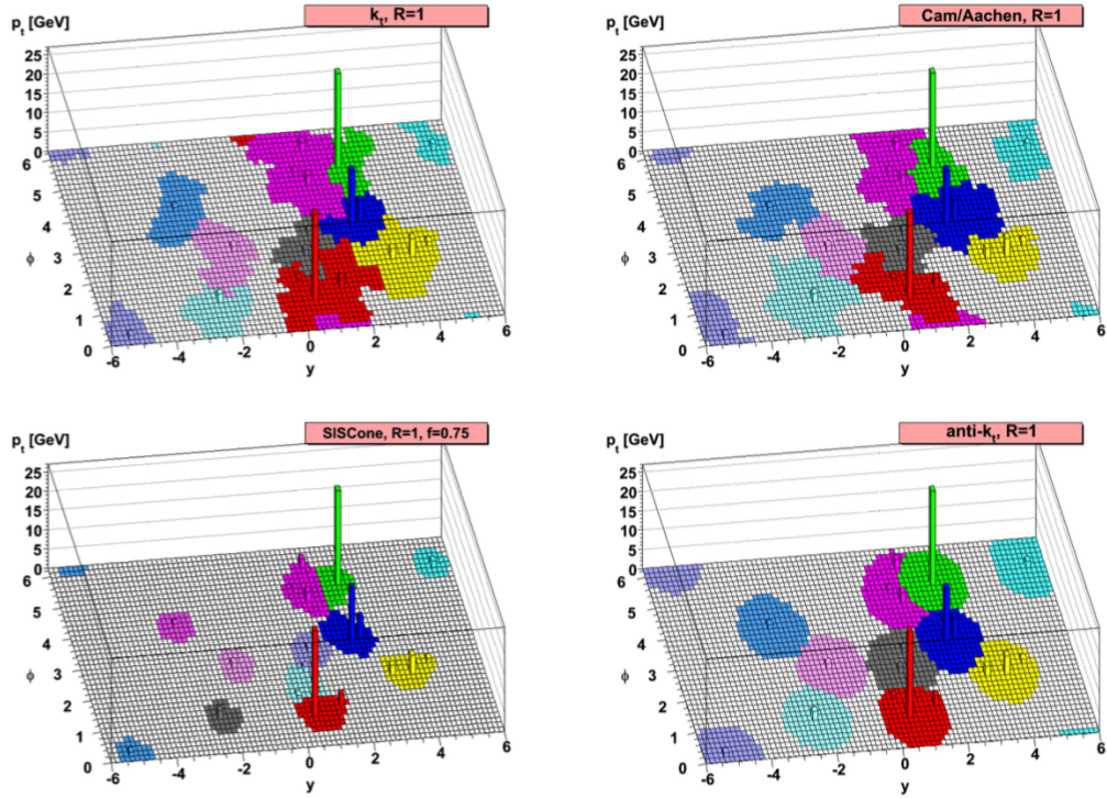
Figure 6.4: Four examples of jet reconstruction on a parton-level event generated with \sim 10^4 random soft particles. The k_T and C/A algorithms show dependency on the distribution of the soft particles. The anti- k_T algorithm is less influenced by soft radiation and produces uniformly shaped jets.
