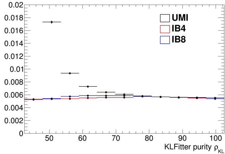
Figure 11.3: The statistical uncertainty on A^{\text{ss}} as measured in the nominal t\bar{t} MC scaled to an integrated luminosity of 20.3 \text{ fb}^{-1} , when using the UMI, IB4 and IB8 unfolding techniques. The uncertainty is found as a function of the KL Fitter purity \rho_{\text{KL}} . All three unfolding techniques converge in statistical uncertainty around \rho_{\text{KL}} = 80\% .
