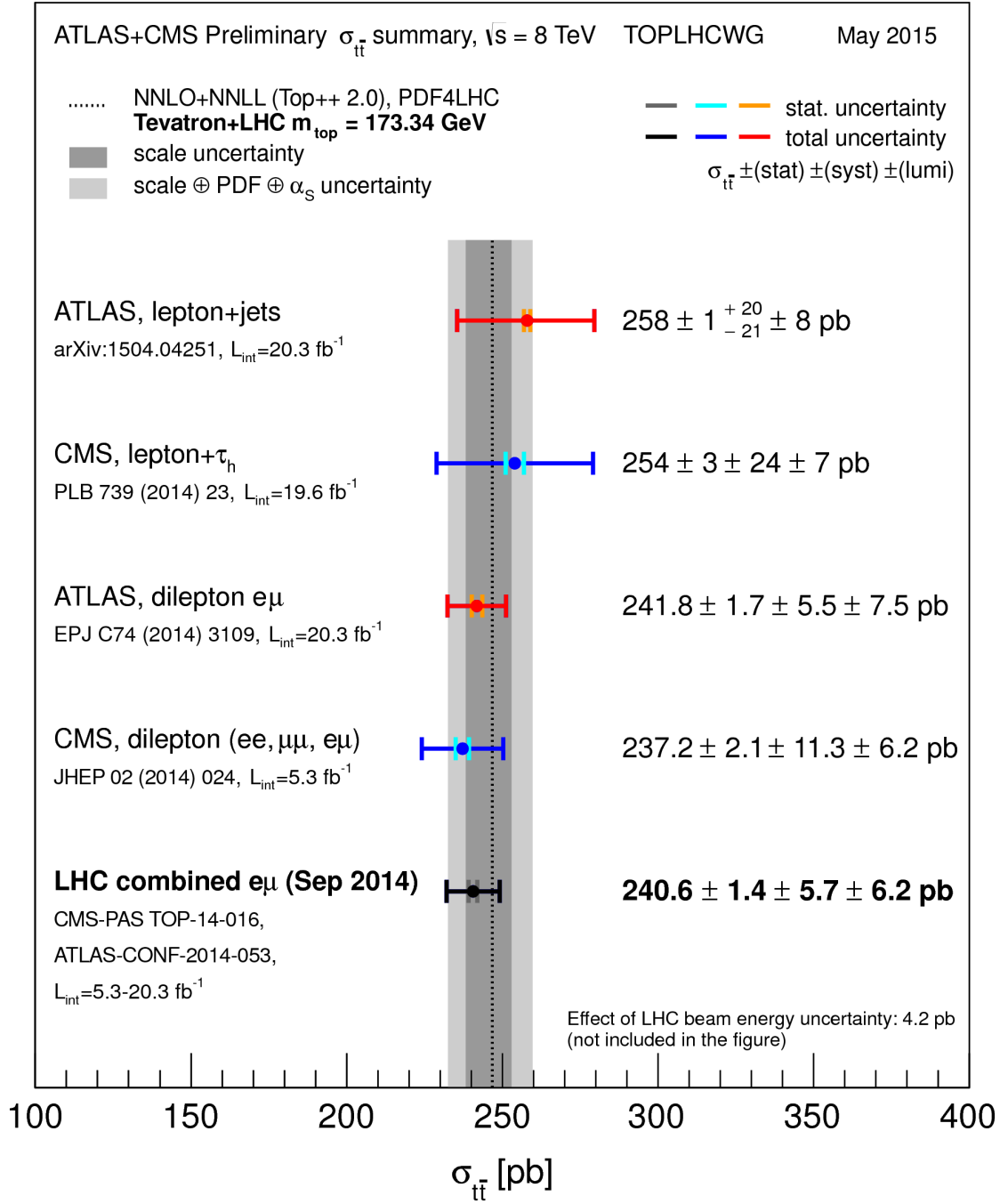
Figure 3.6: Summary of the top-quark pair production cross-section measurements on ATLAS and CMS at 8 TeV in the \ell +jets and dilepton channels, compared with an NNLO QCD calculation.
