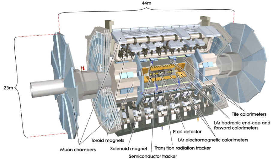
Figure 5.5: A cut-away diagram of the overall construction of the ATLAS detector, labelling the individual components.
