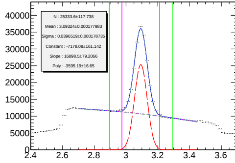
(a) Tag and Probe Invariant Mass.
