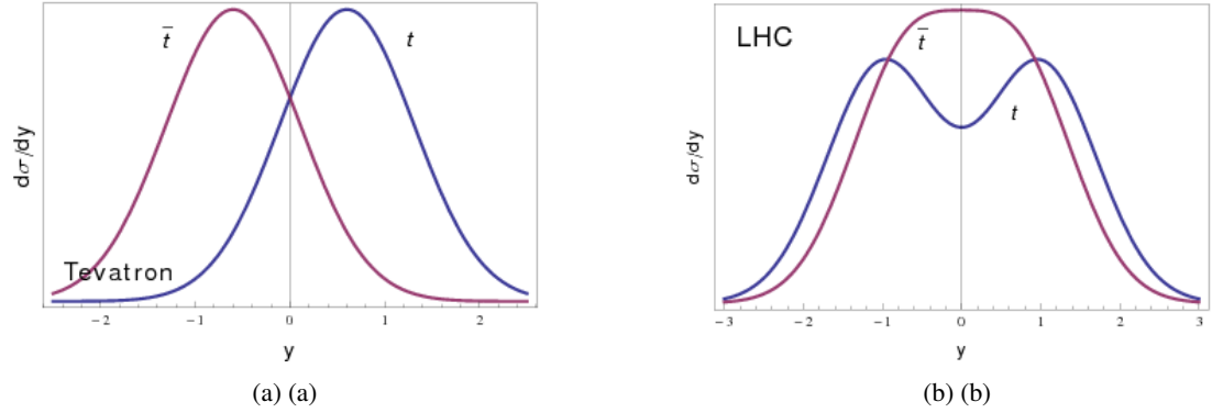
Figure 3.8: Rapidity distributions of top and anti-top quarks at (a) the Tevatron showing a forward-backward asymmetry, and (b) the LHC showing a charge asymmetry.
