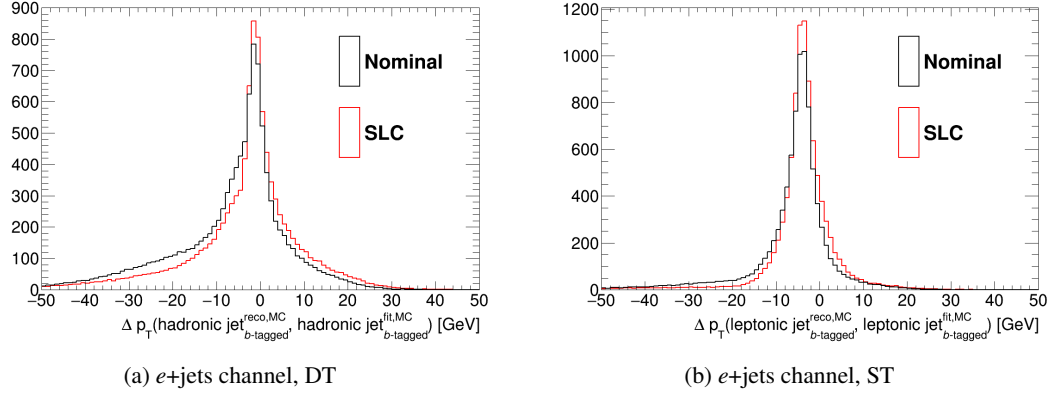
Figure 10.7: Difference between reconstructed jet p_T (with and without SLC correction) and fitted jet p_T returned by the KLFilter. The shift of the mean towards zero in the SLC corrections indicates a less strenuous fit performed, and leads to a higher permutation likelihood. Shown in the e +jets channel, the \mu +jets distribution is analogous
