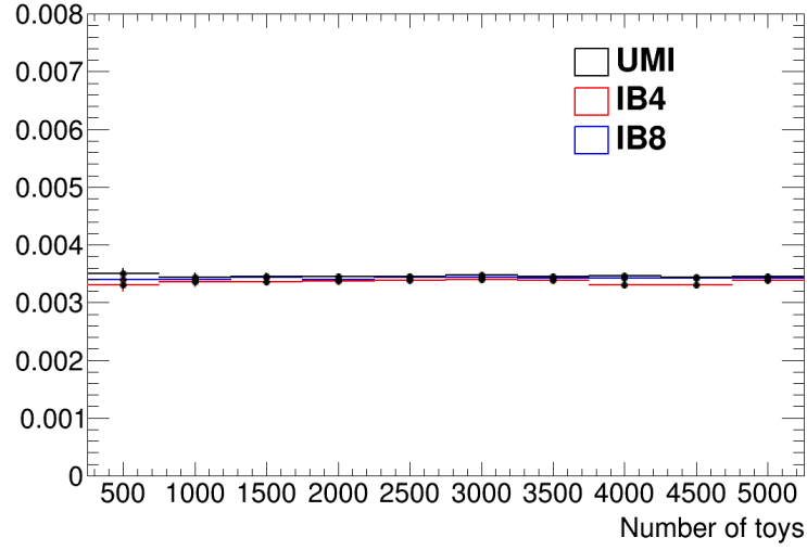
Figure 11.2: The statistical uncertainty on A^{\text{os}} as measured in the nominal t\bar{t} MC scaled to an integrated luminosity of 20.3 \text{ fb}^{-1} , when using the UMI, IB4 and IB8 unfolding techniques. The uncertainty is found to be stable and similar for each.
