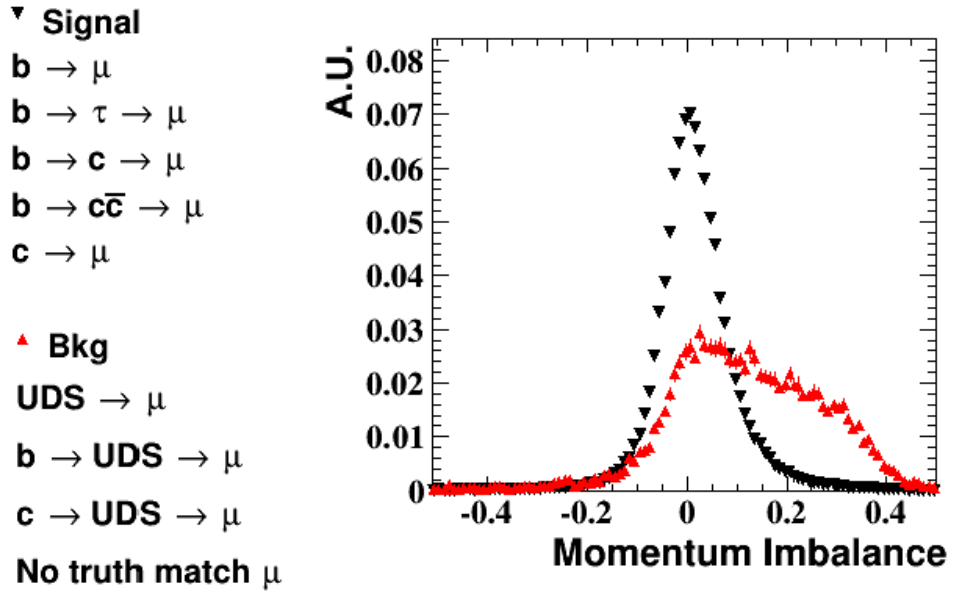
Figure 6.6: The momentum imbalance distribution of ‘signal’ soft muons, and ‘fakes’ from the decay of non- b -hadrons comprised of u -, d - or s -quarks (‘UDS’), using t\bar{t} MC. The area under each distribution has been normalised to unity.
