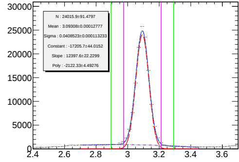
(b) Tag and MuonProbe Invariant Mass.
