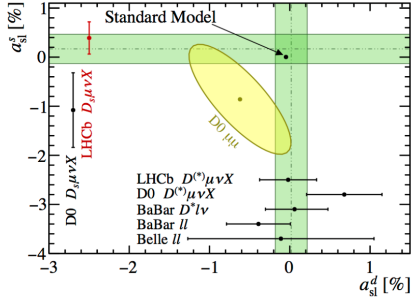
Figure 4.2: Overview of measurements of a_{sl}^d and a_{sl}^s (flavour-dependent CP violation asymmetries in neutral B -meson mixing). The black dot represents the SM expectation value, the yellow ellipse represents interpretation of the D0 dimuon observation, and the green bands represent naive averages of previous measurements.
