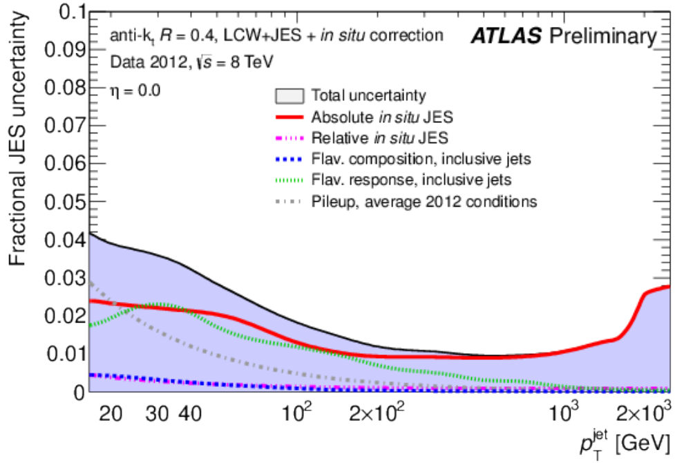
Figure 9.4: The fractional systematic uncertainty components as a function of p_T on the JES for jets with |\eta| = 0.0 . The total uncertainty (all components summed in quadrature) is shown as a filled blue region topped by a solid black line.
