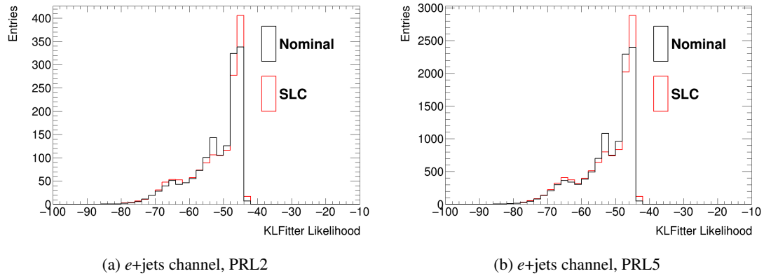
Figure 10.8: Log likelihood distributions for the best permutation in each event as decided by the KLFilter, overlayed for events before and after the jet SLC corrections, for the PRL2 and PRL5 decay channels. The improvement in likelihood leads to a better performance of the KLFilter. Shown in the e +jets channel, the \mu +jets distribution is analogous
