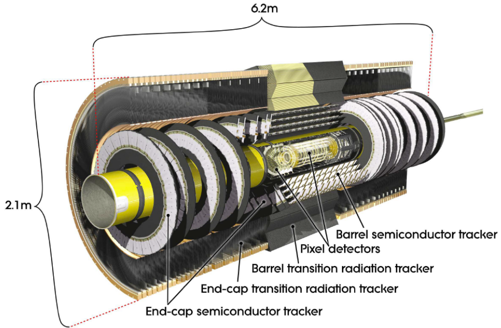
Figure 5.7: A cut-away diagram of the overall construction of the ATLAS inner detector, labelling the individual components.
