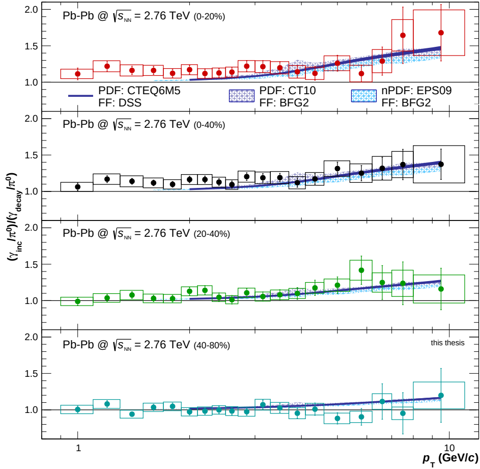
Figure C.2: Direct-photon excess ratios R_\gamma for Pb–Pb at 2.76 TeV in the centrality bins 0-20%, 0-40%, 20-40% and 40-80%. Additionally, three scaled NLO pQCD calculations are shown. They are identical to the calculations shown in Fig. 10.2. Instead of fits to the \pi^0 spectra the spectra are used directly. The figure corresponds to Fig. 10.2.
