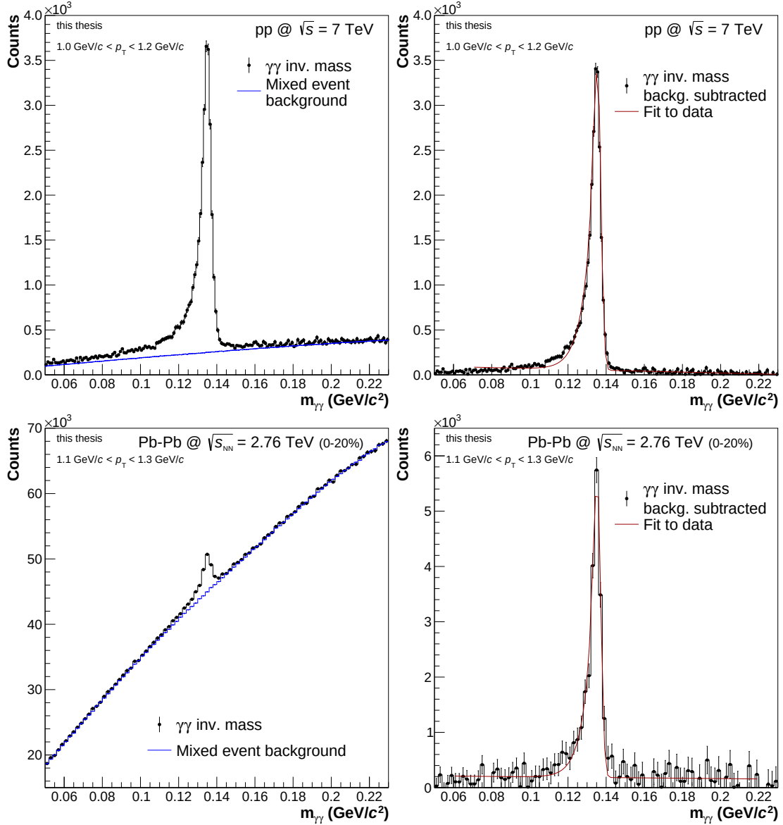
Figure 8.1: \pi^0 peaks without and with combinatorial background for pp at 7 TeV and central (0-20%) Pb-Pb collisions. For both examples a p_T bin slightly above 1.0 \text{GeV}/c is shown. In addition, a fit (Eq. (8.2)) to the peak is plotted. Due to the much higher photon multiplicity, the combinatorial background is magnitudes larger in Pb-Pb.
