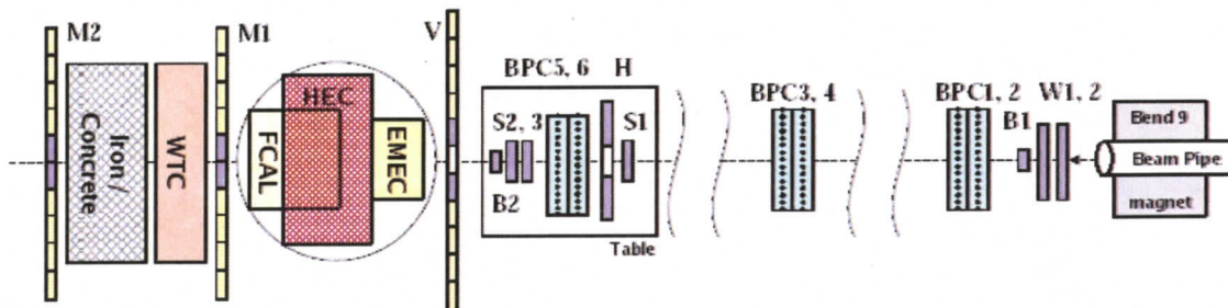
Figure 3.1: Layout of the testbeam setup as viewed from above. Beams of particles emerge from the end of the H6 beam pipe on the right and travel toward the left. The particles pass through various beam monitoring detectors before impacting the LAr calorimeter modules (EMEC, HEC, and FCAL) in the H6 cryostat. Any particles that emerge out the back of the calorimeters are detected with additional detectors: M1, M2, and the warm tail-catcher (WTC).
