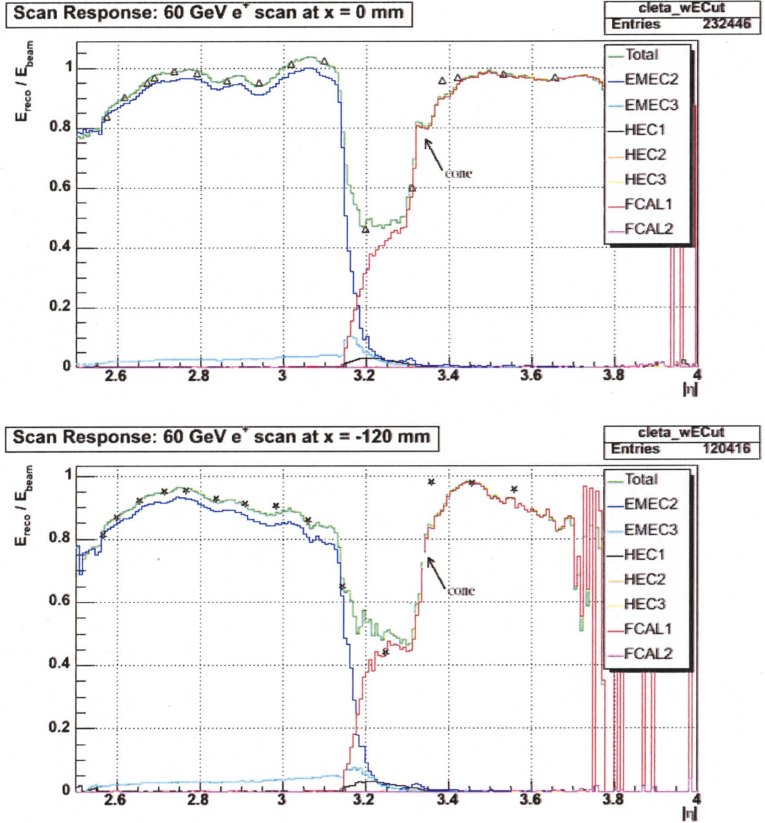
Figure 6.8: Calorimeter response to the 60 GeV positron y -scan at x = 0 mm (top) and the 60 GeV positron y -scan at x = -120 mm (bottom) as a function of mean cluster pseudorapidity. The total cluster energy is shown (green), along with the cluster energy in each sampling layer. The data points are the energy response at the impact points.
