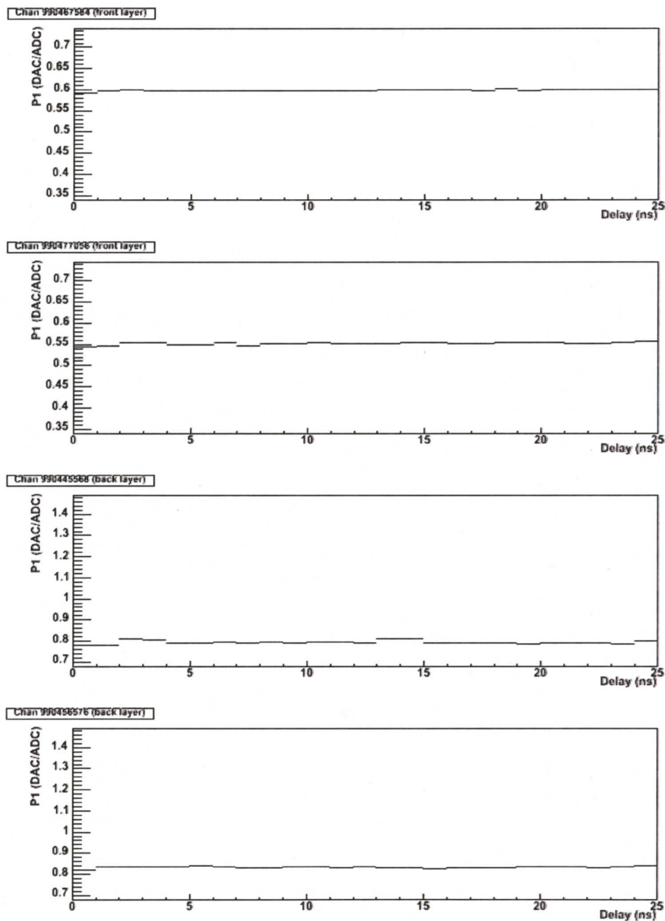
Figure 5.7: Linear ramp coefficient ( P1 ) obtained from the calibration pulse shape method, plotted as a function of delay for four typical EMEC channels. The top (bottom) two plots are for channels in the front (back) layer of the EMEC.
