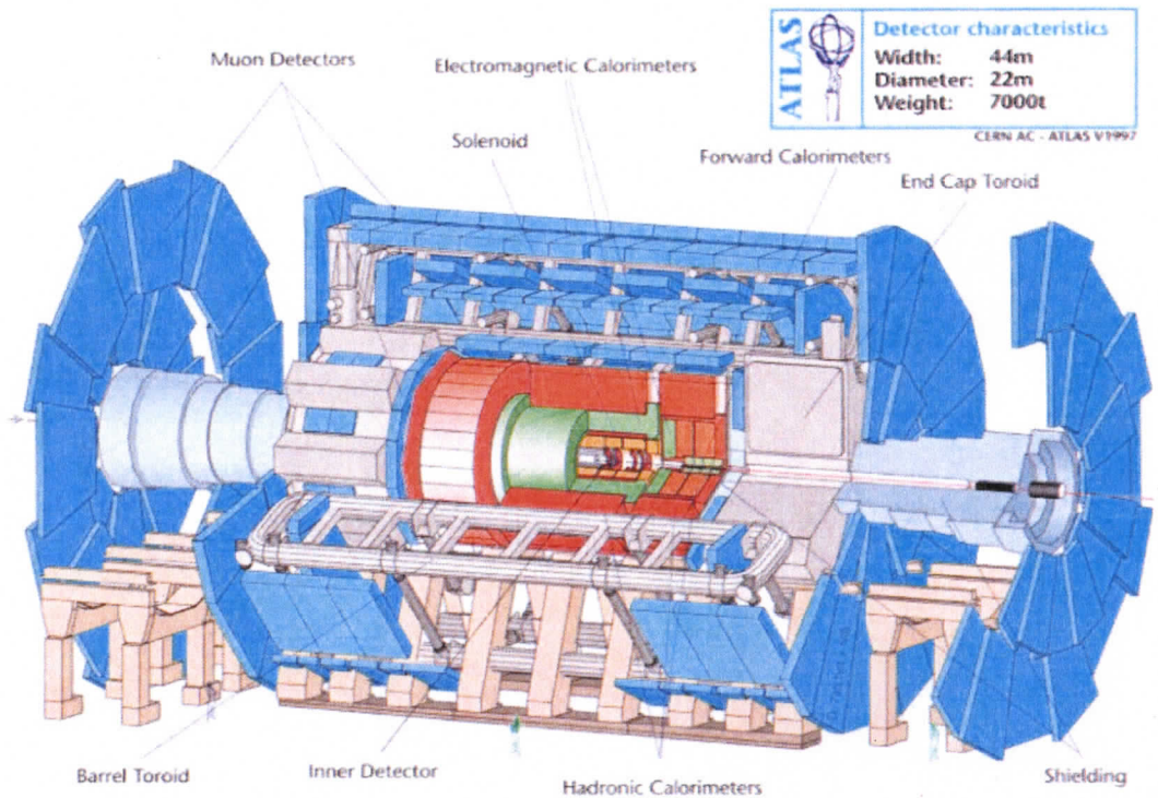
Figure 1.2: The ATLAS detector is a cylindrical apparatus which surrounds the LHC beam pipe, and is comprised of several detector systems. The muon detection system is shown in blue; the electromagnetic and hadronic calorimeters are shown in orange and green, respectively; the inner tracker is yellow. The central solenoid, along with the barrel and end-cap toroids, provide the magnetic fields used to bend the trajectories of charged particles to provide momentum measurement.
