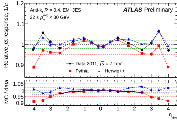
(b) Response correction as a function of \eta_{\text{det}} for 22 < p_T^{\text{avg}} < 30 GeV
