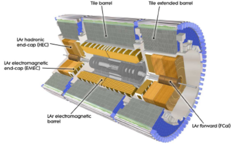
Figure 2.6: An overview of the ATLAS calorimeters [66]
