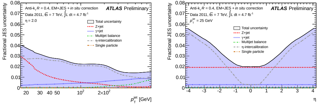
(a) Individual in-situ components for \eta = 2.0 (b) Individual in-situ components for p_T = 25 GeV
