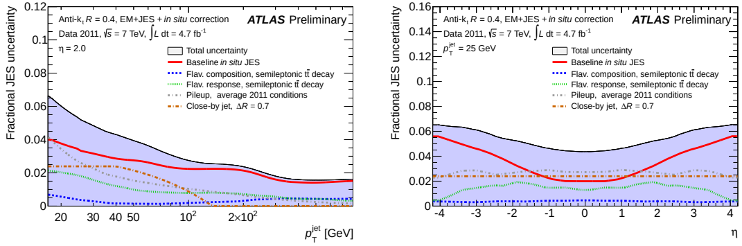
(c) Total JES for \eta = 2.0
