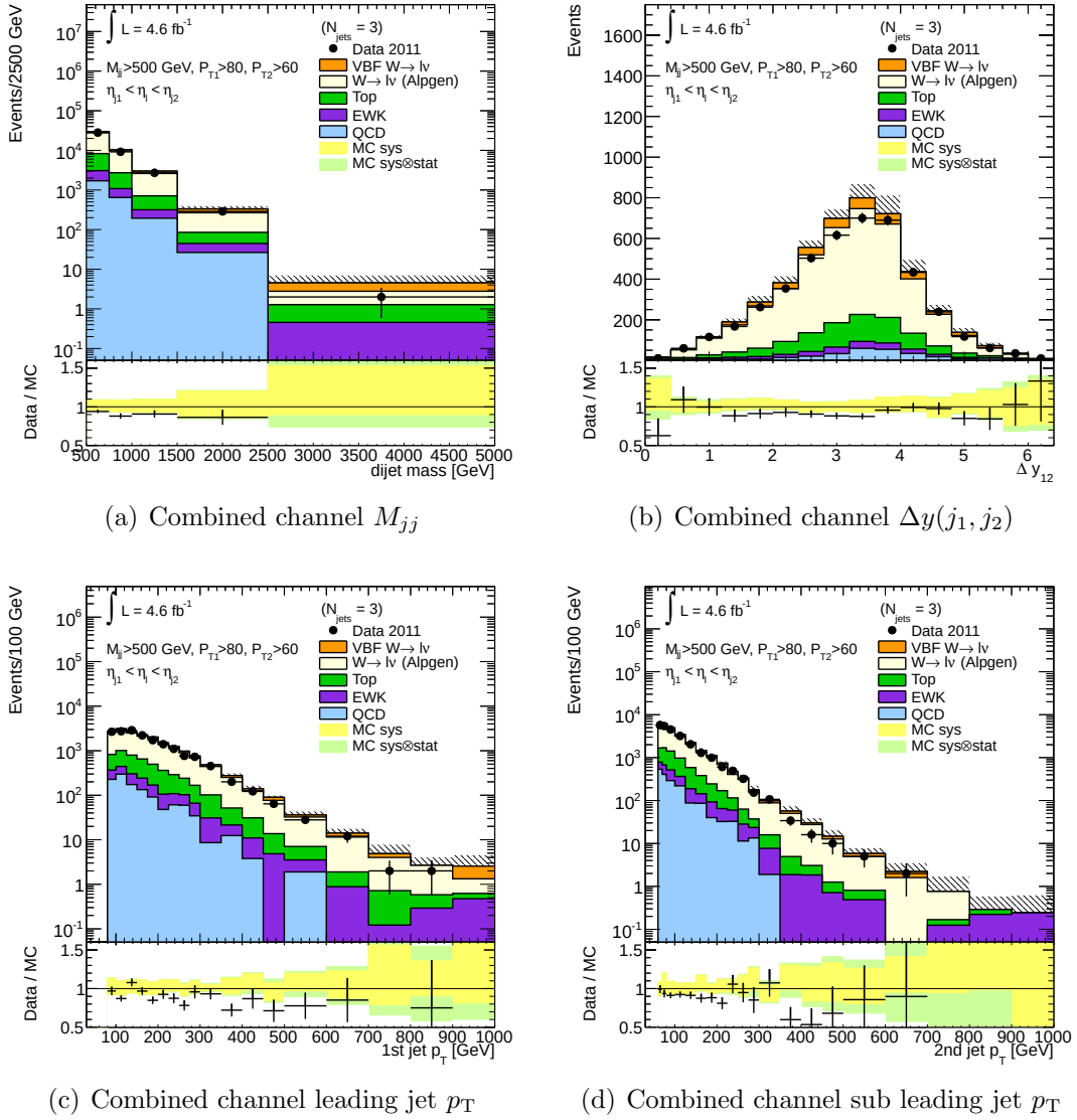
Figure 6.19: Validation region plots in the combined electron and muon channels. The W + \text{EWK} jets and W + \text{QCD} jets have been scaled by the signal strength values extracted in the signal region.
