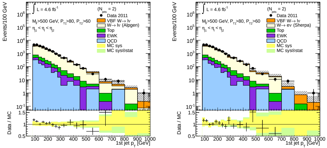
(e) Combined Leading jet p_T (ALPGEN W + \text{QCD jets} ) (f) Combined Leading jet p_T (SHERPA W + \text{QCD jets} )
