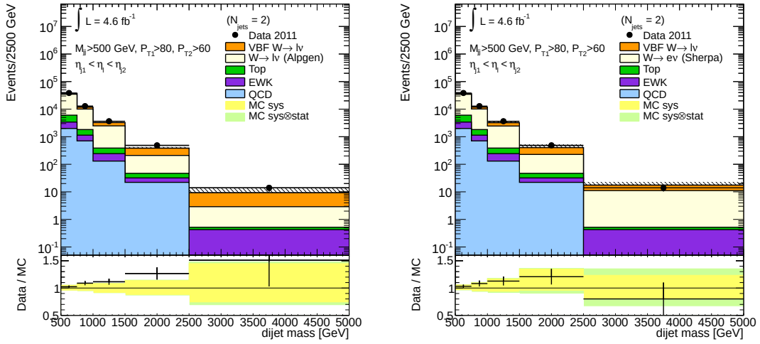
(a) Combined M_{jj} (ALPGEN W + \text{QCD jets} ) (b) Combined M_{jj} (SHERPA W + \text{QCD jets} )
