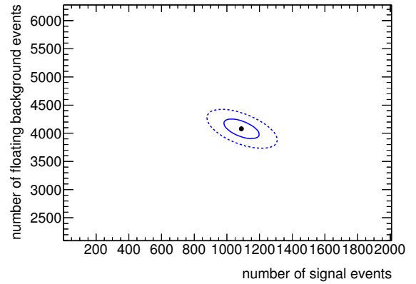
(b) Contour plot of errors in N_S and N_W
