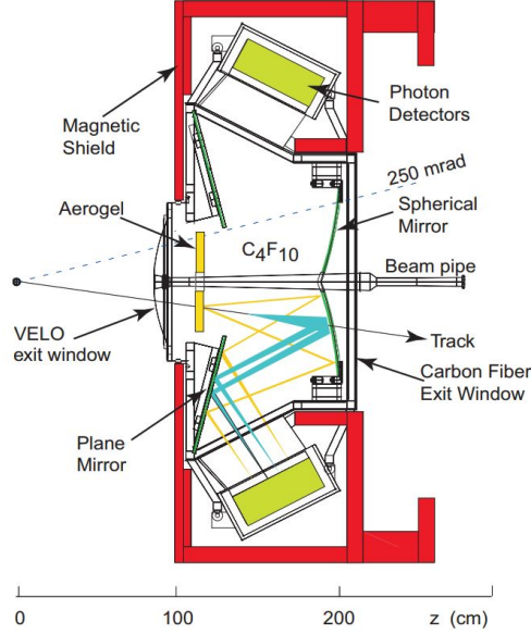
Figure 3.14: Side view of the RICH1 sub-detector [71].
