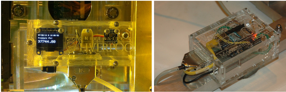
Figure 3.22: Left: upper half of the monitoring device containing the atmospheric sensors and the LCD currently displaying the pressure reading; right: lower half of the monitoring device containing the Arduino micro-controller board, the accelerometer and the power and network connections. The two are connected via a custom-made cable.
