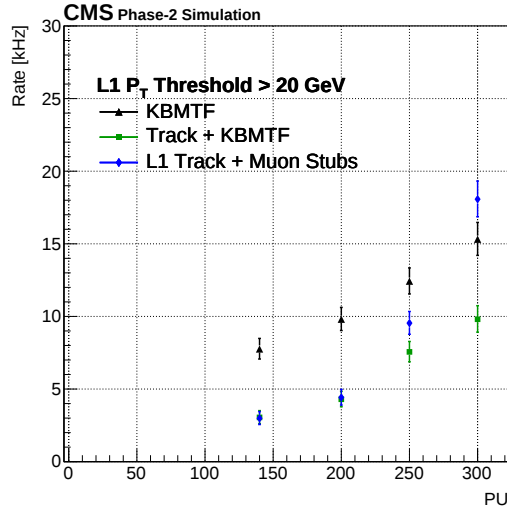
(c) Single muon rates vs pileup for a 20 GeV threshold.
