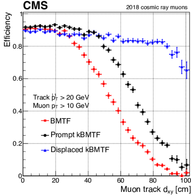
Figure 4.9: Comparison of efficiency vs cosmic track d_{xy} using cosmic data from the 2018 data taking run. The prompt KBMTF takes the reconstructed p_T using the vertex constrained measurement, while the displaced KBMTF uses the vertex unconstrained measurement. The displaced KBMTF shows substantial improvements to the previous BMTF [93].
