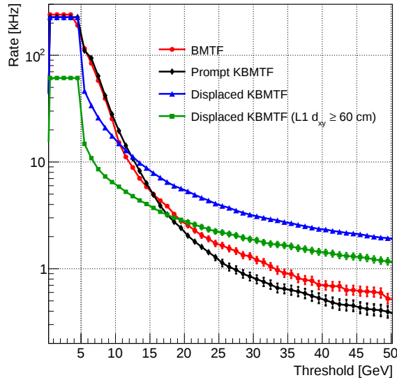
Figure 4.10: Rate comparison calculated using 2017 zero bias data of the Phase I BMTF, vertex constrained (prompt) KBMTF, vertex unconstrained (displaced) KBMTF, and displaced KBMTF for displaced tracks.
