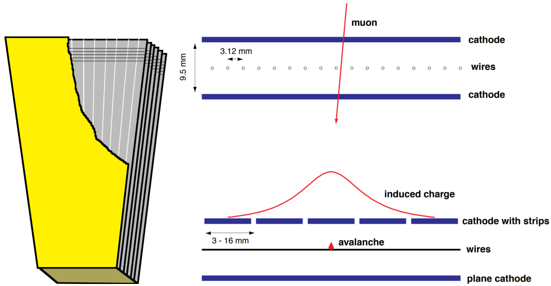
Figure 3.12: Cut-away diagram of a single CSC module showing the six layers of radial cathode strips and transverse anode wires (left). Muons ionize the gas chamber, causing an avalanche of electrons on the anode wires and inducing a charge on the cathode strips (right) [80].
