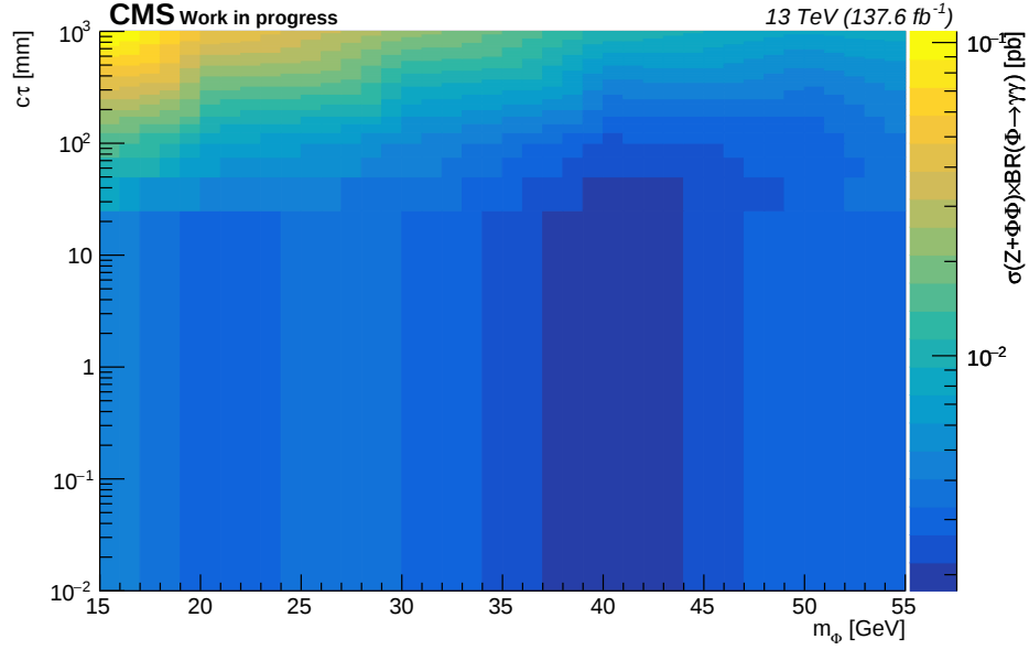
Figure 5.43: Observed model independent limits on \sigma(Z + \Phi\Phi) \times \mathcal{BR}(\Phi \rightarrow \gamma\gamma) as a function of m_\Phi and c\tau under the assumption that \mathcal{BR}(\Phi \rightarrow \gamma\gamma) = 0.5 .
