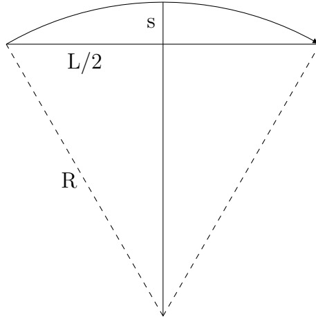
Figure 3.5: Diagram showing the sagitta for a charged particle track
