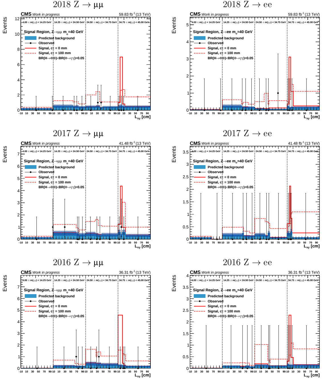
Figure 5.37: Observed number of m_\phi = 40 GeV events in the signal region of the Z \rightarrow \mu\mu category (left) and the Z \rightarrow ee category (right) across all three years.
