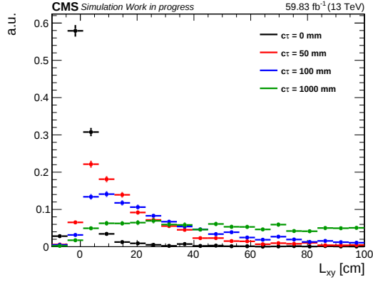
(a) L_{xy} distribution calculated for m_\Phi = 30 GeV, Z \rightarrow \ell\ell signal samples
