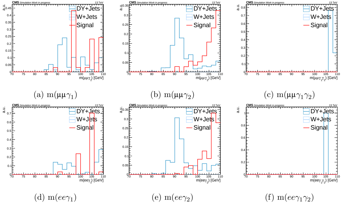
Figure 5.17: Comparison of invariant mass distributions for FSR rejection using simulated m_\Phi = 20 GeV, c\tau = 0 mm signal and background. Background uses normalized anti-ID control region events for improved statistics while signal shows ID signal region events.
