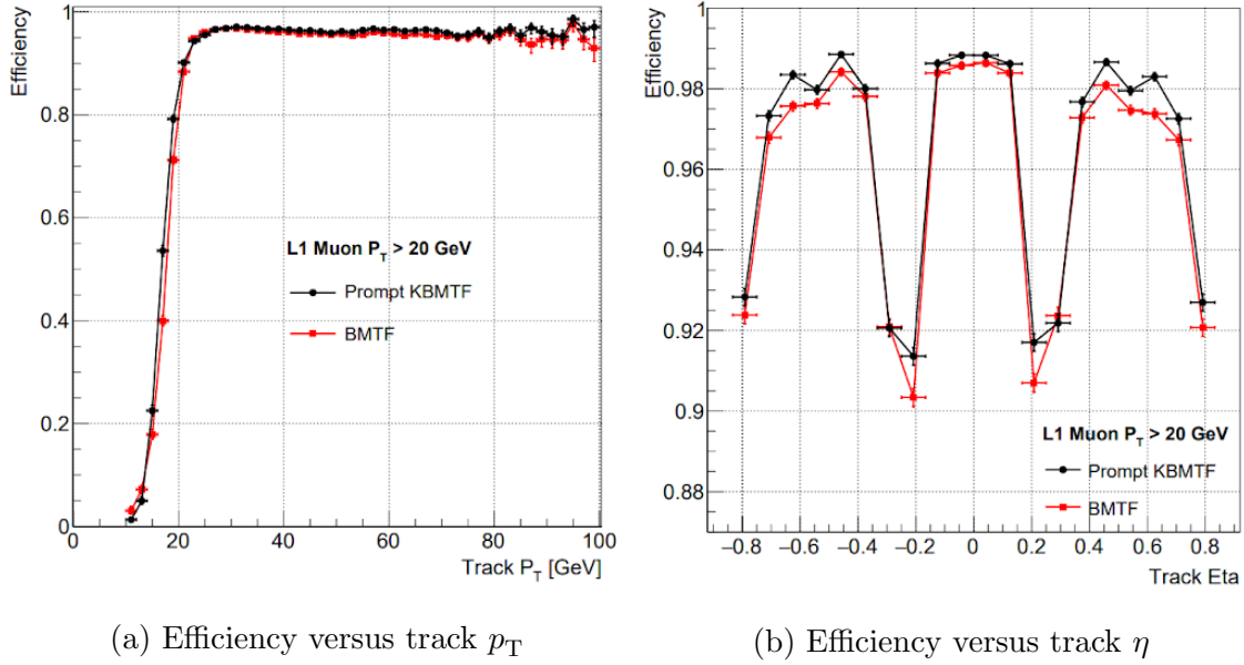
Figure 4.8: Comparison of efficiencies between the KBMTF and phase-1 BMTF algorithm using a Z tag-and-probe sample collected during 2017 data taking. (a) Efficiency versus track p_T , requiring L1 muon p_T > 20 GeV. (b) Efficiency versus track \eta , requiring level-1 muon p_T > 20 GeV and track p_T > 25 GeV in order to show the efficiency on the plateau. The drops in efficiency at \eta = \pm 0.2 are due to gaps between wheels in the muon system.
