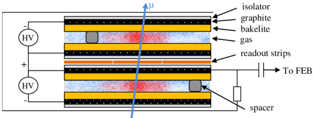
Figure 3.13: Diagram of the double RPC at CMS. Incident muons ionize the gas, causing a cascade of electrons towards the readout strips [81].
