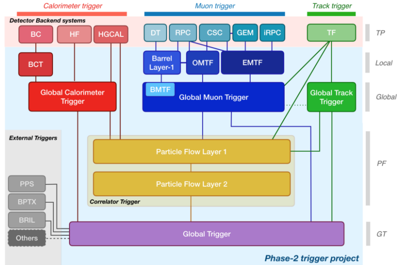
Figure 3.15: Designed trigger architecture of the HL-LHC. The addition of the track primitives allows the computation of more advanced reconstruction algorithms at the L1 level [83].
