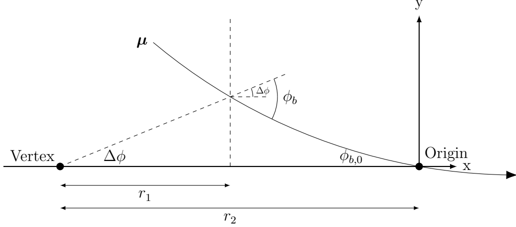
Figure 4.2: Diagram showing a muon trajectory between two stations with the origin set at the outer station. The x-axis is oriented using the detector vertex and the outer station.
