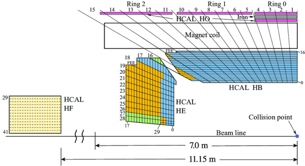
Figure 3.9: r - z slice of the CMS HCAL showing the HB, HE, HF, and HO [77].
