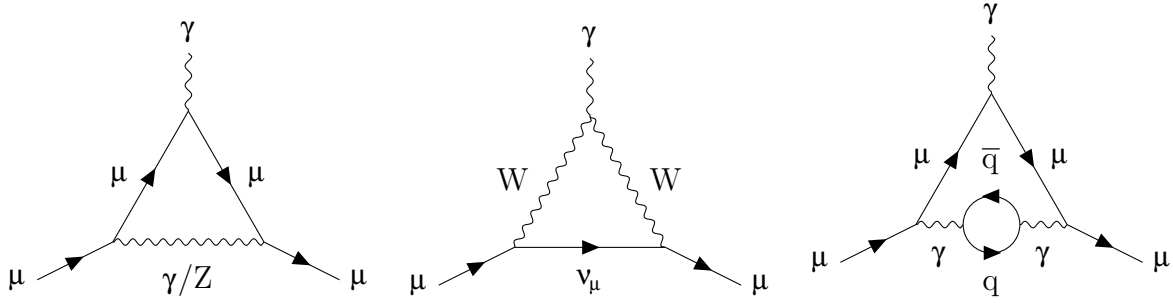
Figure 2.2: First-order QED and lowest-order weak/hadronic contributions to the muon anomalous magnetic moment.
