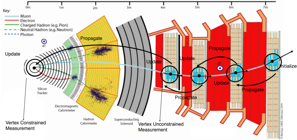
Figure 4.1: The iterative process of propagation and updating a muon track through the KBMTF algorithm. The track properties at the innermost station are stored in order to trigger on muons not originating from the beam axis [68].
