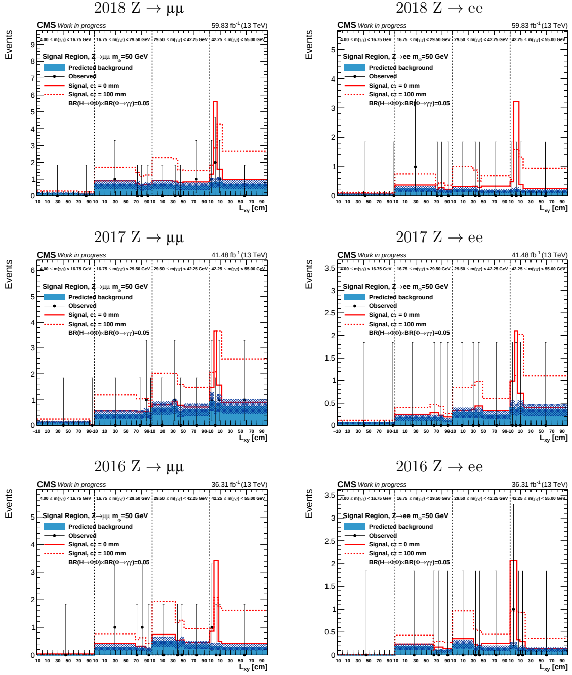
Figure 5.38: Observed number of m_\phi = 50 GeV events in the signal region of the Z \rightarrow \mu\mu category (left) and the Z \rightarrow ee category (right) across all three years.
