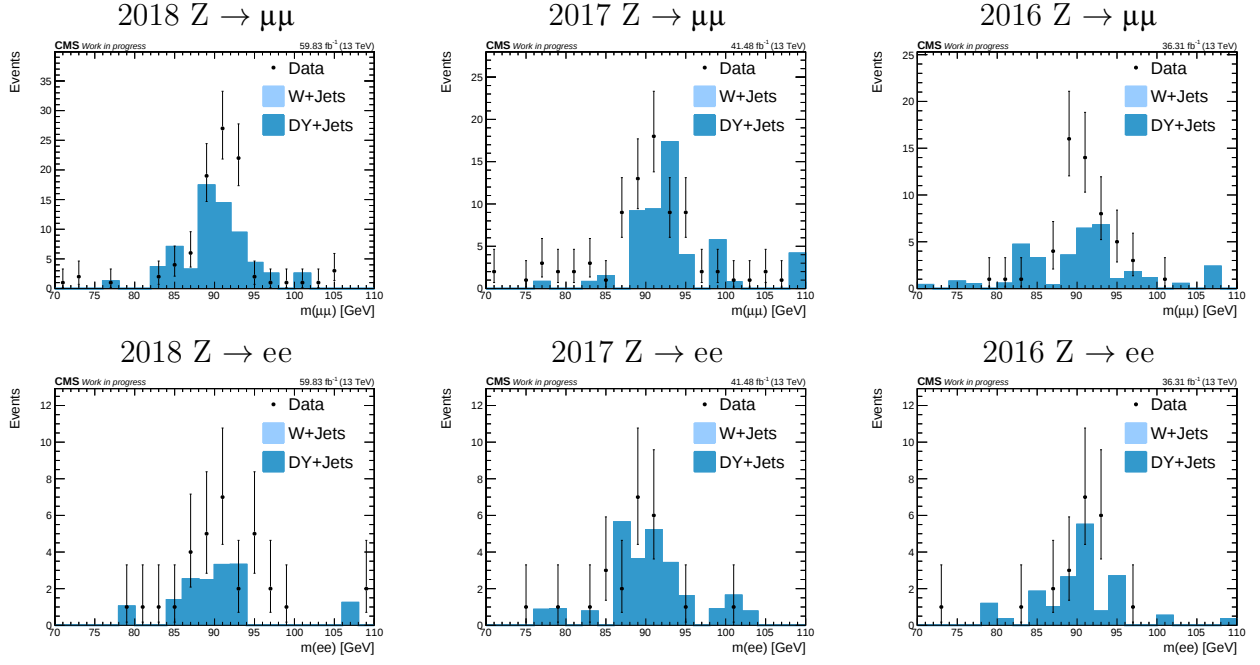
Figure 5.19: m(\ell^+\ell^-) data and simulated background after rejecting FSR events across all years in the ID signal region. Top row: Z \rightarrow \mu\mu category. Bottom row: Z \rightarrow ee category
