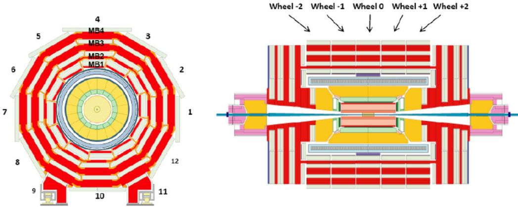
Figure 4.6: Diagram of the CMS muon barrel system [89]. (Left) \hat{r} - \hat{\phi} slice showing the wheel segmented in 12 sectors in \phi and four detector stations in r . (Right) \hat{r} - \hat{z} slice showing the five wheels in z .
