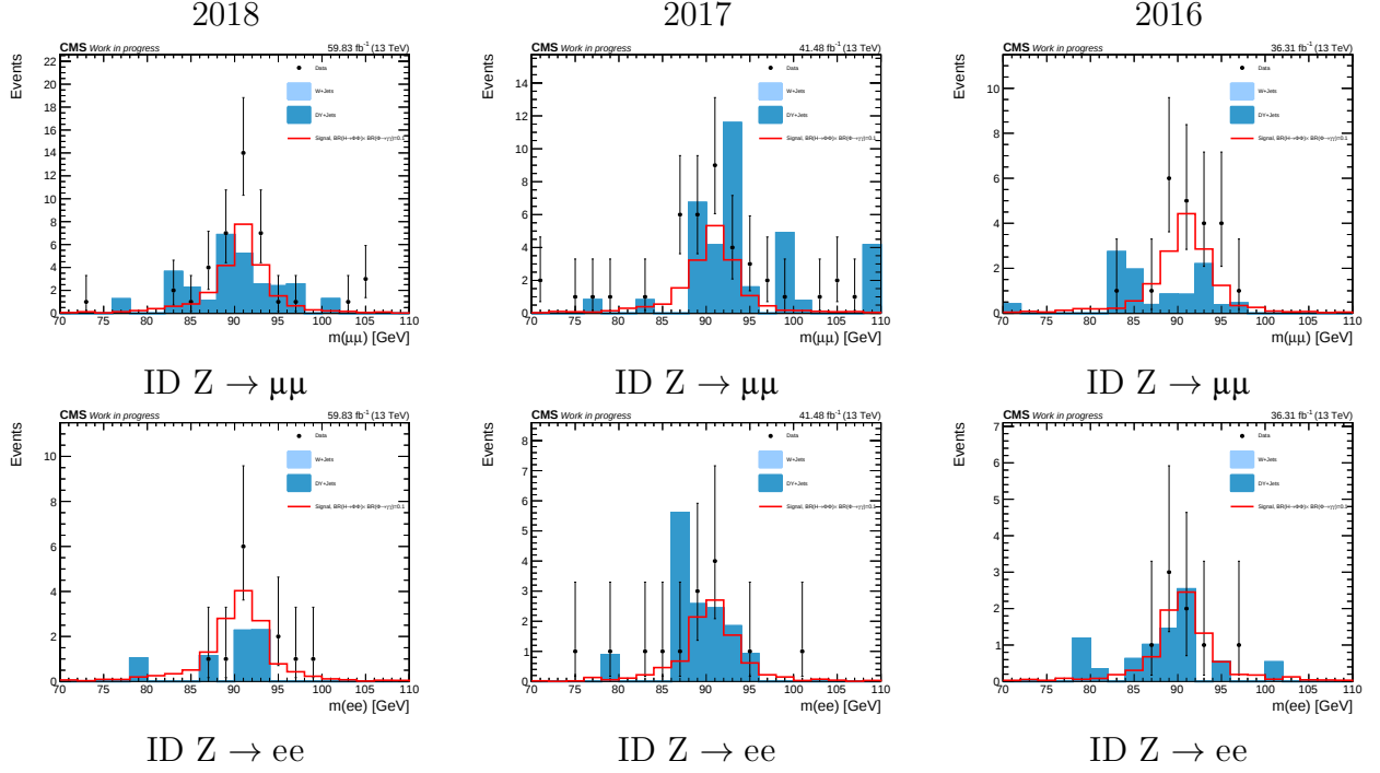
Figure 5.22: Final m(\ell^+\ell^-) distributions for data and simulated samples in the ID signal region. Top row: Z \rightarrow \mu\mu category. Bottom row: Z \rightarrow ee category.
