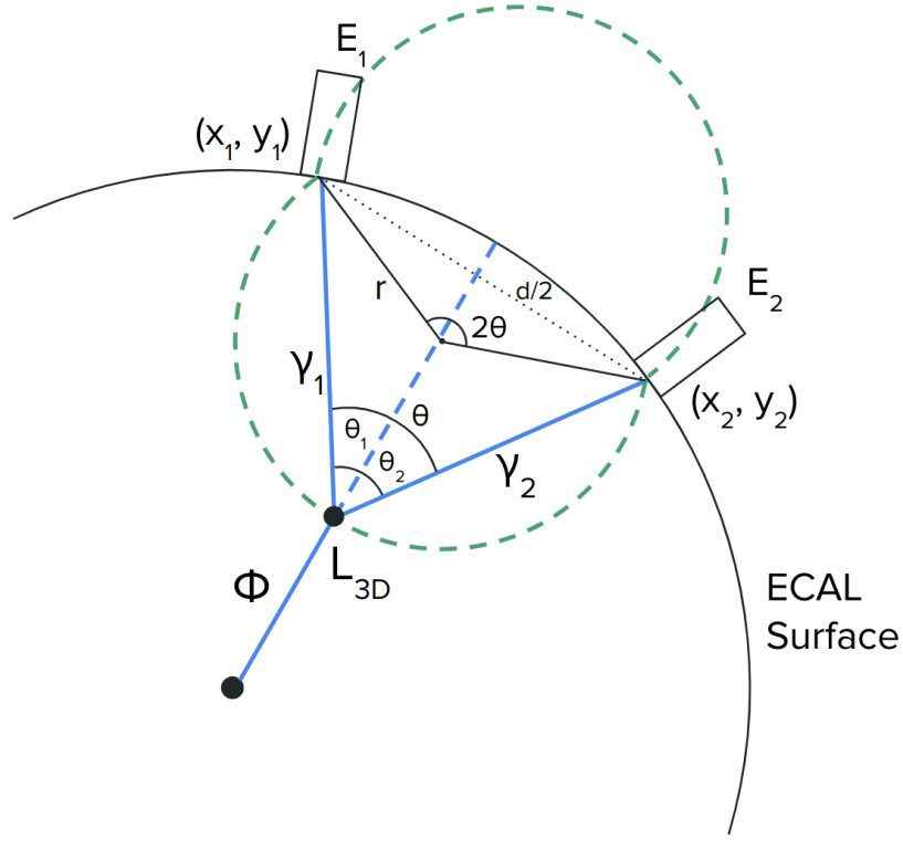
Figure 5.9: Geometrical configuration used to reconstruct the displaced vertex of the di-photon pair
