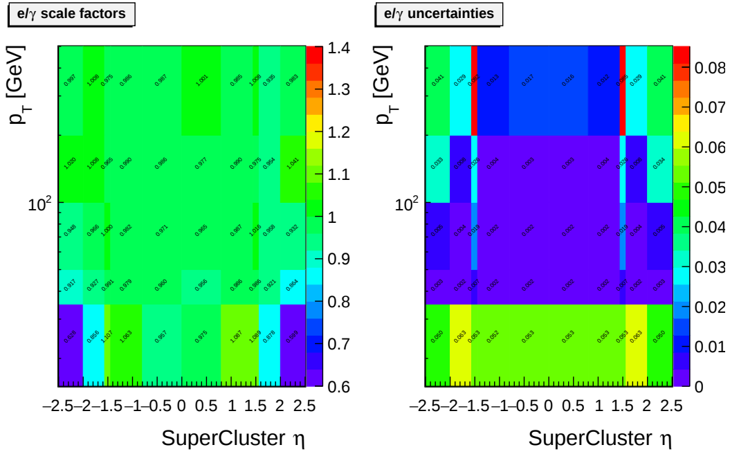
Figure 5.7: 2016 post-VFP electron HLT scale factors and uncertainties.
