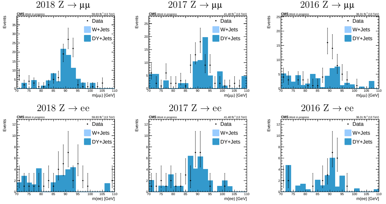
Figure 5.16: m(\ell^+\ell^-) data and simulated background after preselection criteria across all years in the ID signal region. Top row: Z \rightarrow \mu\mu category. Bottom row: Z \rightarrow ee category
