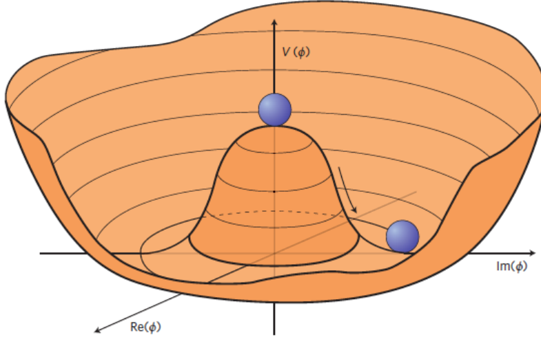
Figure A.1: The complex scalar potential for \lambda^2 > 0 and \mu^2 > 0 , showing an infinite number of minima away from 0 [117]. By inspection this potential possesses a global U(1) gauge invariance due to the rotational symmetry from adding a complex phase.
