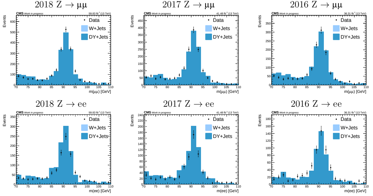
Figure 5.15: m(\ell^+\ell^-) data and simulated background after preselection criteria across all years in the anti-ID control region. Top row: Z \rightarrow \mu\mu category. Bottom row: Z \rightarrow ee category
