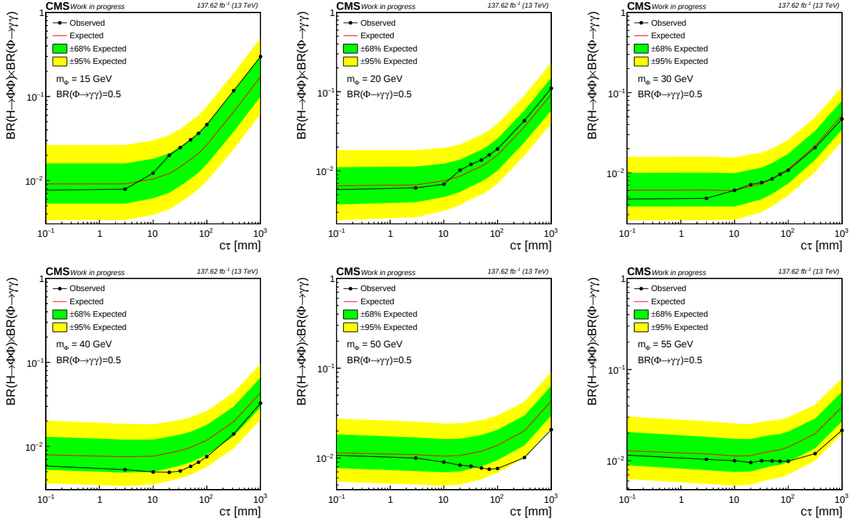
Figure 5.40: Model dependent upper limits for \mathcal{BR}(H \rightarrow \Phi\Phi) \times \mathcal{BR}(\Phi \rightarrow \gamma\gamma) for different values of m_\Phi and c\tau under the assumption that \mathcal{BR}(\Phi \rightarrow \gamma\gamma) = 0.5 .
