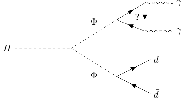
Figure 5.2: Feynman diagram showing the proposed decay channel of the Higgs boson to \Phi\Phi , with one \Phi decaying to a pair of photons and the other decaying to d\bar{d} . The loop in the diphoton decay can contain any particle that could theoretically couple to the \Phi . It is also possible for the \Phi to decay directly to photons.
