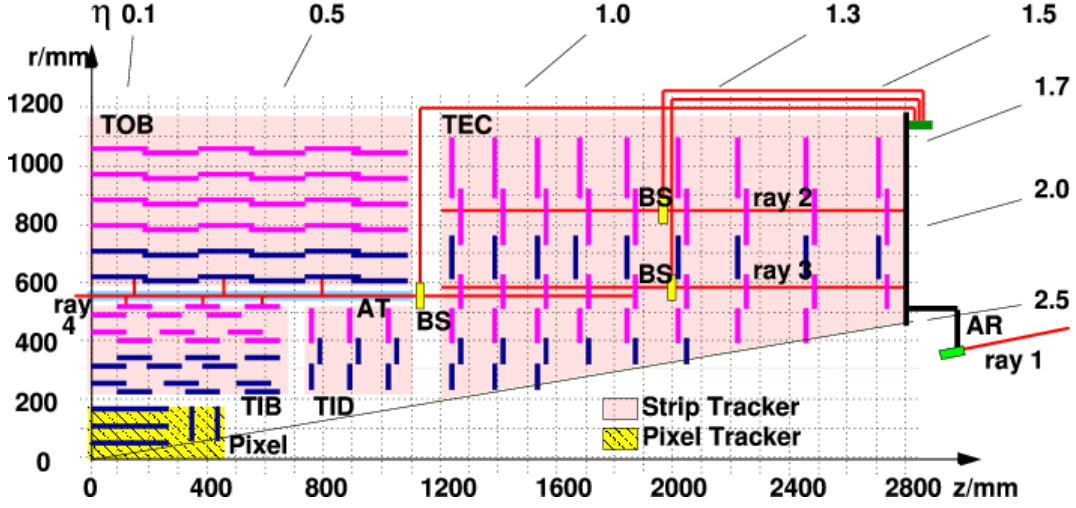
Figure 3.7: r - z slice of the CMS silicon detector, detailing the four main components (TIB, TOB, TID, and TEC) of the strip detector. Pixel detector is shown in its Run I configuration [73].
