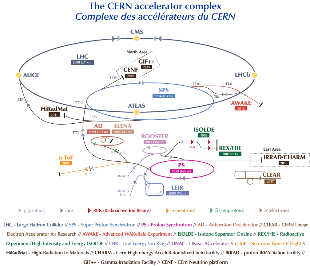
Figure 3.2: Diagram of the CERN accelerator complex during 2018 data taking [67]. Protons begin as hydrogen atoms at Linac2 and are accelerated in several stages to reach 6.5 TeV.
