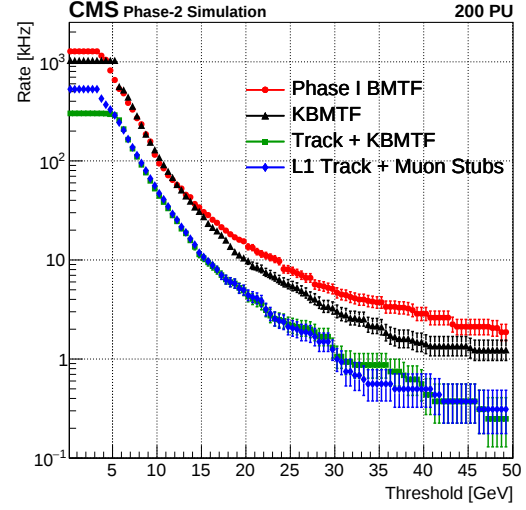
(b) Single muon rates versus threshold.
