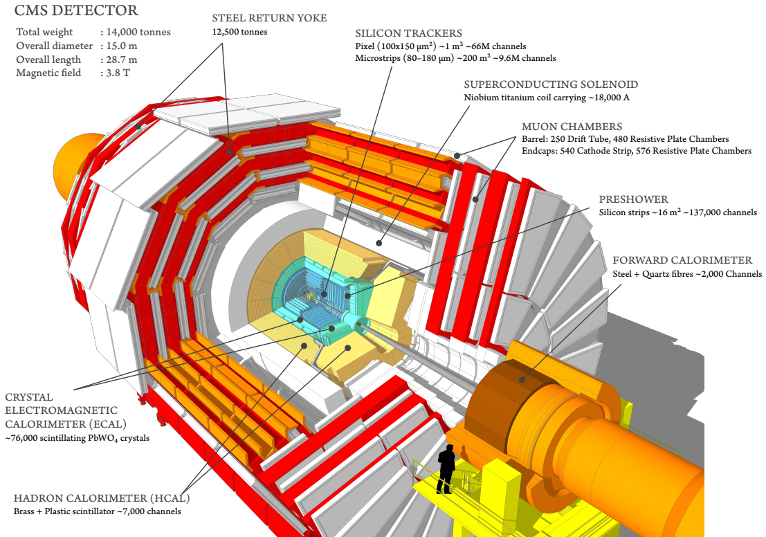
Figure 3.4: Cutaway diagram of CMS showcasing major detector components [70].
