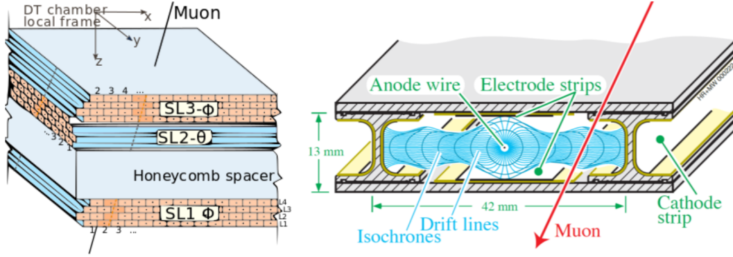
Figure 3.11: Drift tube superlayers are aligned in alternating orientations in order to provide a complete picture of muon trajectories (left). A cross section of a single drift tube chamber (right). Electrons ionized from the muon drift to the anode wire to produce a measurable current [79].
