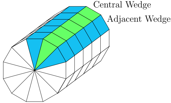
Figure 4.7: Diagram showing the inputs of one MP7 board, consisting of the TwinMux inputs from one central wedge (green) and the two adjacent wedges (blue). The KBMTF reconstructs all tracks with the outermost stub in the central wedge.
