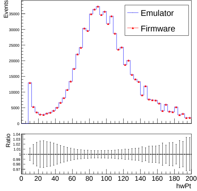
Figure 4.11: Comparison of the track p_T between the firmware and emulator using data from a 2017 Z tag-and-probe sample. hwPt represents the integer value of p_T used in hardware. The emulator and firmware output show 100% agreement across 500000 events.
