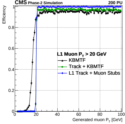
(a) Efficiency vs gen \mu p_T .
