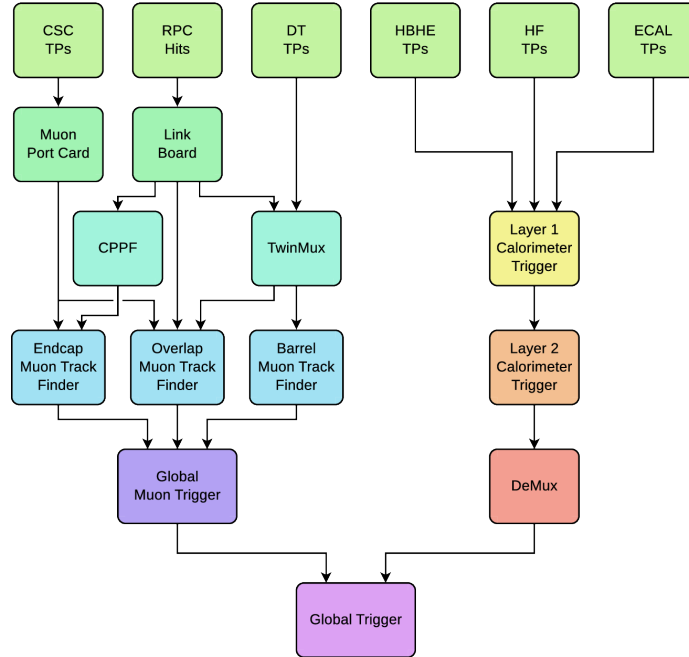
Figure 3.14: Block diagram of the CMS Level-1 Trigger architecture during Run 2 [82]. Muon objects found in the barrel, overlap, and endcap regions are ranked and sorted using their momentum and quality criteria before being passed to the Global Muon Trigger (GMT), which cleans duplicate tracks and selects the top eight muons. The muons are then passed to the global trigger, which combines the muons with objects created from the calorimeters and makes the final decision to pass the event to the HLT.
