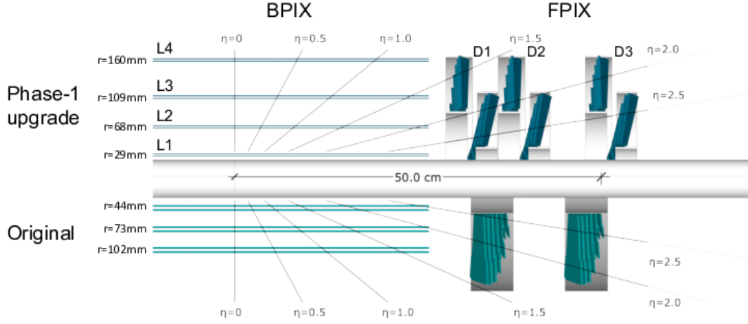
Figure 3.6: r - z slice of the CMS pixel detector comparing original design (bottom, teal) with the Phase-I upgrade implemented in 2016/17, which added one layer to both the FPIX and BPIX (top, blue) [72].
