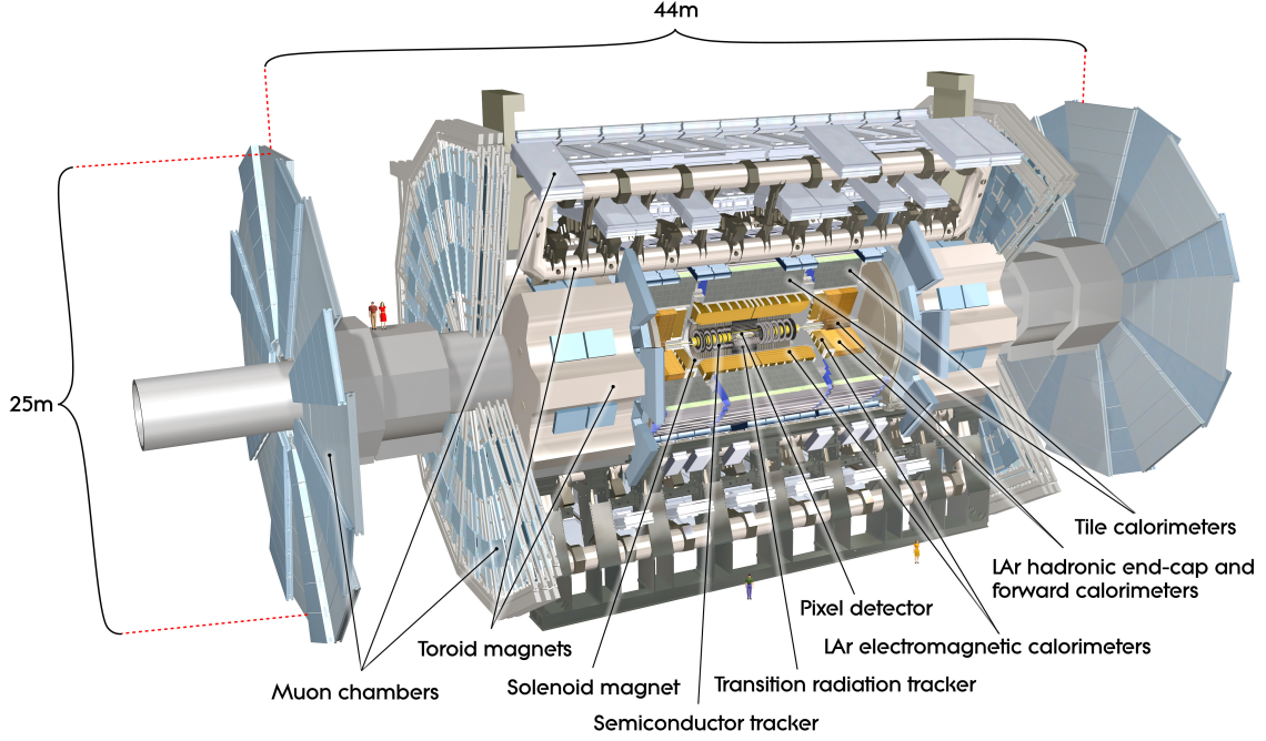
Figure 5: Schematic view of the ATLAS detector where the main detector components are labeled. Figure from the ATLAS experiment official website in [29].
