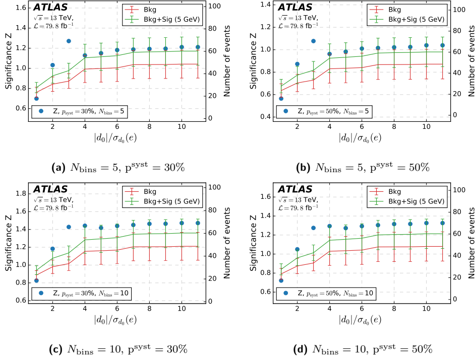
Figure 81: Signal sample with M_N = 5 GeV. Optimization study for the variable |d_0|/\sigma(d_0)(e) . The plots show the significance and number of events as a function of the cut on the variable |d_0|/\sigma(d_0)(e) for which the x-axis value x_0 represents the requirement |d_0|/\sigma(d_0)(e) < x_0 .
