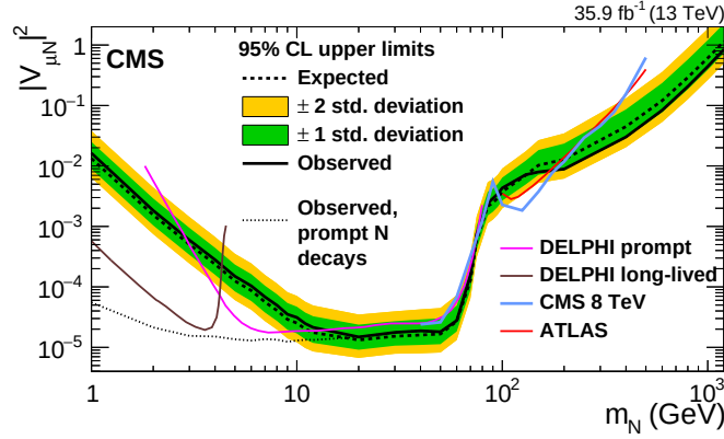
Figure 45: The exclusion region at 95% confidence level (CL) in the |V_{\mu N}|^2 vs M_N plane from the HNL search by the CMS collaboration [22] with 35.9 \text{ fb}^{-1} at \sqrt{s} = 13 \text{ TeV} . The best upper limits at 95% CL from the searches in DELPHI [19], ATLAS [20] at \sqrt{s} = 8 \text{ TeV} ; and CMS [21] at \sqrt{s} = 8 \text{ TeV} . The figure is from [22].
