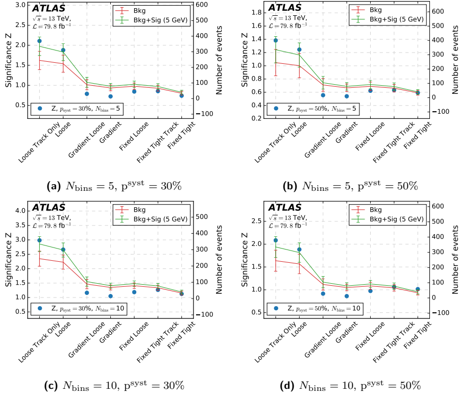
Figure 69: Signal sample with M_N = 5 GeV. Optimization study for the isolation selection of \mu_2 . The plots show the significance and number of background and signal events as a function of the isolation selection of \mu_2 .
