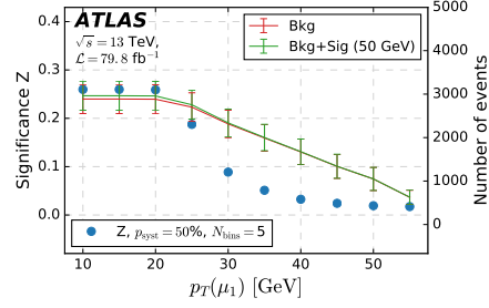
(b) M_N = 50 GeV. Binning variable M(\mu_1, \mu_2, e) .
