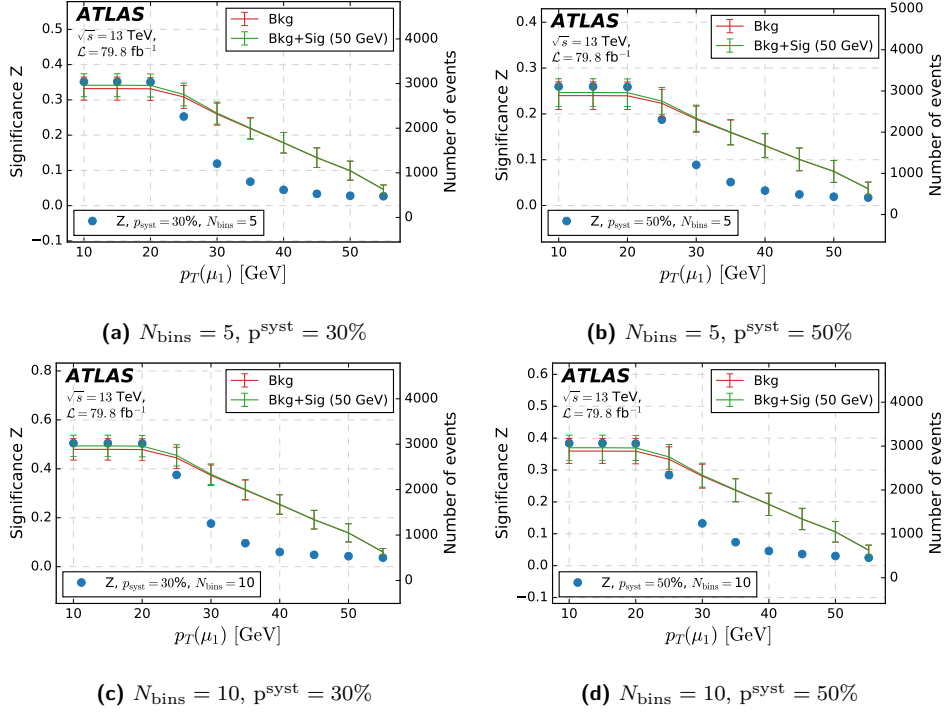
Figure 53: Signal sample with M_N = 50 GeV. Optimization study for the variable p_T(\mu_1) . The plots show the significance and number of background and signal events as a function of the cut on p_T(\mu_1) for which the x-axis value x_0 represents the requirement p_T(\mu_1) \geq x_0 GeV.
