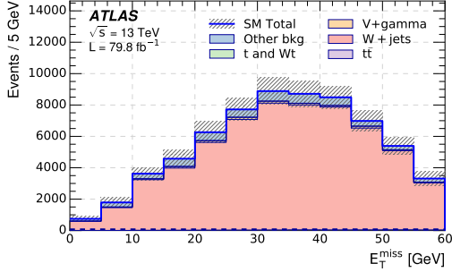
(c) Electron MR with N_{b\text{-jets}} = 0 .
