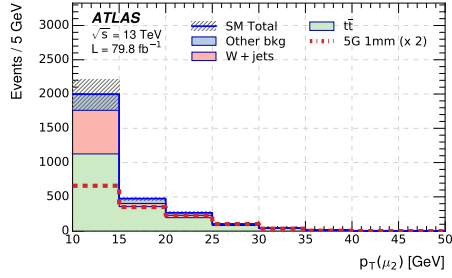
(e) Signal region, p_T(\mu_2) distribution. Signal with M_N = 5 GeV.
