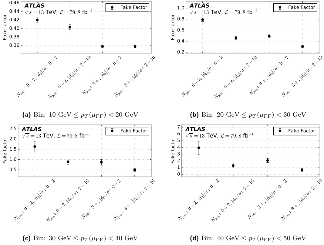
Figure 33: The final muon fake factor binning. The ID and anti-ID criteria are defined using the FixedCutLoose isolation in the muon measurement region with N_{\text{b-jets}} = 0 .
