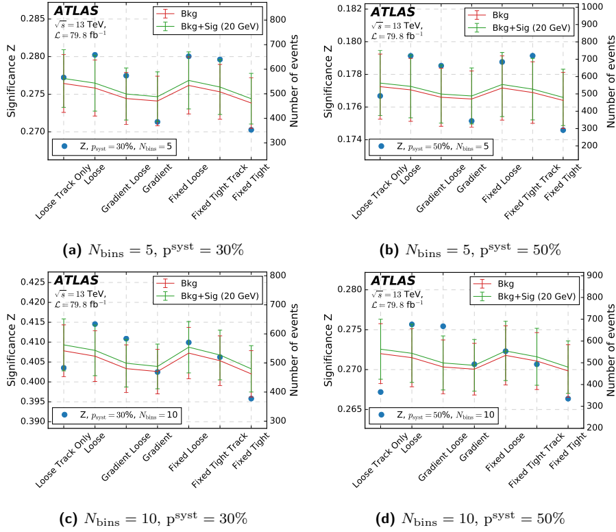
Figure 64: Signal sample with M_N = 20 GeV. Optimization study for the isolation selection of \mu_1 . The plots show the significance and number of background and signal events as a function of the isolation selection of \mu_1 .
