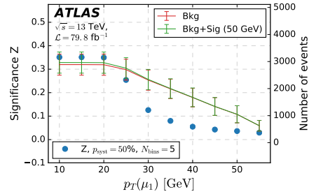
(h) M_N = 50 GeV. Binning variable p_T(e) .
