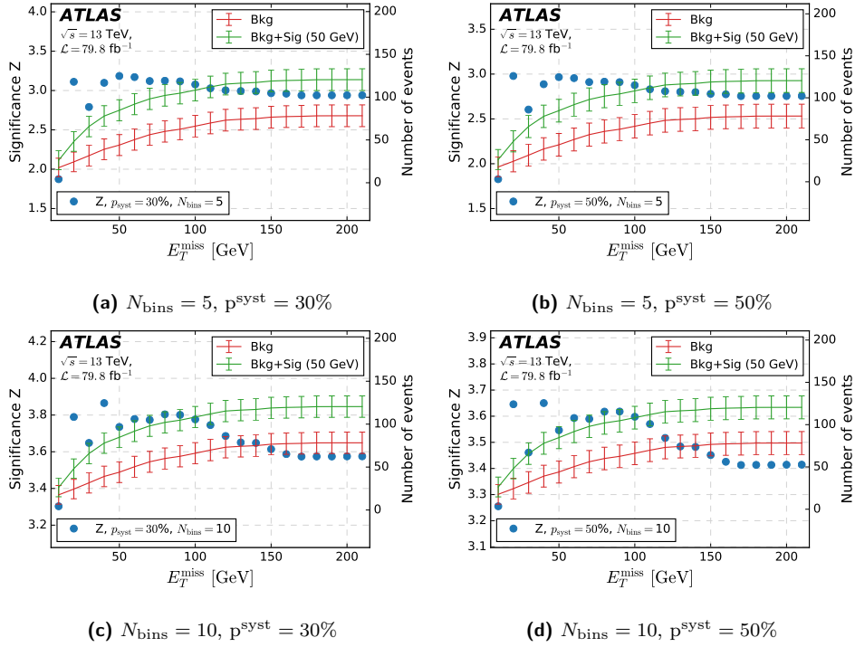
Figure 74: Signal sample with M_N = 50 GeV. Optimization study for the variable E_T^{\text{miss}} . The plots show the significance and number of background and signal events as a function of the cut on E_T^{\text{miss}} for which the x-axis value x_0 represents the requirement E_T^{\text{miss}} \leq x_0 GeV.
