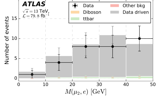
(b) \mu_2 : FixedCutLoose isolation. e: Loose isolation.
