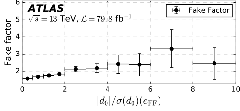
(c) Bin: 13 \text{ GeV} \leq p_T(e_{\text{FF}}) < 15 \text{ GeV} and N_{\text{jets}} \leq 2 .
