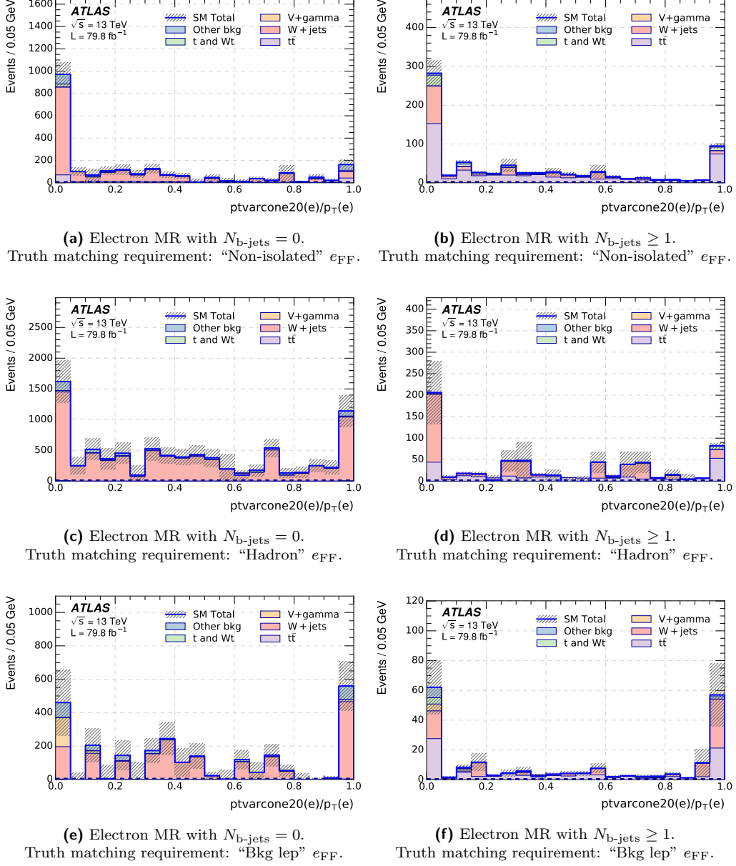
Figure 101: Distribution of the isolation variable: \text{ptvarcone20}/p_T(e_{\text{FF}}) . All electron measurement region (MR) requirements are applied except for the requirement that e_{\text{FF}} satisfies the Gradient isolation selection, see Tab. 15. Additional requirements are used for e_{\text{FF}} : 10 \text{ GeV} < p_T < 15 \text{ GeV} ; |d_0|/\sigma(d_0) < 1 ; |\Delta z_0 \sin(\theta)| < 0.1 \text{ mm} ; |\eta| < 1 . Truth matching is applied for the fake factor electron in each event and required to be: “non-isolated”, “hadron”, or “bkg lep”. The blue line indicates the sum of the SM background processes and the dashed area the corresponding statistical uncertainty. The last bin in the histogram includes all events with values larger than the range of the histogram.
