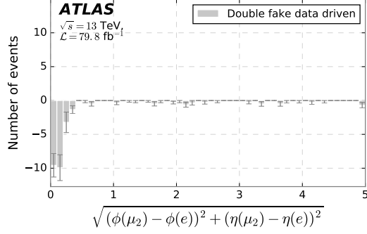
(a) Control region 1: No \Delta R(\mu_2, 3) > 0.2 requirement applied.
