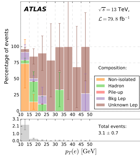
(b) Fake e .
