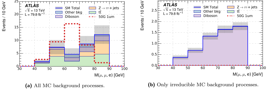
Figure 23: Distribution of M(\mu_1, \mu_2, e) in the signal region for the signal sample with M_N = 50 GeV. All the defined signal region requirements are applied as listed in Tab. 11. The blue line indicates the sum of the SM background processes and the dashed area the corresponding statistical uncertainty. The last bin in the histogram includes all events with values larger than the range of the histogram.
