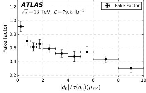
(c) Bin: 20 \text{ GeV} \leq p_T(\mu_{\text{FF}}) < 30 \text{ GeV} and N_{\text{jets}} > 2 .
