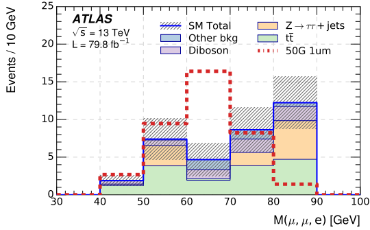
(e) M_N = 50 GeV. Distribution M(\mu_1, \mu_2, e) .
