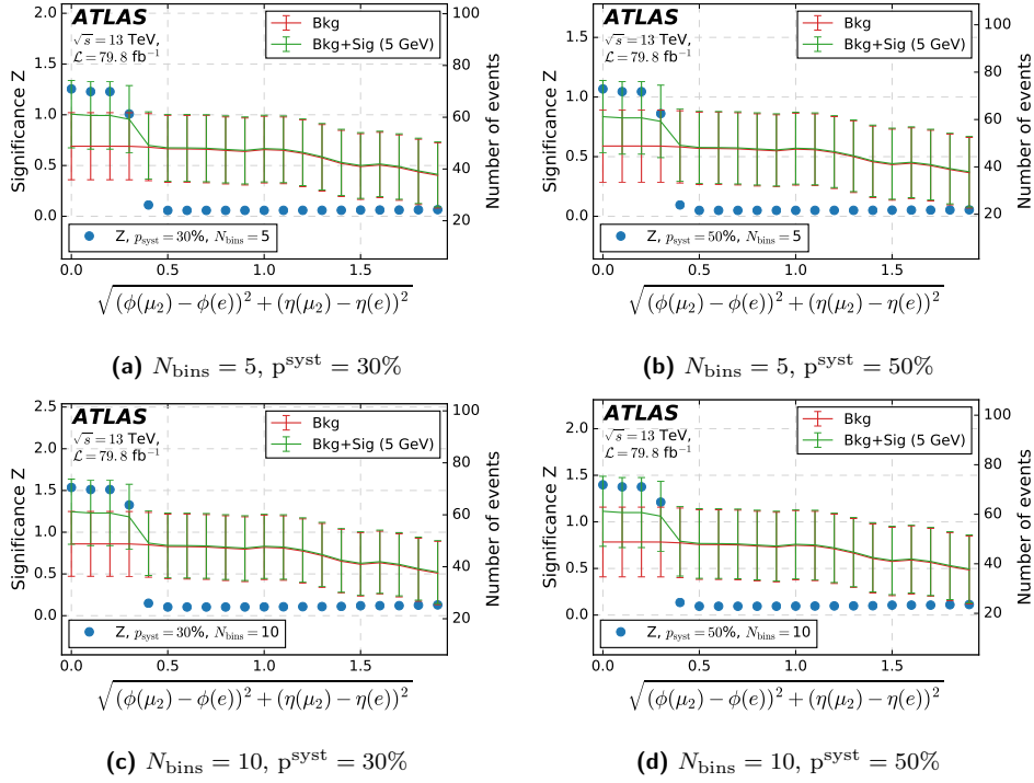
Figure 78: Signal sample with M_N = 5 GeV. Optimization study for variable \Delta R(\mu_2, e) . The plots show the significance and number of events as a function of the cut on \Delta R(\mu_2, e) for which the x-axis value x_0 represents the requirement \Delta R(\mu_2, e) \geq x_0 GeV.
