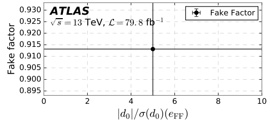
(j) Applied binning for Fig. 125i.
