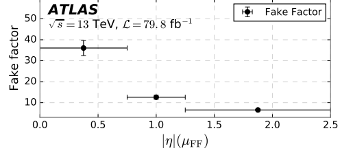
(d) Applied binning as a function of |\eta|(\mu_{\text{FF}}) for Fig. 117c.
