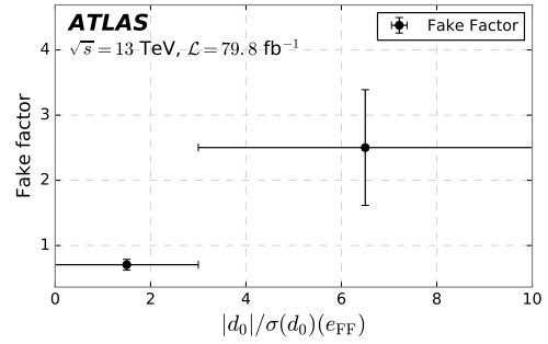
(f) Applied binning for Fig. 133e.
