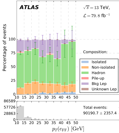
(c) Anti-ID criteria for e_{\text{FF}} . N_{\text{b-jets}}=0 .
