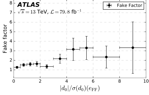
(a) Bin: 10 \text{ GeV} \leq p_T(e_{\text{FF}}) < 15 \text{ GeV} and N_{\text{jets}} \leq 2 .
