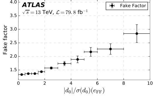
(c) Fake factor as a function of |d_0|/\sigma(d_0)(e_{\text{FF}}) .
