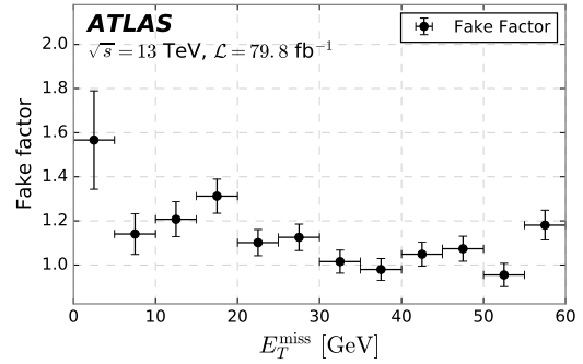
(f) Fake factor as a function of E_T^{\text{miss}} .
