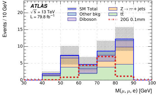
(c) M_N = 20 GeV. Distribution M(\mu_1, \mu_2, e) .
