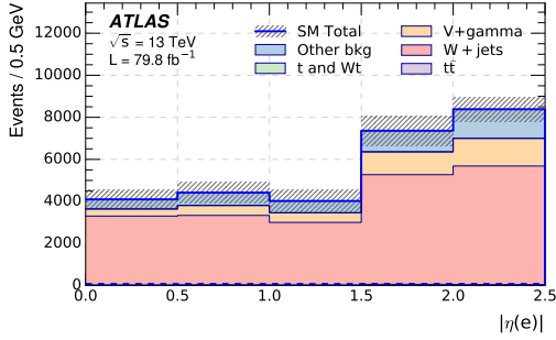
(e) Electron MR with N_{b\text{-jets}} = 0 .
