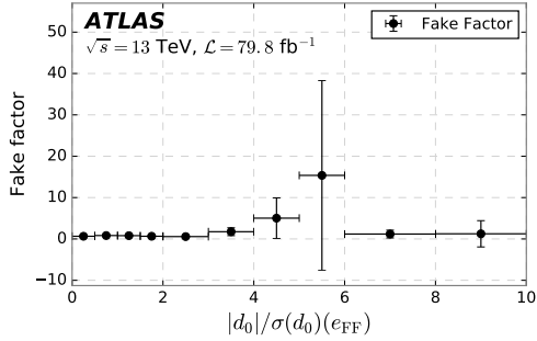
(e) Bin: 22 \text{ GeV} \leq p_T(e_{\text{FF}}) < 50 \text{ GeV} and N_{\text{jets}} \leq 2 .
