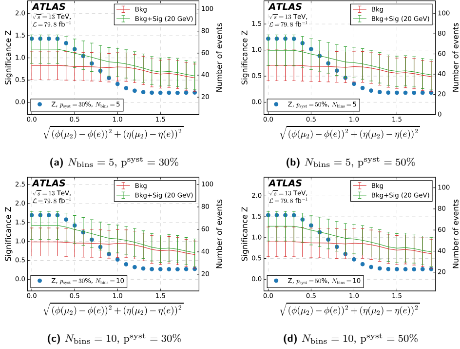
Figure 79: Signal sample with M_N = 20 GeV. Optimization study for variable \Delta R(\mu_2, e) . The plots show the significance and number of events as a function of the cut on \Delta R(\mu_2, e) for which the x-axis value x_0 represents the requirement \Delta R(\mu_2, e) \geq x_0 GeV.
