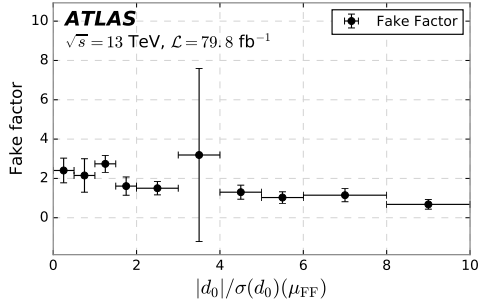
(e) Bin: 30 \text{ GeV} \leq p_T(\mu_{\text{FF}}) < 40 \text{ GeV} and N_{\text{jets}} \leq 2 .
