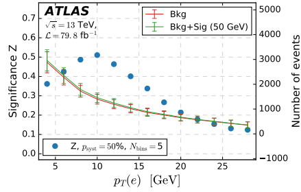
(f) M_N = 50 GeV. Binning variable p_T(\mu_2) .
