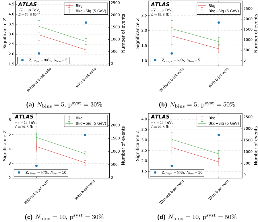
Figure 60: Signal sample with M_N = 5 GeV. Optimization study for the variable N_{\text{b-jets}} . The plots show the significance and number of background and signal events as a function of the cut on N_{\text{b-jets}} .
