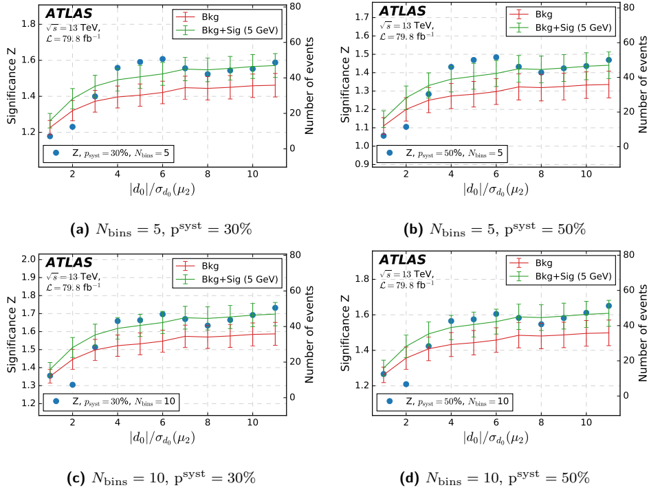
Figure 84: Signal sample with M_N = 5 GeV. Optimization study for the variable |d_0|/\sigma(d_0)(\mu_2) . The plots show the significance and number of events as a function of the cut on the variable |d_0|/\sigma(d_0)(\mu_2) for which the x-axis value x_0 represents the requirement |d_0|/\sigma(d_0)(\mu_2) < x_0 .
