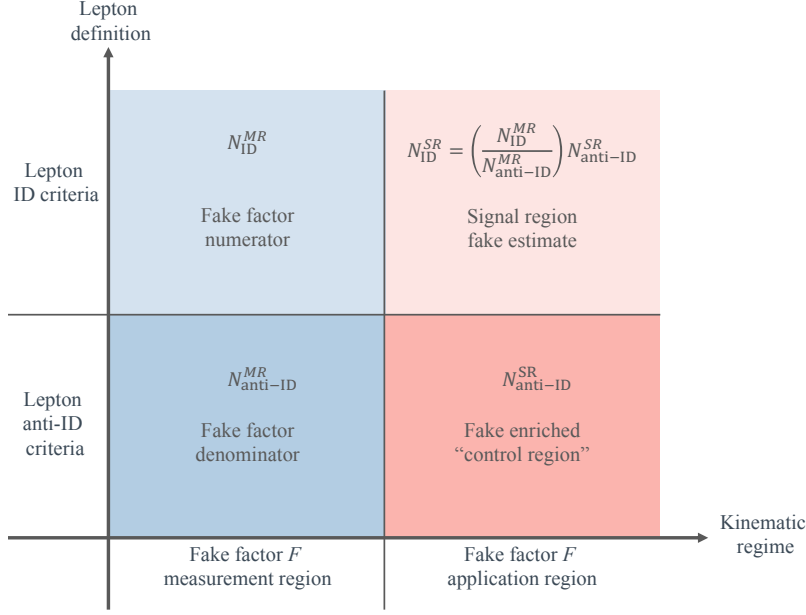
Figure 24: Schematic presentation of the regions applied in the fake factor method. The four regions are all mutually independent.
