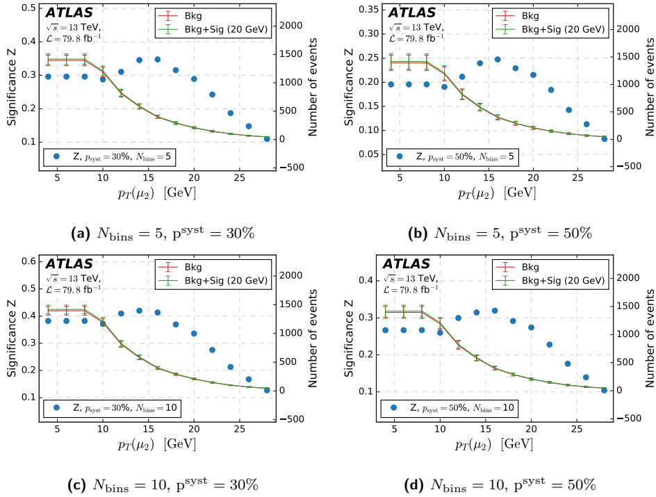
Figure 58: Signal sample with M_N = 20 GeV. Optimization study for the variable p_T(\mu_2) . The plots show the significance and number of background and signal events as a function of the cut on p_T(\mu_2) for which the x-axis value x_0 represents the requirement p_T(\mu_2) \geq x_0 GeV.
