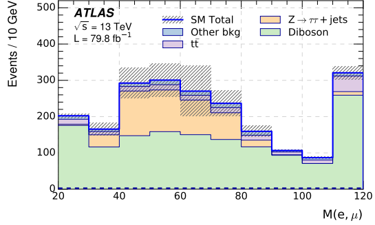
(f) Channel \mu^\pm e^\pm .
