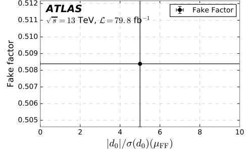
(b) Applied binning as a function of |d_0|/\sigma(d_0)(\mu_{\text{FF}}) for Fig. 112a.
