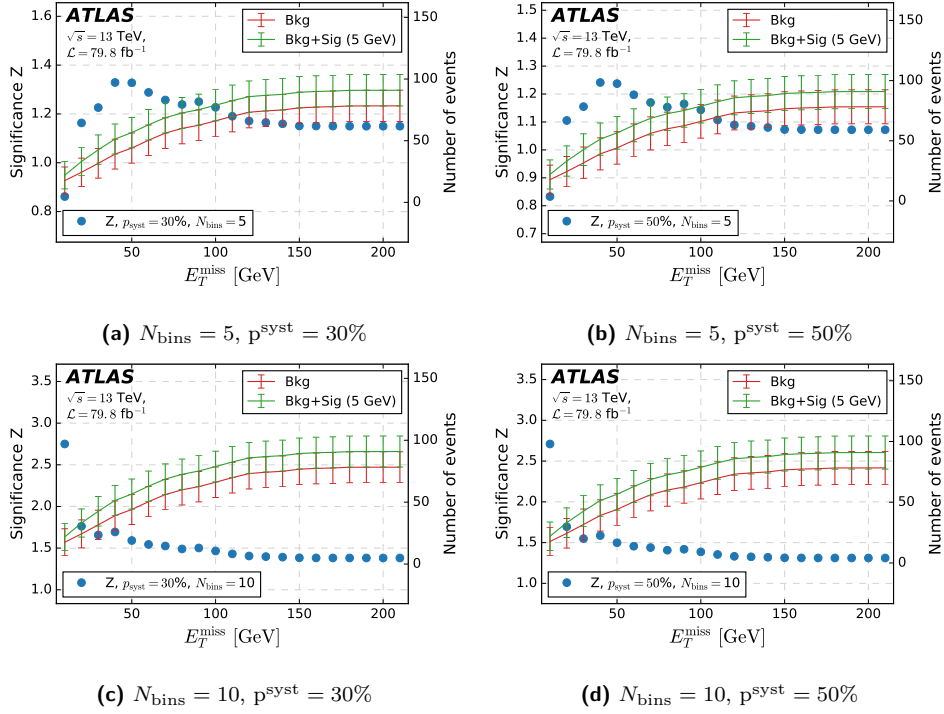
Figure 72: Signal sample with M_N = 5 GeV. Optimization study for the variable E_T^{\text{miss}} . The plots show the significance and number of background and signal events as a function of the cut on E_T^{\text{miss}} for which the x-axis value x_0 represents the requirement E_T^{\text{miss}} \leq x_0 GeV.
