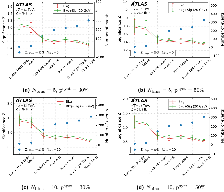
Figure 70: Signal sample with M_N = 20 GeV. Optimization study for the isolation selection of \mu_2 . The plots show the significance and number of background and signal events as a function of the isolation selection of \mu_2 .
