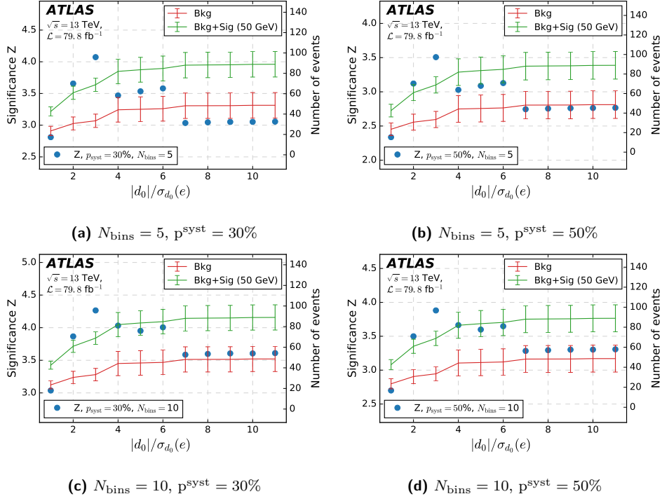
Figure 83: Signal sample with M_N = 50 GeV. Optimization study for the variable |d_0|/\sigma(d_0)(e) . The plots show the significance and number of events as a function of the cut on the variable |d_0|/\sigma(d_0)(e) for which the x-axis value x_0 represents the requirement |d_0|/\sigma(d_0)(e) < x_0 .
