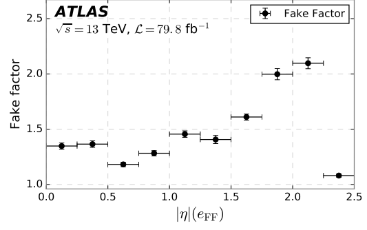
(b) Fake factor as a function of |\eta|(e_{\text{FF}}) .
