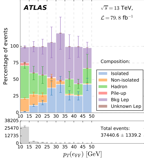
(a) ID criteria for e_{\text{FF}} . N_{\text{b-jets}}=0 .
