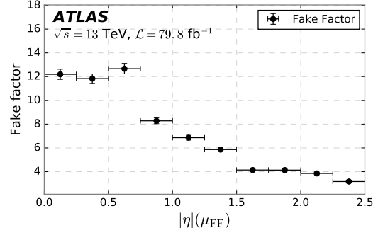
(b) Fake factor as a function of |\eta|(\mu_{\text{FF}}) .
