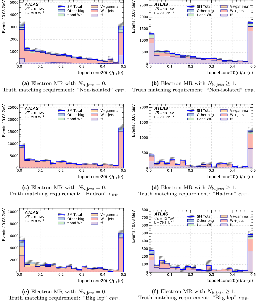
Figure 93: Distribution of the isolation variable: \text{topoetcone20}/p_T(e_{\text{FF}}) . All electron measurement region (MR) requirements are applied except for the requirement that e_{\text{FF}} satisfies the Gradient isolation selection, see Tab. 15. Truth matching is applied for the fake factor electron in each event and required to be: “non-isolated”, “hadron”, or “bkg lep”. The blue line indicates the sum of the SM background processes and the dashed area the corresponding statistical uncertainty. The last bin in the histogram includes all events with values larger than the range of the histogram.
