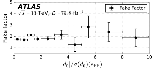
(g) Bin: 17 \text{ GeV} \leq p_T(e_{\text{FF}}) < 20 \text{ GeV} and N_{\text{jets}} \leq 2 .
