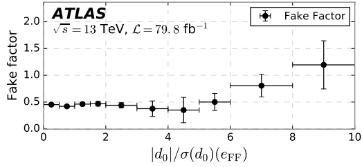
(e) Bin: 15 \text{ GeV} \leq p_T(e_{\text{FF}}) < 17 \text{ GeV} and N_{\text{jets}} \leq 2 .
