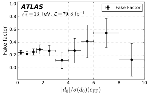
(c) Bin: 15 \text{ GeV} \leq p_T(e_{\text{FF}}) < 25 \text{ GeV} .
