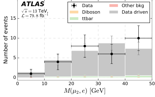
(a) \mu_2 : FixedCutLoose isolation. e: Gradient isolation.
