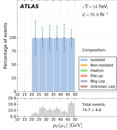
(b) Control region 2. Composition of \mu_1 . Region: \mu_2 : Anti-ID criteria. e : ID criteria.
