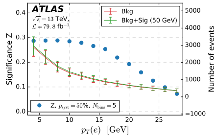
(h) M_N = 50 GeV. Binning variable p_T(e) .
