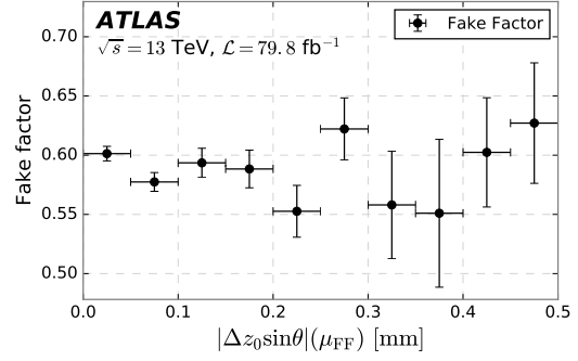
(d) Fake factor as a function of |\Delta z_0 \sin(\theta)|(\mu_{\text{FF}}) .
