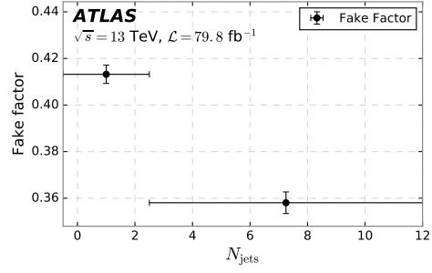
(b) Applied binning as a function of N_{\text{jets}} for Fig. 105a.
