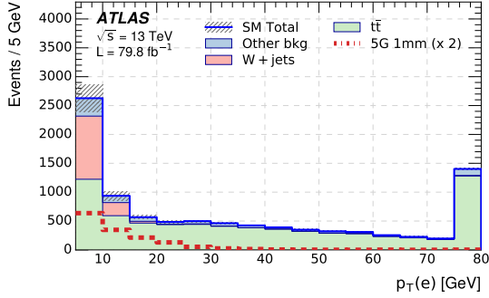
(a) M_N = 5 GeV
