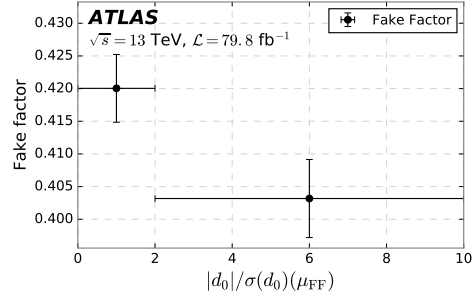
(b) Applied binning as a function of |d_0|/\sigma(d_0)(\mu_{\text{FF}}) for Fig. 106a.
