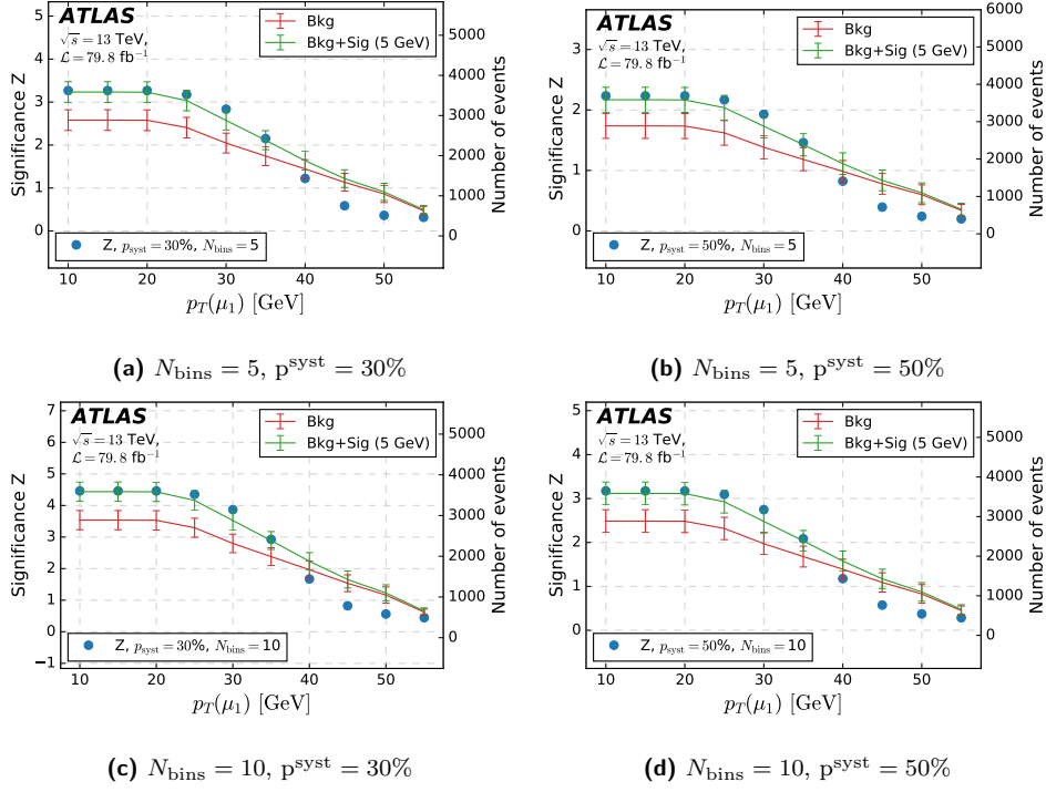
Figure 51: Signal sample with M_N = 5 GeV. Optimization study for the variable p_T(\mu_1) . The plots show the significance and number of background and signal events as a function of the cut on p_T(\mu_1) for which the x-axis value x_0 represents the requirement p_T(\mu_1) \geq x_0 GeV.
