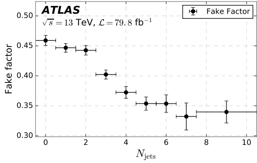
(e) Fake factor as a function of N_{\text{jets}} .
