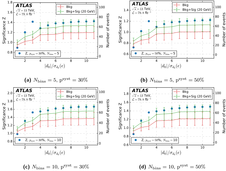
Figure 82: Signal sample with M_N = 20 GeV. Optimization study for the variable |d_0|/\sigma(d_0)(e) . The plots show the significance and number of events as a function of the cut on the variable |d_0|/\sigma(d_0)(e) for which the x-axis value x_0 represents the requirement |d_0|/\sigma(d_0)(e) < x_0 .
