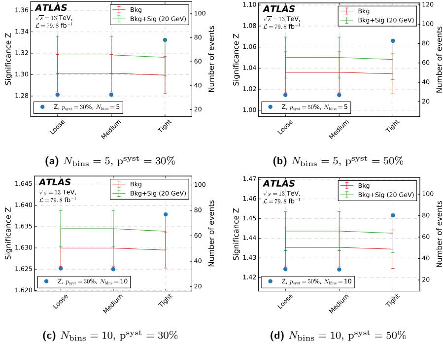
Figure 76: Signal sample with M_N = 20 GeV. Optimization study for the identification quality for \mu_1 . The plots show the significance and number of background and signal events as a function of the cut on the identification quality selection for \mu_1 .
