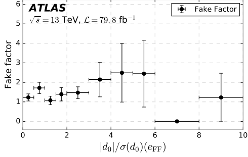
(c) Bin: 15 \text{ GeV} \leq p_T(e_{\text{FF}}) < 22 \text{ GeV} and N_{\text{jets}} \leq 2 .
