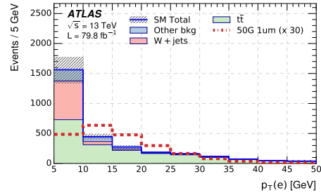
(h) Signal region, p_T(e) distribution. Signal with M_N = 50 GeV.
