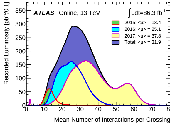
Figure 4: The recorded luminosity as a function of the mean number of interactions per crossing measured by the ATLAS detector. The figure is published by the ATLAS Collaboration in [27].
