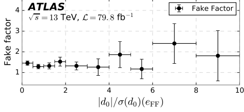
(g) Bin: 17 \text{ GeV} \leq p_T(e_{\text{FF}}) < 20 \text{ GeV} and N_{\text{jets}} > 2 .
