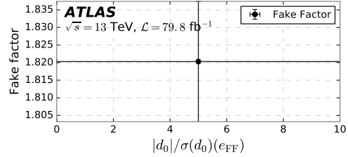
(h) Applied binning for Fig. 130g.
