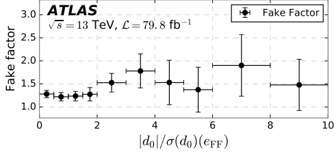
(e) Bin: 15 \text{ GeV} \leq p_T(e_{\text{FF}}) < 17 \text{ GeV} and N_{\text{jets}} > 2 .
