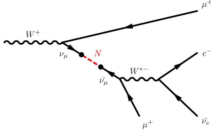
Figure 1: The Feynman diagram for the signal region channel considered in this analysis. Also the Hermitian conjugate of this channel contribute to the signal. The figure is from [15]
