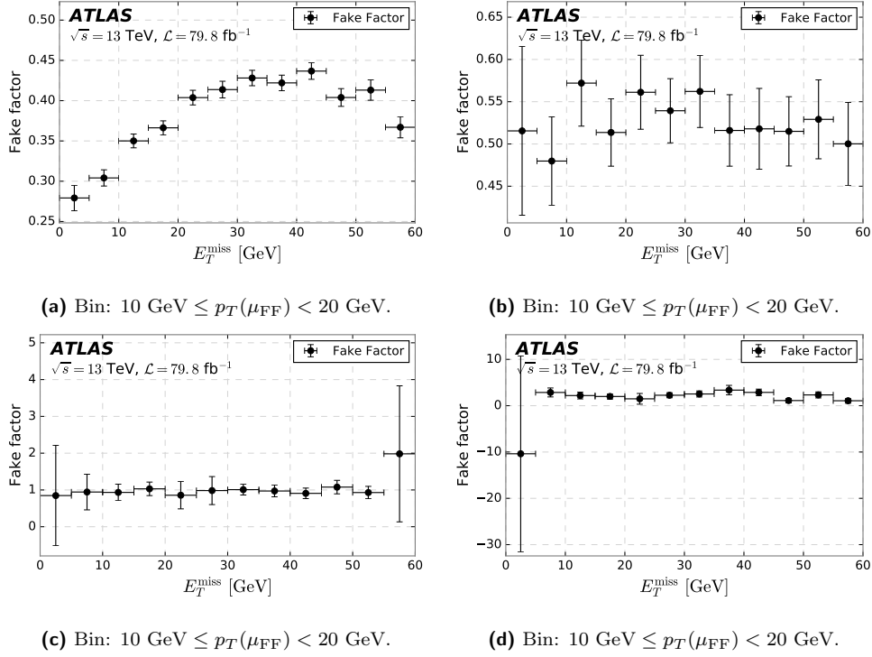
Figure 103: Muon fake factor as a function of E_T^{\text{miss}} . The considered fake factors are binned in p_T(\mu_{\text{FF}}) . The ID and anti-ID criteria are defined using the FixedCutLoose isolation in the muon measurement region with N_{\text{b-jets}} = 0 .
