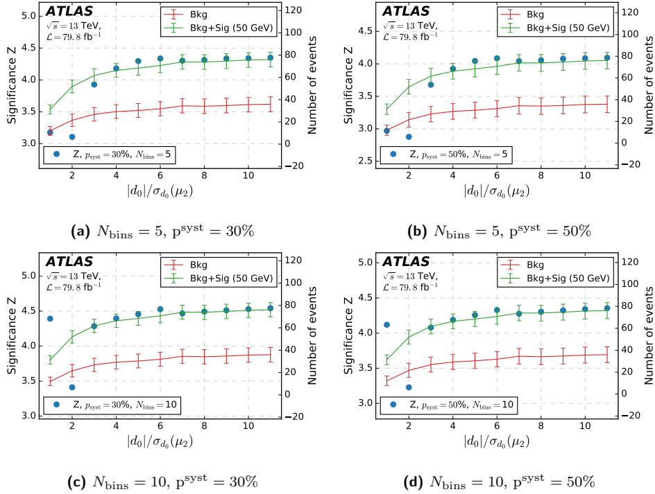
Figure 86: Signal sample with M_N = 50 GeV. Optimization study for the variable |d_0|/\sigma(d_0)(\mu_2) . The plots show the significance and number of events as a function of the cut on the variable |d_0|/\sigma(d_0)(\mu_2) for which the x-axis value x_0 represents the requirement |d_0|/\sigma(d_0)(\mu_2) < x_0 .
