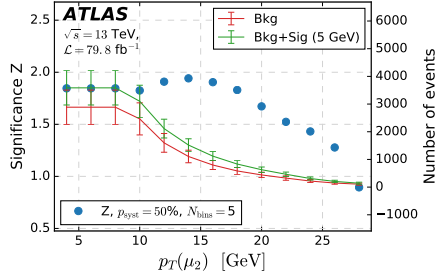
(e) M_N = 5 GeV. Binning variable p_T(\mu_2) .
