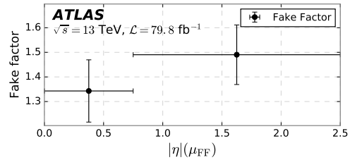
(j) Applied binning as a function of |\eta|(\mu_{\text{FF}}) for Fig. 116i.
