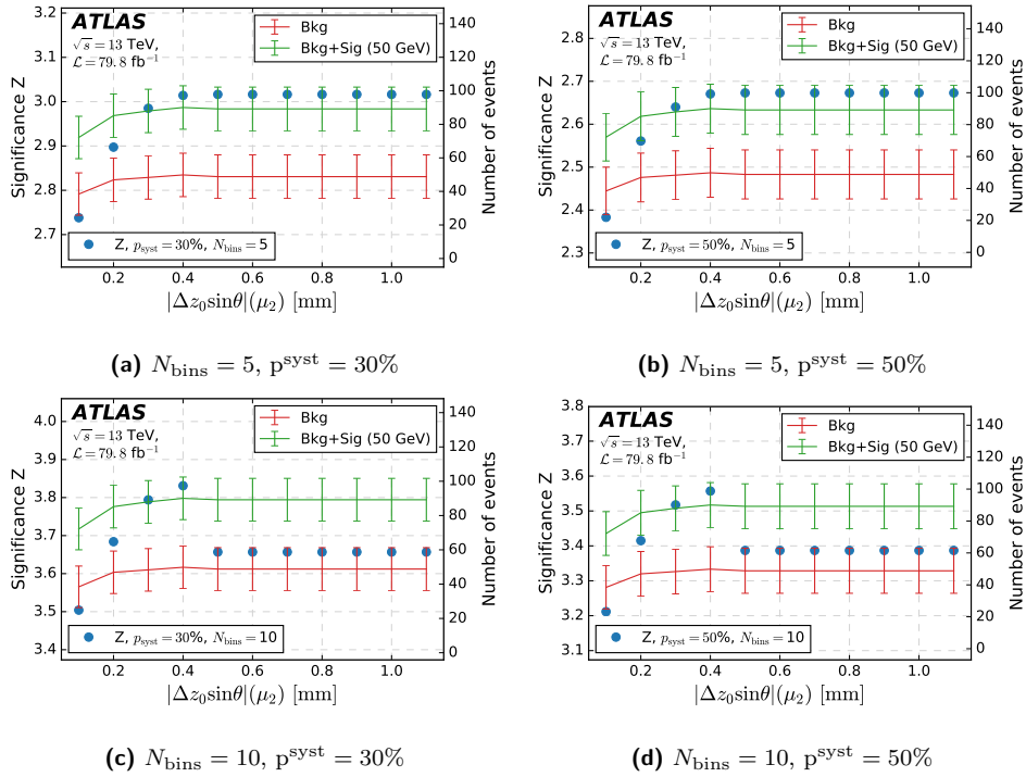
Figure 92: Signal sample with M_N = 50 GeV. Optimization study for the variable |\Delta z_0 \sin(\theta)|(\mu_2) . The plots show the significance and number of events as a function of the cut on the variable |\Delta z_0 \sin(\theta)|(\mu_2) for which the x-axis value x_0 represents the requirement |\Delta z_0 \sin(\theta)|(\mu_2) < x_0 .
