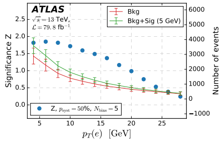
(g) M_N = 5 GeV. Binning variable p_T(e) .
