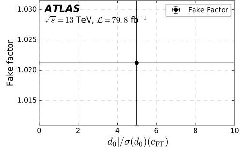
(j) Applied binning for Fig. 131i.
