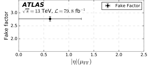
(h) Applied binning as a function of |\eta|(\mu_{\text{FF}}) for Fig. 117g.
