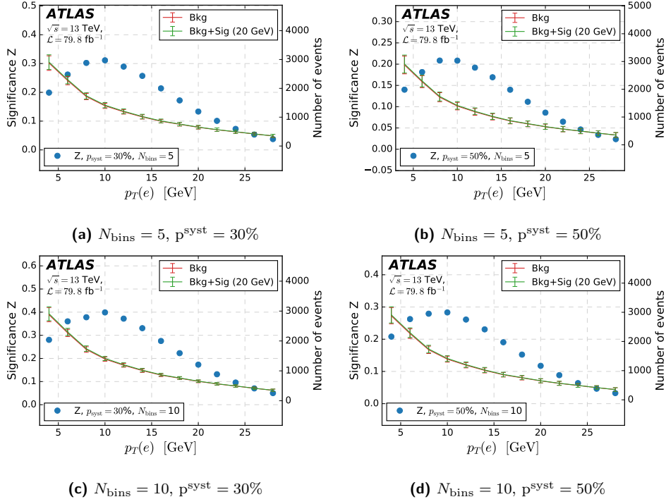
Figure 55: Signal sample with M_N = 20 GeV. Optimization study for the variable p_T(e) . The plots show the significance and number of background and signal events as a function of the cut on p_T(e) for which the x-axis value x_0 represents the requirement p_T(e) \geq x_0 GeV.
