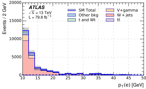
(e) Electron MR with N_{b-jets} = 0 .
