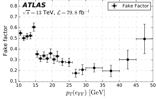
(a) Fake factor as a function of p_T(e_{\text{FF}}) .
