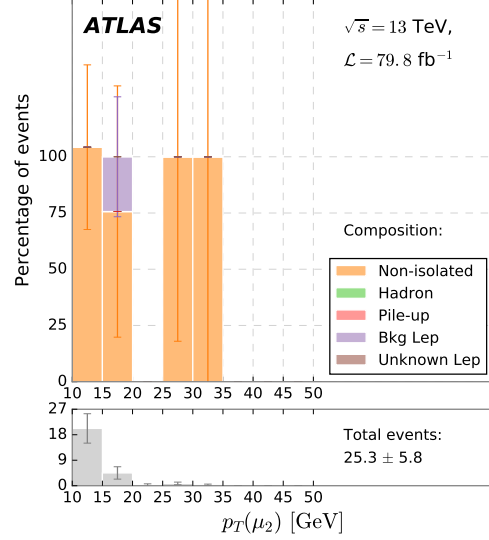
(b) Fake \mu_2 .
