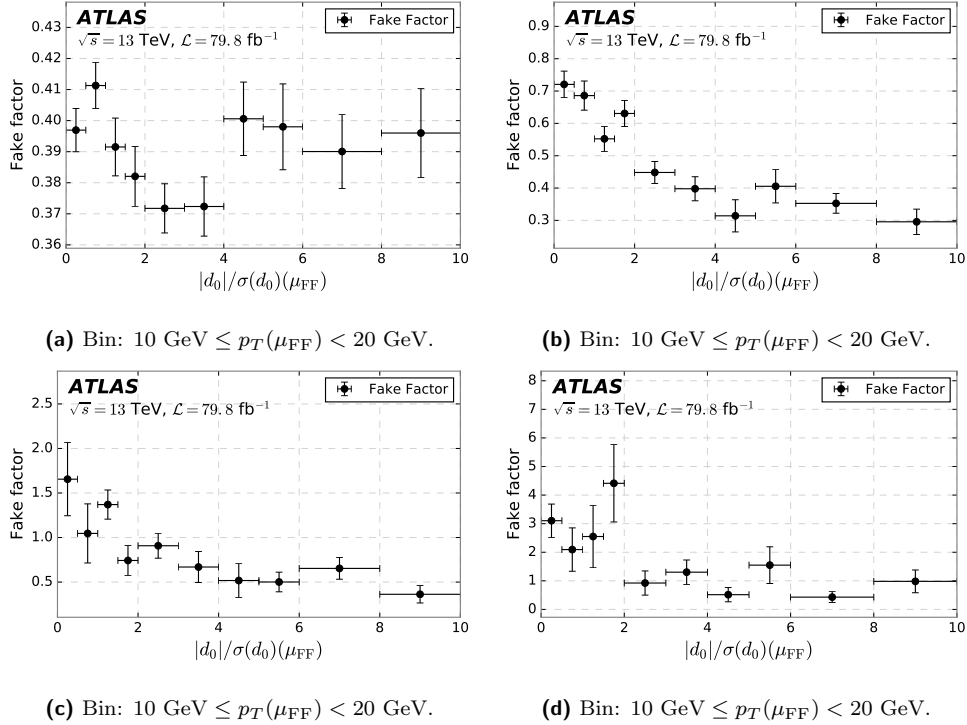
Figure 104: Muon fake factor as a function of |d_0|/\sigma(d_0)(\mu_{\text{FF}}) . The considered fake factors are binned in p_T(\mu_{\text{FF}}) . The ID and anti-ID criteria are defined using the FixedCutLoose isolation in the muon measurement region with N_{\text{b-jets}} = 0 .
