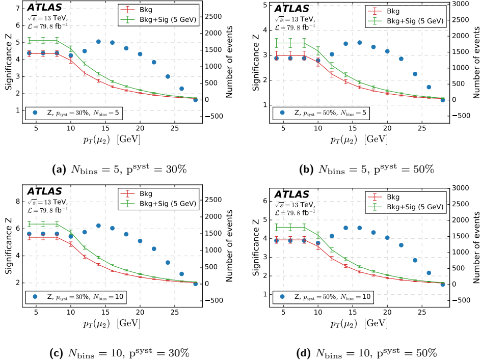
Figure 57: Signal sample with M_N = 5 GeV. Optimization study for the variable p_T(\mu_2) . The plots show the significance and number of background and signal events as a function of the cut on p_T(\mu_2) for which the x-axis value x_0 represents the requirement p_T(\mu_2) \geq x_0 GeV.
