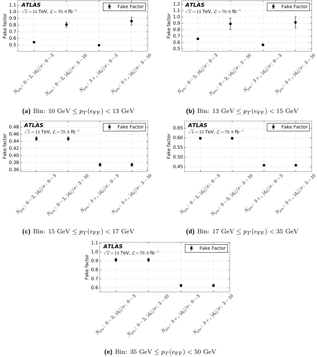
Figure 39: The final binning for the electron fake factor. The ID and anti-ID criteria are defined using the Gradient isolation in the electron measurement region with N_{\text{b-jets}} = 0 .
