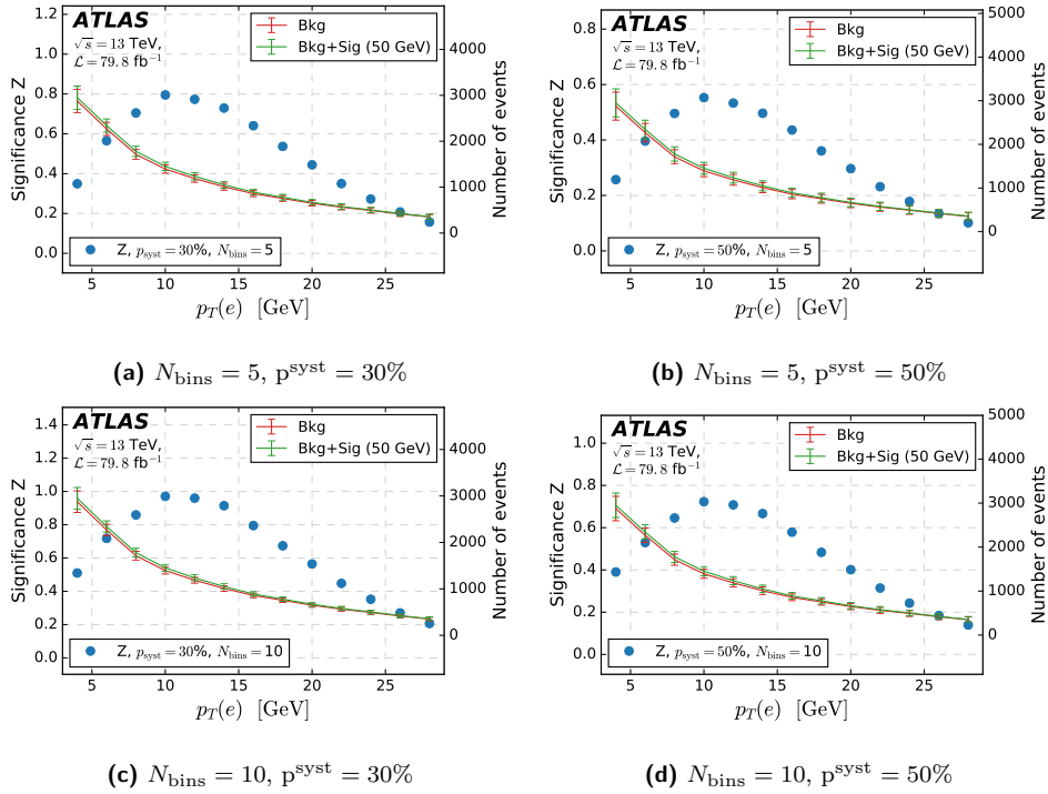
Figure 56: Signal sample with M_N = 50 GeV. Optimization study for the variable p_T(e) . The plots show the significance and number of background and signal events as a function of the cut on p_T(e) for which the x-axis value x_0 represents the requirement p_T(e) \geq x_0 GeV.
