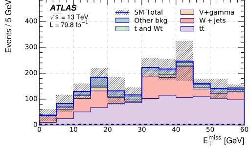
(f) Electron MR with N_{b\text{-jets}} \geq 1 .
