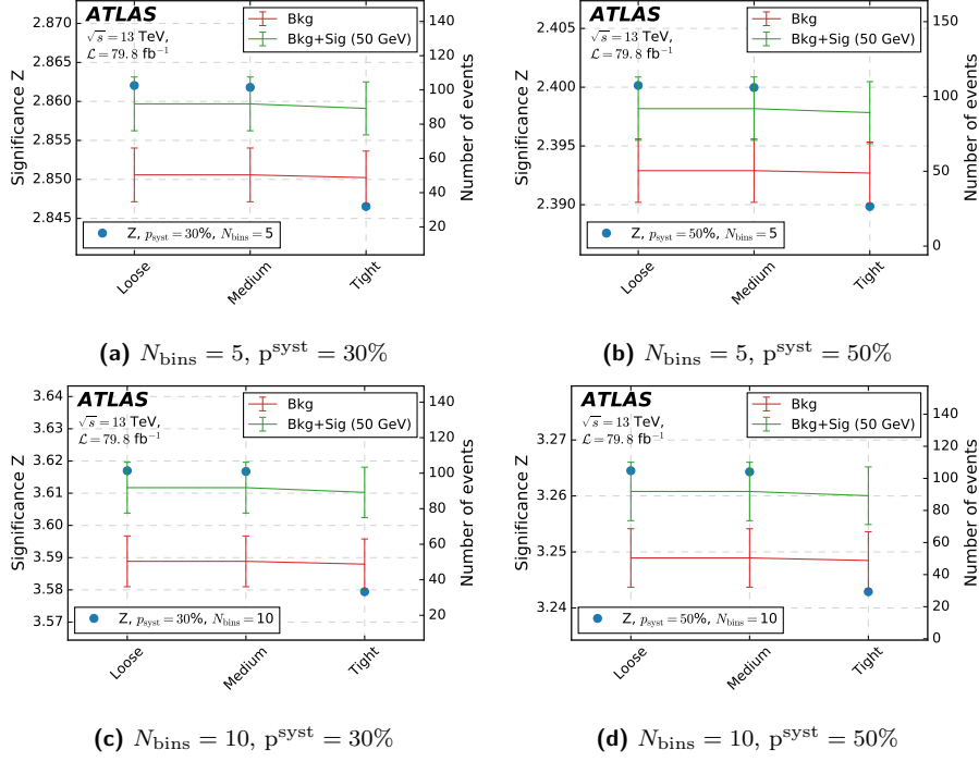
Figure 77: Signal sample with M_N = 50 GeV. Optimization study for the identification quality for \mu_1 . The plots show the significance and number of background and signal events as a function of the cut on the identification quality selection for \mu_1 .
