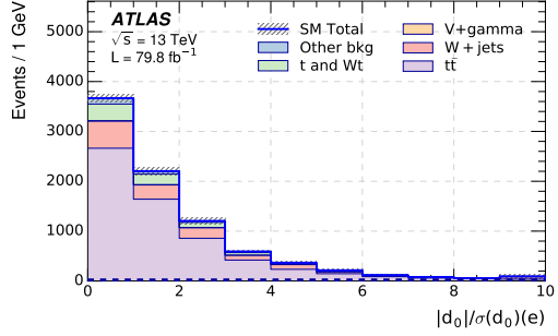
(b) Electron MR with N_{b-jets} \geq 1 .
