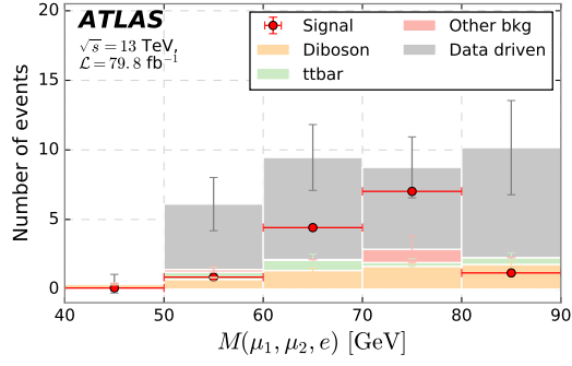
(c) Signal sample: M_N = 20 GeV, c\tau = 0.1 mm.
