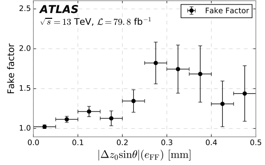
(d) Fake factor as a function of |\Delta z_0 \sin(\theta)|(e_{\text{FF}}) .
