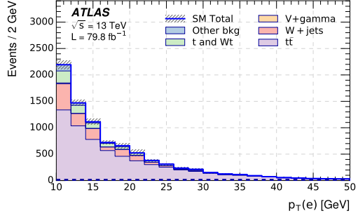
(b) Electron MR with N_{b-jets} \geq 1 .
