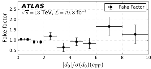
(i) Bin: 20 \text{ GeV} \leq p_T(e_{\text{FF}}) < 50 \text{ GeV} and N_{\text{jets}} > 2 .
