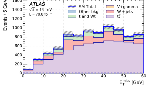
(b) Electron MR with N_{b\text{-jets}} \geq 1 .
