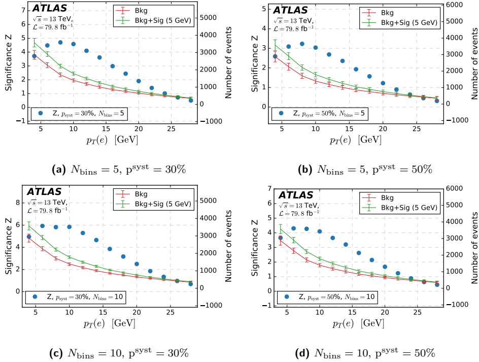
Figure 54: Signal sample with M_N = 5 GeV. Optimization study for the variable p_T(e) . The plots show the significance and number of background and signal events as a function of the cut on p_T(e) for which the x-axis value x_0 represents the requirement p_T(e) \geq x_0 GeV.
