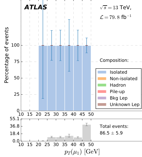
(d) Control region 2. Composition of \mu_1 . Region: \mu_2 : Anti-ID criteria. e : Anti-ID criteria.
