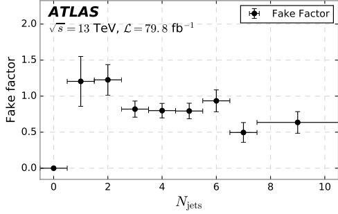
(e) Fake factor as a function of N_{\text{jets}} . Bin: 40 \text{ GeV} \leq p_T(\mu_{\text{FF}}) < 50 \text{ GeV} .
