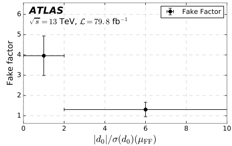
(h) Applied binning as a function of |d_0|/\sigma(d_0)(\mu_{\text{FF}}) for Fig. 106g.
