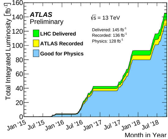
(b) The integrated luminosity for Run 2 of the LHC as a function of time from 2015-2018. In addition to the total luminosity delivered by the LHC, the luminosity recorded by the ATLAS experiment is shown.
