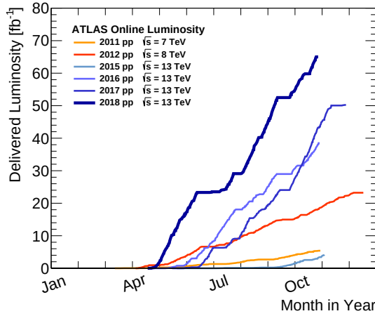
(a) The integrated luminosity for each data taking year from 2011-2012 in Run 1 and 2015-2018 in Run 2 as a function of the month in the year. The delivered luminosity by the LHC is measured in fb -1 .
