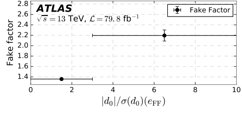
(b) Applied binning for Fig. 130a.
