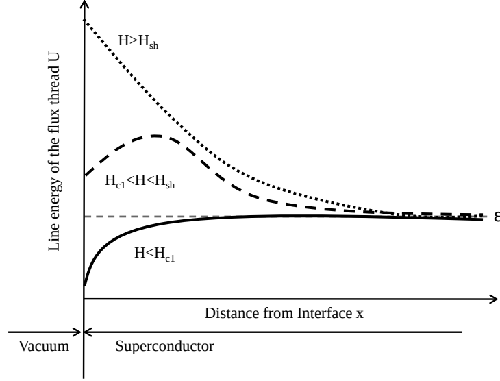
Figure 2.4.: Dependence of the line energy U on distance to the surface x of a flux thread located at the interface between a superconductor and vacuum. When H < H_{c1} the force on the flux thread always points towards the surface. It cannot enter the superconductor (solid line). When H_{c1} < H < H_{sh} it is energetically favorable for the flux thread to be located inside the superconductor. But there is a surface barrier, preventing the entry of the flux thread if the surface is clean (dashed line). When H > H_{sh} , the barrier disappears (dotted line) and the force on the flux thread is directed to the inside.
