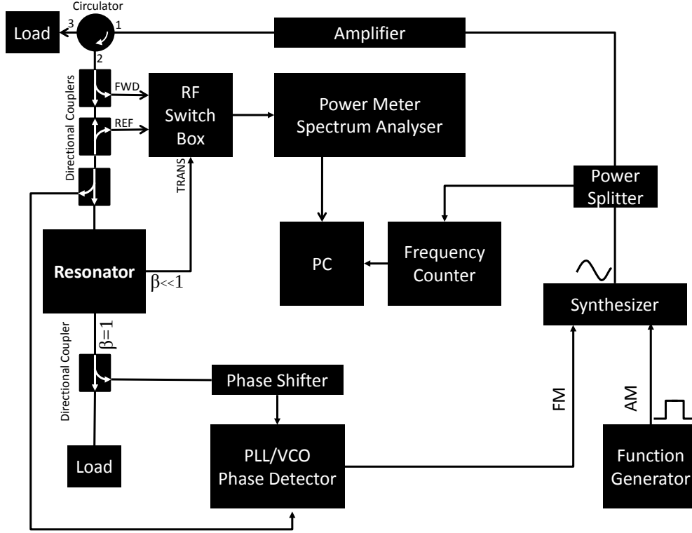
Figure 3.7.: The RF system of the Quadrupole Resonator.
