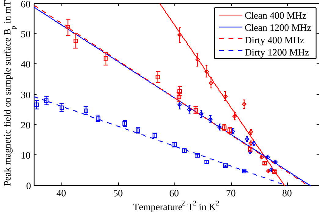
Figure 4.18.: Quench field B_{\max, \text{RF}} of the bulk niobium sample in clean and dirty condition, measured in CW.
