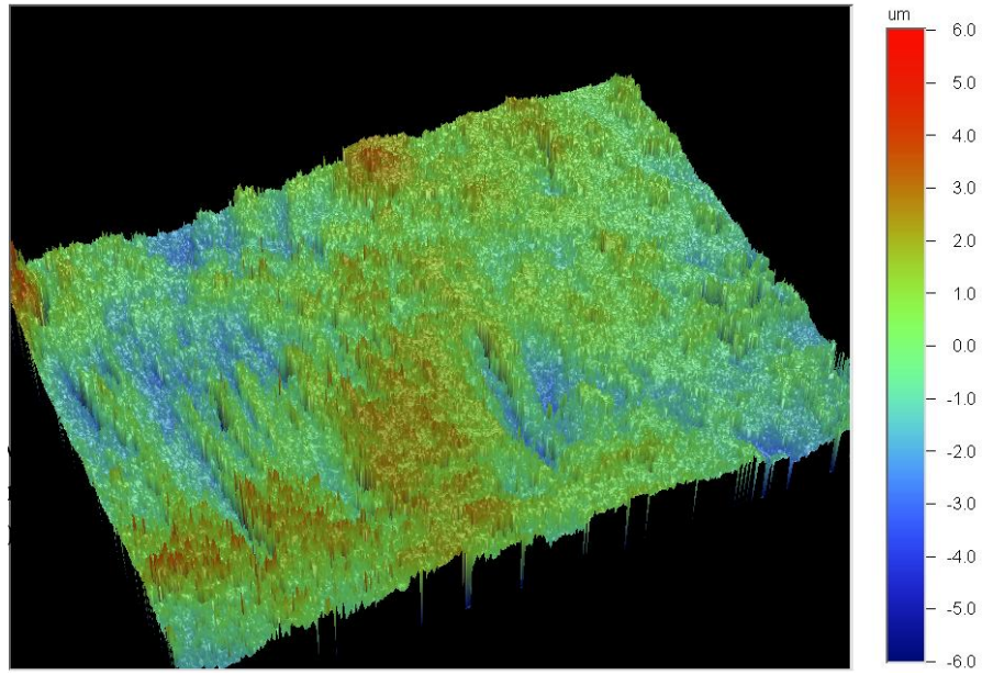
Figure 5.3.: Surface profile of the bulk niobium sample obtained from white light interferometry. The lateral resolution of the image is 500 nm and the surface area displayed 312 \times 234 \mu\text{m} .
