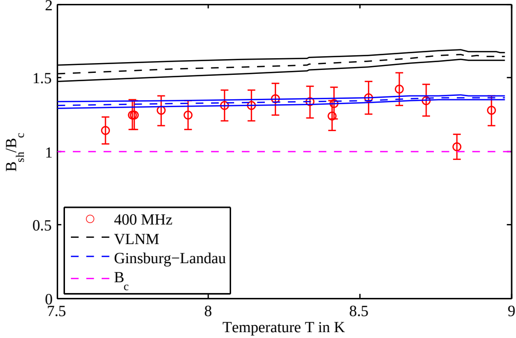
Figure 4.19.: Critical field under RF (short pulses) of the clean bulk niobium sample.
