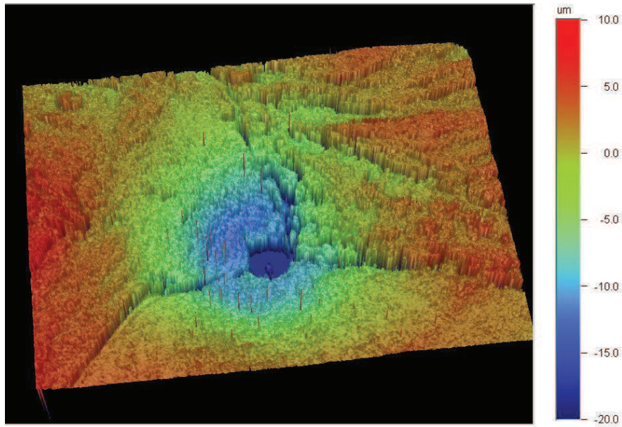
Figure 5.4.: Surface profile of the bulk niobium sample in the vicinity of a boundary between three grains obtained from white light interferometry. The lateral resolution of the image is 500 nm and the surface area displayed 312 \times 234 \mu\text{m} .
